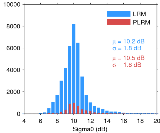
Figure 25. Histogram of flag-valid sigma0 over oceans and lakes for LRM (blue) and PLRM (red) for 01/11/2017. The mean ( \mu ) and standard deviation ( \sigma ) are also shown. Note that values outside [4 20] dB are excluded from the histogram for the sake of readability but not from the computation of \mu and \sigma .
