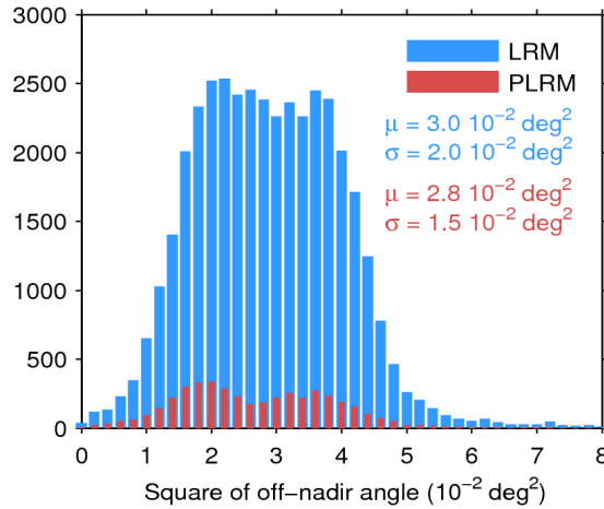
Figure 39. Histogram of flag-valid mispointing over oceans and lakes for LRM (blue) and PLRM (red) for 01/11/2017. Only positive values have been considered. The mean ( \mu ) and standard deviation ( \sigma ) are also shown. Note that values larger than 8 \cdot 10^{-2} \text{ deg}^2 are excluded from the histogram for the sake of readability but not from the computation of \mu and \sigma .
