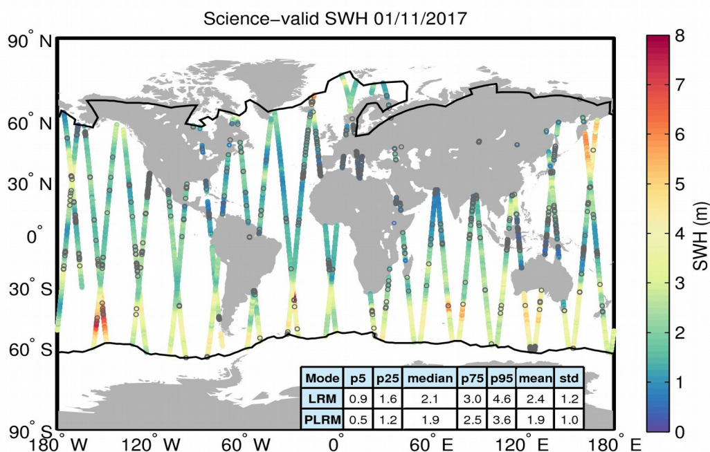
Figure 19. Geographical distribution of science-valid SWH data over oceans and lakes for 01/11/2017. The statistical values shown in the table refer to the SWH in m and are calculated separately for LRM and PLRM regions. The black lines mark the outer limit of the Arctic and Antarctic polar polygons. Gray circles denote records that have been rejected based on the editing criteria described in Table 3.
