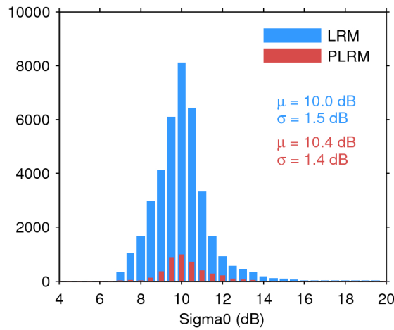
Figure 28. Histogram of science-valid sigma0 over oceans and lakes for LRM (blue) and PLRM (red) for 01/11/2017. The mean ( \mu ) and standard deviation ( \sigma ) are also shown. Note that values outside [4 20] dB are excluded from the histogram for the sake of readability but not from the computation of \mu and \sigma .
