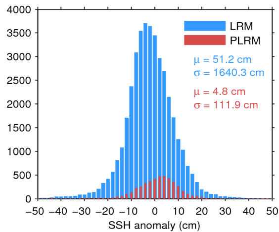
Figure 7. Histogram of flag-valid SSH anomaly over oceans and lakes for LRM (blue) and PLRM (red) for 01/11/2017. The mean ( \mu ) and standard deviation ( \sigma ) are also shown. Note that values outside [-50 \ 50] cm are excluded from the histogram for the sake of readability but not from the computation of \mu and \sigma .
