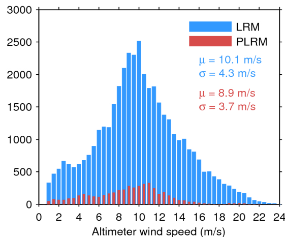
Figure 35. Histogram of science-valid wind over oceans and lakes for LRM (blue) and PLRM (red) for 01/11/2017. The mean ( \mu ) and standard deviation ( \sigma ) are also shown. Note that values larger than 24 m/s are excluded from the histogram for the sake of readability but not from the computation of \mu and \sigma .
