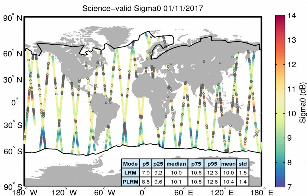
Figure 27. Geographical distribution of science-valid sigma0 data over oceans and lakes for 01/11/2017. The statistical values shown in the table refer to the sigma0 in dB and are calculated separately for LRM and PLRM regions. The black lines mark the outer limit of the Arctic and Antarctic polar polygons. Gray circles denote records that have been rejected based on the editing criteria described in Table 4.
