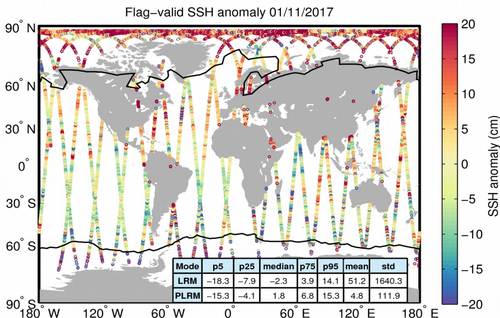
Figure 5. Geographical distribution of flag-valid 1-Hz SSH anomaly data over oceans and lakes for 01/11/2017. The statistical values shown in the table refer to the SSH anomaly in cm and are calculated separately for LRM and PLRM regions. Measurements taken over polar polygons have been excluded from the computation of the statistical values. The black lines mark the outer limit of the Arctic and Antarctic polar polygons.
