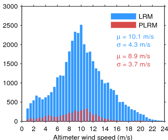
Figure 33. Histogram of flag-valid wind over oceans and lakes for LRM (blue) and PLRM (red) for 01/11/2017. The mean ( \mu ) and standard deviation ( \sigma ) are also shown. Note that values larger than 24 m/s are excluded from the histogram for the sake of readability but not from the computation of \mu and \sigma .
