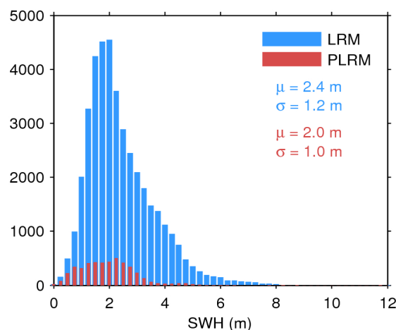
Figure 17. Histogram of flag-valid SWH over oceans and lakes for LRM (blue) and PLRM (red) for 01/11/2017. The mean ( \mu ) and standard deviation ( \sigma ) are also shown. Note that values larger than 12 m are excluded from the histogram for the sake of readability but not from the computation of \mu and \sigma .
