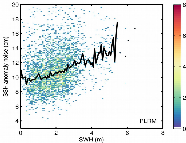
Figure 9. 2D histogram showing flag-valid SSH anomaly noise as a function of SWH for LRM (top) and PLRM (bottom) for 01/11/2017. The black line denotes the median SSH anomaly noise as a function of SWH.
