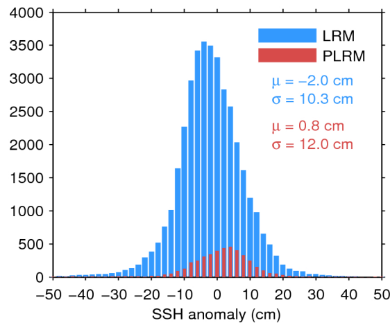
Figure 11. Histogram of science-valid SSH anomaly over oceans and lakes for LRM (blue) and PLRM (red) for 01/11/2017. The mean ( \mu ) and standard deviation ( \sigma ) are also shown. Note that values outside [-50\ 50] cm are excluded from the histogram for the sake of readability but not from the computation of \mu and \sigma .
