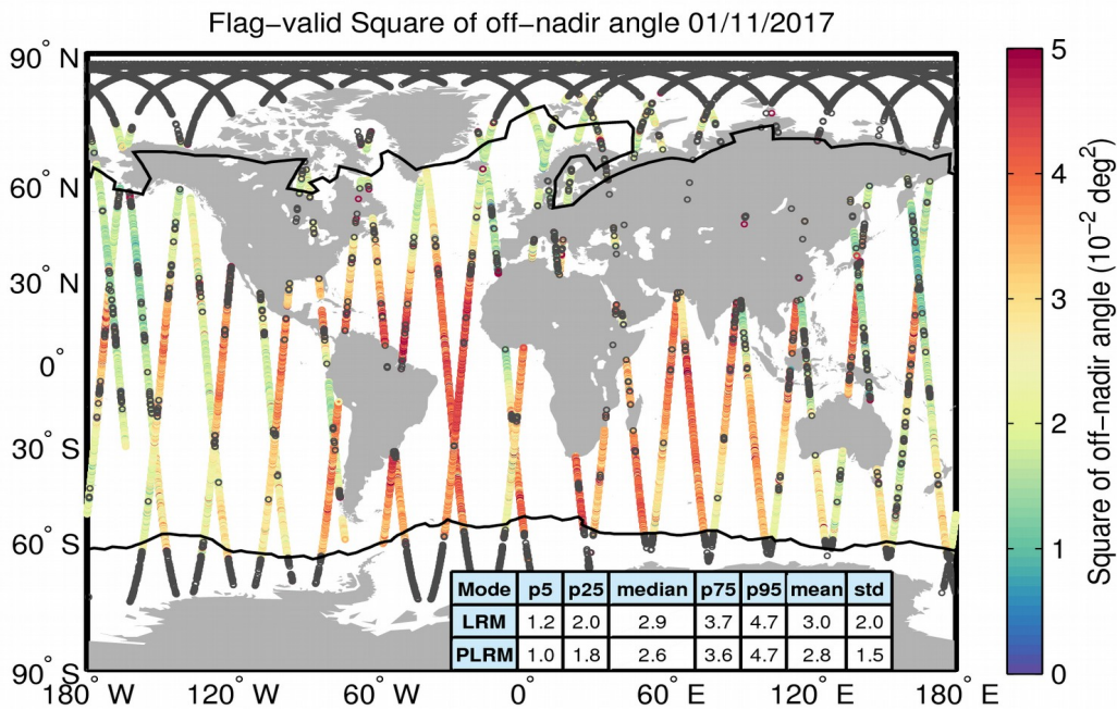
Figure 37. Geographical distribution of flag-valid mispointing data over oceans and lakes for 01/11/2017. The statistical values shown in the table refer to the mispointing in 10^{-2} deg 2 and are calculated separately for LRM and PLRM regions. Measurements taken over polar polygons have been excluded from the computation of the statistical values. The black lines mark the outer limit of the Arctic and Antarctic polar polygons. Gray circles denote negative values.
