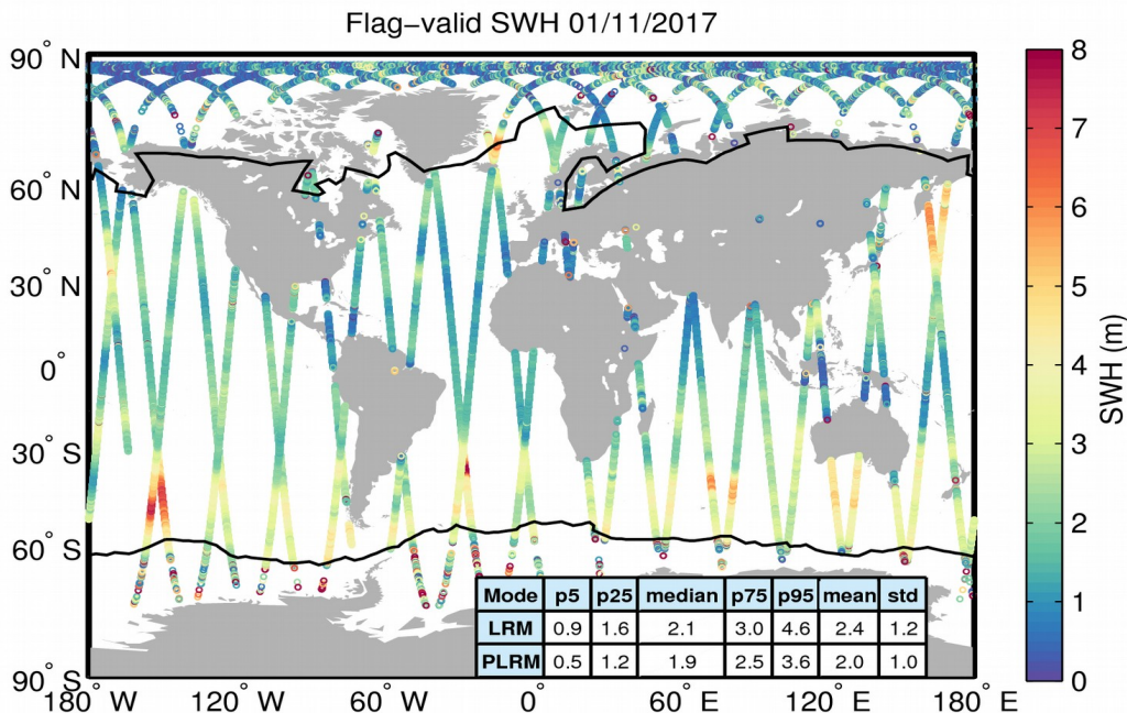
Figure 15. Geographical distribution of flag-valid SWH data over oceans and lakes for 01/11/2017. The statistical values shown in the table refer to the SWH in m and are calculated separately for LRM and PLRM regions. Measurements taken over polar polygons have been excluded from the computation of the statistical values. The black lines mark the outer limit of the Arctic and Antarctic polar polygons.
