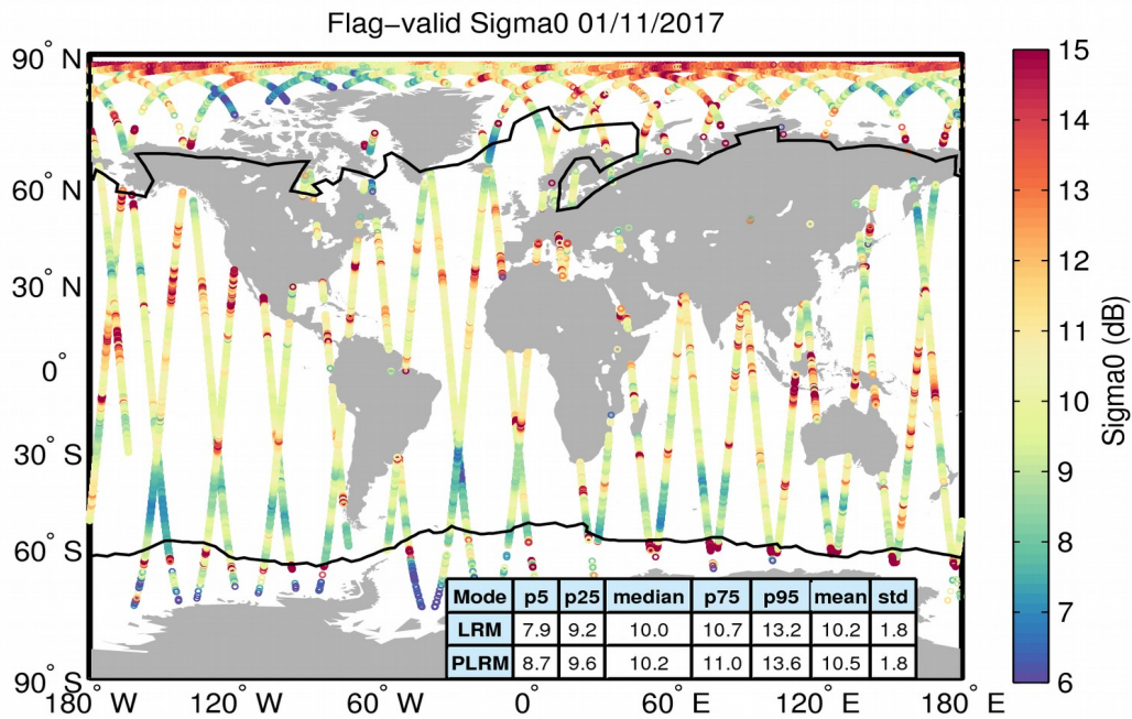
Figure 23. Geographical distribution of flag-valid sigma0 data over oceans and lakes for 01/11/2017. The statistical values shown in the table refer to the sigma0 in dB and are calculated separately for LRM and PLRM regions. Measurements taken over polar polygons have been excluded from the computation of the statistical values. The black lines mark the outer limit of the Arctic and Antarctic polar polygons.
