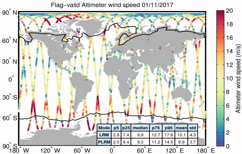
Figure 31. Geographical distribution of flag-valid wind data over oceans and lakes for 01/11/2017. The statistical values shown in the table refer to the wind in m/s and are calculated separately for LRM and PLRM regions. Measurements taken over polar polygons have been excluded from the computation of the statistical values. The black lines mark the outer limit of the Arctic and Antarctic polar polygons.
