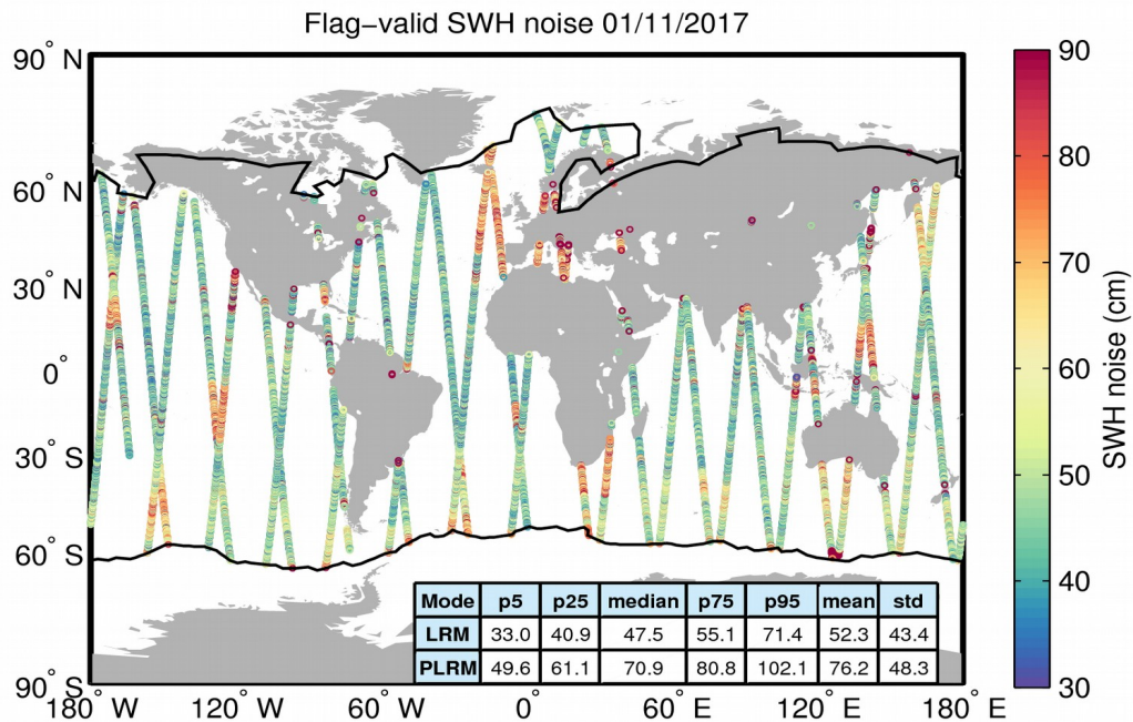
Figure 18. Geographical distribution of flag-valid 20-Hz SWH measurement noise over oceans and lakes for 01/11/2017. The statistical values shown in the table refer to the SWH noise and are calculated separately for LRM and PLRM regions. Measurements taken over polar polygons have been excluded from the computation of the statistical values. The black lines mark the outer limit of the Arctic and Antarctic polar polygons.
