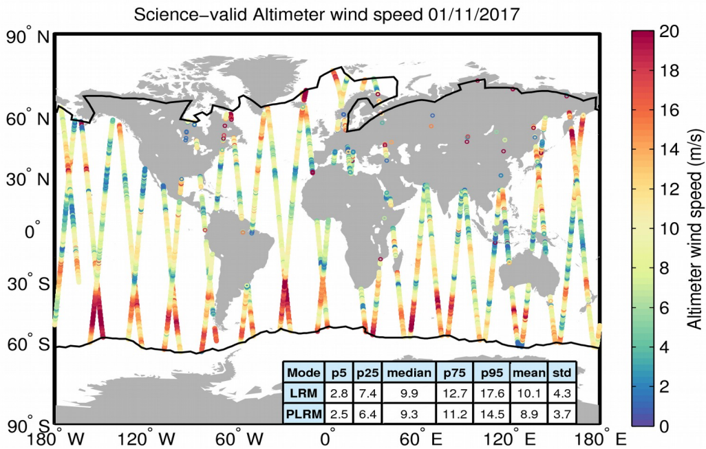
Figure 34. Geographical distribution of science-valid wind data over oceans and lakes for 01/11/2017. The statistical values shown in the table refer to the wind in m/s and are calculated separately for LRM and PLRM regions. The black lines mark the outer limit of the Arctic and Antarctic polar polygons. Gray circles denote records that have been rejected based on the editing criteria described in Table 5.
