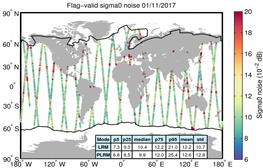
Figure 26. Geographical distribution of flag-valid 20-Hz sigma0 measurement noise over oceans and lakes for 01/11/2017. The statistical values shown in the table refer to the sigma0 noise and are calculated separately for LRM and PLRM regions. Measurements taken over polar polygons have been excluded from the computation of the statistical values. The black lines mark the outer limit of the Arctic and Antarctic polar polygons.
