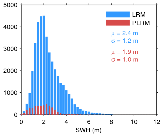
Figure 20. Histogram of science-valid SWH over oceans and lakes for LRM (blue) and PLRM (red) for 01/11/2017. The mean ( \mu ) and standard deviation ( \sigma ) are also shown. Note that values larger than 12 m are excluded from the histogram for the sake of readability but not from the computation of \mu and \sigma .
