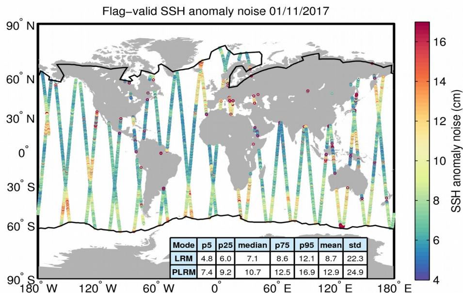
Figure 8. Geographical distribution of flag-valid 20-Hz SSH anomaly measurement noise over oceans and lakes for 01/11/2017. The statistical values shown in the table refer to the SSH anomaly noise and are calculated separately for LRM and PLRM regions. Measurements taken over polar polygons have been excluded from the computation of the statistical values. The black lines mark the outer limit of the Arctic and Antarctic polar polygons.
