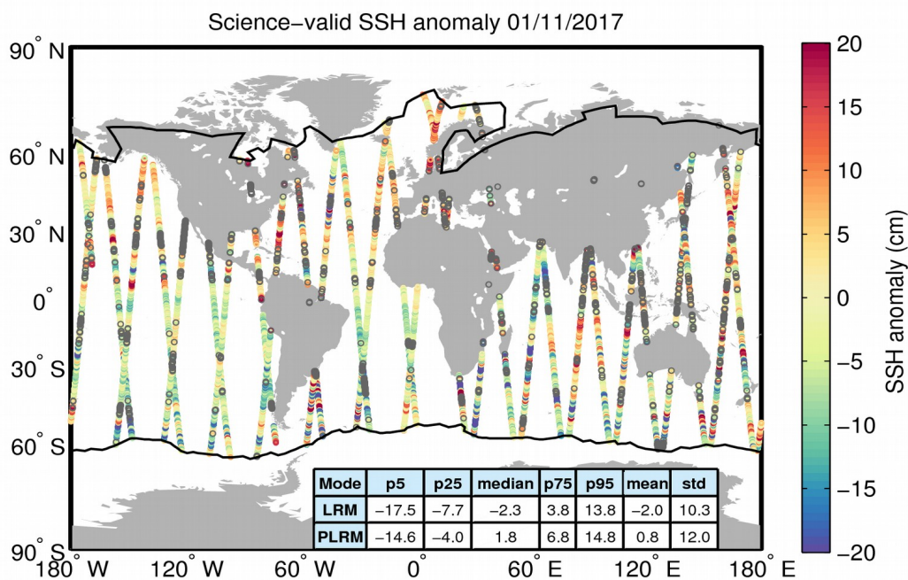
Figure 10. Geographical distribution of science-valid SSH anomaly data over oceans and lakes for 01/11/2017. The statistical values shown in the table refer to the SSH anomaly in cm and are calculated separately for LRM and PLRM regions. The black lines mark the outer limit of the Arctic and Antarctic polar polygons. Gray circles denote records that have been rejected based on the editing criteria described in Table 2.
