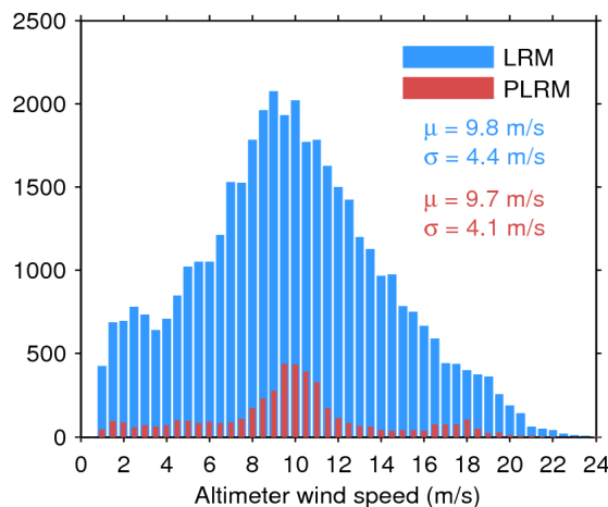
Figure 35. Histogram of science-valid wind over oceans and lakes for LRM (blue) and PLRM (red) for 28/10/2017. The mean ( \mu ) and standard deviation ( \sigma ) are also shown. Note that values larger than 24 m/s are excluded from the histogram for the sake of readability but not from the computation of \mu and \sigma .
