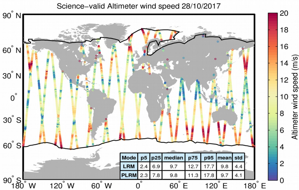
Figure 34. Geographical distribution of science-valid wind data over oceans and lakes for 28/10/2017. The statistical values shown in the table refer to the wind in m/s and are calculated separately for LRM and PLRM regions. The black lines mark the outer limit of the Arctic and Antarctic polar polygons. Gray circles denote records that have been rejected based on the editing criteria described in Table 5.
