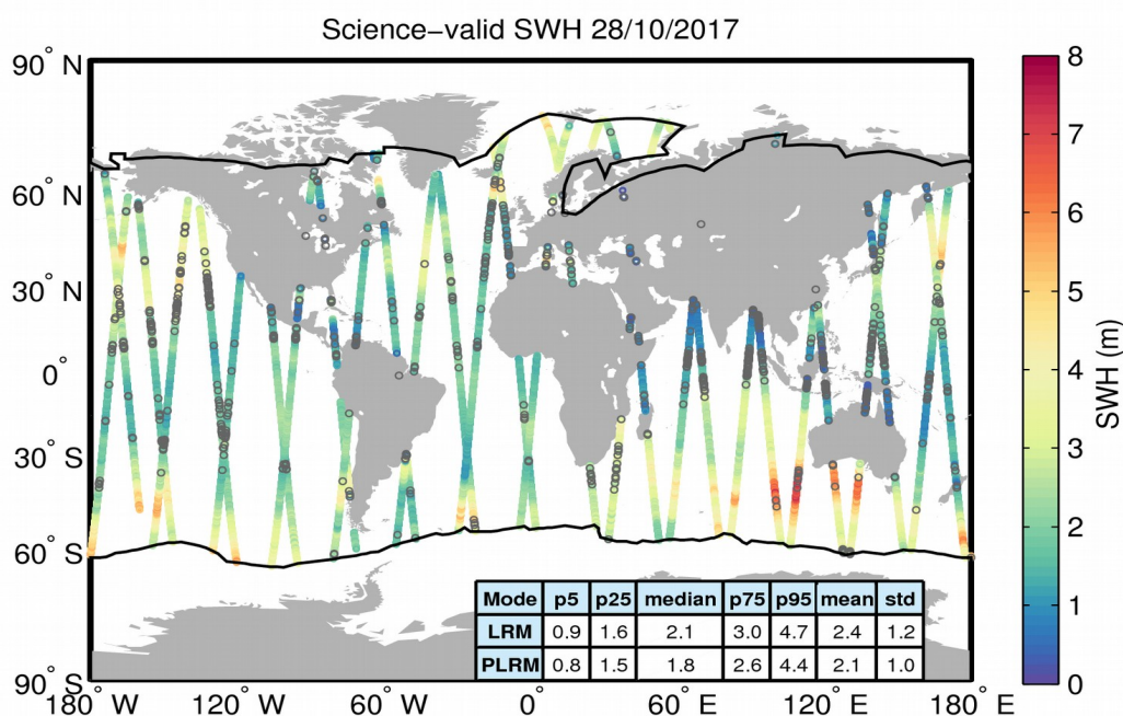
Figure 19. Geographical distribution of science-valid SWH data over oceans and lakes for 28/10/2017. The statistical values shown in the table refer to the SWH in m and are calculated separately for LRM and PLRM regions. The black lines mark the outer limit of the Arctic and Antarctic polar polygons. Gray circles denote records that have been rejected based on the editing criteria described in Table 3.
