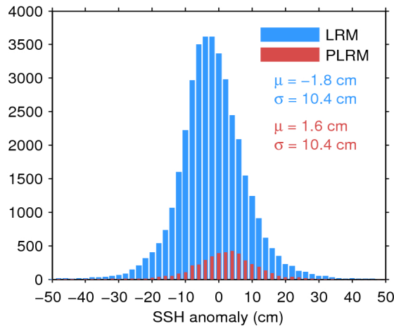
Figure 11. Histogram of science-valid SSH anomaly over oceans and lakes for LRM (blue) and PLRM (red) for 28/10/2017. The mean ( \mu ) and standard deviation ( \sigma ) are also shown. Note that values outside [-50\ 50] cm are excluded from the histogram for the sake of readability but not from the computation of \mu and \sigma .
