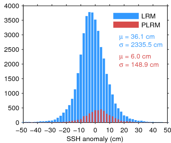
Figure 7. Histogram of flag-valid SSH anomaly over oceans and lakes for LRM (blue) and PLRM (red) for 28/10/2017. The mean ( \mu ) and standard deviation ( \sigma ) are also shown. Note that values outside [-50 50] cm are excluded from the histogram for the sake of readability but not from the computation of \mu and \sigma .
