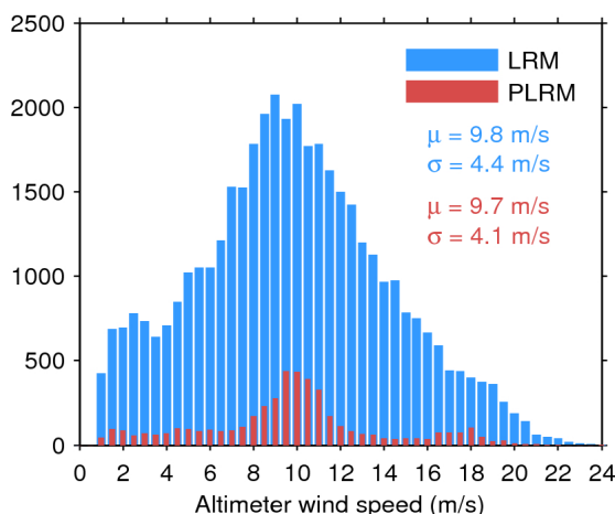
Figure 33. Histogram of flag-valid wind over oceans and lakes for LRM (blue) and PLRM (red) for 28/10/2017. The mean ( \mu ) and standard deviation ( \sigma ) are also shown. Note that values larger than 24 m/s are excluded from the histogram for the sake of readability but not from the computation of \mu and \sigma .
