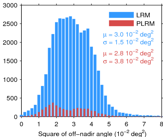
Figure 39. Histogram of flag-valid mispointing over oceans and lakes for LRM (blue) and PLRM (red) for 28/10/2017. Only positive values have been considered. The mean ( \mu ) and standard deviation ( \sigma ) are also shown. Note that values larger than 8 \cdot 10^{-2} \text{ deg}^2 are excluded from the histogram for the sake of readability but not from the computation of \mu and \sigma .
