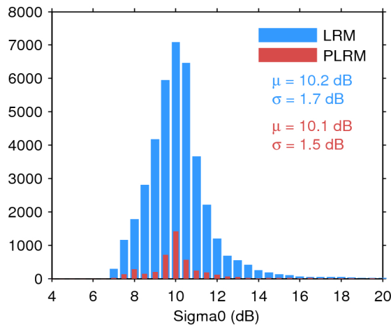
Figure 28. Histogram of science-valid sigma0 over oceans and lakes for LRM (blue) and PLRM (red) for 28/10/2017. The mean ( \mu ) and standard deviation ( \sigma ) are also shown. Note that values outside [4 20] dB are excluded from the histogram for the sake of readability but not from the computation of \mu and \sigma .
