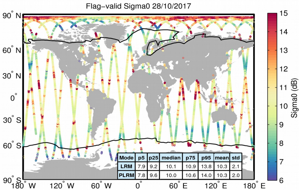
Figure 23. Geographical distribution of flag-valid sigma0 data over oceans and lakes for 28/10/2017. The statistical values shown in the table refer to the sigma0 in dB and are calculated separately for LRM and PLRM regions. Measurements taken over polar polygons have been excluded from the computation of the statistical values. The black lines mark the outer limit of the Arctic and Antarctic polar polygons.
