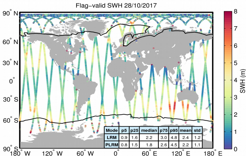
Figure 15. Geographical distribution of flag-valid SWH data over oceans and lakes for 28/10/2017. The statistical values shown in the table refer to the SWH in m and are calculated separately for LRM and PLRM regions. Measurements taken over polar polygons have been excluded from the computation of the statistical values. The black lines mark the outer limit of the Arctic and Antarctic polar polygons.
