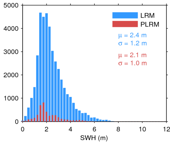
Figure 20. Histogram of science-valid SWH over oceans and lakes for LRM (blue) and PLRM (red) for 28/10/2017. The mean ( \mu ) and standard deviation ( \sigma ) are also shown. Note that values larger than 12 m are excluded from the histogram for the sake of readability but not from the computation of \mu and \sigma .
