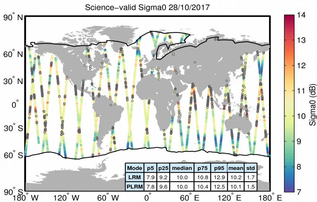
Figure 27. Geographical distribution of science-valid sigma0 data over oceans and lakes for 28/10/2017. The statistical values shown in the table refer to the sigma0 in dB and are calculated separately for LRM and PLRM regions. The black lines mark the outer limit of the Arctic and Antarctic polar polygons. Gray circles denote records that have been rejected based on the editing criteria described in Table 4.
