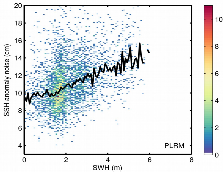
Figure 9. 2D histogram showing flag-valid SSH anomaly noise as a function of SWH for LRM (top) and PLRM (bottom) for 28/10/2017. The black line denotes the median SSH anomaly noise as a function of SWH.
