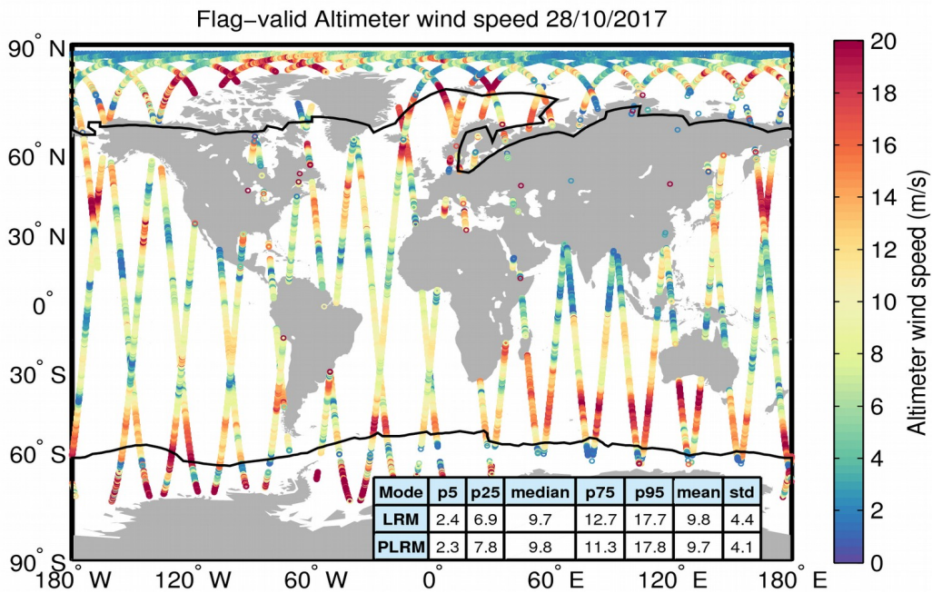
Figure 31. Geographical distribution of flag-valid wind data over oceans and lakes for 28/10/2017. The statistical values shown in the table refer to the wind in m/s and are calculated separately for LRM and PLRM regions. Measurements taken over polar polygons have been excluded from the computation of the statistical values. The black lines mark the outer limit of the Arctic and Antarctic polar polygons.
