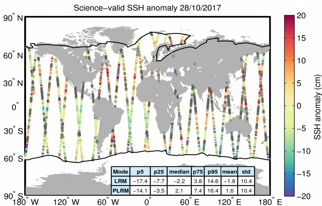
Figure 10. Geographical distribution of science-valid SSH anomaly data over oceans and lakes for 28/10/2017. The statistical values shown in the table refer to the SSH anomaly in cm and are calculated separately for LRM and PLRM regions. The black lines mark the outer limit of the Arctic and Antarctic polar polygons. Gray circles denote records that have been rejected based on the editing criteria described in Table 2.
