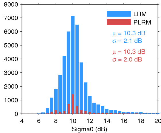
Figure 25. Histogram of flag-valid sigma0 over oceans and lakes for LRM (blue) and PLRM (red) for 28/10/2017. The mean ( \mu ) and standard deviation ( \sigma ) are also shown. Note that values outside [4 20] dB are excluded from the histogram for the sake of readability but not from the computation of \mu and \sigma .
