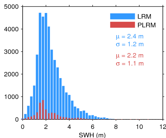
Figure 17. Histogram of flag-valid SWH over oceans and lakes for LRM (blue) and PLRM (red) for 28/10/2017. The mean ( \mu ) and standard deviation ( \sigma ) are also shown. Note that values larger than 12 m are excluded from the histogram for the sake of readability but not from the computation of \mu and \sigma .
