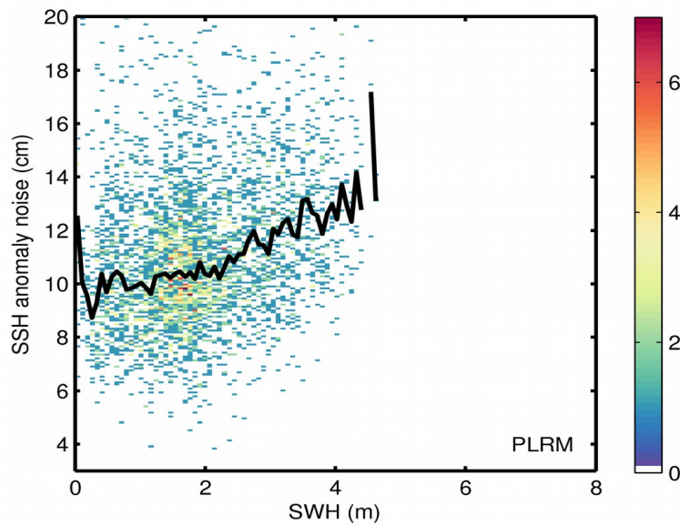
Figure 9. 2D histogram showing flag-valid SSH anomaly noise as a function of SWH for LRM (top) and PLRM (bottom) for 27/10/2017. The black line denotes the median SSH anomaly noise as a function of SWH.
