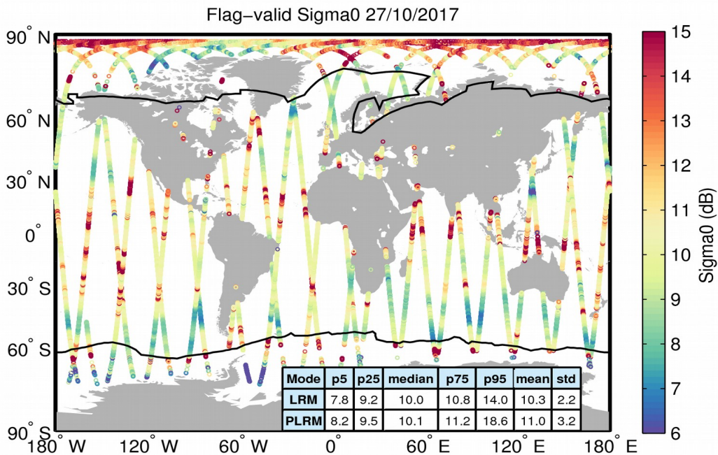
Figure 23. Geographical distribution of flag-valid sigma0 data over oceans and lakes for 27/10/2017. The statistical values shown in the table refer to the sigma0 in dB and are calculated separately for LRM and PLRM regions. Measurements taken over polar polygons have been excluded from the computation of the statistical values. The black lines mark the outer limit of the Arctic and Antarctic polar polygons.
