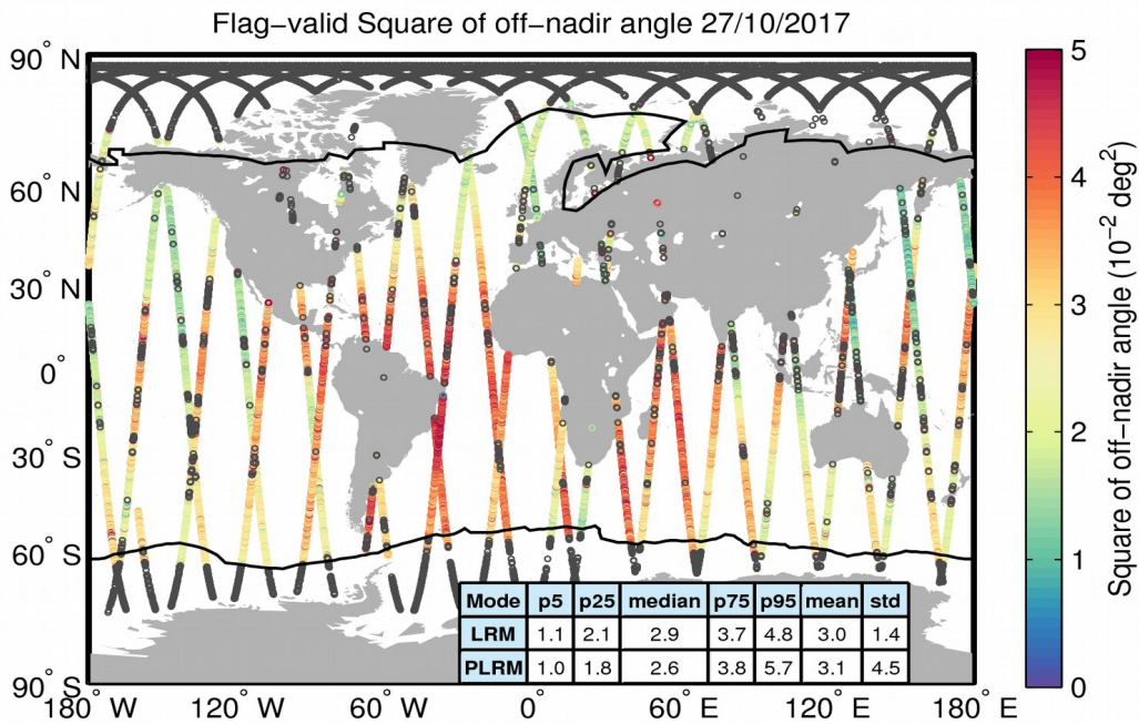
Figure 37. Geographical distribution of flag-valid mispointing data over oceans and lakes for 27/10/2017. The statistical values shown in the table refer to the mispointing in 10^{-2} deg 2 and are calculated separately for LRM and PLRM regions. Measurements taken over polar polygons have been excluded from the computation of the statistical values. The black lines mark the outer limit of the Arctic and Antarctic polar polygons. Gray circles denote negative values.
