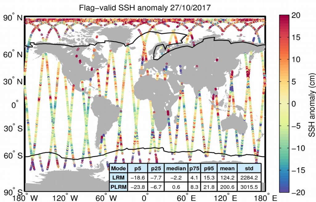
Figure 5. Geographical distribution of flag-valid 1-Hz SSH anomaly data over oceans and lakes for 27/10/2017. The statistical values shown in the table refer to the SSH anomaly in cm and are calculated separately for LRM and PLRM regions. Measurements taken over polar polygons have been excluded from the computation of the statistical values. The black lines mark the outer limit of the Arctic and Antarctic polar polygons.
