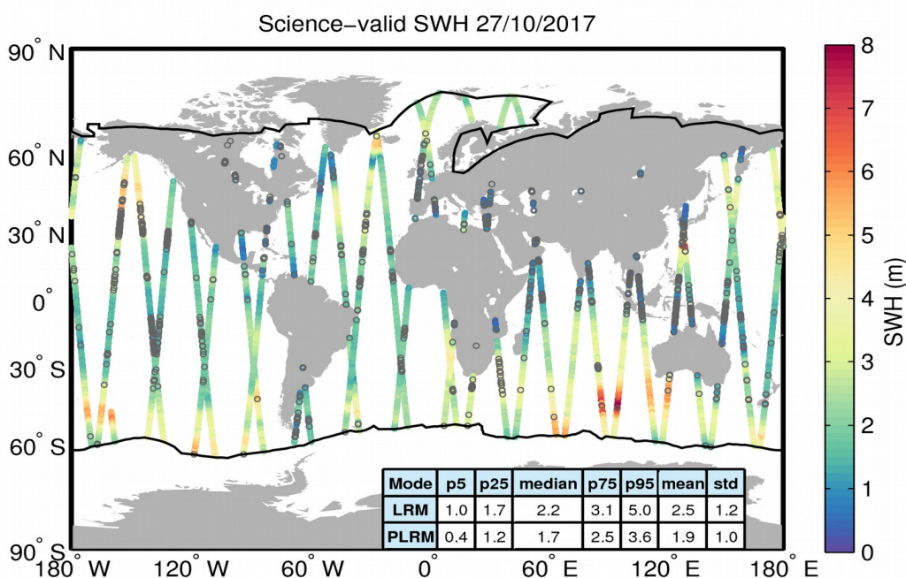
Figure 19. Geographical distribution of science-valid SWH data over oceans and lakes for 27/10/2017. The statistical values shown in the table refer to the SWH in m and are calculated separately for LRM and PLRM regions. The black lines mark the outer limit of the Arctic and Antarctic polar polygons. Gray circles denote records that have been rejected based on the editing criteria described in Table 3.
