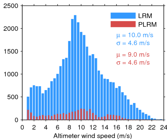
Figure 35. Histogram of science-valid wind over oceans and lakes for LRM (blue) and PLRM (red) for 27/10/2017. The mean ( \mu ) and standard deviation ( \sigma ) are also shown. Note that values larger than 24 m/s are excluded from the histogram for the sake of readability but not from the computation of \mu and \sigma .
