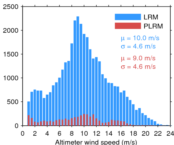
Figure 33. Histogram of flag-valid wind over oceans and lakes for LRM (blue) and PLRM (red) for 27/10/2017. The mean ( \mu ) and standard deviation ( \sigma ) are also shown. Note that values larger than 24 m/s are excluded from the histogram for the sake of readability but not from the computation of \mu and \sigma .
