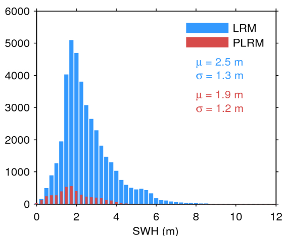
Figure 17. Histogram of flag-valid SWH over oceans and lakes for LRM (blue) and PLRM (red) for 27/10/2017. The mean ( \mu ) and standard deviation ( \sigma ) are also shown. Note that values larger than 12 m are excluded from the histogram for the sake of readability but not from the computation of \mu and \sigma .
