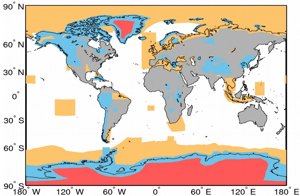
Figure A1. Extent of the regions defining the geographical mode mask for 27/10/2017. The regions where SAR, and SARIn are operated are denoted by the orange and blue polygons, respectively. LRM is operated over areas of the continental ice sheets (red polygons) and over oceans and land not covered by other modes.
