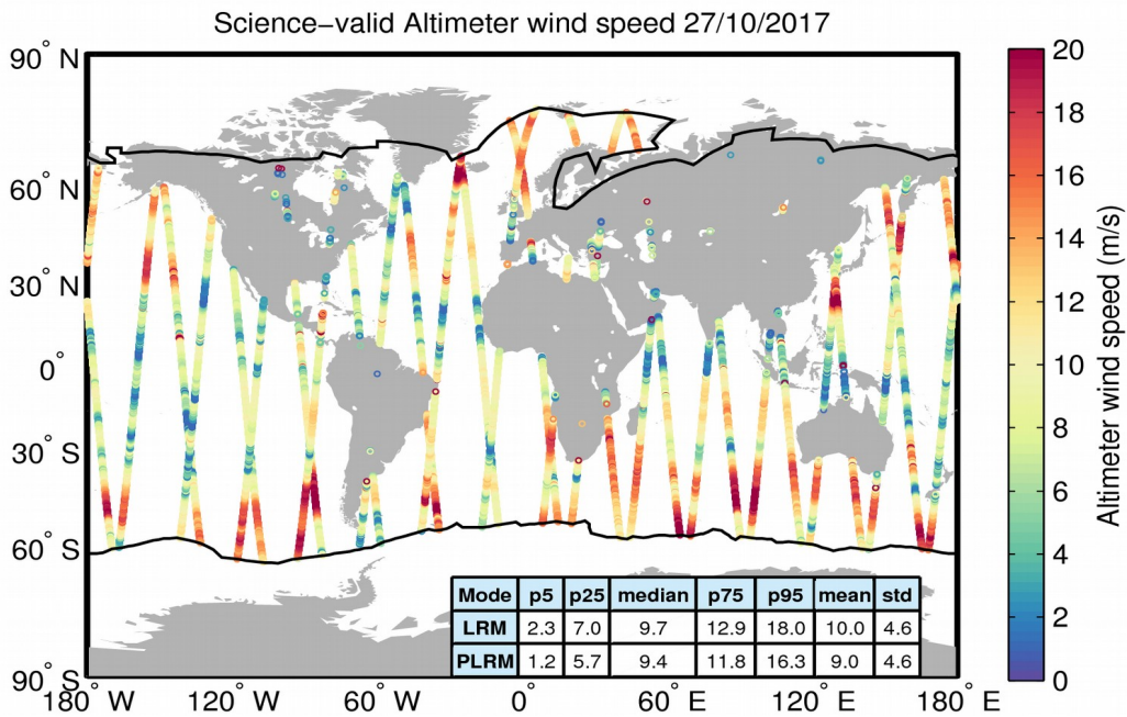
Figure 34. Geographical distribution of science-valid wind data over oceans and lakes for 27/10/2017. The statistical values shown in the table refer to the wind in m/s and are calculated separately for LRM and PLRM regions. The black lines mark the outer limit of the Arctic and Antarctic polar polygons. Gray circles denote records that have been rejected based on the editing criteria described in Table 5.
