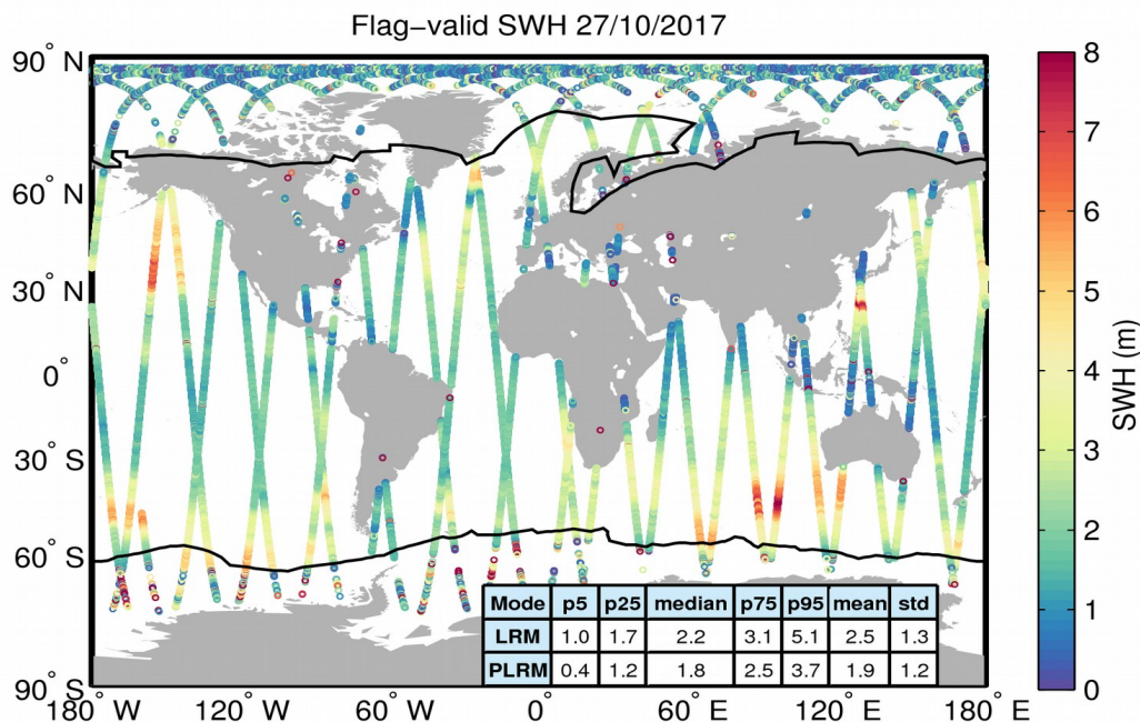
Figure 15. Geographical distribution of flag-valid SWH data over oceans and lakes for 27/10/2017. The statistical values shown in the table refer to the SWH in m and are calculated separately for LRM and PLRM regions. Measurements taken over polar polygons have been excluded from the computation of the statistical values. The black lines mark the outer limit of the Arctic and Antarctic polar polygons.
