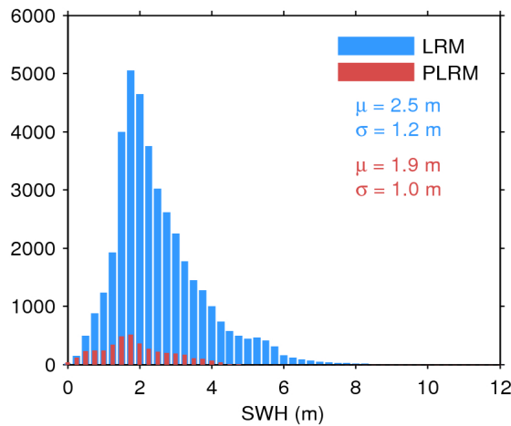
Figure 20. Histogram of science-valid SWH over oceans and lakes for LRM (blue) and PLRM (red) for 27/10/2017. The mean ( \mu ) and standard deviation ( \sigma ) are also shown. Note that values larger than 12 m are excluded from the histogram for the sake of readability but not from the computation of \mu and \sigma .
