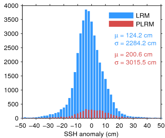
Figure 7. Histogram of flag-valid SSH anomaly over oceans and lakes for LRM (blue) and PLRM (red) for 27/10/2017. The mean ( \mu ) and standard deviation ( \sigma ) are also shown. Note that values outside [-50 50] cm are excluded from the histogram for the sake of readability but not from the computation of \mu and \sigma .
