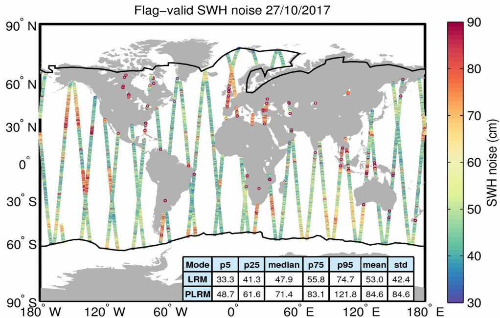
Figure 18. Geographical distribution of flag-valid 20-Hz SWH measurement noise over oceans and lakes for 27/10/2017. The statistical values shown in the table refer to the SWH noise and are calculated separately for LRM and PLRM regions. Measurements taken over polar polygons have been excluded from the computation of the statistical values. The black lines mark the outer limit of the Arctic and Antarctic polar polygons.
