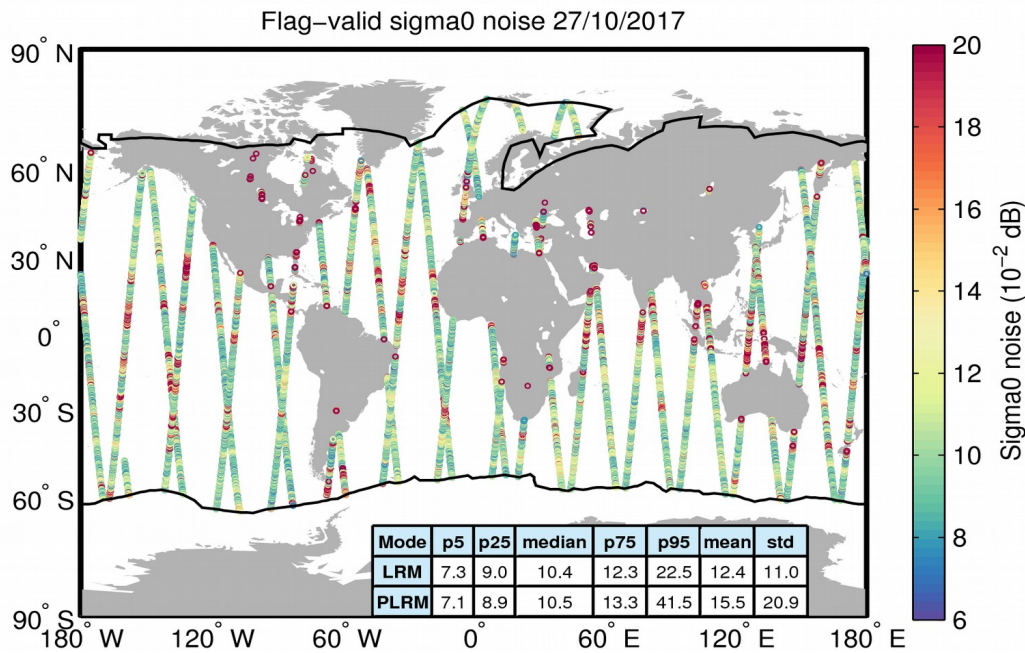
Figure 26. Geographical distribution of flag-valid 20-Hz sigma0 measurement noise over oceans and lakes for 27/10/2017. The statistical values shown in the table refer to the sigma0 noise and are calculated separately for LRM and PLRM regions. Measurements taken over polar polygons have been excluded from the computation of the statistical values. The black lines mark the outer limit of the Arctic and Antarctic polar polygons.
