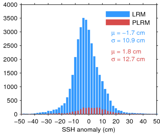
Figure 11. Histogram of science-valid SSH anomaly over oceans and lakes for LRM (blue) and PLRM (red) for 27/10/2017. The mean ( \mu ) and standard deviation ( \sigma ) are also shown. Note that values outside [-50\ 50] cm are excluded from the histogram for the sake of readability but not from the computation of \mu and \sigma .
