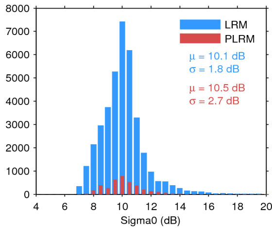
Figure 28. Histogram of science-valid sigma0 over oceans and lakes for LRM (blue) and PLRM (red) for 27/10/2017. The mean ( \mu ) and standard deviation ( \sigma ) are also shown. Note that values outside [4 20] dB are excluded from the histogram for the sake of readability but not from the computation of \mu and \sigma .
