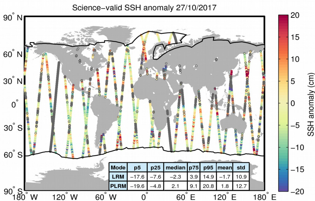
Figure 10. Geographical distribution of science-valid SSH anomaly data over oceans and lakes for 27/10/2017. The statistical values shown in the table refer to the SSH anomaly in cm and are calculated separately for LRM and PLRM regions. The black lines mark the outer limit of the Arctic and Antarctic polar polygons. Gray circles denote records that have been rejected based on the editing criteria described in Table 2.
