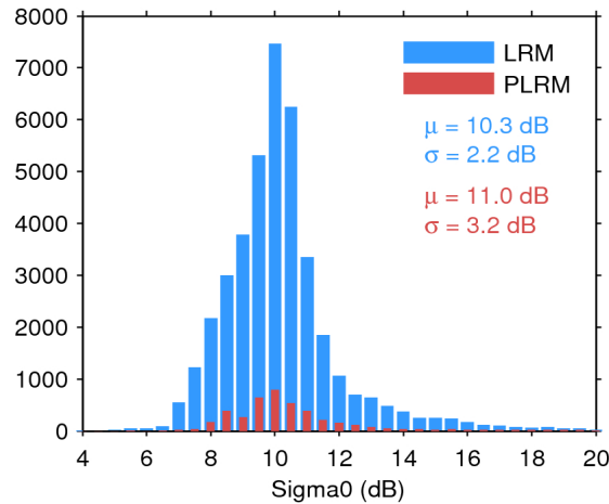
Figure 25. Histogram of flag-valid sigma0 over oceans and lakes for LRM (blue) and PLRM (red) for 27/10/2017. The mean ( \mu ) and standard deviation ( \sigma ) are also shown. Note that values outside [4 20] dB are excluded from the histogram for the sake of readability but not from the computation of \mu and \sigma .
