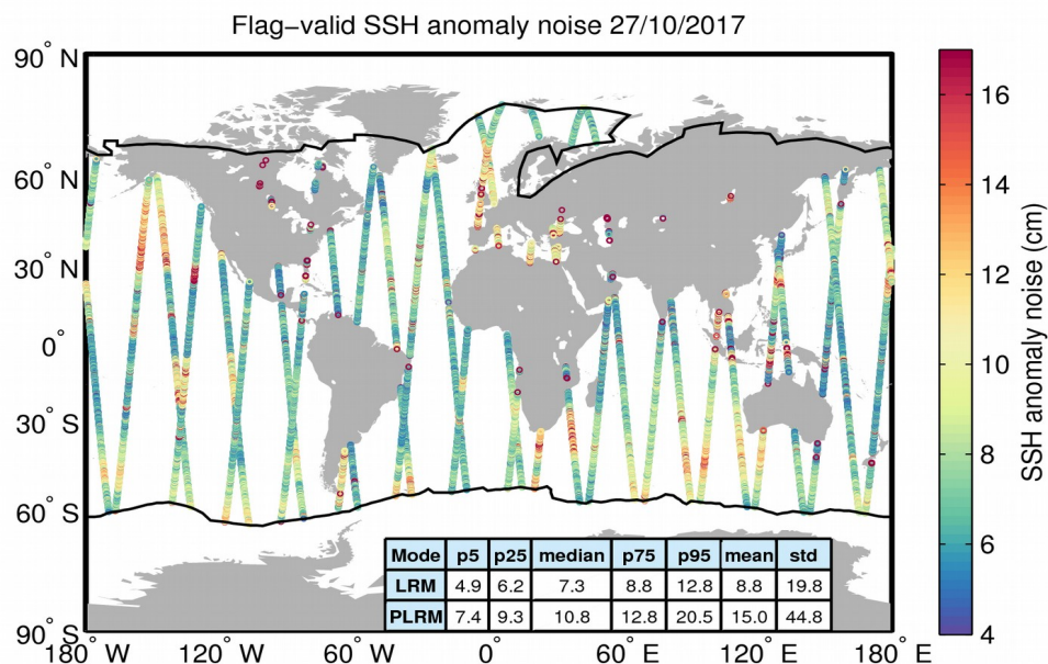
Figure 8. Geographical distribution of flag-valid 20-Hz SSH anomaly measurement noise over oceans and lakes for 27/10/2017. The statistical values shown in the table refer to the SSH anomaly noise and are calculated separately for LRM and PLRM regions. Measurements taken over polar polygons have been excluded from the computation of the statistical values. The black lines mark the outer limit of the Arctic and Antarctic polar polygons.
