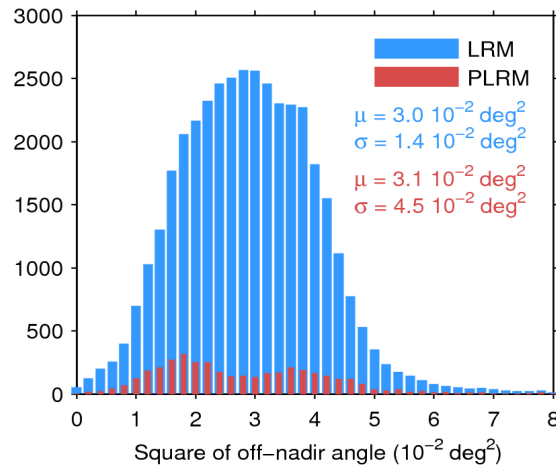
Figure 39. Histogram of flag-valid mispointing over oceans and lakes for LRM (blue) and PLRM (red) for 27/10/2017. Only positive values have been considered. The mean ( \mu ) and standard deviation ( \sigma ) are also shown. Note that values larger than 8 \cdot 10^{-2} \text{ deg}^2 are excluded from the histogram for the sake of readability but not from the computation of \mu and \sigma .
