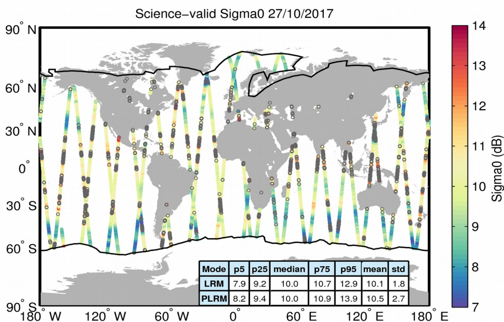
Figure 27. Geographical distribution of science-valid sigma0 data over oceans and lakes for 27/10/2017. The statistical values shown in the table refer to the sigma0 in dB and are calculated separately for LRM and PLRM regions. The black lines mark the outer limit of the Arctic and Antarctic polar polygons. Gray circles denote records that have been rejected based on the editing criteria described in Table 4.
