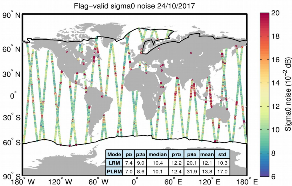
Figure 26. Geographical distribution of flag-valid 20-Hz sigma0 measurement noise over oceans and lakes for 24/10/2017. The statistical values shown in the table refer to the sigma0 noise and are calculated separately for LRM and PLRM regions. Measurements taken over polar polygons have been excluded from the computation of the statistical values. The black lines mark the outer limit of the Arctic and Antarctic polar polygons.
