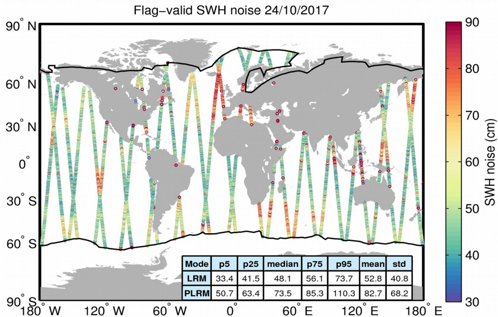
Figure 18. Geographical distribution of flag-valid 20-Hz SWH measurement noise over oceans and lakes for 24/10/2017. The statistical values shown in the table refer to the SWH noise and are calculated separately for LRM and PLRM regions. Measurements taken over polar polygons have been excluded from the computation of the statistical values. The black lines mark the outer limit of the Arctic and Antarctic polar polygons.
