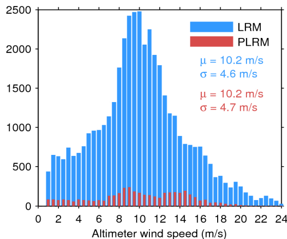
Figure 35. Histogram of science-valid wind over oceans and lakes for LRM (blue) and PLRM (red) for 24/10/2017. The mean ( \mu ) and standard deviation ( \sigma ) are also shown. Note that values larger than 24 m/s are excluded from the histogram for the sake of readability but not from the computation of \mu and \sigma .
