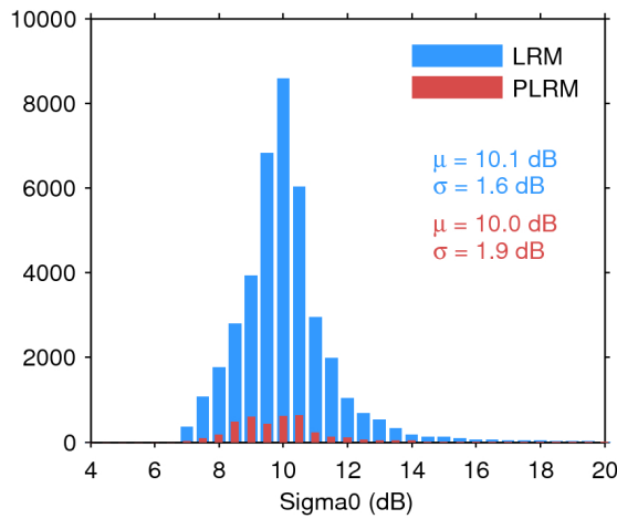
Figure 28. Histogram of science-valid sigma0 over oceans and lakes for LRM (blue) and PLRM (red) for 24/10/2017. The mean ( \mu ) and standard deviation ( \sigma ) are also shown. Note that values outside [4 20] dB are excluded from the histogram for the sake of readability but not from the computation of \mu and \sigma .
