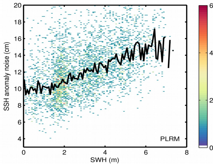
Figure 9. 2D histogram showing flag-valid SSH anomaly noise as a function of SWH for LRM (top) and PLRM (bottom) for 24/10/2017. The black line denotes the median SSH anomaly noise as a function of SWH.
