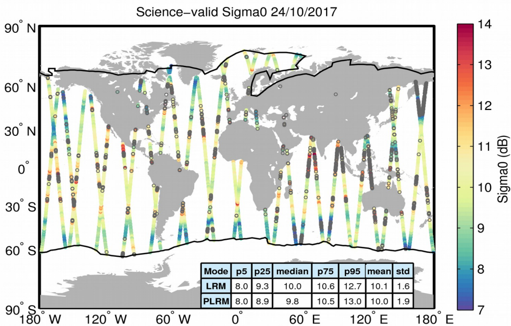
Figure 27. Geographical distribution of science-valid sigma0 data over oceans and lakes for 24/10/2017. The statistical values shown in the table refer to the sigma0 in dB and are calculated separately for LRM and PLRM regions. The black lines mark the outer limit of the Arctic and Antarctic polar polygons. Gray circles denote records that have been rejected based on the editing criteria described in Table 4.
