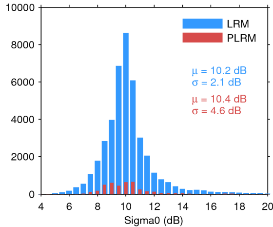
Figure 25. Histogram of flag-valid sigma0 over oceans and lakes for LRM (blue) and PLRM (red) for 24/10/2017. The mean ( \mu ) and standard deviation ( \sigma ) are also shown. Note that values outside [4 20] dB are excluded from the histogram for the sake of readability but not from the computation of \mu and \sigma .
