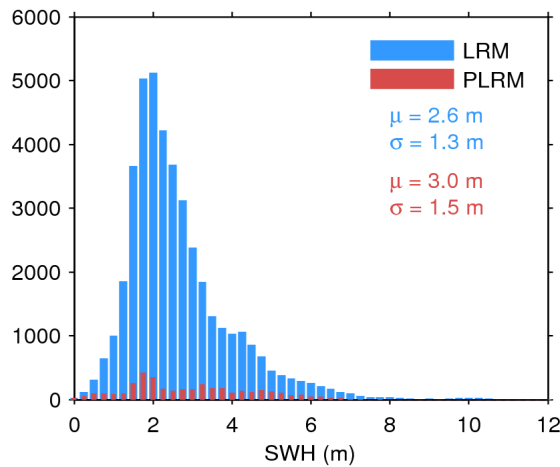
Figure 20. Histogram of science-valid SWH over oceans and lakes for LRM (blue) and PLRM (red) for 24/10/2017. The mean ( \mu ) and standard deviation ( \sigma ) are also shown. Note that values larger than 12 m are excluded from the histogram for the sake of readability but not from the computation of \mu and \sigma .
