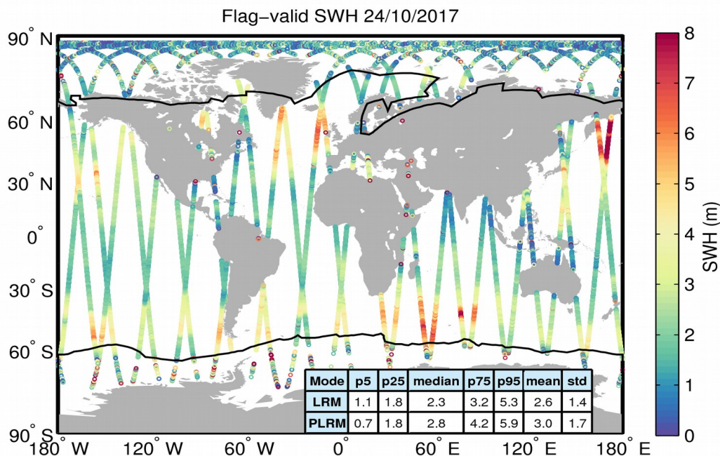
Figure 15. Geographical distribution of flag-valid SWH data over oceans and lakes for 24/10/2017. The statistical values shown in the table refer to the SWH in m and are calculated separately for LRM and PLRM regions. Measurements taken over polar polygons have been excluded from the computation of the statistical values. The black lines mark the outer limit of the Arctic and Antarctic polar polygons.
