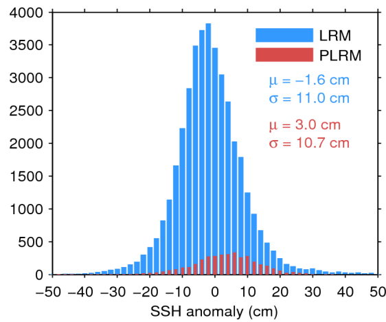
Figure 11. Histogram of science-valid SSH anomaly over oceans and lakes for LRM (blue) and PLRM (red) for 24/10/2017. The mean ( \mu ) and standard deviation ( \sigma ) are also shown. Note that values outside [-50\ 50] cm are excluded from the histogram for the sake of readability but not from the computation of \mu and \sigma .
