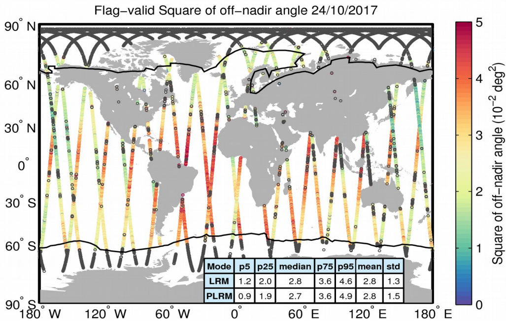
Figure 37. Geographical distribution of flag-valid mispointing data over oceans and lakes for 24/10/2017. The statistical values shown in the table refer to the mispointing in 10^{-2} \text{ deg}^2 and are calculated separately for LRM and PLRM regions. Measurements taken over polar polygons have been excluded from the computation of the statistical values. The black lines mark the outer limit of the Arctic and Antarctic polar polygons. Gray circles denote negative values.
