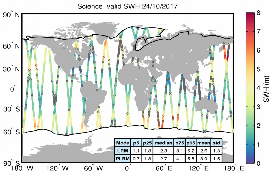
Figure 19. Geographical distribution of science-valid SWH data over oceans and lakes for 24/10/2017. The statistical values shown in the table refer to the SWH in m and are calculated separately for LRM and PLRM regions. The black lines mark the outer limit of the Arctic and Antarctic polar polygons. Gray circles denote records that have been rejected based on the editing criteria described in Table 3.
