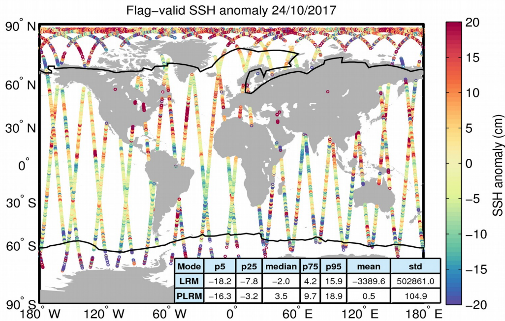
Figure 5. Geographical distribution of flag-valid 1-Hz SSH anomaly data over oceans and lakes for 24/10/2017. The statistical values shown in the table refer to the SSH anomaly in cm and are calculated separately for LRM and PLRM regions. Measurements taken over polar polygons have been excluded from the computation of the statistical values. The black lines mark the outer limit of the Arctic and Antarctic polar polygons.
