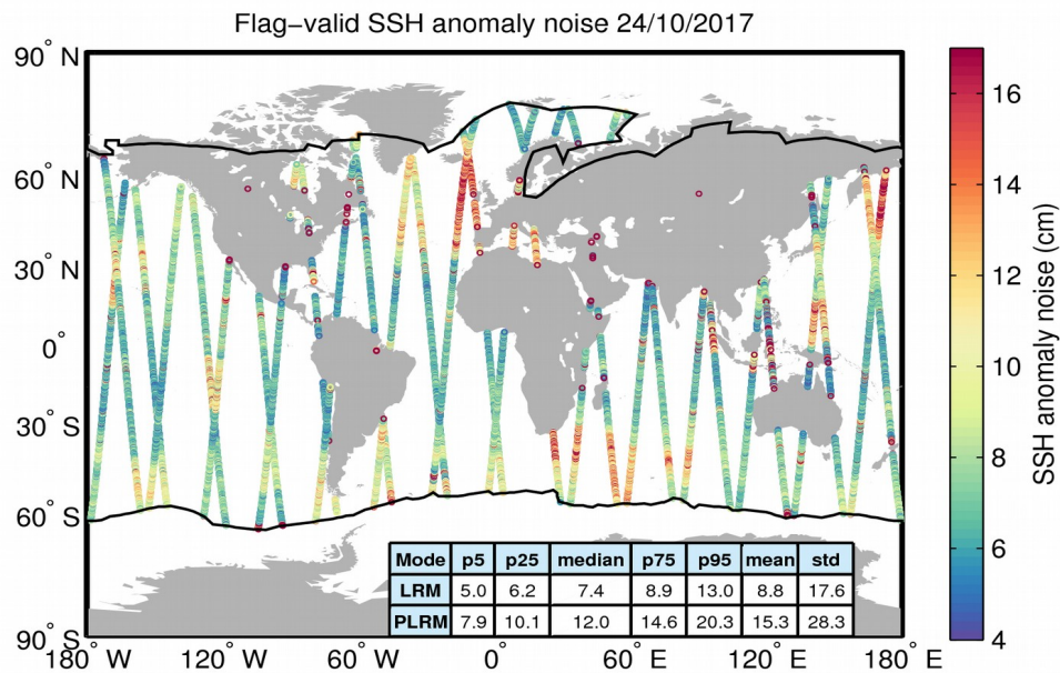
Figure 8. Geographical distribution of flag-valid 20-Hz SSH anomaly measurement noise over oceans and lakes for 24/10/2017. The statistical values shown in the table refer to the SSH anomaly noise and are calculated separately for LRM and PLRM regions. Measurements taken over polar polygons have been excluded from the computation of the statistical values. The black lines mark the outer limit of the Arctic and Antarctic polar polygons.
