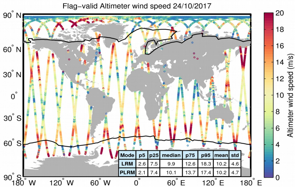
Figure 31. Geographical distribution of flag-valid wind data over oceans and lakes for 24/10/2017. The statistical values shown in the table refer to the wind in m/s and are calculated separately for LRM and PLRM regions. Measurements taken over polar polygons have been excluded from the computation of the statistical values. The black lines mark the outer limit of the Arctic and Antarctic polar polygons.
