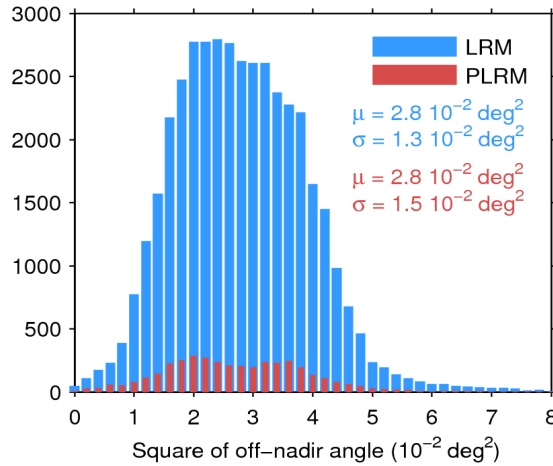
Figure 39. Histogram of flag-valid mispointing over oceans and lakes for LRM (blue) and PLRM (red) for 24/10/2017. Only positive values have been considered. The mean ( \mu ) and standard deviation ( \sigma ) are also shown. Note that values larger than 8 \cdot 10^{-2} \text{ deg}^2 are excluded from the histogram for the sake of readability but not from the computation of \mu and \sigma .
