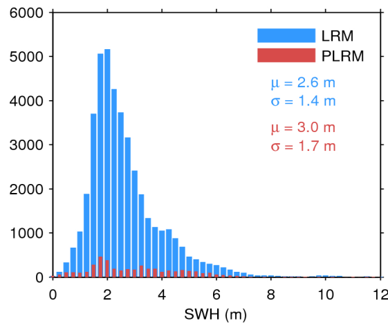
Figure 17. Histogram of flag-valid SWH over oceans and lakes for LRM (blue) and PLRM (red) for 24/10/2017. The mean ( \mu ) and standard deviation ( \sigma ) are also shown. Note that values larger than 12 m are excluded from the histogram for the sake of readability but not from the computation of \mu and \sigma .
