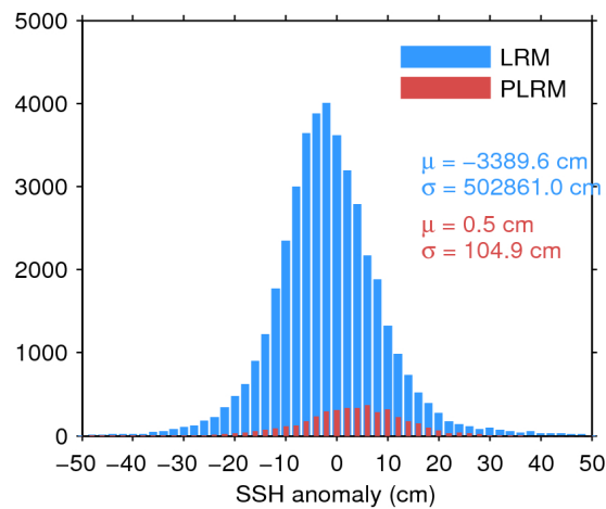
Figure 7. Histogram of flag-valid SSH anomaly over oceans and lakes for LRM (blue) and PLRM (red) for 24/10/2017. The mean ( \mu ) and standard deviation ( \sigma ) are also shown. Note that values outside [-50\ 50] cm are excluded from the histogram for the sake of readability but not from the computation of \mu and \sigma .
