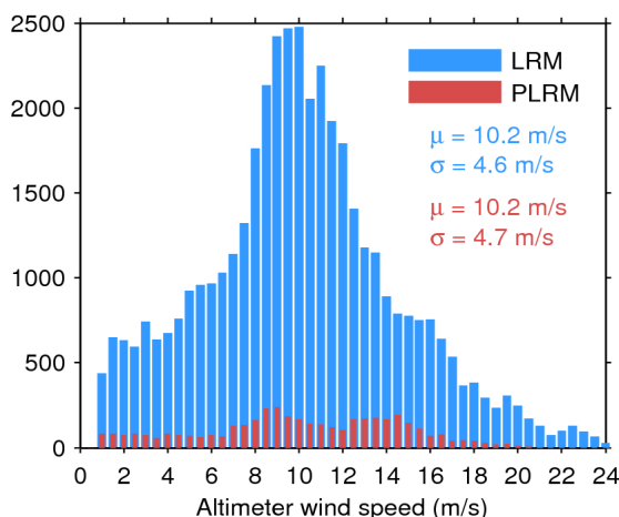
Figure 33. Histogram of flag-valid wind over oceans and lakes for LRM (blue) and PLRM (red) for 24/10/2017. The mean ( \mu ) and standard deviation ( \sigma ) are also shown. Note that values larger than 24 m/s are excluded from the histogram for the sake of readability but not from the computation of \mu and \sigma .
