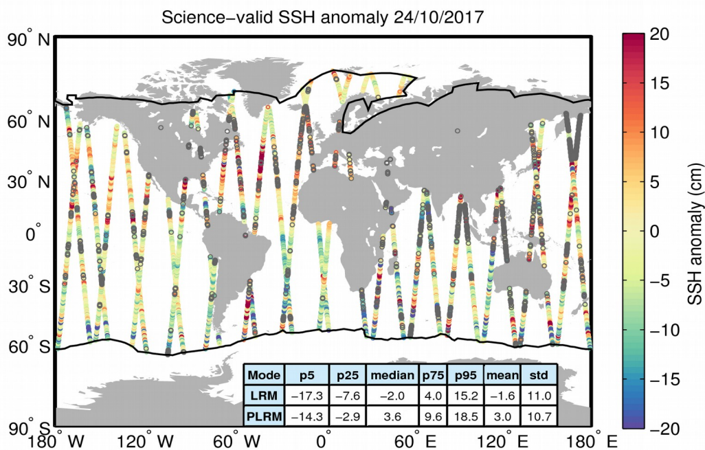
Figure 10. Geographical distribution of science-valid SSH anomaly data over oceans and lakes for 24/10/2017. The statistical values shown in the table refer to the SSH anomaly in cm and are calculated separately for LRM and PLRM regions. The black lines mark the outer limit of the Arctic and Antarctic polar polygons. Gray circles denote records that have been rejected based on the editing criteria described in Table 2.
