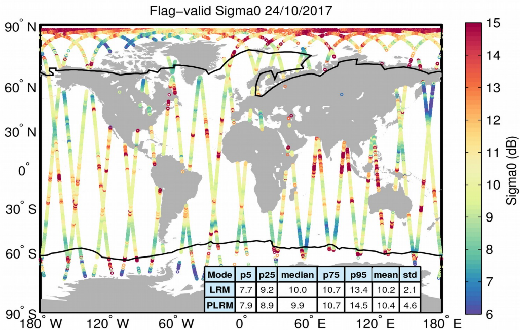
Figure 23. Geographical distribution of flag-valid sigma0 data over oceans and lakes for 24/10/2017. The statistical values shown in the table refer to the sigma0 in dB and are calculated separately for LRM and PLRM regions. Measurements taken over polar polygons have been excluded from the computation of the statistical values. The black lines mark the outer limit of the Arctic and Antarctic polar polygons.
