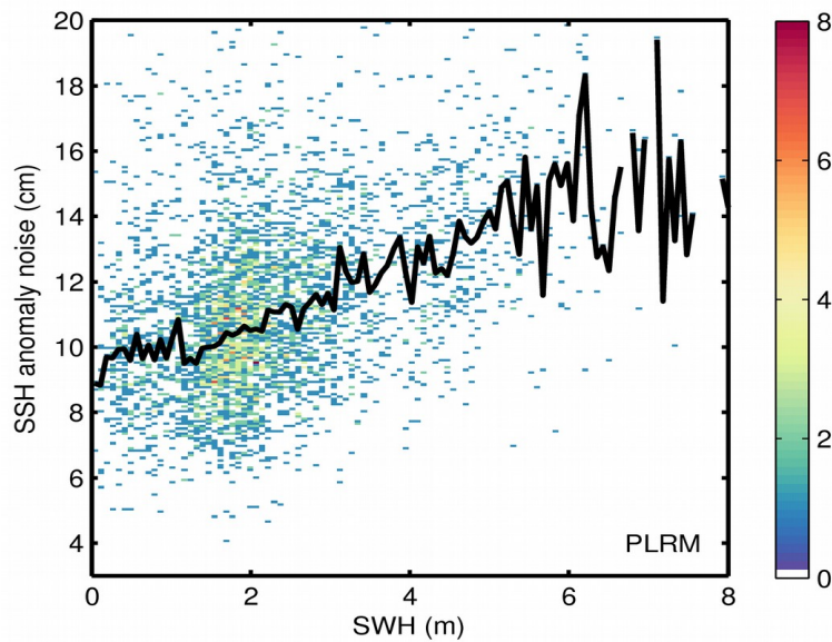
Figure 9. 2D histogram showing flag-valid SSH anomaly noise as a function of SWH for LRM (top) and PLRM (bottom) for 23/10/2017. The black line denotes the median SSH anomaly noise as a function of SWH.
