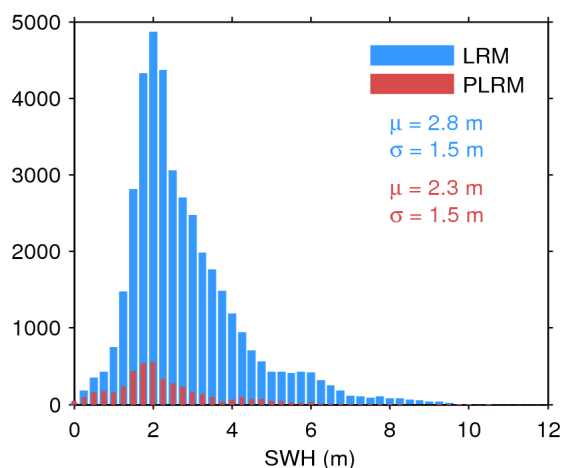
Figure 17. Histogram of flag-valid SWH over oceans and lakes for LRM (blue) and PLRM (red) for 23/10/2017. The mean ( \mu ) and standard deviation ( \sigma ) are also shown. Note that values larger than 12 m are excluded from the histogram for the sake of readability but not from the computation of \mu and \sigma .
