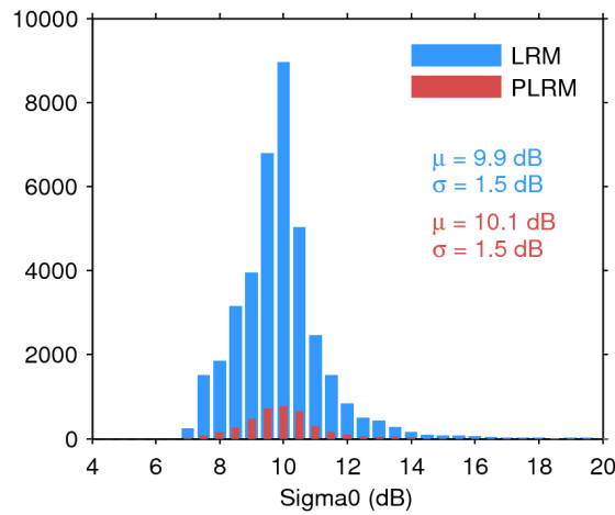
Figure 28. Histogram of science-valid sigma0 over oceans and lakes for LRM (blue) and PLRM (red) for 23/10/2017. The mean ( \mu ) and standard deviation ( \sigma ) are also shown. Note that values outside [4 20] dB are excluded from the histogram for the sake of readability but not from the computation of \mu and \sigma .
