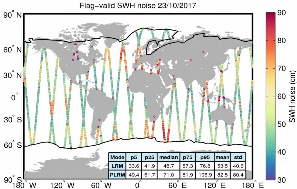
Figure 18. Geographical distribution of flag-valid 20-Hz SWH measurement noise over oceans and lakes for 23/10/2017. The statistical values shown in the table refer to the SWH noise and are calculated separately for LRM and PLRM regions. Measurements taken over polar polygons have been excluded from the computation of the statistical values. The black lines mark the outer limit of the Arctic and Antarctic polar polygons.
