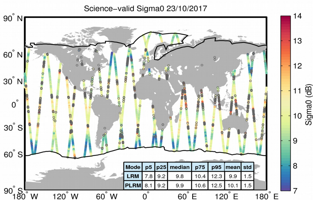
Figure 27. Geographical distribution of science-valid sigma0 data over oceans and lakes for 23/10/2017. The statistical values shown in the table refer to the sigma0 in dB and are calculated separately for LRM and PLRM regions. The black lines mark the outer limit of the Arctic and Antarctic polar polygons. Gray circles denote records that have been rejected based on the editing criteria described in Table 4.
