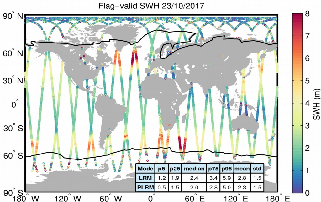
Figure 15. Geographical distribution of flag-valid SWH data over oceans and lakes for 23/10/2017. The statistical values shown in the table refer to the SWH in m and are calculated separately for LRM and PLRM regions. Measurements taken over polar polygons have been excluded from the computation of the statistical values. The black lines mark the outer limit of the Arctic and Antarctic polar polygons.
