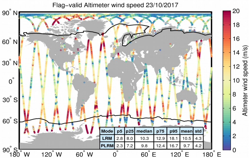
Figure 31. Geographical distribution of flag-valid wind data over oceans and lakes for 23/10/2017. The statistical values shown in the table refer to the wind in m/s and are calculated separately for LRM and PLRM regions. Measurements taken over polar polygons have been excluded from the computation of the statistical values. The black lines mark the outer limit of the Arctic and Antarctic polar polygons.
