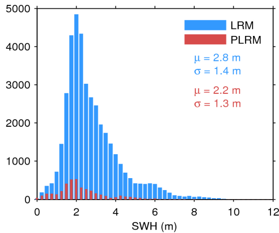
Figure 20. Histogram of science-valid SWH over oceans and lakes for LRM (blue) and PLRM (red) for 23/10/2017. The mean ( \mu ) and standard deviation ( \sigma ) are also shown. Note that values larger than 12 m are excluded from the histogram for the sake of readability but not from the computation of \mu and \sigma .
