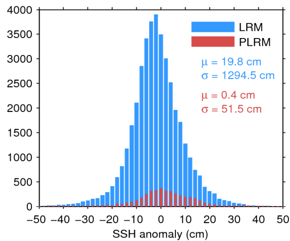
Figure 7. Histogram of flag-valid SSH anomaly over oceans and lakes for LRM (blue) and PLRM (red) for 23/10/2017. The mean ( \mu ) and standard deviation ( \sigma ) are also shown. Note that values outside [-50 50] cm are excluded from the histogram for the sake of readability but not from the computation of \mu and \sigma .
