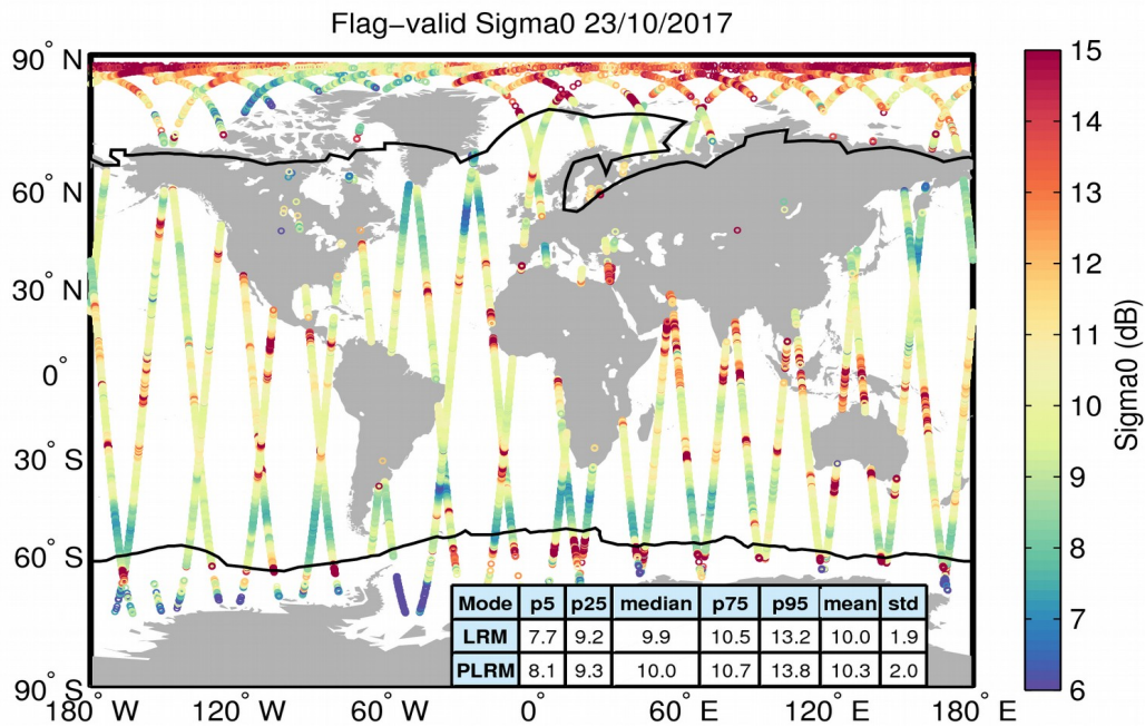
Figure 23. Geographical distribution of flag-valid sigma0 data over oceans and lakes for 23/10/2017. The statistical values shown in the table refer to the sigma0 in dB and are calculated separately for LRM and PLRM regions. Measurements taken over polar polygons have been excluded from the computation of the statistical values. The black lines mark the outer limit of the Arctic and Antarctic polar polygons.
