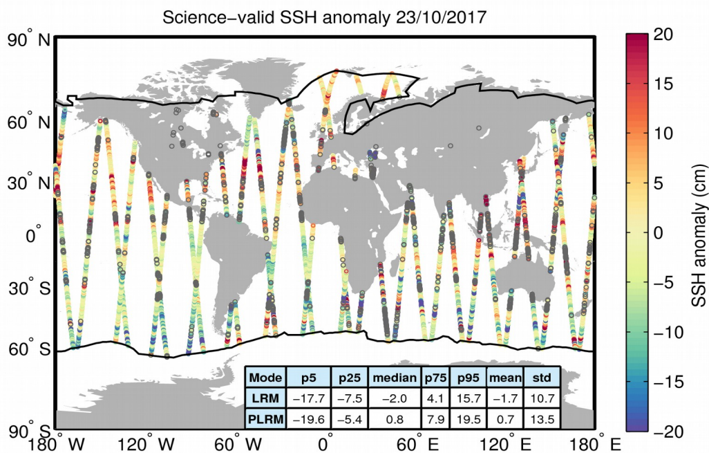
Figure 10. Geographical distribution of science-valid SSH anomaly data over oceans and lakes for 23/10/2017. The statistical values shown in the table refer to the SSH anomaly in cm and are calculated separately for LRM and PLRM regions. The black lines mark the outer limit of the Arctic and Antarctic polar polygons. Gray circles denote records that have been rejected based on the editing criteria described in Table 2.
