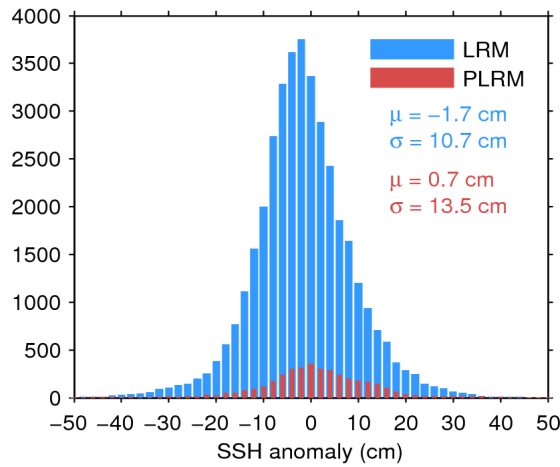
Figure 11. Histogram of science-valid SSH anomaly over oceans and lakes for LRM (blue) and PLRM (red) for 23/10/2017. The mean ( \mu ) and standard deviation ( \sigma ) are also shown. Note that values outside [-50\ 50] cm are excluded from the histogram for the sake of readability but not from the computation of \mu and \sigma .
