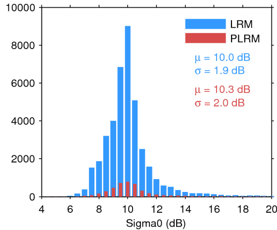
Figure 25. Histogram of flag-valid sigma0 over oceans and lakes for LRM (blue) and PLRM (red) for 23/10/2017. The mean ( \mu ) and standard deviation ( \sigma ) are also shown. Note that values outside [4 20] dB are excluded from the histogram for the sake of readability but not from the computation of \mu and \sigma .
