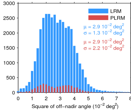
Figure 39. Histogram of flag-valid mispointing over oceans and lakes for LRM (blue) and PLRM (red) for 23/10/2017. Only positive values have been considered. The mean ( \mu ) and standard deviation ( \sigma ) are also shown. Note that values larger than 8 \cdot 10^{-2} \text{ deg}^2 are excluded from the histogram for the sake of readability but not from the computation of \mu and \sigma .
