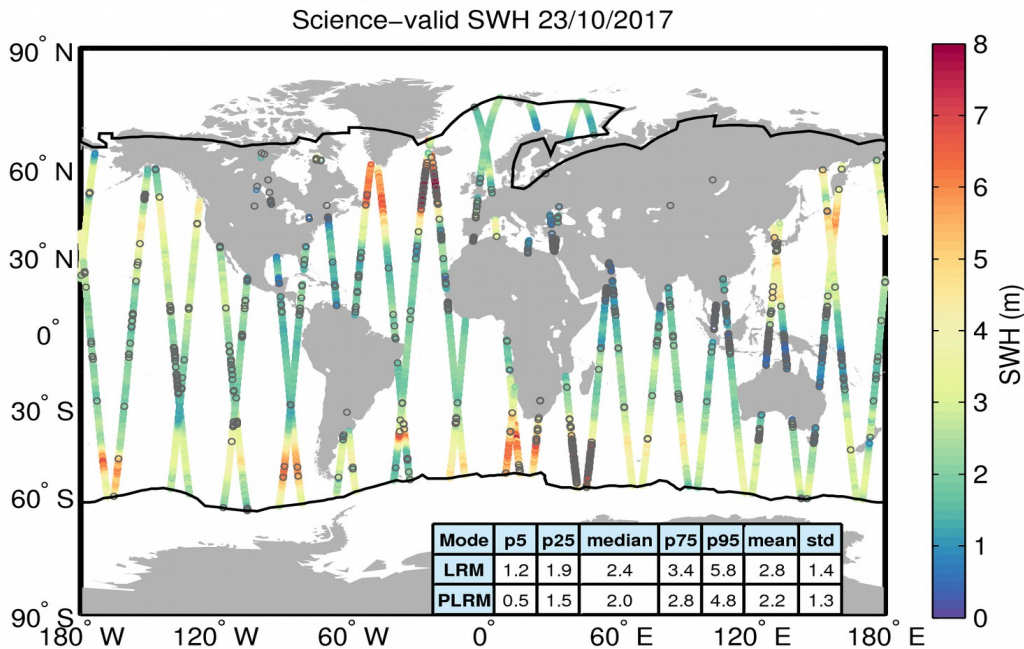
Figure 19. Geographical distribution of science-valid SWH data over oceans and lakes for 23/10/2017. The statistical values shown in the table refer to the SWH in m and are calculated separately for LRM and PLRM regions. The black lines mark the outer limit of the Arctic and Antarctic polar polygons. Gray circles denote records that have been rejected based on the editing criteria described in Table 3.
