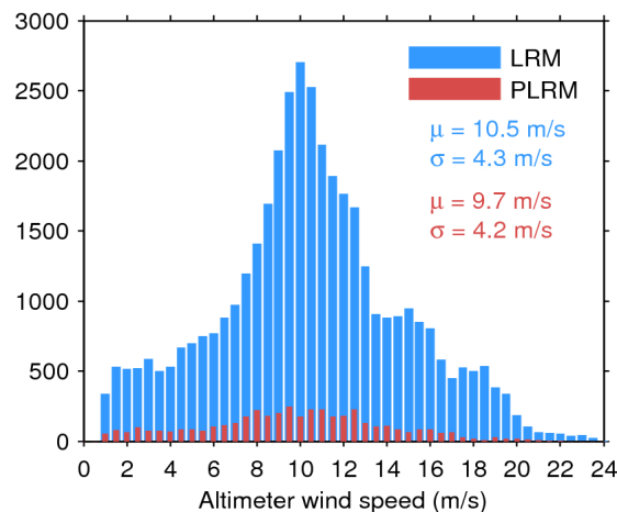
Figure 35. Histogram of science-valid wind over oceans and lakes for LRM (blue) and PLRM (red) for 23/10/2017. The mean ( \mu ) and standard deviation ( \sigma ) are also shown. Note that values larger than 24 m/s are excluded from the histogram for the sake of readability but not from the computation of \mu and \sigma .
