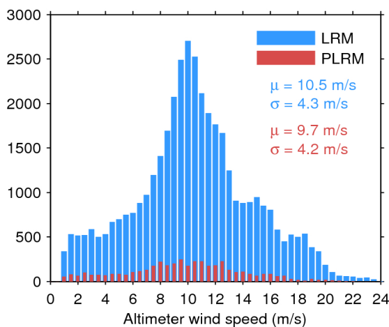
Figure 33. Histogram of flag-valid wind over oceans and lakes for LRM (blue) and PLRM (red) for 23/10/2017. The mean ( \mu ) and standard deviation ( \sigma ) are also shown. Note that values larger than 24 m/s are excluded from the histogram for the sake of readability but not from the computation of \mu and \sigma .
