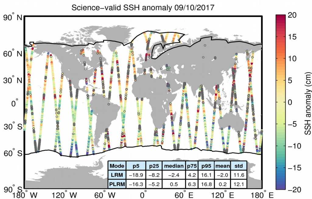
Figure 10. Geographical distribution of science-valid SSH anomaly data over oceans and lakes for 09/10/2017. The statistical values shown in the table refer to the SSH anomaly in cm and are calculated separately for LRM and PLRM regions. The black lines mark the outer limit of the Arctic and Antarctic polar polygons. Gray circles denote records that have been rejected based on the editing criteria described in Table 2.
