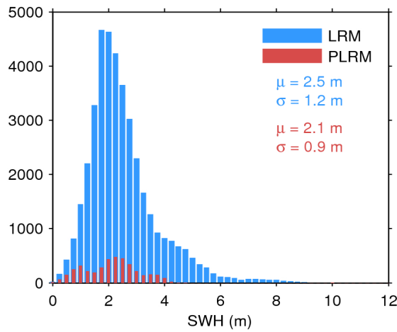
Figure 20. Histogram of science-valid SWH over oceans and lakes for LRM (blue) and PLRM (red) for 09/10/2017. The mean ( \mu ) and standard deviation ( \sigma ) are also shown. Note that values larger than 12 m are excluded from the histogram for the sake of readability but not from the computation of \mu and \sigma .
