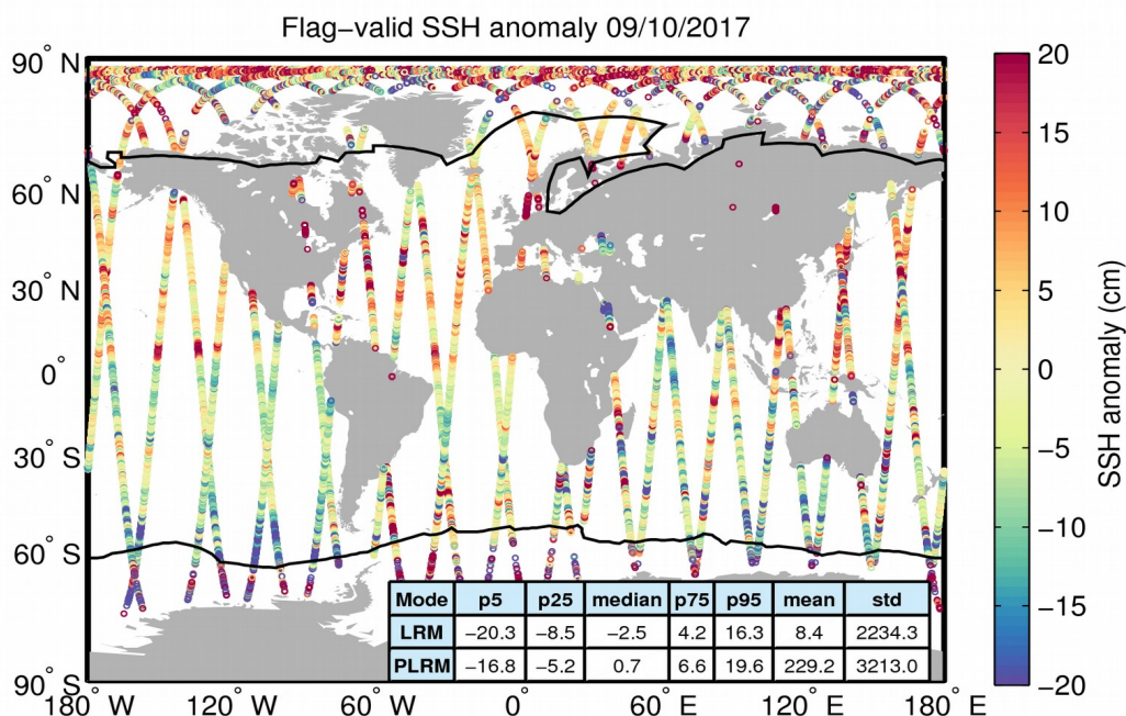
Figure 5. Geographical distribution of flag-valid 1-Hz SSH anomaly data over oceans and lakes for 09/10/2017. The statistical values shown in the table refer to the SSH anomaly in cm and are calculated separately for LRM and PLRM regions. Measurements taken over polar polygons have been excluded from the computation of the statistical values. The black lines mark the outer limit of the Arctic and Antarctic polar polygons.
