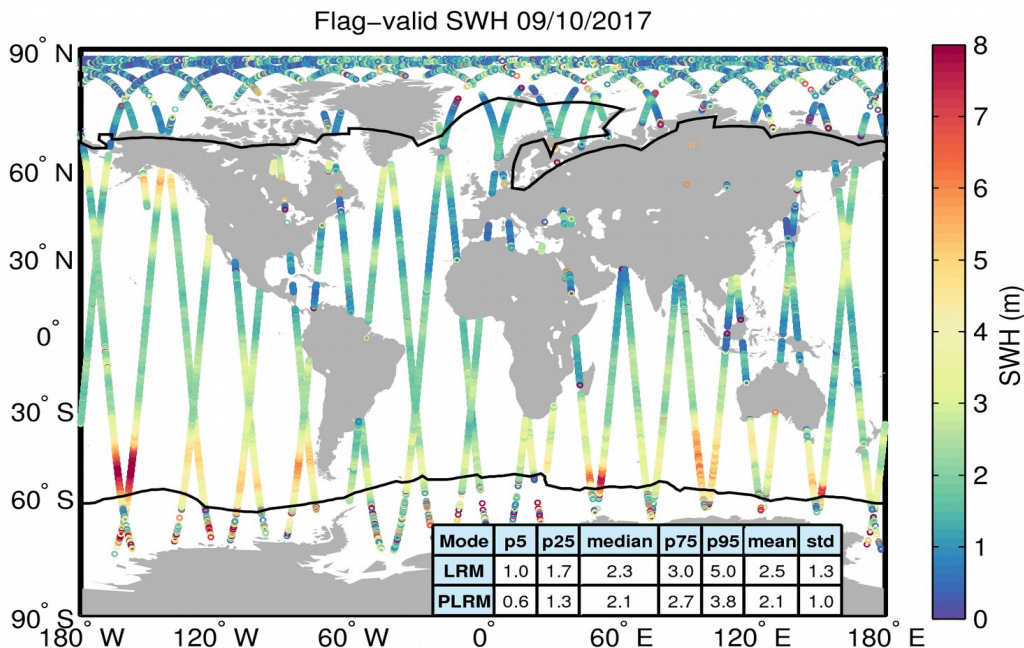
Figure 15. Geographical distribution of flag-valid SWH data over oceans and lakes for 09/10/2017. The statistical values shown in the table refer to the SWH in m and are calculated separately for LRM and PLRM regions. Measurements taken over polar polygons have been excluded from the computation of the statistical values. The black lines mark the outer limit of the Arctic and Antarctic polar polygons.
