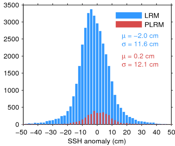
Figure 11. Histogram of science-valid SSH anomaly over oceans and lakes for LRM (blue) and PLRM (red) for 09/10/2017. The mean ( \mu ) and standard deviation ( \sigma ) are also shown. Note that values outside [-50\ 50] cm are excluded from the histogram for the sake of readability but not from the computation of \mu and \sigma .
