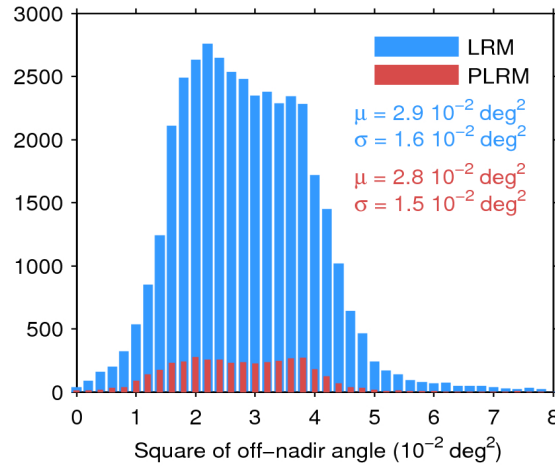
Figure 39. Histogram of flag-valid mispointing over oceans and lakes for LRM (blue) and PLRM (red) for 09/10/2017. Only positive values have been considered. The mean ( \mu ) and standard deviation ( \sigma ) are also shown. Note that values larger than 8 \cdot 10^{-2} \text{ deg}^2 are excluded from the histogram for the sake of readability but not from the computation of \mu and \sigma .
