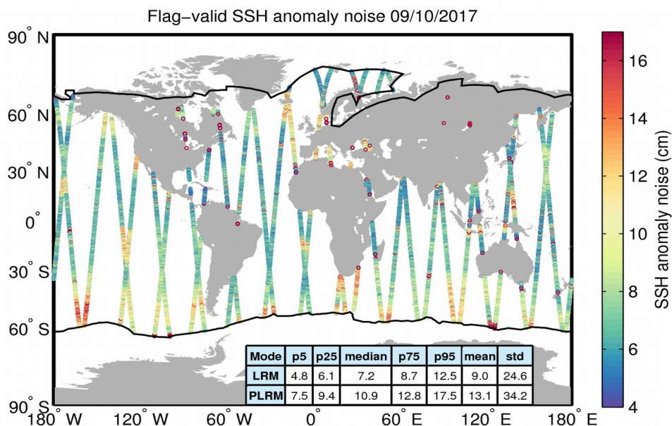
Figure 8. Geographical distribution of flag-valid 20-Hz SSH anomaly measurement noise over oceans and lakes for 09/10/2017. The statistical values shown in the table refer to the SSH anomaly noise and are calculated separately for LRM and PLRM regions. Measurements taken over polar polygons have been excluded from the computation of the statistical values. The black lines mark the outer limit of the Arctic and Antarctic polar polygons.
