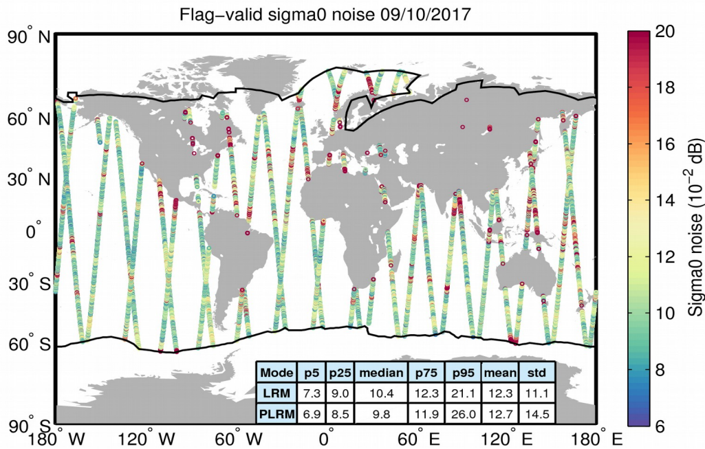
Figure 26. Geographical distribution of flag-valid 20-Hz sigma0 measurement noise over oceans and lakes for 09/10/2017. The statistical values shown in the table refer to the sigma0 noise and are calculated separately for LRM and PLRM regions. Measurements taken over polar polygons have been excluded from the computation of the statistical values. The black lines mark the outer limit of the Arctic and Antarctic polar polygons.
