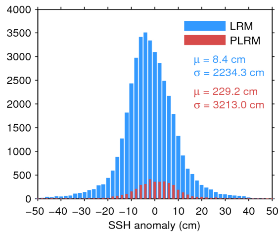
Figure 7. Histogram of flag-valid SSH anomaly over oceans and lakes for LRM (blue) and PLRM (red) for 09/10/2017. The mean ( \mu ) and standard deviation ( \sigma ) are also shown. Note that values outside [-50 \ 50] cm are excluded from the histogram for the sake of readability but not from the computation of \mu and \sigma .
