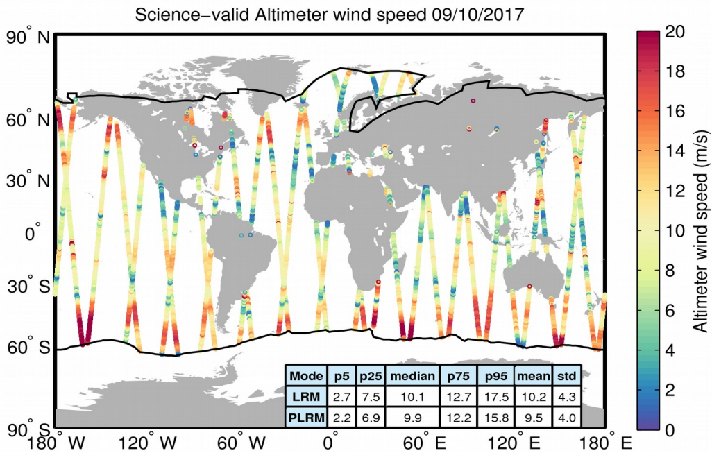
Figure 34. Geographical distribution of science-valid wind data over oceans and lakes for 09/10/2017. The statistical values shown in the table refer to the wind in m/s and are calculated separately for LRM and PLRM regions. The black lines mark the outer limit of the Arctic and Antarctic polar polygons. Gray circles denote records that have been rejected based on the editing criteria described in Table 5.
