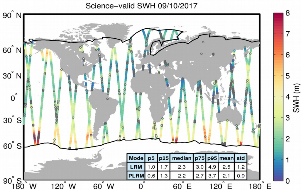
Figure 19. Geographical distribution of science-valid SWH data over oceans and lakes for 09/10/2017. The statistical values shown in the table refer to the SWH in m and are calculated separately for LRM and PLRM regions. The black lines mark the outer limit of the Arctic and Antarctic polar polygons. Gray circles denote records that have been rejected based on the editing criteria described in Table 3.
