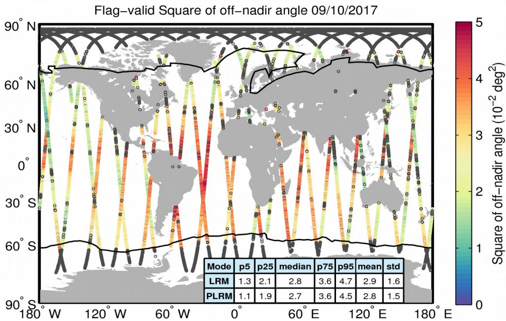
Figure 37. Geographical distribution of flag-valid mispointing data over oceans and lakes for 09/10/2017. The statistical values shown in the table refer to the mispointing in 10^{-2} deg 2 and are calculated separately for LRM and PLRM regions. Measurements taken over polar polygons have been excluded from the computation of the statistical values. The black lines mark the outer limit of the Arctic and Antarctic polar polygons. Gray circles denote negative values.
