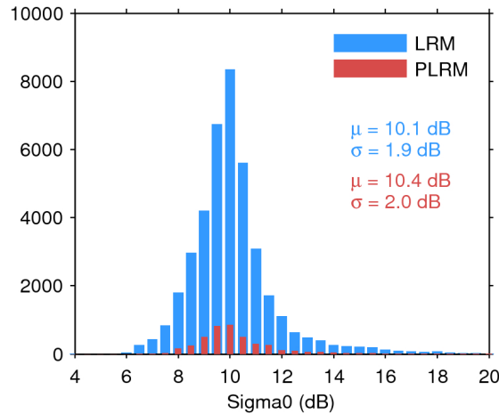
Figure 25. Histogram of flag-valid sigma0 over oceans and lakes for LRM (blue) and PLRM (red) for 09/10/2017. The mean ( \mu ) and standard deviation ( \sigma ) are also shown. Note that values outside [4 20] dB are excluded from the histogram for the sake of readability but not from the computation of \mu and \sigma .
