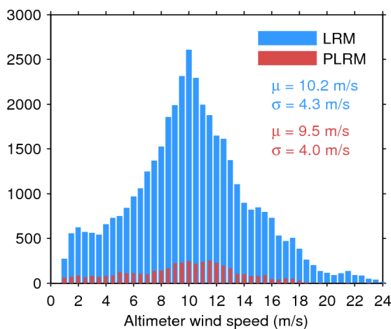
Figure 33. Histogram of flag-valid wind over oceans and lakes for LRM (blue) and PLRM (red) for 09/10/2017. The mean ( \mu ) and standard deviation ( \sigma ) are also shown. Note that values larger than 24 m/s are excluded from the histogram for the sake of readability but not from the computation of \mu and \sigma .
