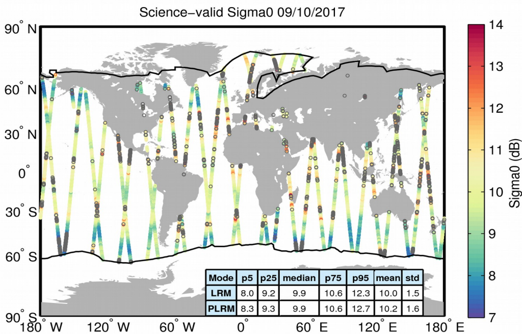
Figure 27. Geographical distribution of science-valid sigma0 data over oceans and lakes for 09/10/2017. The statistical values shown in the table refer to the sigma0 in dB and are calculated separately for LRM and PLRM regions. The black lines mark the outer limit of the Arctic and Antarctic polar polygons. Gray circles denote records that have been rejected based on the editing criteria described in Table 4.
