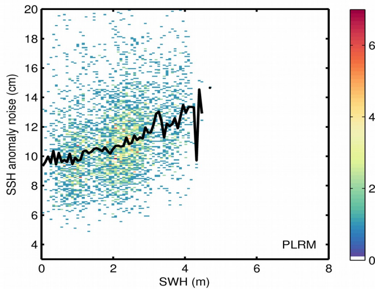
Figure 9. 2D histogram showing flag-valid SSH anomaly noise as a function of SWH for LRM (top) and PLRM (bottom) for 09/10/2017. The black line denotes the median SSH anomaly noise as a function of SWH.
