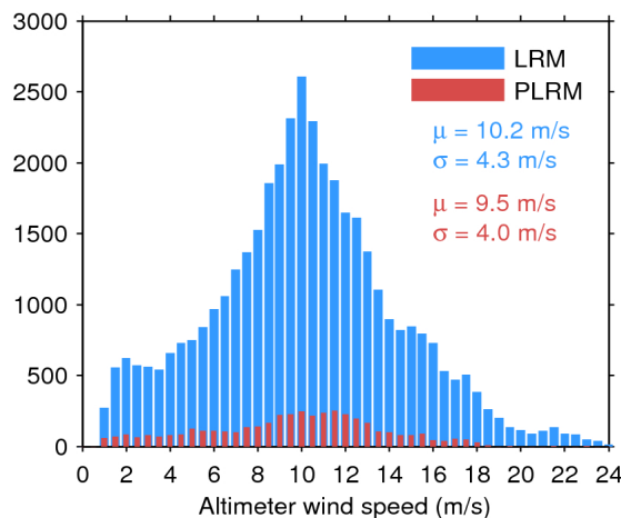
Figure 35. Histogram of science-valid wind over oceans and lakes for LRM (blue) and PLRM (red) for 09/10/2017. The mean ( \mu ) and standard deviation ( \sigma ) are also shown. Note that values larger than 24 m/s are excluded from the histogram for the sake of readability but not from the computation of \mu and \sigma .
