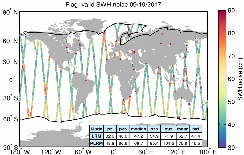
Figure 18. Geographical distribution of flag-valid 20-Hz SWH measurement noise over oceans and lakes for 09/10/2017. The statistical values shown in the table refer to the SWH noise and are calculated separately for LRM and PLRM regions. Measurements taken over polar polygons have been excluded from the computation of the statistical values. The black lines mark the outer limit of the Arctic and Antarctic polar polygons.
