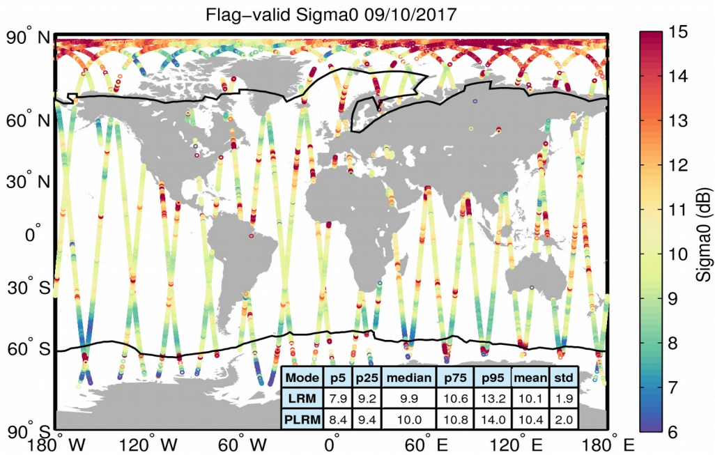
Figure 23. Geographical distribution of flag-valid sigma0 data over oceans and lakes for 09/10/2017. The statistical values shown in the table refer to the sigma0 in dB and are calculated separately for LRM and PLRM regions. Measurements taken over polar polygons have been excluded from the computation of the statistical values. The black lines mark the outer limit of the Arctic and Antarctic polar polygons.
