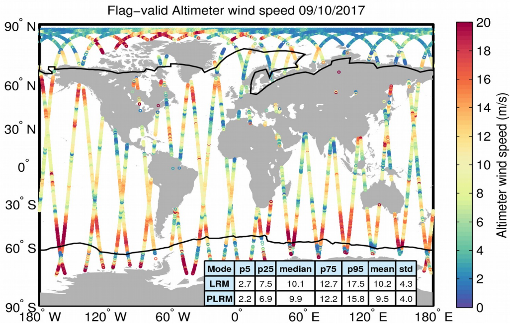
Figure 31. Geographical distribution of flag-valid wind data over oceans and lakes for 09/10/2017. The statistical values shown in the table refer to the wind in m/s and are calculated separately for LRM and PLRM regions. Measurements taken over polar polygons have been excluded from the computation of the statistical values. The black lines mark the outer limit of the Arctic and Antarctic polar polygons.
