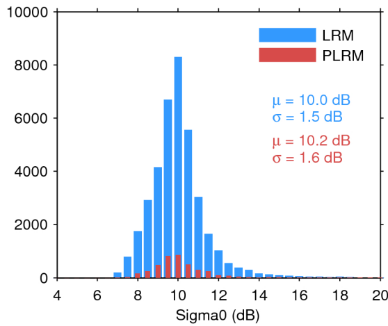
Figure 28. Histogram of science-valid sigma0 over oceans and lakes for LRM (blue) and PLRM (red) for 09/10/2017. The mean ( \mu ) and standard deviation ( \sigma ) are also shown. Note that values outside [4 20] dB are excluded from the histogram for the sake of readability but not from the computation of \mu and \sigma .
