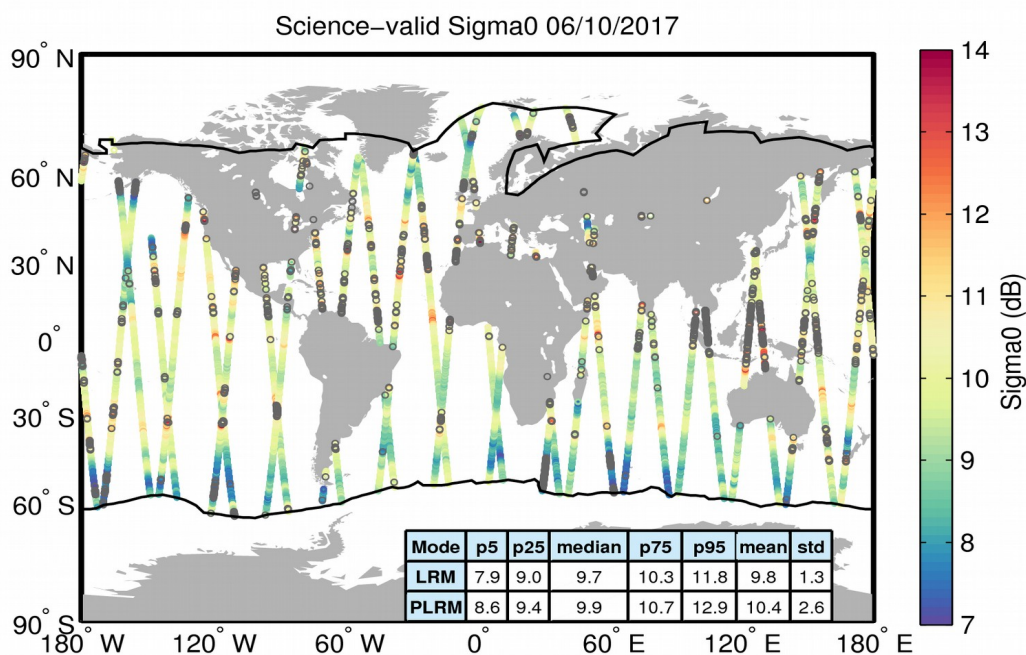
Figure 27. Geographical distribution of science-valid sigma0 data over oceans and lakes for 06/10/2017. The statistical values shown in the table refer to the sigma0 in dB and are calculated separately for LRM and PLRM regions. The black lines mark the outer limit of the Arctic and Antarctic polar polygons. Gray circles denote records that have been rejected based on the editing criteria described in Table 4.
