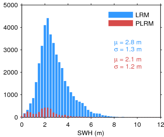
Figure 20. Histogram of science-valid SWH over oceans and lakes for LRM (blue) and PLRM (red) for 06/10/2017. The mean ( \mu ) and standard deviation ( \sigma ) are also shown. Note that values larger than 12 m are excluded from the histogram for the sake of readability but not from the computation of \mu and \sigma .
