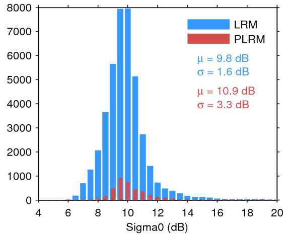
Figure 25. Histogram of flag-valid sigma0 over oceans and lakes for LRM (blue) and PLRM (red) for 06/10/2017. The mean ( \mu ) and standard deviation ( \sigma ) are also shown. Note that values outside [4 20] dB are excluded from the histogram for the sake of readability but not from the computation of \mu and \sigma .
