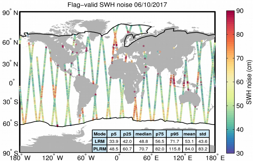
Figure 18. Geographical distribution of flag-valid 20-Hz SWH measurement noise over oceans and lakes for 06/10/2017. The statistical values shown in the table refer to the SWH noise and are calculated separately for LRM and PLRM regions. Measurements taken over polar polygons have been excluded from the computation of the statistical values. The black lines mark the outer limit of the Arctic and Antarctic polar polygons.
