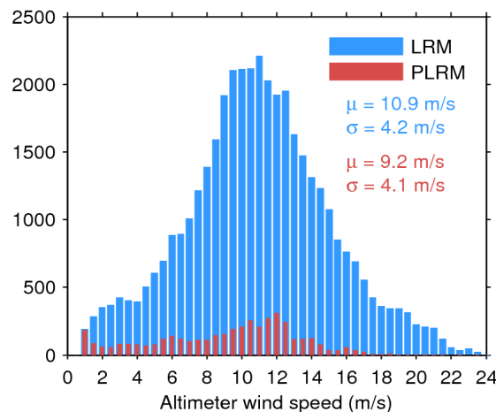
Figure 35. Histogram of science-valid wind over oceans and lakes for LRM (blue) and PLRM (red) for 06/10/2017. The mean ( \mu ) and standard deviation ( \sigma ) are also shown. Note that values larger than 24 m/s are excluded from the histogram for the sake of readability but not from the computation of \mu and \sigma .
