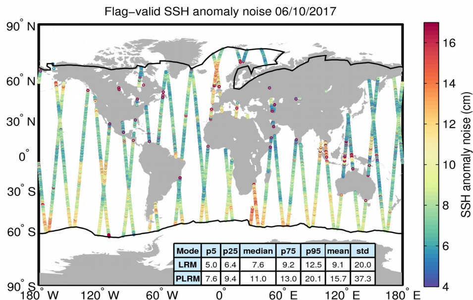
Figure 8. Geographical distribution of flag-valid 20-Hz SSH anomaly measurement noise over oceans and lakes for 06/10/2017. The statistical values shown in the table refer to the SSH anomaly noise and are calculated separately for LRM and PLRM regions. Measurements taken over polar polygons have been excluded from the computation of the statistical values. The black lines mark the outer limit of the Arctic and Antarctic polar polygons.
