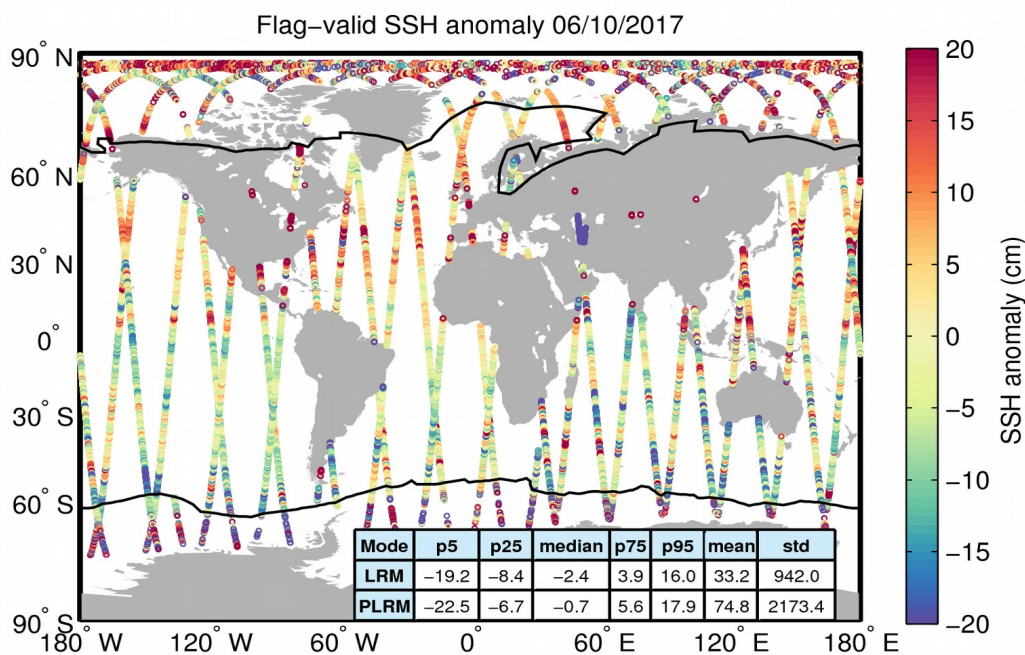
Figure 5. Geographical distribution of flag-valid 1-Hz SSH anomaly data over oceans and lakes for 06/10/2017. The statistical values shown in the table refer to the SSH anomaly in cm and are calculated separately for LRM and PLRM regions. Measurements taken over polar polygons have been excluded from the computation of the statistical values. The black lines mark the outer limit of the Arctic and Antarctic polar polygons.
