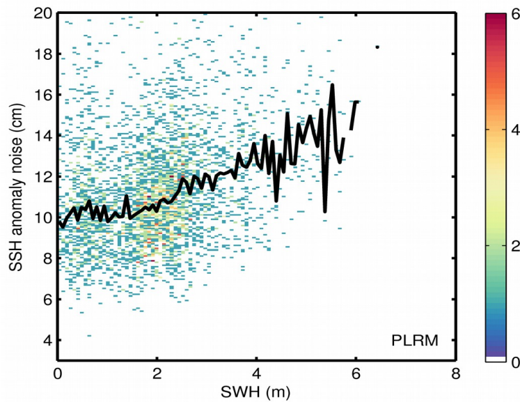
Figure 9. 2D histogram showing flag-valid SSH anomaly noise as a function of SWH for LRM (top) and PLRM (bottom) for 06/10/2017. The black line denotes the median SSH anomaly noise as a function of SWH.
