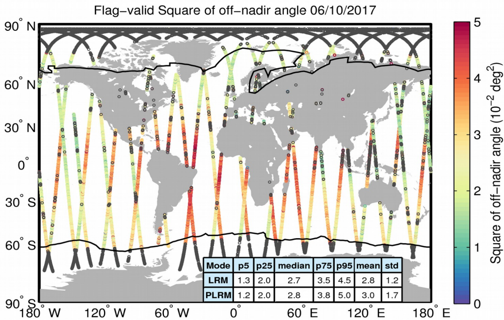
Figure 37. Geographical distribution of flag-valid mispointing data over oceans and lakes for 06/10/2017. The statistical values shown in the table refer to the mispointing in 10^{-2} deg 2 and are calculated separately for LRM and PLRM regions. Measurements taken over polar polygons have been excluded from the computation of the statistical values. The black lines mark the outer limit of the Arctic and Antarctic polar polygons. Gray circles denote negative values.
