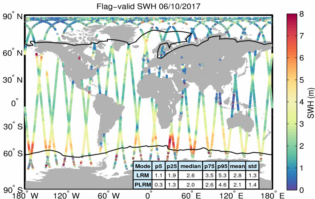
Figure 15. Geographical distribution of flag-valid SWH data over oceans and lakes for 06/10/2017. The statistical values shown in the table refer to the SWH in m and are calculated separately for LRM and PLRM regions. Measurements taken over polar polygons have been excluded from the computation of the statistical values. The black lines mark the outer limit of the Arctic and Antarctic polar polygons.
