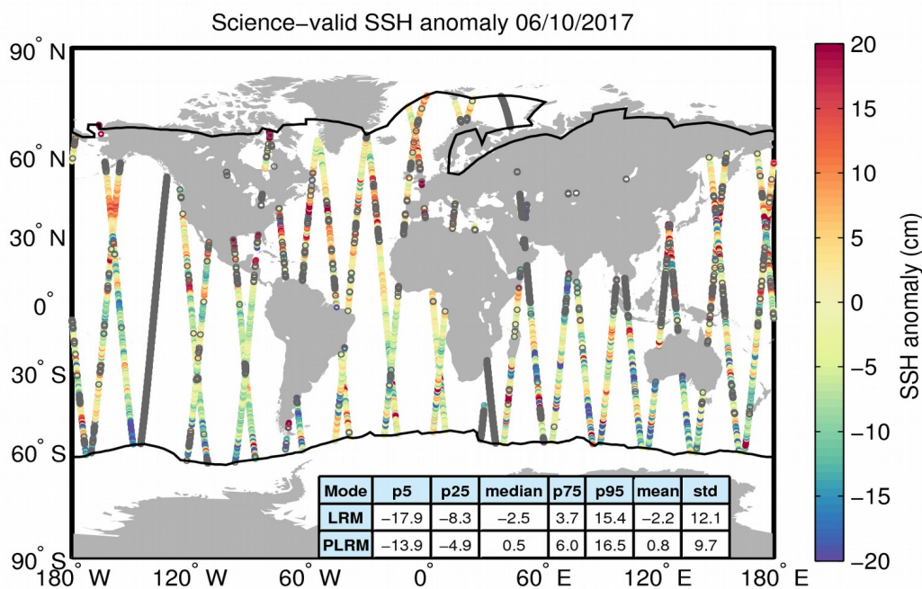
Figure 10. Geographical distribution of science-valid SSH anomaly data over oceans and lakes for 06/10/2017. The statistical values shown in the table refer to the SSH anomaly in cm and are calculated separately for LRM and PLRM regions. The black lines mark the outer limit of the Arctic and Antarctic polar polygons. Gray circles denote records that have been rejected based on the editing criteria described in Table 2.
