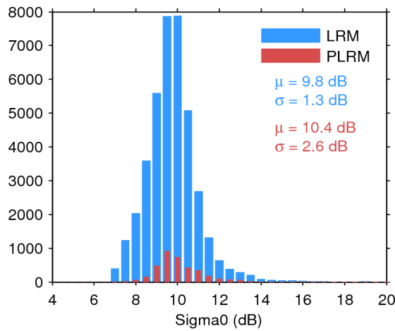
Figure 28. Histogram of science-valid sigma0 over oceans and lakes for LRM (blue) and PLRM (red) for 06/10/2017. The mean ( \mu ) and standard deviation ( \sigma ) are also shown. Note that values outside [4 20] dB are excluded from the histogram for the sake of readability but not from the computation of \mu and \sigma .
