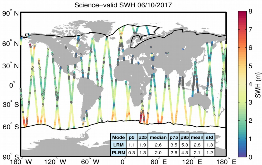
Figure 19. Geographical distribution of science-valid SWH data over oceans and lakes for 06/10/2017. The statistical values shown in the table refer to the SWH in m and are calculated separately for LRM and PLRM regions. The black lines mark the outer limit of the Arctic and Antarctic polar polygons. Gray circles denote records that have been rejected based on the editing criteria described in Table 3.
