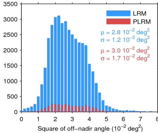
Figure 39. Histogram of flag-valid mispointing over oceans and lakes for LRM (blue) and PLRM (red) for 06/10/2017. Only positive values have been considered. The mean ( \mu ) and standard deviation ( \sigma ) are also shown. Note that values larger than 8 \cdot 10^{-2} \text{ deg}^2 are excluded from the histogram for the sake of readability but not from the computation of \mu and \sigma .
