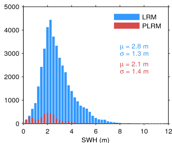
Figure 17. Histogram of flag-valid SWH over oceans and lakes for LRM (blue) and PLRM (red) for 06/10/2017. The mean ( \mu ) and standard deviation ( \sigma ) are also shown. Note that values larger than 12 m are excluded from the histogram for the sake of readability but not from the computation of \mu and \sigma .
