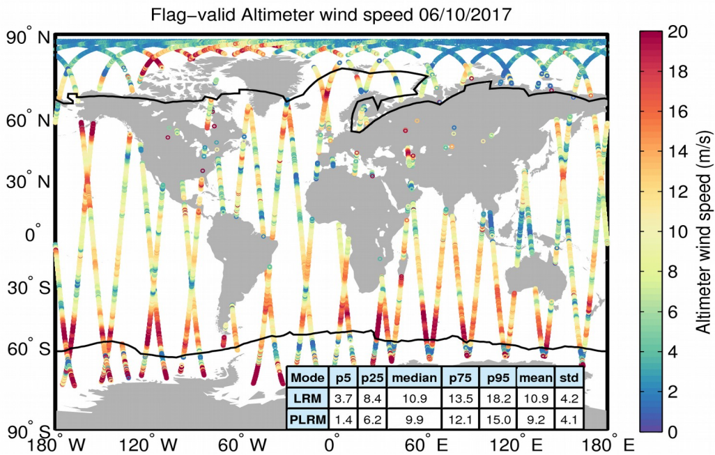
Figure 31. Geographical distribution of flag-valid wind data over oceans and lakes for 06/10/2017. The statistical values shown in the table refer to the wind in m/s and are calculated separately for LRM and PLRM regions. Measurements taken over polar polygons have been excluded from the computation of the statistical values. The black lines mark the outer limit of the Arctic and Antarctic polar polygons.
