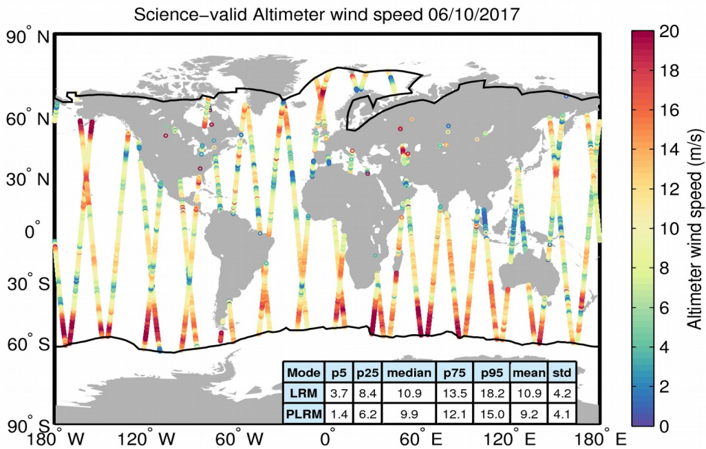
Figure 34. Geographical distribution of science-valid wind data over oceans and lakes for 06/10/2017. The statistical values shown in the table refer to the wind in m/s and are calculated separately for LRM and PLRM regions. The black lines mark the outer limit of the Arctic and Antarctic polar polygons. Gray circles denote records that have been rejected based on the editing criteria described in Table 5.
