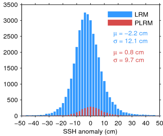
Figure 11. Histogram of science-valid SSH anomaly over oceans and lakes for LRM (blue) and PLRM (red) for 06/10/2017. The mean ( \mu ) and standard deviation ( \sigma ) are also shown. Note that values outside [-50\ 50] cm are excluded from the histogram for the sake of readability but not from the computation of \mu and \sigma .
