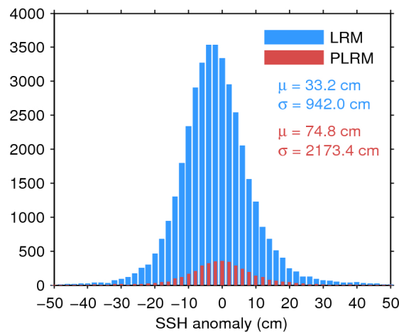
Figure 7. Histogram of flag-valid SSH anomaly over oceans and lakes for LRM (blue) and PLRM (red) for 06/10/2017. The mean ( \mu ) and standard deviation ( \sigma ) are also shown. Note that values outside [-50\ 50] cm are excluded from the histogram for the sake of readability but not from the computation of \mu and \sigma .
