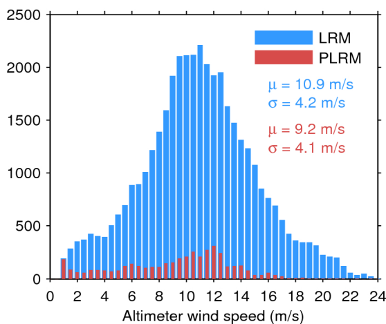
Figure 33. Histogram of flag-valid wind over oceans and lakes for LRM (blue) and PLRM (red) for 06/10/2017. The mean ( \mu ) and standard deviation ( \sigma ) are also shown. Note that values larger than 24 m/s are excluded from the histogram for the sake of readability but not from the computation of \mu and \sigma .
