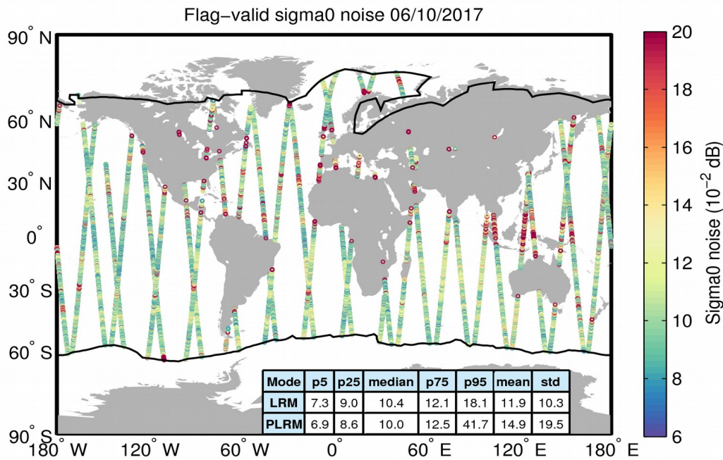
Figure 26. Geographical distribution of flag-valid 20-Hz sigma0 measurement noise over oceans and lakes for 06/10/2017. The statistical values shown in the table refer to the sigma0 noise and are calculated separately for LRM and PLRM regions. Measurements taken over polar polygons have been excluded from the computation of the statistical values. The black lines mark the outer limit of the Arctic and Antarctic polar polygons.
