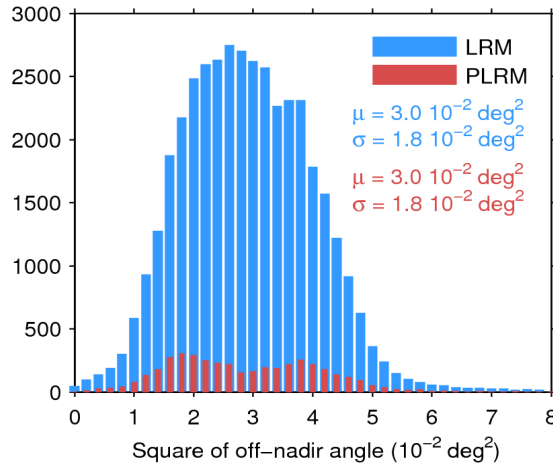
Figure 39. Histogram of flag-valid mispointing over oceans and lakes for LRM (blue) and PLRM (red) for 02/10/2017. Only positive values have been considered. The mean ( \mu ) and standard deviation ( \sigma ) are also shown. Note that values larger than 8 \cdot 10^{-2} \text{ deg}^2 are excluded from the histogram for the sake of readability but not from the computation of \mu and \sigma .
