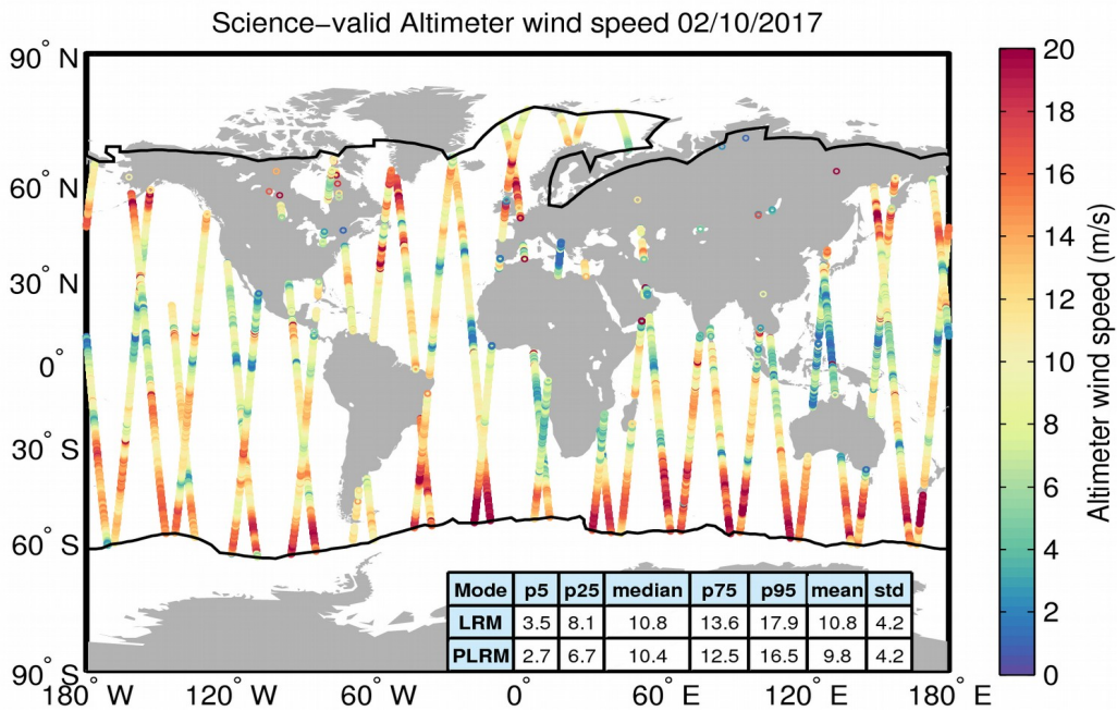
Figure 34. Geographical distribution of science-valid wind data over oceans and lakes for 02/10/2017. The statistical values shown in the table refer to the wind in m/s and are calculated separately for LRM and PLRM regions. The black lines mark the outer limit of the Arctic and Antarctic polar polygons. Gray circles denote records that have been rejected based on the editing criteria described in Table 5.
