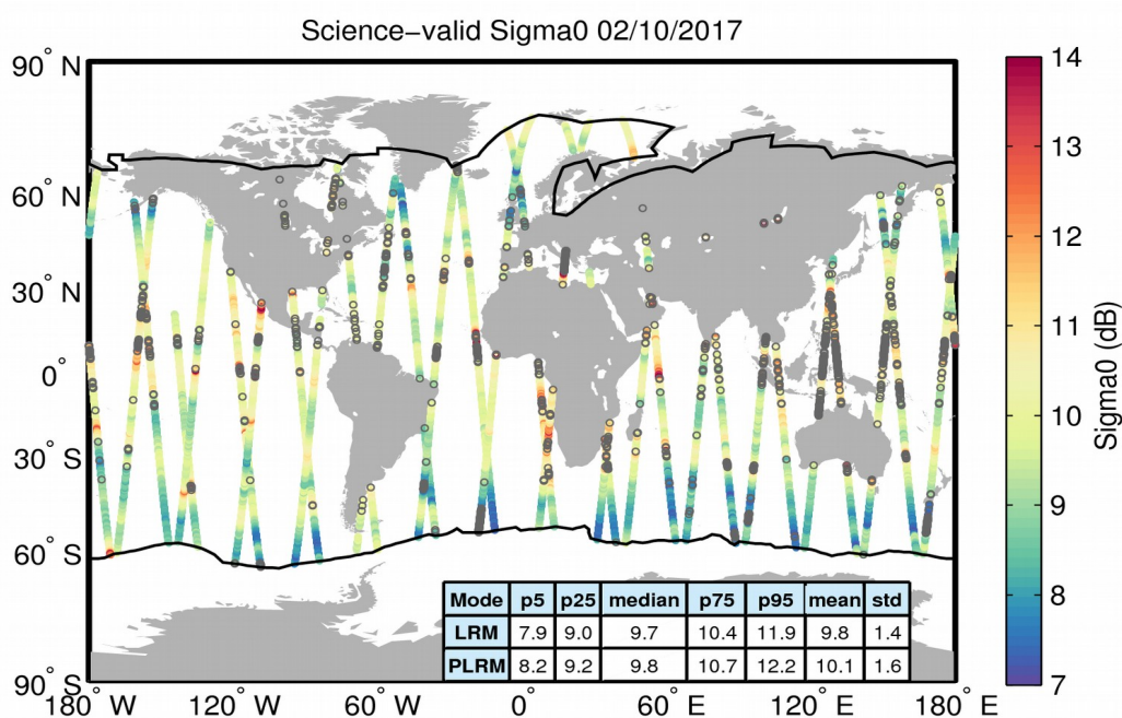
Figure 27. Geographical distribution of science-valid sigma0 data over oceans and lakes for 02/10/2017. The statistical values shown in the table refer to the sigma0 in dB and are calculated separately for LRM and PLRM regions. The black lines mark the outer limit of the Arctic and Antarctic polar polygons. Gray circles denote records that have been rejected based on the editing criteria described in Table 4.
