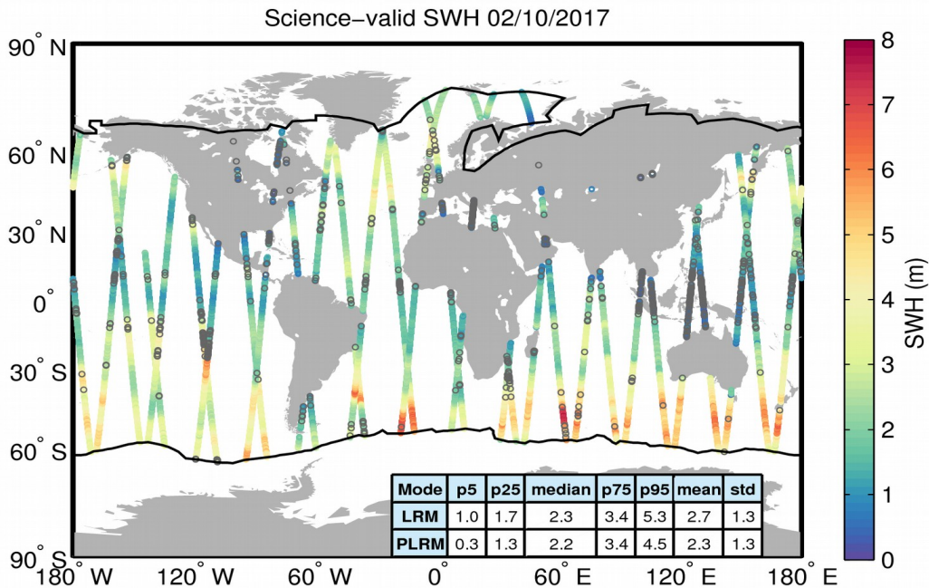
Figure 19. Geographical distribution of science-valid SWH data over oceans and lakes for 02/10/2017. The statistical values shown in the table refer to the SWH in m and are calculated separately for LRM and PLRM regions. The black lines mark the outer limit of the Arctic and Antarctic polar polygons. Gray circles denote records that have been rejected based on the editing criteria described in Table 3.
