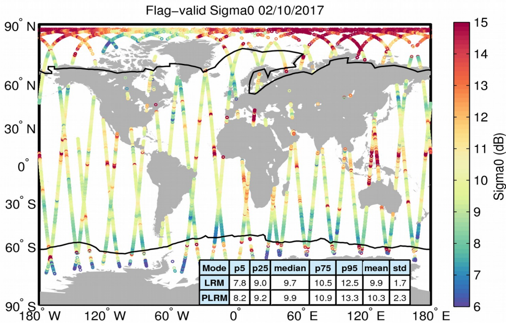
Figure 23. Geographical distribution of flag-valid sigma0 data over oceans and lakes for 02/10/2017. The statistical values shown in the table refer to the sigma0 in dB and are calculated separately for LRM and PLRM regions. Measurements taken over polar polygons have been excluded from the computation of the statistical values. The black lines mark the outer limit of the Arctic and Antarctic polar polygons.
