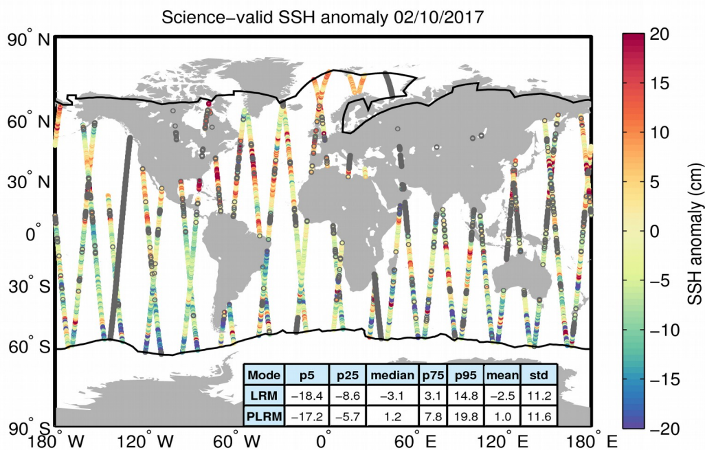
Figure 10. Geographical distribution of science-valid SSH anomaly data over oceans and lakes for 02/10/2017. The statistical values shown in the table refer to the SSH anomaly in cm and are calculated separately for LRM and PLRM regions. The black lines mark the outer limit of the Arctic and Antarctic polar polygons. Gray circles denote records that have been rejected based on the editing criteria described in Table 2.
