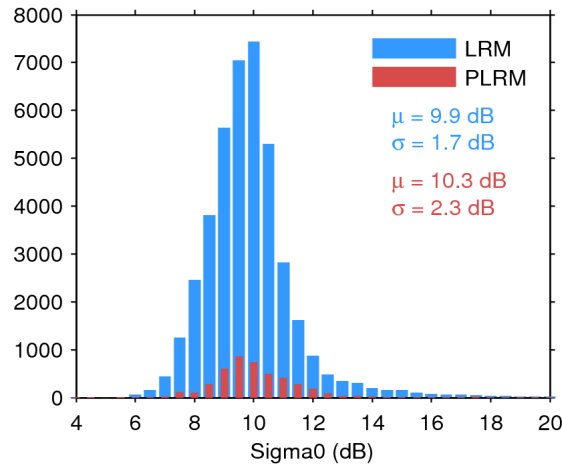
Figure 25. Histogram of flag-valid sigma0 over oceans and lakes for LRM (blue) and PLRM (red) for 02/10/2017. The mean ( \mu ) and standard deviation ( \sigma ) are also shown. Note that values outside [4 20] dB are excluded from the histogram for the sake of readability but not from the computation of \mu and \sigma .
