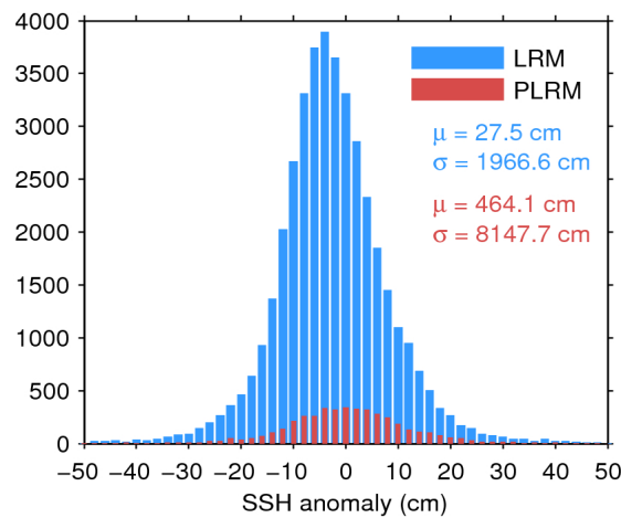
Figure 7. Histogram of flag-valid SSH anomaly over oceans and lakes for LRM (blue) and PLRM (red) for 02/10/2017. The mean ( \mu ) and standard deviation ( \sigma ) are also shown. Note that values outside [-50 50] cm are excluded from the histogram for the sake of readability but not from the computation of \mu and \sigma .
