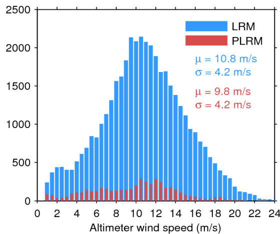
Figure 35. Histogram of science-valid wind over oceans and lakes for LRM (blue) and PLRM (red) for 02/10/2017. The mean ( \mu ) and standard deviation ( \sigma ) are also shown. Note that values larger than 24 m/s are excluded from the histogram for the sake of readability but not from the computation of \mu and \sigma .
