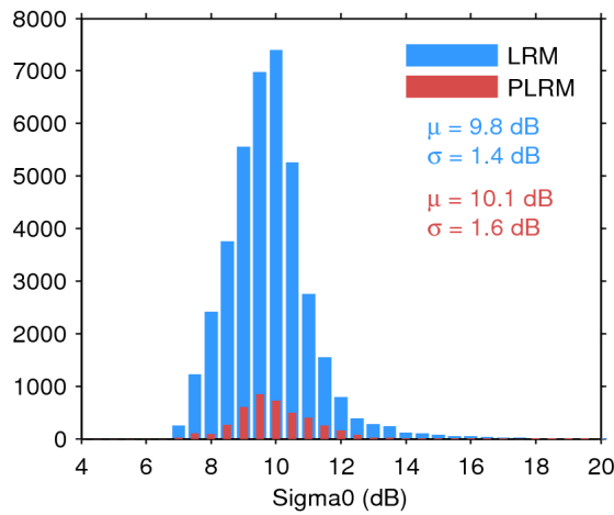
Figure 28. Histogram of science-valid sigma0 over oceans and lakes for LRM (blue) and PLRM (red) for 02/10/2017. The mean ( \mu ) and standard deviation ( \sigma ) are also shown. Note that values outside [4 20] dB are excluded from the histogram for the sake of readability but not from the computation of \mu and \sigma .
