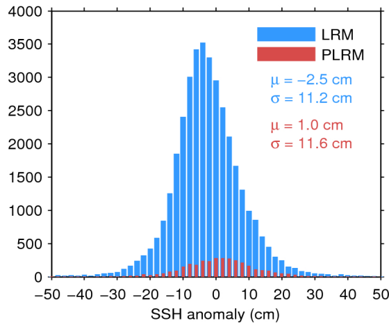
Figure 11. Histogram of science-valid SSH anomaly over oceans and lakes for LRM (blue) and PLRM (red) for 02/10/2017. The mean ( \mu ) and standard deviation ( \sigma ) are also shown. Note that values outside [-50 50] cm are excluded from the histogram for the sake of readability but not from the computation of \mu and \sigma .
