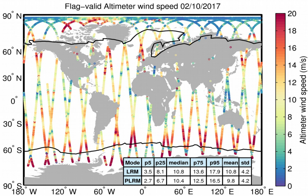
Figure 31. Geographical distribution of flag-valid wind data over oceans and lakes for 02/10/2017. The statistical values shown in the table refer to the wind in m/s and are calculated separately for LRM and PLRM regions. Measurements taken over polar polygons have been excluded from the computation of the statistical values. The black lines mark the outer limit of the Arctic and Antarctic polar polygons.
