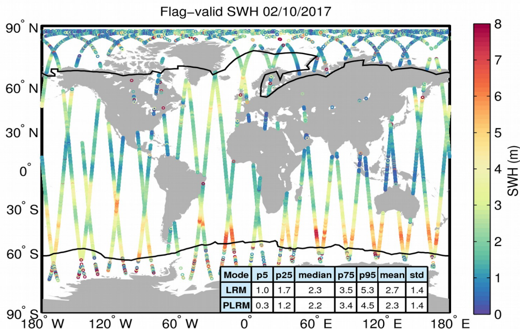
Figure 15. Geographical distribution of flag-valid SWH data over oceans and lakes for 02/10/2017. The statistical values shown in the table refer to the SWH in m and are calculated separately for LRM and PLRM regions. Measurements taken over polar polygons have been excluded from the computation of the statistical values. The black lines mark the outer limit of the Arctic and Antarctic polar polygons.
