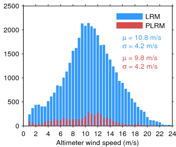
Figure 33. Histogram of flag-valid wind over oceans and lakes for LRM (blue) and PLRM (red) for 02/10/2017. The mean ( \mu ) and standard deviation ( \sigma ) are also shown. Note that values larger than 24 m/s are excluded from the histogram for the sake of readability but not from the computation of \mu and \sigma .
