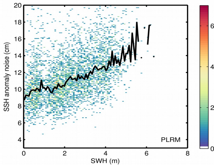
Figure 9. 2D histogram showing flag-valid SSH anomaly noise as a function of SWH for LRM (top) and PLRM (bottom) for 02/10/2017. The black line denotes the median SSH anomaly noise as a function of SWH.
