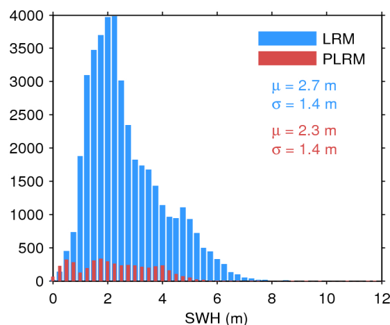
Figure 17. Histogram of flag-valid SWH over oceans and lakes for LRM (blue) and PLRM (red) for 02/10/2017. The mean ( \mu ) and standard deviation ( \sigma ) are also shown. Note that values larger than 12 m are excluded from the histogram for the sake of readability but not from the computation of \mu and \sigma .
