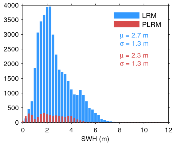
Figure 20. Histogram of science-valid SWH over oceans and lakes for LRM (blue) and PLRM (red) for 02/10/2017. The mean ( \mu ) and standard deviation ( \sigma ) are also shown. Note that values larger than 12 m are excluded from the histogram for the sake of readability but not from the computation of \mu and \sigma .
