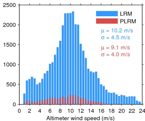
Figure 35. Histogram of science-valid wind over oceans and lakes for LRM (blue) and PLRM (red) for 26/09/2017. The mean ( \mu ) and standard deviation ( \sigma ) are also shown. Note that values larger than 24 m/s are excluded from the histogram for the sake of readability but not from the computation of \mu and \sigma .
