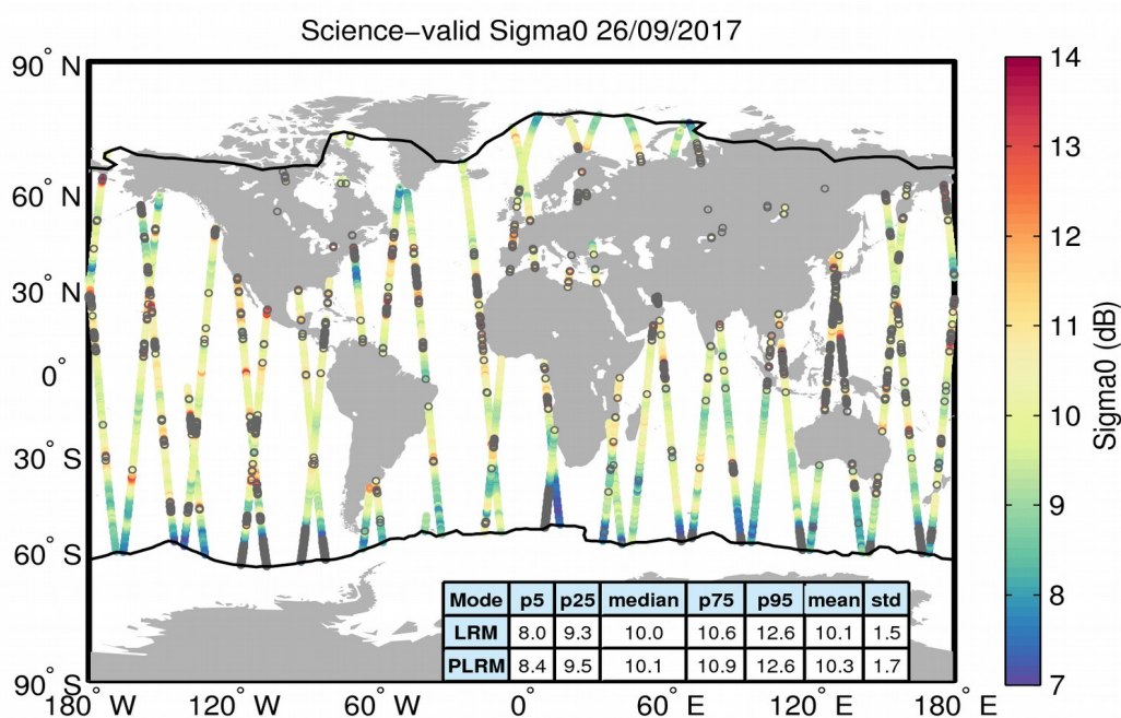
Figure 27. Geographical distribution of science-valid sigma0 data over oceans and lakes for 26/09/2017. The statistical values shown in the table refer to the sigma0 in dB and are calculated separately for LRM and PLRM regions. The black lines mark the outer limit of the Arctic and Antarctic polar polygons. Gray circles denote records that have been rejected based on the editing criteria described in Table 4.
