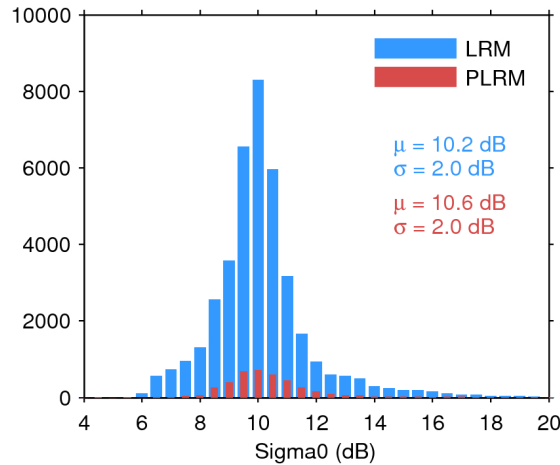
Figure 25. Histogram of flag-valid sigma0 over oceans and lakes for LRM (blue) and PLRM (red) for 26/09/2017. The mean ( \mu ) and standard deviation ( \sigma ) are also shown. Note that values outside [4 20] dB are excluded from the histogram for the sake of readability but not from the computation of \mu and \sigma .
