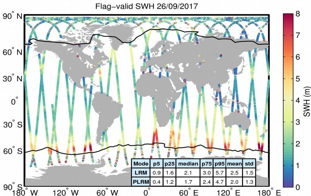
Figure 15. Geographical distribution of flag-valid SWH data over oceans and lakes for 26/09/2017. The statistical values shown in the table refer to the SWH in m and are calculated separately for LRM and PLRM regions. Measurements taken over polar polygons have been excluded from the computation of the statistical values. The black lines mark the outer limit of the Arctic and Antarctic polar polygons.
