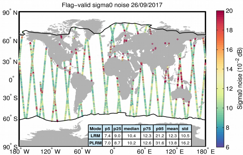
Figure 26. Geographical distribution of flag-valid 20-Hz sigma0 measurement noise over oceans and lakes for 26/09/2017. The statistical values shown in the table refer to the sigma0 noise and are calculated separately for LRM and PLRM regions. Measurements taken over polar polygons have been excluded from the computation of the statistical values. The black lines mark the outer limit of the Arctic and Antarctic polar polygons.
