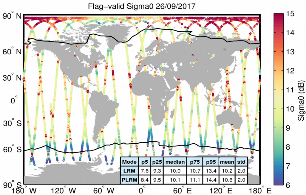
Figure 23. Geographical distribution of flag-valid sigma0 data over oceans and lakes for 26/09/2017. The statistical values shown in the table refer to the sigma0 in dB and are calculated separately for LRM and PLRM regions. Measurements taken over polar polygons have been excluded from the computation of the statistical values. The black lines mark the outer limit of the Arctic and Antarctic polar polygons.
