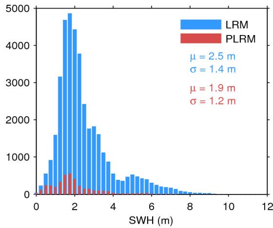
Figure 20. Histogram of science-valid SWH over oceans and lakes for LRM (blue) and PLRM (red) for 26/09/2017. The mean ( \mu ) and standard deviation ( \sigma ) are also shown. Note that values larger than 12 m are excluded from the histogram for the sake of readability but not from the computation of \mu and \sigma .
