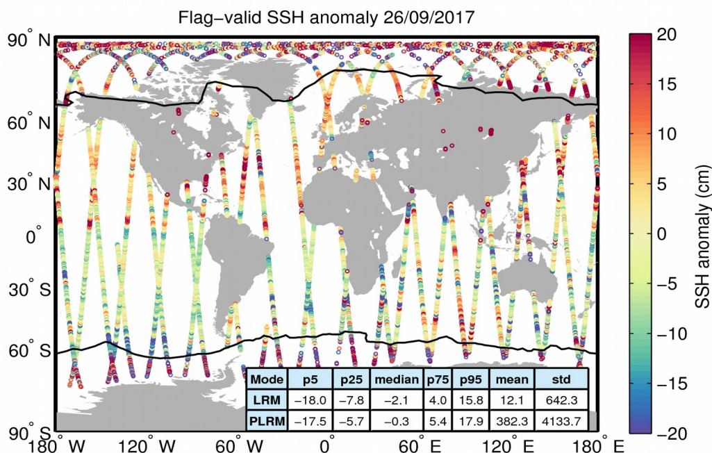
Figure 5. Geographical distribution of flag-valid 1-Hz SSH anomaly data over oceans and lakes for 26/09/2017. The statistical values shown in the table refer to the SSH anomaly in cm and are calculated separately for LRM and PLRM regions. Measurements taken over polar polygons have been excluded from the computation of the statistical values. The black lines mark the outer limit of the Arctic and Antarctic polar polygons.
