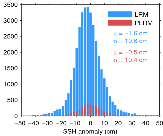
Figure 11. Histogram of science-valid SSH anomaly over oceans and lakes for LRM (blue) and PLRM (red) for 26/09/2017. The mean ( \mu ) and standard deviation ( \sigma ) are also shown. Note that values outside [-50\ 50] cm are excluded from the histogram for the sake of readability but not from the computation of \mu and \sigma .
