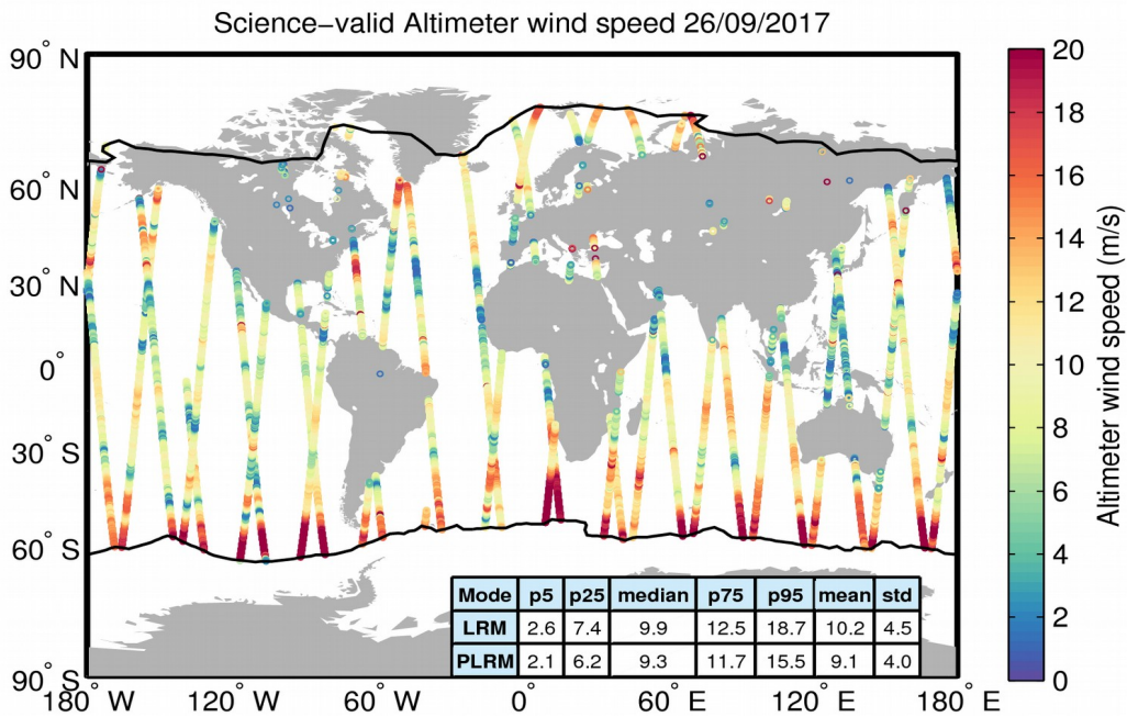
Figure 34. Geographical distribution of science-valid wind data over oceans and lakes for 26/09/2017. The statistical values shown in the table refer to the wind in m/s and are calculated separately for LRM and PLRM regions. The black lines mark the outer limit of the Arctic and Antarctic polar polygons. Gray circles denote records that have been rejected based on the editing criteria described in Table 5.
