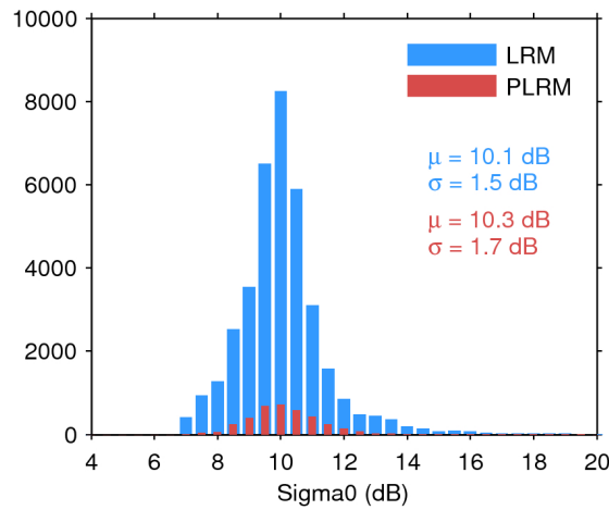
Figure 28. Histogram of science-valid sigma0 over oceans and lakes for LRM (blue) and PLRM (red) for 26/09/2017. The mean ( \mu ) and standard deviation ( \sigma ) are also shown. Note that values outside [4 20] dB are excluded from the histogram for the sake of readability but not from the computation of \mu and \sigma .
