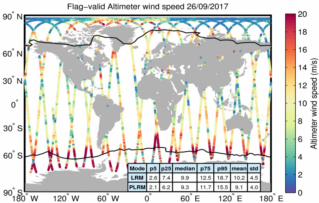
Figure 31. Geographical distribution of flag-valid wind data over oceans and lakes for 26/09/2017. The statistical values shown in the table refer to the wind in m/s and are calculated separately for LRM and PLRM regions. Measurements taken over polar polygons have been excluded from the computation of the statistical values. The black lines mark the outer limit of the Arctic and Antarctic polar polygons.
