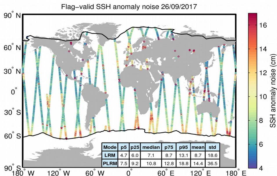
Figure 8. Geographical distribution of flag-valid 20-Hz SSH anomaly measurement noise over oceans and lakes for 26/09/2017. The statistical values shown in the table refer to the SSH anomaly noise and are calculated separately for LRM and PLRM regions. Measurements taken over polar polygons have been excluded from the computation of the statistical values. The black lines mark the outer limit of the Arctic and Antarctic polar polygons.
