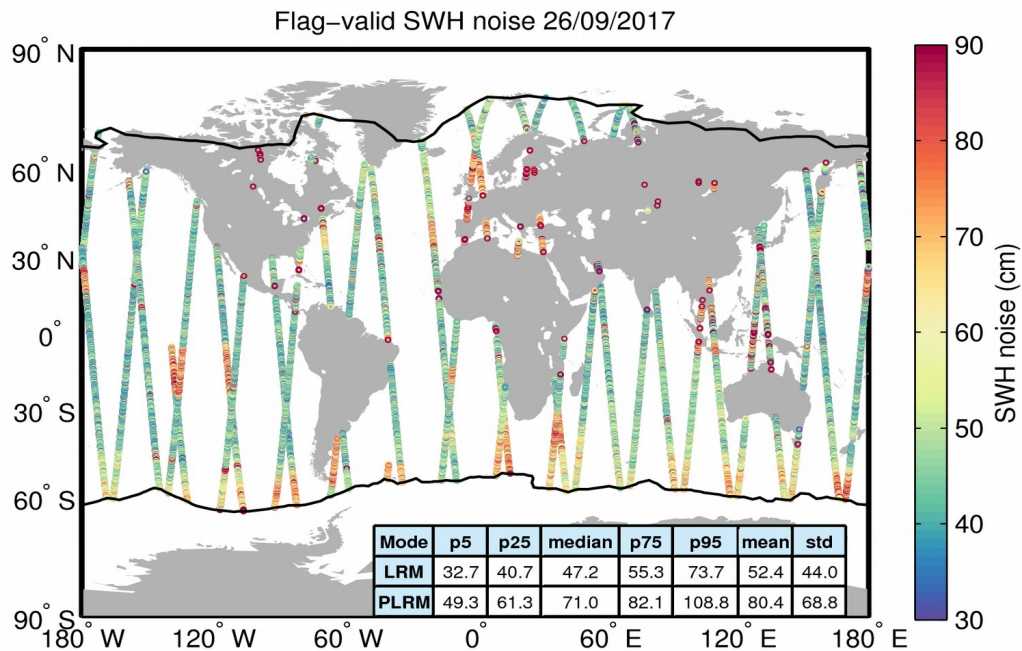
Figure 18. Geographical distribution of flag-valid 20-Hz SWH measurement noise over oceans and lakes for 26/09/2017. The statistical values shown in the table refer to the SWH noise and are calculated separately for LRM and PLRM regions. Measurements taken over polar polygons have been excluded from the computation of the statistical values. The black lines mark the outer limit of the Arctic and Antarctic polar polygons.
