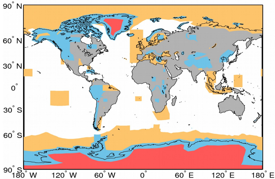
Figure A1. Extent of the regions defining the geographical mode mask for 26/09/2017. The regions where SAR, and SARIn are operated are denoted by the orange and blue polygons, respectively. LRM is operated over areas of the continental ice sheets (red polygons) and over oceans and land not covered by other modes.
