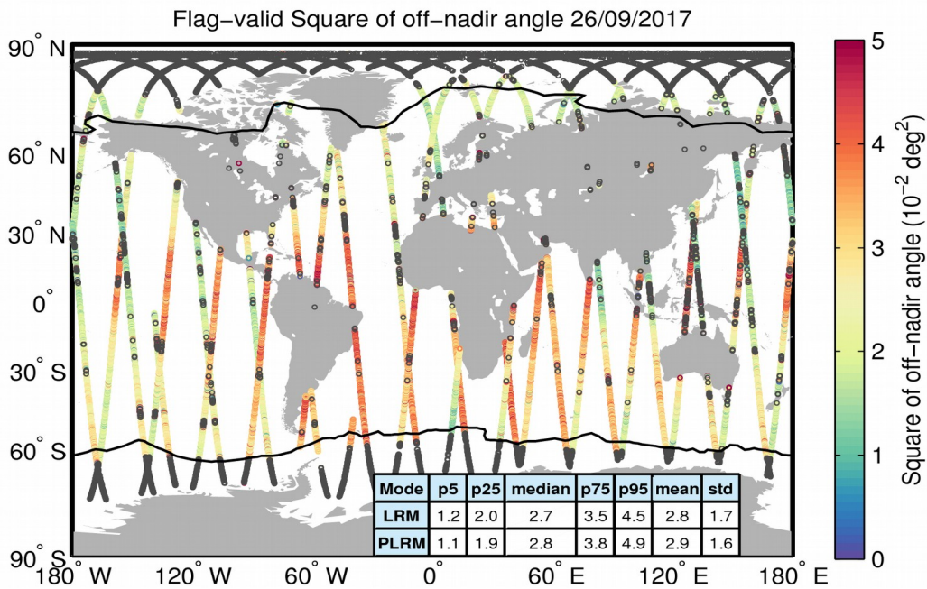
Figure 37. Geographical distribution of flag-valid mispointing data over oceans and lakes for 26/09/2017. The statistical values shown in the table refer to the mispointing in 10^{-2} deg 2 and are calculated separately for LRM and PLRM regions. Measurements taken over polar polygons have been excluded from the computation of the statistical values. The black lines mark the outer limit of the Arctic and Antarctic polar polygons. Gray circles denote negative values.
