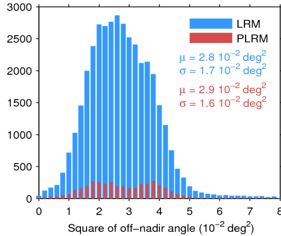
Figure 39. Histogram of flag-valid mispointing over oceans and lakes for LRM (blue) and PLRM (red) for 26/09/2017. Only positive values have been considered. The mean ( \mu ) and standard deviation ( \sigma ) are also shown. Note that values larger than 8 \cdot 10^{-2} \text{ deg}^2 are excluded from the histogram for the sake of readability but not from the computation of \mu and \sigma .
