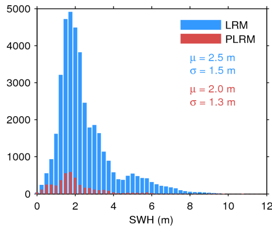
Figure 17. Histogram of flag-valid SWH over oceans and lakes for LRM (blue) and PLRM (red) for 26/09/2017. The mean ( \mu ) and standard deviation ( \sigma ) are also shown. Note that values larger than 12 m are excluded from the histogram for the sake of readability but not from the computation of \mu and \sigma .
