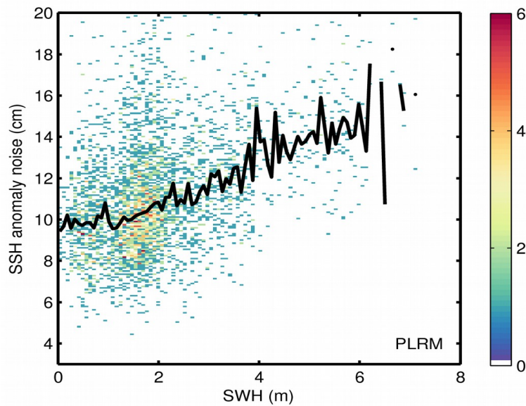
Figure 9. 2D histogram showing flag-valid SSH anomaly noise as a function of SWH for LRM (top) and PLRM (bottom) for 26/09/2017. The black line denotes the median SSH anomaly noise as a function of SWH.
