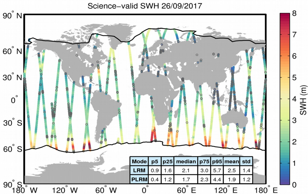
Figure 19. Geographical distribution of science-valid SWH data over oceans and lakes for 26/09/2017. The statistical values shown in the table refer to the SWH in m and are calculated separately for LRM and PLRM regions. The black lines mark the outer limit of the Arctic and Antarctic polar polygons. Gray circles denote records that have been rejected based on the editing criteria described in Table 3.
