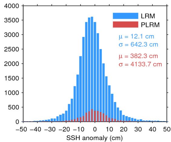
Figure 7. Histogram of flag-valid SSH anomaly over oceans and lakes for LRM (blue) and PLRM (red) for 26/09/2017. The mean ( \mu ) and standard deviation ( \sigma ) are also shown. Note that values outside [-50 \ 50] cm are excluded from the histogram for the sake of readability but not from the computation of \mu and \sigma .
