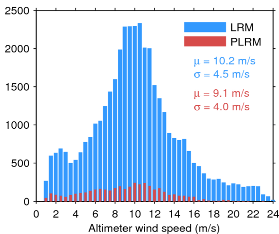
Figure 33. Histogram of flag-valid wind over oceans and lakes for LRM (blue) and PLRM (red) for 26/09/2017. The mean ( \mu ) and standard deviation ( \sigma ) are also shown. Note that values larger than 24 m/s are excluded from the histogram for the sake of readability but not from the computation of \mu and \sigma .
