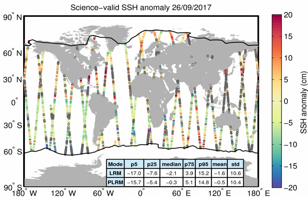
Figure 10. Geographical distribution of science-valid SSH anomaly data over oceans and lakes for 26/09/2017. The statistical values shown in the table refer to the SSH anomaly in cm and are calculated separately for LRM and PLRM regions. The black lines mark the outer limit of the Arctic and Antarctic polar polygons. Gray circles denote records that have been rejected based on the editing criteria described in Table 2.
