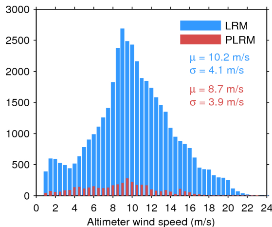
Figure 35. Histogram of science-valid wind over oceans and lakes for LRM (blue) and PLRM (red) for 24/09/2017. The mean ( \mu ) and standard deviation ( \sigma ) are also shown. Note that values larger than 24 m/s are excluded from the histogram for the sake of readability but not from the computation of \mu and \sigma .
