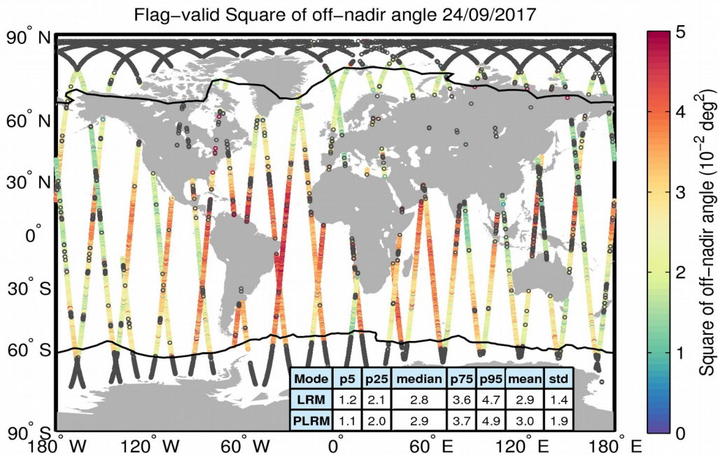
Figure 37. Geographical distribution of flag-valid mispointing data over oceans and lakes for 24/09/2017. The statistical values shown in the table refer to the mispointing in 10^{-2} deg 2 and are calculated separately for LRM and PLRM regions. Measurements taken over polar polygons have been excluded from the computation of the statistical values. The black lines mark the outer limit of the Arctic and Antarctic polar polygons. Gray circles denote negative values.
