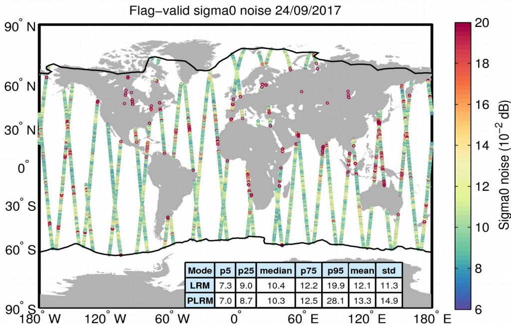
Figure 26. Geographical distribution of flag-valid 20-Hz sigma0 measurement noise over oceans and lakes for 24/09/2017. The statistical values shown in the table refer to the sigma0 noise and are calculated separately for LRM and PLRM regions. Measurements taken over polar polygons have been excluded from the computation of the statistical values. The black lines mark the outer limit of the Arctic and Antarctic polar polygons.
