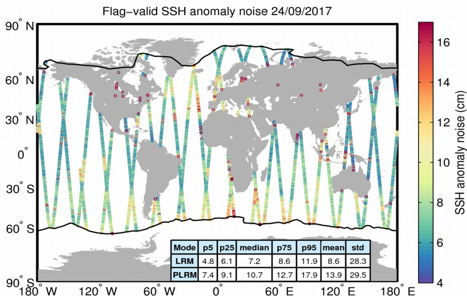
Figure 8. Geographical distribution of flag-valid 20-Hz SSH anomaly measurement noise over oceans and lakes for 24/09/2017. The statistical values shown in the table refer to the SSH anomaly noise and are calculated separately for LRM and PLRM regions. Measurements taken over polar polygons have been excluded from the computation of the statistical values. The black lines mark the outer limit of the Arctic and Antarctic polar polygons.
