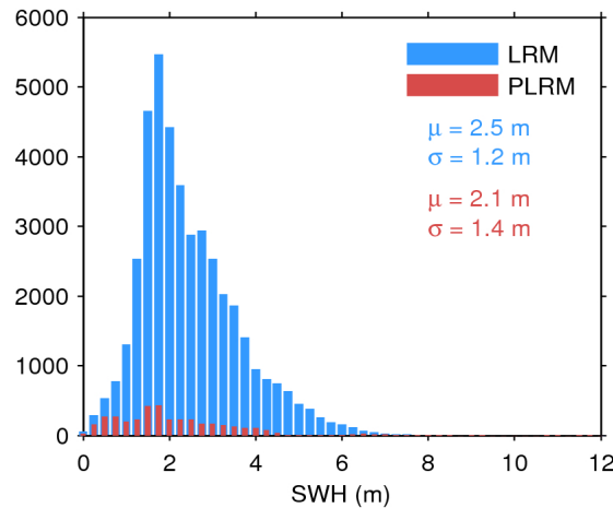
Figure 17. Histogram of flag-valid SWH over oceans and lakes for LRM (blue) and PLRM (red) for 24/09/2017. The mean ( \mu ) and standard deviation ( \sigma ) are also shown. Note that values larger than 12 m are excluded from the histogram for the sake of readability but not from the computation of \mu and \sigma .
