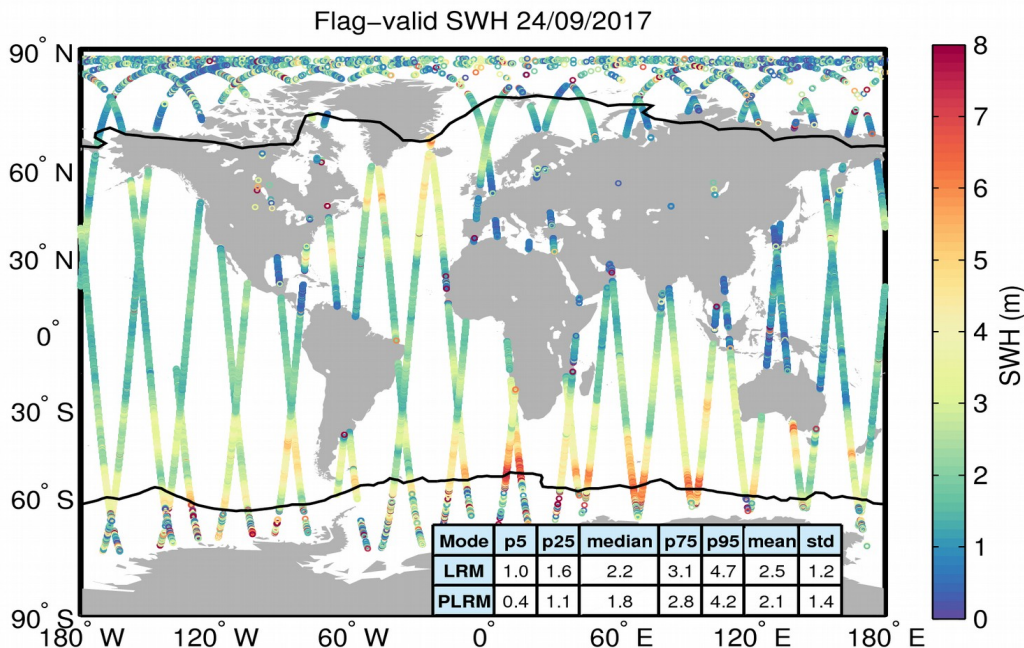
Figure 15. Geographical distribution of flag-valid SWH data over oceans and lakes for 24/09/2017. The statistical values shown in the table refer to the SWH in m and are calculated separately for LRM and PLRM regions. Measurements taken over polar polygons have been excluded from the computation of the statistical values. The black lines mark the outer limit of the Arctic and Antarctic polar polygons.
