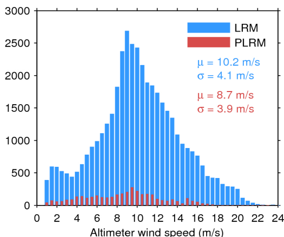
Figure 33. Histogram of flag-valid wind over oceans and lakes for LRM (blue) and PLRM (red) for 24/09/2017. The mean ( \mu ) and standard deviation ( \sigma ) are also shown. Note that values larger than 24 m/s are excluded from the histogram for the sake of readability but not from the computation of \mu and \sigma .
