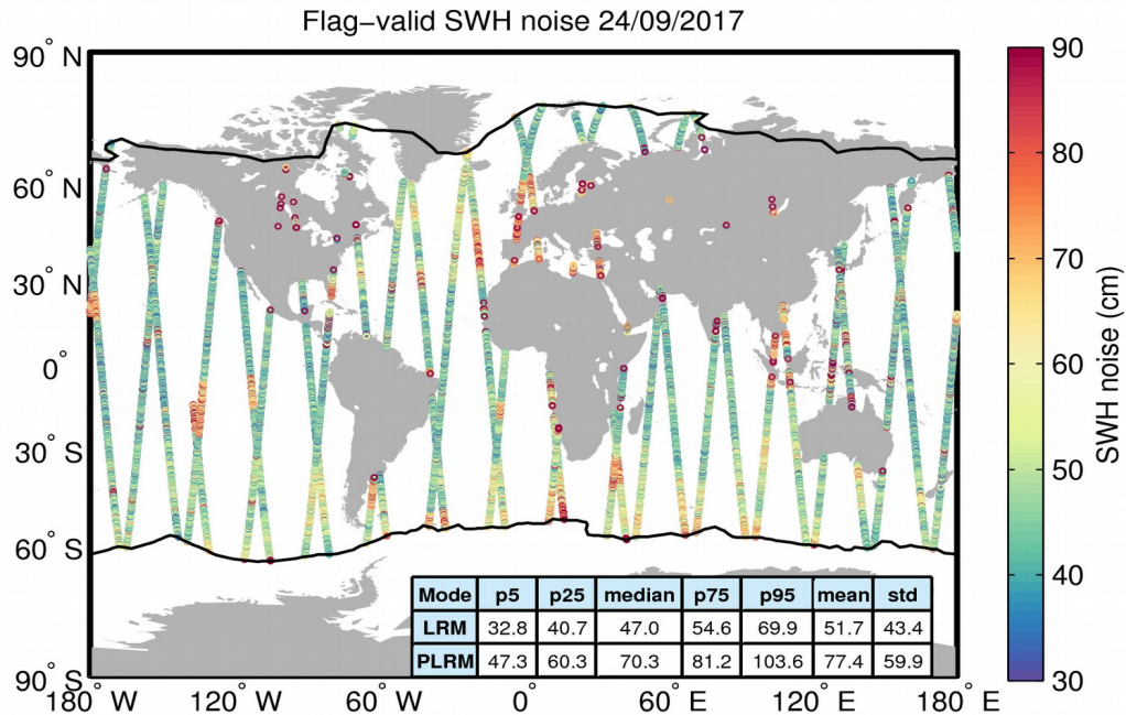
Figure 18. Geographical distribution of flag-valid 20-Hz SWH measurement noise over oceans and lakes for 24/09/2017. The statistical values shown in the table refer to the SWH noise and are calculated separately for LRM and PLRM regions. Measurements taken over polar polygons have been excluded from the computation of the statistical values. The black lines mark the outer limit of the Arctic and Antarctic polar polygons.
