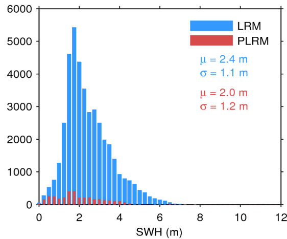
Figure 20. Histogram of science-valid SWH over oceans and lakes for LRM (blue) and PLRM (red) for 24/09/2017. The mean ( \mu ) and standard deviation ( \sigma ) are also shown. Note that values larger than 12 m are excluded from the histogram for the sake of readability but not from the computation of \mu and \sigma .
