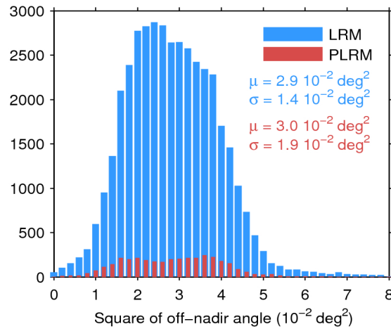
Figure 39. Histogram of flag-valid mispointing over oceans and lakes for LRM (blue) and PLRM (red) for 24/09/2017. Only positive values have been considered. The mean ( \mu ) and standard deviation ( \sigma ) are also shown. Note that values larger than 8 \cdot 10^{-2} \text{ deg}^2 are excluded from the histogram for the sake of readability but not from the computation of \mu and \sigma .
