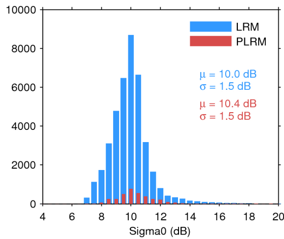
Figure 28. Histogram of science-valid sigma0 over oceans and lakes for LRM (blue) and PLRM (red) for 24/09/2017. The mean ( \mu ) and standard deviation ( \sigma ) are also shown. Note that values outside [4 20] dB are excluded from the histogram for the sake of readability but not from the computation of \mu and \sigma .
