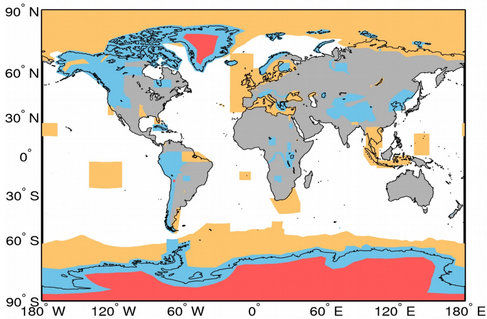
Figure A1. Extent of the regions defining the geographical mode mask for 24/09/2017. The regions where SAR, and SARIn are operated are denoted by the orange and blue polygons, respectively. LRM is operated over areas of the continental ice sheets (red polygons) and over oceans and land not covered by other modes.
