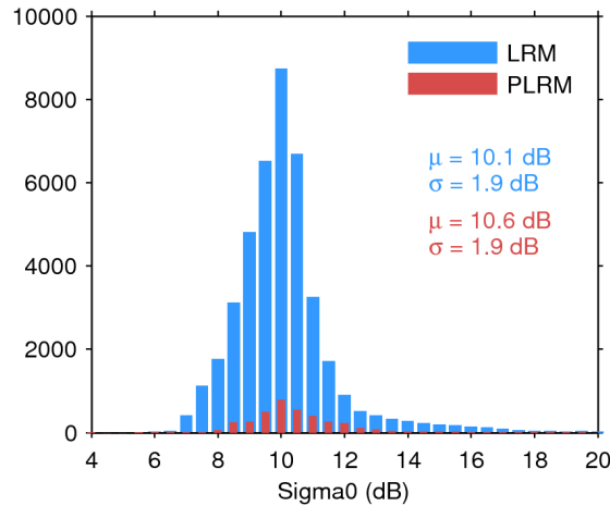
Figure 25. Histogram of flag-valid sigma0 over oceans and lakes for LRM (blue) and PLRM (red) for 24/09/2017. The mean ( \mu ) and standard deviation ( \sigma ) are also shown. Note that values outside [4 20] dB are excluded from the histogram for the sake of readability but not from the computation of \mu and \sigma .
