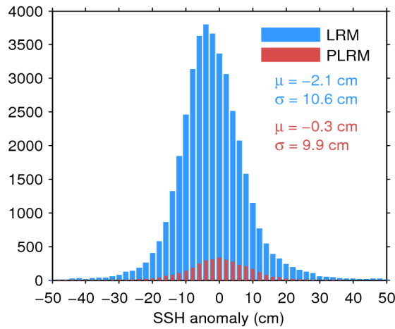
Figure 11. Histogram of science-valid SSH anomaly over oceans and lakes for LRM (blue) and PLRM (red) for 24/09/2017. The mean ( \mu ) and standard deviation ( \sigma ) are also shown. Note that values outside [-50 50] cm are excluded from the histogram for the sake of readability but not from the computation of \mu and \sigma .
