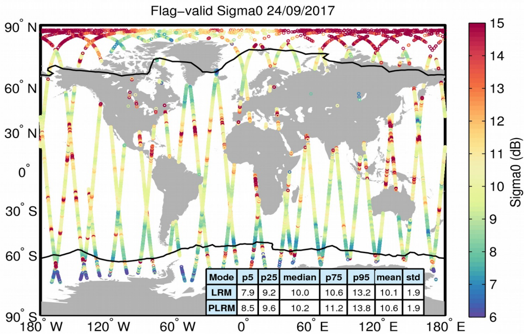
Figure 23. Geographical distribution of flag-valid sigma0 data over oceans and lakes for 24/09/2017. The statistical values shown in the table refer to the sigma0 in dB and are calculated separately for LRM and PLRM regions. Measurements taken over polar polygons have been excluded from the computation of the statistical values. The black lines mark the outer limit of the Arctic and Antarctic polar polygons.
