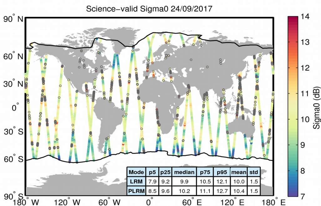
Figure 27. Geographical distribution of science-valid sigma0 data over oceans and lakes for 24/09/2017. The statistical values shown in the table refer to the sigma0 in dB and are calculated separately for LRM and PLRM regions. The black lines mark the outer limit of the Arctic and Antarctic polar polygons. Gray circles denote records that have been rejected based on the editing criteria described in Table 4.
