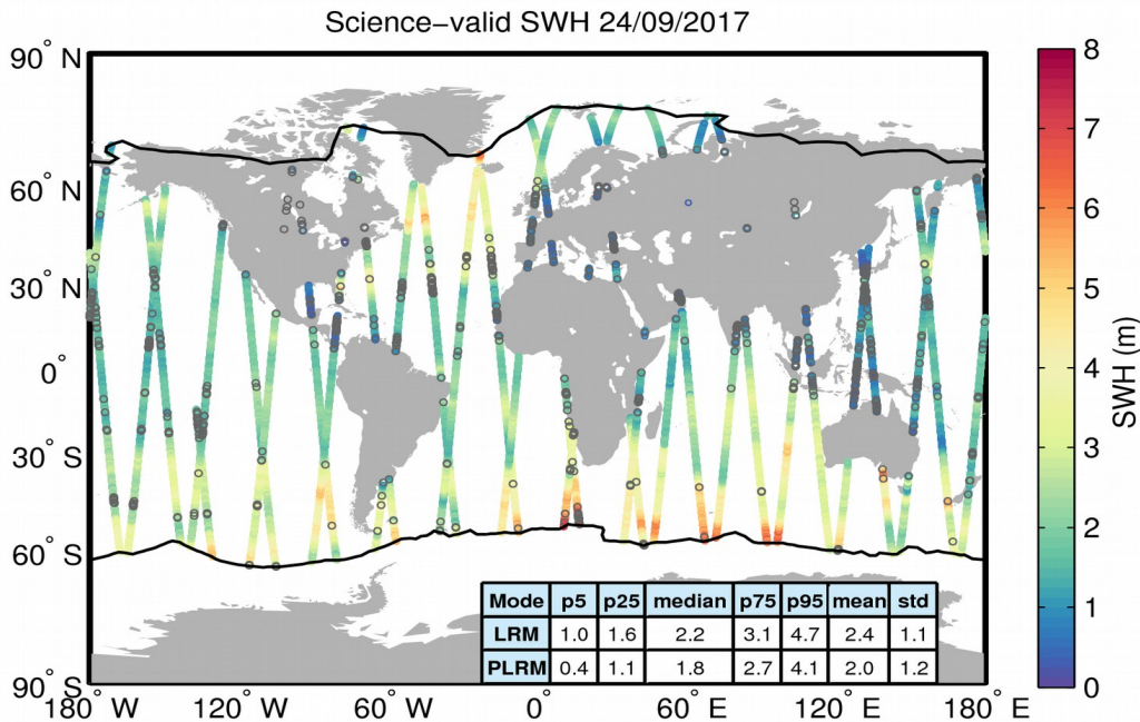
Figure 19. Geographical distribution of science-valid SWH data over oceans and lakes for 24/09/2017. The statistical values shown in the table refer to the SWH in m and are calculated separately for LRM and PLRM regions. The black lines mark the outer limit of the Arctic and Antarctic polar polygons. Gray circles denote records that have been rejected based on the editing criteria described in Table 3.
