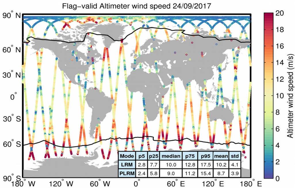
Figure 31. Geographical distribution of flag-valid wind data over oceans and lakes for 24/09/2017. The statistical values shown in the table refer to the wind in m/s and are calculated separately for LRM and PLRM regions. Measurements taken over polar polygons have been excluded from the computation of the statistical values. The black lines mark the outer limit of the Arctic and Antarctic polar polygons.
