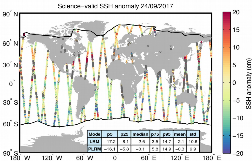
Figure 10. Geographical distribution of science-valid SSH anomaly data over oceans and lakes for 24/09/2017. The statistical values shown in the table refer to the SSH anomaly in cm and are calculated separately for LRM and PLRM regions. The black lines mark the outer limit of the Arctic and Antarctic polar polygons. Gray circles denote records that have been rejected based on the editing criteria described in Table 2.
