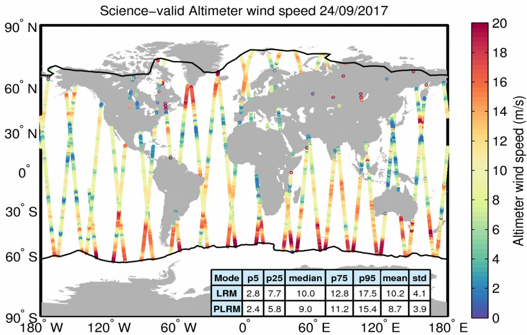
Figure 34. Geographical distribution of science-valid wind data over oceans and lakes for 24/09/2017. The statistical values shown in the table refer to the wind in m/s and are calculated separately for LRM and PLRM regions. The black lines mark the outer limit of the Arctic and Antarctic polar polygons. Gray circles denote records that have been rejected based on the editing criteria described in Table 5.
