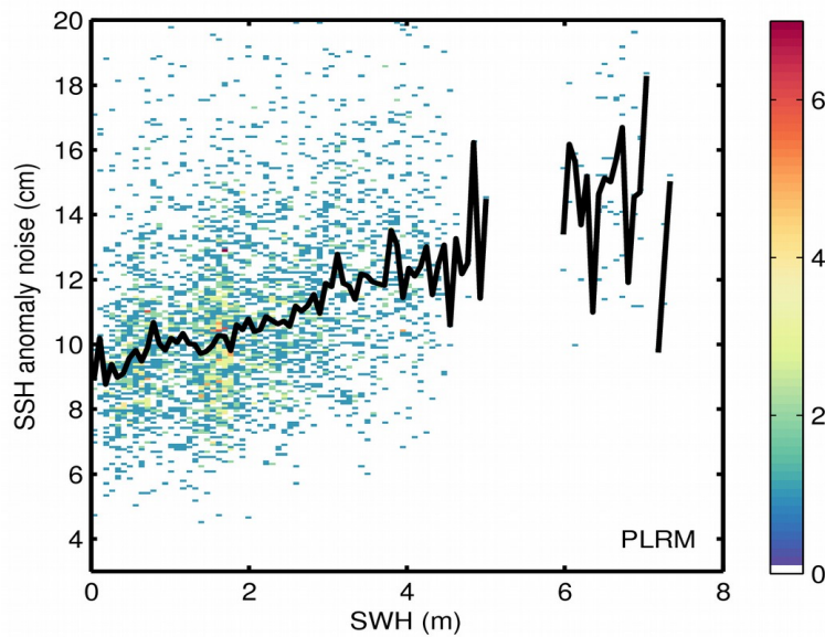
Figure 9. 2D histogram showing flag-valid SSH anomaly noise as a function of SWH for LRM (top) and PLRM (bottom) for 24/09/2017. The black line denotes the median SSH anomaly noise as a function of SWH.
