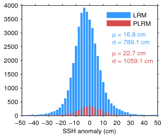
Figure 7. Histogram of flag-valid SSH anomaly over oceans and lakes for LRM (blue) and PLRM (red) for 24/09/2017. The mean ( \mu ) and standard deviation ( \sigma ) are also shown. Note that values outside [-50 \ 50] cm are excluded from the histogram for the sake of readability but not from the computation of \mu and \sigma .
