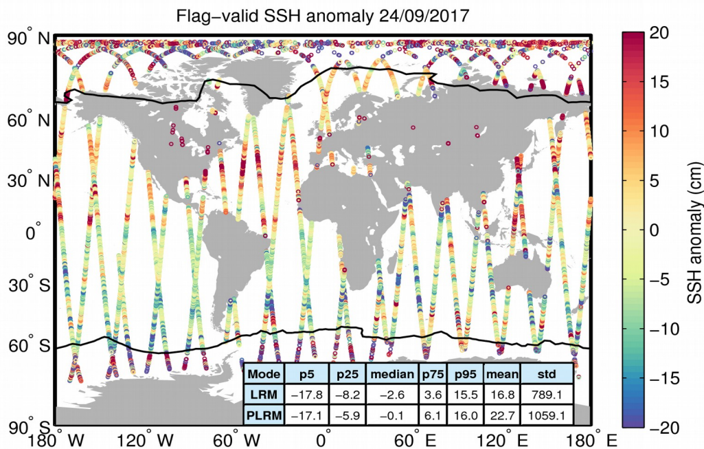
Figure 5. Geographical distribution of flag-valid 1-Hz SSH anomaly data over oceans and lakes for 24/09/2017. The statistical values shown in the table refer to the SSH anomaly in cm and are calculated separately for LRM and PLRM regions. Measurements taken over polar polygons have been excluded from the computation of the statistical values. The black lines mark the outer limit of the Arctic and Antarctic polar polygons.
