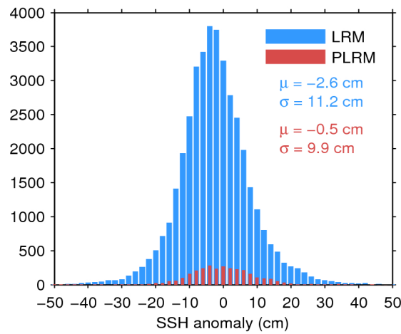
Figure 11. Histogram of science-valid SSH anomaly over oceans and lakes for LRM (blue) and PLRM (red) for 22/09/2017. The mean ( \mu ) and standard deviation ( \sigma ) are also shown. Note that values outside [-50\ 50] cm are excluded from the histogram for the sake of readability but not from the computation of \mu and \sigma .
