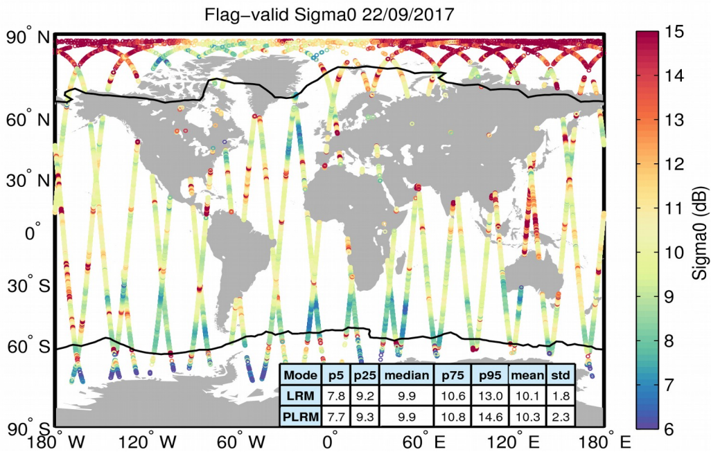
Figure 23. Geographical distribution of flag-valid sigma0 data over oceans and lakes for 22/09/2017. The statistical values shown in the table refer to the sigma0 in dB and are calculated separately for LRM and PLRM regions. Measurements taken over polar polygons have been excluded from the computation of the statistical values. The black lines mark the outer limit of the Arctic and Antarctic polar polygons.
