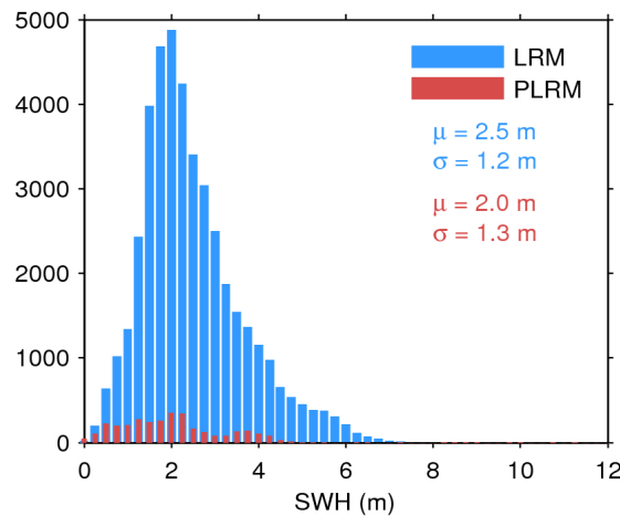
Figure 17. Histogram of flag-valid SWH over oceans and lakes for LRM (blue) and PLRM (red) for 22/09/2017. The mean ( \mu ) and standard deviation ( \sigma ) are also shown. Note that values larger than 12 m are excluded from the histogram for the sake of readability but not from the computation of \mu and \sigma .
