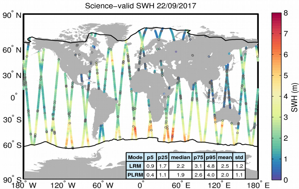
Figure 19. Geographical distribution of science-valid SWH data over oceans and lakes for 22/09/2017. The statistical values shown in the table refer to the SWH in m and are calculated separately for LRM and PLRM regions. The black lines mark the outer limit of the Arctic and Antarctic polar polygons. Gray circles denote records that have been rejected based on the editing criteria described in Table 3.
