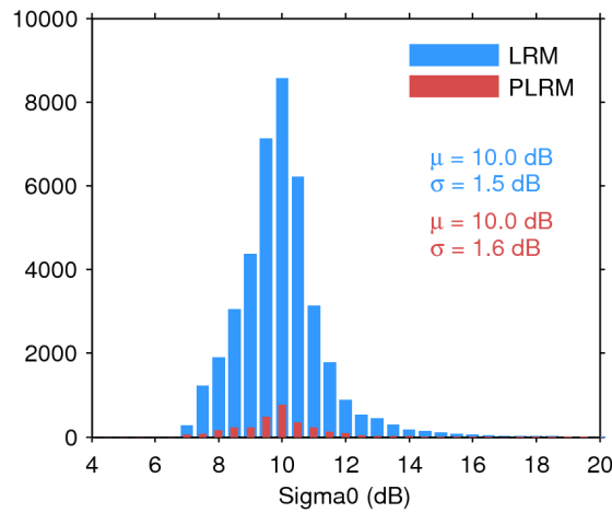
Figure 28. Histogram of science-valid sigma0 over oceans and lakes for LRM (blue) and PLRM (red) for 22/09/2017. The mean ( \mu ) and standard deviation ( \sigma ) are also shown. Note that values outside [4 20] dB are excluded from the histogram for the sake of readability but not from the computation of \mu and \sigma .
