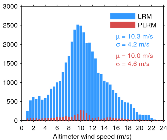
Figure 33. Histogram of flag-valid wind over oceans and lakes for LRM (blue) and PLRM (red) for 22/09/2017. The mean ( \mu ) and standard deviation ( \sigma ) are also shown. Note that values larger than 24 m/s are excluded from the histogram for the sake of readability but not from the computation of \mu and \sigma .
