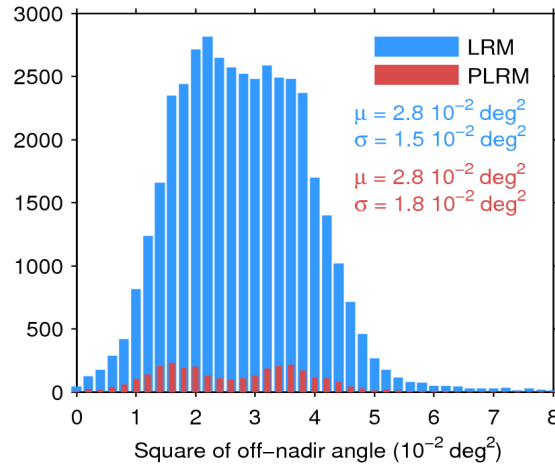
Figure 39. Histogram of flag-valid mispointing over oceans and lakes for LRM (blue) and PLRM (red) for 22/09/2017. Only positive values have been considered. The mean ( \mu ) and standard deviation ( \sigma ) are also shown. Note that values larger than 8 \cdot 10^{-2} \text{ deg}^2 are excluded from the histogram for the sake of readability but not from the computation of \mu and \sigma .
