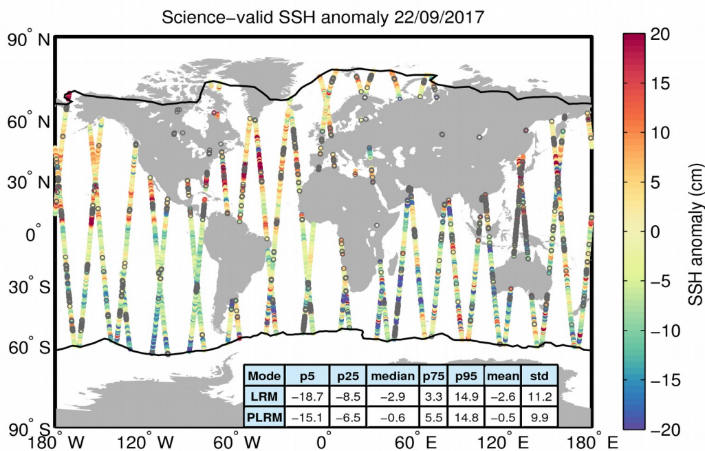
Figure 10. Geographical distribution of science-valid SSH anomaly data over oceans and lakes for 22/09/2017. The statistical values shown in the table refer to the SSH anomaly in cm and are calculated separately for LRM and PLRM regions. The black lines mark the outer limit of the Arctic and Antarctic polar polygons. Gray circles denote records that have been rejected based on the editing criteria described in Table 2.
