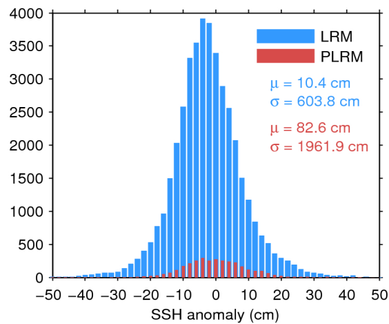
Figure 7. Histogram of flag-valid SSH anomaly over oceans and lakes for LRM (blue) and PLRM (red) for 22/09/2017. The mean ( \mu ) and standard deviation ( \sigma ) are also shown. Note that values outside [-50 50] cm are excluded from the histogram for the sake of readability but not from the computation of \mu and \sigma .
