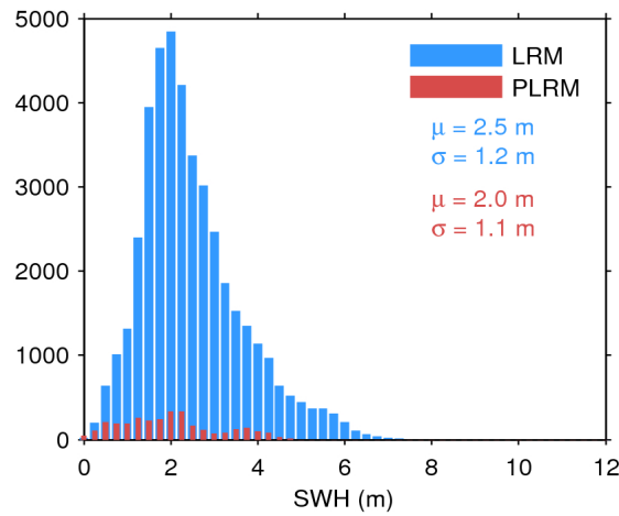
Figure 20. Histogram of science-valid SWH over oceans and lakes for LRM (blue) and PLRM (red) for 22/09/2017. The mean ( \mu ) and standard deviation ( \sigma ) are also shown. Note that values larger than 12 m are excluded from the histogram for the sake of readability but not from the computation of \mu and \sigma .
