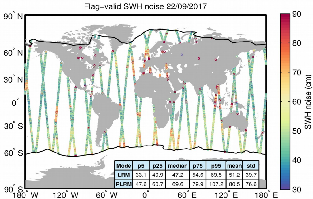
Figure 18. Geographical distribution of flag-valid 20-Hz SWH measurement noise over oceans and lakes for 22/09/2017. The statistical values shown in the table refer to the SWH noise and are calculated separately for LRM and PLRM regions. Measurements taken over polar polygons have been excluded from the computation of the statistical values. The black lines mark the outer limit of the Arctic and Antarctic polar polygons.
