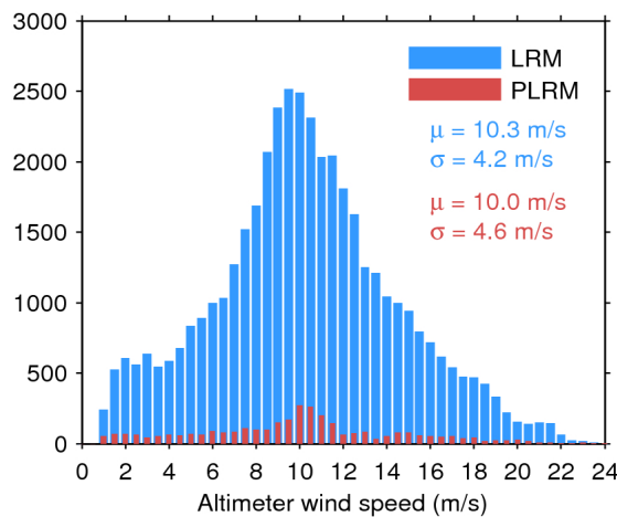
Figure 35. Histogram of science-valid wind over oceans and lakes for LRM (blue) and PLRM (red) for 22/09/2017. The mean ( \mu ) and standard deviation ( \sigma ) are also shown. Note that values larger than 24 m/s are excluded from the histogram for the sake of readability but not from the computation of \mu and \sigma .
