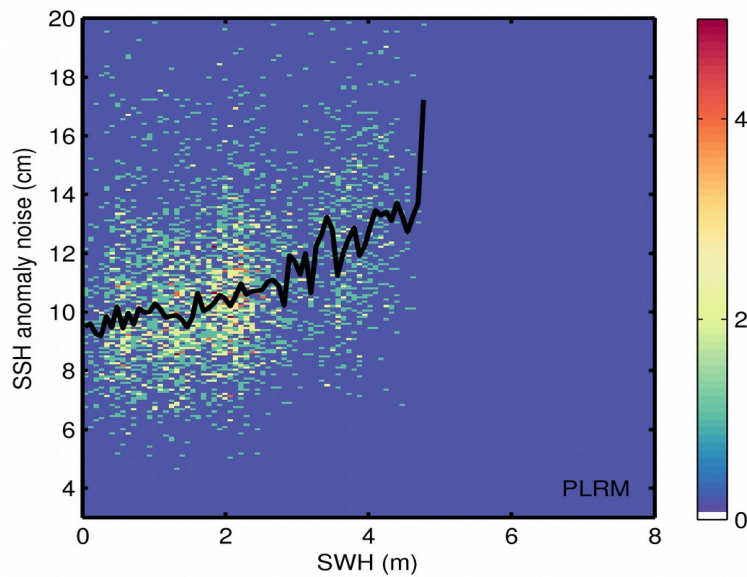
Figure 9. 2D histogram showing flag-valid SSH anomaly noise as a function of SWH for LRM (top) and PLRM (bottom) for 22/09/2017. The black line denotes the median SSH anomaly noise as a function of SWH.
