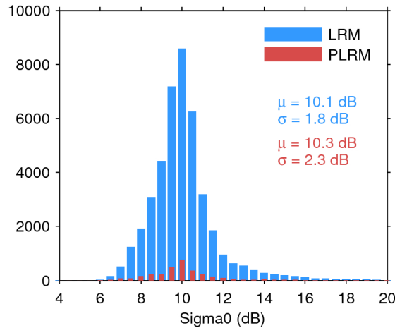
Figure 25. Histogram of flag-valid sigma0 over oceans and lakes for LRM (blue) and PLRM (red) for 22/09/2017. The mean ( \mu ) and standard deviation ( \sigma ) are also shown. Note that values outside [4 20] dB are excluded from the histogram for the sake of readability but not from the computation of \mu and \sigma .
