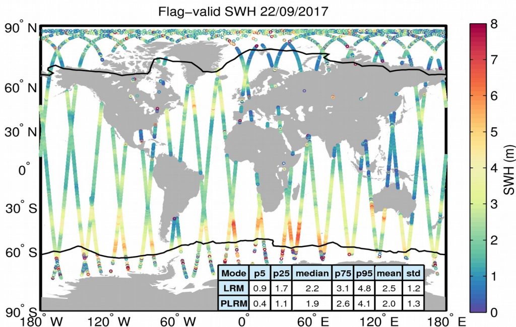
Figure 15. Geographical distribution of flag-valid SWH data over oceans and lakes for 22/09/2017. The statistical values shown in the table refer to the SWH in m and are calculated separately for LRM and PLRM regions. Measurements taken over polar polygons have been excluded from the computation of the statistical values. The black lines mark the outer limit of the Arctic and Antarctic polar polygons.
