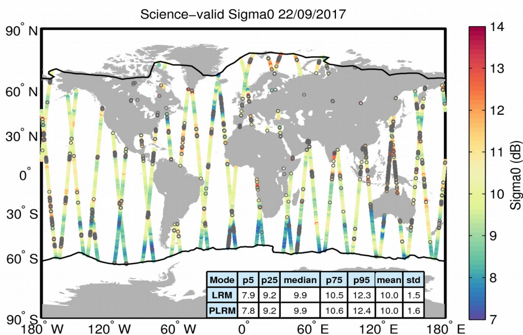
Figure 27. Geographical distribution of science-valid sigma0 data over oceans and lakes for 22/09/2017. The statistical values shown in the table refer to the sigma0 in dB and are calculated separately for LRM and PLRM regions. The black lines mark the outer limit of the Arctic and Antarctic polar polygons. Gray circles denote records that have been rejected based on the editing criteria described in Table 4.
