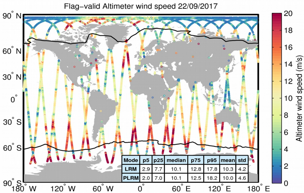
Figure 31. Geographical distribution of flag-valid wind data over oceans and lakes for 22/09/2017. The statistical values shown in the table refer to the wind in m/s and are calculated separately for LRM and PLRM regions. Measurements taken over polar polygons have been excluded from the computation of the statistical values. The black lines mark the outer limit of the Arctic and Antarctic polar polygons.
