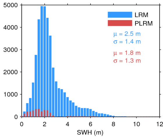
Figure 20. Histogram of science-valid SWH over oceans and lakes for LRM (blue) and PLRM (red) for 18/09/2017. The mean ( \mu ) and standard deviation ( \sigma ) are also shown. Note that values larger than 12 m are excluded from the histogram for the sake of readability but not from the computation of \mu and \sigma .
