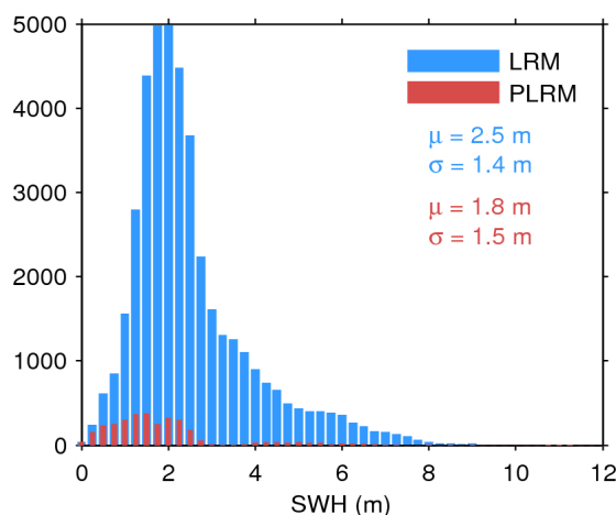
Figure 17. Histogram of flag-valid SWH over oceans and lakes for LRM (blue) and PLRM (red) for 18/09/2017. The mean ( \mu ) and standard deviation ( \sigma ) are also shown. Note that values larger than 12 m are excluded from the histogram for the sake of readability but not from the computation of \mu and \sigma .
