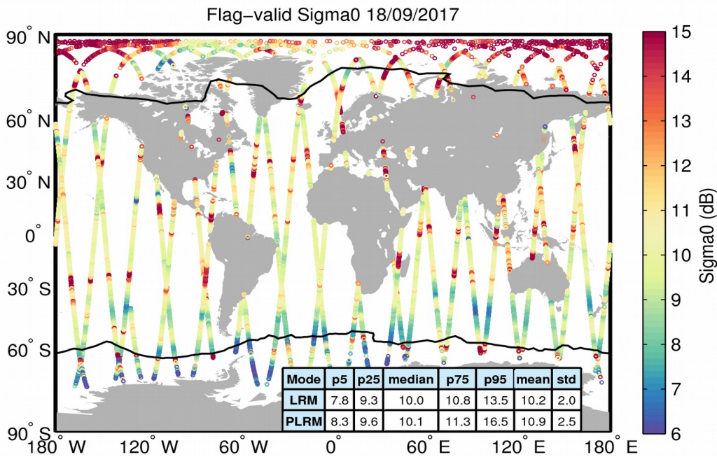
Figure 23. Geographical distribution of flag-valid sigma0 data over oceans and lakes for 18/09/2017. The statistical values shown in the table refer to the sigma0 in dB and are calculated separately for LRM and PLRM regions. Measurements taken over polar polygons have been excluded from the computation of the statistical values. The black lines mark the outer limit of the Arctic and Antarctic polar polygons.
