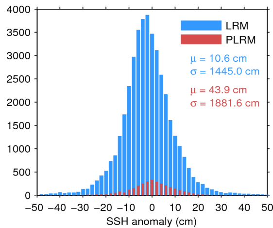
Figure 7. Histogram of flag-valid SSH anomaly over oceans and lakes for LRM (blue) and PLRM (red) for 18/09/2017. The mean ( \mu ) and standard deviation ( \sigma ) are also shown. Note that values outside [-50\ 50] cm are excluded from the histogram for the sake of readability but not from the computation of \mu and \sigma .
