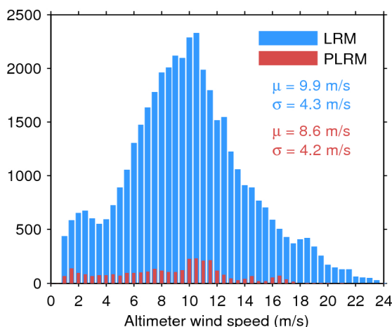
Figure 33. Histogram of flag-valid wind over oceans and lakes for LRM (blue) and PLRM (red) for 18/09/2017. The mean ( \mu ) and standard deviation ( \sigma ) are also shown. Note that values larger than 24 m/s are excluded from the histogram for the sake of readability but not from the computation of \mu and \sigma .
