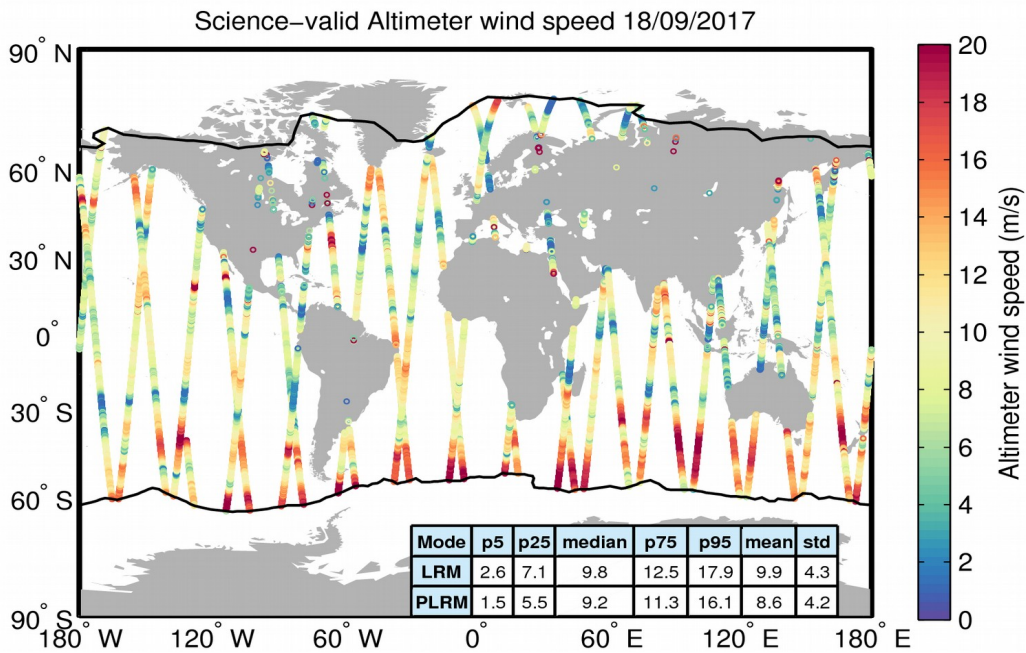
Figure 34. Geographical distribution of science-valid wind data over oceans and lakes for 18/09/2017. The statistical values shown in the table refer to the wind in m/s and are calculated separately for LRM and PLRM regions. The black lines mark the outer limit of the Arctic and Antarctic polar polygons. Gray circles denote records that have been rejected based on the editing criteria described in Table 5.
