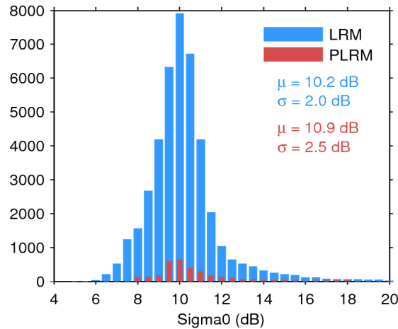
Figure 25. Histogram of flag-valid sigma0 over oceans and lakes for LRM (blue) and PLRM (red) for 18/09/2017. The mean ( \mu ) and standard deviation ( \sigma ) are also shown. Note that values outside [4 20] dB are excluded from the histogram for the sake of readability but not from the computation of \mu and \sigma .
