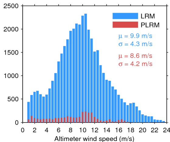
Figure 35. Histogram of science-valid wind over oceans and lakes for LRM (blue) and PLRM (red) for 18/09/2017. The mean ( \mu ) and standard deviation ( \sigma ) are also shown. Note that values larger than 24 m/s are excluded from the histogram for the sake of readability but not from the computation of \mu and \sigma .
