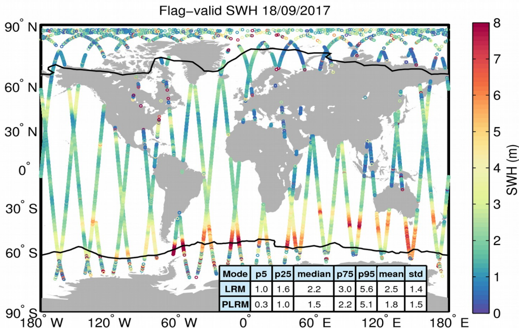
Figure 15. Geographical distribution of flag-valid SWH data over oceans and lakes for 18/09/2017. The statistical values shown in the table refer to the SWH in m and are calculated separately for LRM and PLRM regions. Measurements taken over polar polygons have been excluded from the computation of the statistical values. The black lines mark the outer limit of the Arctic and Antarctic polar polygons.
