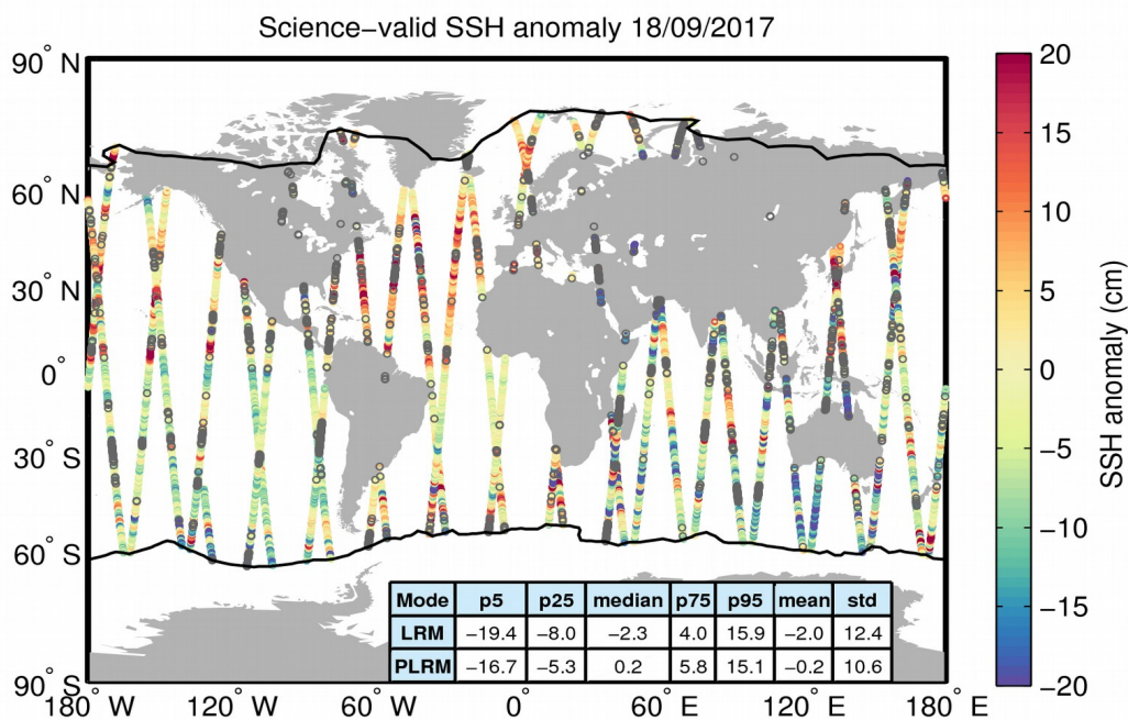
Figure 10. Geographical distribution of science-valid SSH anomaly data over oceans and lakes for 18/09/2017. The statistical values shown in the table refer to the SSH anomaly in cm and are calculated separately for LRM and PLRM regions. The black lines mark the outer limit of the Arctic and Antarctic polar polygons. Gray circles denote records that have been rejected based on the editing criteria described in Table 2.
