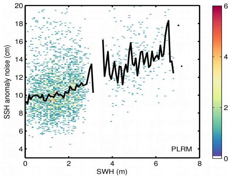
Figure 9. 2D histogram showing flag-valid SSH anomaly noise as a function of SWH for LRM (top) and PLRM (bottom) for 18/09/2017. The black line denotes the median SSH anomaly noise as a function of SWH.
