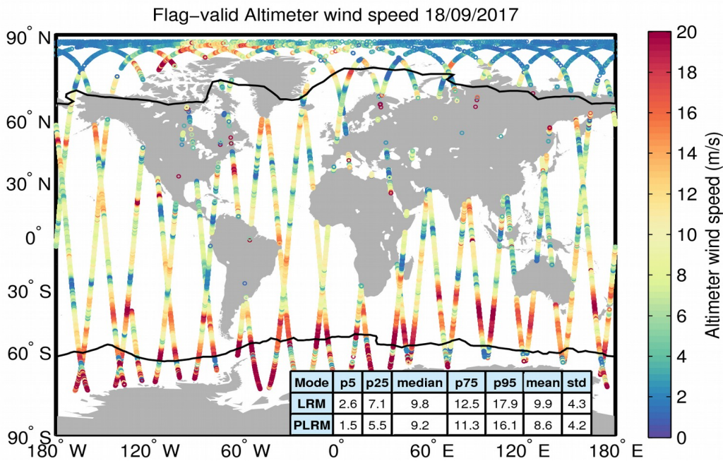
Figure 31. Geographical distribution of flag-valid wind data over oceans and lakes for 18/09/2017. The statistical values shown in the table refer to the wind in m/s and are calculated separately for LRM and PLRM regions. Measurements taken over polar polygons have been excluded from the computation of the statistical values. The black lines mark the outer limit of the Arctic and Antarctic polar polygons.
