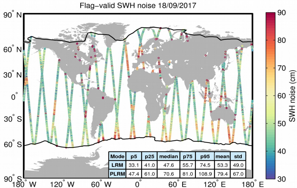
Figure 18. Geographical distribution of flag-valid 20-Hz SWH measurement noise over oceans and lakes for 18/09/2017. The statistical values shown in the table refer to the SWH noise and are calculated separately for LRM and PLRM regions. Measurements taken over polar polygons have been excluded from the computation of the statistical values. The black lines mark the outer limit of the Arctic and Antarctic polar polygons.
