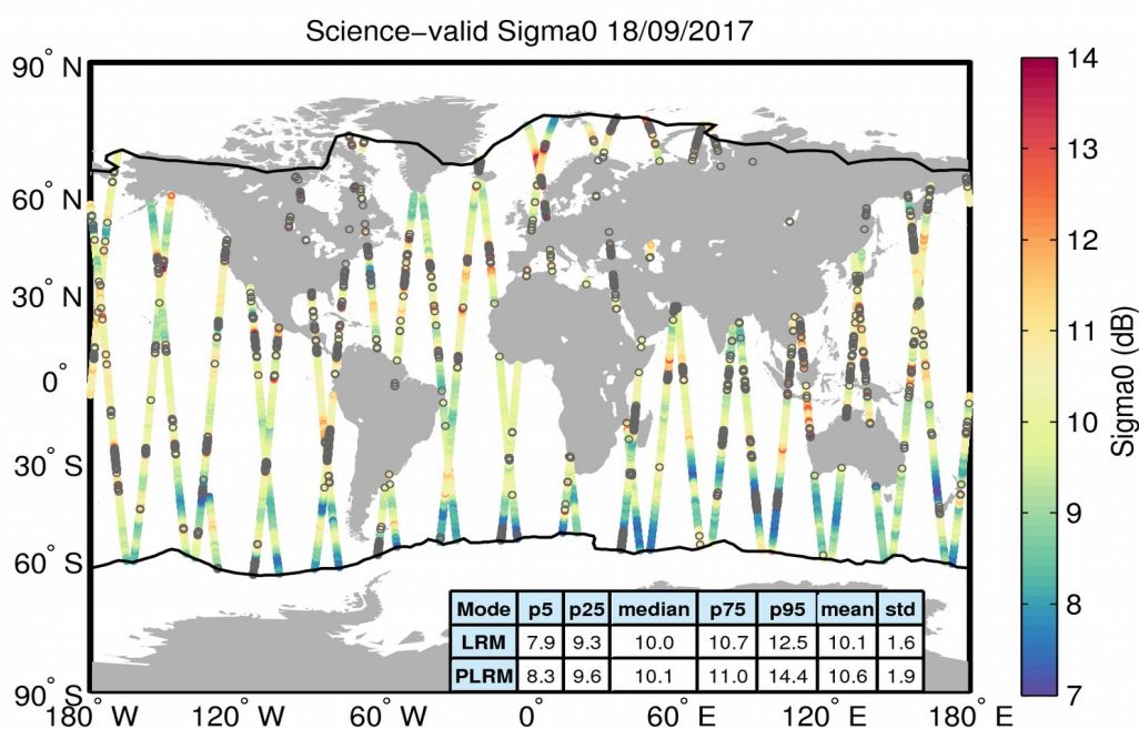
Figure 27. Geographical distribution of science-valid sigma0 data over oceans and lakes for 18/09/2017. The statistical values shown in the table refer to the sigma0 in dB and are calculated separately for LRM and PLRM regions. The black lines mark the outer limit of the Arctic and Antarctic polar polygons. Gray circles denote records that have been rejected based on the editing criteria described in Table 4.
