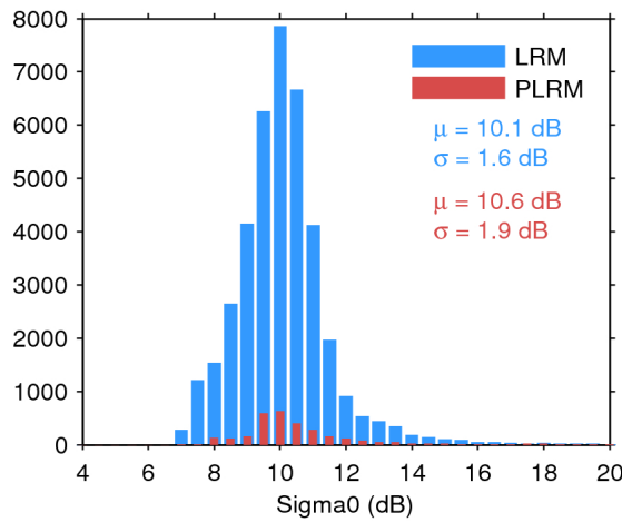
Figure 28. Histogram of science-valid sigma0 over oceans and lakes for LRM (blue) and PLRM (red) for 18/09/2017. The mean ( \mu ) and standard deviation ( \sigma ) are also shown. Note that values outside [4 20] dB are excluded from the histogram for the sake of readability but not from the computation of \mu and \sigma .
