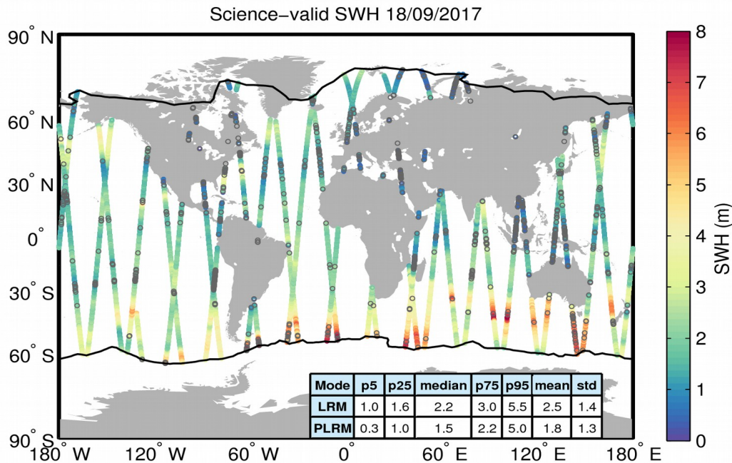
Figure 19. Geographical distribution of science-valid SWH data over oceans and lakes for 18/09/2017. The statistical values shown in the table refer to the SWH in m and are calculated separately for LRM and PLRM regions. The black lines mark the outer limit of the Arctic and Antarctic polar polygons. Gray circles denote records that have been rejected based on the editing criteria described in Table 3.
