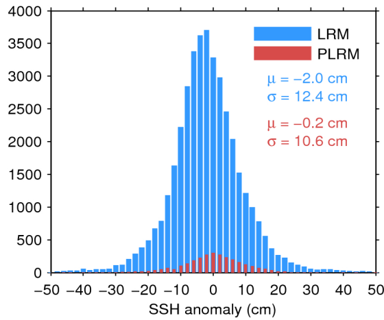
Figure 11. Histogram of science-valid SSH anomaly over oceans and lakes for LRM (blue) and PLRM (red) for 18/09/2017. The mean ( \mu ) and standard deviation ( \sigma ) are also shown. Note that values outside [-50\ 50] cm are excluded from the histogram for the sake of readability but not from the computation of \mu and \sigma .
