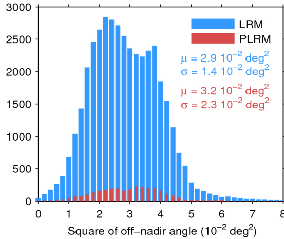
Figure 39. Histogram of flag-valid mispointing over oceans and lakes for LRM (blue) and PLRM (red) for 18/09/2017. Only positive values have been considered. The mean ( \mu ) and standard deviation ( \sigma ) are also shown. Note that values larger than 8 \cdot 10^{-2} \text{ deg}^2 are excluded from the histogram for the sake of readability but not from the computation of \mu and \sigma .
