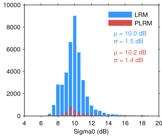
Figure 28. Histogram of science-valid sigma0 over oceans and lakes for LRM (blue) and PLRM (red) for 16/09/2017. The mean ( \mu ) and standard deviation ( \sigma ) are also shown. Note that values outside [4 20] dB are excluded from the histogram for the sake of readability but not from the computation of \mu and \sigma .
