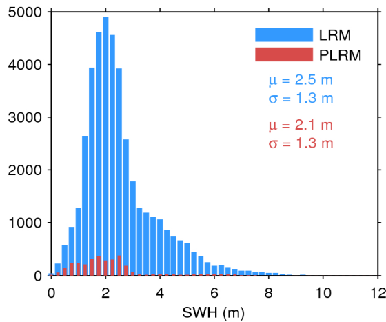
Figure 20. Histogram of science-valid SWH over oceans and lakes for LRM (blue) and PLRM (red) for 16/09/2017. The mean ( \mu ) and standard deviation ( \sigma ) are also shown. Note that values larger than 12 m are excluded from the histogram for the sake of readability but not from the computation of \mu and \sigma .
