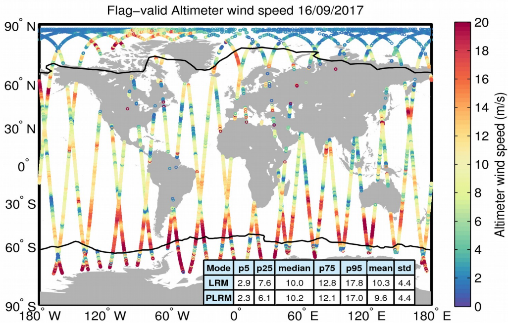
Figure 31. Geographical distribution of flag-valid wind data over oceans and lakes for 16/09/2017. The statistical values shown in the table refer to the wind in m/s and are calculated separately for LRM and PLRM regions. Measurements taken over polar polygons have been excluded from the computation of the statistical values. The black lines mark the outer limit of the Arctic and Antarctic polar polygons.
