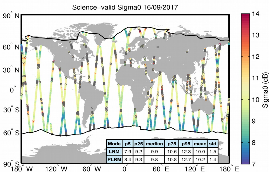
Figure 27. Geographical distribution of science-valid sigma0 data over oceans and lakes for 16/09/2017. The statistical values shown in the table refer to the sigma0 in dB and are calculated separately for LRM and PLRM regions. The black lines mark the outer limit of the Arctic and Antarctic polar polygons. Gray circles denote records that have been rejected based on the editing criteria described in Table 4.
