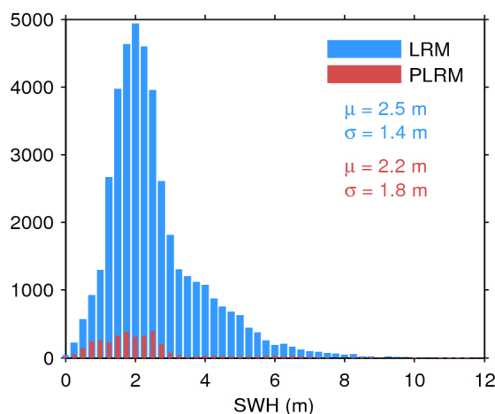
Figure 17. Histogram of flag-valid SWH over oceans and lakes for LRM (blue) and PLRM (red) for 16/09/2017. The mean ( \mu ) and standard deviation ( \sigma ) are also shown. Note that values larger than 12 m are excluded from the histogram for the sake of readability but not from the computation of \mu and \sigma .
