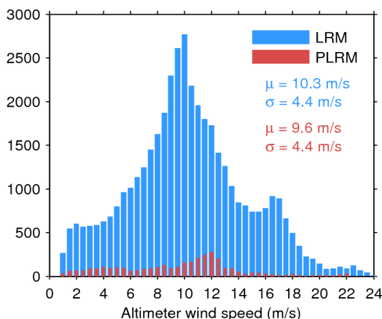
Figure 33. Histogram of flag-valid wind over oceans and lakes for LRM (blue) and PLRM (red) for 16/09/2017. The mean ( \mu ) and standard deviation ( \sigma ) are also shown. Note that values larger than 24 m/s are excluded from the histogram for the sake of readability but not from the computation of \mu and \sigma .
