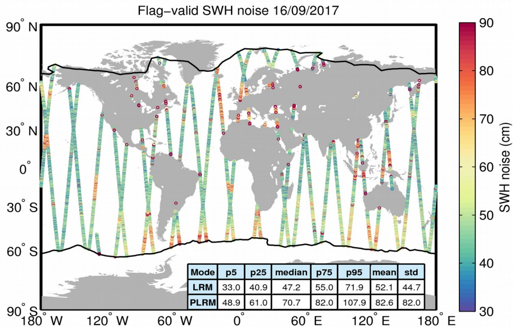
Figure 18. Geographical distribution of flag-valid 20-Hz SWH measurement noise over oceans and lakes for 16/09/2017. The statistical values shown in the table refer to the SWH noise and are calculated separately for LRM and PLRM regions. Measurements taken over polar polygons have been excluded from the computation of the statistical values. The black lines mark the outer limit of the Arctic and Antarctic polar polygons.
