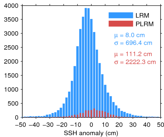
Figure 7. Histogram of flag-valid SSH anomaly over oceans and lakes for LRM (blue) and PLRM (red) for 16/09/2017. The mean ( \mu ) and standard deviation ( \sigma ) are also shown. Note that values outside [-50\ 50] cm are excluded from the histogram for the sake of readability but not from the computation of \mu and \sigma .
