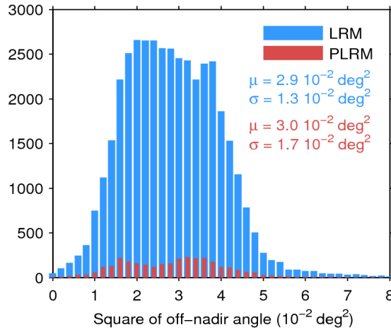
Figure 39. Histogram of flag-valid mispointing over oceans and lakes for LRM (blue) and PLRM (red) for 16/09/2017. Only positive values have been considered. The mean ( \mu ) and standard deviation ( \sigma ) are also shown. Note that values larger than 8 \cdot 10^{-2} \text{ deg}^2 are excluded from the histogram for the sake of readability but not from the computation of \mu and \sigma .
