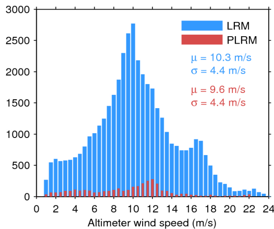
Figure 35. Histogram of science-valid wind over oceans and lakes for LRM (blue) and PLRM (red) for 16/09/2017. The mean ( \mu ) and standard deviation ( \sigma ) are also shown. Note that values larger than 24 m/s are excluded from the histogram for the sake of readability but not from the computation of \mu and \sigma .
