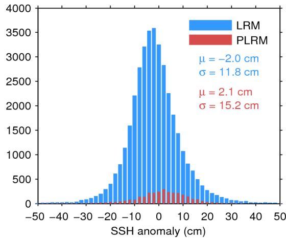
Figure 11. Histogram of science-valid SSH anomaly over oceans and lakes for LRM (blue) and PLRM (red) for 16/09/2017. The mean ( \mu ) and standard deviation ( \sigma ) are also shown. Note that values outside [-50 50] cm are excluded from the histogram for the sake of readability but not from the computation of \mu and \sigma .
