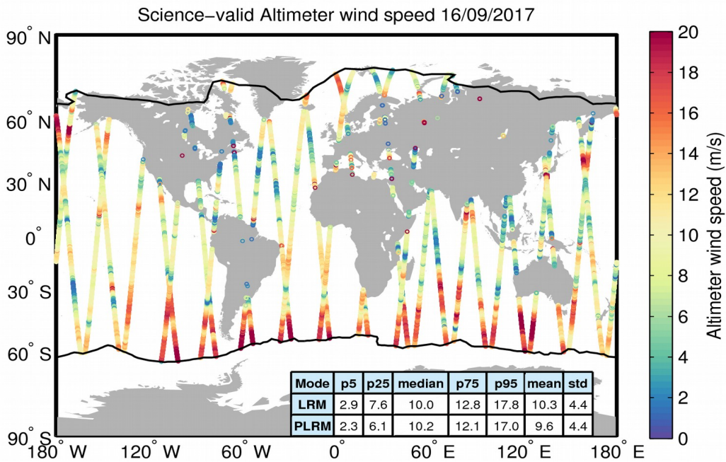
Figure 34. Geographical distribution of science-valid wind data over oceans and lakes for 16/09/2017. The statistical values shown in the table refer to the wind in m/s and are calculated separately for LRM and PLRM regions. The black lines mark the outer limit of the Arctic and Antarctic polar polygons. Gray circles denote records that have been rejected based on the editing criteria described in Table 5.
