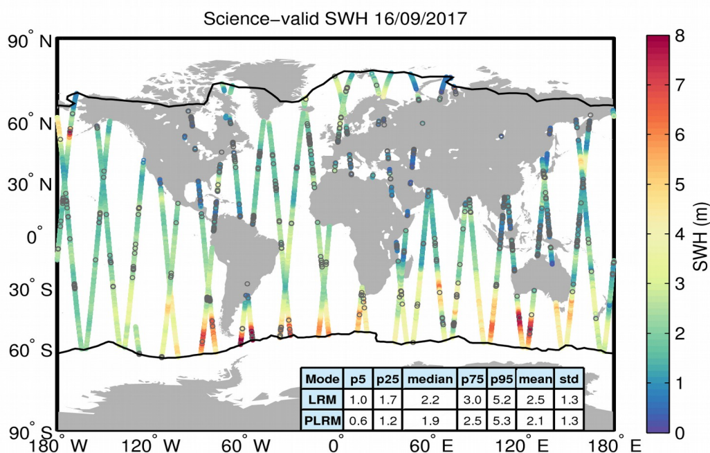
Figure 19. Geographical distribution of science-valid SWH data over oceans and lakes for 16/09/2017. The statistical values shown in the table refer to the SWH in m and are calculated separately for LRM and PLRM regions. The black lines mark the outer limit of the Arctic and Antarctic polar polygons. Gray circles denote records that have been rejected based on the editing criteria described in Table 3.
