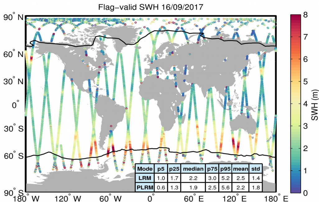
Figure 15. Geographical distribution of flag-valid SWH data over oceans and lakes for 16/09/2017. The statistical values shown in the table refer to the SWH in m and are calculated separately for LRM and PLRM regions. Measurements taken over polar polygons have been excluded from the computation of the statistical values. The black lines mark the outer limit of the Arctic and Antarctic polar polygons.
