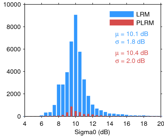
Figure 25. Histogram of flag-valid sigma0 over oceans and lakes for LRM (blue) and PLRM (red) for 16/09/2017. The mean ( \mu ) and standard deviation ( \sigma ) are also shown. Note that values outside [4 20] dB are excluded from the histogram for the sake of readability but not from the computation of \mu and \sigma .
