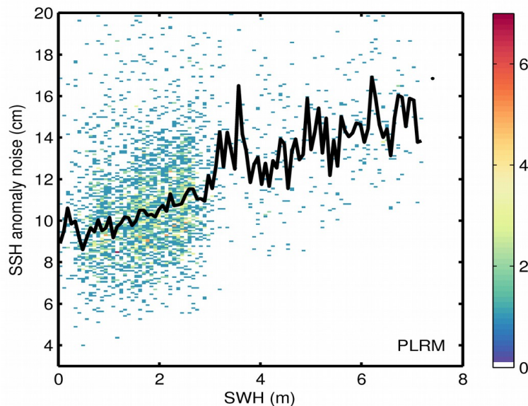
Figure 9. 2D histogram showing flag-valid SSH anomaly noise as a function of SWH for LRM (top) and PLRM (bottom) for 16/09/2017. The black line denotes the median SSH anomaly noise as a function of SWH.
