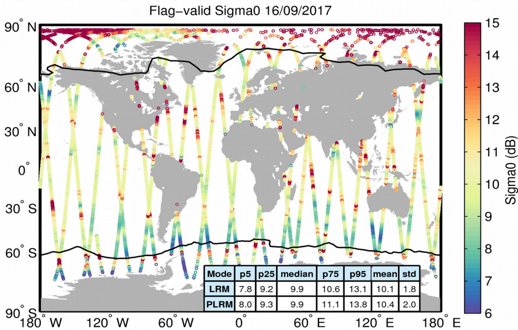
Figure 23. Geographical distribution of flag-valid sigma0 data over oceans and lakes for 16/09/2017. The statistical values shown in the table refer to the sigma0 in dB and are calculated separately for LRM and PLRM regions. Measurements taken over polar polygons have been excluded from the computation of the statistical values. The black lines mark the outer limit of the Arctic and Antarctic polar polygons.
