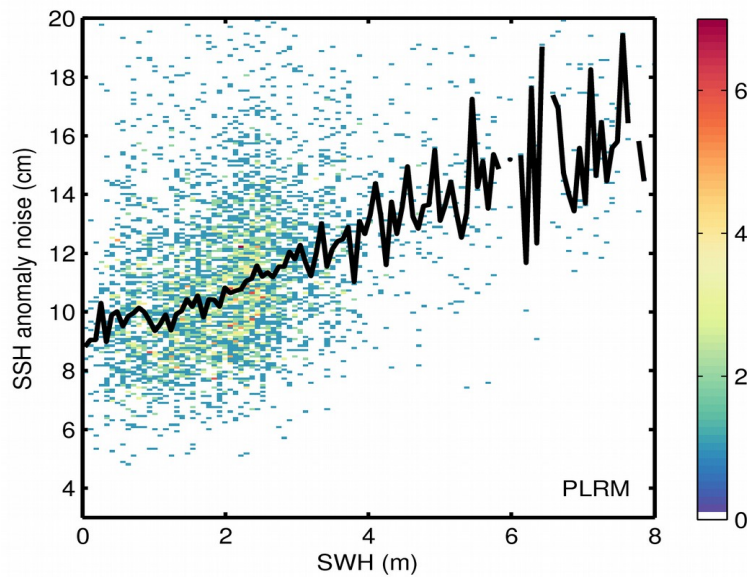
Figure 9. 2D histogram showing flag-valid SSH anomaly noise as a function of SWH for LRM (top) and PLRM (bottom) for 15/09/2017. The black line denotes the median SSH anomaly noise as a function of SWH.
