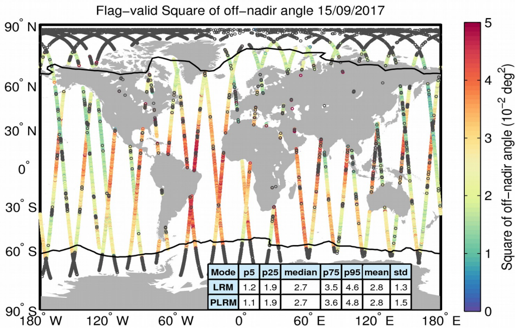
Figure 37. Geographical distribution of flag-valid mispointing data over oceans and lakes for 15/09/2017. The statistical values shown in the table refer to the mispointing in 10^{-2} deg 2 and are calculated separately for LRM and PLRM regions. Measurements taken over polar polygons have been excluded from the computation of the statistical values. The black lines mark the outer limit of the Arctic and Antarctic polar polygons. Gray circles denote negative values.
