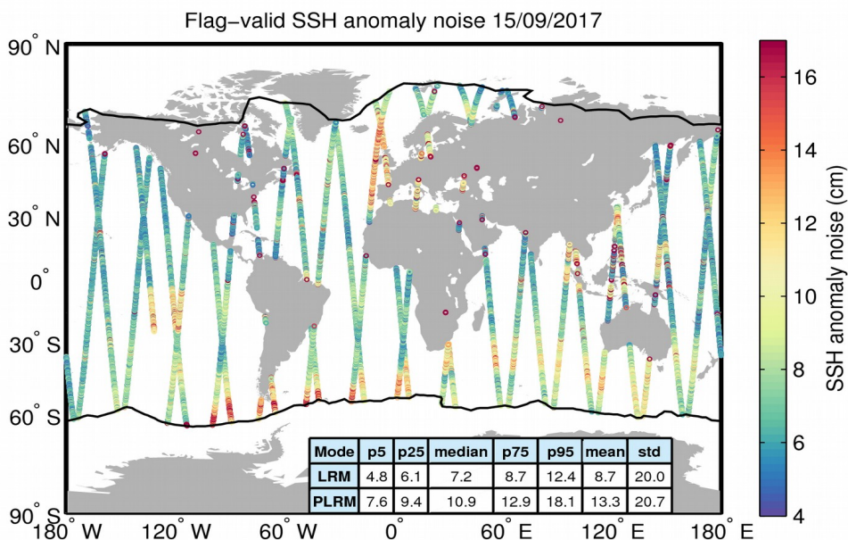
Figure 8. Geographical distribution of flag-valid 20-Hz SSH anomaly measurement noise over oceans and lakes for 15/09/2017. The statistical values shown in the table refer to the SSH anomaly noise and are calculated separately for LRM and PLRM regions. Measurements taken over polar polygons have been excluded from the computation of the statistical values. The black lines mark the outer limit of the Arctic and Antarctic polar polygons.
