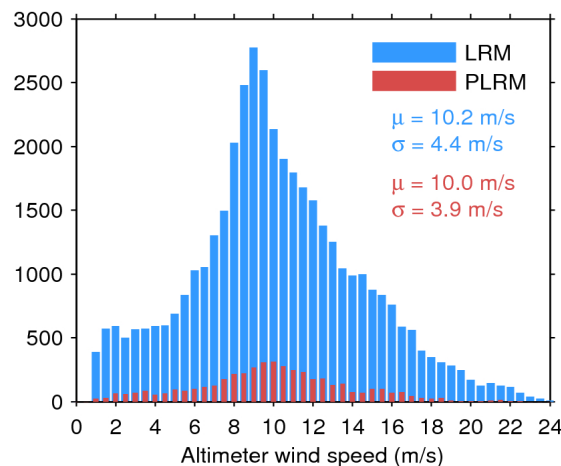
Figure 35. Histogram of science-valid wind over oceans and lakes for LRM (blue) and PLRM (red) for 15/09/2017. The mean ( \mu ) and standard deviation ( \sigma ) are also shown. Note that values larger than 24 m/s are excluded from the histogram for the sake of readability but not from the computation of \mu and \sigma .
