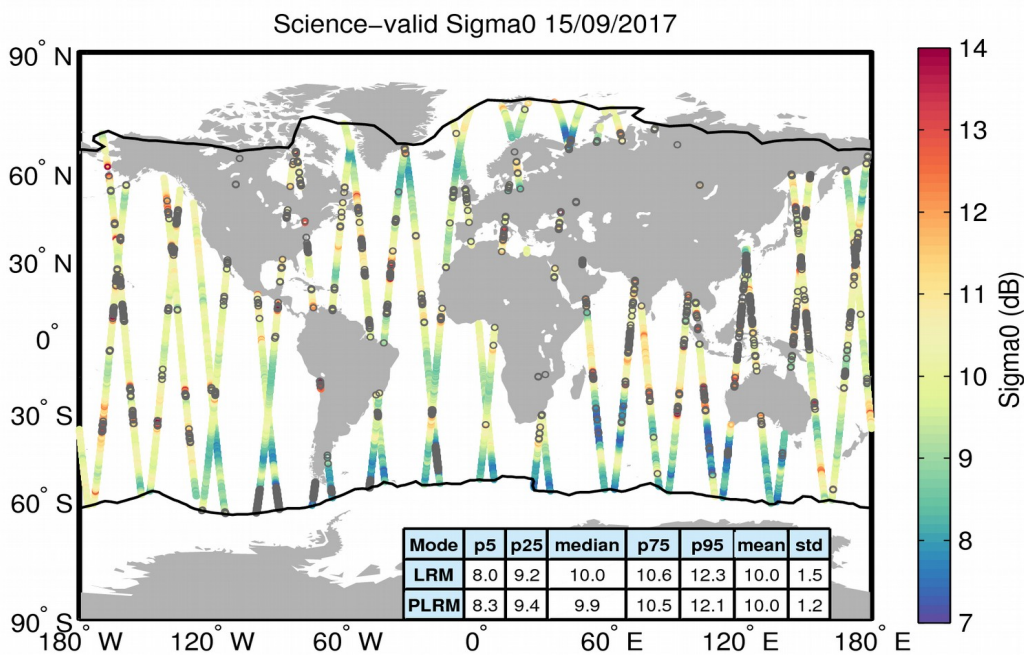
Figure 27. Geographical distribution of science-valid sigma0 data over oceans and lakes for 15/09/2017. The statistical values shown in the table refer to the sigma0 in dB and are calculated separately for LRM and PLRM regions. The black lines mark the outer limit of the Arctic and Antarctic polar polygons. Gray circles denote records that have been rejected based on the editing criteria described in Table 4.
