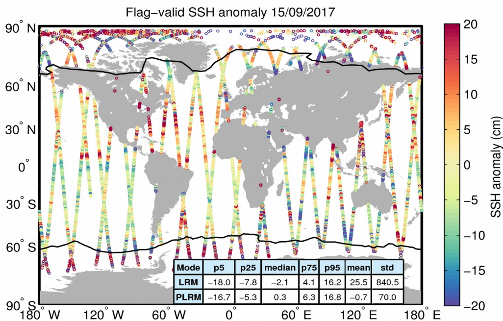
Figure 5. Geographical distribution of flag-valid 1-Hz SSH anomaly data over oceans and lakes for 15/09/2017. The statistical values shown in the table refer to the SSH anomaly in cm and are calculated separately for LRM and PLRM regions. Measurements taken over polar polygons have been excluded from the computation of the statistical values. The black lines mark the outer limit of the Arctic and Antarctic polar polygons.
