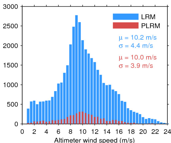
Figure 33. Histogram of flag-valid wind over oceans and lakes for LRM (blue) and PLRM (red) for 15/09/2017. The mean ( \mu ) and standard deviation ( \sigma ) are also shown. Note that values larger than 24 m/s are excluded from the histogram for the sake of readability but not from the computation of \mu and \sigma .
