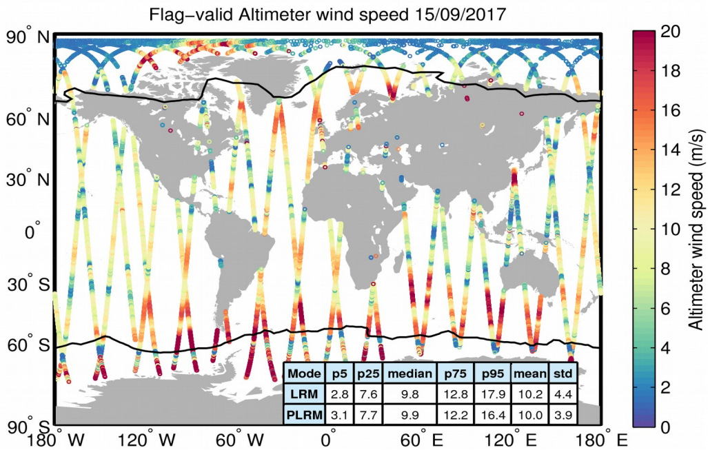
Figure 31. Geographical distribution of flag-valid wind data over oceans and lakes for 15/09/2017. The statistical values shown in the table refer to the wind in m/s and are calculated separately for LRM and PLRM regions. Measurements taken over polar polygons have been excluded from the computation of the statistical values. The black lines mark the outer limit of the Arctic and Antarctic polar polygons.
