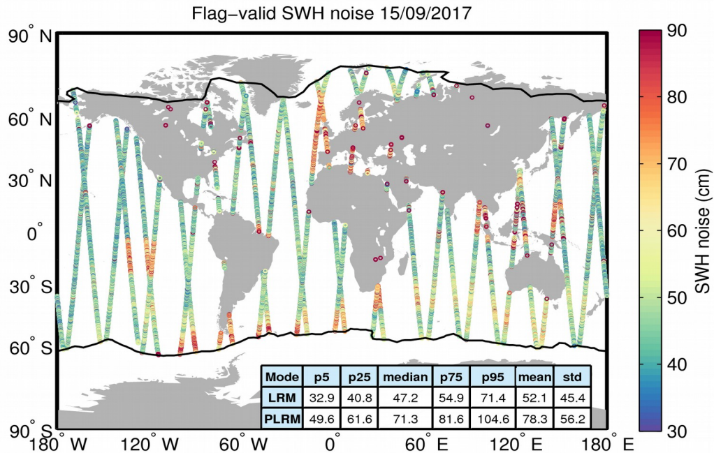
Figure 18. Geographical distribution of flag-valid 20-Hz SWH measurement noise over oceans and lakes for 15/09/2017. The statistical values shown in the table refer to the SWH noise and are calculated separately for LRM and PLRM regions. Measurements taken over polar polygons have been excluded from the computation of the statistical values. The black lines mark the outer limit of the Arctic and Antarctic polar polygons.
