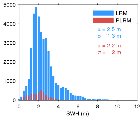
Figure 20. Histogram of science-valid SWH over oceans and lakes for LRM (blue) and PLRM (red) for 15/09/2017. The mean ( \mu ) and standard deviation ( \sigma ) are also shown. Note that values larger than 12 m are excluded from the histogram for the sake of readability but not from the computation of \mu and \sigma .
