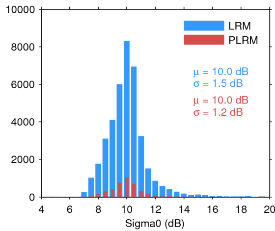
Figure 28. Histogram of science-valid sigma0 over oceans and lakes for LRM (blue) and PLRM (red) for 15/09/2017. The mean ( \mu ) and standard deviation ( \sigma ) are also shown. Note that values outside [4 20] dB are excluded from the histogram for the sake of readability but not from the computation of \mu and \sigma .
