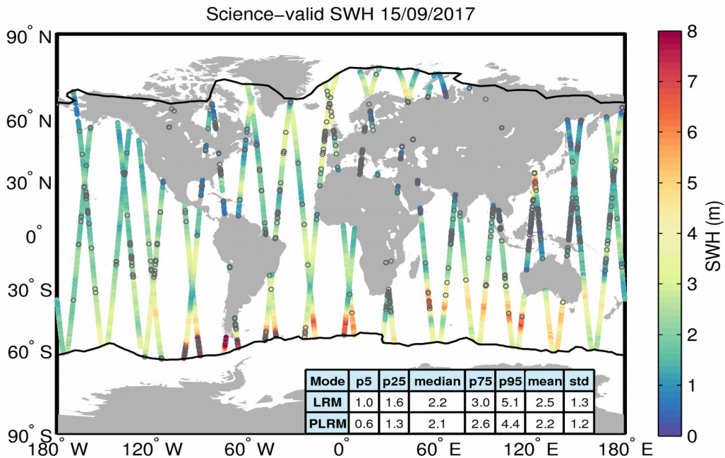
Figure 19. Geographical distribution of science-valid SWH data over oceans and lakes for 15/09/2017. The statistical values shown in the table refer to the SWH in m and are calculated separately for LRM and PLRM regions. The black lines mark the outer limit of the Arctic and Antarctic polar polygons. Gray circles denote records that have been rejected based on the editing criteria described in Table 3.
