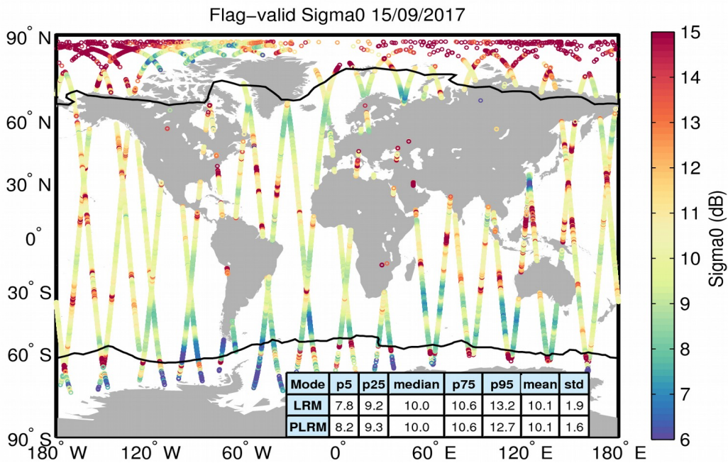
Figure 23. Geographical distribution of flag-valid sigma0 data over oceans and lakes for 15/09/2017. The statistical values shown in the table refer to the sigma0 in dB and are calculated separately for LRM and PLRM regions. Measurements taken over polar polygons have been excluded from the computation of the statistical values. The black lines mark the outer limit of the Arctic and Antarctic polar polygons.
