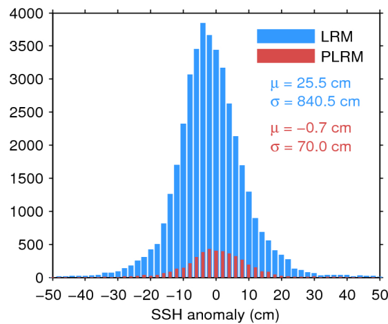
Figure 7. Histogram of flag-valid SSH anomaly over oceans and lakes for LRM (blue) and PLRM (red) for 15/09/2017. The mean ( \mu ) and standard deviation ( \sigma ) are also shown. Note that values outside [-50\ 50] cm are excluded from the histogram for the sake of readability but not from the computation of \mu and \sigma .
