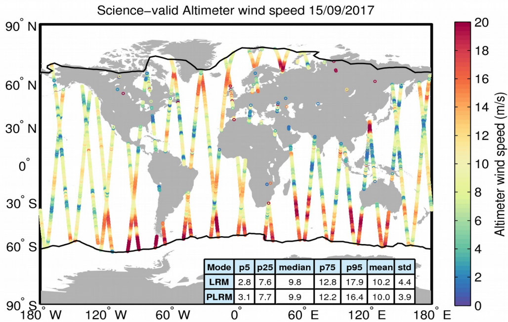
Figure 34. Geographical distribution of science-valid wind data over oceans and lakes for 15/09/2017. The statistical values shown in the table refer to the wind in m/s and are calculated separately for LRM and PLRM regions. The black lines mark the outer limit of the Arctic and Antarctic polar polygons. Gray circles denote records that have been rejected based on the editing criteria described in Table 5.
