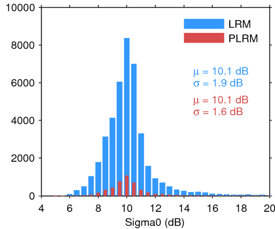
Figure 25. Histogram of flag-valid sigma0 over oceans and lakes for LRM (blue) and PLRM (red) for 15/09/2017. The mean ( \mu ) and standard deviation ( \sigma ) are also shown. Note that values outside [4 20] dB are excluded from the histogram for the sake of readability but not from the computation of \mu and \sigma .
