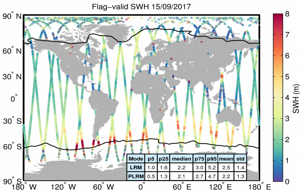
Figure 15. Geographical distribution of flag-valid SWH data over oceans and lakes for 15/09/2017. The statistical values shown in the table refer to the SWH in m and are calculated separately for LRM and PLRM regions. Measurements taken over polar polygons have been excluded from the computation of the statistical values. The black lines mark the outer limit of the Arctic and Antarctic polar polygons.
