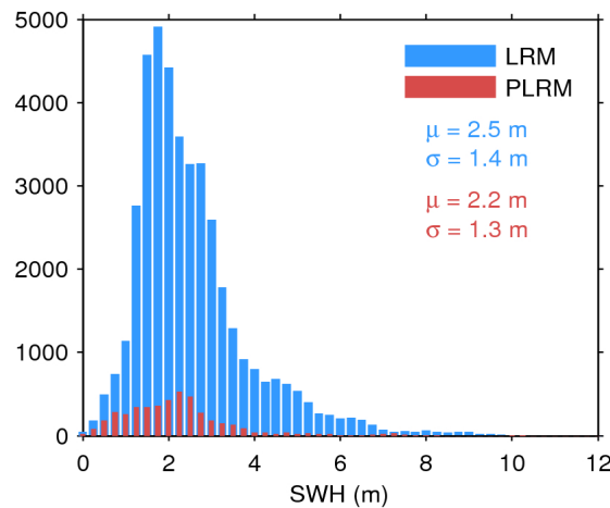
Figure 17. Histogram of flag-valid SWH over oceans and lakes for LRM (blue) and PLRM (red) for 15/09/2017. The mean ( \mu ) and standard deviation ( \sigma ) are also shown. Note that values larger than 12 m are excluded from the histogram for the sake of readability but not from the computation of \mu and \sigma .
