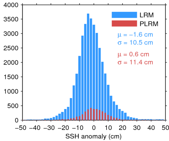
Figure 11. Histogram of science-valid SSH anomaly over oceans and lakes for LRM (blue) and PLRM (red) for 15/09/2017. The mean ( \mu ) and standard deviation ( \sigma ) are also shown. Note that values outside [-50 50] cm are excluded from the histogram for the sake of readability but not from the computation of \mu and \sigma .
