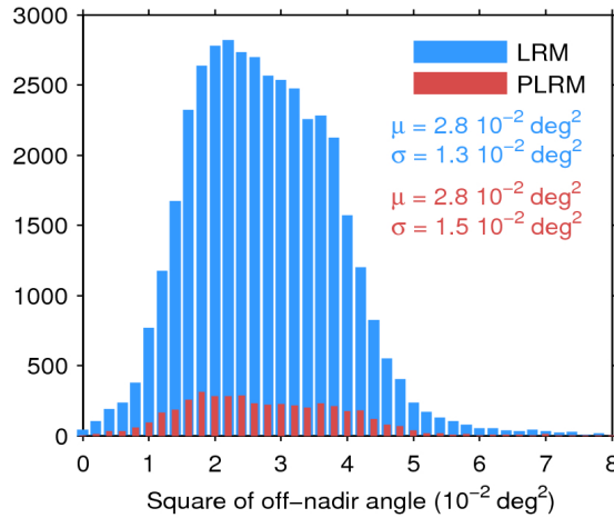
Figure 39. Histogram of flag-valid mispointing over oceans and lakes for LRM (blue) and PLRM (red) for 15/09/2017. Only positive values have been considered. The mean ( \mu ) and standard deviation ( \sigma ) are also shown. Note that values larger than 8 \cdot 10^{-2} \text{ deg}^2 are excluded from the histogram for the sake of readability but not from the computation of \mu and \sigma .
