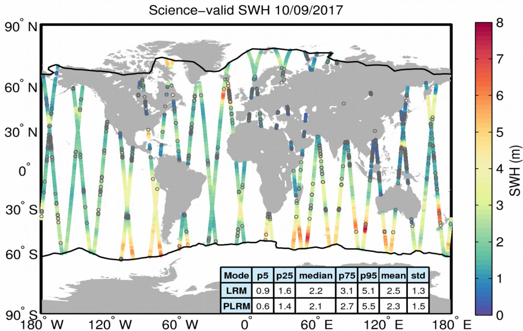
Figure 19. Geographical distribution of science-valid SWH data over oceans and lakes for 10/09/2017. The statistical values shown in the table refer to the SWH in m and are calculated separately for LRM and PLRM regions. The black lines mark the outer limit of the Arctic and Antarctic polar polygons. Gray circles denote records that have been rejected based on the editing criteria described in Table 3.
