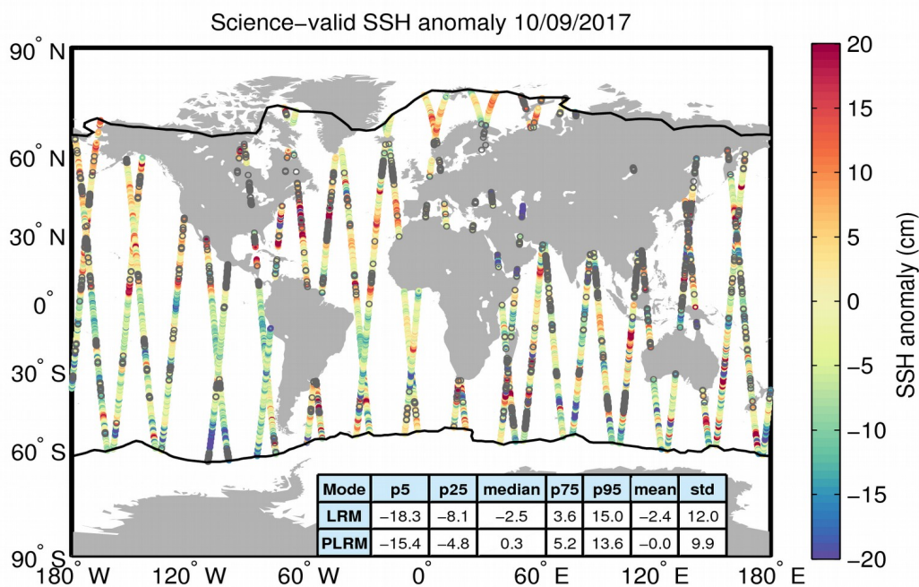
Figure 10. Geographical distribution of science-valid SSH anomaly data over oceans and lakes for 10/09/2017. The statistical values shown in the table refer to the SSH anomaly in cm and are calculated separately for LRM and PLRM regions. The black lines mark the outer limit of the Arctic and Antarctic polar polygons. Gray circles denote records that have been rejected based on the editing criteria described in Table 2.
