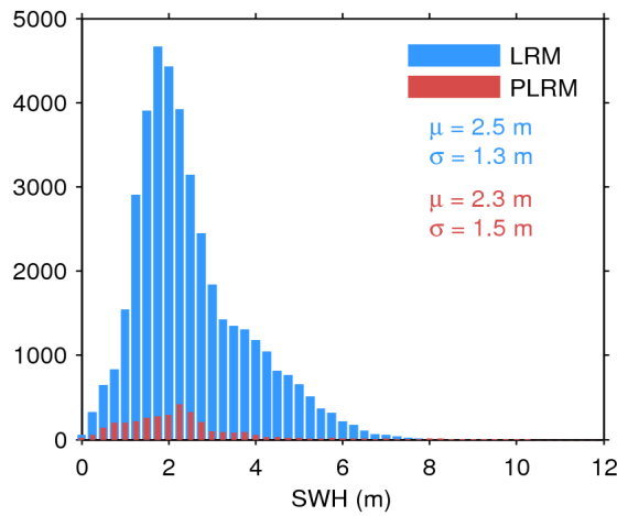
Figure 20. Histogram of science-valid SWH over oceans and lakes for LRM (blue) and PLRM (red) for 10/09/2017. The mean ( \mu ) and standard deviation ( \sigma ) are also shown. Note that values larger than 12 m are excluded from the histogram for the sake of readability but not from the computation of \mu and \sigma .
