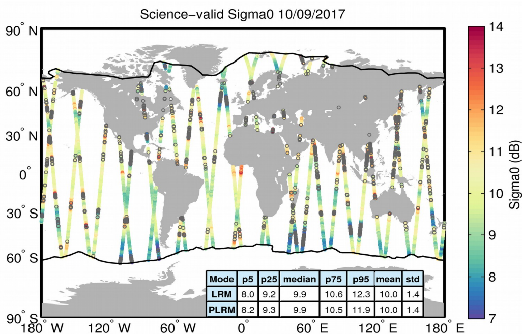
Figure 27. Geographical distribution of science-valid sigma0 data over oceans and lakes for 10/09/2017. The statistical values shown in the table refer to the sigma0 in dB and are calculated separately for LRM and PLRM regions. The black lines mark the outer limit of the Arctic and Antarctic polar polygons. Gray circles denote records that have been rejected based on the editing criteria described in Table 4.
