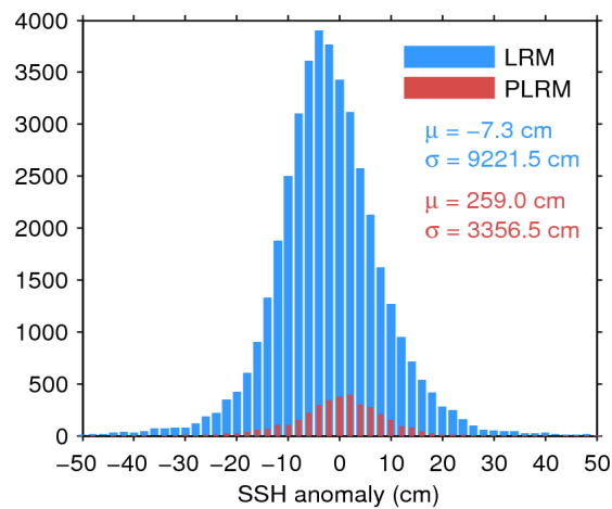
Figure 7. Histogram of flag-valid SSH anomaly over oceans and lakes for LRM (blue) and PLRM (red) for 10/09/2017. The mean ( \mu ) and standard deviation ( \sigma ) are also shown. Note that values outside [-50\ 50] cm are excluded from the histogram for the sake of readability but not from the computation of \mu and \sigma .
