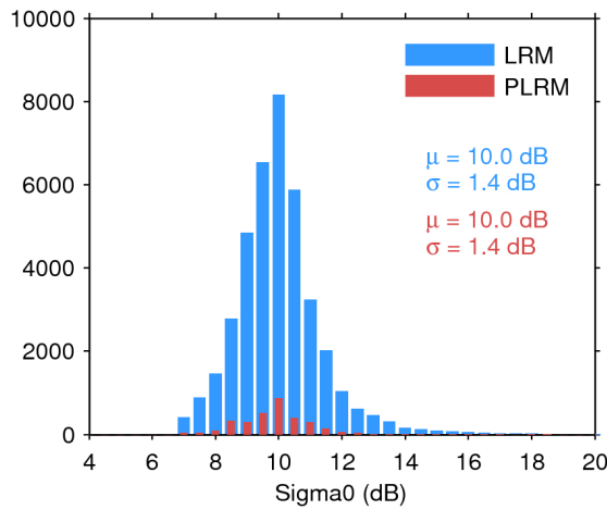
Figure 28. Histogram of science-valid sigma0 over oceans and lakes for LRM (blue) and PLRM (red) for 10/09/2017. The mean ( \mu ) and standard deviation ( \sigma ) are also shown. Note that values outside [4 20] dB are excluded from the histogram for the sake of readability but not from the computation of \mu and \sigma .
