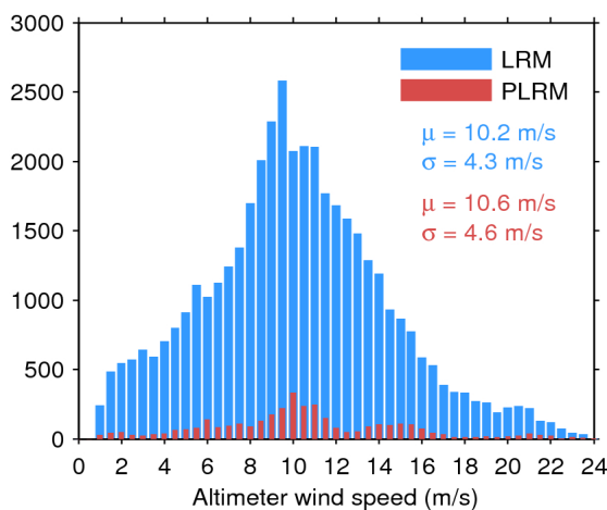
Figure 33. Histogram of flag-valid wind over oceans and lakes for LRM (blue) and PLRM (red) for 10/09/2017. The mean ( \mu ) and standard deviation ( \sigma ) are also shown. Note that values larger than 24 m/s are excluded from the histogram for the sake of readability but not from the computation of \mu and \sigma .
