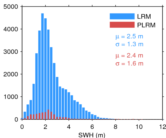
Figure 17. Histogram of flag-valid SWH over oceans and lakes for LRM (blue) and PLRM (red) for 10/09/2017. The mean ( \mu ) and standard deviation ( \sigma ) are also shown. Note that values larger than 12 m are excluded from the histogram for the sake of readability but not from the computation of \mu and \sigma .
