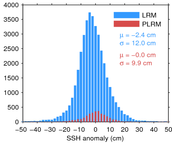
Figure 11. Histogram of science-valid SSH anomaly over oceans and lakes for LRM (blue) and PLRM (red) for 10/09/2017. The mean ( \mu ) and standard deviation ( \sigma ) are also shown. Note that values outside [-50 50] cm are excluded from the histogram for the sake of readability but not from the computation of \mu and \sigma .
