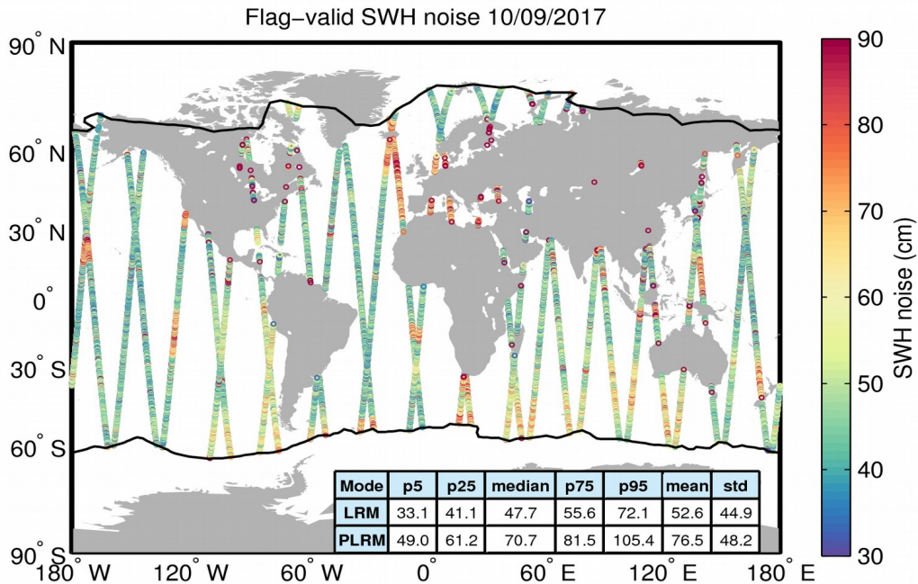
Figure 18. Geographical distribution of flag-valid 20-Hz SWH measurement noise over oceans and lakes for 10/09/2017. The statistical values shown in the table refer to the SWH noise and are calculated separately for LRM and PLRM regions. Measurements taken over polar polygons have been excluded from the computation of the statistical values. The black lines mark the outer limit of the Arctic and Antarctic polar polygons.
