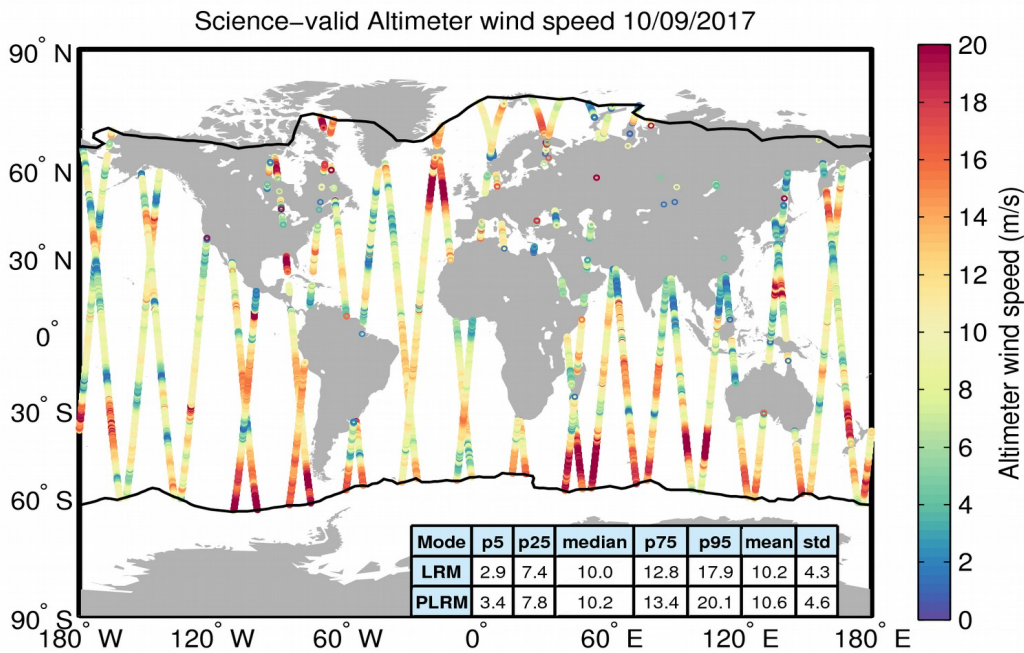
Figure 34. Geographical distribution of science-valid wind data over oceans and lakes for 10/09/2017. The statistical values shown in the table refer to the wind in m/s and are calculated separately for LRM and PLRM regions. The black lines mark the outer limit of the Arctic and Antarctic polar polygons. Gray circles denote records that have been rejected based on the editing criteria described in Table 5.
