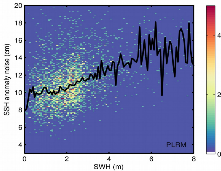
Figure 9. 2D histogram showing flag-valid SSH anomaly noise as a function of SWH for LRM (top) and PLRM (bottom) for 10/09/2017. The black line denotes the median SSH anomaly noise as a function of SWH.
