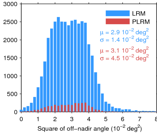
Figure 39. Histogram of flag-valid mispointing over oceans and lakes for LRM (blue) and PLRM (red) for 10/09/2017. Only positive values have been considered. The mean ( \mu ) and standard deviation ( \sigma ) are also shown. Note that values larger than 8 \cdot 10^{-2} \text{ deg}^2 are excluded from the histogram for the sake of readability but not from the computation of \mu and \sigma .
