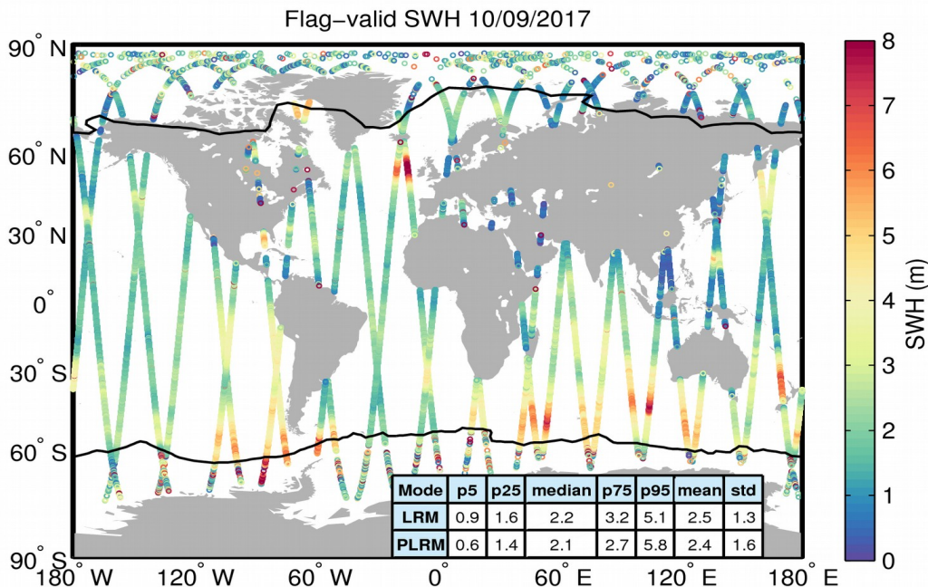
Figure 15. Geographical distribution of flag-valid SWH data over oceans and lakes for 10/09/2017. The statistical values shown in the table refer to the SWH in m and are calculated separately for LRM and PLRM regions. Measurements taken over polar polygons have been excluded from the computation of the statistical values. The black lines mark the outer limit of the Arctic and Antarctic polar polygons.
