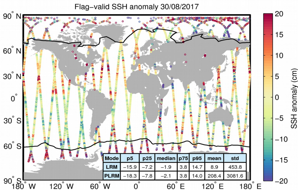
Figure 5. Geographical distribution of flag-valid 1-Hz SSH anomaly data over oceans and lakes for 30/08/2017. The statistical values shown in the table refer to the SSH anomaly in cm and are calculated separately for LRM and PLRM regions. Measurements taken over polar polygons have been excluded from the computation of the statistical values. The black lines mark the outer limit of the Arctic and Antarctic polar polygons.
