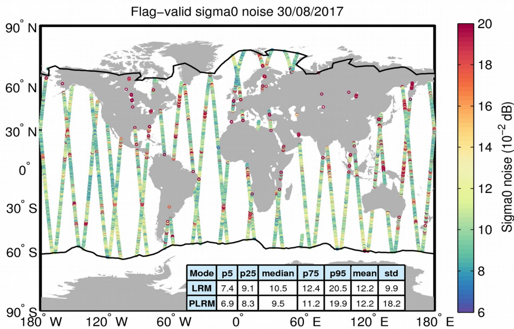
Figure 26. Geographical distribution of flag-valid 20-Hz sigma0 measurement noise over oceans and lakes for 30/08/2017. The statistical values shown in the table refer to the sigma0 noise and are calculated separately for LRM and PLRM regions. Measurements taken over polar polygons have been excluded from the computation of the statistical values. The black lines mark the outer limit of the Arctic and Antarctic polar polygons.
