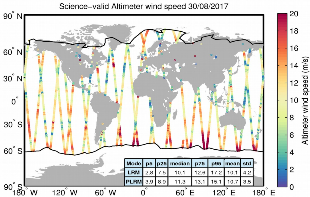
Figure 34. Geographical distribution of science-valid wind data over oceans and lakes for 30/08/2017. The statistical values shown in the table refer to the wind in m/s and are calculated separately for LRM and PLRM regions. The black lines mark the outer limit of the Arctic and Antarctic polar polygons. Gray circles denote records that have been rejected based on the editing criteria described in Table 5.
