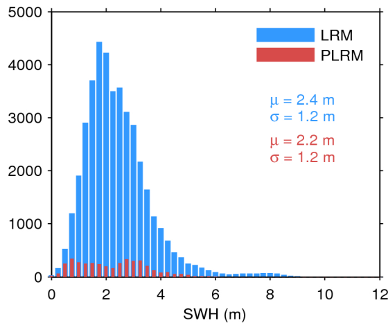
Figure 20. Histogram of science-valid SWH over oceans and lakes for LRM (blue) and PLRM (red) for 30/08/2017. The mean ( \mu ) and standard deviation ( \sigma ) are also shown. Note that values larger than 12 m are excluded from the histogram for the sake of readability but not from the computation of \mu and \sigma .
