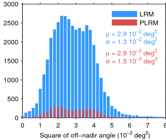
Figure 39. Histogram of flag-valid mispointing over oceans and lakes for LRM (blue) and PLRM (red) for 30/08/2017. Only positive values have been considered. The mean ( \mu ) and standard deviation ( \sigma ) are also shown. Note that values larger than 8 \cdot 10^{-2} \text{ deg}^2 are excluded from the histogram for the sake of readability but not from the computation of \mu and \sigma .
