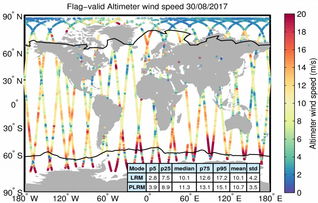
Figure 31. Geographical distribution of flag-valid wind data over oceans and lakes for 30/08/2017. The statistical values shown in the table refer to the wind in m/s and are calculated separately for LRM and PLRM regions. Measurements taken over polar polygons have been excluded from the computation of the statistical values. The black lines mark the outer limit of the Arctic and Antarctic polar polygons.
