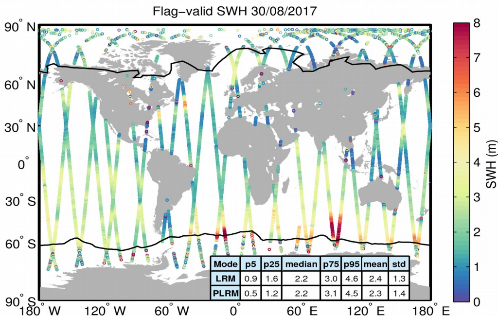
Figure 15. Geographical distribution of flag-valid SWH data over oceans and lakes for 30/08/2017. The statistical values shown in the table refer to the SWH in m and are calculated separately for LRM and PLRM regions. Measurements taken over polar polygons have been excluded from the computation of the statistical values. The black lines mark the outer limit of the Arctic and Antarctic polar polygons.
