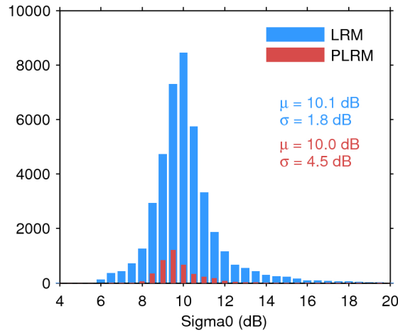
Figure 25. Histogram of flag-valid sigma0 over oceans and lakes for LRM (blue) and PLRM (red) for 30/08/2017. The mean ( \mu ) and standard deviation ( \sigma ) are also shown. Note that values outside [4 20] dB are excluded from the histogram for the sake of readability but not from the computation of \mu and \sigma .
