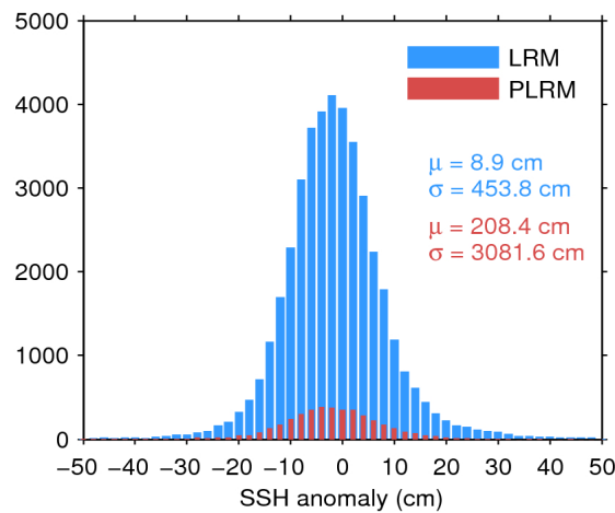
Figure 7. Histogram of flag-valid SSH anomaly over oceans and lakes for LRM (blue) and PLRM (red) for 30/08/2017. The mean ( \mu ) and standard deviation ( \sigma ) are also shown. Note that values outside [-50 50] cm are excluded from the histogram for the sake of readability but not from the computation of \mu and \sigma .
