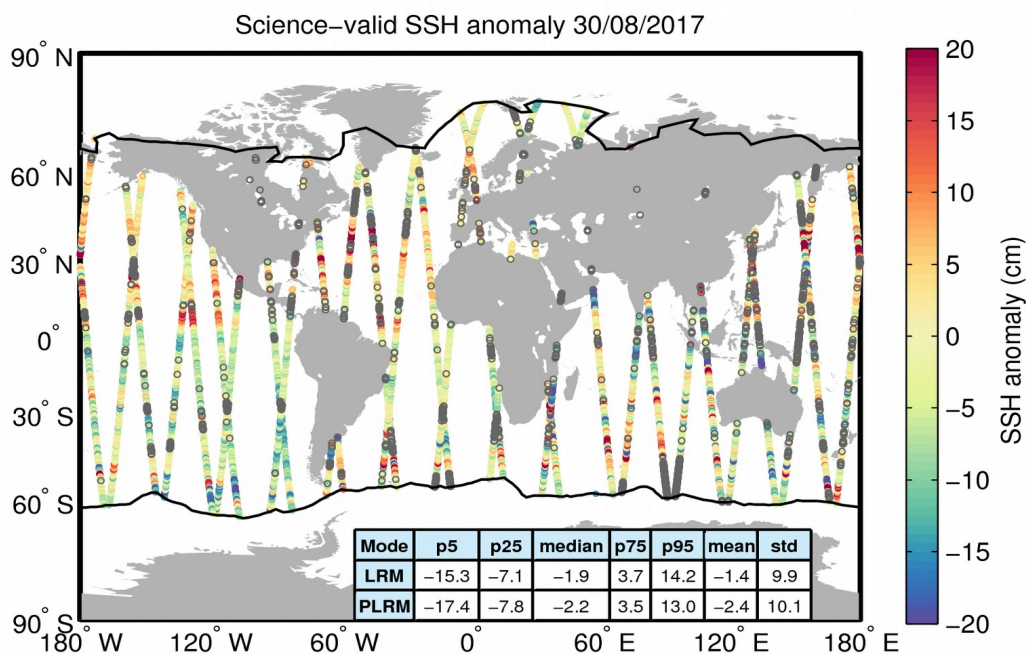
Figure 10. Geographical distribution of science-valid SSH anomaly data over oceans and lakes for 30/08/2017. The statistical values shown in the table refer to the SSH anomaly in cm and are calculated separately for LRM and PLRM regions. The black lines mark the outer limit of the Arctic and Antarctic polar polygons. Gray circles denote records that have been rejected based on the editing criteria described in Table 2.
