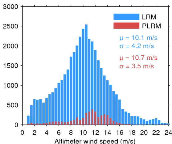
Figure 33. Histogram of flag-valid wind over oceans and lakes for LRM (blue) and PLRM (red) for 30/08/2017. The mean ( \mu ) and standard deviation ( \sigma ) are also shown. Note that values larger than 24 m/s are excluded from the histogram for the sake of readability but not from the computation of \mu and \sigma .
