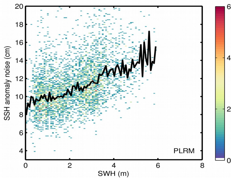
Figure 9. 2D histogram showing flag-valid SSH anomaly noise as a function of SWH for LRM (top) and PLRM (bottom) for 30/08/2017. The black line denotes the median SSH anomaly noise as a function of SWH.
