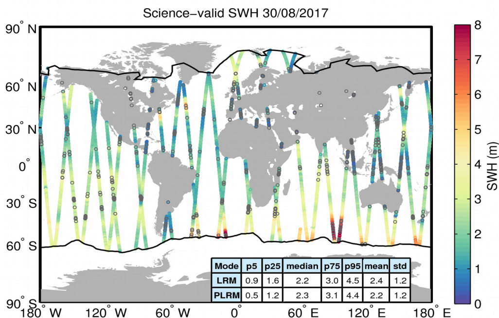
Figure 19. Geographical distribution of science-valid SWH data over oceans and lakes for 30/08/2017. The statistical values shown in the table refer to the SWH in m and are calculated separately for LRM and PLRM regions. The black lines mark the outer limit of the Arctic and Antarctic polar polygons. Gray circles denote records that have been rejected based on the editing criteria described in Table 3.
