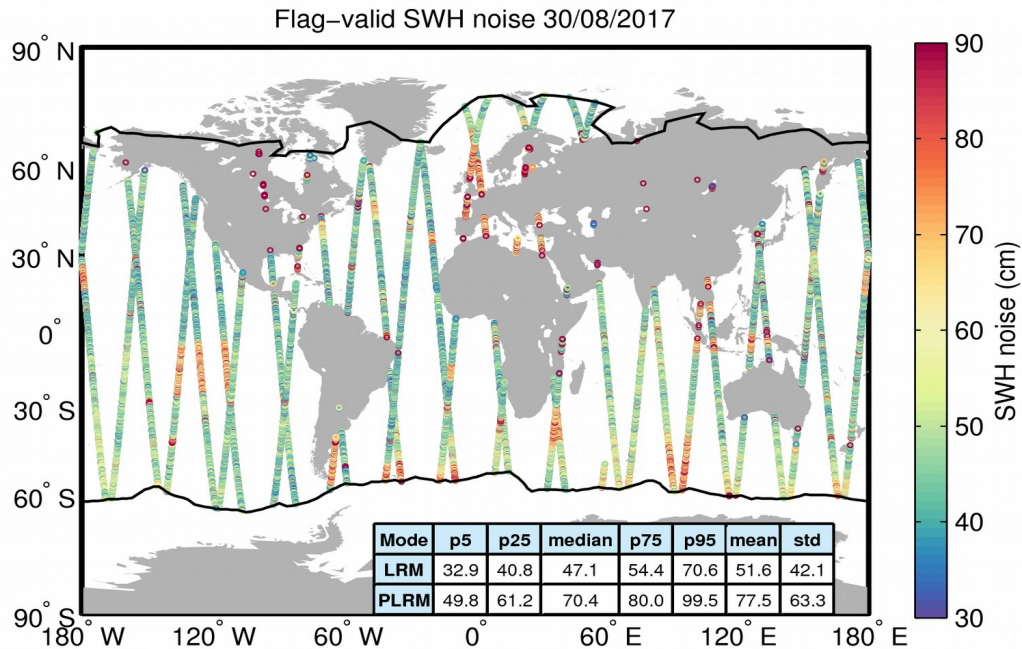
Figure 18. Geographical distribution of flag-valid 20-Hz SWH measurement noise over oceans and lakes for 30/08/2017. The statistical values shown in the table refer to the SWH noise and are calculated separately for LRM and PLRM regions. Measurements taken over polar polygons have been excluded from the computation of the statistical values. The black lines mark the outer limit of the Arctic and Antarctic polar polygons.
