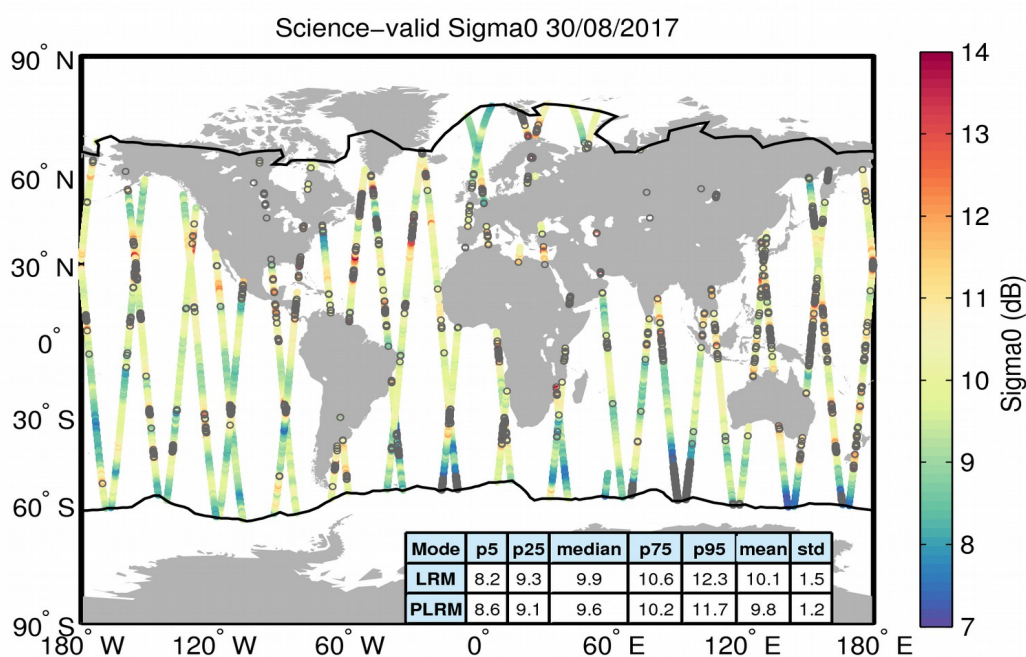
Figure 27. Geographical distribution of science-valid sigma0 data over oceans and lakes for 30/08/2017. The statistical values shown in the table refer to the sigma0 in dB and are calculated separately for LRM and PLRM regions. The black lines mark the outer limit of the Arctic and Antarctic polar polygons. Gray circles denote records that have been rejected based on the editing criteria described in Table 4.
