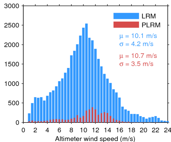
Figure 35. Histogram of science-valid wind over oceans and lakes for LRM (blue) and PLRM (red) for 30/08/2017. The mean ( \mu ) and standard deviation ( \sigma ) are also shown. Note that values larger than 24 m/s are excluded from the histogram for the sake of readability but not from the computation of \mu and \sigma .
