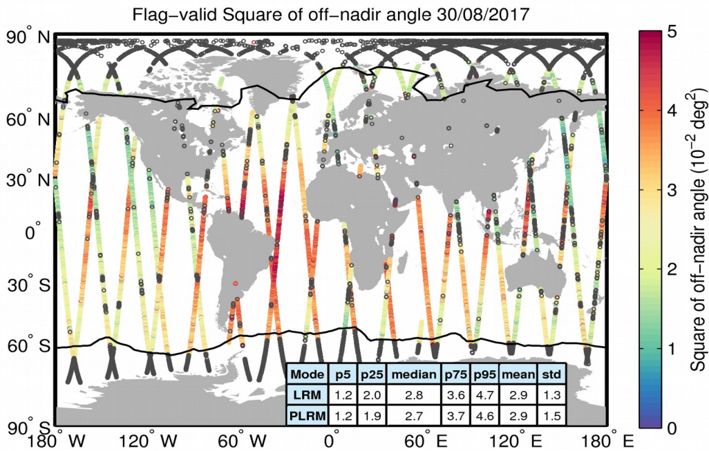
Figure 37. Geographical distribution of flag-valid mispointing data over oceans and lakes for 30/08/2017. The statistical values shown in the table refer to the mispointing in 10^{-2} deg 2 and are calculated separately for LRM and PLRM regions. Measurements taken over polar polygons have been excluded from the computation of the statistical values. The black lines mark the outer limit of the Arctic and Antarctic polar polygons. Gray circles denote negative values.
