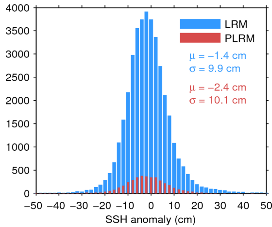
Figure 11. Histogram of science-valid SSH anomaly over oceans and lakes for LRM (blue) and PLRM (red) for 30/08/2017. The mean ( \mu ) and standard deviation ( \sigma ) are also shown. Note that values outside [-50 50] cm are excluded from the histogram for the sake of readability but not from the computation of \mu and \sigma .
