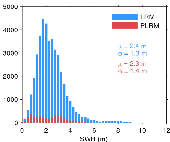
Figure 17. Histogram of flag-valid SWH over oceans and lakes for LRM (blue) and PLRM (red) for 30/08/2017. The mean ( \mu ) and standard deviation ( \sigma ) are also shown. Note that values larger than 12 m are excluded from the histogram for the sake of readability but not from the computation of \mu and \sigma .
