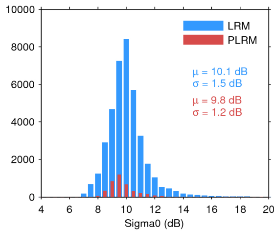
Figure 28. Histogram of science-valid sigma0 over oceans and lakes for LRM (blue) and PLRM (red) for 30/08/2017. The mean ( \mu ) and standard deviation ( \sigma ) are also shown. Note that values outside [4 20] dB are excluded from the histogram for the sake of readability but not from the computation of \mu and \sigma .
