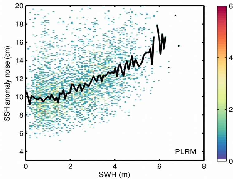
Figure 9. 2D histogram showing flag-valid SSH anomaly noise as a function of SWH for LRM (top) and PLRM (bottom) for 29/08/2017. The black line denotes the median SSH anomaly noise as a function of SWH.
