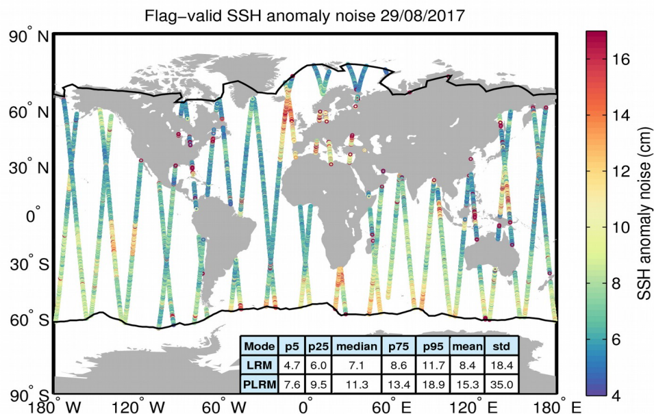
Figure 8. Geographical distribution of flag-valid 20-Hz SSH anomaly measurement noise over oceans and lakes for 29/08/2017. The statistical values shown in the table refer to the SSH anomaly noise and are calculated separately for LRM and PLRM regions. Measurements taken over polar polygons have been excluded from the computation of the statistical values. The black lines mark the outer limit of the Arctic and Antarctic polar polygons.
