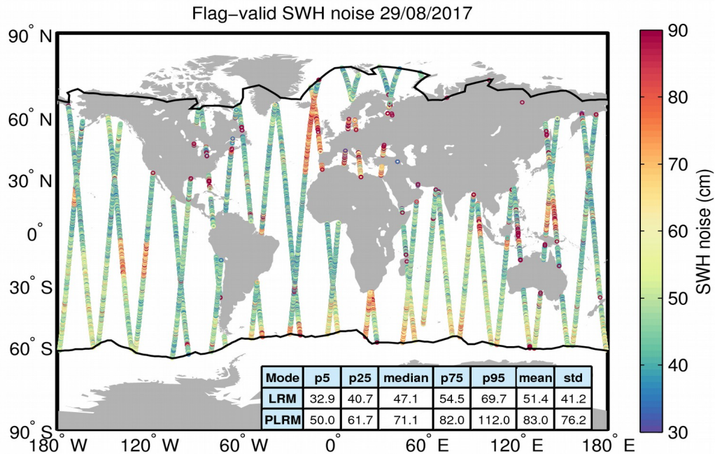
Figure 18. Geographical distribution of flag-valid 20-Hz SWH measurement noise over oceans and lakes for 29/08/2017. The statistical values shown in the table refer to the SWH noise and are calculated separately for LRM and PLRM regions. Measurements taken over polar polygons have been excluded from the computation of the statistical values. The black lines mark the outer limit of the Arctic and Antarctic polar polygons.
