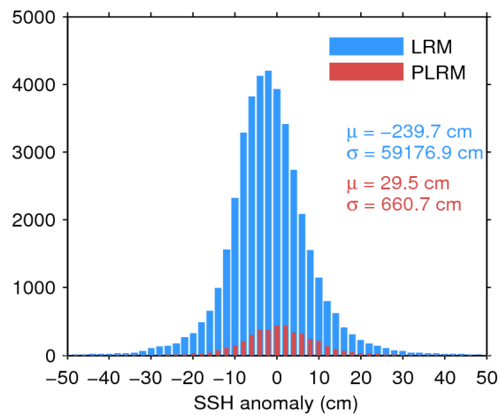
Figure 7. Histogram of flag-valid SSH anomaly over oceans and lakes for LRM (blue) and PLRM (red) for 29/08/2017. The mean ( \mu ) and standard deviation ( \sigma ) are also shown. Note that values outside [-50 50] cm are excluded from the histogram for the sake of readability but not from the computation of \mu and \sigma .
