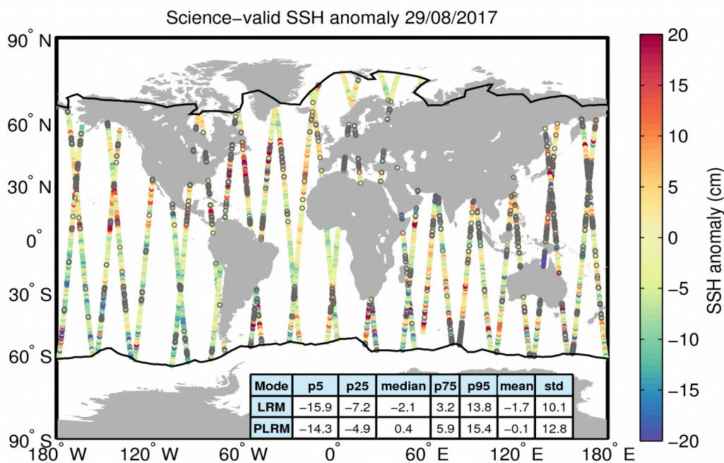
Figure 10. Geographical distribution of science-valid SSH anomaly data over oceans and lakes for 29/08/2017. The statistical values shown in the table refer to the SSH anomaly in cm and are calculated separately for LRM and PLRM regions. The black lines mark the outer limit of the Arctic and Antarctic polar polygons. Gray circles denote records that have been rejected based on the editing criteria described in Table 2.
