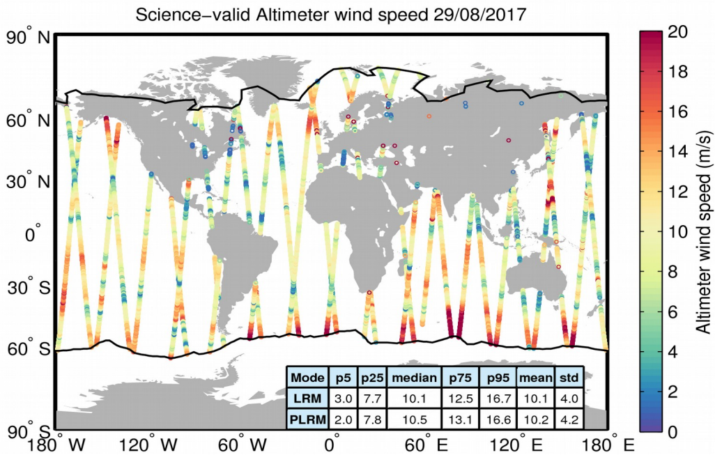
Figure 34. Geographical distribution of science-valid wind data over oceans and lakes for 29/08/2017. The statistical values shown in the table refer to the wind in m/s and are calculated separately for LRM and PLRM regions. The black lines mark the outer limit of the Arctic and Antarctic polar polygons. Gray circles denote records that have been rejected based on the editing criteria described in Table 5.
