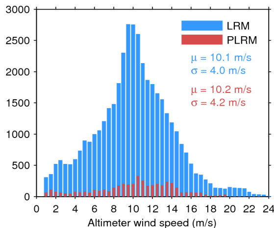
Figure 35. Histogram of science-valid wind over oceans and lakes for LRM (blue) and PLRM (red) for 29/08/2017. The mean ( \mu ) and standard deviation ( \sigma ) are also shown. Note that values larger than 24 m/s are excluded from the histogram for the sake of readability but not from the computation of \mu and \sigma .
