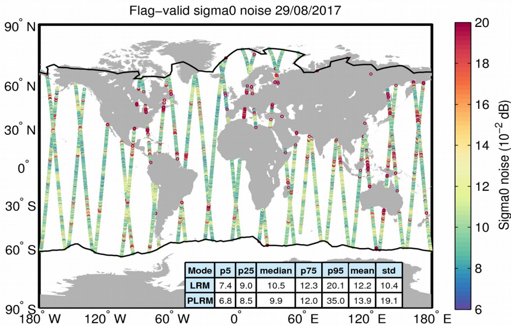
Figure 26. Geographical distribution of flag-valid 20-Hz sigma0 measurement noise over oceans and lakes for 29/08/2017. The statistical values shown in the table refer to the sigma0 noise and are calculated separately for LRM and PLRM regions. Measurements taken over polar polygons have been excluded from the computation of the statistical values. The black lines mark the outer limit of the Arctic and Antarctic polar polygons.
