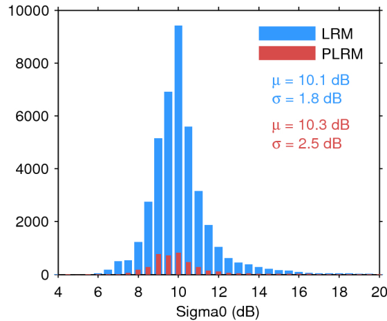
Figure 25. Histogram of flag-valid sigma0 over oceans and lakes for LRM (blue) and PLRM (red) for 29/08/2017. The mean ( \mu ) and standard deviation ( \sigma ) are also shown. Note that values outside [4 20] dB are excluded from the histogram for the sake of readability but not from the computation of \mu and \sigma .
