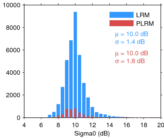
Figure 28. Histogram of science-valid sigma0 over oceans and lakes for LRM (blue) and PLRM (red) for 29/08/2017. The mean ( \mu ) and standard deviation ( \sigma ) are also shown. Note that values outside [4 20] dB are excluded from the histogram for the sake of readability but not from the computation of \mu and \sigma .
