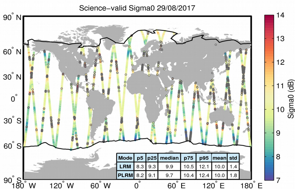
Figure 27. Geographical distribution of science-valid sigma0 data over oceans and lakes for 29/08/2017. The statistical values shown in the table refer to the sigma0 in dB and are calculated separately for LRM and PLRM regions. The black lines mark the outer limit of the Arctic and Antarctic polar polygons. Gray circles denote records that have been rejected based on the editing criteria described in Table 4.
