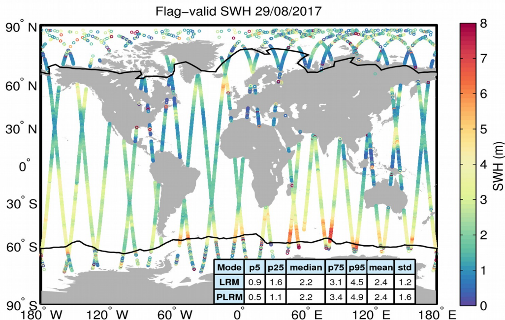
Figure 15. Geographical distribution of flag-valid SWH data over oceans and lakes for 29/08/2017. The statistical values shown in the table refer to the SWH in m and are calculated separately for LRM and PLRM regions. Measurements taken over polar polygons have been excluded from the computation of the statistical values. The black lines mark the outer limit of the Arctic and Antarctic polar polygons.
