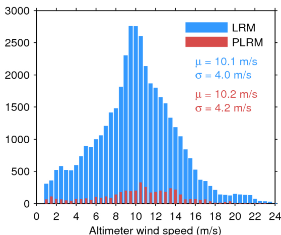
Figure 33. Histogram of flag-valid wind over oceans and lakes for LRM (blue) and PLRM (red) for 29/08/2017. The mean ( \mu ) and standard deviation ( \sigma ) are also shown. Note that values larger than 24 m/s are excluded from the histogram for the sake of readability but not from the computation of \mu and \sigma .
