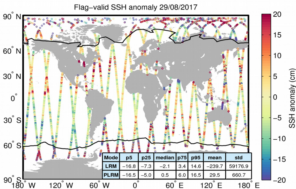
Figure 5. Geographical distribution of flag-valid 1-Hz SSH anomaly data over oceans and lakes for 29/08/2017. The statistical values shown in the table refer to the SSH anomaly in cm and are calculated separately for LRM and PLRM regions. Measurements taken over polar polygons have been excluded from the computation of the statistical values. The black lines mark the outer limit of the Arctic and Antarctic polar polygons.
