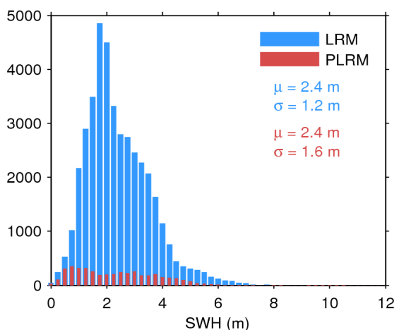
Figure 17. Histogram of flag-valid SWH over oceans and lakes for LRM (blue) and PLRM (red) for 29/08/2017. The mean ( \mu ) and standard deviation ( \sigma ) are also shown. Note that values larger than 12 m are excluded from the histogram for the sake of readability but not from the computation of \mu and \sigma .
