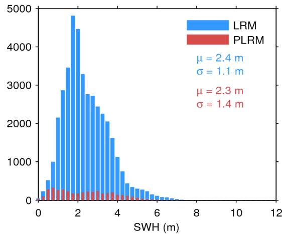
Figure 20. Histogram of science-valid SWH over oceans and lakes for LRM (blue) and PLRM (red) for 29/08/2017. The mean ( \mu ) and standard deviation ( \sigma ) are also shown. Note that values larger than 12 m are excluded from the histogram for the sake of readability but not from the computation of \mu and \sigma .
