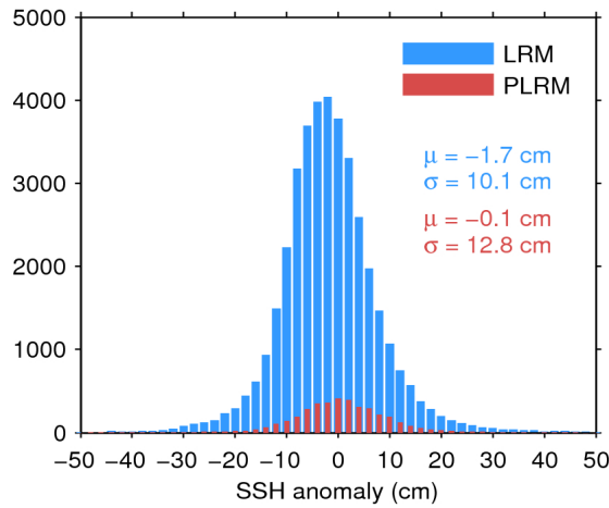
Figure 11. Histogram of science-valid SSH anomaly over oceans and lakes for LRM (blue) and PLRM (red) for 29/08/2017. The mean ( \mu ) and standard deviation ( \sigma ) are also shown. Note that values outside [-50 50] cm are excluded from the histogram for the sake of readability but not from the computation of \mu and \sigma .
