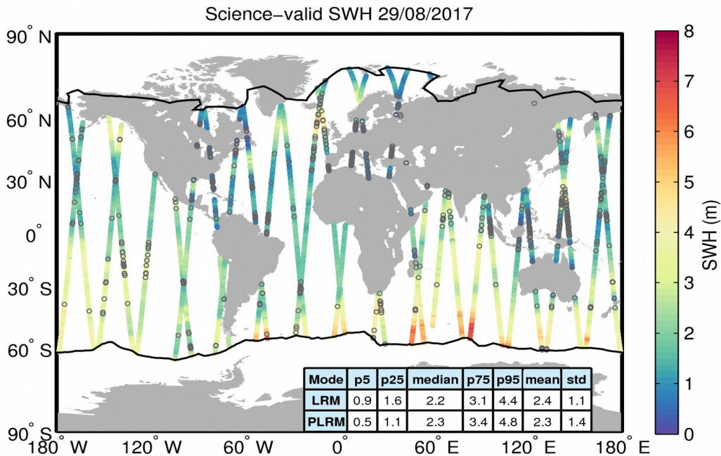
Figure 19. Geographical distribution of science-valid SWH data over oceans and lakes for 29/08/2017. The statistical values shown in the table refer to the SWH in m and are calculated separately for LRM and PLRM regions. The black lines mark the outer limit of the Arctic and Antarctic polar polygons. Gray circles denote records that have been rejected based on the editing criteria described in Table 3.
