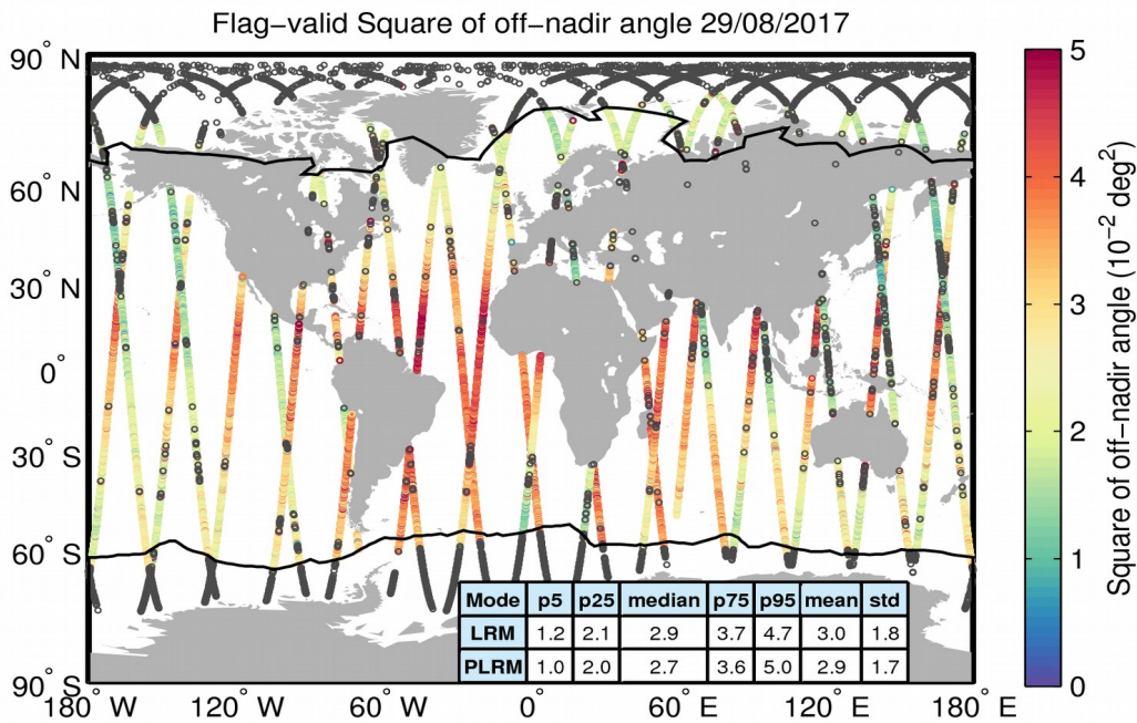
Figure 37. Geographical distribution of flag-valid mispointing data over oceans and lakes for 29/08/2017. The statistical values shown in the table refer to the mispointing in 10^{-2} \text{deg}^2 and are calculated separately for LRM and PLRM regions. Measurements taken over polar polygons have been excluded from the computation of the statistical values. The black lines mark the outer limit of the Arctic and Antarctic polar polygons. Gray circles denote negative values.
