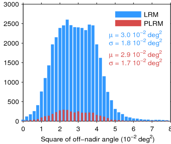
Figure 39. Histogram of flag-valid mispointing over oceans and lakes for LRM (blue) and PLRM (red) for 29/08/2017. Only positive values have been considered. The mean ( \mu ) and standard deviation ( \sigma ) are also shown. Note that values larger than 8 \cdot 10^{-2} \text{ deg}^2 are excluded from the histogram for the sake of readability but not from the computation of \mu and \sigma .
