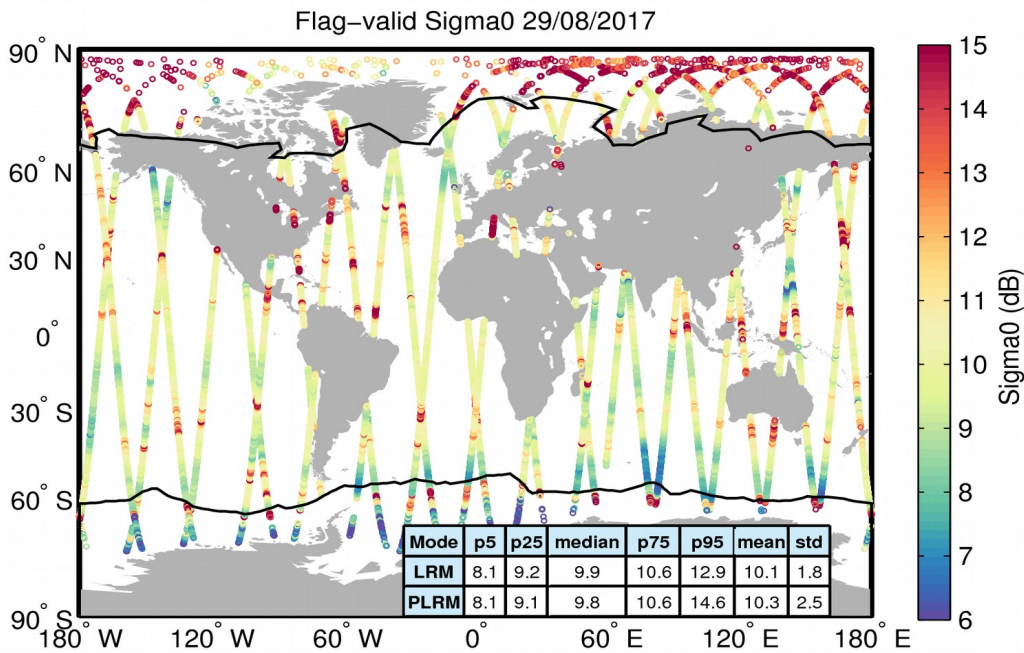
Figure 23. Geographical distribution of flag-valid sigma0 data over oceans and lakes for 29/08/2017. The statistical values shown in the table refer to the sigma0 in dB and are calculated separately for LRM and PLRM regions. Measurements taken over polar polygons have been excluded from the computation of the statistical values. The black lines mark the outer limit of the Arctic and Antarctic polar polygons.
