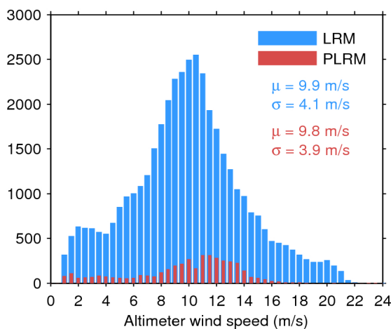
Figure 33. Histogram of flag-valid wind over oceans and lakes for LRM (blue) and PLRM (red) for 28/08/2017. The mean ( \mu ) and standard deviation ( \sigma ) are also shown. Note that values larger than 24 m/s are excluded from the histogram for the sake of readability but not from the computation of \mu and \sigma .
