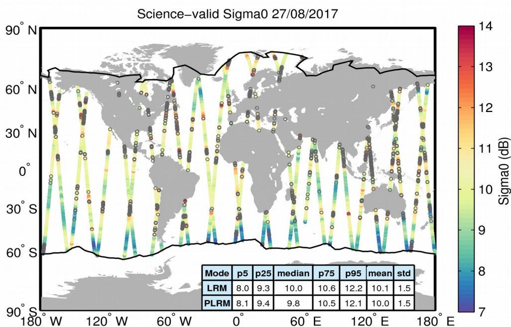
Figure 27. Geographical distribution of science-valid sigma0 data over oceans and lakes for 27/08/2017. The statistical values shown in the table refer to the sigma0 in dB and are calculated separately for LRM and PLRM regions. The black lines mark the outer limit of the Arctic and Antarctic polar polygons. Gray circles denote records that have been rejected based on the editing criteria described in Table 4.
