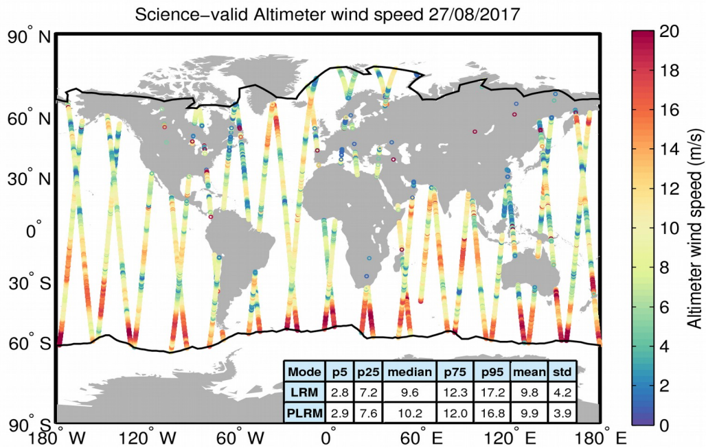
Figure 34. Geographical distribution of science-valid wind data over oceans and lakes for 27/08/2017. The statistical values shown in the table refer to the wind in m/s and are calculated separately for LRM and PLRM regions. The black lines mark the outer limit of the Arctic and Antarctic polar polygons. Gray circles denote records that have been rejected based on the editing criteria described in Table 5.
