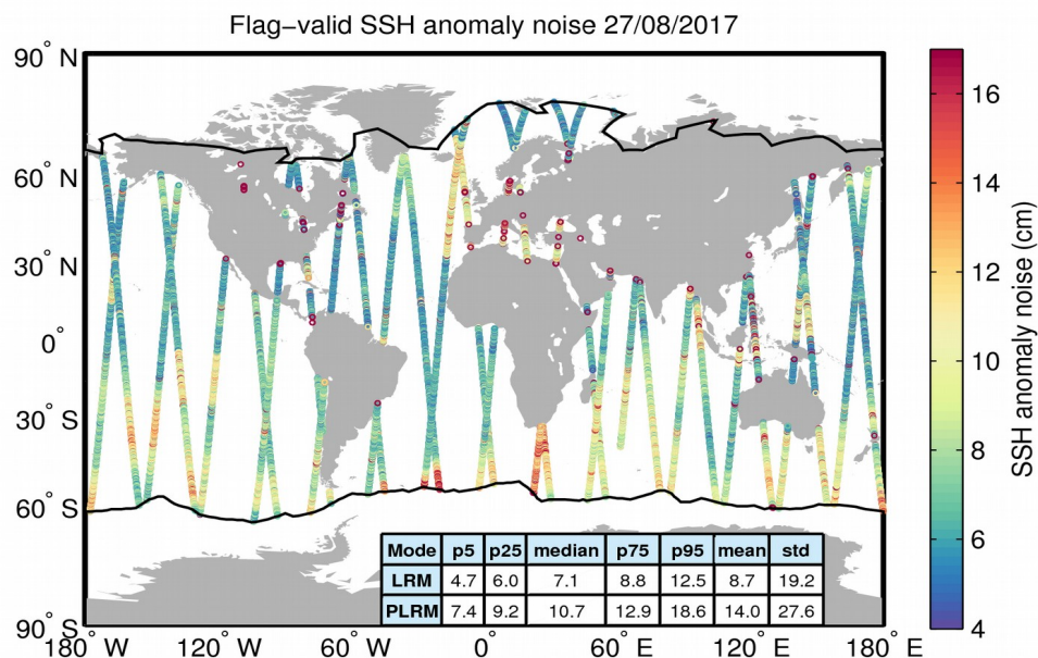
Figure 8. Geographical distribution of flag-valid 20-Hz SSH anomaly measurement noise over oceans and lakes for 27/08/2017. The statistical values shown in the table refer to the SSH anomaly noise and are calculated separately for LRM and PLRM regions. Measurements taken over polar polygons have been excluded from the computation of the statistical values. The black lines mark the outer limit of the Arctic and Antarctic polar polygons.
