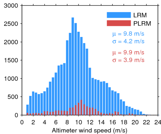
Figure 35. Histogram of science-valid wind over oceans and lakes for LRM (blue) and PLRM (red) for 27/08/2017. The mean ( \mu ) and standard deviation ( \sigma ) are also shown. Note that values larger than 24 m/s are excluded from the histogram for the sake of readability but not from the computation of \mu and \sigma .
