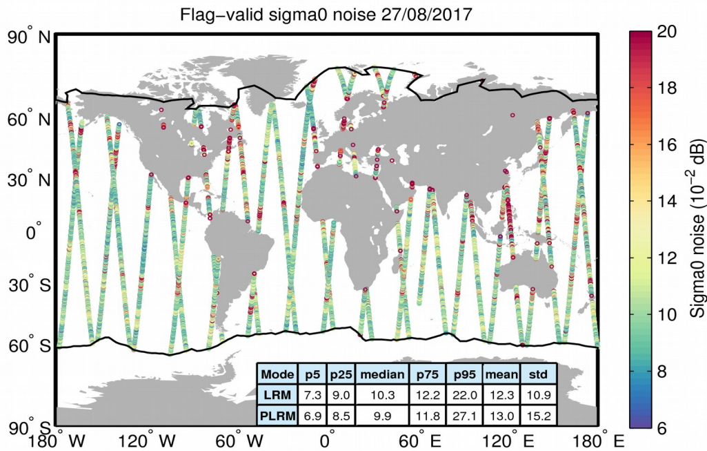
Figure 26. Geographical distribution of flag-valid 20-Hz sigma0 measurement noise over oceans and lakes for 27/08/2017. The statistical values shown in the table refer to the sigma0 noise and are calculated separately for LRM and PLRM regions. Measurements taken over polar polygons have been excluded from the computation of the statistical values. The black lines mark the outer limit of the Arctic and Antarctic polar polygons.
