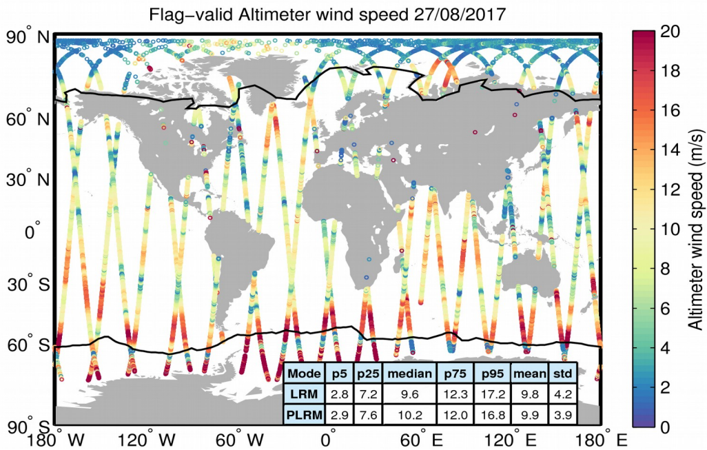
Figure 31. Geographical distribution of flag-valid wind data over oceans and lakes for 27/08/2017. The statistical values shown in the table refer to the wind in m/s and are calculated separately for LRM and PLRM regions. Measurements taken over polar polygons have been excluded from the computation of the statistical values. The black lines mark the outer limit of the Arctic and Antarctic polar polygons.
