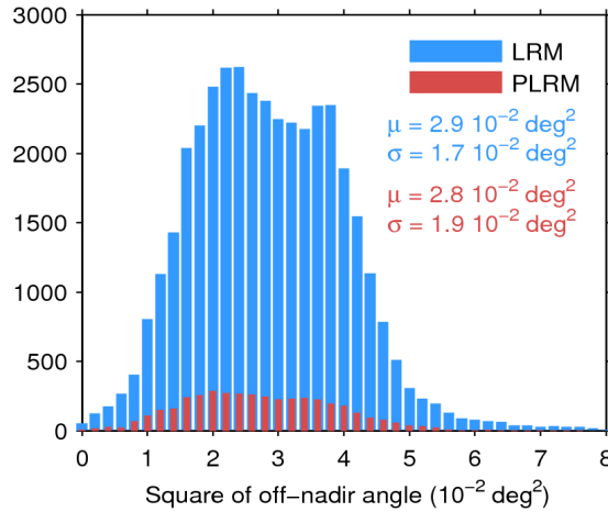
Figure 39. Histogram of flag-valid mispointing over oceans and lakes for LRM (blue) and PLRM (red) for 27/08/2017. Only positive values have been considered. The mean ( \mu ) and standard deviation ( \sigma ) are also shown. Note that values larger than 8 \cdot 10^{-2} \text{ deg}^2 are excluded from the histogram for the sake of readability but not from the computation of \mu and \sigma .
