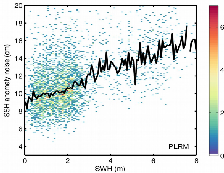
Figure 9. 2D histogram showing flag-valid SSH anomaly noise as a function of SWH for LRM (top) and PLRM (bottom) for 27/08/2017. The black line denotes the median SSH anomaly noise as a function of SWH.
