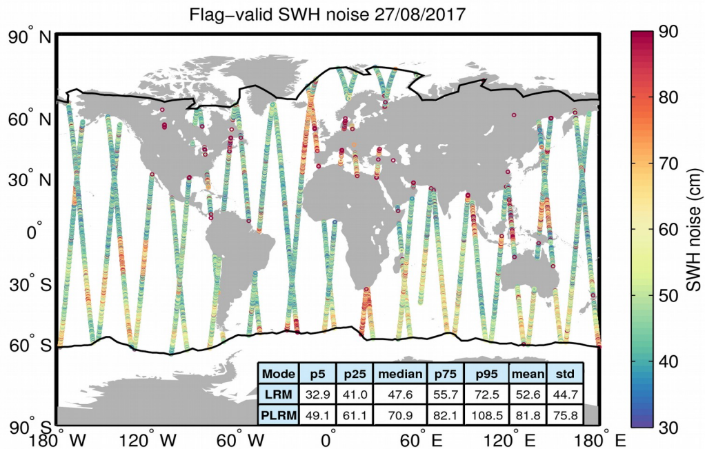
Figure 18. Geographical distribution of flag-valid 20-Hz SWH measurement noise over oceans and lakes for 27/08/2017. The statistical values shown in the table refer to the SWH noise and are calculated separately for LRM and PLRM regions. Measurements taken over polar polygons have been excluded from the computation of the statistical values. The black lines mark the outer limit of the Arctic and Antarctic polar polygons.
