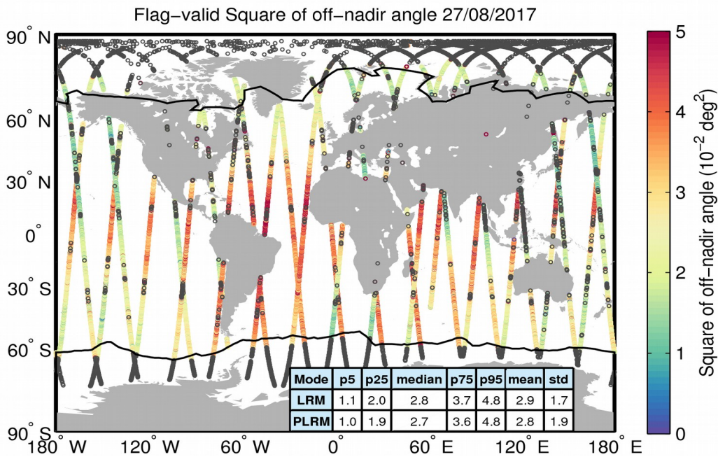
Figure 37. Geographical distribution of flag-valid mispointing data over oceans and lakes for 27/08/2017. The statistical values shown in the table refer to the mispointing in 10^{-2} deg 2 and are calculated separately for LRM and PLRM regions. Measurements taken over polar polygons have been excluded from the computation of the statistical values. The black lines mark the outer limit of the Arctic and Antarctic polar polygons. Gray circles denote negative values.
