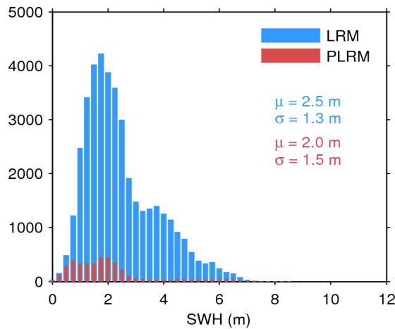
Figure 20. Histogram of science-valid SWH over oceans and lakes for LRM (blue) and PLRM (red) for 27/08/2017. The mean ( \mu ) and standard deviation ( \sigma ) are also shown. Note that values larger than 12 m are excluded from the histogram for the sake of readability but not from the computation of \mu and \sigma .
