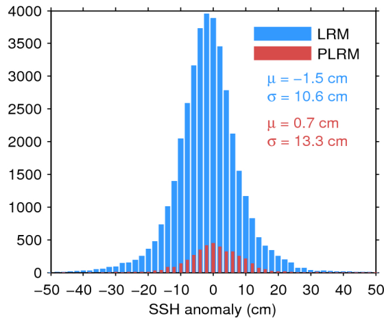
Figure 11. Histogram of science-valid SSH anomaly over oceans and lakes for LRM (blue) and PLRM (red) for 27/08/2017. The mean ( \mu ) and standard deviation ( \sigma ) are also shown. Note that values outside [-50\ 50] cm are excluded from the histogram for the sake of readability but not from the computation of \mu and \sigma .
