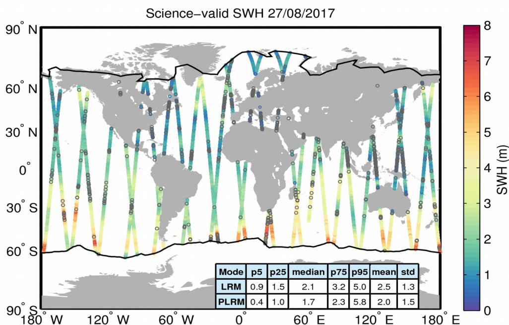
Figure 19. Geographical distribution of science-valid SWH data over oceans and lakes for 27/08/2017. The statistical values shown in the table refer to the SWH in m and are calculated separately for LRM and PLRM regions. The black lines mark the outer limit of the Arctic and Antarctic polar polygons. Gray circles denote records that have been rejected based on the editing criteria described in Table 3.
