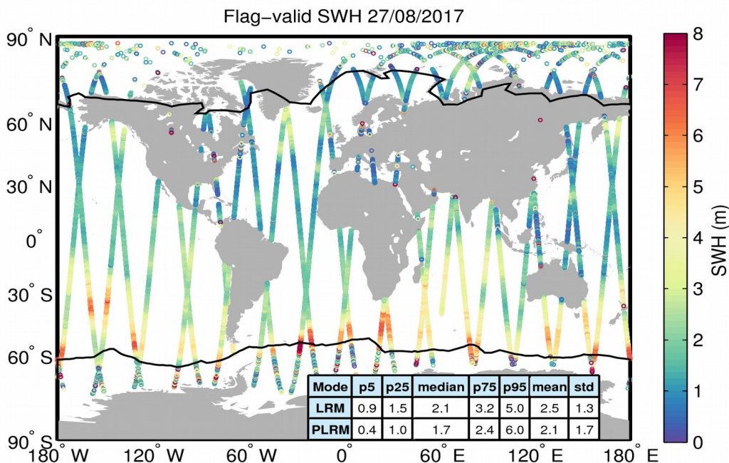
Figure 15. Geographical distribution of flag-valid SWH data over oceans and lakes for 27/08/2017. The statistical values shown in the table refer to the SWH in m and are calculated separately for LRM and PLRM regions. Measurements taken over polar polygons have been excluded from the computation of the statistical values. The black lines mark the outer limit of the Arctic and Antarctic polar polygons.
