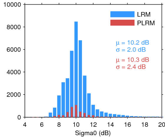
Figure 25. Histogram of flag-valid sigma0 over oceans and lakes for LRM (blue) and PLRM (red) for 27/08/2017. The mean ( \mu ) and standard deviation ( \sigma ) are also shown. Note that values outside [4 20] dB are excluded from the histogram for the sake of readability but not from the computation of \mu and \sigma .
