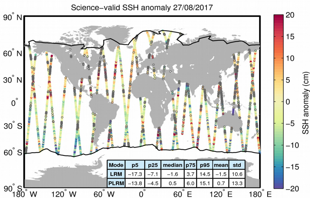
Figure 10. Geographical distribution of science-valid SSH anomaly data over oceans and lakes for 27/08/2017. The statistical values shown in the table refer to the SSH anomaly in cm and are calculated separately for LRM and PLRM regions. The black lines mark the outer limit of the Arctic and Antarctic polar polygons. Gray circles denote records that have been rejected based on the editing criteria described in Table 2.
