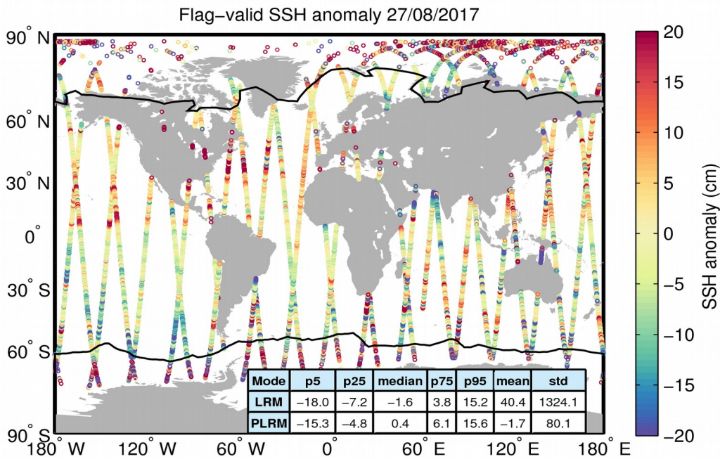
Figure 5. Geographical distribution of flag-valid 1-Hz SSH anomaly data over oceans and lakes for 27/08/2017. The statistical values shown in the table refer to the SSH anomaly in cm and are calculated separately for LRM and PLRM regions. Measurements taken over polar polygons have been excluded from the computation of the statistical values. The black lines mark the outer limit of the Arctic and Antarctic polar polygons.
