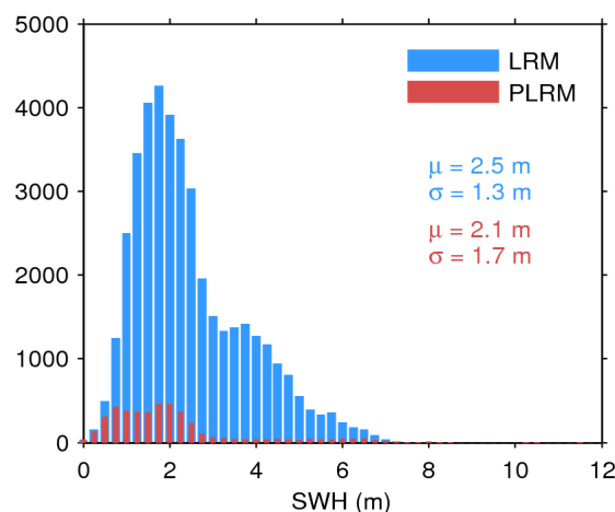
Figure 17. Histogram of flag-valid SWH over oceans and lakes for LRM (blue) and PLRM (red) for 27/08/2017. The mean ( \mu ) and standard deviation ( \sigma ) are also shown. Note that values larger than 12 m are excluded from the histogram for the sake of readability but not from the computation of \mu and \sigma .
