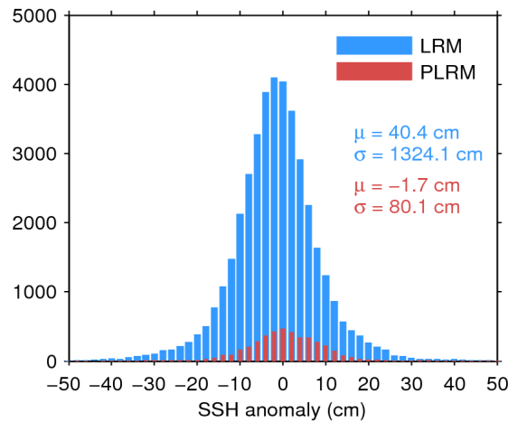
Figure 7. Histogram of flag-valid SSH anomaly over oceans and lakes for LRM (blue) and PLRM (red) for 27/08/2017. The mean ( \mu ) and standard deviation ( \sigma ) are also shown. Note that values outside [-50\ 50] cm are excluded from the histogram for the sake of readability but not from the computation of \mu and \sigma .
