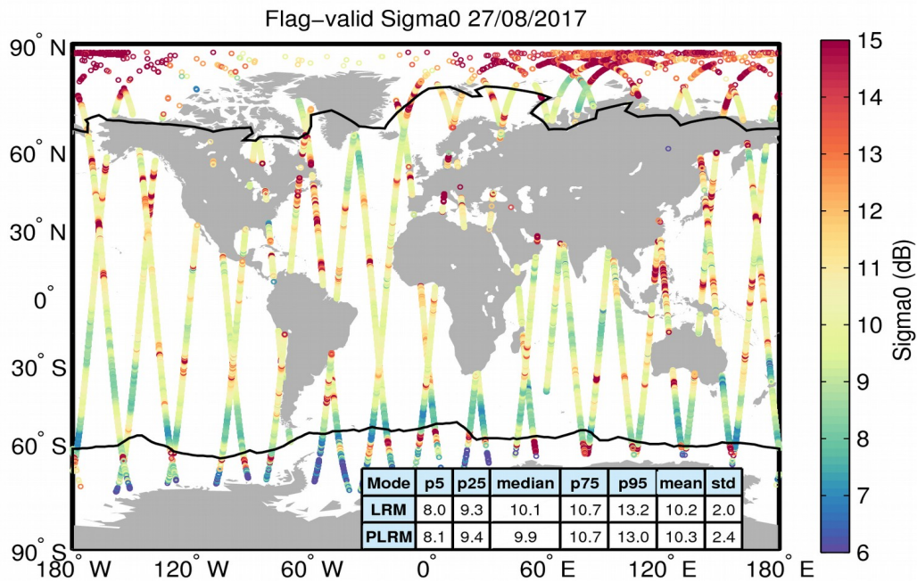
Figure 23. Geographical distribution of flag-valid sigma0 data over oceans and lakes for 27/08/2017. The statistical values shown in the table refer to the sigma0 in dB and are calculated separately for LRM and PLRM regions. Measurements taken over polar polygons have been excluded from the computation of the statistical values. The black lines mark the outer limit of the Arctic and Antarctic polar polygons.
