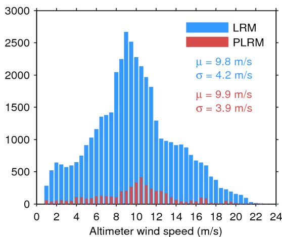
Figure 33. Histogram of flag-valid wind over oceans and lakes for LRM (blue) and PLRM (red) for 27/08/2017. The mean ( \mu ) and standard deviation ( \sigma ) are also shown. Note that values larger than 24 m/s are excluded from the histogram for the sake of readability but not from the computation of \mu and \sigma .
