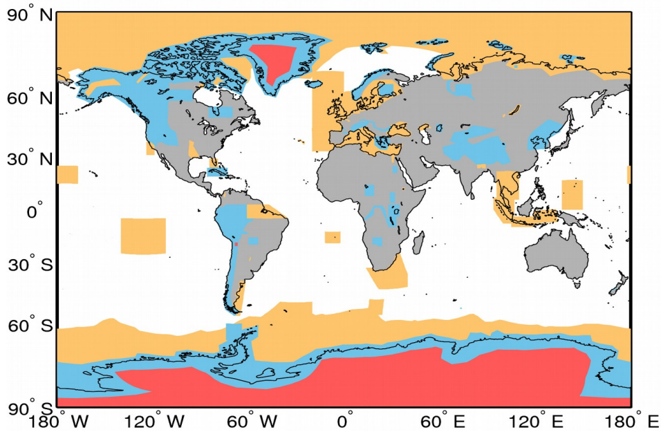
Figure A1. Extent of the regions defining the geographical mode mask for 27/08/2017. The regions where SAR, and SARIn are operated are denoted by the orange and blue polygons, respectively. LRM is operated over areas of the continental ice sheets (red polygons) and over oceans and land not covered by other modes.
