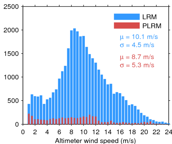
Figure 35. Histogram of science-valid wind over oceans and lakes for LRM (blue) and PLRM (red) for 23/08/2017. The mean ( \mu ) and standard deviation ( \sigma ) are also shown. Note that values larger than 24 m/s are excluded from the histogram for the sake of readability but not from the computation of \mu and \sigma .
