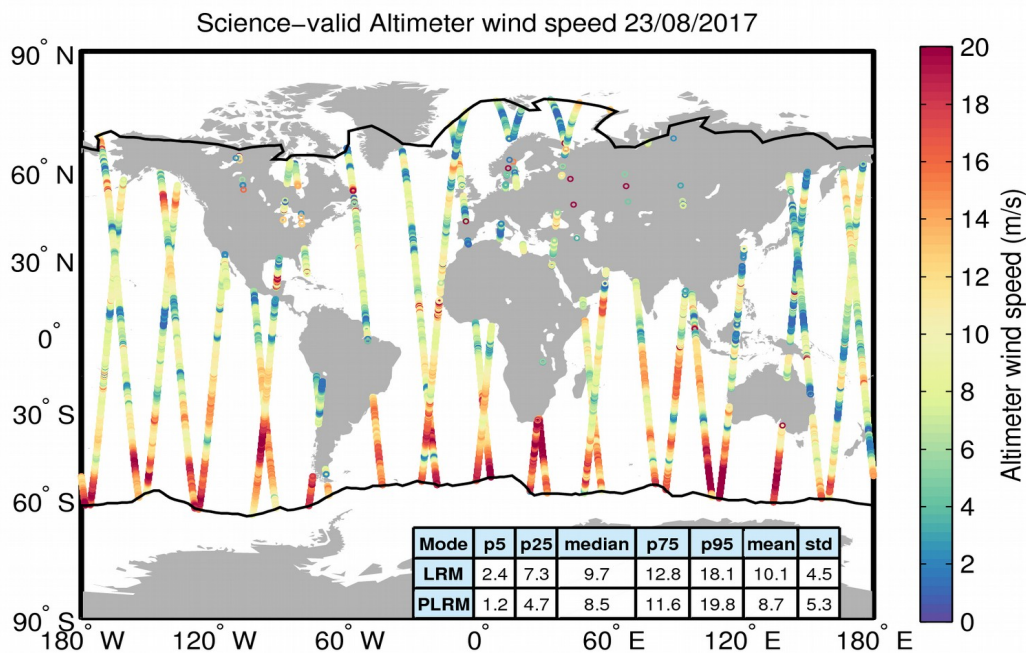
Figure 34. Geographical distribution of science-valid wind data over oceans and lakes for 23/08/2017. The statistical values shown in the table refer to the wind in m/s and are calculated separately for LRM and PLRM regions. The black lines mark the outer limit of the Arctic and Antarctic polar polygons. Gray circles denote records that have been rejected based on the editing criteria described in Table 5.
