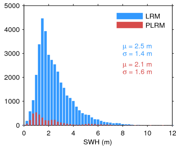
Figure 17. Histogram of flag-valid SWH over oceans and lakes for LRM (blue) and PLRM (red) for 23/08/2017. The mean ( \mu ) and standard deviation ( \sigma ) are also shown. Note that values larger than 12 m are excluded from the histogram for the sake of readability but not from the computation of \mu and \sigma .
