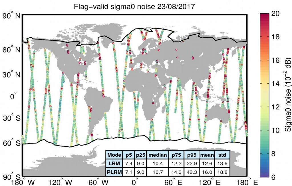
Figure 26. Geographical distribution of flag-valid 20-Hz sigma0 measurement noise over oceans and lakes for 23/08/2017. The statistical values shown in the table refer to the sigma0 noise and are calculated separately for LRM and PLRM regions. Measurements taken over polar polygons have been excluded from the computation of the statistical values. The black lines mark the outer limit of the Arctic and Antarctic polar polygons.
