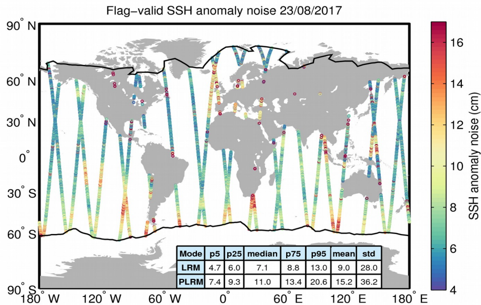
Figure 8. Geographical distribution of flag-valid 20-Hz SSH anomaly measurement noise over oceans and lakes for 23/08/2017. The statistical values shown in the table refer to the SSH anomaly noise and are calculated separately for LRM and PLRM regions. Measurements taken over polar polygons have been excluded from the computation of the statistical values. The black lines mark the outer limit of the Arctic and Antarctic polar polygons.
