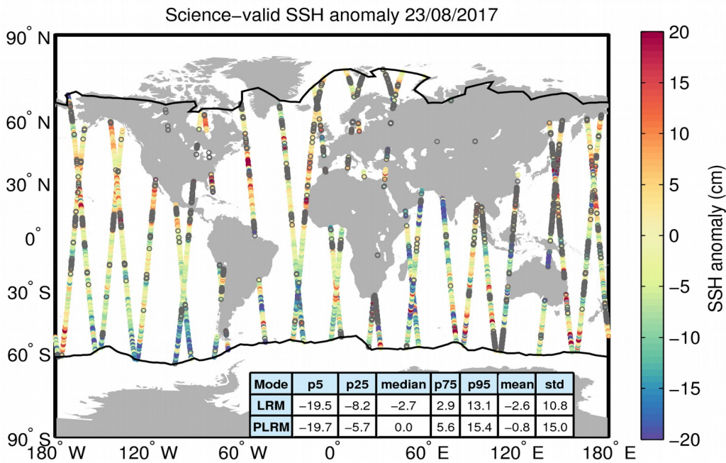
Figure 10. Geographical distribution of science-valid SSH anomaly data over oceans and lakes for 23/08/2017. The statistical values shown in the table refer to the SSH anomaly in cm and are calculated separately for LRM and PLRM regions. The black lines mark the outer limit of the Arctic and Antarctic polar polygons. Gray circles denote records that have been rejected based on the editing criteria described in Table 2.
