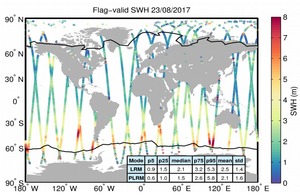
Figure 15. Geographical distribution of flag-valid SWH data over oceans and lakes for 23/08/2017. The statistical values shown in the table refer to the SWH in m and are calculated separately for LRM and PLRM regions. Measurements taken over polar polygons have been excluded from the computation of the statistical values. The black lines mark the outer limit of the Arctic and Antarctic polar polygons.
