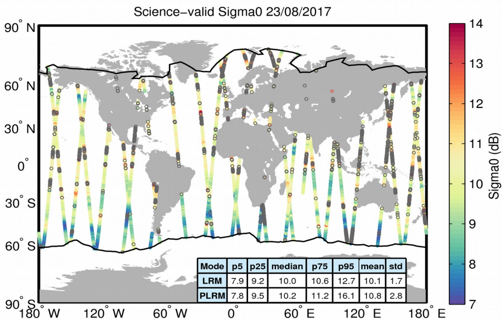
Figure 27. Geographical distribution of science-valid sigma0 data over oceans and lakes for 23/08/2017. The statistical values shown in the table refer to the sigma0 in dB and are calculated separately for LRM and PLRM regions. The black lines mark the outer limit of the Arctic and Antarctic polar polygons. Gray circles denote records that have been rejected based on the editing criteria described in Table 4.
