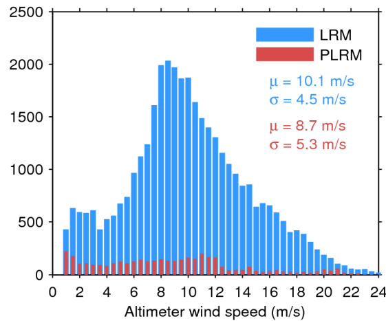
Figure 33. Histogram of flag-valid wind over oceans and lakes for LRM (blue) and PLRM (red) for 23/08/2017. The mean ( \mu ) and standard deviation ( \sigma ) are also shown. Note that values larger than 24 m/s are excluded from the histogram for the sake of readability but not from the computation of \mu and \sigma .
