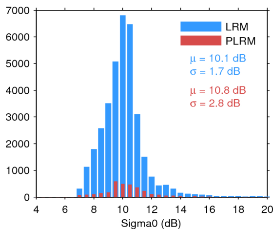
Figure 28. Histogram of science-valid sigma0 over oceans and lakes for LRM (blue) and PLRM (red) for 23/08/2017. The mean ( \mu ) and standard deviation ( \sigma ) are also shown. Note that values outside [4 20] dB are excluded from the histogram for the sake of readability but not from the computation of \mu and \sigma .
