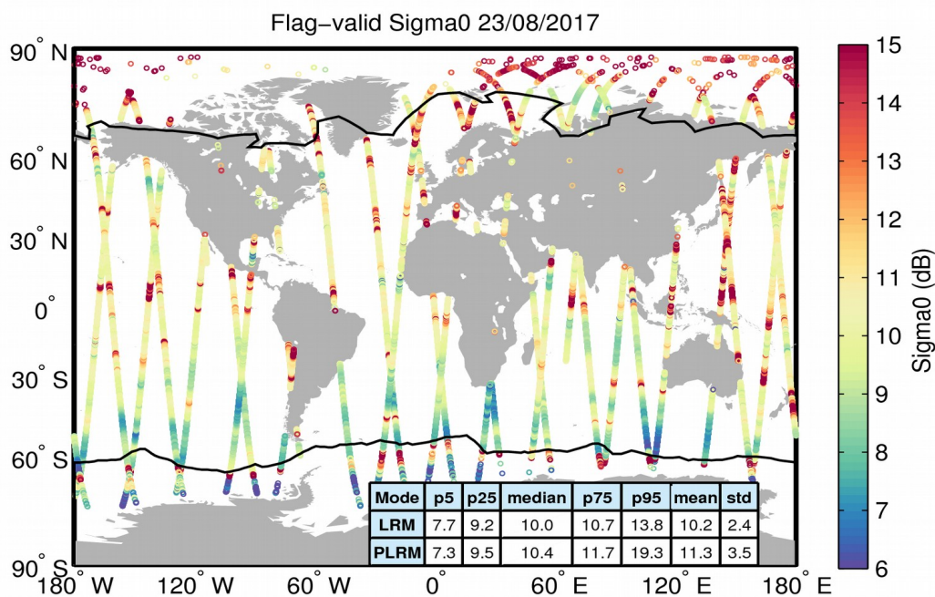
Figure 23. Geographical distribution of flag-valid sigma0 data over oceans and lakes for 23/08/2017. The statistical values shown in the table refer to the sigma0 in dB and are calculated separately for LRM and PLRM regions. Measurements taken over polar polygons have been excluded from the computation of the statistical values. The black lines mark the outer limit of the Arctic and Antarctic polar polygons.
