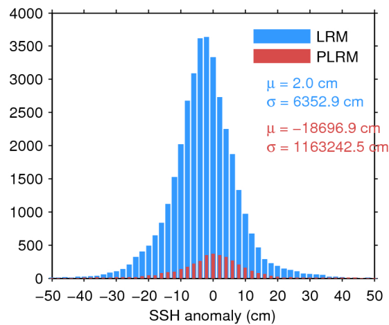
Figure 7. Histogram of flag-valid SSH anomaly over oceans and lakes for LRM (blue) and PLRM (red) for 23/08/2017. The mean ( \mu ) and standard deviation ( \sigma ) are also shown. Note that values outside [-50\ 50] cm are excluded from the histogram for the sake of readability but not from the computation of \mu and \sigma .
