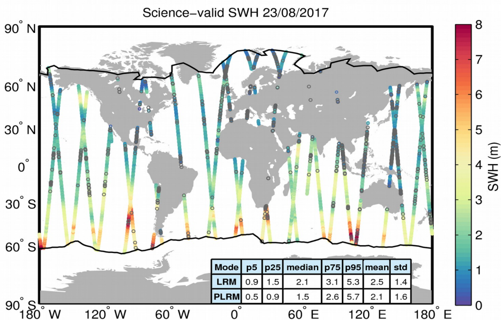
Figure 19. Geographical distribution of science-valid SWH data over oceans and lakes for 23/08/2017. The statistical values shown in the table refer to the SWH in m and are calculated separately for LRM and PLRM regions. The black lines mark the outer limit of the Arctic and Antarctic polar polygons. Gray circles denote records that have been rejected based on the editing criteria described in Table 3.
