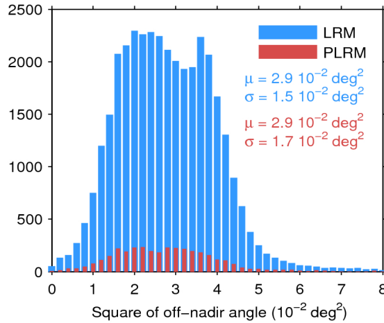
Figure 39. Histogram of flag-valid mispointing over oceans and lakes for LRM (blue) and PLRM (red) for 23/08/2017. Only positive values have been considered. The mean ( \mu ) and standard deviation ( \sigma ) are also shown. Note that values larger than 8 \cdot 10^{-2} \text{ deg}^2 are excluded from the histogram for the sake of readability but not from the computation of \mu and \sigma .
