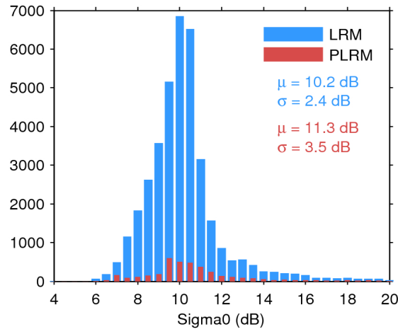
Figure 25. Histogram of flag-valid sigma0 over oceans and lakes for LRM (blue) and PLRM (red) for 23/08/2017. The mean ( \mu ) and standard deviation ( \sigma ) are also shown. Note that values outside [4 20] dB are excluded from the histogram for the sake of readability but not from the computation of \mu and \sigma .
