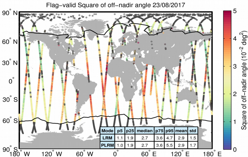
Figure 37. Geographical distribution of flag-valid mispointing data over oceans and lakes for 23/08/2017. The statistical values shown in the table refer to the mispointing in 10^{-2} deg 2 and are calculated separately for LRM and PLRM regions. Measurements taken over polar polygons have been excluded from the computation of the statistical values. The black lines mark the outer limit of the Arctic and Antarctic polar polygons. Gray circles denote negative values.
