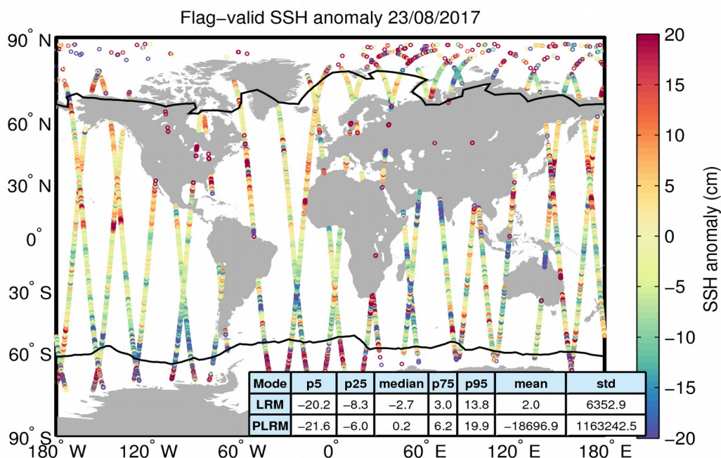
Figure 5. Geographical distribution of flag-valid 1-Hz SSH anomaly data over oceans and lakes for 23/08/2017. The statistical values shown in the table refer to the SSH anomaly in cm and are calculated separately for LRM and PLRM regions. Measurements taken over polar polygons have been excluded from the computation of the statistical values. The black lines mark the outer limit of the Arctic and Antarctic polar polygons.
