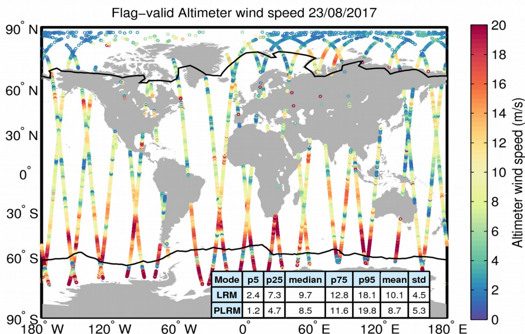
Figure 31. Geographical distribution of flag-valid wind data over oceans and lakes for 23/08/2017. The statistical values shown in the table refer to the wind in m/s and are calculated separately for LRM and PLRM regions. Measurements taken over polar polygons have been excluded from the computation of the statistical values. The black lines mark the outer limit of the Arctic and Antarctic polar polygons.
