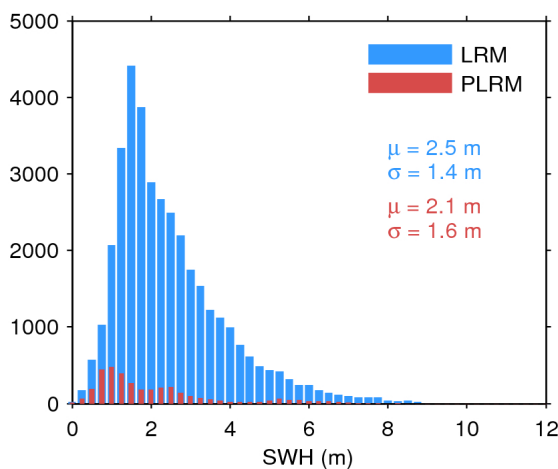
Figure 20. Histogram of science-valid SWH over oceans and lakes for LRM (blue) and PLRM (red) for 23/08/2017. The mean ( \mu ) and standard deviation ( \sigma ) are also shown. Note that values larger than 12 m are excluded from the histogram for the sake of readability but not from the computation of \mu and \sigma .
