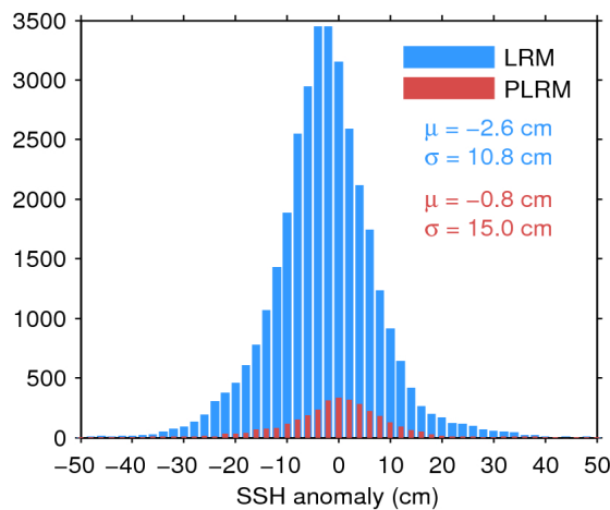
Figure 11. Histogram of science-valid SSH anomaly over oceans and lakes for LRM (blue) and PLRM (red) for 23/08/2017. The mean ( \mu ) and standard deviation ( \sigma ) are also shown. Note that values outside [-50 50] cm are excluded from the histogram for the sake of readability but not from the computation of \mu and \sigma .
