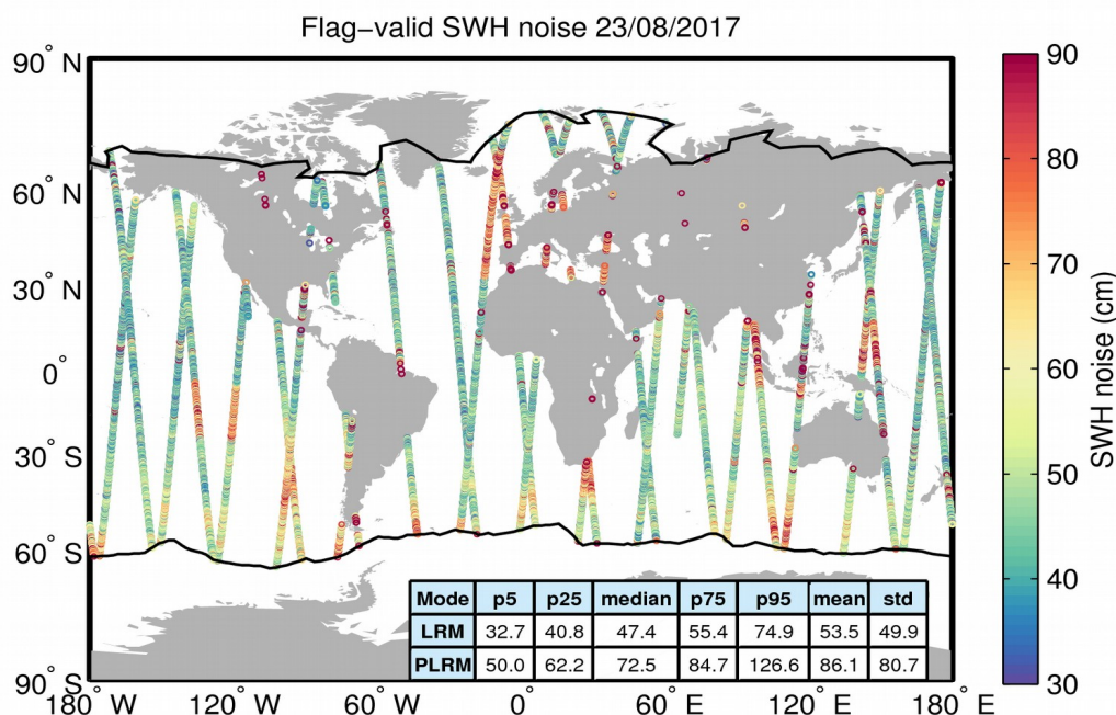
Figure 18. Geographical distribution of flag-valid 20-Hz SWH measurement noise over oceans and lakes for 23/08/2017. The statistical values shown in the table refer to the SWH noise and are calculated separately for LRM and PLRM regions. Measurements taken over polar polygons have been excluded from the computation of the statistical values. The black lines mark the outer limit of the Arctic and Antarctic polar polygons.
