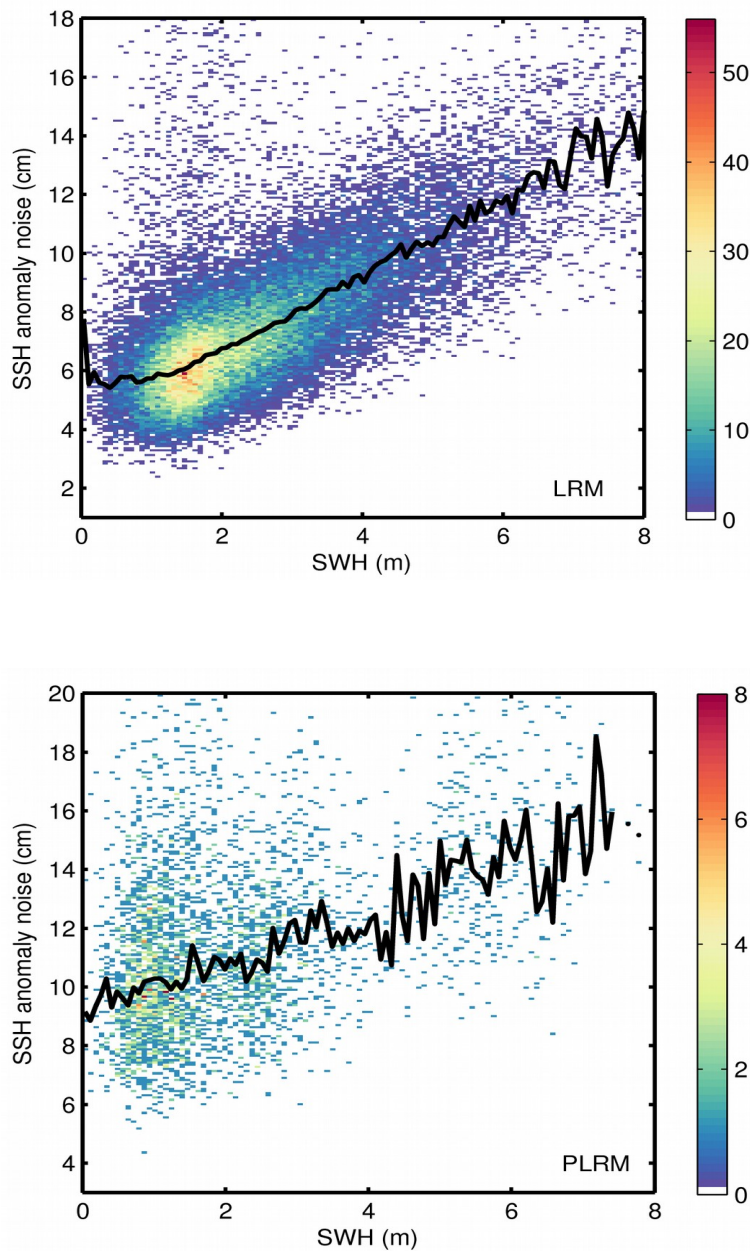
Figure 9. 2D histogram showing flag-valid SSH anomaly noise as a function of SWH for LRM (top) and PLRM (bottom) for 23/08/2017. The black line denotes the median SSH anomaly noise as a function of SWH.
