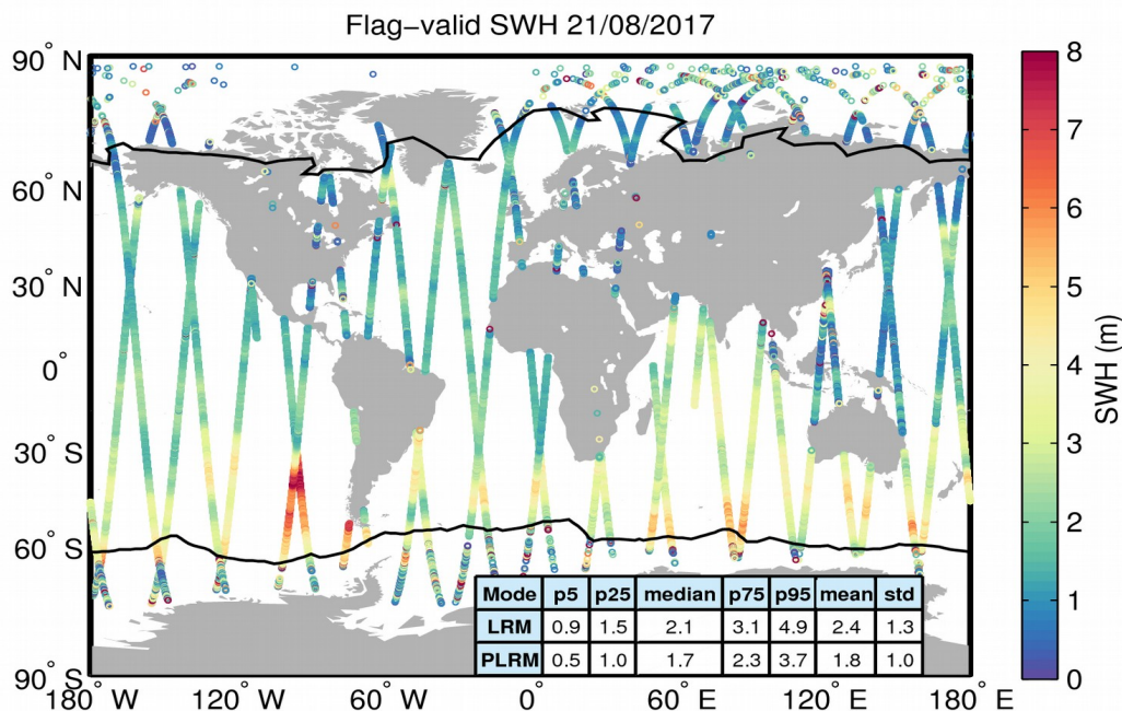
Figure 15. Geographical distribution of flag-valid SWH data over oceans and lakes for 21/08/2017. The statistical values shown in the table refer to the SWH in m and are calculated separately for LRM and PLRM regions. Measurements taken over polar polygons have been excluded from the computation of the statistical values. The black lines mark the outer limit of the Arctic and Antarctic polar polygons.
