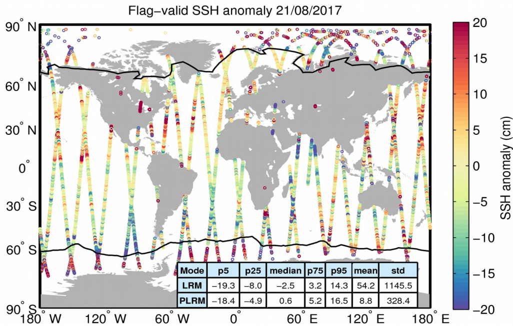
Figure 5. Geographical distribution of flag-valid 1-Hz SSH anomaly data over oceans and lakes for 21/08/2017. The statistical values shown in the table refer to the SSH anomaly in cm and are calculated separately for LRM and PLRM regions. Measurements taken over polar polygons have been excluded from the computation of the statistical values. The black lines mark the outer limit of the Arctic and Antarctic polar polygons.
