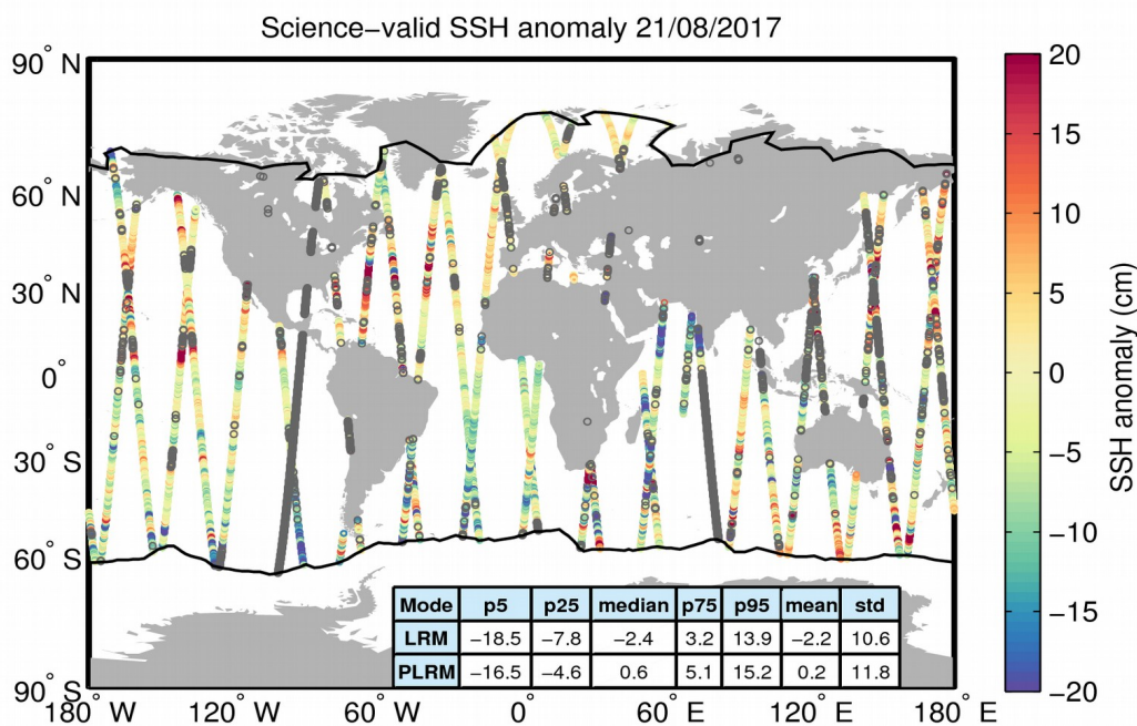
Figure 10. Geographical distribution of science-valid SSH anomaly data over oceans and lakes for 21/08/2017. The statistical values shown in the table refer to the SSH anomaly in cm and are calculated separately for LRM and PLRM regions. The black lines mark the outer limit of the Arctic and Antarctic polar polygons. Gray circles denote records that have been rejected based on the editing criteria described in Table 2.
