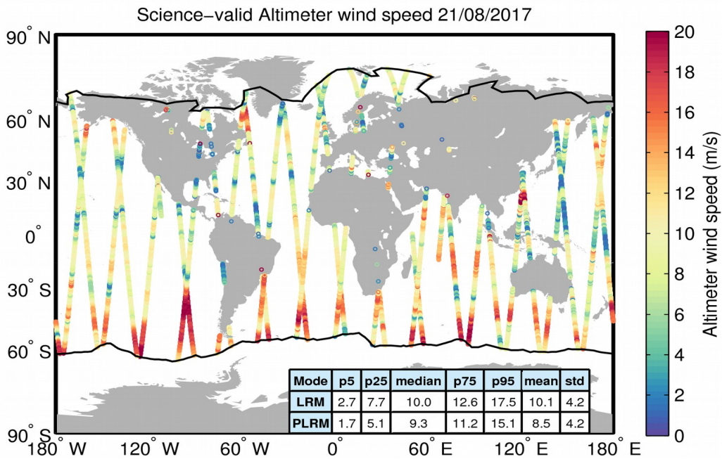
Figure 34. Geographical distribution of science-valid wind data over oceans and lakes for 21/08/2017. The statistical values shown in the table refer to the wind in m/s and are calculated separately for LRM and PLRM regions. The black lines mark the outer limit of the Arctic and Antarctic polar polygons. Gray circles denote records that have been rejected based on the editing criteria described in Table 5.
