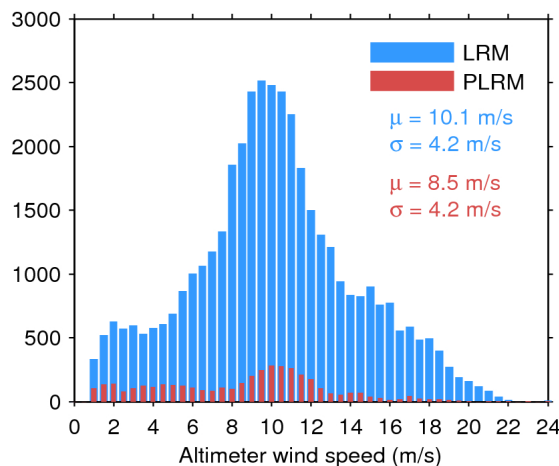
Figure 35. Histogram of science-valid wind over oceans and lakes for LRM (blue) and PLRM (red) for 21/08/2017. The mean ( \mu ) and standard deviation ( \sigma ) are also shown. Note that values larger than 24 m/s are excluded from the histogram for the sake of readability but not from the computation of \mu and \sigma .
