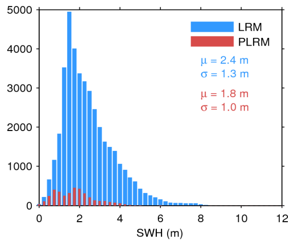
Figure 20. Histogram of science-valid SWH over oceans and lakes for LRM (blue) and PLRM (red) for 21/08/2017. The mean ( \mu ) and standard deviation ( \sigma ) are also shown. Note that values larger than 12 m are excluded from the histogram for the sake of readability but not from the computation of \mu and \sigma .
