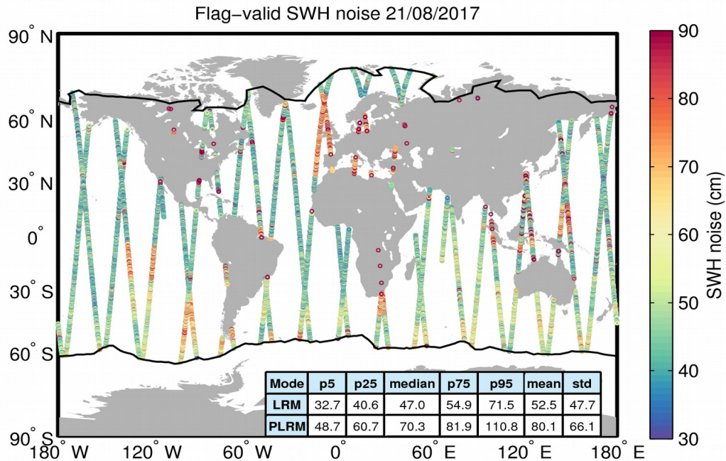
Figure 18. Geographical distribution of flag-valid 20-Hz SWH measurement noise over oceans and lakes for 21/08/2017. The statistical values shown in the table refer to the SWH noise and are calculated separately for LRM and PLRM regions. Measurements taken over polar polygons have been excluded from the computation of the statistical values. The black lines mark the outer limit of the Arctic and Antarctic polar polygons.
