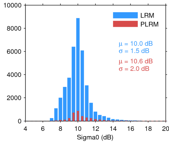
Figure 28. Histogram of science-valid sigma0 over oceans and lakes for LRM (blue) and PLRM (red) for 21/08/2017. The mean ( \mu ) and standard deviation ( \sigma ) are also shown. Note that values outside [4 20] dB are excluded from the histogram for the sake of readability but not from the computation of \mu and \sigma .
