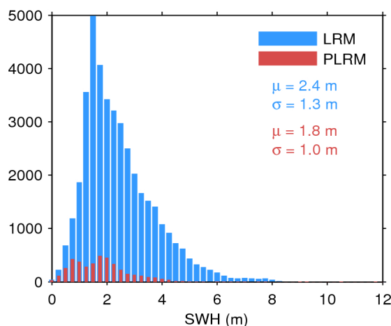
Figure 17. Histogram of flag-valid SWH over oceans and lakes for LRM (blue) and PLRM (red) for 21/08/2017. The mean ( \mu ) and standard deviation ( \sigma ) are also shown. Note that values larger than 12 m are excluded from the histogram for the sake of readability but not from the computation of \mu and \sigma .
