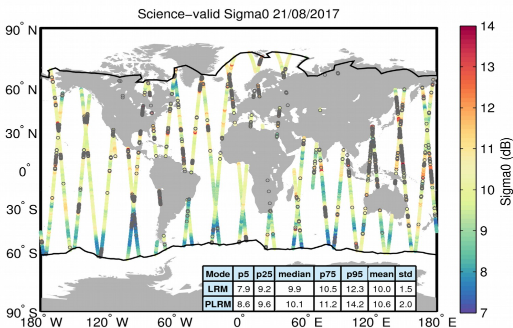
Figure 27. Geographical distribution of science-valid sigma0 data over oceans and lakes for 21/08/2017. The statistical values shown in the table refer to the sigma0 in dB and are calculated separately for LRM and PLRM regions. The black lines mark the outer limit of the Arctic and Antarctic polar polygons. Gray circles denote records that have been rejected based on the editing criteria described in Table 4.
