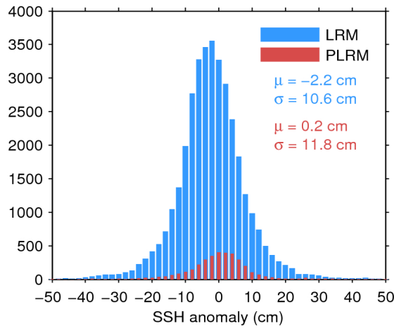
Figure 11. Histogram of science-valid SSH anomaly over oceans and lakes for LRM (blue) and PLRM (red) for 21/08/2017. The mean ( \mu ) and standard deviation ( \sigma ) are also shown. Note that values outside [-50 50] cm are excluded from the histogram for the sake of readability but not from the computation of \mu and \sigma .
