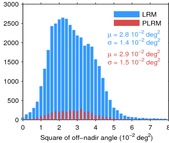
Figure 39. Histogram of flag-valid mispointing over oceans and lakes for LRM (blue) and PLRM (red) for 21/08/2017. Only positive values have been considered. The mean ( \mu ) and standard deviation ( \sigma ) are also shown. Note that values larger than 8 \cdot 10^{-2} \text{ deg}^2 are excluded from the histogram for the sake of readability but not from the computation of \mu and \sigma .
