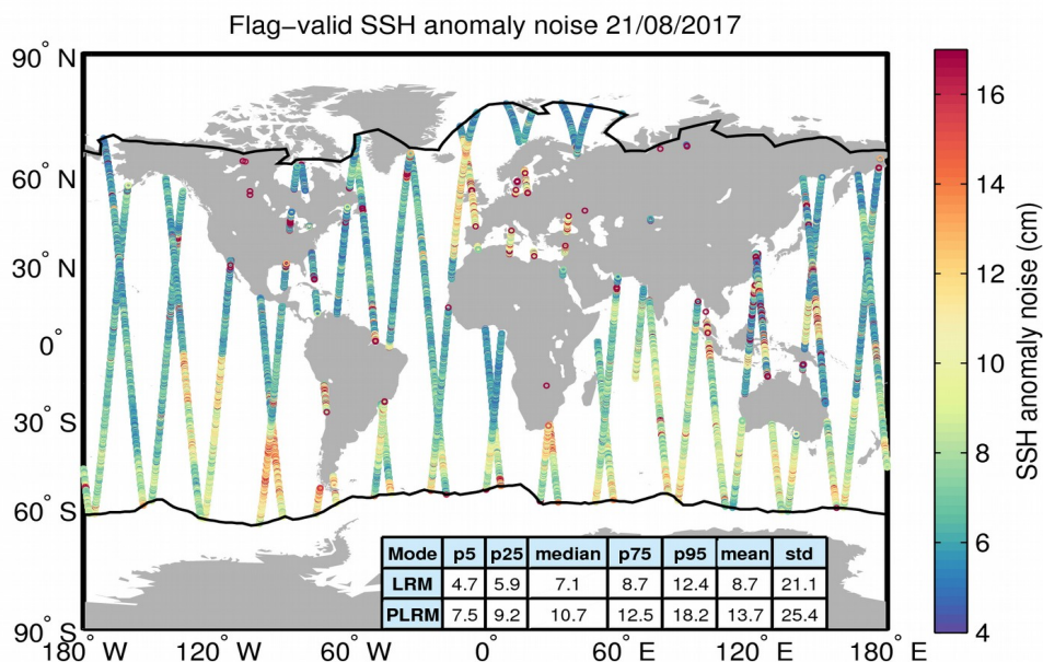
Figure 8. Geographical distribution of flag-valid 20-Hz SSH anomaly measurement noise over oceans and lakes for 21/08/2017. The statistical values shown in the table refer to the SSH anomaly noise and are calculated separately for LRM and PLRM regions. Measurements taken over polar polygons have been excluded from the computation of the statistical values. The black lines mark the outer limit of the Arctic and Antarctic polar polygons.
