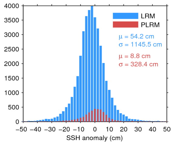
Figure 7. Histogram of flag-valid SSH anomaly over oceans and lakes for LRM (blue) and PLRM (red) for 21/08/2017. The mean ( \mu ) and standard deviation ( \sigma ) are also shown. Note that values outside [-50 50] cm are excluded from the histogram for the sake of readability but not from the computation of \mu and \sigma .
