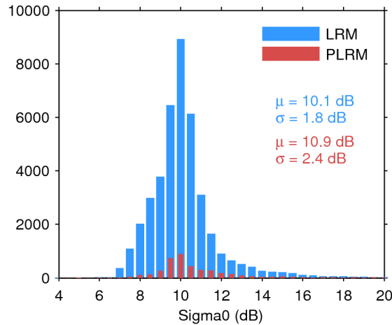
Figure 25. Histogram of flag-valid sigma0 over oceans and lakes for LRM (blue) and PLRM (red) for 21/08/2017. The mean ( \mu ) and standard deviation ( \sigma ) are also shown. Note that values outside [4 20] dB are excluded from the histogram for the sake of readability but not from the computation of \mu and \sigma .
