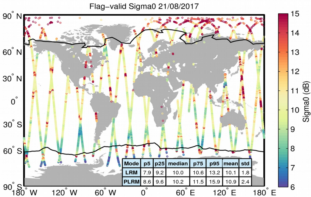
Figure 23. Geographical distribution of flag-valid sigma0 data over oceans and lakes for 21/08/2017. The statistical values shown in the table refer to the sigma0 in dB and are calculated separately for LRM and PLRM regions. Measurements taken over polar polygons have been excluded from the computation of the statistical values. The black lines mark the outer limit of the Arctic and Antarctic polar polygons.
