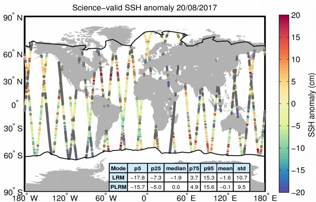
Figure 10. Geographical distribution of science-valid SSH anomaly data over oceans and lakes for 20/08/2017. The statistical values shown in the table refer to the SSH anomaly in cm and are calculated separately for LRM and PLRM regions. The black lines mark the outer limit of the Arctic and Antarctic polar polygons. Gray circles denote records that have been rejected based on the editing criteria described in Table 2.
