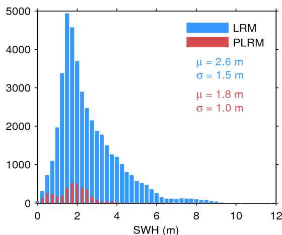
Figure 17. Histogram of flag-valid SWH over oceans and lakes for LRM (blue) and PLRM (red) for 20/08/2017. The mean ( \mu ) and standard deviation ( \sigma ) are also shown. Note that values larger than 12 m are excluded from the histogram for the sake of readability but not from the computation of \mu and \sigma .
