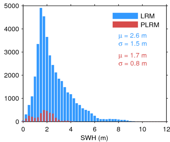
Figure 20. Histogram of science-valid SWH over oceans and lakes for LRM (blue) and PLRM (red) for 20/08/2017. The mean ( \mu ) and standard deviation ( \sigma ) are also shown. Note that values larger than 12 m are excluded from the histogram for the sake of readability but not from the computation of \mu and \sigma .
