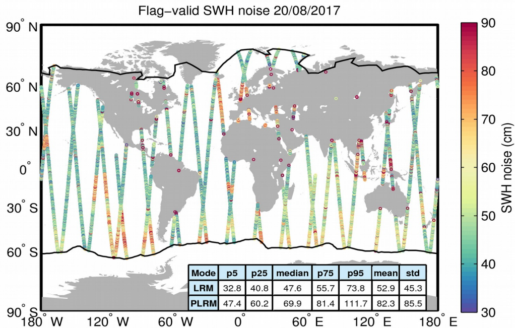
Figure 18. Geographical distribution of flag-valid 20-Hz SWH measurement noise over oceans and lakes for 20/08/2017. The statistical values shown in the table refer to the SWH noise and are calculated separately for LRM and PLRM regions. Measurements taken over polar polygons have been excluded from the computation of the statistical values. The black lines mark the outer limit of the Arctic and Antarctic polar polygons.
