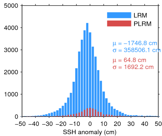
Figure 7. Histogram of flag-valid SSH anomaly over oceans and lakes for LRM (blue) and PLRM (red) for 20/08/2017. The mean ( \mu ) and standard deviation ( \sigma ) are also shown. Note that values outside [-50 \ 50] cm are excluded from the histogram for the sake of readability but not from the computation of \mu and \sigma .
