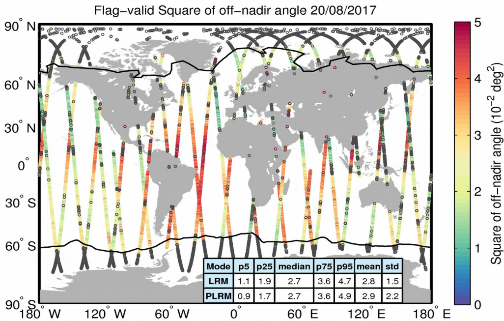
Figure 37. Geographical distribution of flag-valid mispointing data over oceans and lakes for 20/08/2017. The statistical values shown in the table refer to the mispointing in 10^{-2} deg 2 and are calculated separately for LRM and PLRM regions. Measurements taken over polar polygons have been excluded from the computation of the statistical values. The black lines mark the outer limit of the Arctic and Antarctic polar polygons. Gray circles denote negative values.
