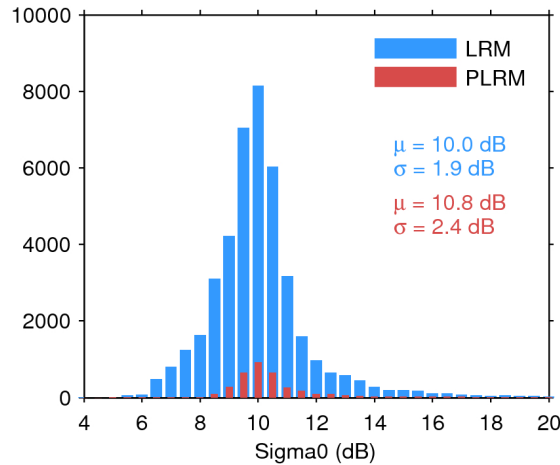
Figure 25. Histogram of flag-valid sigma0 over oceans and lakes for LRM (blue) and PLRM (red) for 20/08/2017. The mean ( \mu ) and standard deviation ( \sigma ) are also shown. Note that values outside [4 20] dB are excluded from the histogram for the sake of readability but not from the computation of \mu and \sigma .
