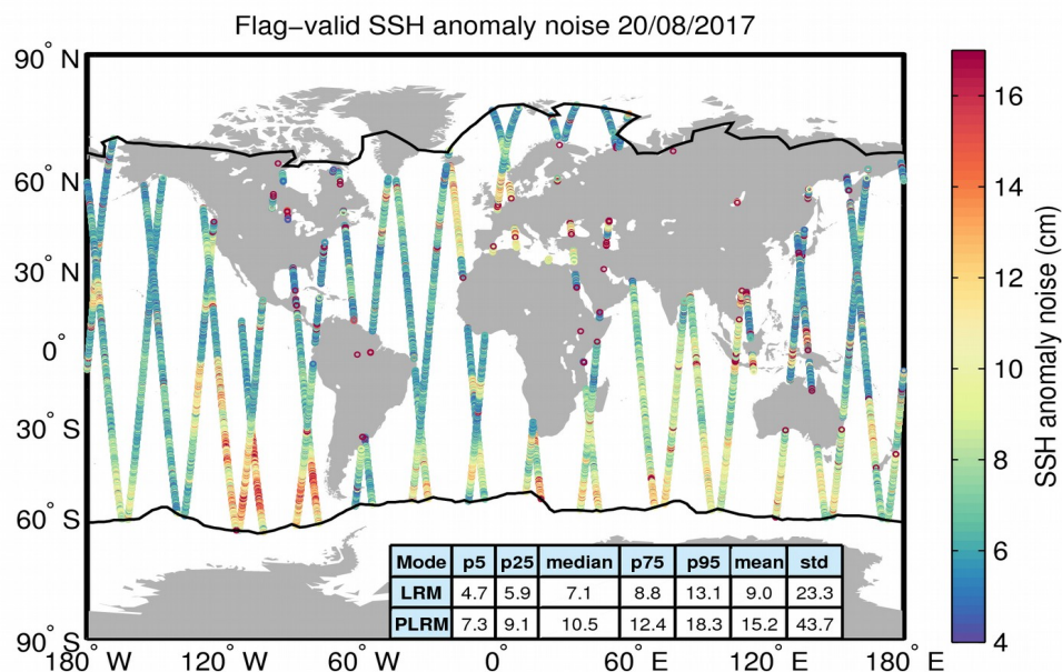
Figure 8. Geographical distribution of flag-valid 20-Hz SSH anomaly measurement noise over oceans and lakes for 20/08/2017. The statistical values shown in the table refer to the SSH anomaly noise and are calculated separately for LRM and PLRM regions. Measurements taken over polar polygons have been excluded from the computation of the statistical values. The black lines mark the outer limit of the Arctic and Antarctic polar polygons.
