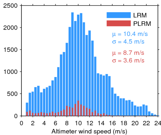
Figure 35. Histogram of science-valid wind over oceans and lakes for LRM (blue) and PLRM (red) for 20/08/2017. The mean ( \mu ) and standard deviation ( \sigma ) are also shown. Note that values larger than 24 m/s are excluded from the histogram for the sake of readability but not from the computation of \mu and \sigma .
