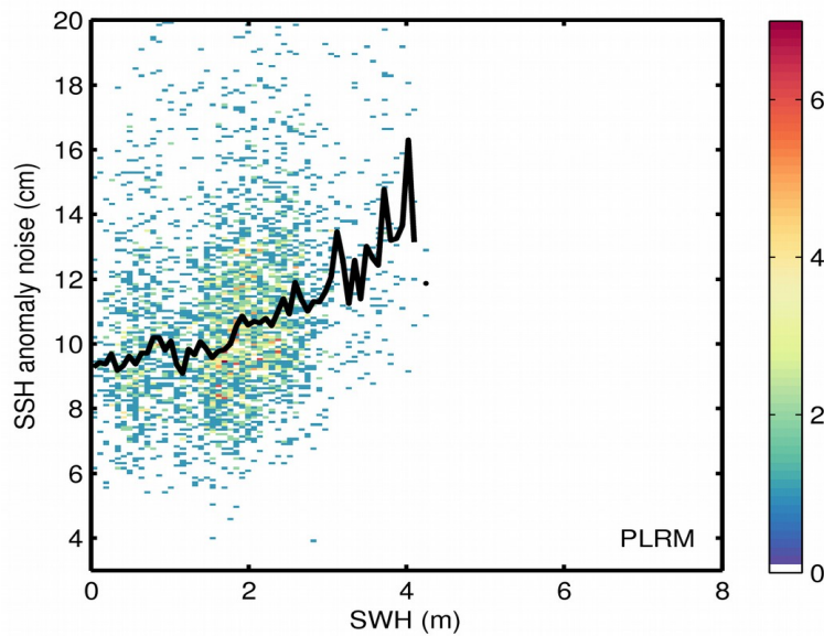
Figure 9. 2D histogram showing flag-valid SSH anomaly noise as a function of SWH for LRM (top) and PLRM (bottom) for 20/08/2017. The black line denotes the median SSH anomaly noise as a function of SWH.
