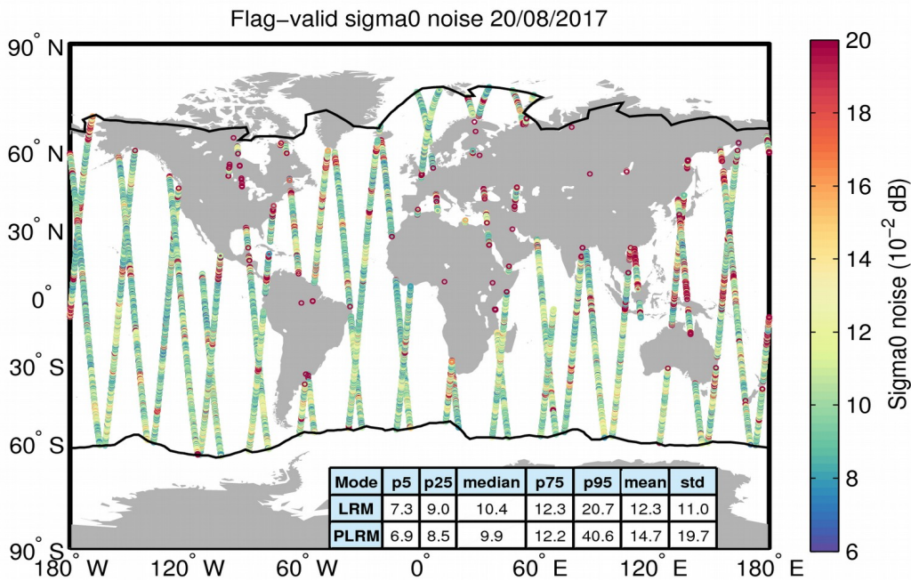
Figure 26. Geographical distribution of flag-valid 20-Hz sigma0 measurement noise over oceans and lakes for 20/08/2017. The statistical values shown in the table refer to the sigma0 noise and are calculated separately for LRM and PLRM regions. Measurements taken over polar polygons have been excluded from the computation of the statistical values. The black lines mark the outer limit of the Arctic and Antarctic polar polygons.
