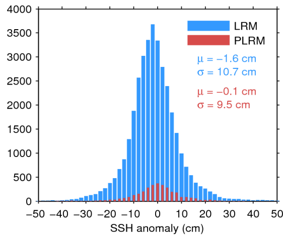
Figure 11. Histogram of science-valid SSH anomaly over oceans and lakes for LRM (blue) and PLRM (red) for 20/08/2017. The mean ( \mu ) and standard deviation ( \sigma ) are also shown. Note that values outside [-50 50] cm are excluded from the histogram for the sake of readability but not from the computation of \mu and \sigma .
