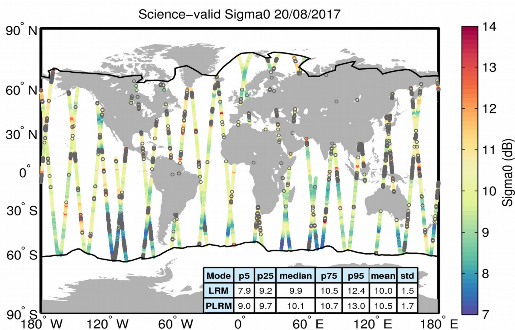
Figure 27. Geographical distribution of science-valid sigma0 data over oceans and lakes for 20/08/2017. The statistical values shown in the table refer to the sigma0 in dB and are calculated separately for LRM and PLRM regions. The black lines mark the outer limit of the Arctic and Antarctic polar polygons. Gray circles denote records that have been rejected based on the editing criteria described in Table 4.
