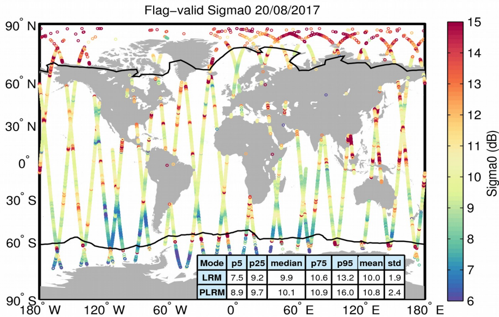
Figure 23. Geographical distribution of flag-valid sigma0 data over oceans and lakes for 20/08/2017. The statistical values shown in the table refer to the sigma0 in dB and are calculated separately for LRM and PLRM regions. Measurements taken over polar polygons have been excluded from the computation of the statistical values. The black lines mark the outer limit of the Arctic and Antarctic polar polygons.
