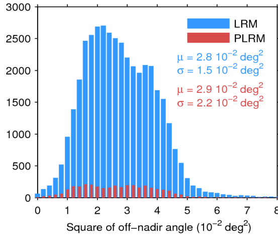
Figure 39. Histogram of flag-valid mispointing over oceans and lakes for LRM (blue) and PLRM (red) for 20/08/2017. Only positive values have been considered. The mean ( \mu ) and standard deviation ( \sigma ) are also shown. Note that values larger than 8 \cdot 10^{-2} \text{ deg}^2 are excluded from the histogram for the sake of readability but not from the computation of \mu and \sigma .
