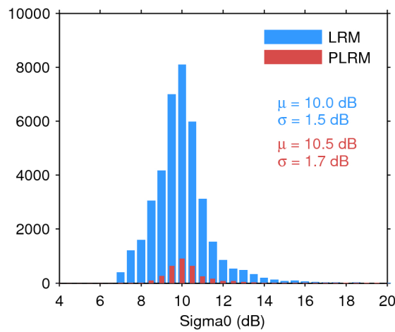
Figure 28. Histogram of science-valid sigma0 over oceans and lakes for LRM (blue) and PLRM (red) for 20/08/2017. The mean ( \mu ) and standard deviation ( \sigma ) are also shown. Note that values outside [4 20] dB are excluded from the histogram for the sake of readability but not from the computation of \mu and \sigma .
