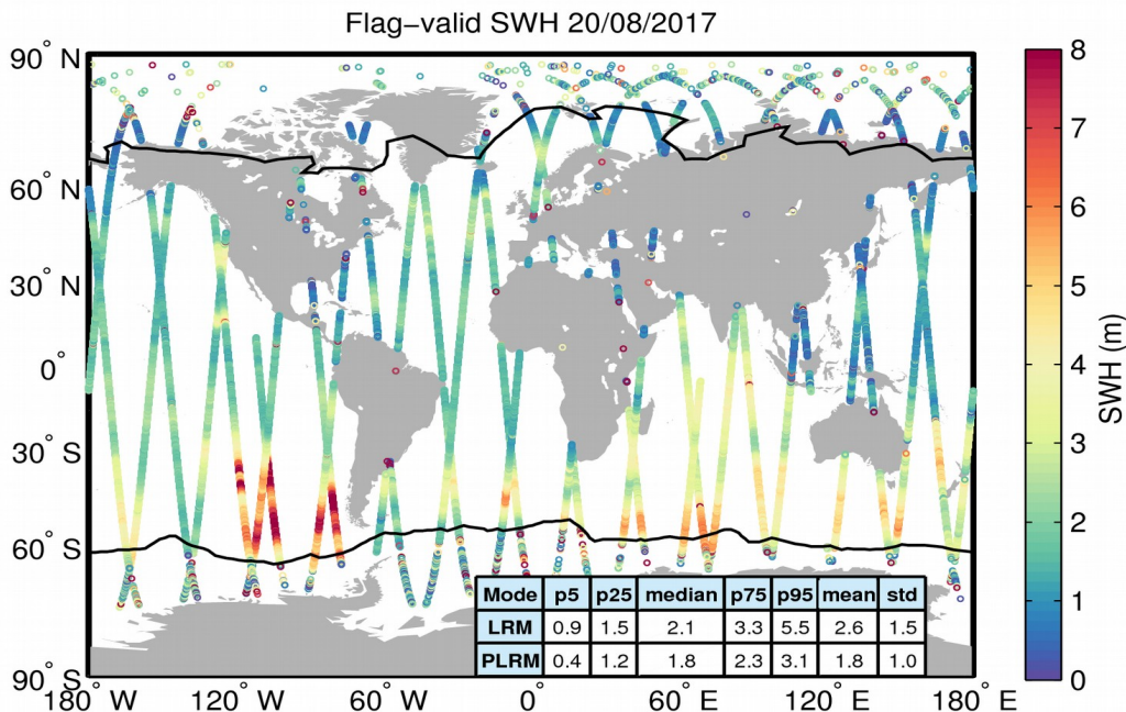
Figure 15. Geographical distribution of flag-valid SWH data over oceans and lakes for 20/08/2017. The statistical values shown in the table refer to the SWH in m and are calculated separately for LRM and PLRM regions. Measurements taken over polar polygons have been excluded from the computation of the statistical values. The black lines mark the outer limit of the Arctic and Antarctic polar polygons.
