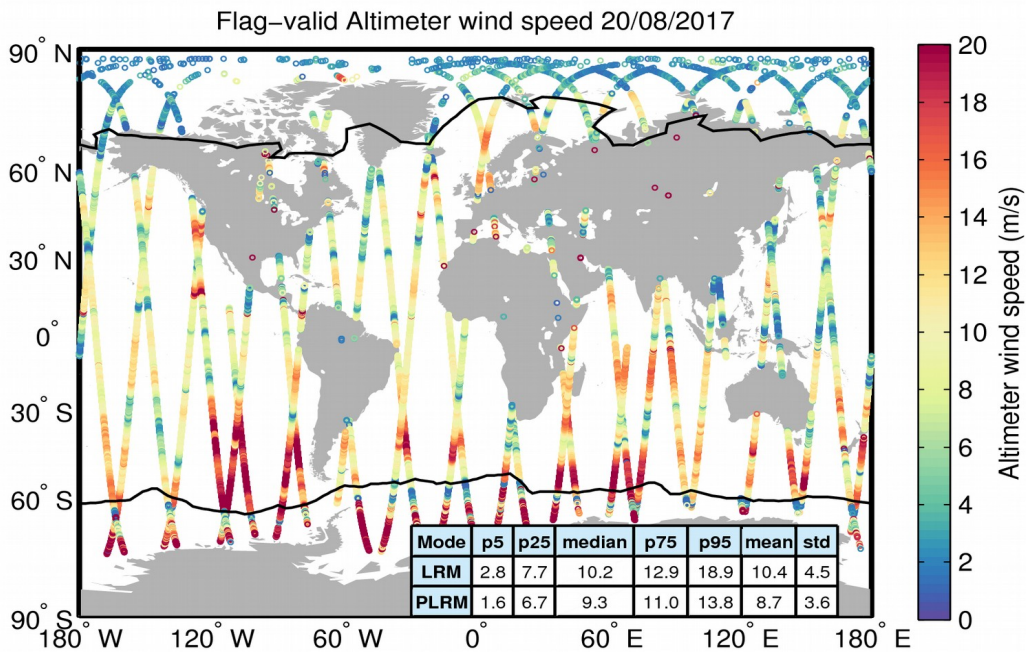
Figure 31. Geographical distribution of flag-valid wind data over oceans and lakes for 20/08/2017. The statistical values shown in the table refer to the wind in m/s and are calculated separately for LRM and PLRM regions. Measurements taken over polar polygons have been excluded from the computation of the statistical values. The black lines mark the outer limit of the Arctic and Antarctic polar polygons.
