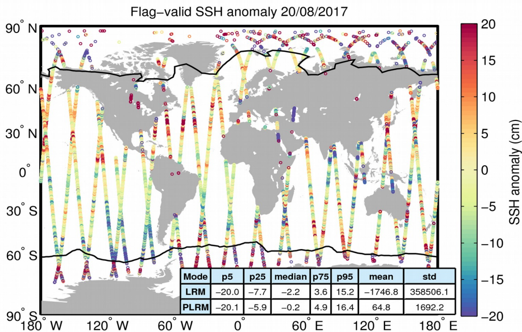
Figure 5. Geographical distribution of flag-valid 1-Hz SSH anomaly data over oceans and lakes for 20/08/2017. The statistical values shown in the table refer to the SSH anomaly in cm and are calculated separately for LRM and PLRM regions. Measurements taken over polar polygons have been excluded from the computation of the statistical values. The black lines mark the outer limit of the Arctic and Antarctic polar polygons.
