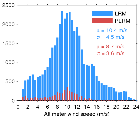
Figure 33. Histogram of flag-valid wind over oceans and lakes for LRM (blue) and PLRM (red) for 20/08/2017. The mean ( \mu ) and standard deviation ( \sigma ) are also shown. Note that values larger than 24 m/s are excluded from the histogram for the sake of readability but not from the computation of \mu and \sigma .
