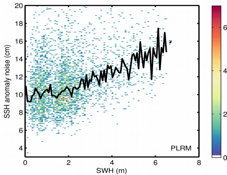
Figure 9. 2D histogram showing flag-valid SSH anomaly noise as a function of SWH for LRM (top) and PLRM (bottom) for 16/08/2017. The black line denotes the median SSH anomaly noise as a function of SWH.
