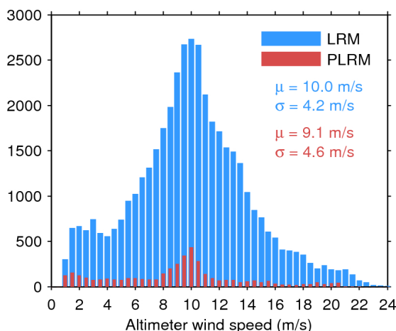
Figure 33. Histogram of flag-valid wind over oceans and lakes for LRM (blue) and PLRM (red) for 16/08/2017. The mean ( \mu ) and standard deviation ( \sigma ) are also shown. Note that values larger than 24 m/s are excluded from the histogram for the sake of readability but not from the computation of \mu and \sigma .
