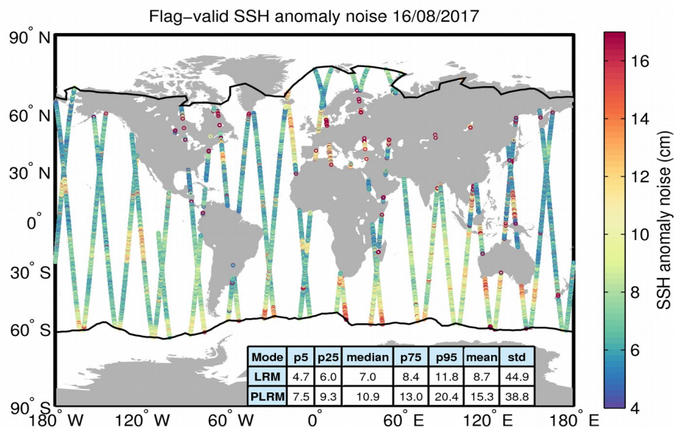
Figure 8. Geographical distribution of flag-valid 20-Hz SSH anomaly measurement noise over oceans and lakes for 16/08/2017. The statistical values shown in the table refer to the SSH anomaly noise and are calculated separately for LRM and PLRM regions. Measurements taken over polar polygons have been excluded from the computation of the statistical values. The black lines mark the outer limit of the Arctic and Antarctic polar polygons.
