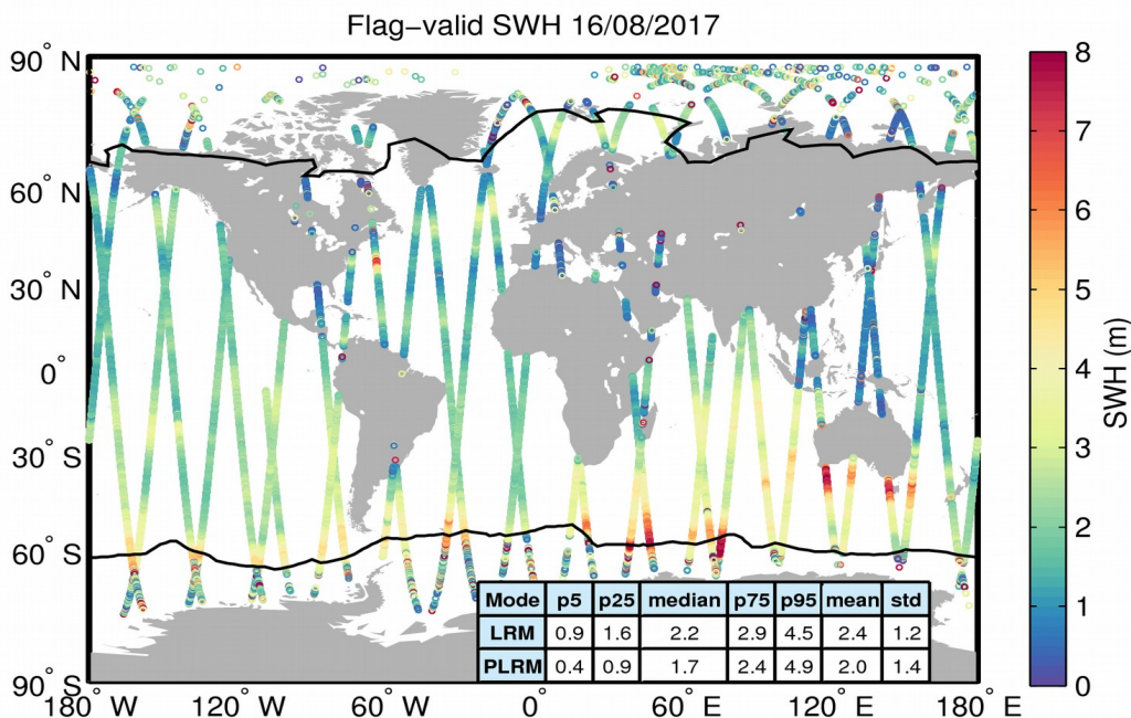
Figure 15. Geographical distribution of flag-valid SWH data over oceans and lakes for 16/08/2017. The statistical values shown in the table refer to the SWH in m and are calculated separately for LRM and PLRM regions. Measurements taken over polar polygons have been excluded from the computation of the statistical values. The black lines mark the outer limit of the Arctic and Antarctic polar polygons.
