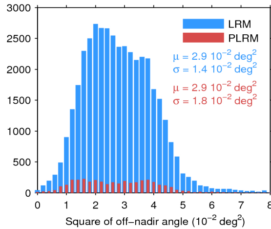
Figure 39. Histogram of flag-valid mispointing over oceans and lakes for LRM (blue) and PLRM (red) for 16/08/2017. Only positive values have been considered. The mean ( \mu ) and standard deviation ( \sigma ) are also shown. Note that values larger than 8 \cdot 10^{-2} \text{ deg}^2 are excluded from the histogram for the sake of readability but not from the computation of \mu and \sigma .
