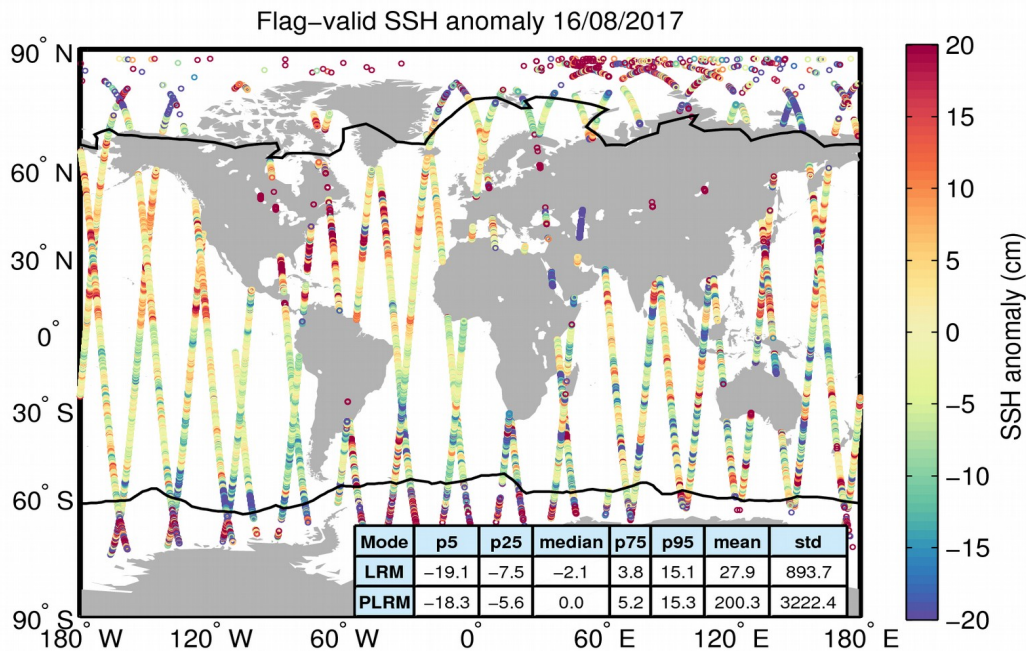
Figure 5. Geographical distribution of flag-valid 1-Hz SSH anomaly data over oceans and lakes for 16/08/2017. The statistical values shown in the table refer to the SSH anomaly in cm and are calculated separately for LRM and PLRM regions. Measurements taken over polar polygons have been excluded from the computation of the statistical values. The black lines mark the outer limit of the Arctic and Antarctic polar polygons.
