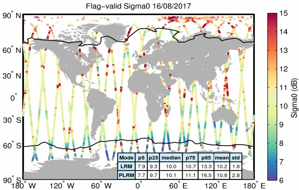
Figure 23. Geographical distribution of flag-valid sigma0 data over oceans and lakes for 16/08/2017. The statistical values shown in the table refer to the sigma0 in dB and are calculated separately for LRM and PLRM regions. Measurements taken over polar polygons have been excluded from the computation of the statistical values. The black lines mark the outer limit of the Arctic and Antarctic polar polygons.
