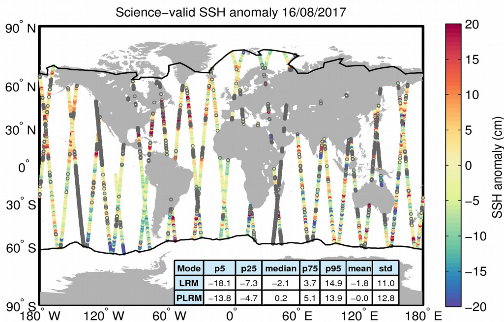
Figure 10. Geographical distribution of science-valid SSH anomaly data over oceans and lakes for 16/08/2017. The statistical values shown in the table refer to the SSH anomaly in cm and are calculated separately for LRM and PLRM regions. The black lines mark the outer limit of the Arctic and Antarctic polar polygons. Gray circles denote records that have been rejected based on the editing criteria described in Table 2.
