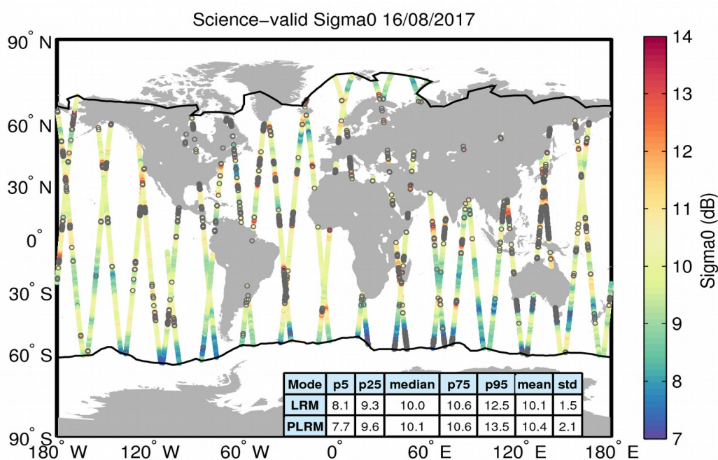
Figure 27. Geographical distribution of science-valid sigma0 data over oceans and lakes for 16/08/2017. The statistical values shown in the table refer to the sigma0 in dB and are calculated separately for LRM and PLRM regions. The black lines mark the outer limit of the Arctic and Antarctic polar polygons. Gray circles denote records that have been rejected based on the editing criteria described in Table 4.
