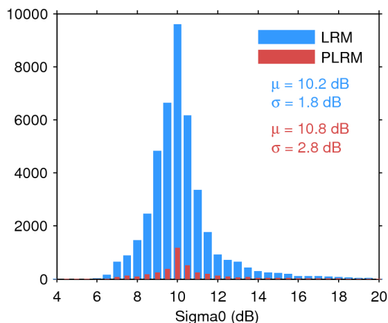
Figure 25. Histogram of flag-valid sigma0 over oceans and lakes for LRM (blue) and PLRM (red) for 16/08/2017. The mean ( \mu ) and standard deviation ( \sigma ) are also shown. Note that values outside [4 20] dB are excluded from the histogram for the sake of readability but not from the computation of \mu and \sigma .
