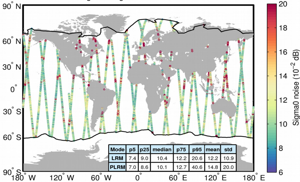
Flag-valid sigma0 noise 16/08/2017
