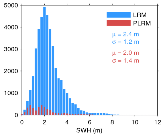
Figure 17. Histogram of flag-valid SWH over oceans and lakes for LRM (blue) and PLRM (red) for 16/08/2017. The mean ( \mu ) and standard deviation ( \sigma ) are also shown. Note that values larger than 12 m are excluded from the histogram for the sake of readability but not from the computation of \mu and \sigma .
