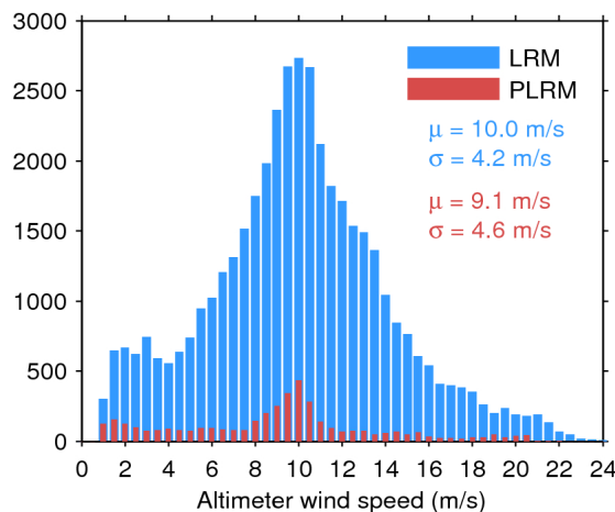
Figure 35. Histogram of science-valid wind over oceans and lakes for LRM (blue) and PLRM (red) for 16/08/2017. The mean ( \mu ) and standard deviation ( \sigma ) are also shown. Note that values larger than 24 m/s are excluded from the histogram for the sake of readability but not from the computation of \mu and \sigma .
