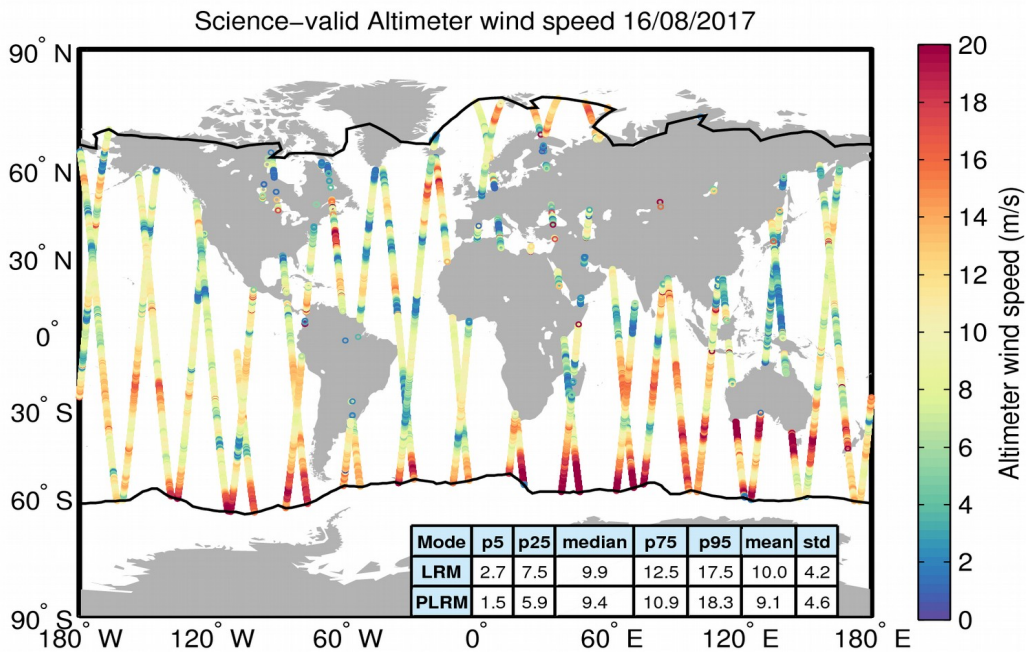
Figure 34. Geographical distribution of science-valid wind data over oceans and lakes for 16/08/2017. The statistical values shown in the table refer to the wind in m/s and are calculated separately for LRM and PLRM regions. The black lines mark the outer limit of the Arctic and Antarctic polar polygons. Gray circles denote records that have been rejected based on the editing criteria described in Table 5.
