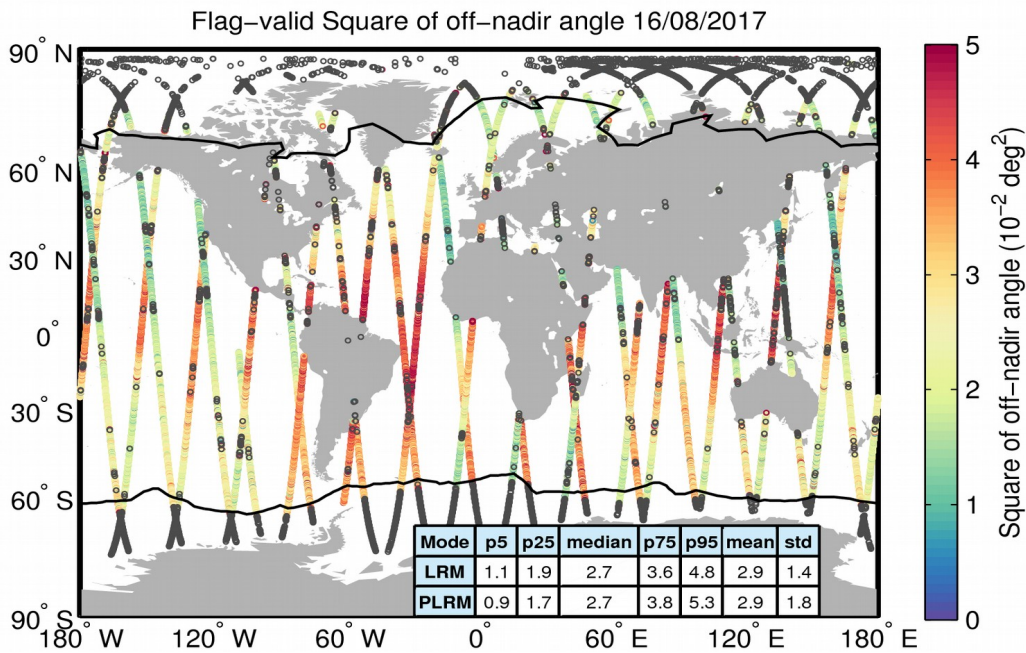
Figure 37. Geographical distribution of flag-valid mispointing data over oceans and lakes for 16/08/2017. The statistical values shown in the table refer to the mispointing in 10^{-2} deg 2 and are calculated separately for LRM and PLRM regions. Measurements taken over polar polygons have been excluded from the computation of the statistical values. The black lines mark the outer limit of the Arctic and Antarctic polar polygons. Gray circles denote negative values.
