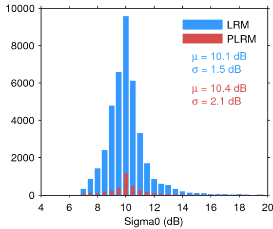
Figure 28. Histogram of science-valid sigma0 over oceans and lakes for LRM (blue) and PLRM (red) for 16/08/2017. The mean ( \mu ) and standard deviation ( \sigma ) are also shown. Note that values outside [4 20] dB are excluded from the histogram for the sake of readability but not from the computation of \mu and \sigma .
