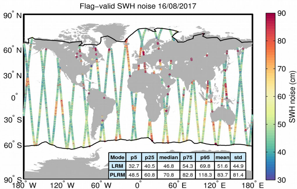
Figure 18. Geographical distribution of flag-valid 20-Hz SWH measurement noise over oceans and lakes for 16/08/2017. The statistical values shown in the table refer to the SWH noise and are calculated separately for LRM and PLRM regions. Measurements taken over polar polygons have been excluded from the computation of the statistical values. The black lines mark the outer limit of the Arctic and Antarctic polar polygons.
