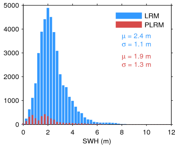
Figure 20. Histogram of science-valid SWH over oceans and lakes for LRM (blue) and PLRM (red) for 16/08/2017. The mean ( \mu ) and standard deviation ( \sigma ) are also shown. Note that values larger than 12 m are excluded from the histogram for the sake of readability but not from the computation of \mu and \sigma .
