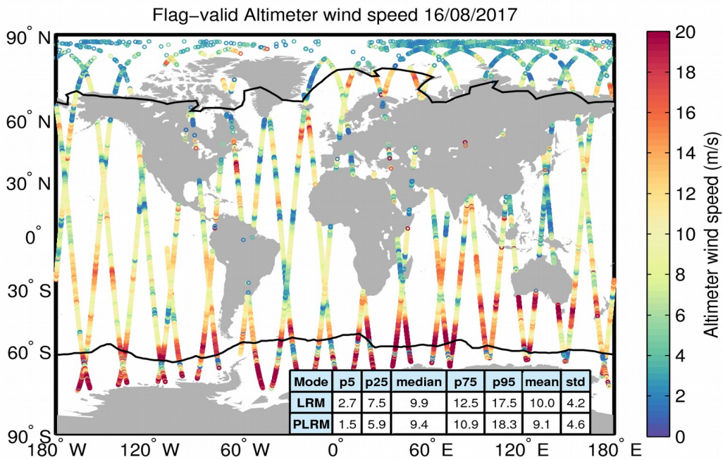
Figure 31. Geographical distribution of flag-valid wind data over oceans and lakes for 16/08/2017. The statistical values shown in the table refer to the wind in m/s and are calculated separately for LRM and PLRM regions. Measurements taken over polar polygons have been excluded from the computation of the statistical values. The black lines mark the outer limit of the Arctic and Antarctic polar polygons.
