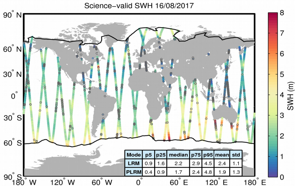
Figure 19. Geographical distribution of science-valid SWH data over oceans and lakes for 16/08/2017. The statistical values shown in the table refer to the SWH in m and are calculated separately for LRM and PLRM regions. The black lines mark the outer limit of the Arctic and Antarctic polar polygons. Gray circles denote records that have been rejected based on the editing criteria described in Table 3.
