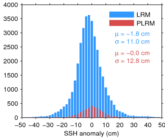
Figure 11. Histogram of science-valid SSH anomaly over oceans and lakes for LRM (blue) and PLRM (red) for 16/08/2017. The mean ( \mu ) and standard deviation ( \sigma ) are also shown. Note that values outside [-50\ 50] cm are excluded from the histogram for the sake of readability but not from the computation of \mu and \sigma .
