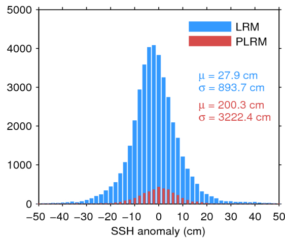
Figure 7. Histogram of flag-valid SSH anomaly over oceans and lakes for LRM (blue) and PLRM (red) for 16/08/2017. The mean ( \mu ) and standard deviation ( \sigma ) are also shown. Note that values outside [-50\ 50] cm are excluded from the histogram for the sake of readability but not from the computation of \mu and \sigma .
