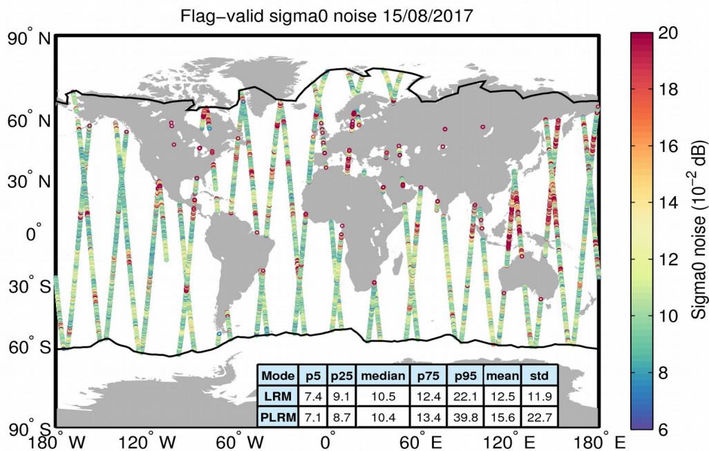
Figure 26. Geographical distribution of flag-valid 20-Hz sigma0 measurement noise over oceans and lakes for 15/08/2017. The statistical values shown in the table refer to the sigma0 noise and are calculated separately for LRM and PLRM regions. Measurements taken over polar polygons have been excluded from the computation of the statistical values. The black lines mark the outer limit of the Arctic and Antarctic polar polygons.
