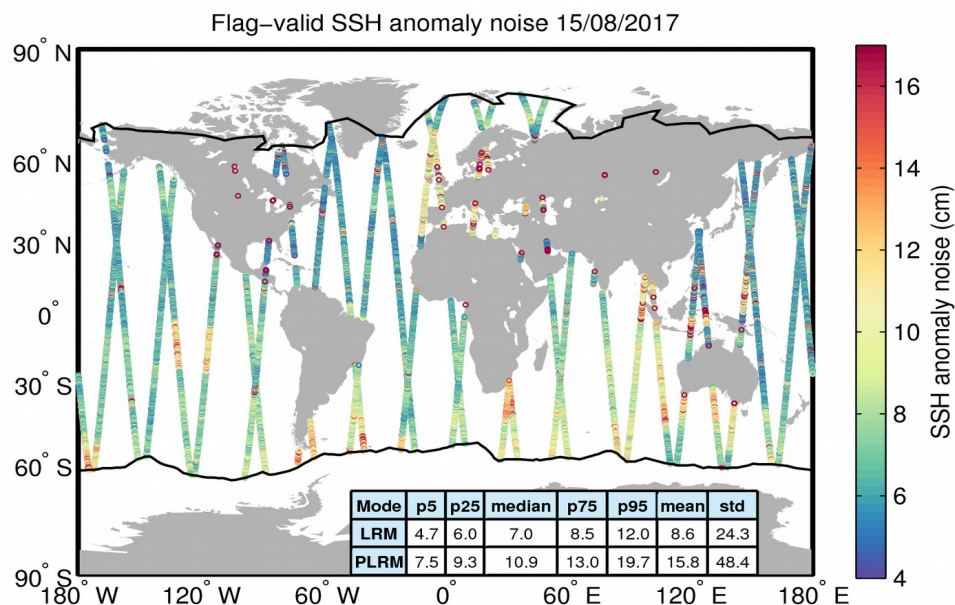
Figure 8. Geographical distribution of flag-valid 20-Hz SSH anomaly measurement noise over oceans and lakes for 15/08/2017. The statistical values shown in the table refer to the SSH anomaly noise and are calculated separately for LRM and PLRM regions. Measurements taken over polar polygons have been excluded from the computation of the statistical values. The black lines mark the outer limit of the Arctic and Antarctic polar polygons.
