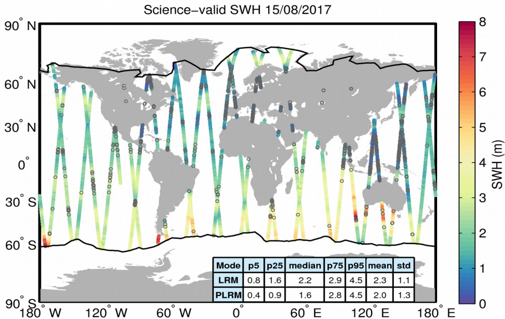
Figure 19. Geographical distribution of science-valid SWH data over oceans and lakes for 15/08/2017. The statistical values shown in the table refer to the SWH in m and are calculated separately for LRM and PLRM regions. The black lines mark the outer limit of the Arctic and Antarctic polar polygons. Gray circles denote records that have been rejected based on the editing criteria described in Table 3.
