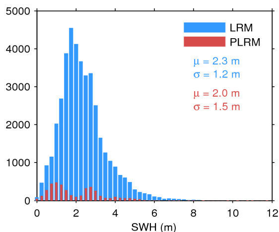
Figure 17. Histogram of flag-valid SWH over oceans and lakes for LRM (blue) and PLRM (red) for 15/08/2017. The mean ( \mu ) and standard deviation ( \sigma ) are also shown. Note that values larger than 12 m are excluded from the histogram for the sake of readability but not from the computation of \mu and \sigma .
