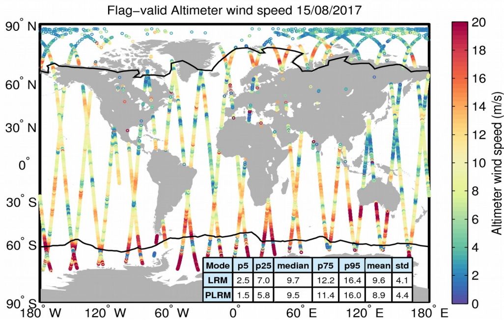
Figure 31. Geographical distribution of flag-valid wind data over oceans and lakes for 15/08/2017. The statistical values shown in the table refer to the wind in m/s and are calculated separately for LRM and PLRM regions. Measurements taken over polar polygons have been excluded from the computation of the statistical values. The black lines mark the outer limit of the Arctic and Antarctic polar polygons.
