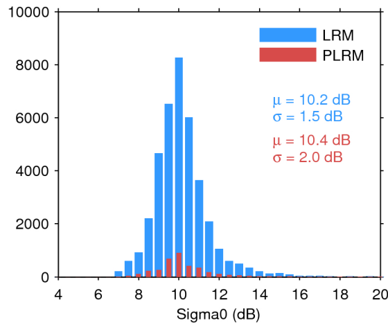
Figure 28. Histogram of science-valid sigma0 over oceans and lakes for LRM (blue) and PLRM (red) for 15/08/2017. The mean ( \mu ) and standard deviation ( \sigma ) are also shown. Note that values outside [4 20] dB are excluded from the histogram for the sake of readability but not from the computation of \mu and \sigma .
