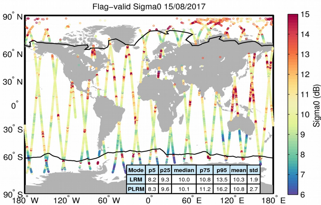
Figure 23. Geographical distribution of flag-valid sigma0 data over oceans and lakes for 15/08/2017. The statistical values shown in the table refer to the sigma0 in dB and are calculated separately for LRM and PLRM regions. Measurements taken over polar polygons have been excluded from the computation of the statistical values. The black lines mark the outer limit of the Arctic and Antarctic polar polygons.
