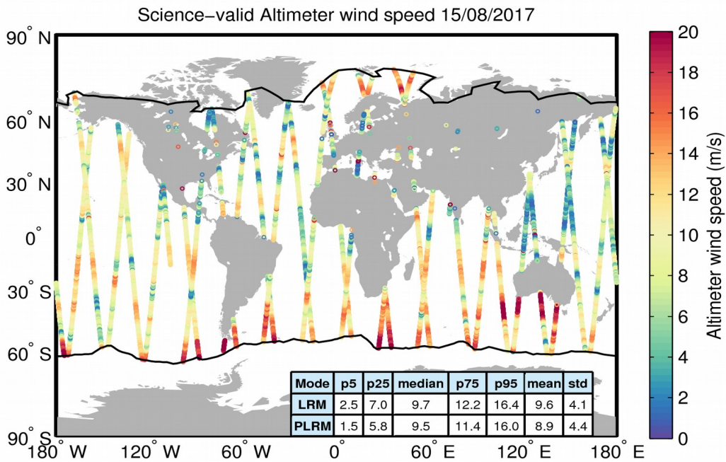
Figure 34. Geographical distribution of science-valid wind data over oceans and lakes for 15/08/2017. The statistical values shown in the table refer to the wind in m/s and are calculated separately for LRM and PLRM regions. The black lines mark the outer limit of the Arctic and Antarctic polar polygons. Gray circles denote records that have been rejected based on the editing criteria described in Table 5.
