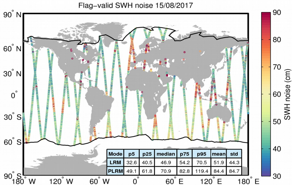
Figure 18. Geographical distribution of flag-valid 20-Hz SWH measurement noise over oceans and lakes for 15/08/2017. The statistical values shown in the table refer to the SWH noise and are calculated separately for LRM and PLRM regions. Measurements taken over polar polygons have been excluded from the computation of the statistical values. The black lines mark the outer limit of the Arctic and Antarctic polar polygons.
