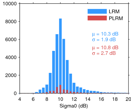
Figure 25. Histogram of flag-valid sigma0 over oceans and lakes for LRM (blue) and PLRM (red) for 15/08/2017. The mean ( \mu ) and standard deviation ( \sigma ) are also shown. Note that values outside [4 20] dB are excluded from the histogram for the sake of readability but not from the computation of \mu and \sigma .
