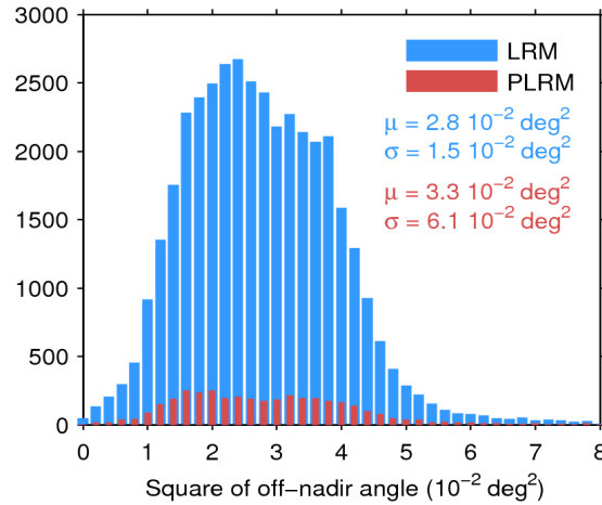
Figure 39. Histogram of flag-valid mispointing over oceans and lakes for LRM (blue) and PLRM (red) for 15/08/2017. Only positive values have been considered. The mean ( \mu ) and standard deviation ( \sigma ) are also shown. Note that values larger than 8 \cdot 10^{-2} \text{ deg}^2 are excluded from the histogram for the sake of readability but not from the computation of \mu and \sigma .
