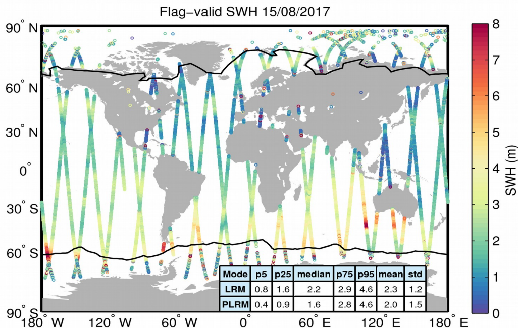
Figure 15. Geographical distribution of flag-valid SWH data over oceans and lakes for 15/08/2017. The statistical values shown in the table refer to the SWH in m and are calculated separately for LRM and PLRM regions. Measurements taken over polar polygons have been excluded from the computation of the statistical values. The black lines mark the outer limit of the Arctic and Antarctic polar polygons.
