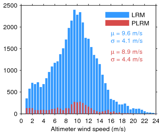
Figure 35. Histogram of science-valid wind over oceans and lakes for LRM (blue) and PLRM (red) for 15/08/2017. The mean ( \mu ) and standard deviation ( \sigma ) are also shown. Note that values larger than 24 m/s are excluded from the histogram for the sake of readability but not from the computation of \mu and \sigma .
