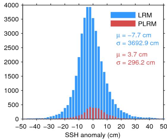
Figure 7. Histogram of flag-valid SSH anomaly over oceans and lakes for LRM (blue) and PLRM (red) for 15/08/2017. The mean ( \mu ) and standard deviation ( \sigma ) are also shown. Note that values outside [-50 50] cm are excluded from the histogram for the sake of readability but not from the computation of \mu and \sigma .
