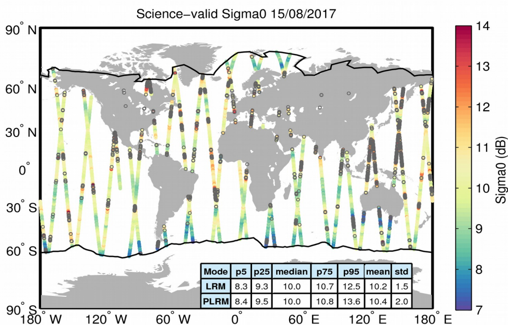
Figure 27. Geographical distribution of science-valid sigma0 data over oceans and lakes for 15/08/2017. The statistical values shown in the table refer to the sigma0 in dB and are calculated separately for LRM and PLRM regions. The black lines mark the outer limit of the Arctic and Antarctic polar polygons. Gray circles denote records that have been rejected based on the editing criteria described in Table 4.
