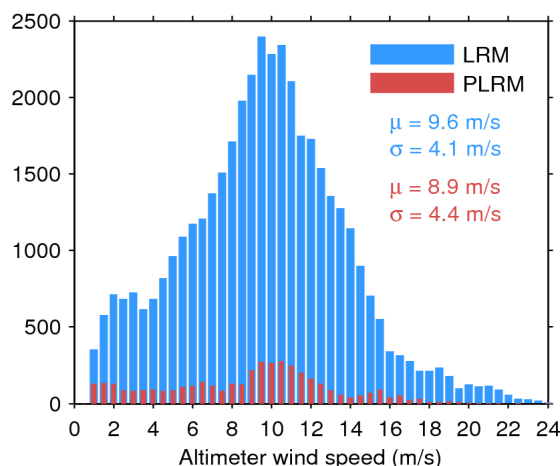
Figure 33. Histogram of flag-valid wind over oceans and lakes for LRM (blue) and PLRM (red) for 15/08/2017. The mean ( \mu ) and standard deviation ( \sigma ) are also shown. Note that values larger than 24 m/s are excluded from the histogram for the sake of readability but not from the computation of \mu and \sigma .
