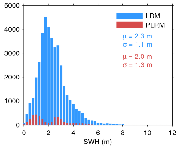
Figure 20. Histogram of science-valid SWH over oceans and lakes for LRM (blue) and PLRM (red) for 15/08/2017. The mean ( \mu ) and standard deviation ( \sigma ) are also shown. Note that values larger than 12 m are excluded from the histogram for the sake of readability but not from the computation of \mu and \sigma .
