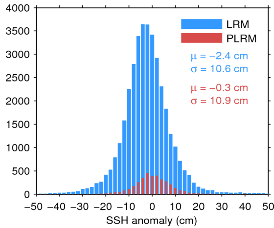
Figure 11. Histogram of science-valid SSH anomaly over oceans and lakes for LRM (blue) and PLRM (red) for 14/08/2017. The mean ( \mu ) and standard deviation ( \sigma ) are also shown. Note that values outside [-50 50] cm are excluded from the histogram for the sake of readability but not from the computation of \mu and \sigma .
