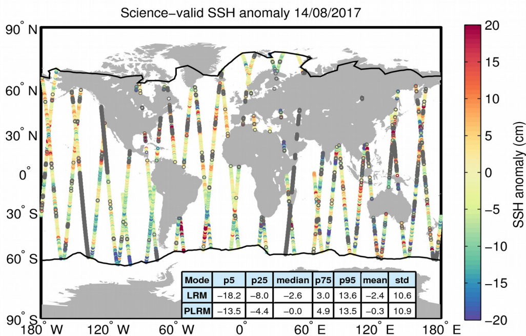
Figure 10. Geographical distribution of science-valid SSH anomaly data over oceans and lakes for 14/08/2017. The statistical values shown in the table refer to the SSH anomaly in cm and are calculated separately for LRM and PLRM regions. The black lines mark the outer limit of the Arctic and Antarctic polar polygons. Gray circles denote records that have been rejected based on the editing criteria described in Table 2.
