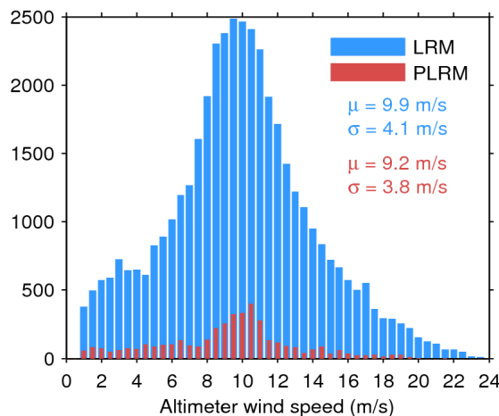
Figure 35. Histogram of science-valid wind over oceans and lakes for LRM (blue) and PLRM (red) for 14/08/2017. The mean ( \mu ) and standard deviation ( \sigma ) are also shown. Note that values larger than 24 m/s are excluded from the histogram for the sake of readability but not from the computation of \mu and \sigma .
