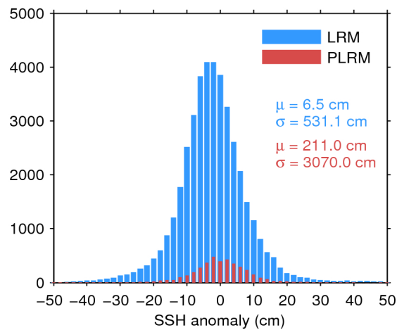
Figure 7. Histogram of flag-valid SSH anomaly over oceans and lakes for LRM (blue) and PLRM (red) for 14/08/2017. The mean ( \mu ) and standard deviation ( \sigma ) are also shown. Note that values outside [-50\ 50] cm are excluded from the histogram for the sake of readability but not from the computation of \mu and \sigma .
