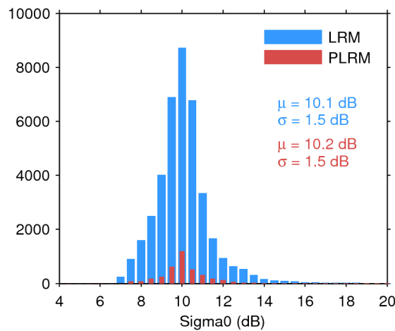
Figure 28. Histogram of science-valid sigma0 over oceans and lakes for LRM (blue) and PLRM (red) for 14/08/2017. The mean ( \mu ) and standard deviation ( \sigma ) are also shown. Note that values outside [4 20] dB are excluded from the histogram for the sake of readability but not from the computation of \mu and \sigma .
