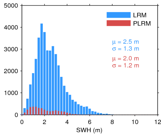
Figure 20. Histogram of science-valid SWH over oceans and lakes for LRM (blue) and PLRM (red) for 14/08/2017. The mean ( \mu ) and standard deviation ( \sigma ) are also shown. Note that values larger than 12 m are excluded from the histogram for the sake of readability but not from the computation of \mu and \sigma .
