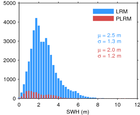
Figure 17. Histogram of flag-valid SWH over oceans and lakes for LRM (blue) and PLRM (red) for 14/08/2017. The mean ( \mu ) and standard deviation ( \sigma ) are also shown. Note that values larger than 12 m are excluded from the histogram for the sake of readability but not from the computation of \mu and \sigma .
