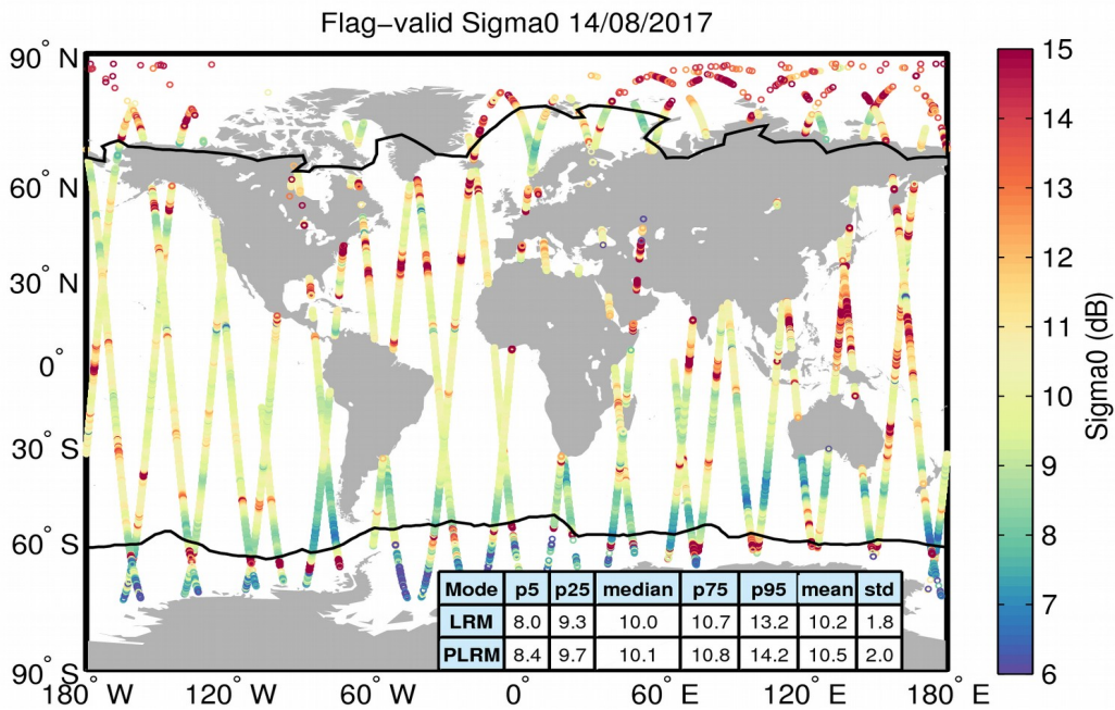
Figure 23. Geographical distribution of flag-valid sigma0 data over oceans and lakes for 14/08/2017. The statistical values shown in the table refer to the sigma0 in dB and are calculated separately for LRM and PLRM regions. Measurements taken over polar polygons have been excluded from the computation of the statistical values. The black lines mark the outer limit of the Arctic and Antarctic polar polygons.
