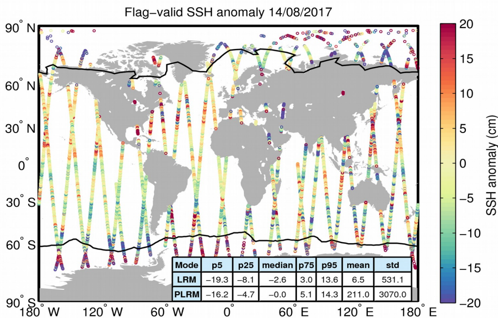
Figure 5. Geographical distribution of flag-valid 1-Hz SSH anomaly data over oceans and lakes for 14/08/2017. The statistical values shown in the table refer to the SSH anomaly in cm and are calculated separately for LRM and PLRM regions. Measurements taken over polar polygons have been excluded from the computation of the statistical values. The black lines mark the outer limit of the Arctic and Antarctic polar polygons.
