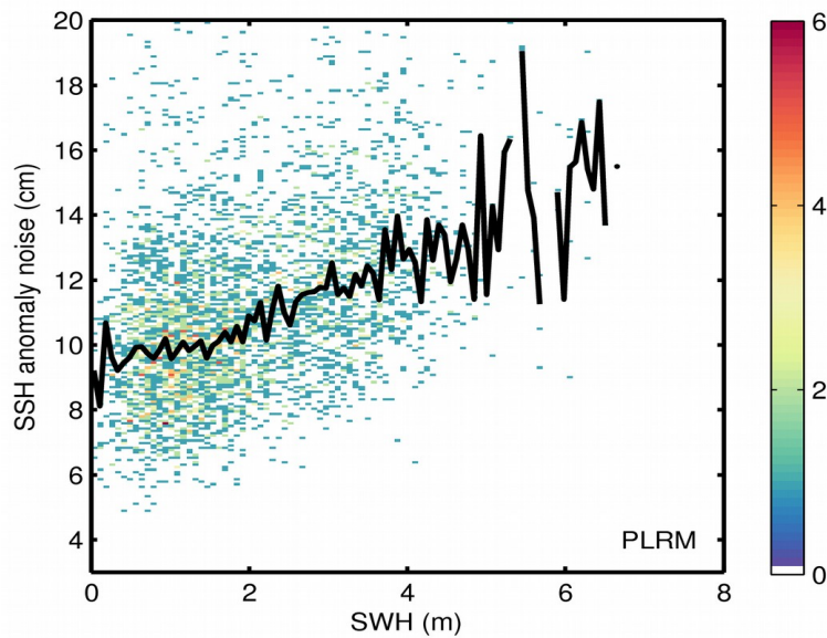
Figure 9. 2D histogram showing flag-valid SSH anomaly noise as a function of SWH for LRM (top) and PLRM (bottom) for 14/08/2017. The black line denotes the median SSH anomaly noise as a function of SWH.
