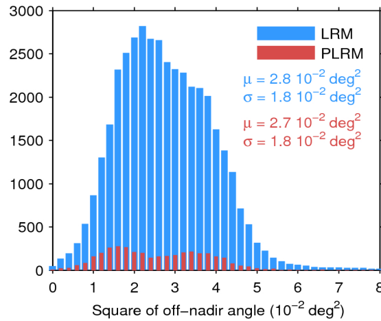
Figure 39. Histogram of flag-valid mispointing over oceans and lakes for LRM (blue) and PLRM (red) for 14/08/2017. Only positive values have been considered. The mean ( \mu ) and standard deviation ( \sigma ) are also shown. Note that values larger than 8 \cdot 10^{-2} \text{ deg}^2 are excluded from the histogram for the sake of readability but not from the computation of \mu and \sigma .
