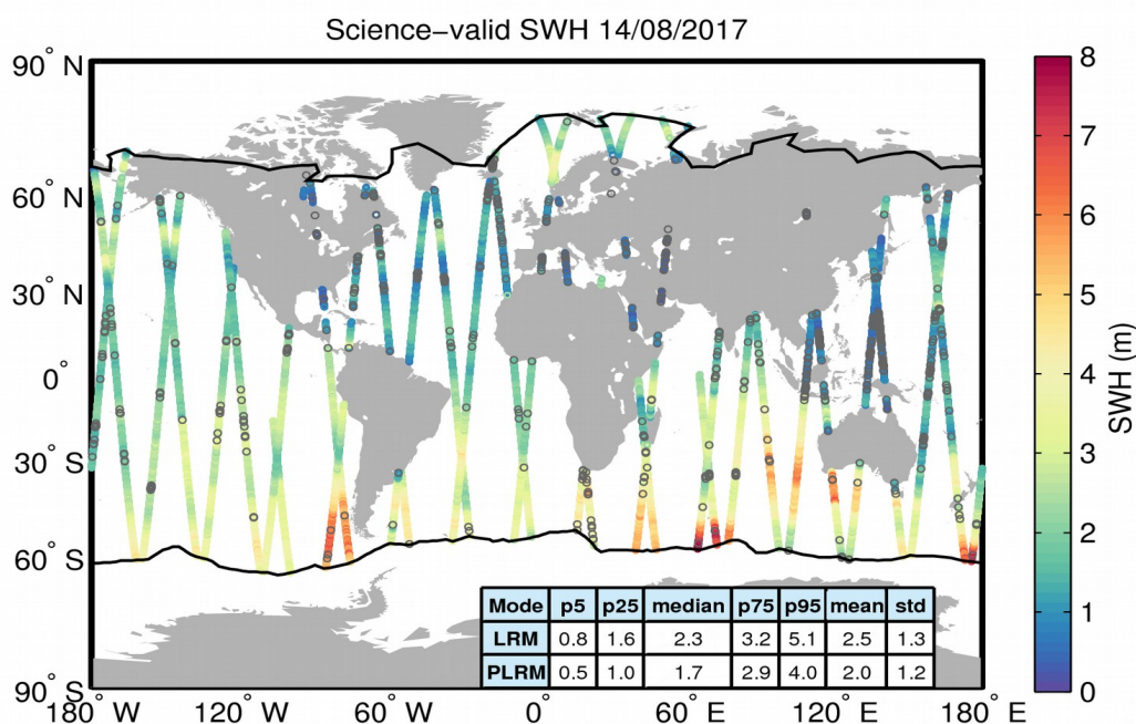
Figure 19. Geographical distribution of science-valid SWH data over oceans and lakes for 14/08/2017. The statistical values shown in the table refer to the SWH in m and are calculated separately for LRM and PLRM regions. The black lines mark the outer limit of the Arctic and Antarctic polar polygons. Gray circles denote records that have been rejected based on the editing criteria described in Table 3.
