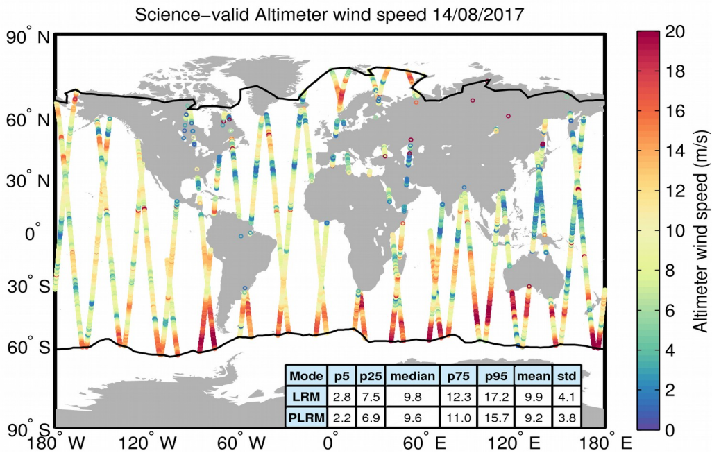
Figure 34. Geographical distribution of science-valid wind data over oceans and lakes for 14/08/2017. The statistical values shown in the table refer to the wind in m/s and are calculated separately for LRM and PLRM regions. The black lines mark the outer limit of the Arctic and Antarctic polar polygons. Gray circles denote records that have been rejected based on the editing criteria described in Table 5.
