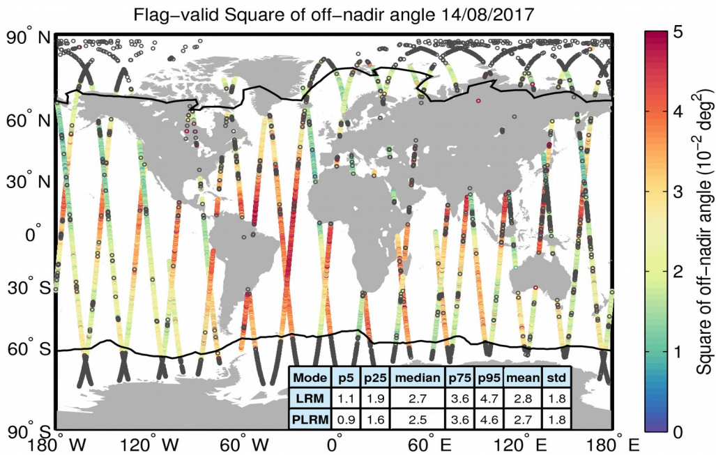
Figure 37. Geographical distribution of flag-valid mispointing data over oceans and lakes for 14/08/2017. The statistical values shown in the table refer to the mispointing in 10^{-2} deg 2 and are calculated separately for LRM and PLRM regions. Measurements taken over polar polygons have been excluded from the computation of the statistical values. The black lines mark the outer limit of the Arctic and Antarctic polar polygons. Gray circles denote negative values.
