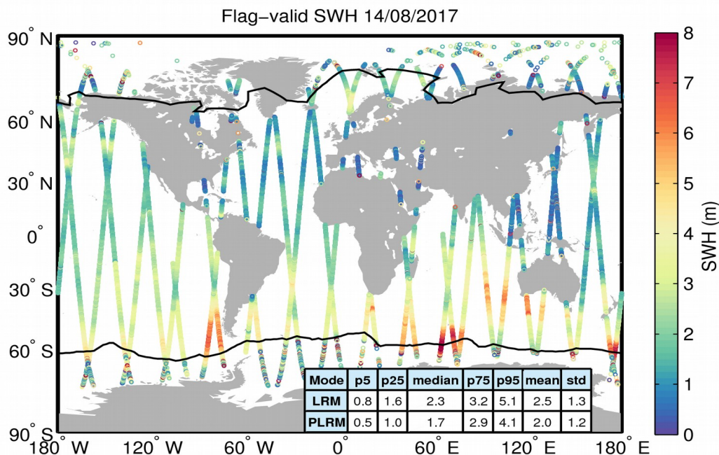
Figure 15. Geographical distribution of flag-valid SWH data over oceans and lakes for 14/08/2017. The statistical values shown in the table refer to the SWH in m and are calculated separately for LRM and PLRM regions. Measurements taken over polar polygons have been excluded from the computation of the statistical values. The black lines mark the outer limit of the Arctic and Antarctic polar polygons.
