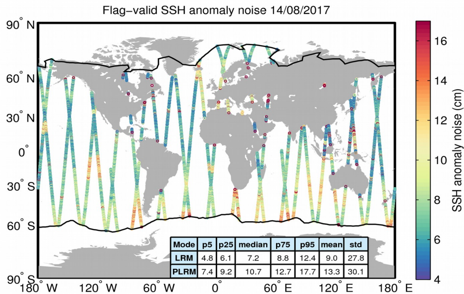
Figure 8. Geographical distribution of flag-valid 20-Hz SSH anomaly measurement noise over oceans and lakes for 14/08/2017. The statistical values shown in the table refer to the SSH anomaly noise and are calculated separately for LRM and PLRM regions. Measurements taken over polar polygons have been excluded from the computation of the statistical values. The black lines mark the outer limit of the Arctic and Antarctic polar polygons.
