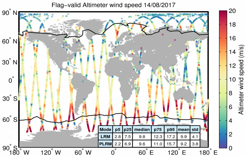
Figure 31. Geographical distribution of flag-valid wind data over oceans and lakes for 14/08/2017. The statistical values shown in the table refer to the wind in m/s and are calculated separately for LRM and PLRM regions. Measurements taken over polar polygons have been excluded from the computation of the statistical values. The black lines mark the outer limit of the Arctic and Antarctic polar polygons.
