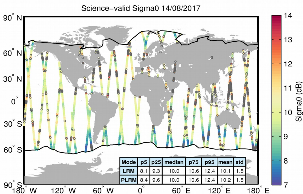
Figure 27. Geographical distribution of science-valid sigma0 data over oceans and lakes for 14/08/2017. The statistical values shown in the table refer to the sigma0 in dB and are calculated separately for LRM and PLRM regions. The black lines mark the outer limit of the Arctic and Antarctic polar polygons. Gray circles denote records that have been rejected based on the editing criteria described in Table 4.
