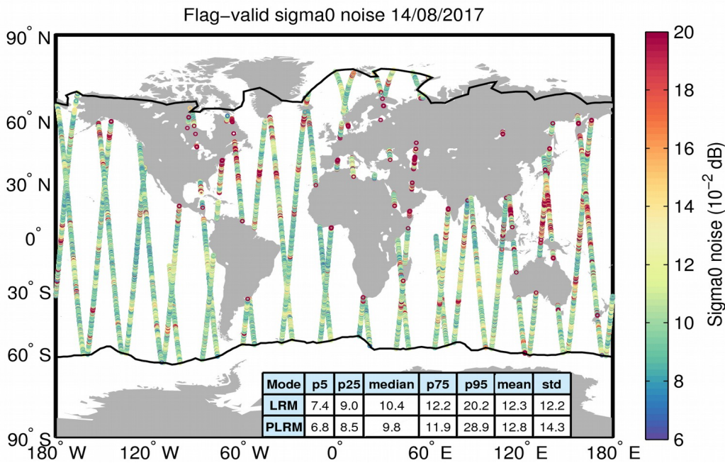
Figure 26. Geographical distribution of flag-valid 20-Hz sigma0 measurement noise over oceans and lakes for 14/08/2017. The statistical values shown in the table refer to the sigma0 noise and are calculated separately for LRM and PLRM regions. Measurements taken over polar polygons have been excluded from the computation of the statistical values. The black lines mark the outer limit of the Arctic and Antarctic polar polygons.
