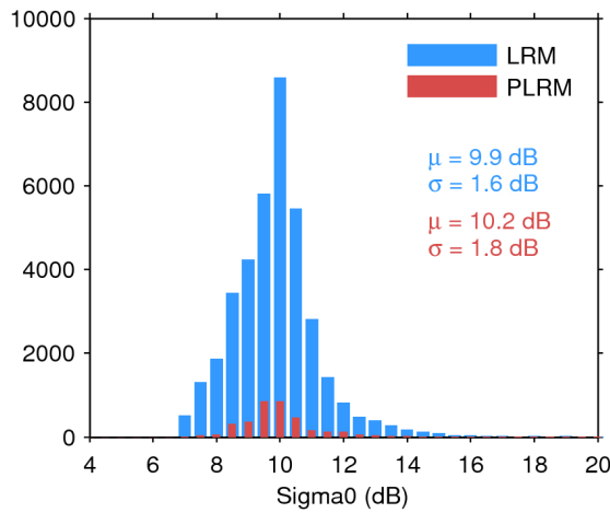
Figure 28. Histogram of science-valid sigma0 over oceans and lakes for LRM (blue) and PLRM (red) for 13/08/2017. The mean ( \mu ) and standard deviation ( \sigma ) are also shown. Note that values outside [4 20] dB are excluded from the histogram for the sake of readability but not from the computation of \mu and \sigma .
