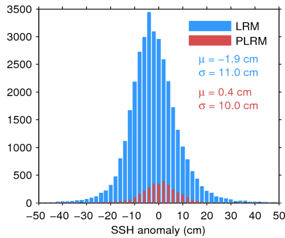
Figure 11. Histogram of science-valid SSH anomaly over oceans and lakes for LRM (blue) and PLRM (red) for 13/08/2017. The mean ( \mu ) and standard deviation ( \sigma ) are also shown. Note that values outside [-50\ 50] cm are excluded from the histogram for the sake of readability but not from the computation of \mu and \sigma .
