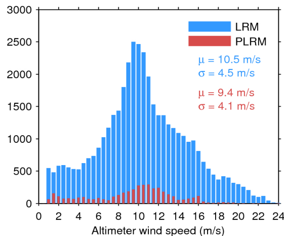
Figure 35. Histogram of science-valid wind over oceans and lakes for LRM (blue) and PLRM (red) for 13/08/2017. The mean ( \mu ) and standard deviation ( \sigma ) are also shown. Note that values larger than 24 m/s are excluded from the histogram for the sake of readability but not from the computation of \mu and \sigma .
