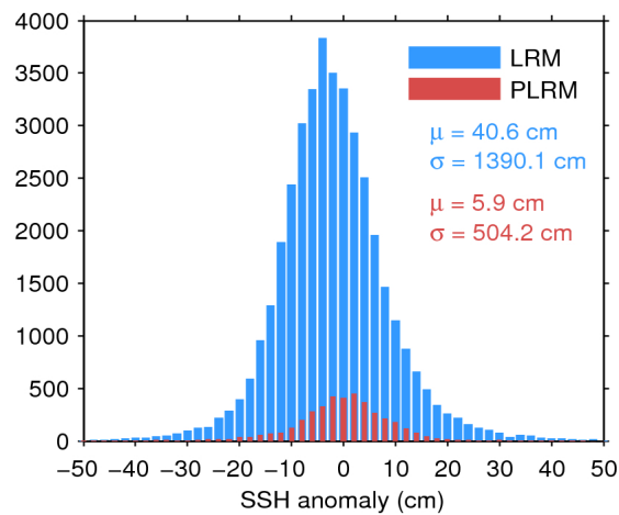
Figure 7. Histogram of flag-valid SSH anomaly over oceans and lakes for LRM (blue) and PLRM (red) for 13/08/2017. The mean ( \mu ) and standard deviation ( \sigma ) are also shown. Note that values outside [-50\ 50] cm are excluded from the histogram for the sake of readability but not from the computation of \mu and \sigma .
