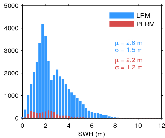
Figure 20. Histogram of science-valid SWH over oceans and lakes for LRM (blue) and PLRM (red) for 13/08/2017. The mean ( \mu ) and standard deviation ( \sigma ) are also shown. Note that values larger than 12 m are excluded from the histogram for the sake of readability but not from the computation of \mu and \sigma .
