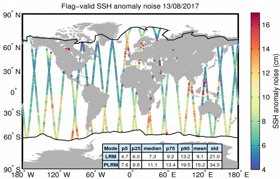
Figure 8. Geographical distribution of flag-valid 20-Hz SSH anomaly measurement noise over oceans and lakes for 13/08/2017. The statistical values shown in the table refer to the SSH anomaly noise and are calculated separately for LRM and PLRM regions. Measurements taken over polar polygons have been excluded from the computation of the statistical values. The black lines mark the outer limit of the Arctic and Antarctic polar polygons.
