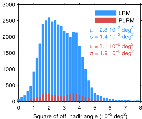
Figure 39. Histogram of flag-valid mispointing over oceans and lakes for LRM (blue) and PLRM (red) for 13/08/2017. Only positive values have been considered. The mean ( \mu ) and standard deviation ( \sigma ) are also shown. Note that values larger than 8 \cdot 10^{-2} \text{ deg}^2 are excluded from the histogram for the sake of readability but not from the computation of \mu and \sigma .
