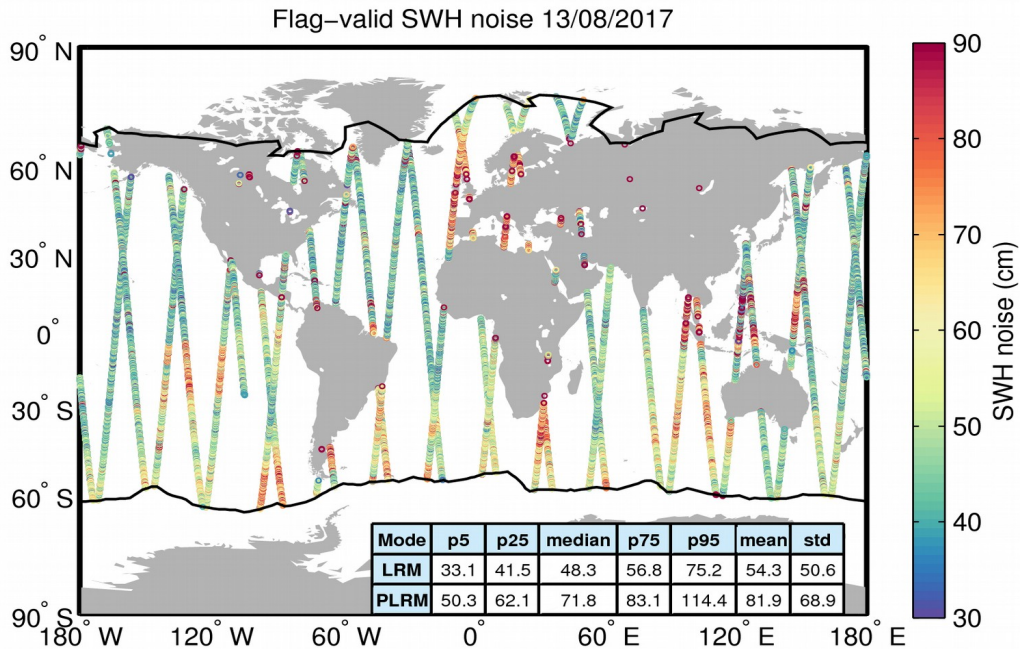
Figure 18. Geographical distribution of flag-valid 20-Hz SWH measurement noise over oceans and lakes for 13/08/2017. The statistical values shown in the table refer to the SWH noise and are calculated separately for LRM and PLRM regions. Measurements taken over polar polygons have been excluded from the computation of the statistical values. The black lines mark the outer limit of the Arctic and Antarctic polar polygons.
