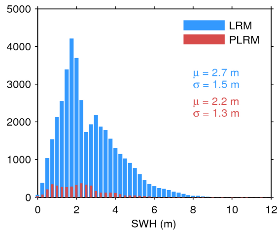
Figure 17. Histogram of flag-valid SWH over oceans and lakes for LRM (blue) and PLRM (red) for 13/08/2017. The mean ( \mu ) and standard deviation ( \sigma ) are also shown. Note that values larger than 12 m are excluded from the histogram for the sake of readability but not from the computation of \mu and \sigma .
