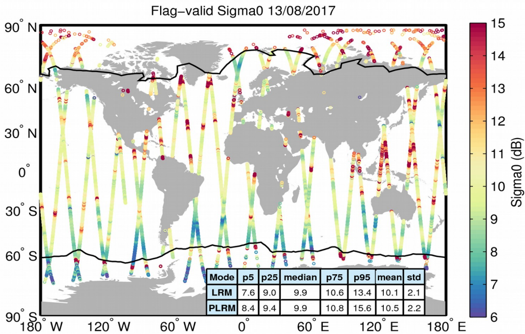
Figure 23. Geographical distribution of flag-valid sigma0 data over oceans and lakes for 13/08/2017. The statistical values shown in the table refer to the sigma0 in dB and are calculated separately for LRM and PLRM regions. Measurements taken over polar polygons have been excluded from the computation of the statistical values. The black lines mark the outer limit of the Arctic and Antarctic polar polygons.
