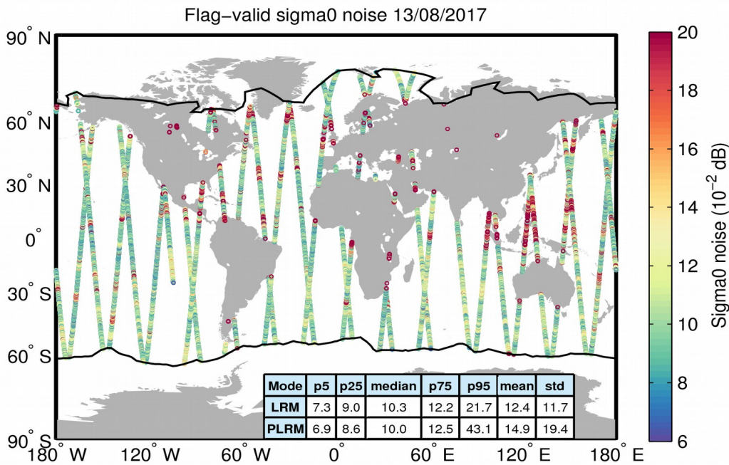
Figure 26. Geographical distribution of flag-valid 20-Hz sigma0 measurement noise over oceans and lakes for 13/08/2017. The statistical values shown in the table refer to the sigma0 noise and are calculated separately for LRM and PLRM regions. Measurements taken over polar polygons have been excluded from the computation of the statistical values. The black lines mark the outer limit of the Arctic and Antarctic polar polygons.
