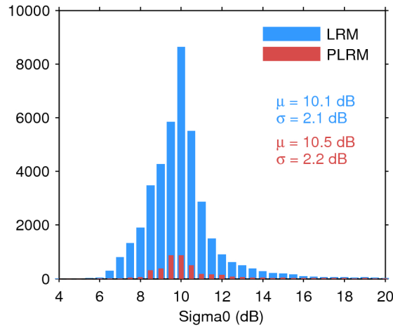
Figure 25. Histogram of flag-valid sigma0 over oceans and lakes for LRM (blue) and PLRM (red) for 13/08/2017. The mean ( \mu ) and standard deviation ( \sigma ) are also shown. Note that values outside [4 20] dB are excluded from the histogram for the sake of readability but not from the computation of \mu and \sigma .
