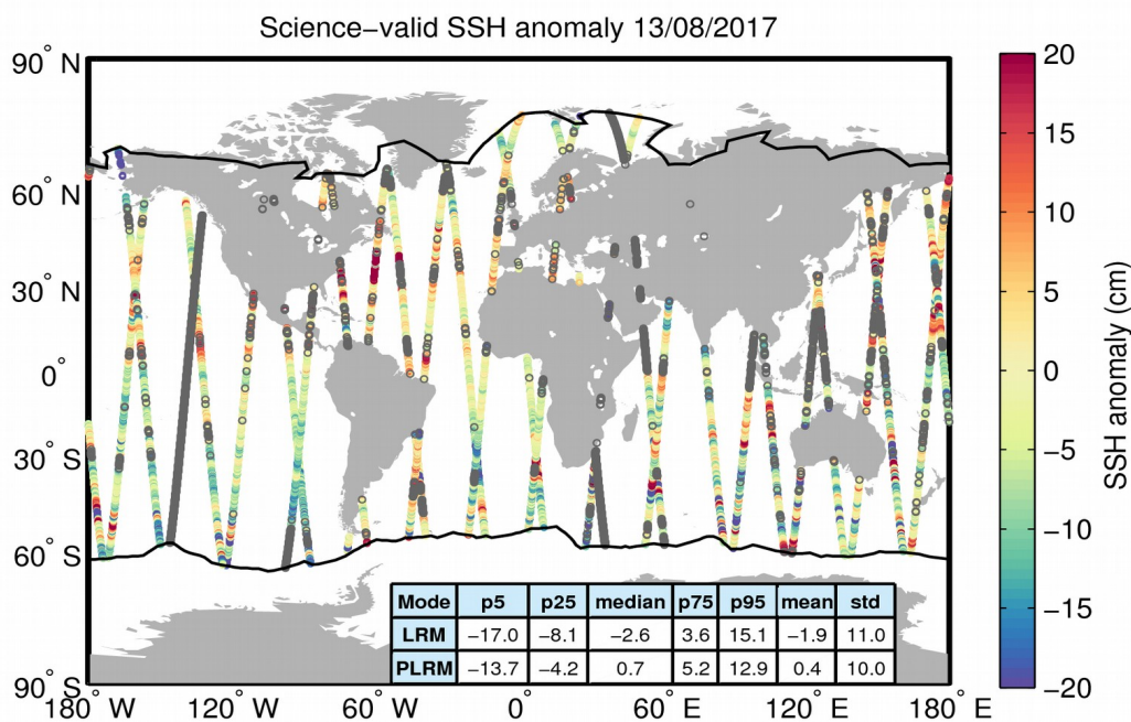
Figure 10. Geographical distribution of science-valid SSH anomaly data over oceans and lakes for 13/08/2017. The statistical values shown in the table refer to the SSH anomaly in cm and are calculated separately for LRM and PLRM regions. The black lines mark the outer limit of the Arctic and Antarctic polar polygons. Gray circles denote records that have been rejected based on the editing criteria described in Table 2.
