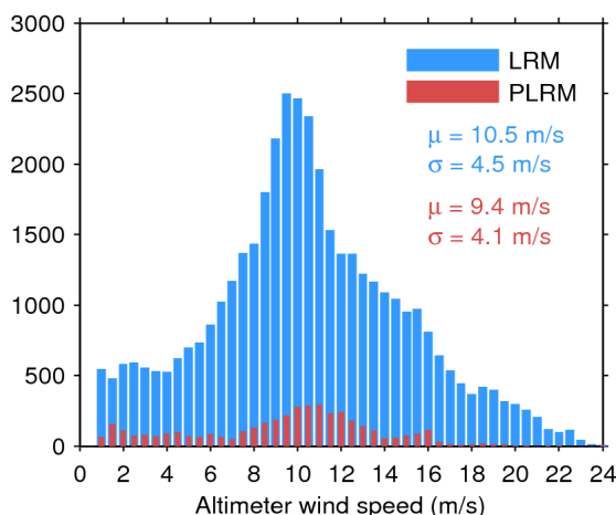
Figure 33. Histogram of flag-valid wind over oceans and lakes for LRM (blue) and PLRM (red) for 13/08/2017. The mean ( \mu ) and standard deviation ( \sigma ) are also shown. Note that values larger than 24 m/s are excluded from the histogram for the sake of readability but not from the computation of \mu and \sigma .
