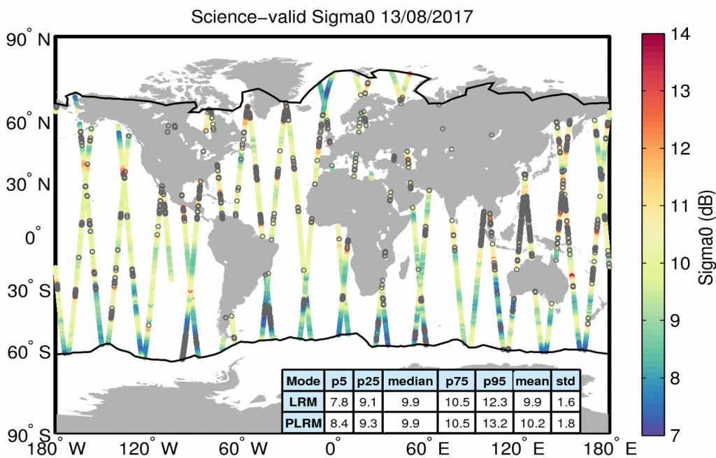
Figure 27. Geographical distribution of science-valid sigma0 data over oceans and lakes for 13/08/2017. The statistical values shown in the table refer to the sigma0 in dB and are calculated separately for LRM and PLRM regions. The black lines mark the outer limit of the Arctic and Antarctic polar polygons. Gray circles denote records that have been rejected based on the editing criteria described in Table 4.
