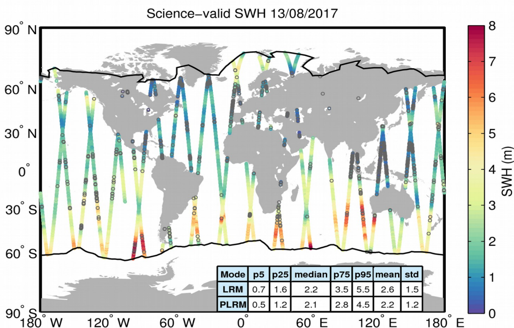
Figure 19. Geographical distribution of science-valid SWH data over oceans and lakes for 13/08/2017. The statistical values shown in the table refer to the SWH in m and are calculated separately for LRM and PLRM regions. The black lines mark the outer limit of the Arctic and Antarctic polar polygons. Gray circles denote records that have been rejected based on the editing criteria described in Table 3.
