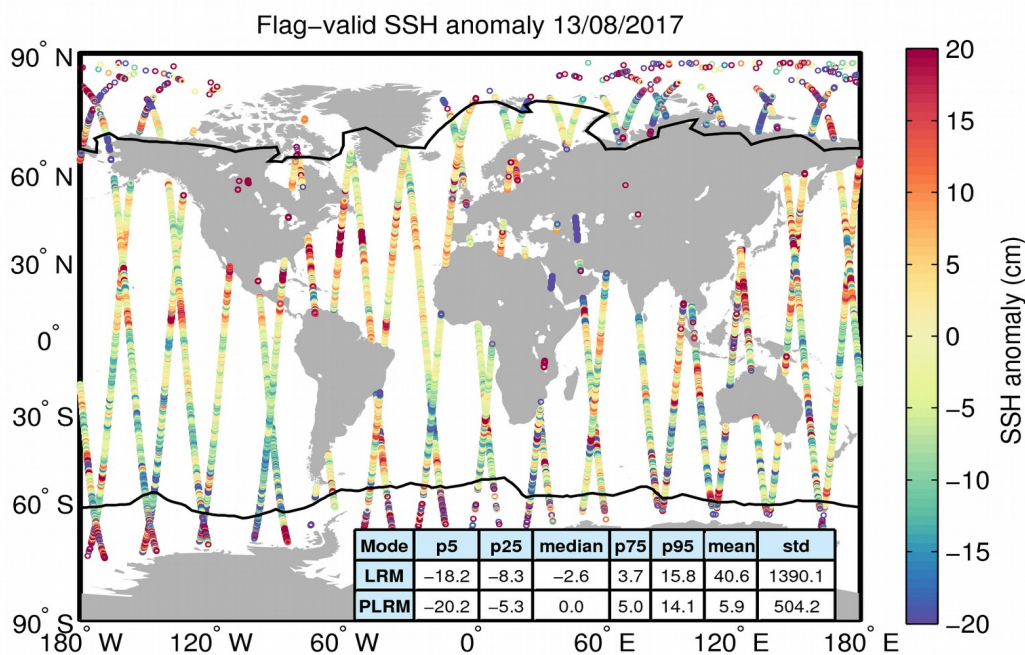
Figure 5. Geographical distribution of flag-valid 1-Hz SSH anomaly data over oceans and lakes for 13/08/2017. The statistical values shown in the table refer to the SSH anomaly in cm and are calculated separately for LRM and PLRM regions. Measurements taken over polar polygons have been excluded from the computation of the statistical values. The black lines mark the outer limit of the Arctic and Antarctic polar polygons.
