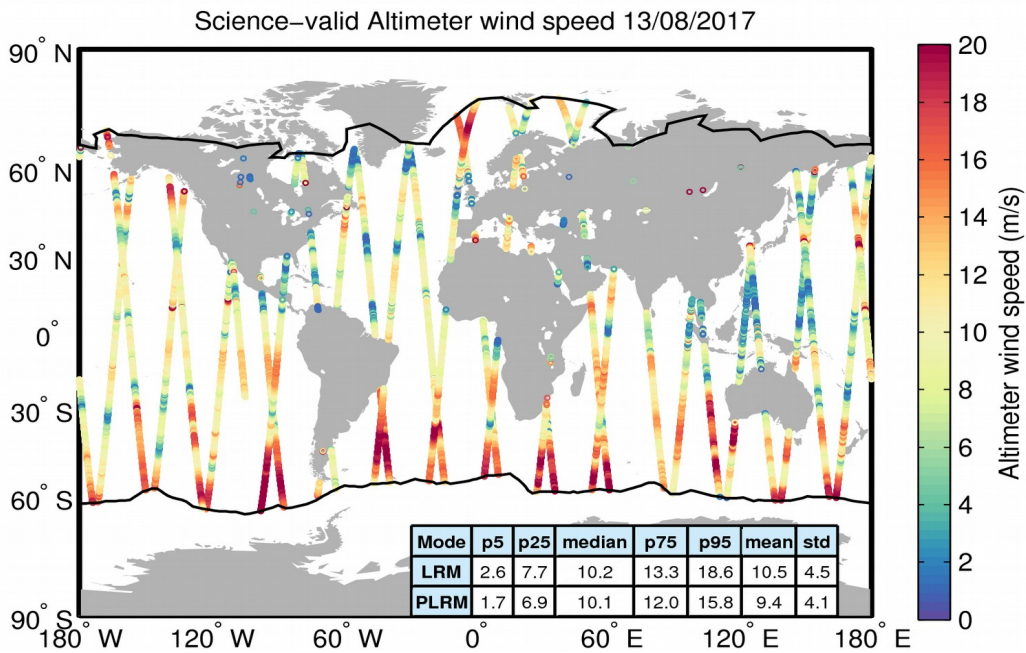
Figure 34. Geographical distribution of science-valid wind data over oceans and lakes for 13/08/2017. The statistical values shown in the table refer to the wind in m/s and are calculated separately for LRM and PLRM regions. The black lines mark the outer limit of the Arctic and Antarctic polar polygons. Gray circles denote records that have been rejected based on the editing criteria described in Table 5.
