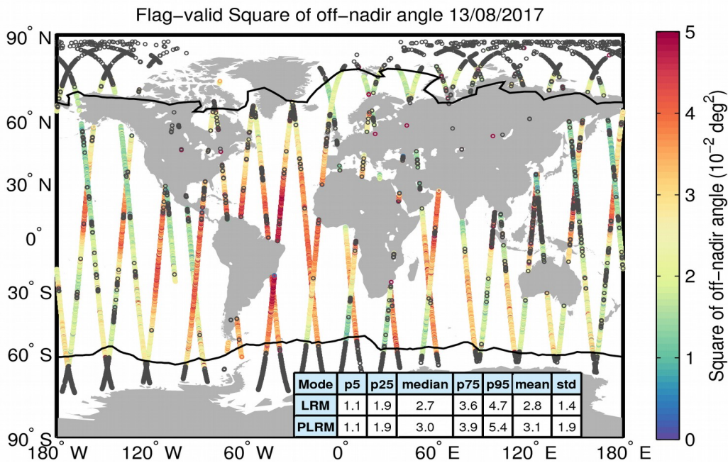
Figure 37. Geographical distribution of flag-valid mispointing data over oceans and lakes for 13/08/2017. The statistical values shown in the table refer to the mispointing in 10^{-2} deg 2 and are calculated separately for LRM and PLRM regions. Measurements taken over polar polygons have been excluded from the computation of the statistical values. The black lines mark the outer limit of the Arctic and Antarctic polar polygons. Gray circles denote negative values.
