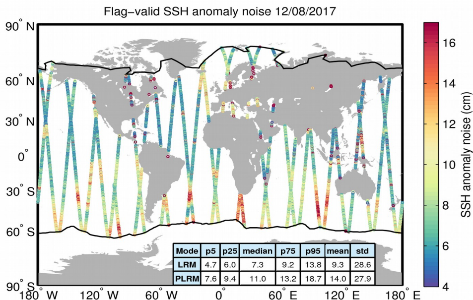
Figure 8. Geographical distribution of flag-valid 20-Hz SSH anomaly measurement noise over oceans and lakes for 12/08/2017. The statistical values shown in the table refer to the SSH anomaly noise and are calculated separately for LRM and PLRM regions. Measurements taken over polar polygons have been excluded from the computation of the statistical values. The black lines mark the outer limit of the Arctic and Antarctic polar polygons.
