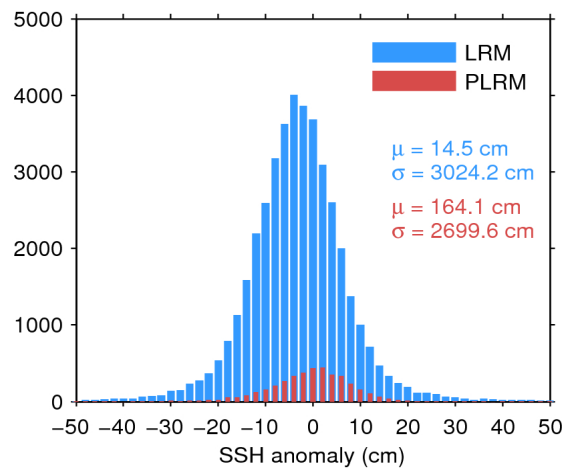
Figure 7. Histogram of flag-valid SSH anomaly over oceans and lakes for LRM (blue) and PLRM (red) for 12/08/2017. The mean ( \mu ) and standard deviation ( \sigma ) are also shown. Note that values outside [-50\ 50] cm are excluded from the histogram for the sake of readability but not from the computation of \mu and \sigma .
