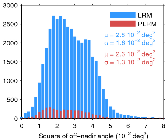
Figure 39. Histogram of flag-valid mispointing over oceans and lakes for LRM (blue) and PLRM (red) for 12/08/2017. Only positive values have been considered. The mean ( \mu ) and standard deviation ( \sigma ) are also shown. Note that values larger than 8 \cdot 10^{-2} \text{ deg}^2 are excluded from the histogram for the sake of readability but not from the computation of \mu and \sigma .
