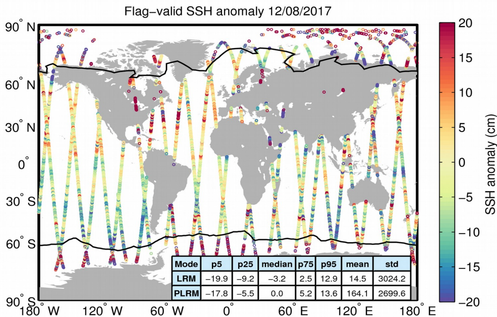
Figure 5. Geographical distribution of flag-valid 1-Hz SSH anomaly data over oceans and lakes for 12/08/2017. The statistical values shown in the table refer to the SSH anomaly in cm and are calculated separately for LRM and PLRM regions. Measurements taken over polar polygons have been excluded from the computation of the statistical values. The black lines mark the outer limit of the Arctic and Antarctic polar polygons.
