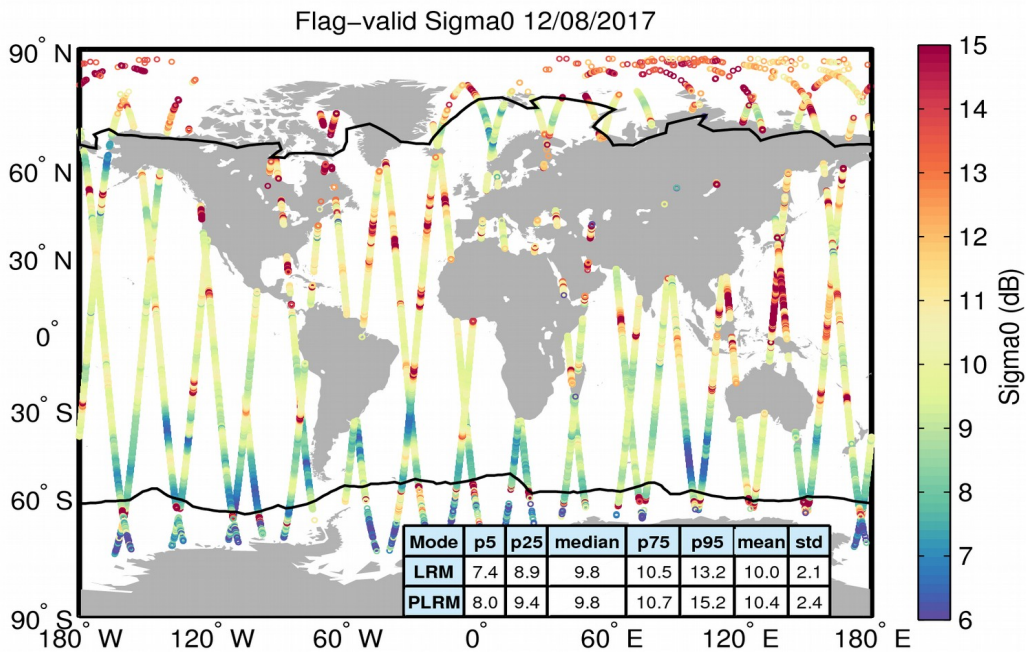
Figure 23. Geographical distribution of flag-valid sigma0 data over oceans and lakes for 12/08/2017. The statistical values shown in the table refer to the sigma0 in dB and are calculated separately for LRM and PLRM regions. Measurements taken over polar polygons have been excluded from the computation of the statistical values. The black lines mark the outer limit of the Arctic and Antarctic polar polygons.
