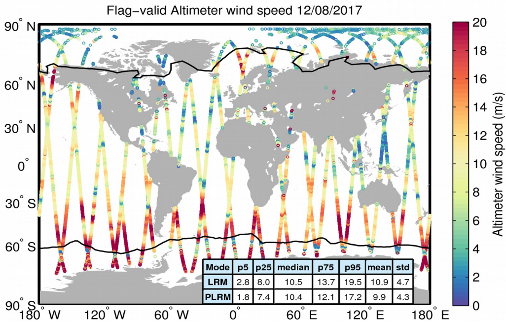
Figure 31. Geographical distribution of flag-valid wind data over oceans and lakes for 12/08/2017. The statistical values shown in the table refer to the wind in m/s and are calculated separately for LRM and PLRM regions. Measurements taken over polar polygons have been excluded from the computation of the statistical values. The black lines mark the outer limit of the Arctic and Antarctic polar polygons.
