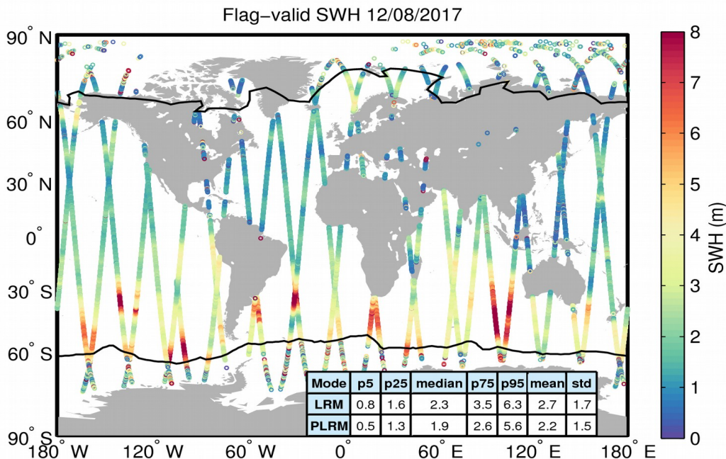
Figure 15. Geographical distribution of flag-valid SWH data over oceans and lakes for 12/08/2017. The statistical values shown in the table refer to the SWH in m and are calculated separately for LRM and PLRM regions. Measurements taken over polar polygons have been excluded from the computation of the statistical values. The black lines mark the outer limit of the Arctic and Antarctic polar polygons.
