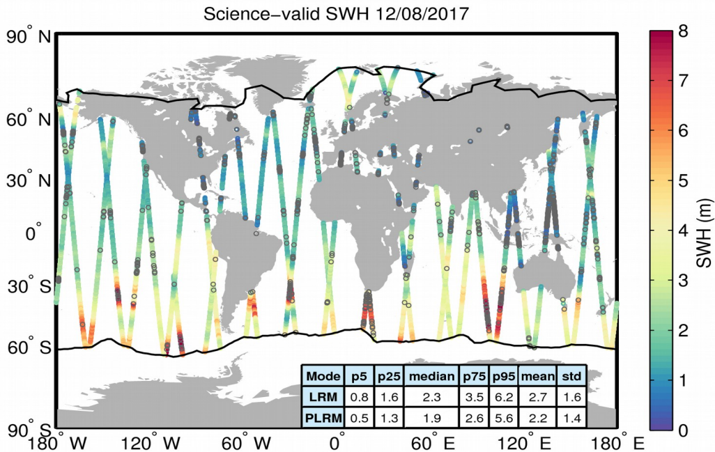
Figure 19. Geographical distribution of science-valid SWH data over oceans and lakes for 12/08/2017. The statistical values shown in the table refer to the SWH in m and are calculated separately for LRM and PLRM regions. The black lines mark the outer limit of the Arctic and Antarctic polar polygons. Gray circles denote records that have been rejected based on the editing criteria described in Table 3.
