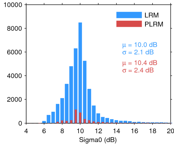
Figure 25. Histogram of flag-valid sigma0 over oceans and lakes for LRM (blue) and PLRM (red) for 12/08/2017. The mean ( \mu ) and standard deviation ( \sigma ) are also shown. Note that values outside [4 20] dB are excluded from the histogram for the sake of readability but not from the computation of \mu and \sigma .
