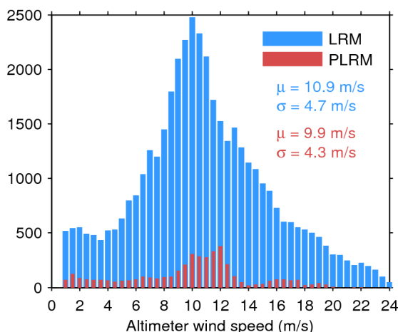
Figure 33. Histogram of flag-valid wind over oceans and lakes for LRM (blue) and PLRM (red) for 12/08/2017. The mean ( \mu ) and standard deviation ( \sigma ) are also shown. Note that values larger than 24 m/s are excluded from the histogram for the sake of readability but not from the computation of \mu and \sigma .
