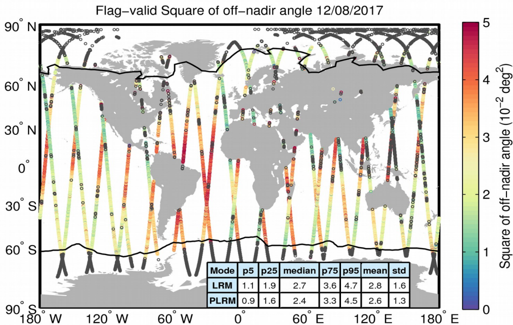
Figure 37. Geographical distribution of flag-valid mispointing data over oceans and lakes for 12/08/2017. The statistical values shown in the table refer to the mispointing in 10^{-2} \text{ deg}^2 and are calculated separately for LRM and PLRM regions. Measurements taken over polar polygons have been excluded from the computation of the statistical values. The black lines mark the outer limit of the Arctic and Antarctic polar polygons. Gray circles denote negative values.
