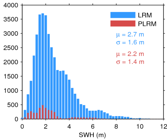
Figure 20. Histogram of science-valid SWH over oceans and lakes for LRM (blue) and PLRM (red) for 12/08/2017. The mean ( \mu ) and standard deviation ( \sigma ) are also shown. Note that values larger than 12 m are excluded from the histogram for the sake of readability but not from the computation of \mu and \sigma .
