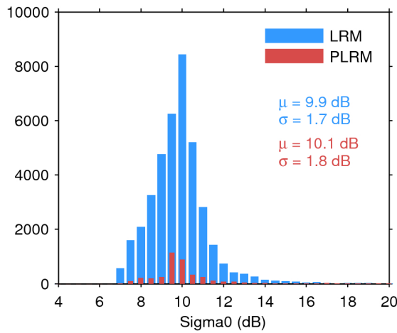
Figure 28. Histogram of science-valid sigma0 over oceans and lakes for LRM (blue) and PLRM (red) for 12/08/2017. The mean ( \mu ) and standard deviation ( \sigma ) are also shown. Note that values outside [4 20] dB are excluded from the histogram for the sake of readability but not from the computation of \mu and \sigma .
