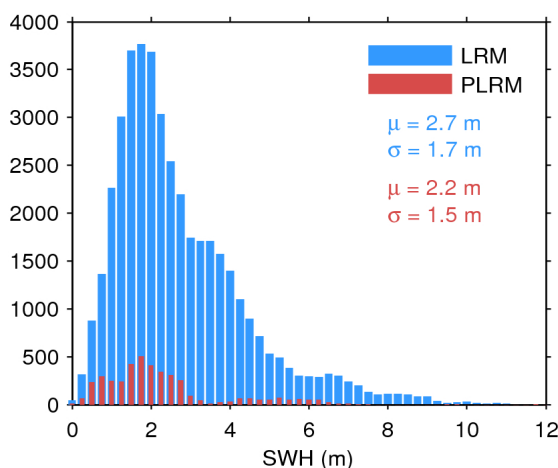
Figure 17. Histogram of flag-valid SWH over oceans and lakes for LRM (blue) and PLRM (red) for 12/08/2017. The mean ( \mu ) and standard deviation ( \sigma ) are also shown. Note that values larger than 12 m are excluded from the histogram for the sake of readability but not from the computation of \mu and \sigma .
