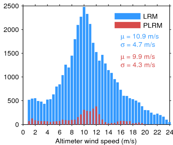
Figure 35. Histogram of science-valid wind over oceans and lakes for LRM (blue) and PLRM (red) for 12/08/2017. The mean ( \mu ) and standard deviation ( \sigma ) are also shown. Note that values larger than 24 m/s are excluded from the histogram for the sake of readability but not from the computation of \mu and \sigma .
