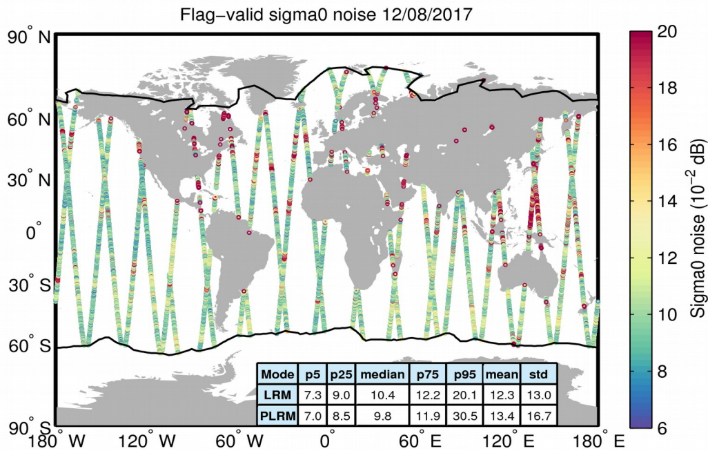
Figure 26. Geographical distribution of flag-valid 20-Hz sigma0 measurement noise over oceans and lakes for 12/08/2017. The statistical values shown in the table refer to the sigma0 noise and are calculated separately for LRM and PLRM regions. Measurements taken over polar polygons have been excluded from the computation of the statistical values. The black lines mark the outer limit of the Arctic and Antarctic polar polygons.
