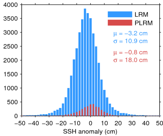
Figure 11. Histogram of science-valid SSH anomaly over oceans and lakes for LRM (blue) and PLRM (red) for 12/08/2017. The mean ( \mu ) and standard deviation ( \sigma ) are also shown. Note that values outside [-50 50] cm are excluded from the histogram for the sake of readability but not from the computation of \mu and \sigma .
