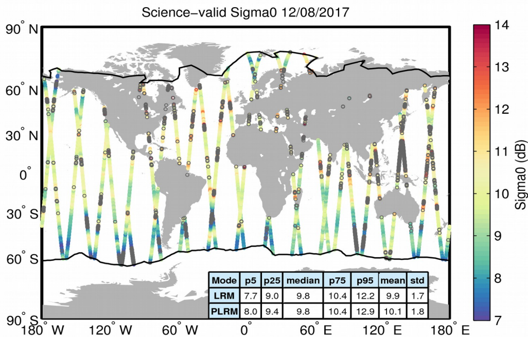
Figure 27. Geographical distribution of science-valid sigma0 data over oceans and lakes for 12/08/2017. The statistical values shown in the table refer to the sigma0 in dB and are calculated separately for LRM and PLRM regions. The black lines mark the outer limit of the Arctic and Antarctic polar polygons. Gray circles denote records that have been rejected based on the editing criteria described in Table 4.
