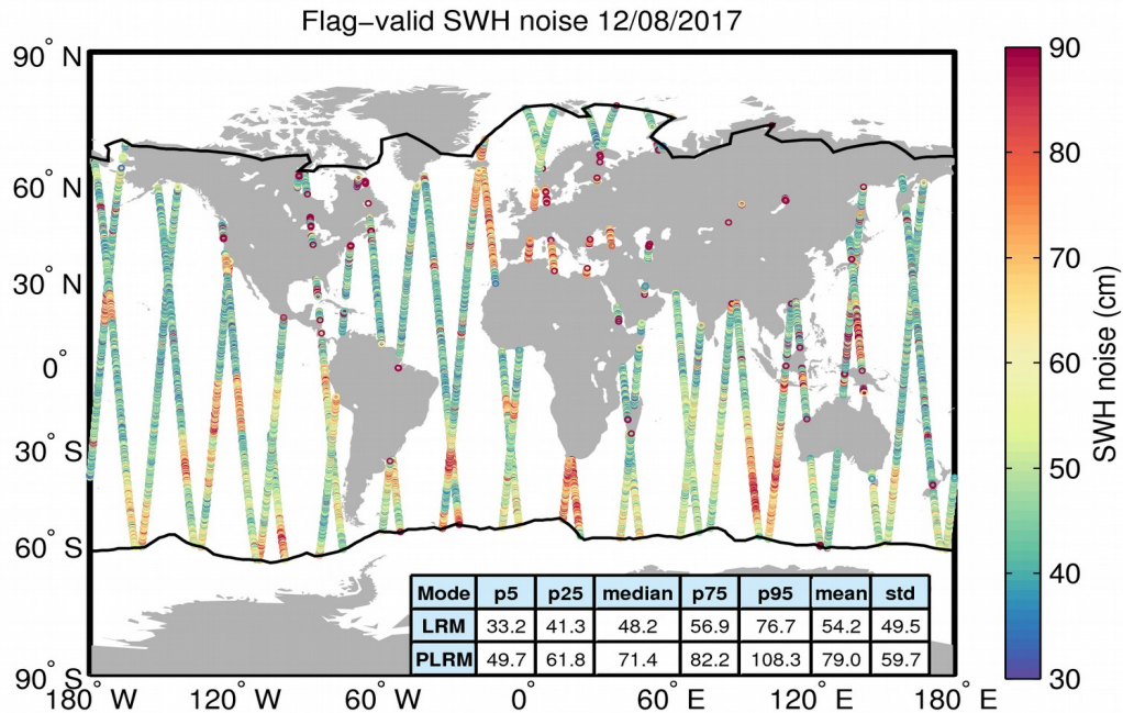
Figure 18. Geographical distribution of flag-valid 20-Hz SWH measurement noise over oceans and lakes for 12/08/2017. The statistical values shown in the table refer to the SWH noise and are calculated separately for LRM and PLRM regions. Measurements taken over polar polygons have been excluded from the computation of the statistical values. The black lines mark the outer limit of the Arctic and Antarctic polar polygons.
