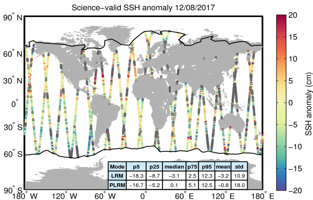
Figure 10. Geographical distribution of science-valid SSH anomaly data over oceans and lakes for 12/08/2017. The statistical values shown in the table refer to the SSH anomaly in cm and are calculated separately for LRM and PLRM regions. The black lines mark the outer limit of the Arctic and Antarctic polar polygons. Gray circles denote records that have been rejected based on the editing criteria described in Table 2.
