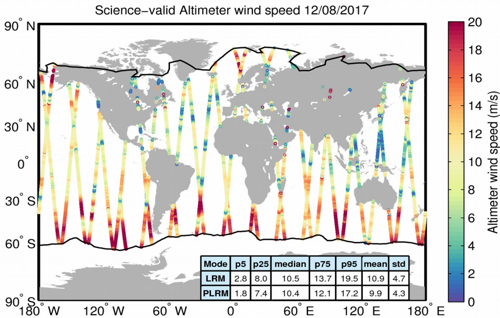
Figure 34. Geographical distribution of science-valid wind data over oceans and lakes for 12/08/2017. The statistical values shown in the table refer to the wind in m/s and are calculated separately for LRM and PLRM regions. The black lines mark the outer limit of the Arctic and Antarctic polar polygons. Gray circles denote records that have been rejected based on the editing criteria described in Table 5.
