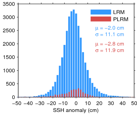
Figure 11. Histogram of science-valid SSH anomaly over oceans and lakes for LRM (blue) and PLRM (red) for 11/08/2017. The mean ( \mu ) and standard deviation ( \sigma ) are also shown. Note that values outside [-50\ 50] cm are excluded from the histogram for the sake of readability but not from the computation of \mu and \sigma .
