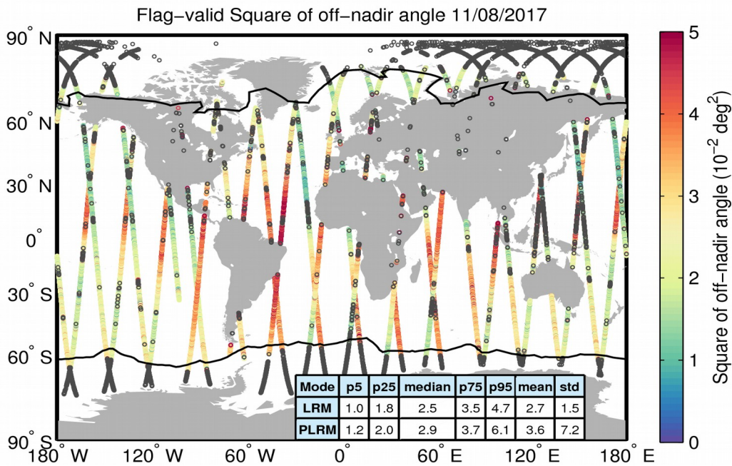
Figure 37. Geographical distribution of flag-valid mispointing data over oceans and lakes for 11/08/2017. The statistical values shown in the table refer to the mispointing in 10^{-2} deg 2 and are calculated separately for LRM and PLRM regions. Measurements taken over polar polygons have been excluded from the computation of the statistical values. The black lines mark the outer limit of the Arctic and Antarctic polar polygons. Gray circles denote negative values.
