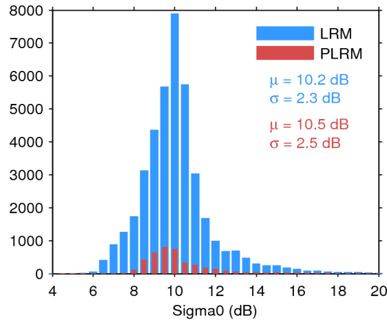
Figure 25. Histogram of flag-valid sigma0 over oceans and lakes for LRM (blue) and PLRM (red) for 11/08/2017. The mean ( \mu ) and standard deviation ( \sigma ) are also shown. Note that values outside [4 20] dB are excluded from the histogram for the sake of readability but not from the computation of \mu and \sigma .
