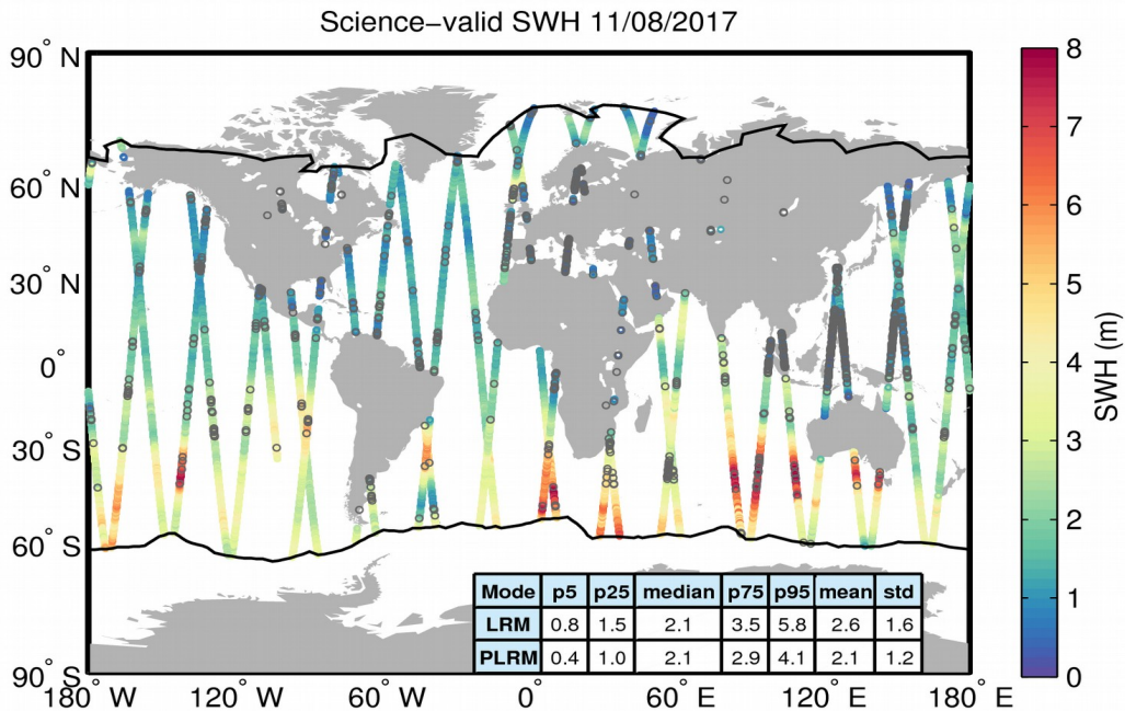
Figure 19. Geographical distribution of science-valid SWH data over oceans and lakes for 11/08/2017. The statistical values shown in the table refer to the SWH in m and are calculated separately for LRM and PLRM regions. The black lines mark the outer limit of the Arctic and Antarctic polar polygons. Gray circles denote records that have been rejected based on the editing criteria described in Table 3.
