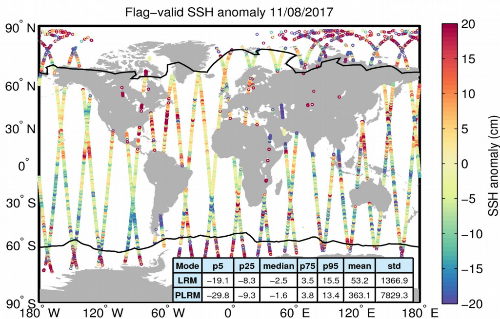
Figure 5. Geographical distribution of flag-valid 1-Hz SSH anomaly data over oceans and lakes for 11/08/2017. The statistical values shown in the table refer to the SSH anomaly in cm and are calculated separately for LRM and PLRM regions. Measurements taken over polar polygons have been excluded from the computation of the statistical values. The black lines mark the outer limit of the Arctic and Antarctic polar polygons.
