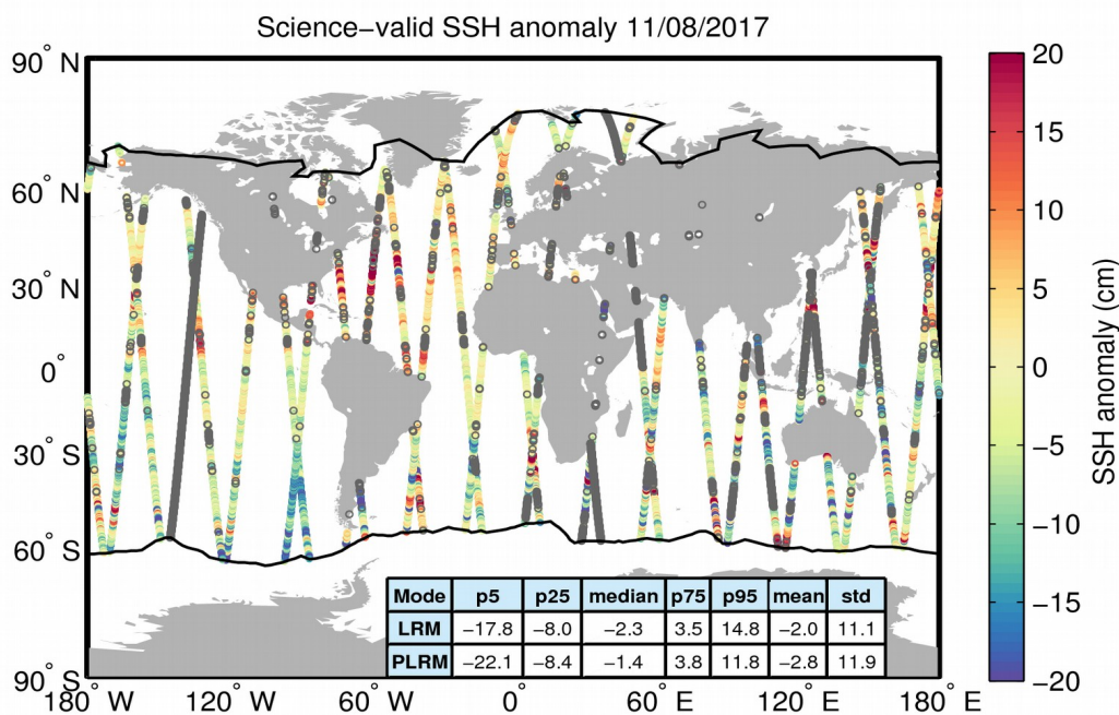
Figure 10. Geographical distribution of science-valid SSH anomaly data over oceans and lakes for 11/08/2017. The statistical values shown in the table refer to the SSH anomaly in cm and are calculated separately for LRM and PLRM regions. The black lines mark the outer limit of the Arctic and Antarctic polar polygons. Gray circles denote records that have been rejected based on the editing criteria described in Table 2.
