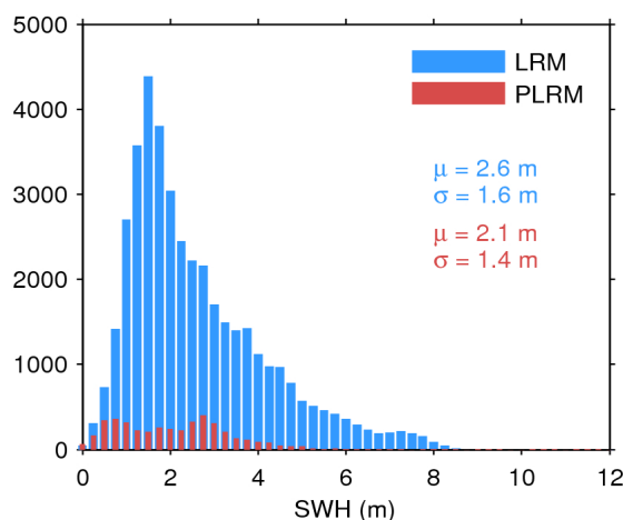
Figure 17. Histogram of flag-valid SWH over oceans and lakes for LRM (blue) and PLRM (red) for 11/08/2017. The mean ( \mu ) and standard deviation ( \sigma ) are also shown. Note that values larger than 12 m are excluded from the histogram for the sake of readability but not from the computation of \mu and \sigma .
