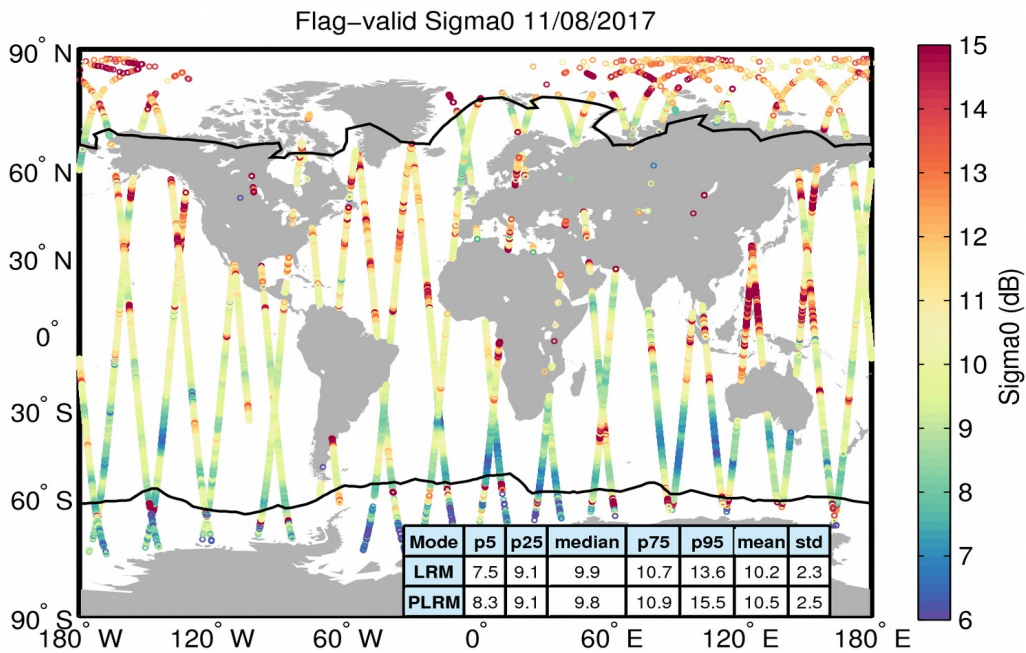
Figure 23. Geographical distribution of flag-valid sigma0 data over oceans and lakes for 11/08/2017. The statistical values shown in the table refer to the sigma0 in dB and are calculated separately for LRM and PLRM regions. Measurements taken over polar polygons have been excluded from the computation of the statistical values. The black lines mark the outer limit of the Arctic and Antarctic polar polygons.
