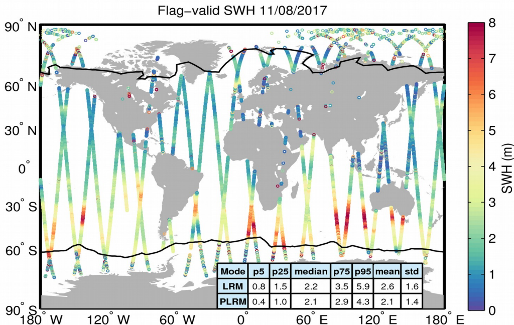
Figure 15. Geographical distribution of flag-valid SWH data over oceans and lakes for 11/08/2017. The statistical values shown in the table refer to the SWH in m and are calculated separately for LRM and PLRM regions. Measurements taken over polar polygons have been excluded from the computation of the statistical values. The black lines mark the outer limit of the Arctic and Antarctic polar polygons.
