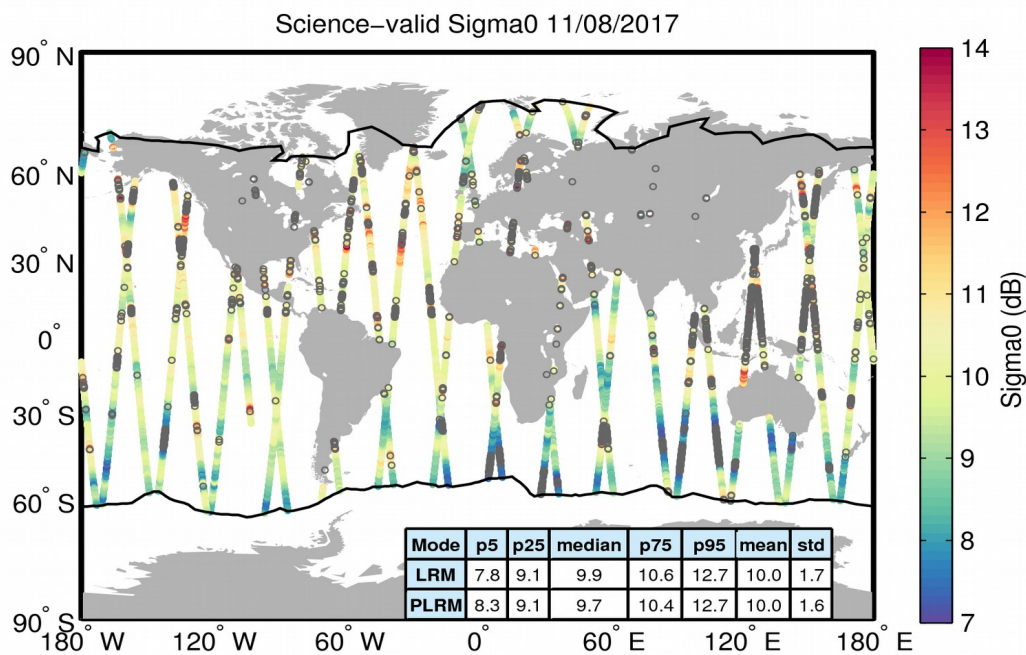
Figure 27. Geographical distribution of science-valid sigma0 data over oceans and lakes for 11/08/2017. The statistical values shown in the table refer to the sigma0 in dB and are calculated separately for LRM and PLRM regions. The black lines mark the outer limit of the Arctic and Antarctic polar polygons. Gray circles denote records that have been rejected based on the editing criteria described in Table 4.
