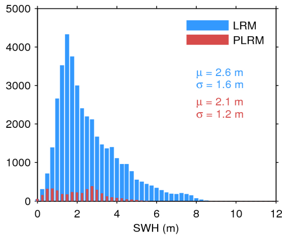
Figure 20. Histogram of science-valid SWH over oceans and lakes for LRM (blue) and PLRM (red) for 11/08/2017. The mean ( \mu ) and standard deviation ( \sigma ) are also shown. Note that values larger than 12 m are excluded from the histogram for the sake of readability but not from the computation of \mu and \sigma .
