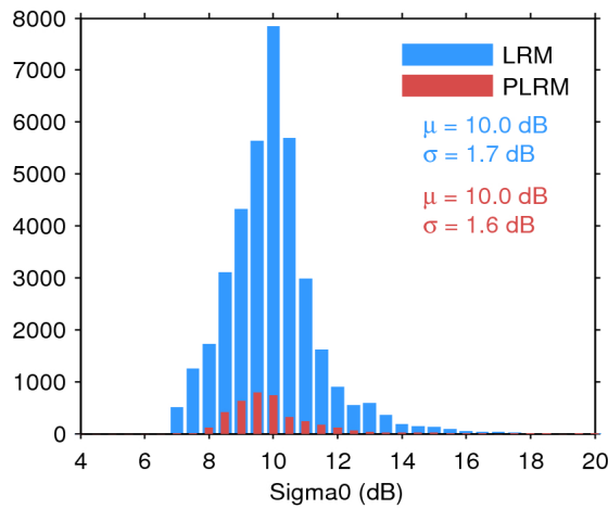
Figure 28. Histogram of science-valid sigma0 over oceans and lakes for LRM (blue) and PLRM (red) for 11/08/2017. The mean ( \mu ) and standard deviation ( \sigma ) are also shown. Note that values outside [4 20] dB are excluded from the histogram for the sake of readability but not from the computation of \mu and \sigma .
