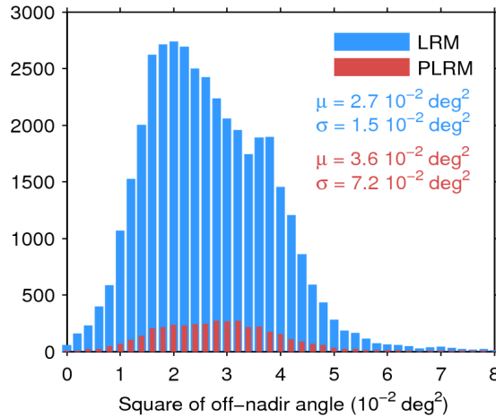
Figure 39. Histogram of flag-valid mispointing over oceans and lakes for LRM (blue) and PLRM (red) for 11/08/2017. Only positive values have been considered. The mean ( \mu ) and standard deviation ( \sigma ) are also shown. Note that values larger than 8 \cdot 10^{-2} \text{ deg}^2 are excluded from the histogram for the sake of readability but not from the computation of \mu and \sigma .
