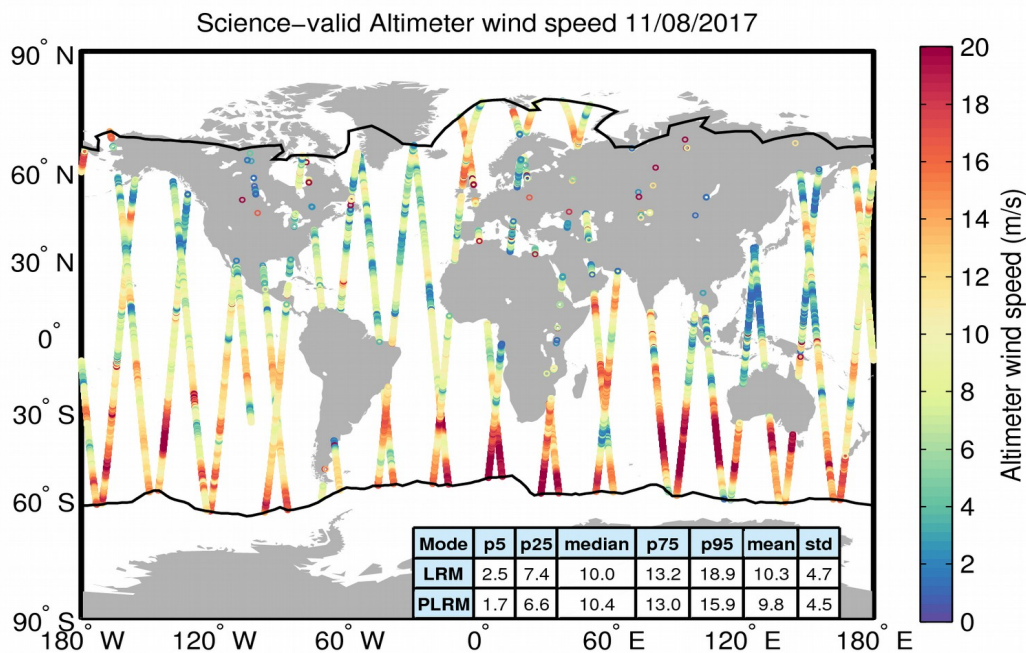
Figure 34. Geographical distribution of science-valid wind data over oceans and lakes for 11/08/2017. The statistical values shown in the table refer to the wind in m/s and are calculated separately for LRM and PLRM regions. The black lines mark the outer limit of the Arctic and Antarctic polar polygons. Gray circles denote records that have been rejected based on the editing criteria described in Table 5.
