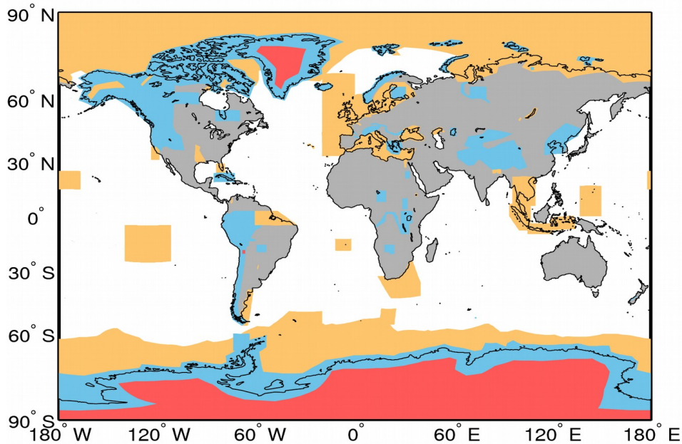
Figure A1. Extent of the regions defining the geographical mode mask for 11/08/2017. The regions where SAR, and SARIn are operated are denoted by the orange and blue polygons, respectively. LRM is operated over areas of the continental ice sheets (red polygons) and over oceans and land not covered by other modes.
