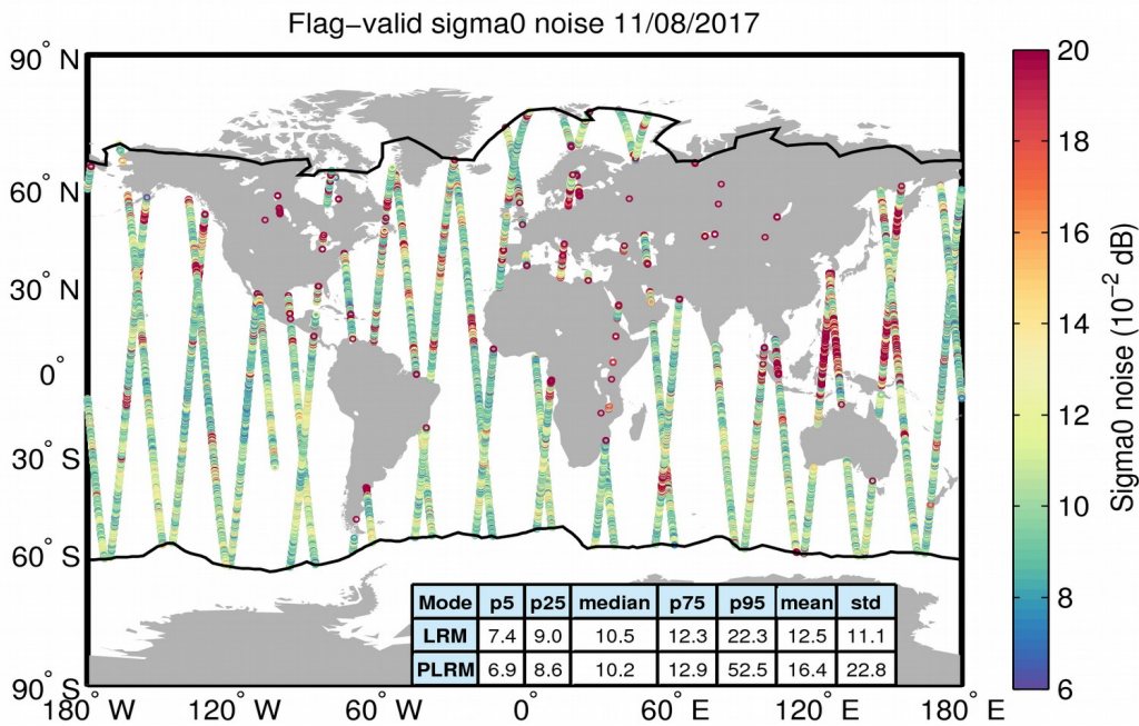
Figure 26. Geographical distribution of flag-valid 20-Hz sigma0 measurement noise over oceans and lakes for 11/08/2017. The statistical values shown in the table refer to the sigma0 noise and are calculated separately for LRM and PLRM regions. Measurements taken over polar polygons have been excluded from the computation of the statistical values. The black lines mark the outer limit of the Arctic and Antarctic polar polygons.
