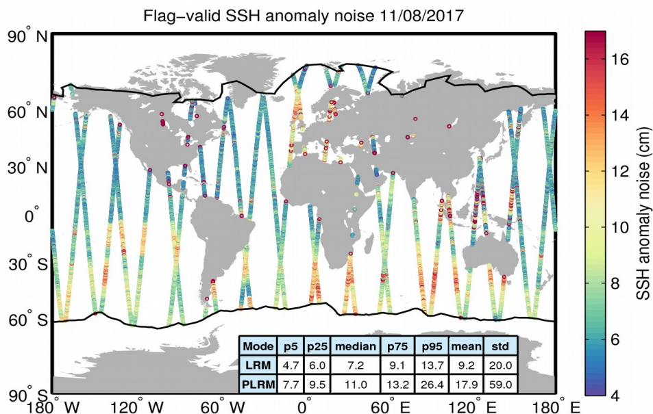
Figure 8. Geographical distribution of flag-valid 20-Hz SSH anomaly measurement noise over oceans and lakes for 11/08/2017. The statistical values shown in the table refer to the SSH anomaly noise and are calculated separately for LRM and PLRM regions. Measurements taken over polar polygons have been excluded from the computation of the statistical values. The black lines mark the outer limit of the Arctic and Antarctic polar polygons.
