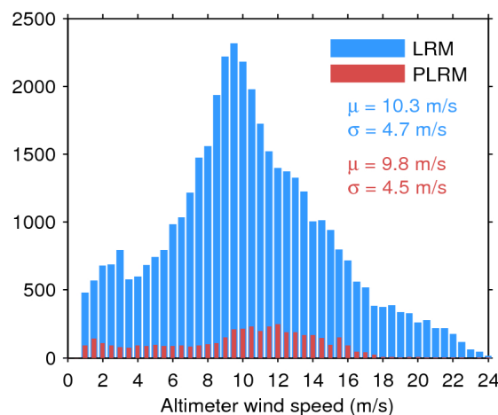
Figure 35. Histogram of science-valid wind over oceans and lakes for LRM (blue) and PLRM (red) for 11/08/2017. The mean ( \mu ) and standard deviation ( \sigma ) are also shown. Note that values larger than 24 m/s are excluded from the histogram for the sake of readability but not from the computation of \mu and \sigma .
