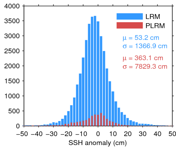
Figure 7. Histogram of flag-valid SSH anomaly over oceans and lakes for LRM (blue) and PLRM (red) for 11/08/2017. The mean ( \mu ) and standard deviation ( \sigma ) are also shown. Note that values outside [-50 50] cm are excluded from the histogram for the sake of readability but not from the computation of \mu and \sigma .
