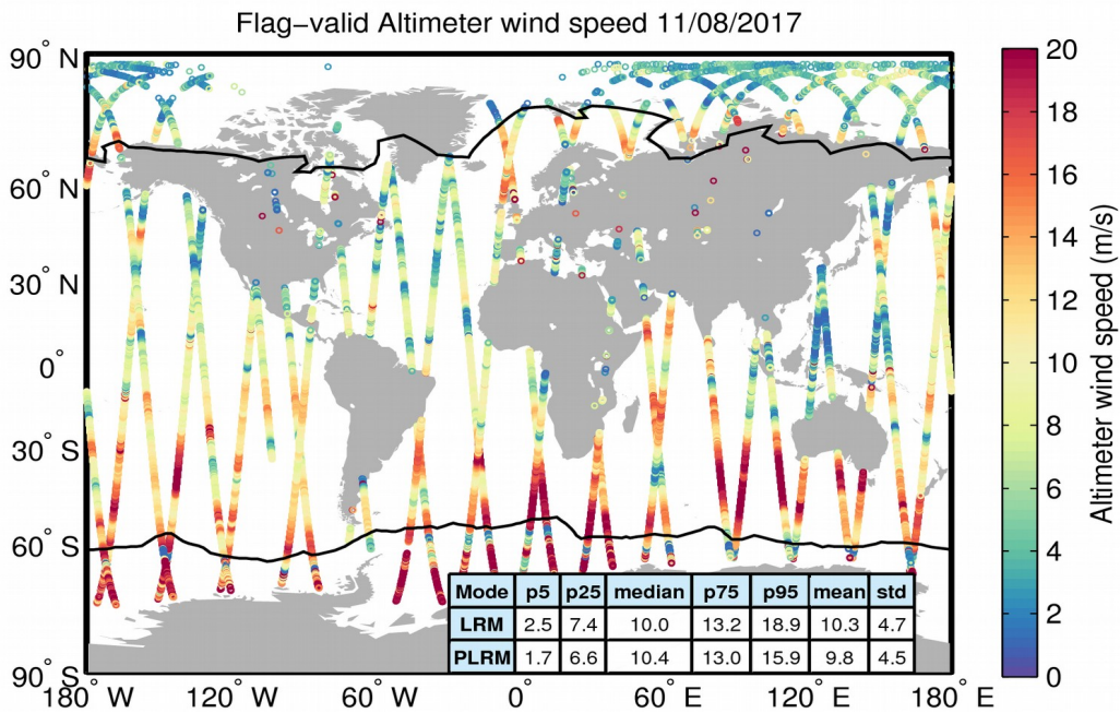
Figure 31. Geographical distribution of flag-valid wind data over oceans and lakes for 11/08/2017. The statistical values shown in the table refer to the wind in m/s and are calculated separately for LRM and PLRM regions. Measurements taken over polar polygons have been excluded from the computation of the statistical values. The black lines mark the outer limit of the Arctic and Antarctic polar polygons.
