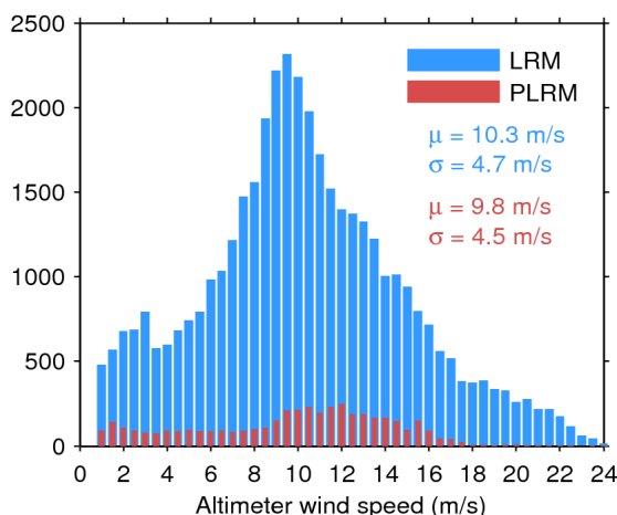
Figure 33. Histogram of flag-valid wind over oceans and lakes for LRM (blue) and PLRM (red) for 11/08/2017. The mean ( \mu ) and standard deviation ( \sigma ) are also shown. Note that values larger than 24 m/s are excluded from the histogram for the sake of readability but not from the computation of \mu and \sigma .
