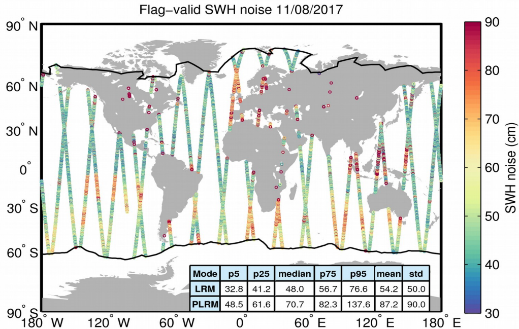
Figure 18. Geographical distribution of flag-valid 20-Hz SWH measurement noise over oceans and lakes for 11/08/2017. The statistical values shown in the table refer to the SWH noise and are calculated separately for LRM and PLRM regions. Measurements taken over polar polygons have been excluded from the computation of the statistical values. The black lines mark the outer limit of the Arctic and Antarctic polar polygons.
