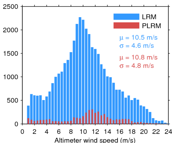
Figure 33. Histogram of flag-valid wind over oceans and lakes for LRM (blue) and PLRM (red) for 10/08/2017. The mean ( \mu ) and standard deviation ( \sigma ) are also shown. Note that values larger than 24 m/s are excluded from the histogram for the sake of readability but not from the computation of \mu and \sigma .
