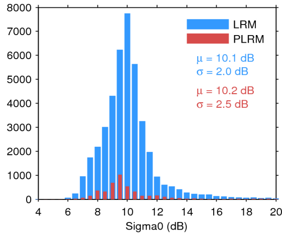
Figure 25. Histogram of flag-valid sigma0 over oceans and lakes for LRM (blue) and PLRM (red) for 10/08/2017. The mean ( \mu ) and standard deviation ( \sigma ) are also shown. Note that values outside [4 20] dB are excluded from the histogram for the sake of readability but not from the computation of \mu and \sigma .
