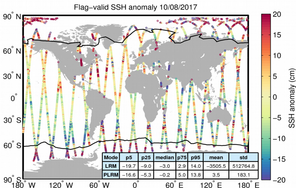
Figure 5. Geographical distribution of flag-valid 1-Hz SSH anomaly data over oceans and lakes for 10/08/2017. The statistical values shown in the table refer to the SSH anomaly in cm and are calculated separately for LRM and PLRM regions. Measurements taken over polar polygons have been excluded from the computation of the statistical values. The black lines mark the outer limit of the Arctic and Antarctic polar polygons.
