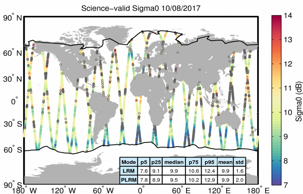
Figure 27. Geographical distribution of science-valid sigma0 data over oceans and lakes for 10/08/2017. The statistical values shown in the table refer to the sigma0 in dB and are calculated separately for LRM and PLRM regions. The black lines mark the outer limit of the Arctic and Antarctic polar polygons. Gray circles denote records that have been rejected based on the editing criteria described in Table 4.
