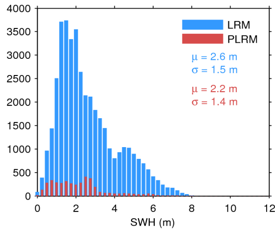
Figure 20. Histogram of science-valid SWH over oceans and lakes for LRM (blue) and PLRM (red) for 10/08/2017. The mean ( \mu ) and standard deviation ( \sigma ) are also shown. Note that values larger than 12 m are excluded from the histogram for the sake of readability but not from the computation of \mu and \sigma .
