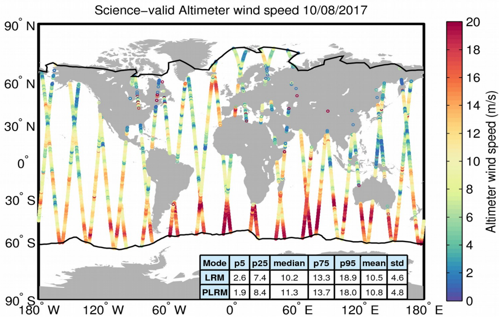
Figure 34. Geographical distribution of science-valid wind data over oceans and lakes for 10/08/2017. The statistical values shown in the table refer to the wind in m/s and are calculated separately for LRM and PLRM regions. The black lines mark the outer limit of the Arctic and Antarctic polar polygons. Gray circles denote records that have been rejected based on the editing criteria described in Table 5.
