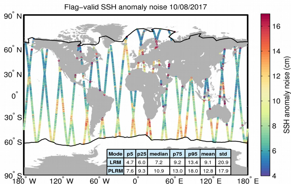
Figure 8. Geographical distribution of flag-valid 20-Hz SSH anomaly measurement noise over oceans and lakes for 10/08/2017. The statistical values shown in the table refer to the SSH anomaly noise and are calculated separately for LRM and PLRM regions. Measurements taken over polar polygons have been excluded from the computation of the statistical values. The black lines mark the outer limit of the Arctic and Antarctic polar polygons.
