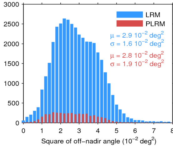
Figure 39. Histogram of flag-valid mispointing over oceans and lakes for LRM (blue) and PLRM (red) for 10/08/2017. Only positive values have been considered. The mean ( \mu ) and standard deviation ( \sigma ) are also shown. Note that values larger than 8 \cdot 10^{-2} \text{ deg}^2 are excluded from the histogram for the sake of readability but not from the computation of \mu and \sigma .
