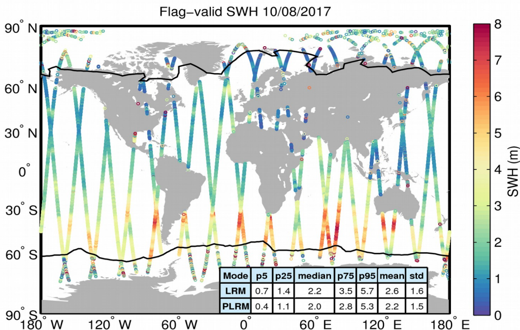
Figure 15. Geographical distribution of flag-valid SWH data over oceans and lakes for 10/08/2017. The statistical values shown in the table refer to the SWH in m and are calculated separately for LRM and PLRM regions. Measurements taken over polar polygons have been excluded from the computation of the statistical values. The black lines mark the outer limit of the Arctic and Antarctic polar polygons.
