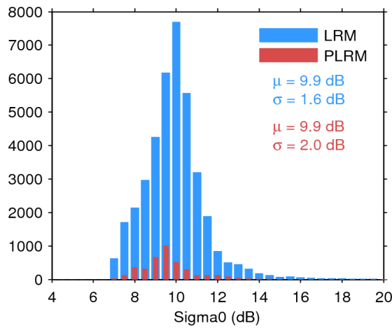
Figure 28. Histogram of science-valid sigma0 over oceans and lakes for LRM (blue) and PLRM (red) for 10/08/2017. The mean ( \mu ) and standard deviation ( \sigma ) are also shown. Note that values outside [4 20] dB are excluded from the histogram for the sake of readability but not from the computation of \mu and \sigma .
