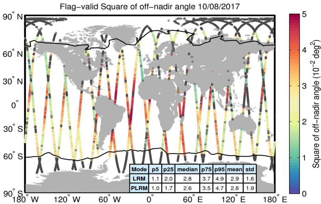
Figure 37. Geographical distribution of flag-valid mispointing data over oceans and lakes for 10/08/2017. The statistical values shown in the table refer to the mispointing in 10^{-2} deg 2 and are calculated separately for LRM and PLRM regions. Measurements taken over polar polygons have been excluded from the computation of the statistical values. The black lines mark the outer limit of the Arctic and Antarctic polar polygons. Gray circles denote negative values.
