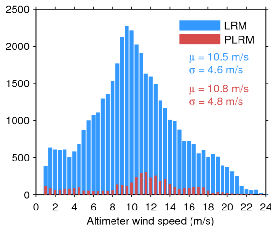
Figure 35. Histogram of science-valid wind over oceans and lakes for LRM (blue) and PLRM (red) for 10/08/2017. The mean ( \mu ) and standard deviation ( \sigma ) are also shown. Note that values larger than 24 m/s are excluded from the histogram for the sake of readability but not from the computation of \mu and \sigma .
