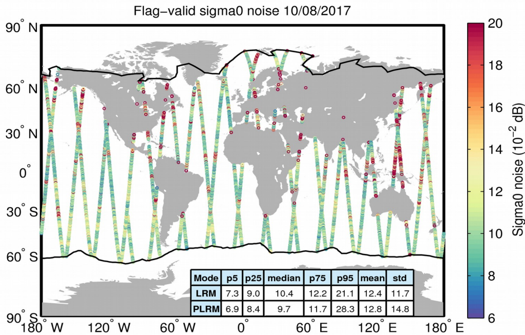
Figure 26. Geographical distribution of flag-valid 20-Hz sigma0 measurement noise over oceans and lakes for 10/08/2017. The statistical values shown in the table refer to the sigma0 noise and are calculated separately for LRM and PLRM regions. Measurements taken over polar polygons have been excluded from the computation of the statistical values. The black lines mark the outer limit of the Arctic and Antarctic polar polygons.
