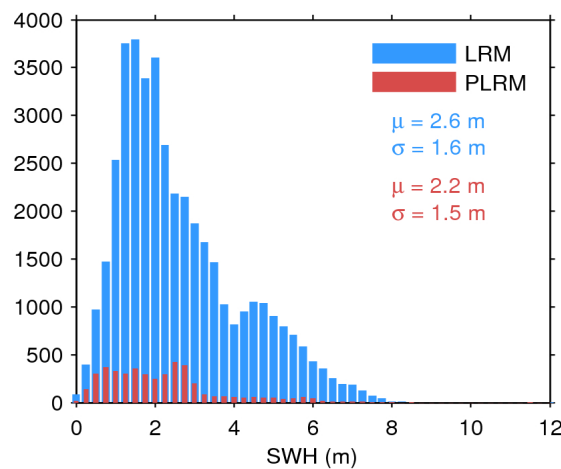
Figure 17. Histogram of flag-valid SWH over oceans and lakes for LRM (blue) and PLRM (red) for 10/08/2017. The mean ( \mu ) and standard deviation ( \sigma ) are also shown. Note that values larger than 12 m are excluded from the histogram for the sake of readability but not from the computation of \mu and \sigma .
