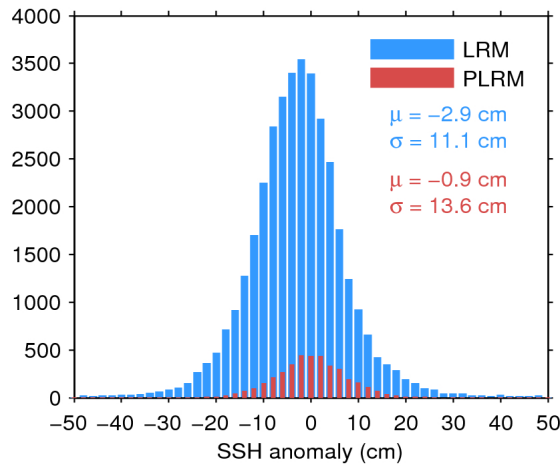
Figure 11. Histogram of science-valid SSH anomaly over oceans and lakes for LRM (blue) and PLRM (red) for 10/08/2017. The mean ( \mu ) and standard deviation ( \sigma ) are also shown. Note that values outside [-50 50] cm are excluded from the histogram for the sake of readability but not from the computation of \mu and \sigma .
