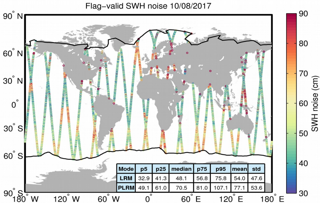
Figure 18. Geographical distribution of flag-valid 20-Hz SWH measurement noise over oceans and lakes for 10/08/2017. The statistical values shown in the table refer to the SWH noise and are calculated separately for LRM and PLRM regions. Measurements taken over polar polygons have been excluded from the computation of the statistical values. The black lines mark the outer limit of the Arctic and Antarctic polar polygons.
