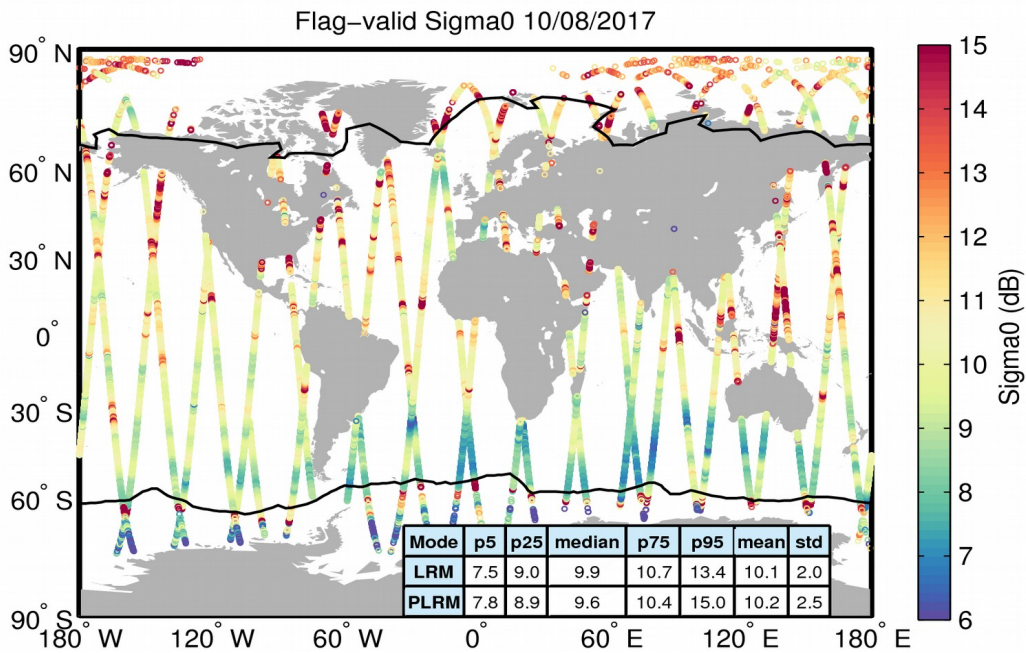
Figure 23. Geographical distribution of flag-valid sigma0 data over oceans and lakes for 10/08/2017. The statistical values shown in the table refer to the sigma0 in dB and are calculated separately for LRM and PLRM regions. Measurements taken over polar polygons have been excluded from the computation of the statistical values. The black lines mark the outer limit of the Arctic and Antarctic polar polygons.
