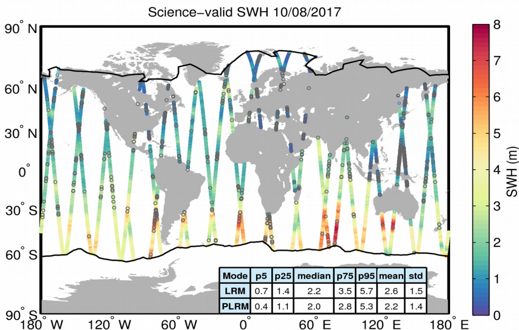
Figure 19. Geographical distribution of science-valid SWH data over oceans and lakes for 10/08/2017. The statistical values shown in the table refer to the SWH in m and are calculated separately for LRM and PLRM regions. The black lines mark the outer limit of the Arctic and Antarctic polar polygons. Gray circles denote records that have been rejected based on the editing criteria described in Table 3.
