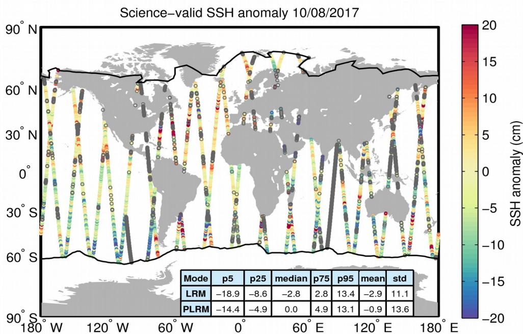
Figure 10. Geographical distribution of science-valid SSH anomaly data over oceans and lakes for 10/08/2017. The statistical values shown in the table refer to the SSH anomaly in cm and are calculated separately for LRM and PLRM regions. The black lines mark the outer limit of the Arctic and Antarctic polar polygons. Gray circles denote records that have been rejected based on the editing criteria described in Table 2.
