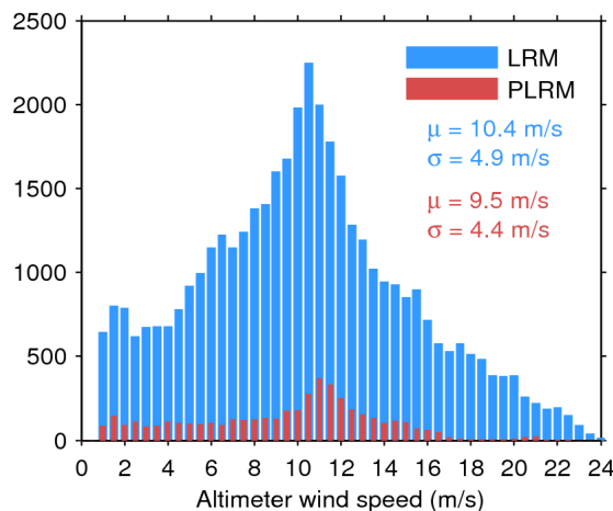
Figure 35. Histogram of science-valid wind over oceans and lakes for LRM (blue) and PLRM (red) for 09/08/2017. The mean ( \mu ) and standard deviation ( \sigma ) are also shown. Note that values larger than 24 m/s are excluded from the histogram for the sake of readability but not from the computation of \mu and \sigma .
