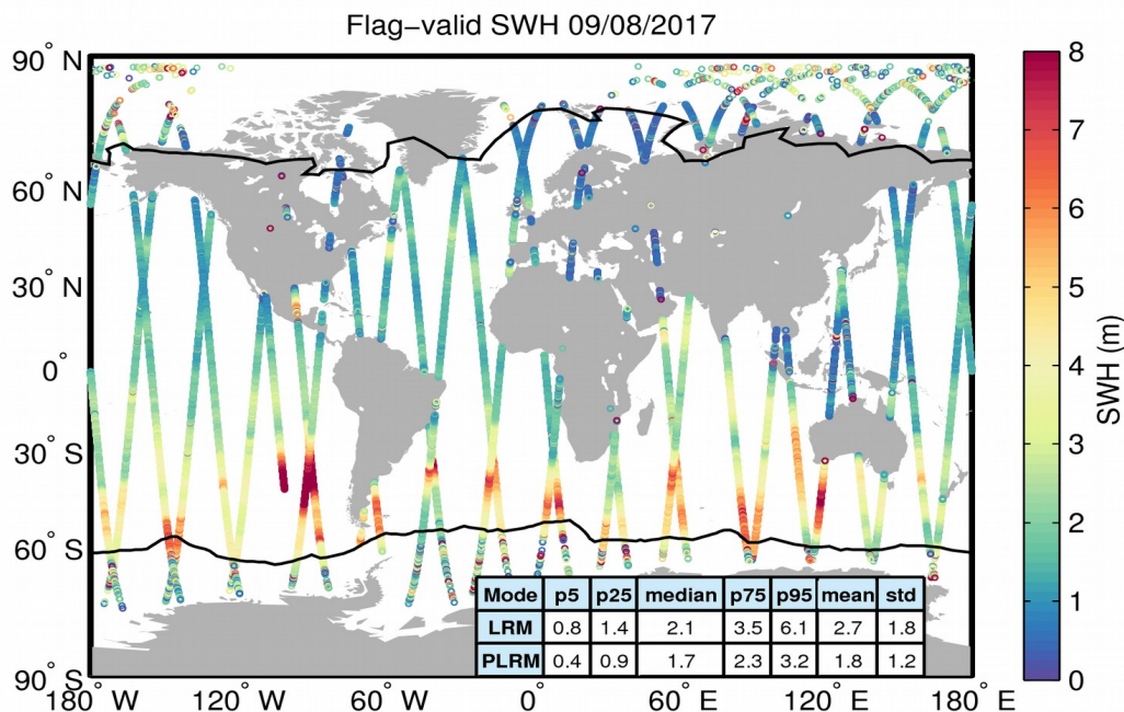
Figure 15. Geographical distribution of flag-valid SWH data over oceans and lakes for 09/08/2017. The statistical values shown in the table refer to the SWH in m and are calculated separately for LRM and PLRM regions. Measurements taken over polar polygons have been excluded from the computation of the statistical values. The black lines mark the outer limit of the Arctic and Antarctic polar polygons.
