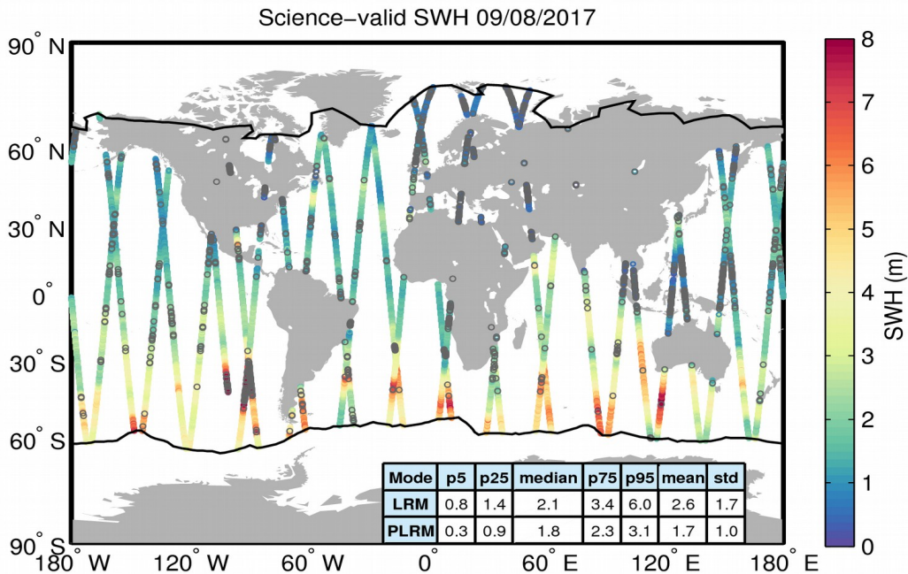
Figure 19. Geographical distribution of science-valid SWH data over oceans and lakes for 09/08/2017. The statistical values shown in the table refer to the SWH in m and are calculated separately for LRM and PLRM regions. The black lines mark the outer limit of the Arctic and Antarctic polar polygons. Gray circles denote records that have been rejected based on the editing criteria described in Table 3.
