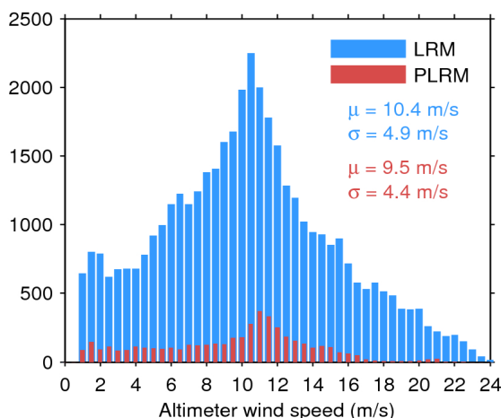
Figure 33. Histogram of flag-valid wind over oceans and lakes for LRM (blue) and PLRM (red) for 09/08/2017. The mean ( \mu ) and standard deviation ( \sigma ) are also shown. Note that values larger than 24 m/s are excluded from the histogram for the sake of readability but not from the computation of \mu and \sigma .
