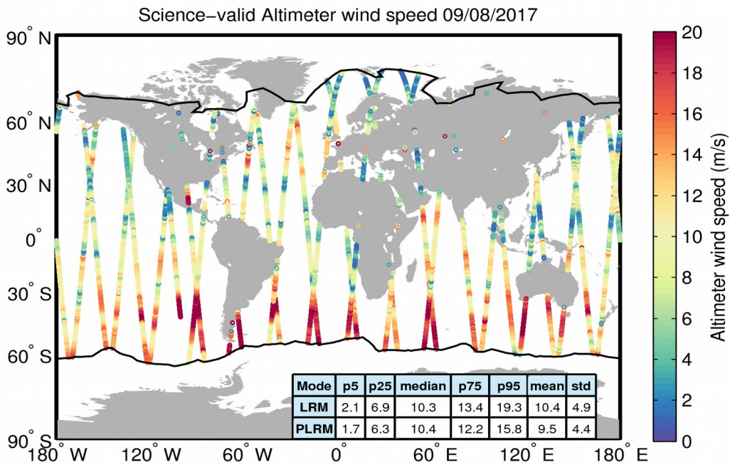
Figure 34. Geographical distribution of science-valid wind data over oceans and lakes for 09/08/2017. The statistical values shown in the table refer to the wind in m/s and are calculated separately for LRM and PLRM regions. The black lines mark the outer limit of the Arctic and Antarctic polar polygons. Gray circles denote records that have been rejected based on the editing criteria described in Table 5.
