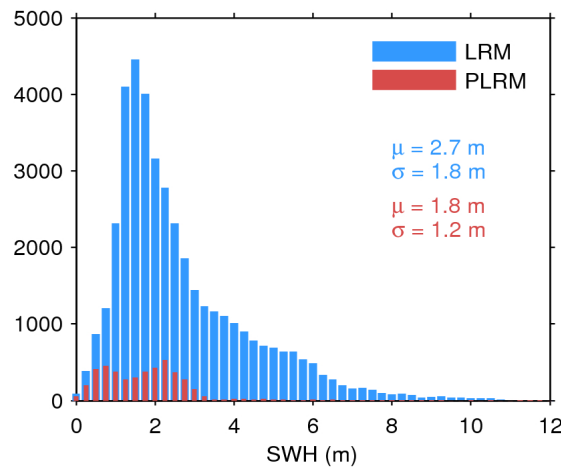
Figure 17. Histogram of flag-valid SWH over oceans and lakes for LRM (blue) and PLRM (red) for 09/08/2017. The mean ( \mu ) and standard deviation ( \sigma ) are also shown. Note that values larger than 12 m are excluded from the histogram for the sake of readability but not from the computation of \mu and \sigma .
