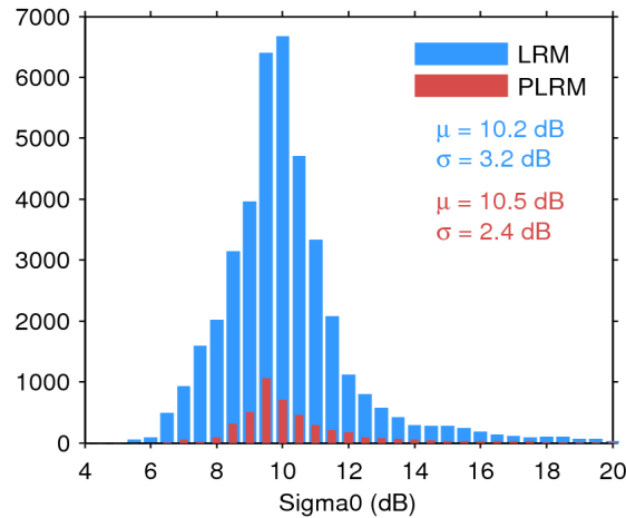
Figure 25. Histogram of flag-valid sigma0 over oceans and lakes for LRM (blue) and PLRM (red) for 09/08/2017. The mean ( \mu ) and standard deviation ( \sigma ) are also shown. Note that values outside [4 20] dB are excluded from the histogram for the sake of readability but not from the computation of \mu and \sigma .
