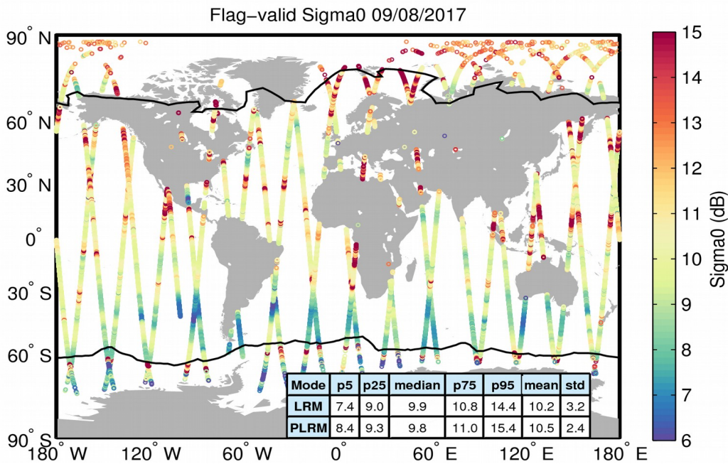
Figure 23. Geographical distribution of flag-valid sigma0 data over oceans and lakes for 09/08/2017. The statistical values shown in the table refer to the sigma0 in dB and are calculated separately for LRM and PLRM regions. Measurements taken over polar polygons have been excluded from the computation of the statistical values. The black lines mark the outer limit of the Arctic and Antarctic polar polygons.
