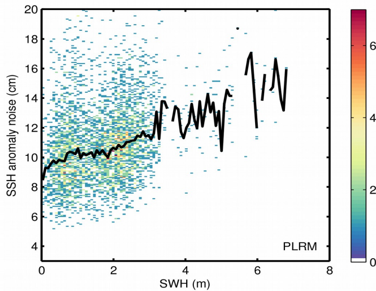
Figure 9. 2D histogram showing flag-valid SSH anomaly noise as a function of SWH for LRM (top) and PLRM (bottom) for 09/08/2017. The black line denotes the median SSH anomaly noise as a function of SWH.
