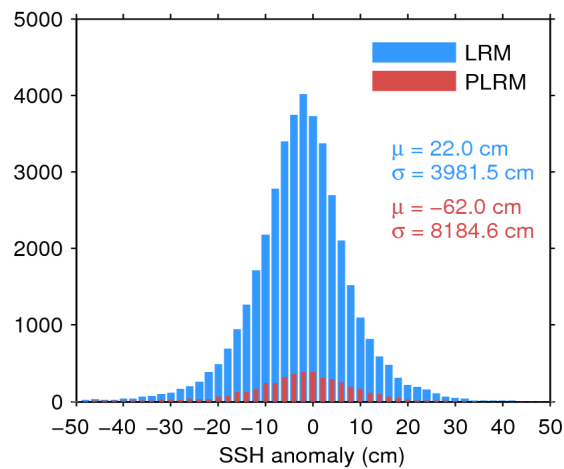
Figure 7. Histogram of flag-valid SSH anomaly over oceans and lakes for LRM (blue) and PLRM (red) for 09/08/2017. The mean ( \mu ) and standard deviation ( \sigma ) are also shown. Note that values outside [-50\ 50] cm are excluded from the histogram for the sake of readability but not from the computation of \mu and \sigma .
