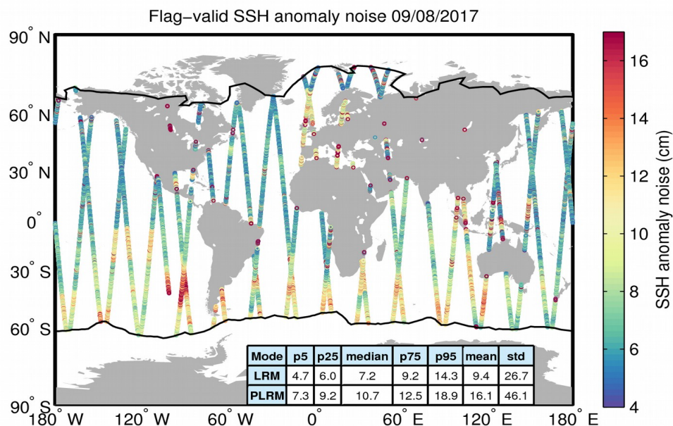
Figure 8. Geographical distribution of flag-valid 20-Hz SSH anomaly measurement noise over oceans and lakes for 09/08/2017. The statistical values shown in the table refer to the SSH anomaly noise and are calculated separately for LRM and PLRM regions. Measurements taken over polar polygons have been excluded from the computation of the statistical values. The black lines mark the outer limit of the Arctic and Antarctic polar polygons.
