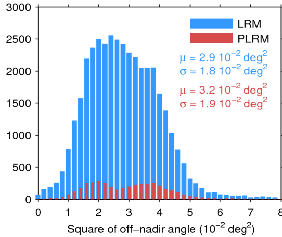
Figure 39. Histogram of flag-valid mispointing over oceans and lakes for LRM (blue) and PLRM (red) for 09/08/2017. Only positive values have been considered. The mean ( \mu ) and standard deviation ( \sigma ) are also shown. Note that values larger than 8 \cdot 10^{-2} \text{ deg}^2 are excluded from the histogram for the sake of readability but not from the computation of \mu and \sigma .
