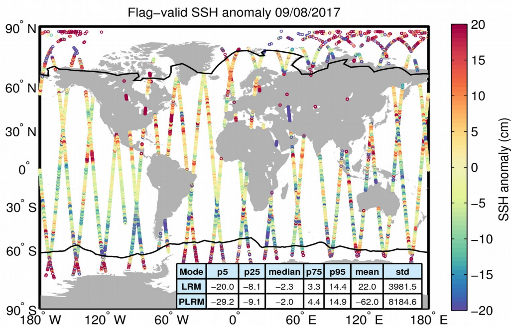
Figure 5. Geographical distribution of flag-valid 1-Hz SSH anomaly data over oceans and lakes for 09/08/2017. The statistical values shown in the table refer to the SSH anomaly in cm and are calculated separately for LRM and PLRM regions. Measurements taken over polar polygons have been excluded from the computation of the statistical values. The black lines mark the outer limit of the Arctic and Antarctic polar polygons.
