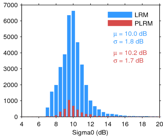
Figure 28. Histogram of science-valid sigma0 over oceans and lakes for LRM (blue) and PLRM (red) for 09/08/2017. The mean ( \mu ) and standard deviation ( \sigma ) are also shown. Note that values outside [4 20] dB are excluded from the histogram for the sake of readability but not from the computation of \mu and \sigma .
