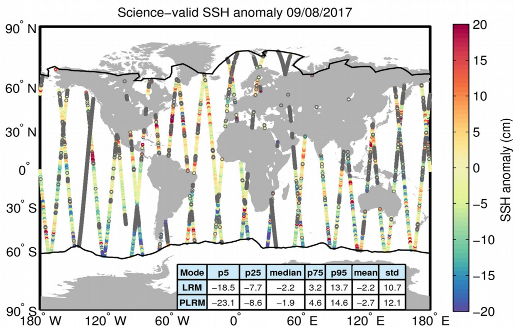
Figure 10. Geographical distribution of science-valid SSH anomaly data over oceans and lakes for 09/08/2017. The statistical values shown in the table refer to the SSH anomaly in cm and are calculated separately for LRM and PLRM regions. The black lines mark the outer limit of the Arctic and Antarctic polar polygons. Gray circles denote records that have been rejected based on the editing criteria described in Table 2.
