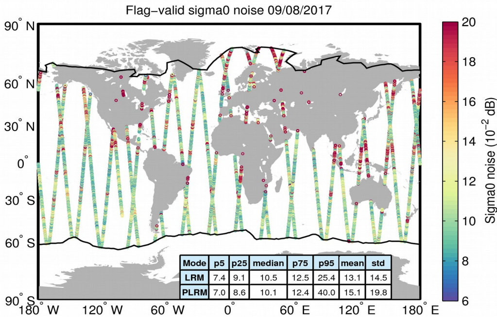
Figure 26. Geographical distribution of flag-valid 20-Hz sigma0 measurement noise over oceans and lakes for 09/08/2017. The statistical values shown in the table refer to the sigma0 noise and are calculated separately for LRM and PLRM regions. Measurements taken over polar polygons have been excluded from the computation of the statistical values. The black lines mark the outer limit of the Arctic and Antarctic polar polygons.
