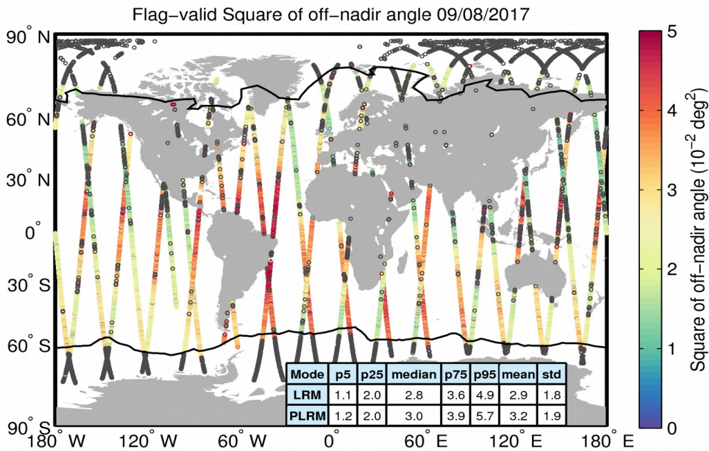
Figure 37. Geographical distribution of flag-valid mispointing data over oceans and lakes for 09/08/2017. The statistical values shown in the table refer to the mispointing in 10^{-2} deg 2 and are calculated separately for LRM and PLRM regions. Measurements taken over polar polygons have been excluded from the computation of the statistical values. The black lines mark the outer limit of the Arctic and Antarctic polar polygons. Gray circles denote negative values.
