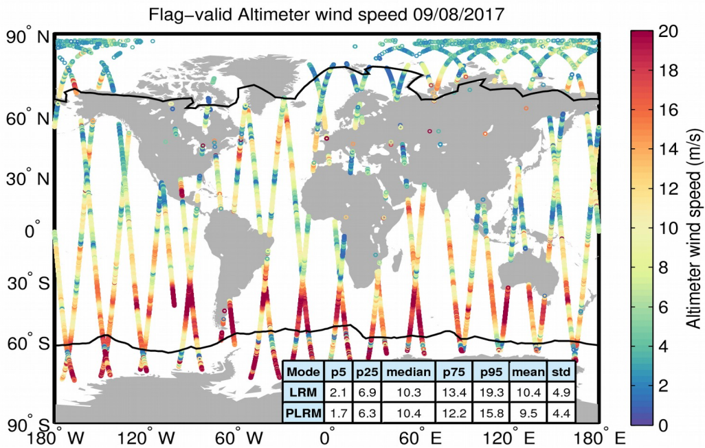
Figure 31. Geographical distribution of flag-valid wind data over oceans and lakes for 09/08/2017. The statistical values shown in the table refer to the wind in m/s and are calculated separately for LRM and PLRM regions. Measurements taken over polar polygons have been excluded from the computation of the statistical values. The black lines mark the outer limit of the Arctic and Antarctic polar polygons.
