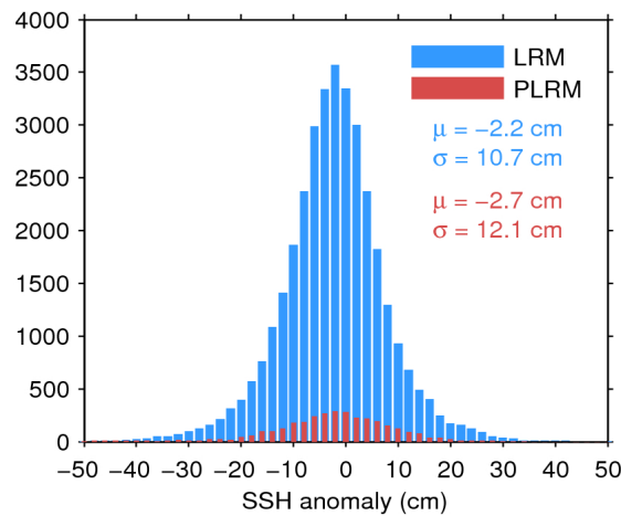
Figure 11. Histogram of science-valid SSH anomaly over oceans and lakes for LRM (blue) and PLRM (red) for 09/08/2017. The mean ( \mu ) and standard deviation ( \sigma ) are also shown. Note that values outside [-50\ 50] cm are excluded from the histogram for the sake of readability but not from the computation of \mu and \sigma .
