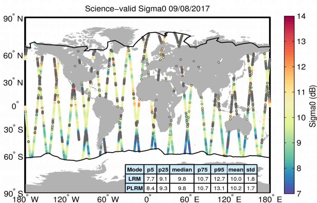
Figure 27. Geographical distribution of science-valid sigma0 data over oceans and lakes for 09/08/2017. The statistical values shown in the table refer to the sigma0 in dB and are calculated separately for LRM and PLRM regions. The black lines mark the outer limit of the Arctic and Antarctic polar polygons. Gray circles denote records that have been rejected based on the editing criteria described in Table 4.
