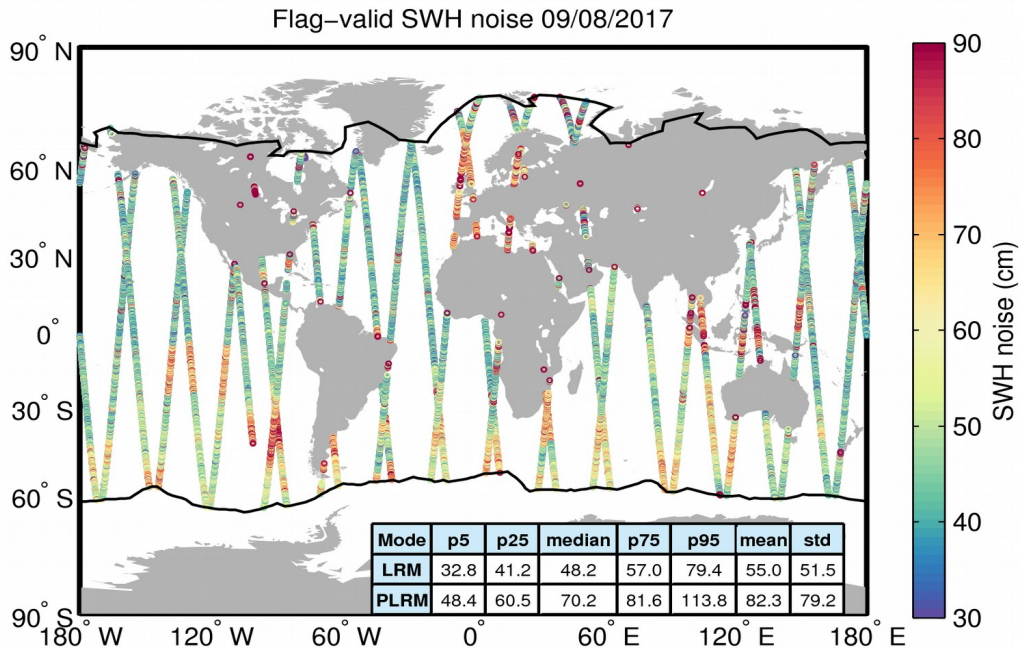
Figure 18. Geographical distribution of flag-valid 20-Hz SWH measurement noise over oceans and lakes for 09/08/2017. The statistical values shown in the table refer to the SWH noise and are calculated separately for LRM and PLRM regions. Measurements taken over polar polygons have been excluded from the computation of the statistical values. The black lines mark the outer limit of the Arctic and Antarctic polar polygons.
