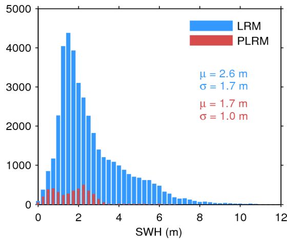
Figure 20. Histogram of science-valid SWH over oceans and lakes for LRM (blue) and PLRM (red) for 09/08/2017. The mean ( \mu ) and standard deviation ( \sigma ) are also shown. Note that values larger than 12 m are excluded from the histogram for the sake of readability but not from the computation of \mu and \sigma .
