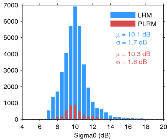
Figure 28. Histogram of science-valid sigma0 over oceans and lakes for LRM (blue) and PLRM (red) for 07/08/2017. The mean ( \mu ) and standard deviation ( \sigma ) are also shown. Note that values outside [4 20] dB are excluded from the histogram for the sake of readability but not from the computation of \mu and \sigma .
