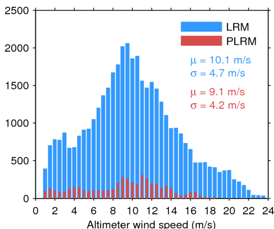
Figure 33. Histogram of flag-valid wind over oceans and lakes for LRM (blue) and PLRM (red) for 07/08/2017. The mean ( \mu ) and standard deviation ( \sigma ) are also shown. Note that values larger than 24 m/s are excluded from the histogram for the sake of readability but not from the computation of \mu and \sigma .
