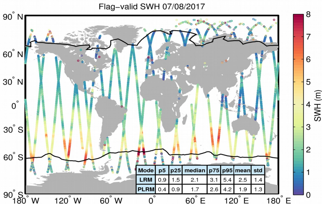
Figure 15. Geographical distribution of flag-valid SWH data over oceans and lakes for 07/08/2017. The statistical values shown in the table refer to the SWH in m and are calculated separately for LRM and PLRM regions. Measurements taken over polar polygons have been excluded from the computation of the statistical values. The black lines mark the outer limit of the Arctic and Antarctic polar polygons.
