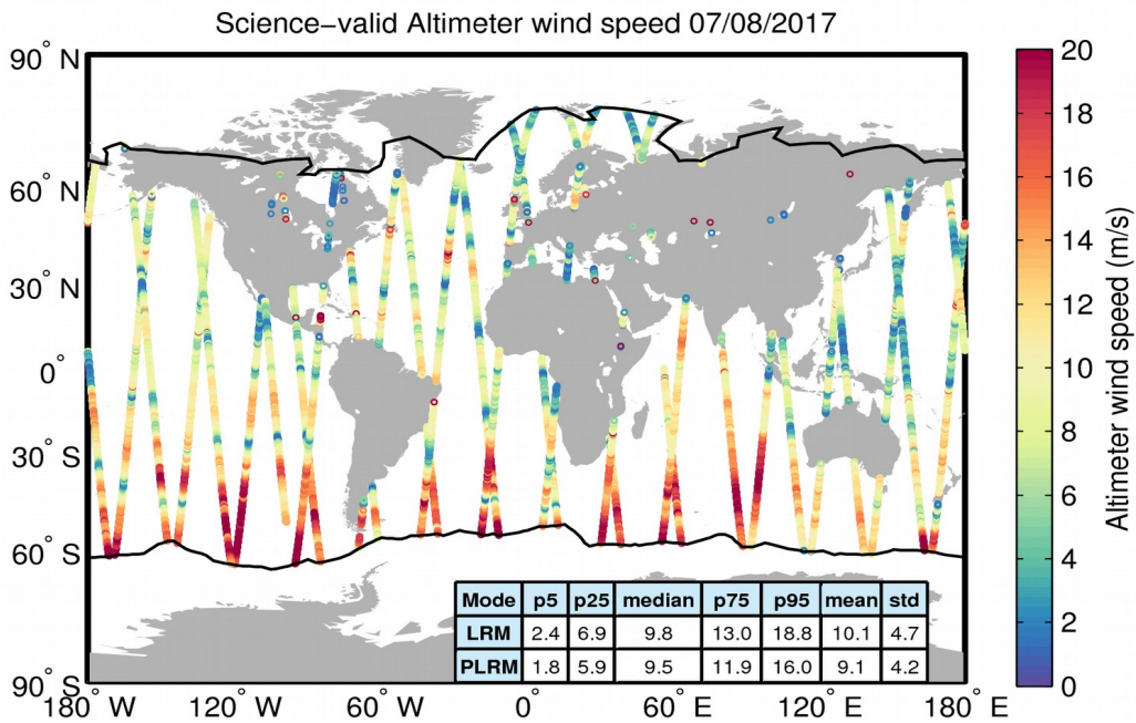
Figure 34. Geographical distribution of science-valid wind data over oceans and lakes for 07/08/2017. The statistical values shown in the table refer to the wind in m/s and are calculated separately for LRM and PLRM regions. The black lines mark the outer limit of the Arctic and Antarctic polar polygons. Gray circles denote records that have been rejected based on the editing criteria described in Table 5.
