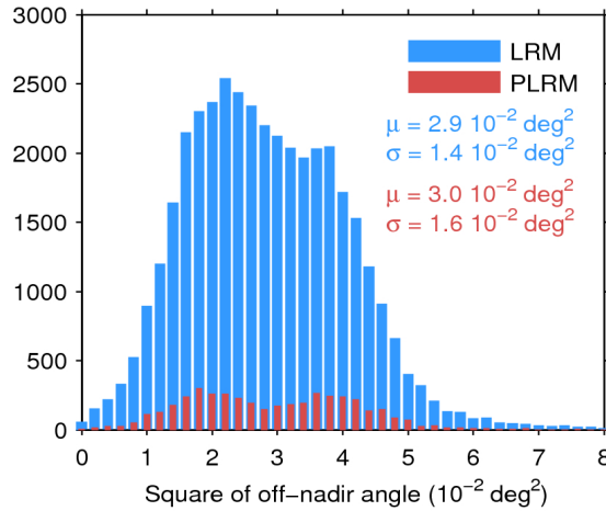
Figure 39. Histogram of flag-valid mispointing over oceans and lakes for LRM (blue) and PLRM (red) for 07/08/2017. Only positive values have been considered. The mean ( \mu ) and standard deviation ( \sigma ) are also shown. Note that values larger than 8 \cdot 10^{-2} \text{ deg}^2 are excluded from the histogram for the sake of readability but not from the computation of \mu and \sigma .
