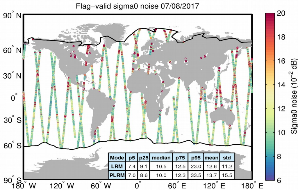
Figure 26. Geographical distribution of flag-valid 20-Hz sigma0 measurement noise over oceans and lakes for 07/08/2017. The statistical values shown in the table refer to the sigma0 noise and are calculated separately for LRM and PLRM regions. Measurements taken over polar polygons have been excluded from the computation of the statistical values. The black lines mark the outer limit of the Arctic and Antarctic polar polygons.
