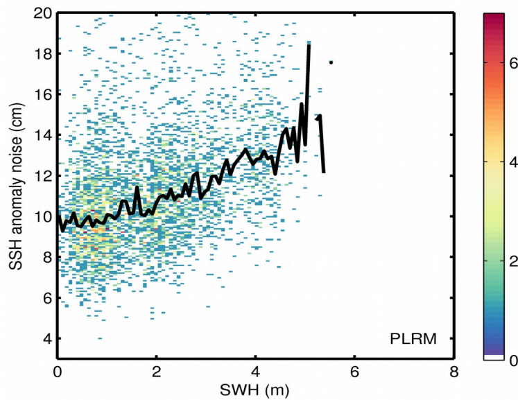
Figure 9. 2D histogram showing flag-valid SSH anomaly noise as a function of SWH for LRM (top) and PLRM (bottom) for 07/08/2017. The black line denotes the median SSH anomaly noise as a function of SWH.
