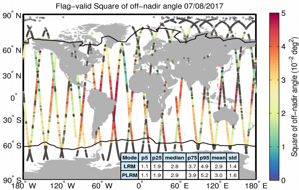
Figure 37. Geographical distribution of flag-valid mispointing data over oceans and lakes for 07/08/2017. The statistical values shown in the table refer to the mispointing in 10^{-2} deg 2 and are calculated separately for LRM and PLRM regions. Measurements taken over polar polygons have been excluded from the computation of the statistical values. The black lines mark the outer limit of the Arctic and Antarctic polar polygons. Gray circles denote negative values.
