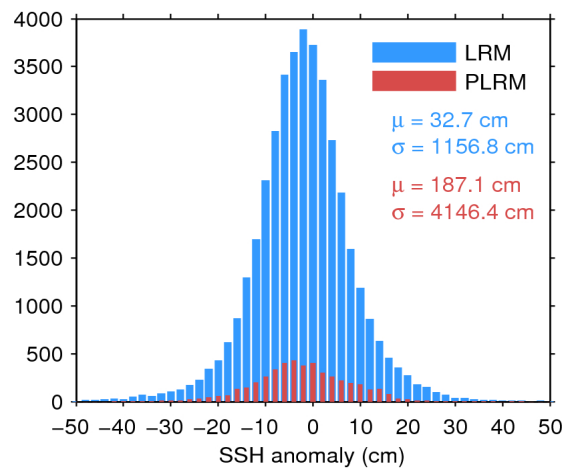
Figure 7. Histogram of flag-valid SSH anomaly over oceans and lakes for LRM (blue) and PLRM (red) for 07/08/2017. The mean ( \mu ) and standard deviation ( \sigma ) are also shown. Note that values outside [-50 \ 50] cm are excluded from the histogram for the sake of readability but not from the computation of \mu and \sigma .
