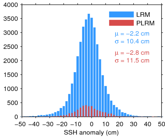
Figure 11. Histogram of science-valid SSH anomaly over oceans and lakes for LRM (blue) and PLRM (red) for 07/08/2017. The mean ( \mu ) and standard deviation ( \sigma ) are also shown. Note that values outside [-50\ 50] cm are excluded from the histogram for the sake of readability but not from the computation of \mu and \sigma .
