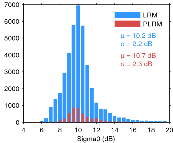
Figure 25. Histogram of flag-valid sigma0 over oceans and lakes for LRM (blue) and PLRM (red) for 07/08/2017. The mean ( \mu ) and standard deviation ( \sigma ) are also shown. Note that values outside [4 20] dB are excluded from the histogram for the sake of readability but not from the computation of \mu and \sigma .
