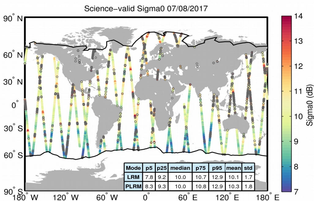
Figure 27. Geographical distribution of science-valid sigma0 data over oceans and lakes for 07/08/2017. The statistical values shown in the table refer to the sigma0 in dB and are calculated separately for LRM and PLRM regions. The black lines mark the outer limit of the Arctic and Antarctic polar polygons. Gray circles denote records that have been rejected based on the editing criteria described in Table 4.
