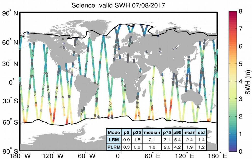
Figure 19. Geographical distribution of science-valid SWH data over oceans and lakes for 07/08/2017. The statistical values shown in the table refer to the SWH in m and are calculated separately for LRM and PLRM regions. The black lines mark the outer limit of the Arctic and Antarctic polar polygons. Gray circles denote records that have been rejected based on the editing criteria described in Table 3.
