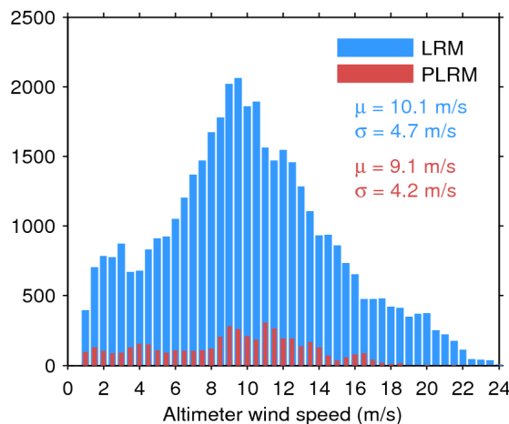
Figure 35. Histogram of science-valid wind over oceans and lakes for LRM (blue) and PLRM (red) for 07/08/2017. The mean ( \mu ) and standard deviation ( \sigma ) are also shown. Note that values larger than 24 m/s are excluded from the histogram for the sake of readability but not from the computation of \mu and \sigma .
