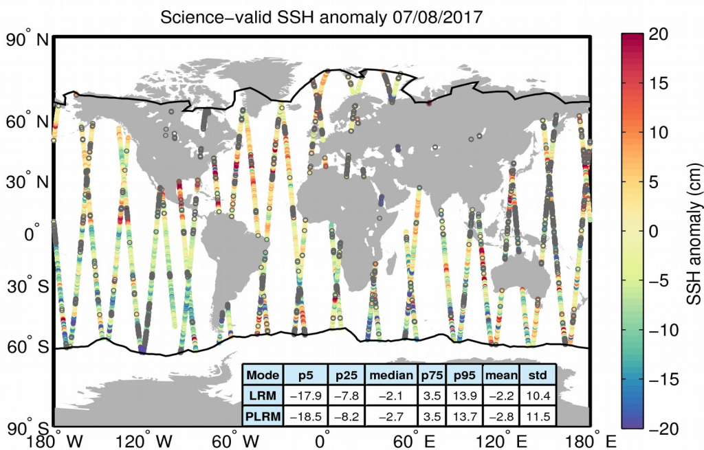
Figure 10. Geographical distribution of science-valid SSH anomaly data over oceans and lakes for 07/08/2017. The statistical values shown in the table refer to the SSH anomaly in cm and are calculated separately for LRM and PLRM regions. The black lines mark the outer limit of the Arctic and Antarctic polar polygons. Gray circles denote records that have been rejected based on the editing criteria described in Table 2.
