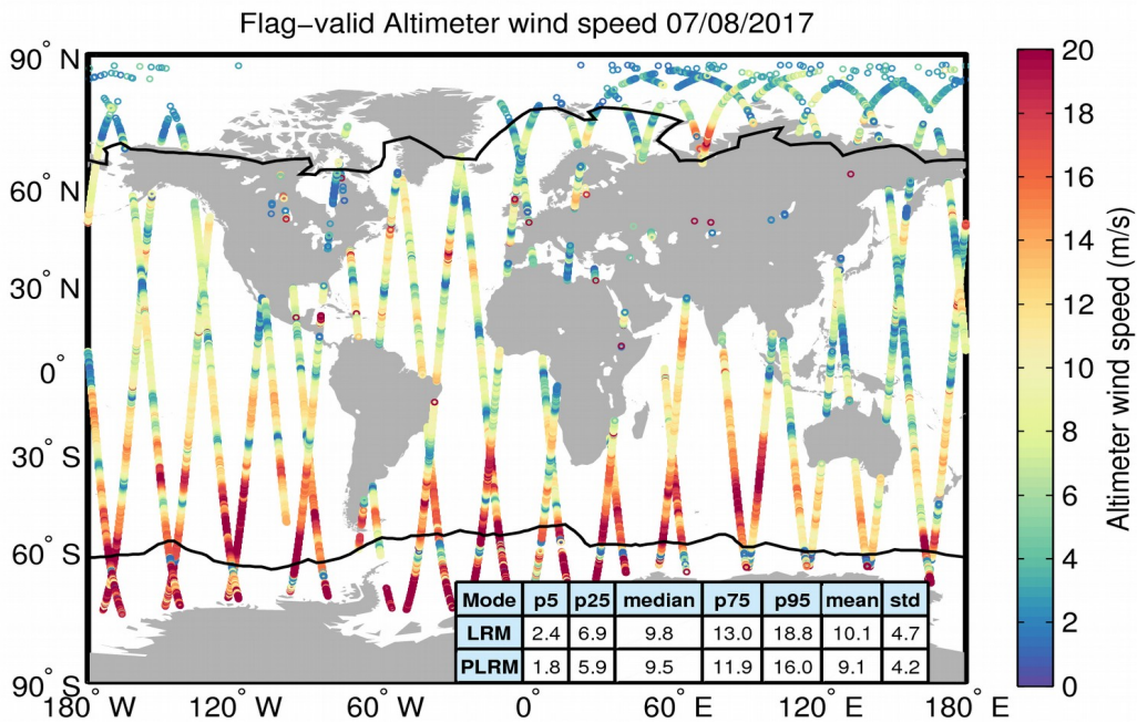
Figure 31. Geographical distribution of flag-valid wind data over oceans and lakes for 07/08/2017. The statistical values shown in the table refer to the wind in m/s and are calculated separately for LRM and PLRM regions. Measurements taken over polar polygons have been excluded from the computation of the statistical values. The black lines mark the outer limit of the Arctic and Antarctic polar polygons.
