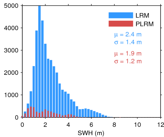
Figure 20. Histogram of science-valid SWH over oceans and lakes for LRM (blue) and PLRM (red) for 07/08/2017. The mean ( \mu ) and standard deviation ( \sigma ) are also shown. Note that values larger than 12 m are excluded from the histogram for the sake of readability but not from the computation of \mu and \sigma .
