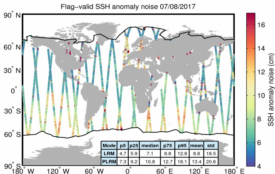
Figure 8. Geographical distribution of flag-valid 20-Hz SSH anomaly measurement noise over oceans and lakes for 07/08/2017. The statistical values shown in the table refer to the SSH anomaly noise and are calculated separately for LRM and PLRM regions. Measurements taken over polar polygons have been excluded from the computation of the statistical values. The black lines mark the outer limit of the Arctic and Antarctic polar polygons.
