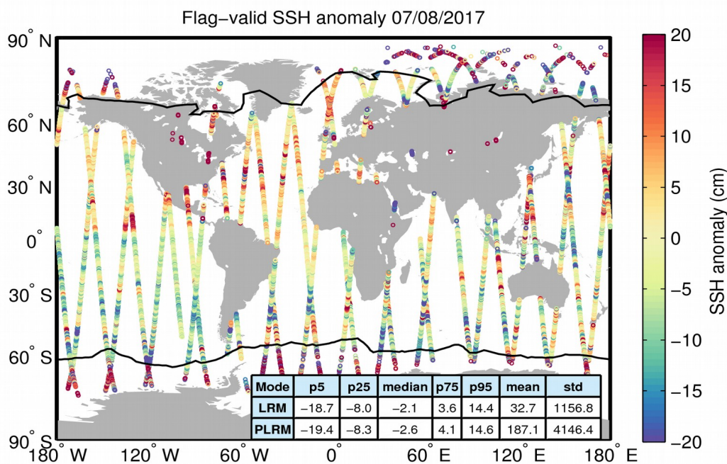
Figure 5. Geographical distribution of flag-valid 1-Hz SSH anomaly data over oceans and lakes for 07/08/2017. The statistical values shown in the table refer to the SSH anomaly in cm and are calculated separately for LRM and PLRM regions. Measurements taken over polar polygons have been excluded from the computation of the statistical values. The black lines mark the outer limit of the Arctic and Antarctic polar polygons.
