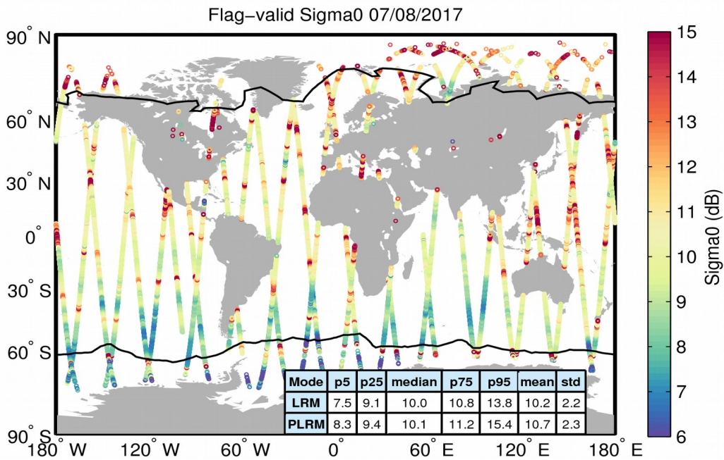
Figure 23. Geographical distribution of flag-valid sigma0 data over oceans and lakes for 07/08/2017. The statistical values shown in the table refer to the sigma0 in dB and are calculated separately for LRM and PLRM regions. Measurements taken over polar polygons have been excluded from the computation of the statistical values. The black lines mark the outer limit of the Arctic and Antarctic polar polygons.
