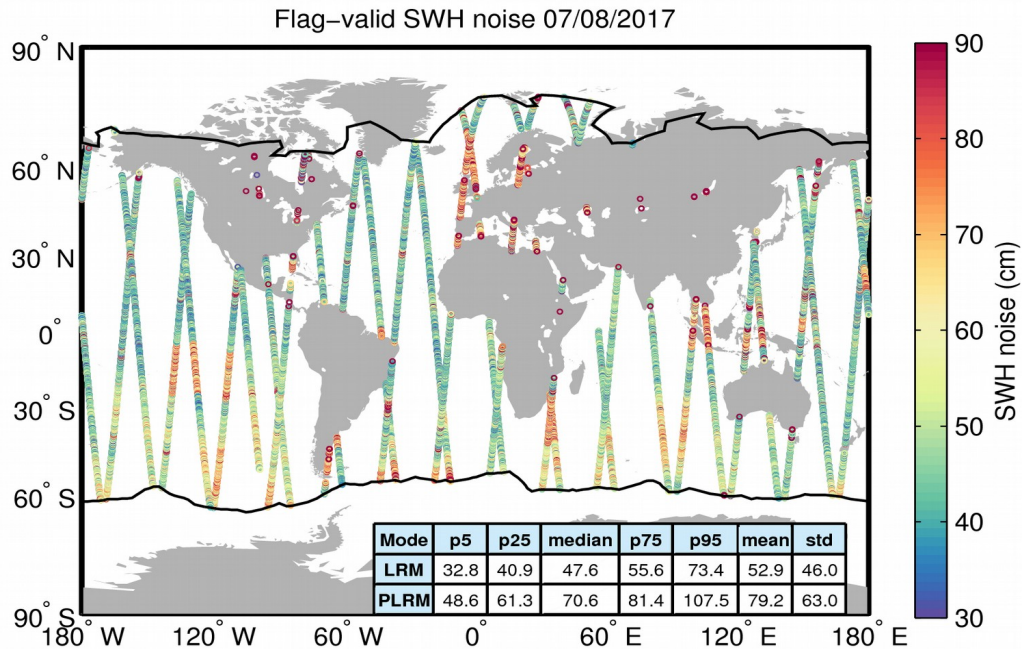
Figure 18. Geographical distribution of flag-valid 20-Hz SWH measurement noise over oceans and lakes for 07/08/2017. The statistical values shown in the table refer to the SWH noise and are calculated separately for LRM and PLRM regions. Measurements taken over polar polygons have been excluded from the computation of the statistical values. The black lines mark the outer limit of the Arctic and Antarctic polar polygons.
