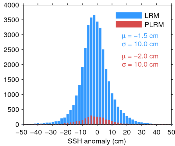
Figure 11. Histogram of science-valid SSH anomaly over oceans and lakes for LRM (blue) and PLRM (red) for 05/08/2017. The mean ( \mu ) and standard deviation ( \sigma ) are also shown. Note that values outside [-50 50] cm are excluded from the histogram for the sake of readability but not from the computation of \mu and \sigma .
