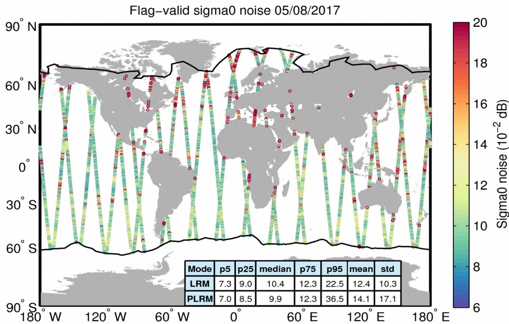
Figure 26. Geographical distribution of flag-valid 20-Hz sigma0 measurement noise over oceans and lakes for 05/08/2017. The statistical values shown in the table refer to the sigma0 noise and are calculated separately for LRM and PLRM regions. Measurements taken over polar polygons have been excluded from the computation of the statistical values. The black lines mark the outer limit of the Arctic and Antarctic polar polygons.
