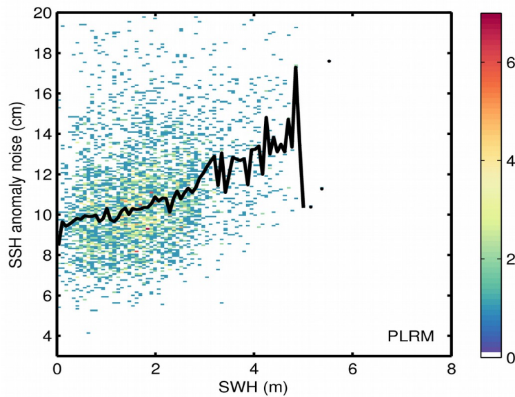
Figure 9. 2D histogram showing flag-valid SSH anomaly noise as a function of SWH for LRM (top) and PLRM (bottom) for 05/08/2017. The black line denotes the median SSH anomaly noise as a function of SWH.
