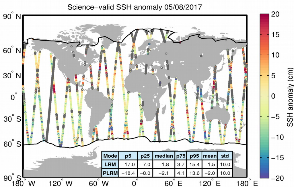
Figure 10. Geographical distribution of science-valid SSH anomaly data over oceans and lakes for 05/08/2017. The statistical values shown in the table refer to the SSH anomaly in cm and are calculated separately for LRM and PLRM regions. The black lines mark the outer limit of the Arctic and Antarctic polar polygons. Gray circles denote records that have been rejected based on the editing criteria described in Table 2.
