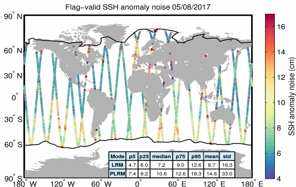
Figure 8. Geographical distribution of flag-valid 20-Hz SSH anomaly measurement noise over oceans and lakes for 05/08/2017. The statistical values shown in the table refer to the SSH anomaly noise and are calculated separately for LRM and PLRM regions. Measurements taken over polar polygons have been excluded from the computation of the statistical values. The black lines mark the outer limit of the Arctic and Antarctic polar polygons.
