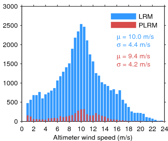
Figure 33. Histogram of flag-valid wind over oceans and lakes for LRM (blue) and PLRM (red) for 05/08/2017. The mean ( \mu ) and standard deviation ( \sigma ) are also shown. Note that values larger than 24 m/s are excluded from the histogram for the sake of readability but not from the computation of \mu and \sigma .
