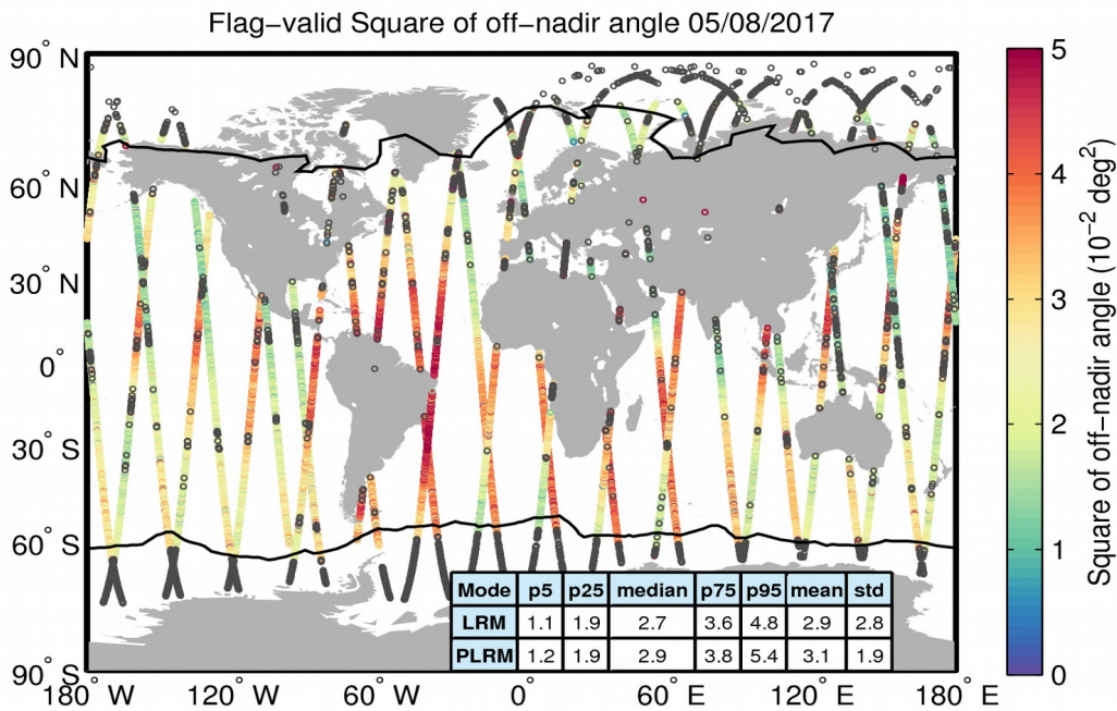
Figure 37. Geographical distribution of flag-valid mispointing data over oceans and lakes for 05/08/2017. The statistical values shown in the table refer to the mispointing in 10^{-2} deg 2 and are calculated separately for LRM and PLRM regions. Measurements taken over polar polygons have been excluded from the computation of the statistical values. The black lines mark the outer limit of the Arctic and Antarctic polar polygons. Gray circles denote negative values.
