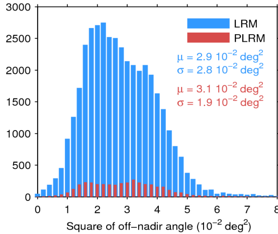
Figure 39. Histogram of flag-valid mispointing over oceans and lakes for LRM (blue) and PLRM (red) for 05/08/2017. Only positive values have been considered. The mean ( \mu ) and standard deviation ( \sigma ) are also shown. Note that values larger than 8 \cdot 10^{-2} \text{ deg}^2 are excluded from the histogram for the sake of readability but not from the computation of \mu and \sigma .
