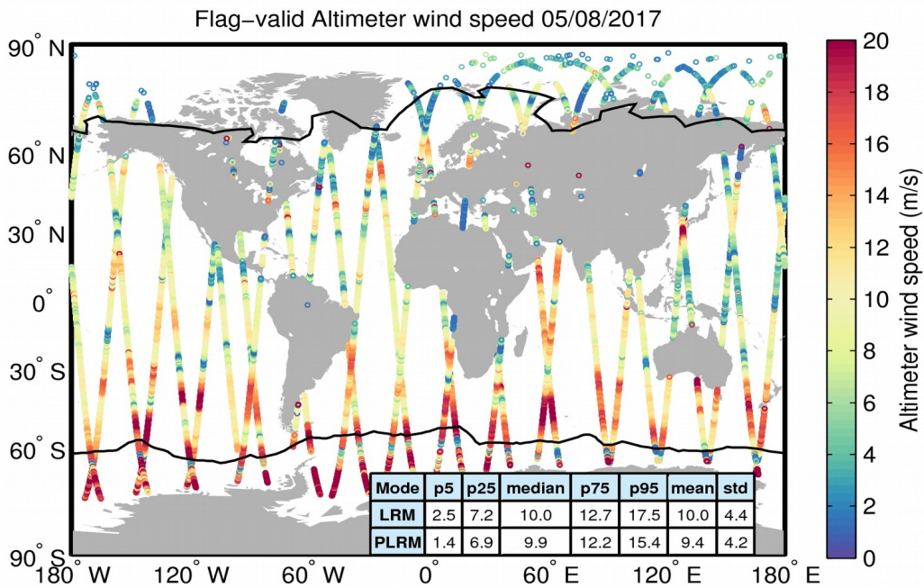
Figure 31. Geographical distribution of flag-valid wind data over oceans and lakes for 05/08/2017. The statistical values shown in the table refer to the wind in m/s and are calculated separately for LRM and PLRM regions. Measurements taken over polar polygons have been excluded from the computation of the statistical values. The black lines mark the outer limit of the Arctic and Antarctic polar polygons.
