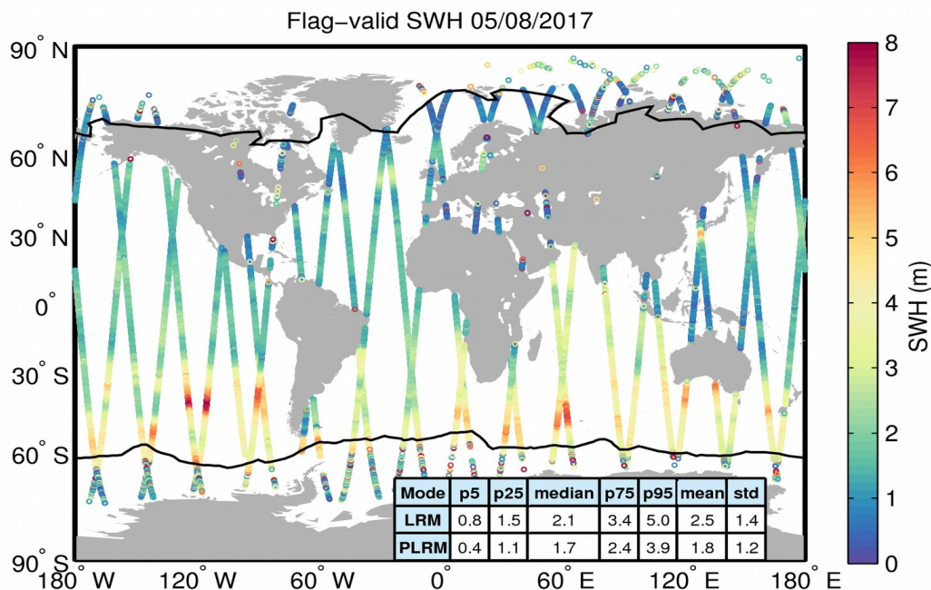
Figure 15. Geographical distribution of flag-valid SWH data over oceans and lakes for 05/08/2017. The statistical values shown in the table refer to the SWH in m and are calculated separately for LRM and PLRM regions. Measurements taken over polar polygons have been excluded from the computation of the statistical values. The black lines mark the outer limit of the Arctic and Antarctic polar polygons.
