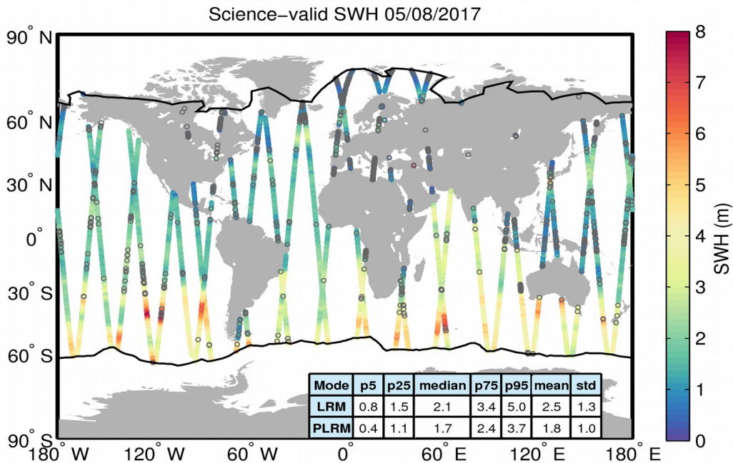
Figure 19. Geographical distribution of science-valid SWH data over oceans and lakes for 05/08/2017. The statistical values shown in the table refer to the SWH in m and are calculated separately for LRM and PLRM regions. The black lines mark the outer limit of the Arctic and Antarctic polar polygons. Gray circles denote records that have been rejected based on the editing criteria described in Table 3.
