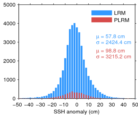
Figure 7. Histogram of flag-valid SSH anomaly over oceans and lakes for LRM (blue) and PLRM (red) for 05/08/2017. The mean ( \mu ) and standard deviation ( \sigma ) are also shown. Note that values outside [-50\ 50] cm are excluded from the histogram for the sake of readability but not from the computation of \mu and \sigma .
