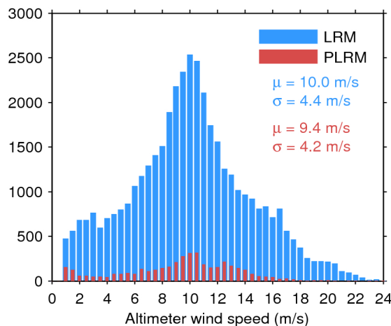
Figure 35. Histogram of science-valid wind over oceans and lakes for LRM (blue) and PLRM (red) for 05/08/2017. The mean ( \mu ) and standard deviation ( \sigma ) are also shown. Note that values larger than 24 m/s are excluded from the histogram for the sake of readability but not from the computation of \mu and \sigma .
