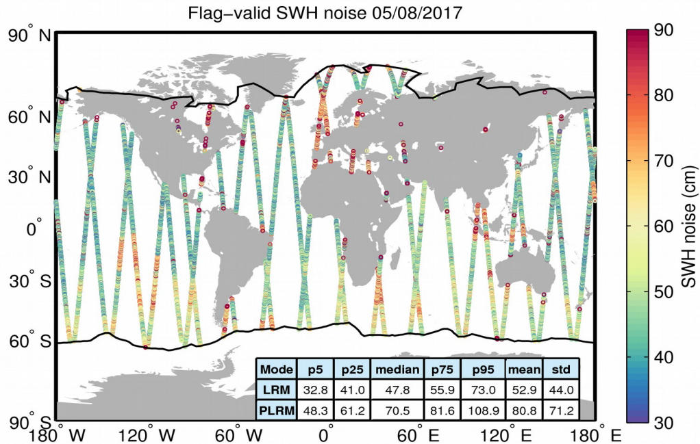
Figure 18. Geographical distribution of flag-valid 20-Hz SWH measurement noise over oceans and lakes for 05/08/2017. The statistical values shown in the table refer to the SWH noise and are calculated separately for LRM and PLRM regions. Measurements taken over polar polygons have been excluded from the computation of the statistical values. The black lines mark the outer limit of the Arctic and Antarctic polar polygons.
