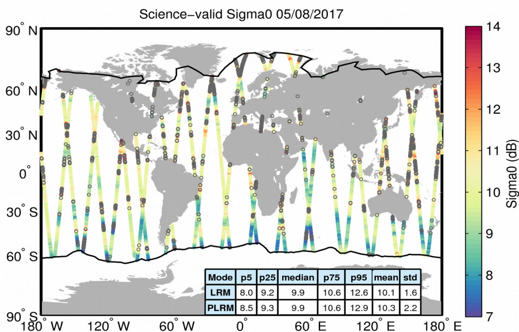
Figure 27. Geographical distribution of science-valid sigma0 data over oceans and lakes for 05/08/2017. The statistical values shown in the table refer to the sigma0 in dB and are calculated separately for LRM and PLRM regions. The black lines mark the outer limit of the Arctic and Antarctic polar polygons. Gray circles denote records that have been rejected based on the editing criteria described in Table 4.
