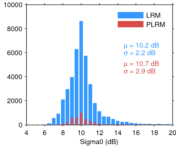
Figure 25. Histogram of flag-valid sigma0 over oceans and lakes for LRM (blue) and PLRM (red) for 05/08/2017. The mean ( \mu ) and standard deviation ( \sigma ) are also shown. Note that values outside [4 20] dB are excluded from the histogram for the sake of readability but not from the computation of \mu and \sigma .
