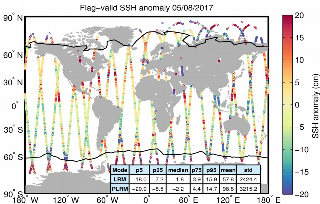
Figure 5. Geographical distribution of flag-valid 1-Hz SSH anomaly data over oceans and lakes for 05/08/2017. The statistical values shown in the table refer to the SSH anomaly in cm and are calculated separately for LRM and PLRM regions. Measurements taken over polar polygons have been excluded from the computation of the statistical values. The black lines mark the outer limit of the Arctic and Antarctic polar polygons.
