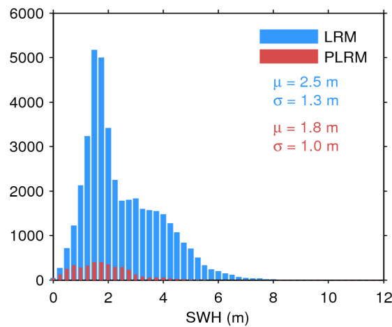
Figure 20. Histogram of science-valid SWH over oceans and lakes for LRM (blue) and PLRM (red) for 05/08/2017. The mean ( \mu ) and standard deviation ( \sigma ) are also shown. Note that values larger than 12 m are excluded from the histogram for the sake of readability but not from the computation of \mu and \sigma .
