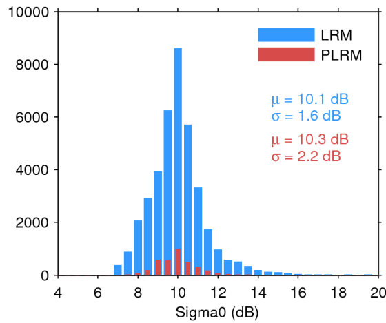
Figure 28. Histogram of science-valid sigma0 over oceans and lakes for LRM (blue) and PLRM (red) for 05/08/2017. The mean ( \mu ) and standard deviation ( \sigma ) are also shown. Note that values outside [4 20] dB are excluded from the histogram for the sake of readability but not from the computation of \mu and \sigma .
