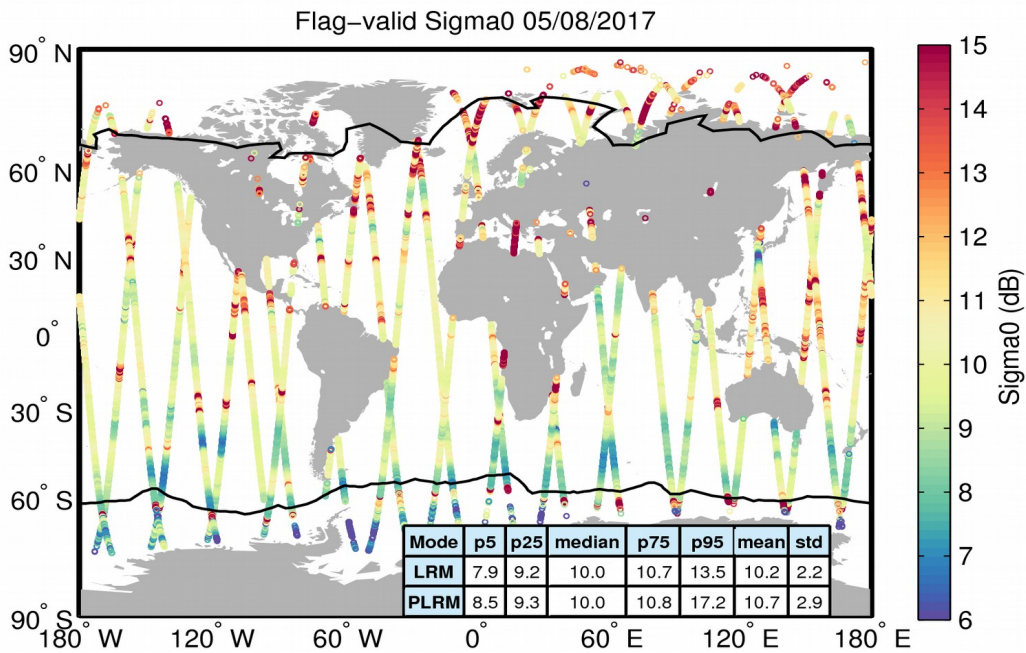
Figure 23. Geographical distribution of flag-valid sigma0 data over oceans and lakes for 05/08/2017. The statistical values shown in the table refer to the sigma0 in dB and are calculated separately for LRM and PLRM regions. Measurements taken over polar polygons have been excluded from the computation of the statistical values. The black lines mark the outer limit of the Arctic and Antarctic polar polygons.
