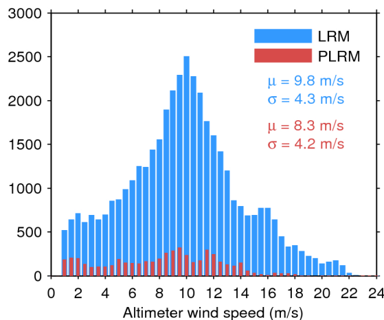
Figure 35. Histogram of science-valid wind over oceans and lakes for LRM (blue) and PLRM (red) for 04/08/2017. The mean ( \mu ) and standard deviation ( \sigma ) are also shown. Note that values larger than 24 m/s are excluded from the histogram for the sake of readability but not from the computation of \mu and \sigma .
