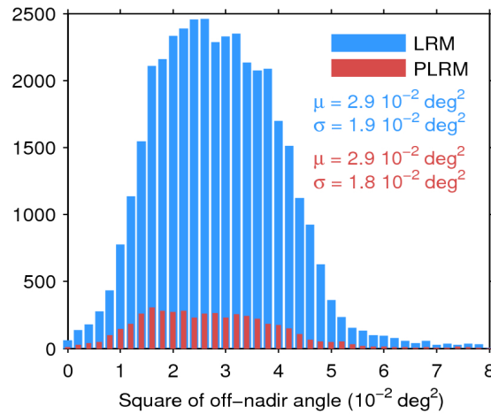
Figure 39. Histogram of flag-valid mispointing over oceans and lakes for LRM (blue) and PLRM (red) for 04/08/2017. Only positive values have been considered. The mean ( \mu ) and standard deviation ( \sigma ) are also shown. Note that values larger than 8 \cdot 10^{-2} \text{ deg}^2 are excluded from the histogram for the sake of readability but not from the computation of \mu and \sigma .
