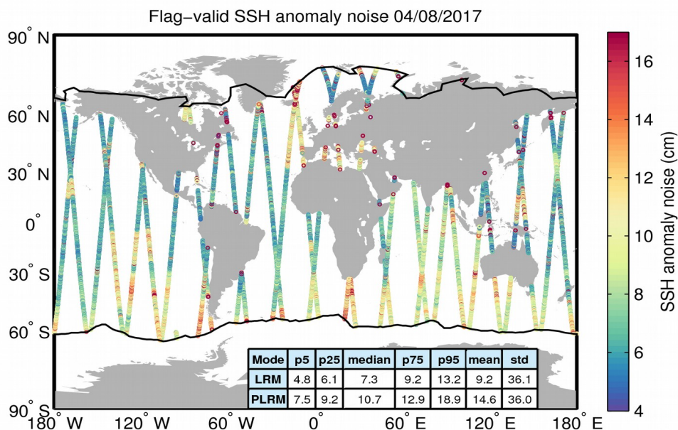
Figure 8. Geographical distribution of flag-valid 20-Hz SSH anomaly measurement noise over oceans and lakes for 04/08/2017. The statistical values shown in the table refer to the SSH anomaly noise and are calculated separately for LRM and PLRM regions. Measurements taken over polar polygons have been excluded from the computation of the statistical values. The black lines mark the outer limit of the Arctic and Antarctic polar polygons.
