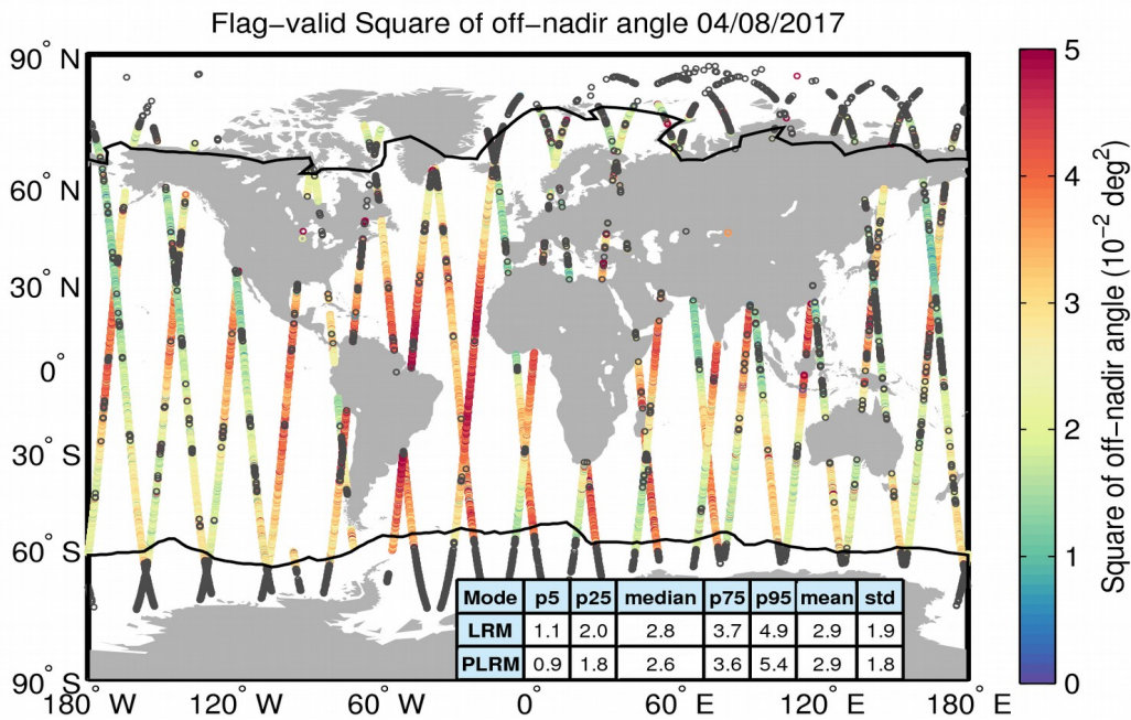
Figure 37. Geographical distribution of flag-valid mispointing data over oceans and lakes for 04/08/2017. The statistical values shown in the table refer to the mispointing in 10^{-2} deg 2 and are calculated separately for LRM and PLRM regions. Measurements taken over polar polygons have been excluded from the computation of the statistical values. The black lines mark the outer limit of the Arctic and Antarctic polar polygons. Gray circles denote negative values.
