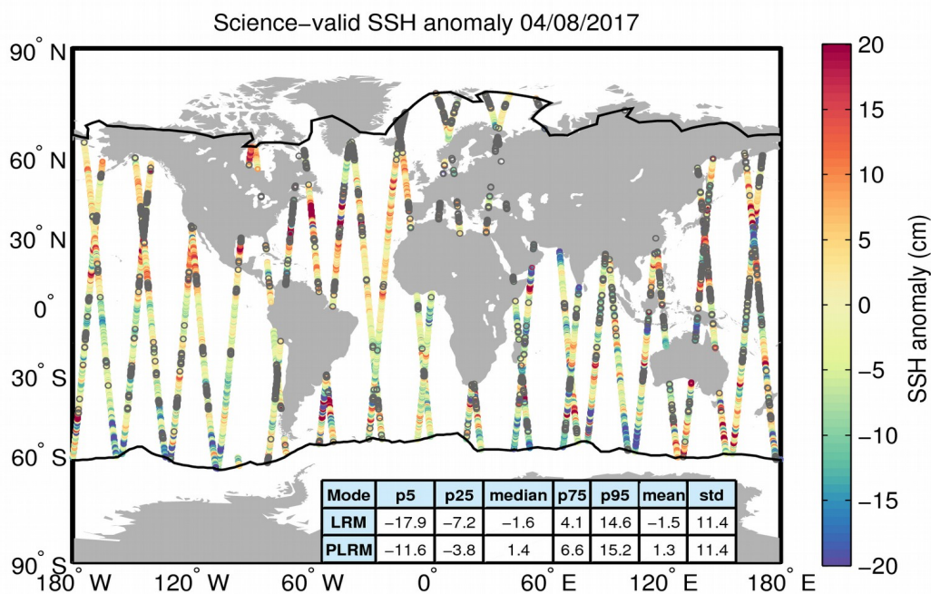
Figure 10. Geographical distribution of science-valid SSH anomaly data over oceans and lakes for 04/08/2017. The statistical values shown in the table refer to the SSH anomaly in cm and are calculated separately for LRM and PLRM regions. The black lines mark the outer limit of the Arctic and Antarctic polar polygons. Gray circles denote records that have been rejected based on the editing criteria described in Table 2.
