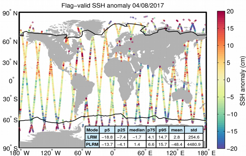
Figure 5. Geographical distribution of flag-valid 1-Hz SSH anomaly data over oceans and lakes for 04/08/2017. The statistical values shown in the table refer to the SSH anomaly in cm and are calculated separately for LRM and PLRM regions. Measurements taken over polar polygons have been excluded from the computation of the statistical values. The black lines mark the outer limit of the Arctic and Antarctic polar polygons.
