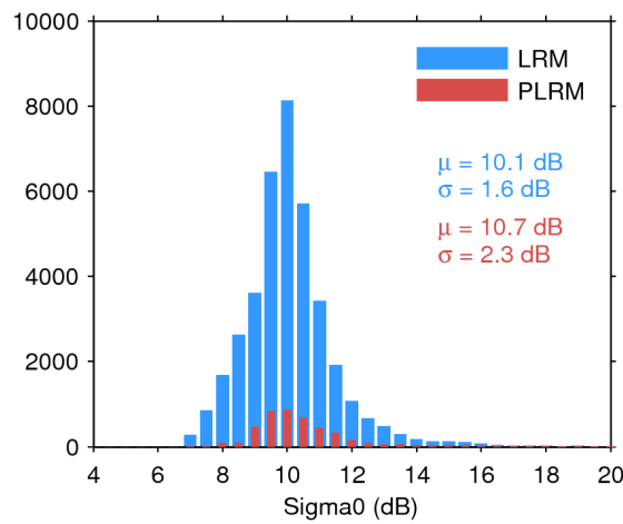
Figure 28. Histogram of science-valid sigma0 over oceans and lakes for LRM (blue) and PLRM (red) for 04/08/2017. The mean ( \mu ) and standard deviation ( \sigma ) are also shown. Note that values outside [4 20] dB are excluded from the histogram for the sake of readability but not from the computation of \mu and \sigma .
