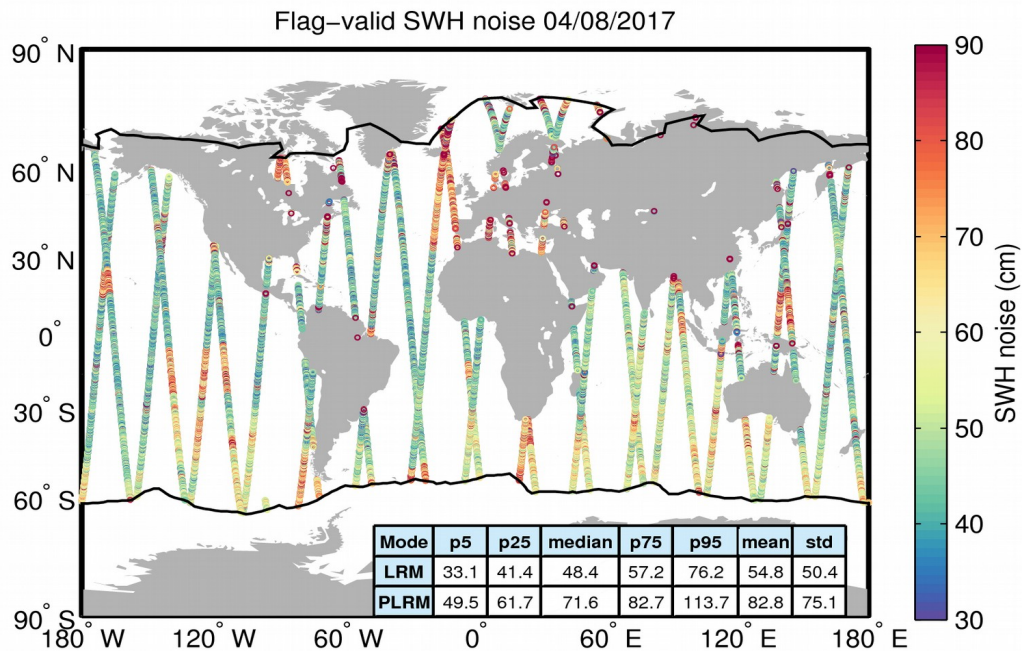
Figure 18. Geographical distribution of flag-valid 20-Hz SWH measurement noise over oceans and lakes for 04/08/2017. The statistical values shown in the table refer to the SWH noise and are calculated separately for LRM and PLRM regions. Measurements taken over polar polygons have been excluded from the computation of the statistical values. The black lines mark the outer limit of the Arctic and Antarctic polar polygons.
