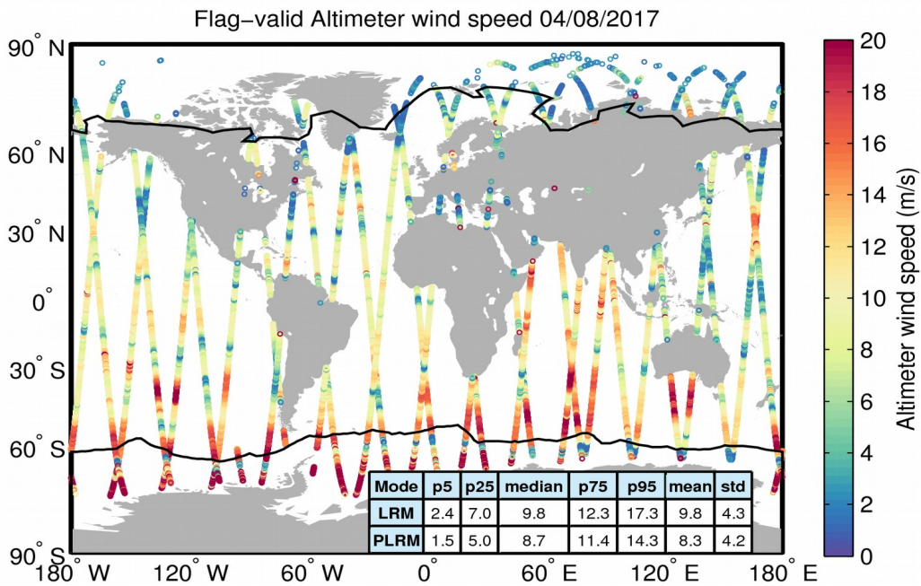
Figure 31. Geographical distribution of flag-valid wind data over oceans and lakes for 04/08/2017. The statistical values shown in the table refer to the wind in m/s and are calculated separately for LRM and PLRM regions. Measurements taken over polar polygons have been excluded from the computation of the statistical values. The black lines mark the outer limit of the Arctic and Antarctic polar polygons.
