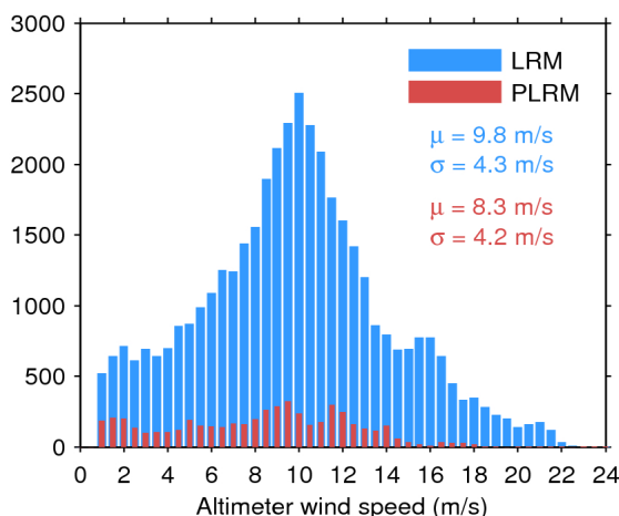
Figure 33. Histogram of flag-valid wind over oceans and lakes for LRM (blue) and PLRM (red) for 04/08/2017. The mean ( \mu ) and standard deviation ( \sigma ) are also shown. Note that values larger than 24 m/s are excluded from the histogram for the sake of readability but not from the computation of \mu and \sigma .
