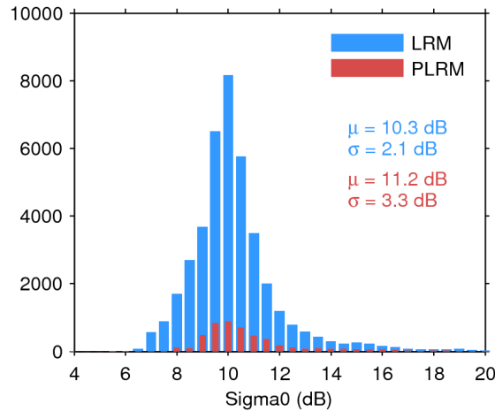
Figure 25. Histogram of flag-valid sigma0 over oceans and lakes for LRM (blue) and PLRM (red) for 04/08/2017. The mean ( \mu ) and standard deviation ( \sigma ) are also shown. Note that values outside [4 20] dB are excluded from the histogram for the sake of readability but not from the computation of \mu and \sigma .
