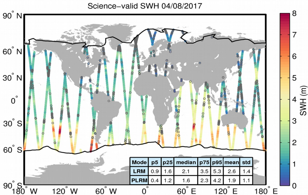
Figure 19. Geographical distribution of science-valid SWH data over oceans and lakes for 04/08/2017. The statistical values shown in the table refer to the SWH in m and are calculated separately for LRM and PLRM regions. The black lines mark the outer limit of the Arctic and Antarctic polar polygons. Gray circles denote records that have been rejected based on the editing criteria described in Table 3.
