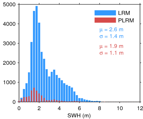
Figure 20. Histogram of science-valid SWH over oceans and lakes for LRM (blue) and PLRM (red) for 04/08/2017. The mean ( \mu ) and standard deviation ( \sigma ) are also shown. Note that values larger than 12 m are excluded from the histogram for the sake of readability but not from the computation of \mu and \sigma .
