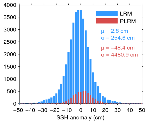
Figure 7. Histogram of flag-valid SSH anomaly over oceans and lakes for LRM (blue) and PLRM (red) for 04/08/2017. The mean ( \mu ) and standard deviation ( \sigma ) are also shown. Note that values outside [-50 \ 50] cm are excluded from the histogram for the sake of readability but not from the computation of \mu and \sigma .
