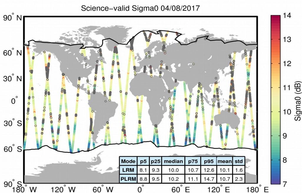
Figure 27. Geographical distribution of science-valid sigma0 data over oceans and lakes for 04/08/2017. The statistical values shown in the table refer to the sigma0 in dB and are calculated separately for LRM and PLRM regions. The black lines mark the outer limit of the Arctic and Antarctic polar polygons. Gray circles denote records that have been rejected based on the editing criteria described in Table 4.
