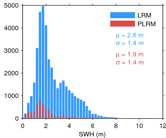
Figure 17. Histogram of flag-valid SWH over oceans and lakes for LRM (blue) and PLRM (red) for 04/08/2017. The mean ( \mu ) and standard deviation ( \sigma ) are also shown. Note that values larger than 12 m are excluded from the histogram for the sake of readability but not from the computation of \mu and \sigma .
