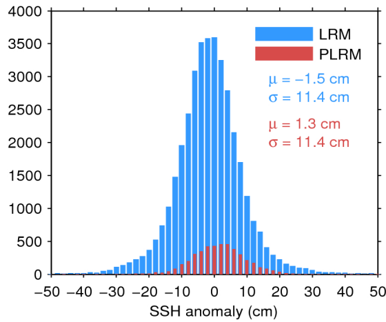
Figure 11. Histogram of science-valid SSH anomaly over oceans and lakes for LRM (blue) and PLRM (red) for 04/08/2017. The mean ( \mu ) and standard deviation ( \sigma ) are also shown. Note that values outside [-50\ 50] cm are excluded from the histogram for the sake of readability but not from the computation of \mu and \sigma .
