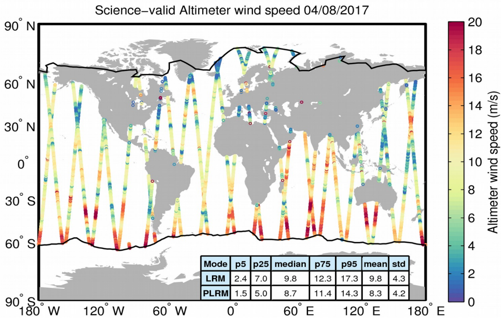
Figure 34. Geographical distribution of science-valid wind data over oceans and lakes for 04/08/2017. The statistical values shown in the table refer to the wind in m/s and are calculated separately for LRM and PLRM regions. The black lines mark the outer limit of the Arctic and Antarctic polar polygons. Gray circles denote records that have been rejected based on the editing criteria described in Table 5.
