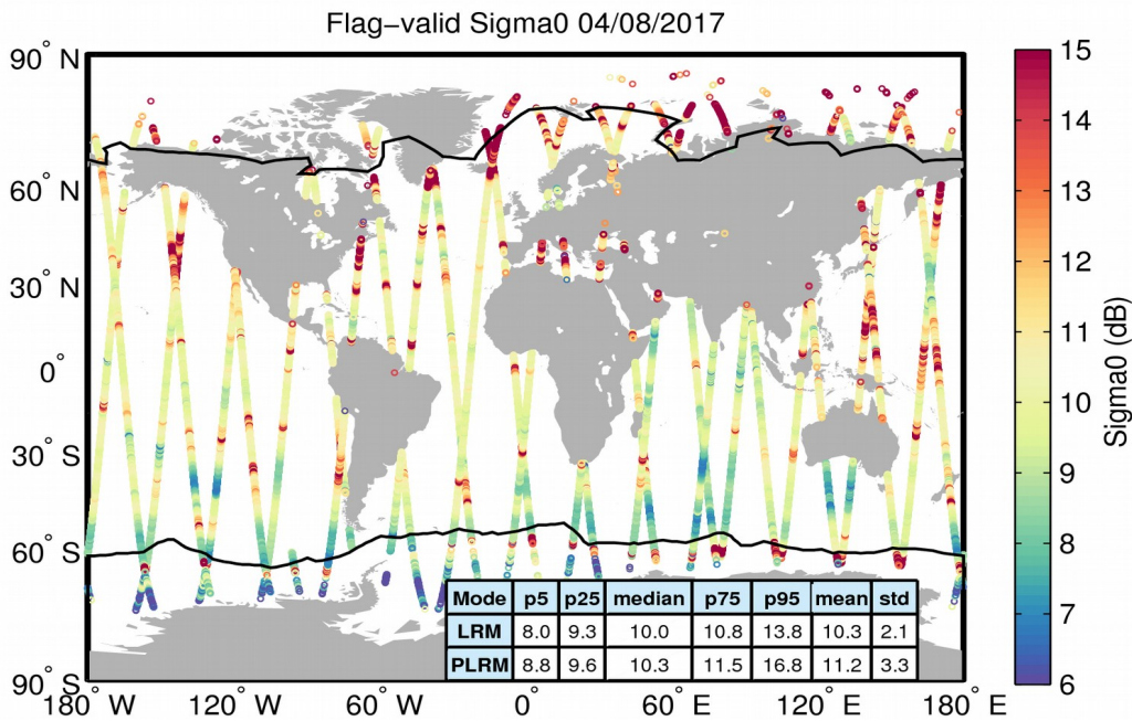
Figure 23. Geographical distribution of flag-valid sigma0 data over oceans and lakes for 04/08/2017. The statistical values shown in the table refer to the sigma0 in dB and are calculated separately for LRM and PLRM regions. Measurements taken over polar polygons have been excluded from the computation of the statistical values. The black lines mark the outer limit of the Arctic and Antarctic polar polygons.
