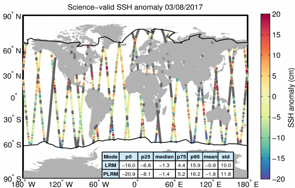
Figure 10. Geographical distribution of science-valid SSH anomaly data over oceans and lakes for 03/08/2017. The statistical values shown in the table refer to the SSH anomaly in cm and are calculated separately for LRM and PLRM regions. The black lines mark the outer limit of the Arctic and Antarctic polar polygons. Gray circles denote records that have been rejected based on the editing criteria described in Table 2.
