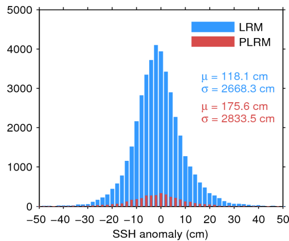
Figure 7. Histogram of flag-valid SSH anomaly over oceans and lakes for LRM (blue) and PLRM (red) for 03/08/2017. The mean ( \mu ) and standard deviation ( \sigma ) are also shown. Note that values outside [-50\ 50] cm are excluded from the histogram for the sake of readability but not from the computation of \mu and \sigma .
