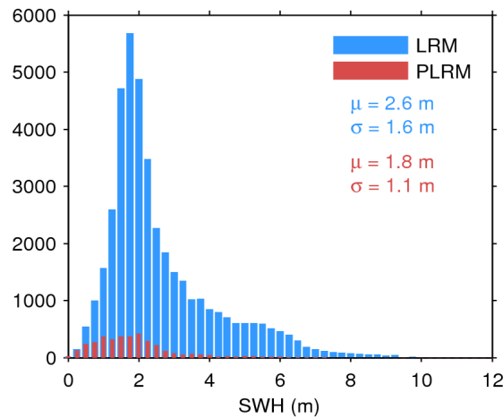
Figure 20. Histogram of science-valid SWH over oceans and lakes for LRM (blue) and PLRM (red) for 03/08/2017. The mean ( \mu ) and standard deviation ( \sigma ) are also shown. Note that values larger than 12 m are excluded from the histogram for the sake of readability but not from the computation of \mu and \sigma .
