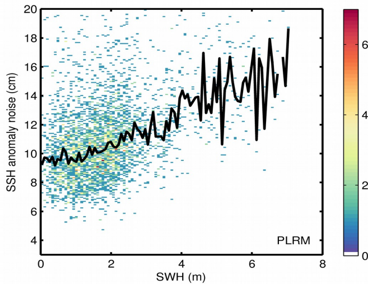
Figure 9. 2D histogram showing flag-valid SSH anomaly noise as a function of SWH for LRM (top) and PLRM (bottom) for 03/08/2017. The black line denotes the median SSH anomaly noise as a function of SWH.
