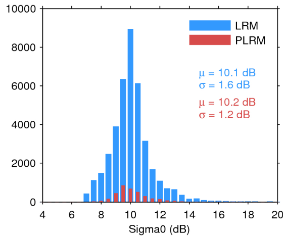
Figure 28. Histogram of science-valid sigma0 over oceans and lakes for LRM (blue) and PLRM (red) for 03/08/2017. The mean ( \mu ) and standard deviation ( \sigma ) are also shown. Note that values outside [4 20] dB are excluded from the histogram for the sake of readability but not from the computation of \mu and \sigma .
