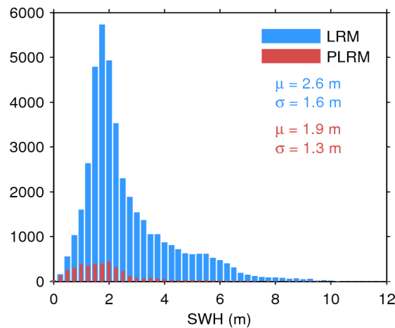
Figure 17. Histogram of flag-valid SWH over oceans and lakes for LRM (blue) and PLRM (red) for 03/08/2017. The mean ( \mu ) and standard deviation ( \sigma ) are also shown. Note that values larger than 12 m are excluded from the histogram for the sake of readability but not from the computation of \mu and \sigma .
