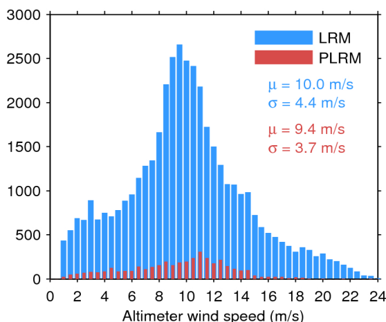
Figure 33. Histogram of flag-valid wind over oceans and lakes for LRM (blue) and PLRM (red) for 03/08/2017. The mean ( \mu ) and standard deviation ( \sigma ) are also shown. Note that values larger than 24 m/s are excluded from the histogram for the sake of readability but not from the computation of \mu and \sigma .
