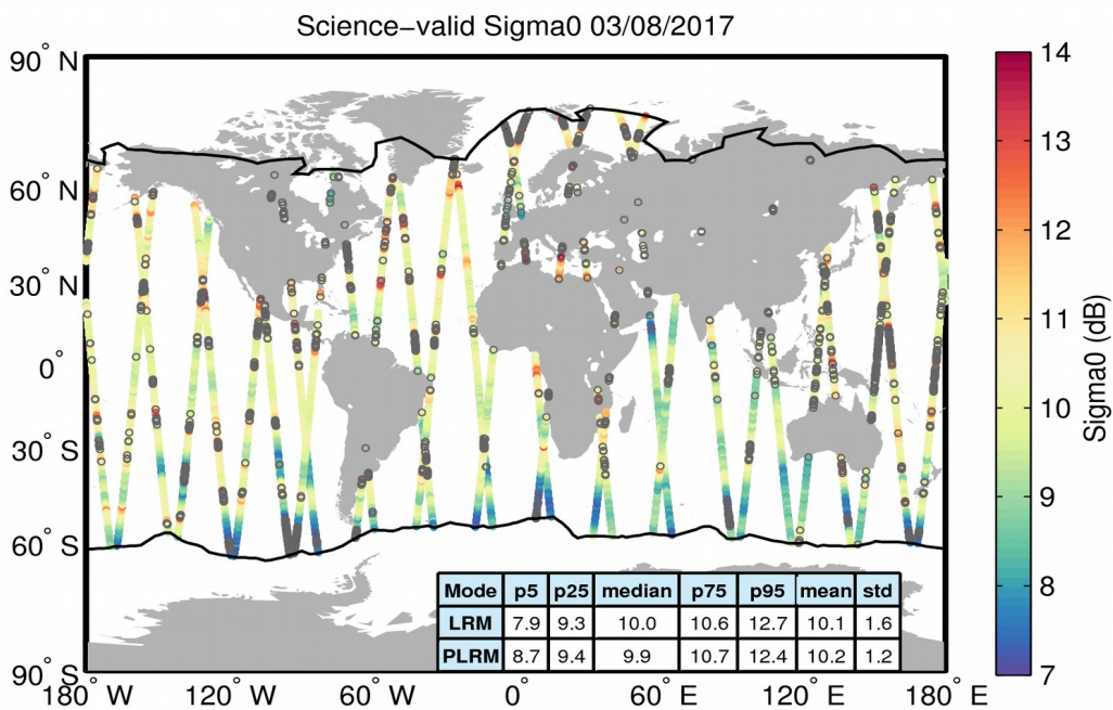
Figure 27. Geographical distribution of science-valid sigma0 data over oceans and lakes for 03/08/2017. The statistical values shown in the table refer to the sigma0 in dB and are calculated separately for LRM and PLRM regions. The black lines mark the outer limit of the Arctic and Antarctic polar polygons. Gray circles denote records that have been rejected based on the editing criteria described in Table 4.
