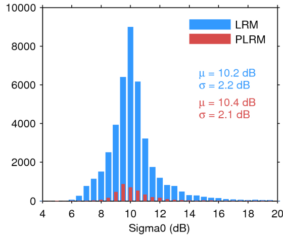
Figure 25. Histogram of flag-valid sigma0 over oceans and lakes for LRM (blue) and PLRM (red) for 03/08/2017. The mean ( \mu ) and standard deviation ( \sigma ) are also shown. Note that values outside [4 20] dB are excluded from the histogram for the sake of readability but not from the computation of \mu and \sigma .
