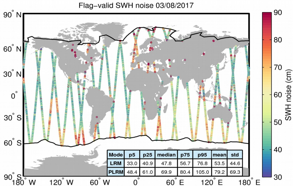
Figure 18. Geographical distribution of flag-valid 20-Hz SWH measurement noise over oceans and lakes for 03/08/2017. The statistical values shown in the table refer to the SWH noise and are calculated separately for LRM and PLRM regions. Measurements taken over polar polygons have been excluded from the computation of the statistical values. The black lines mark the outer limit of the Arctic and Antarctic polar polygons.
