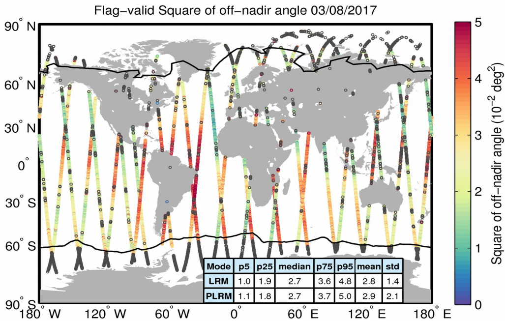
Figure 37. Geographical distribution of flag-valid mispointing data over oceans and lakes for 03/08/2017. The statistical values shown in the table refer to the mispointing in 10^{-2} deg 2 and are calculated separately for LRM and PLRM regions. Measurements taken over polar polygons have been excluded from the computation of the statistical values. The black lines mark the outer limit of the Arctic and Antarctic polar polygons. Gray circles denote negative values.
