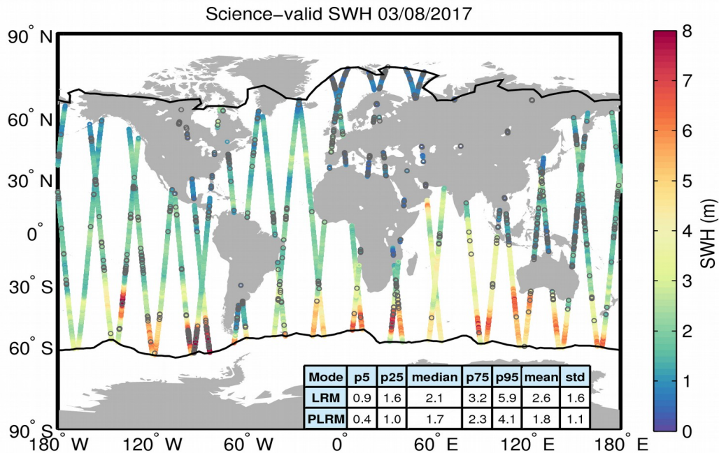
Figure 19. Geographical distribution of science-valid SWH data over oceans and lakes for 03/08/2017. The statistical values shown in the table refer to the SWH in m and are calculated separately for LRM and PLRM regions. The black lines mark the outer limit of the Arctic and Antarctic polar polygons. Gray circles denote records that have been rejected based on the editing criteria described in Table 3.
