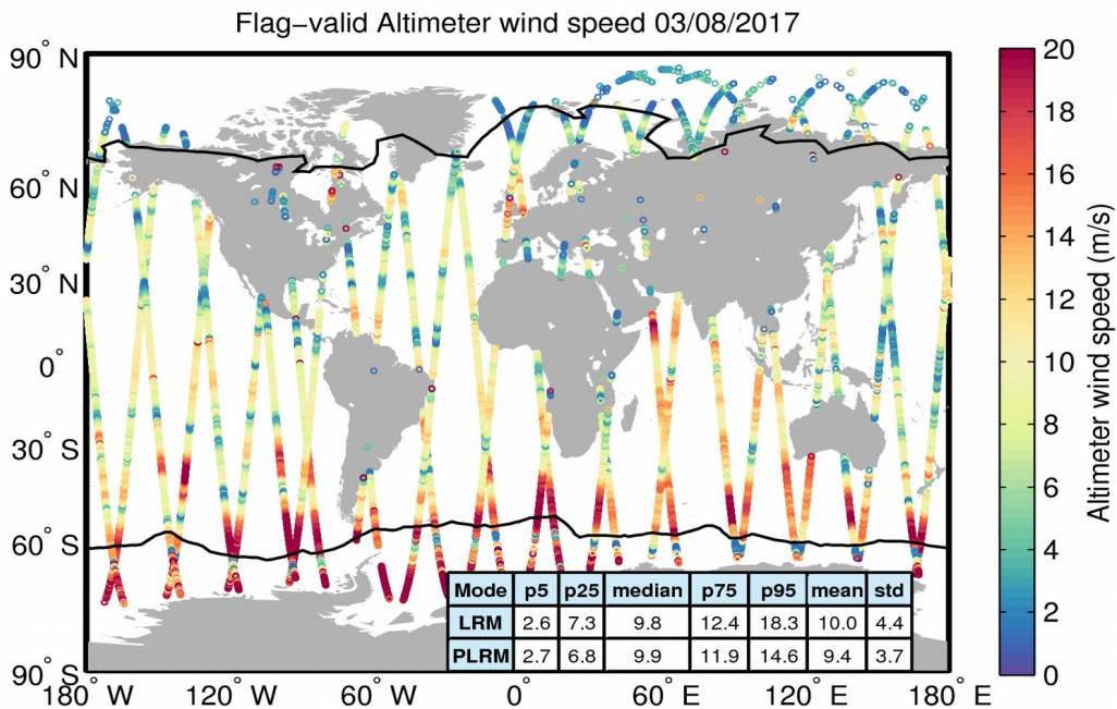
Figure 31. Geographical distribution of flag-valid wind data over oceans and lakes for 03/08/2017. The statistical values shown in the table refer to the wind in m/s and are calculated separately for LRM and PLRM regions. Measurements taken over polar polygons have been excluded from the computation of the statistical values. The black lines mark the outer limit of the Arctic and Antarctic polar polygons.
