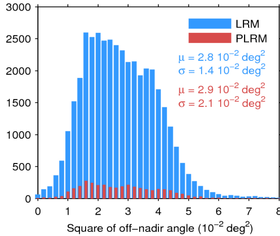
Figure 39. Histogram of flag-valid mispointing over oceans and lakes for LRM (blue) and PLRM (red) for 03/08/2017. Only positive values have been considered. The mean ( \mu ) and standard deviation ( \sigma ) are also shown. Note that values larger than 8 \cdot 10^{-2} \text{ deg}^2 are excluded from the histogram for the sake of readability but not from the computation of \mu and \sigma .
