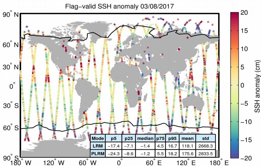
Figure 5. Geographical distribution of flag-valid 1-Hz SSH anomaly data over oceans and lakes for 03/08/2017. The statistical values shown in the table refer to the SSH anomaly in cm and are calculated separately for LRM and PLRM regions. Measurements taken over polar polygons have been excluded from the computation of the statistical values. The black lines mark the outer limit of the Arctic and Antarctic polar polygons.
