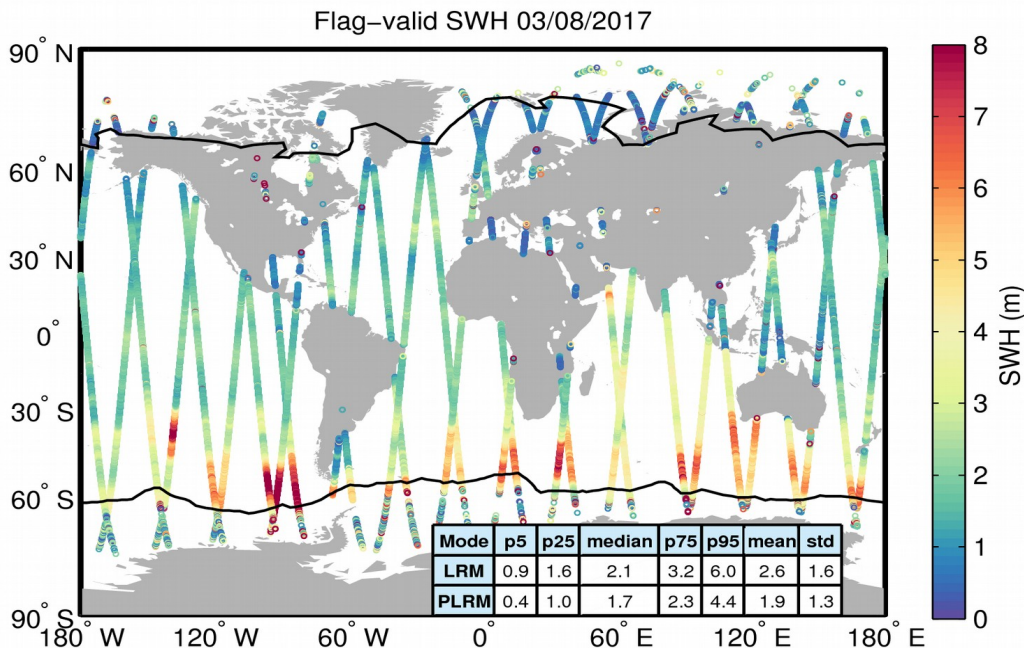
Figure 15. Geographical distribution of flag-valid SWH data over oceans and lakes for 03/08/2017. The statistical values shown in the table refer to the SWH in m and are calculated separately for LRM and PLRM regions. Measurements taken over polar polygons have been excluded from the computation of the statistical values. The black lines mark the outer limit of the Arctic and Antarctic polar polygons.
