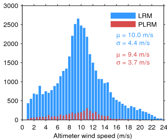
Figure 35. Histogram of science-valid wind over oceans and lakes for LRM (blue) and PLRM (red) for 03/08/2017. The mean ( \mu ) and standard deviation ( \sigma ) are also shown. Note that values larger than 24 m/s are excluded from the histogram for the sake of readability but not from the computation of \mu and \sigma .
