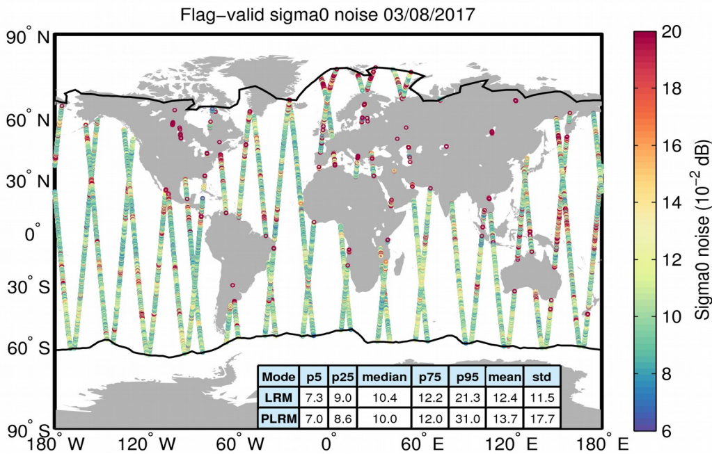
Figure 26. Geographical distribution of flag-valid 20-Hz sigma0 measurement noise over oceans and lakes for 03/08/2017. The statistical values shown in the table refer to the sigma0 noise and are calculated separately for LRM and PLRM regions. Measurements taken over polar polygons have been excluded from the computation of the statistical values. The black lines mark the outer limit of the Arctic and Antarctic polar polygons.
