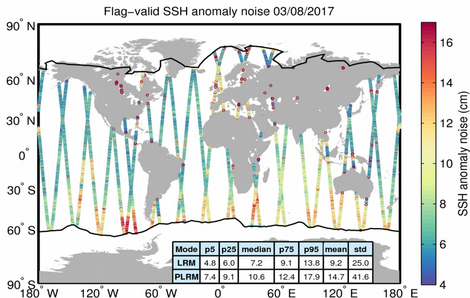
Figure 8. Geographical distribution of flag-valid 20-Hz SSH anomaly measurement noise over oceans and lakes for 03/08/2017. The statistical values shown in the table refer to the SSH anomaly noise and are calculated separately for LRM and PLRM regions. Measurements taken over polar polygons have been excluded from the computation of the statistical values. The black lines mark the outer limit of the Arctic and Antarctic polar polygons.
