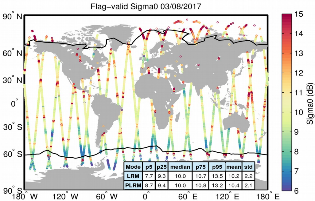
Figure 23. Geographical distribution of flag-valid sigma0 data over oceans and lakes for 03/08/2017. The statistical values shown in the table refer to the sigma0 in dB and are calculated separately for LRM and PLRM regions. Measurements taken over polar polygons have been excluded from the computation of the statistical values. The black lines mark the outer limit of the Arctic and Antarctic polar polygons.
