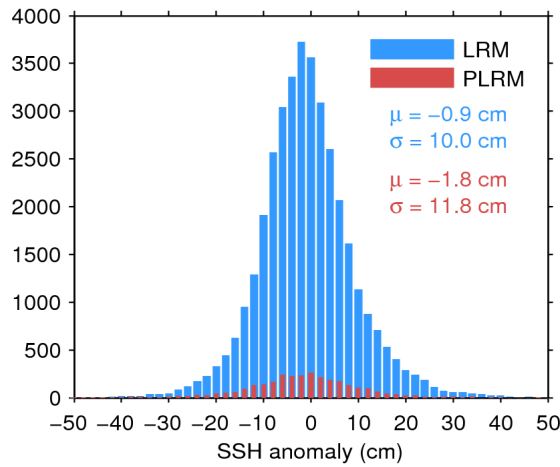
Figure 11. Histogram of science-valid SSH anomaly over oceans and lakes for LRM (blue) and PLRM (red) for 03/08/2017. The mean ( \mu ) and standard deviation ( \sigma ) are also shown. Note that values outside [-50\ 50] cm are excluded from the histogram for the sake of readability but not from the computation of \mu and \sigma .
