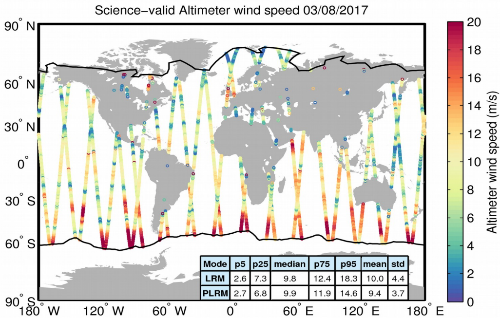
Figure 34. Geographical distribution of science-valid wind data over oceans and lakes for 03/08/2017. The statistical values shown in the table refer to the wind in m/s and are calculated separately for LRM and PLRM regions. The black lines mark the outer limit of the Arctic and Antarctic polar polygons. Gray circles denote records that have been rejected based on the editing criteria described in Table 5.
