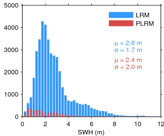
Figure 17. Histogram of flag-valid SWH over oceans and lakes for LRM (blue) and PLRM (red) for 30/07/2017. The mean ( \mu ) and standard deviation ( \sigma ) are also shown. Note that values larger than 12 m are excluded from the histogram for the sake of readability but not from the computation of \mu and \sigma .
