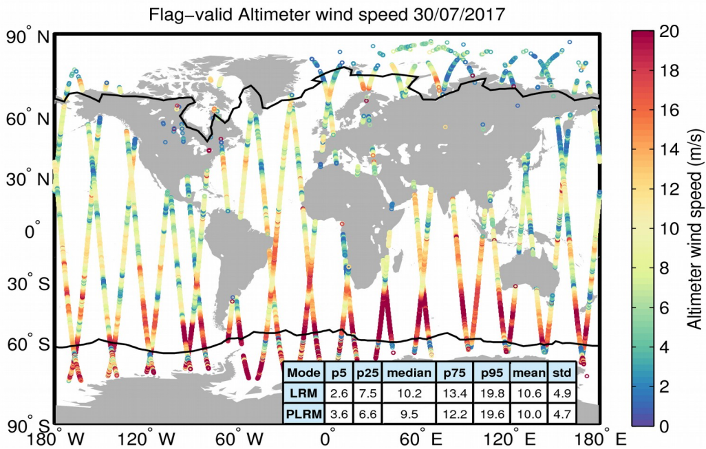
Figure 31. Geographical distribution of flag-valid wind data over oceans and lakes for 30/07/2017. The statistical values shown in the table refer to the wind in m/s and are calculated separately for LRM and PLRM regions. Measurements taken over polar polygons have been excluded from the computation of the statistical values. The black lines mark the outer limit of the Arctic and Antarctic polar polygons.
