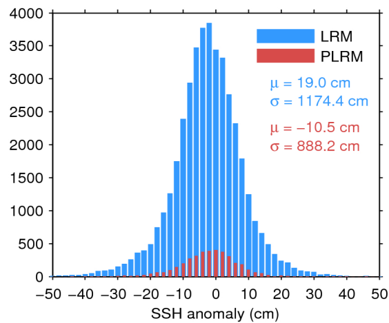
Figure 7. Histogram of flag-valid SSH anomaly over oceans and lakes for LRM (blue) and PLRM (red) for 30/07/2017. The mean ( \mu ) and standard deviation ( \sigma ) are also shown. Note that values outside [-50 50] cm are excluded from the histogram for the sake of readability but not from the computation of \mu and \sigma .
