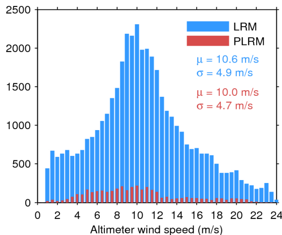
Figure 35. Histogram of science-valid wind over oceans and lakes for LRM (blue) and PLRM (red) for 30/07/2017. The mean ( \mu ) and standard deviation ( \sigma ) are also shown. Note that values larger than 24 m/s are excluded from the histogram for the sake of readability but not from the computation of \mu and \sigma .
