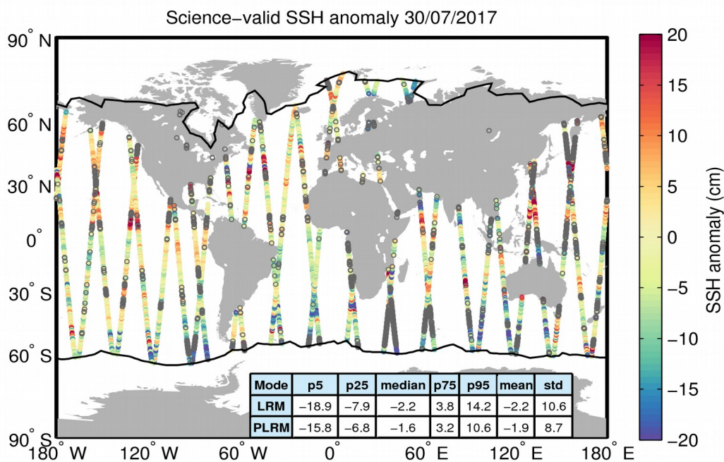
Figure 10. Geographical distribution of science-valid SSH anomaly data over oceans and lakes for 30/07/2017. The statistical values shown in the table refer to the SSH anomaly in cm and are calculated separately for LRM and PLRM regions. The black lines mark the outer limit of the Arctic and Antarctic polar polygons. Gray circles denote records that have been rejected based on the editing criteria described in Table 2.
