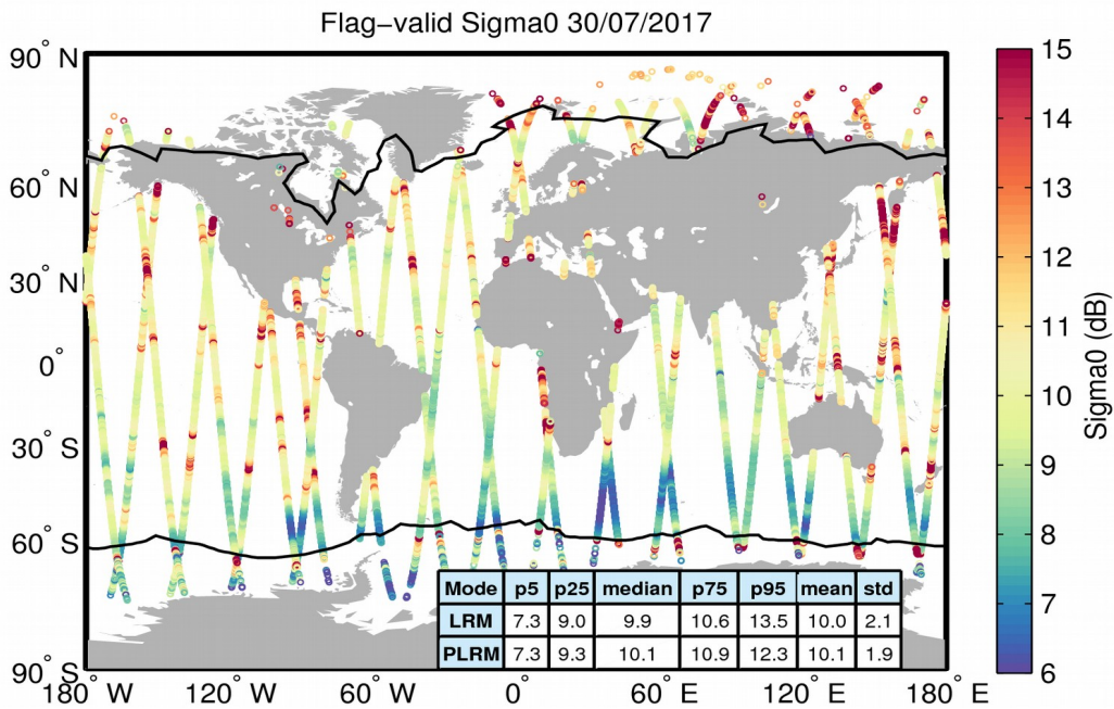
Figure 23. Geographical distribution of flag-valid sigma0 data over oceans and lakes for 30/07/2017. The statistical values shown in the table refer to the sigma0 in dB and are calculated separately for LRM and PLRM regions. Measurements taken over polar polygons have been excluded from the computation of the statistical values. The black lines mark the outer limit of the Arctic and Antarctic polar polygons.
