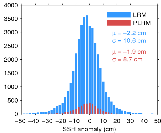
Figure 11. Histogram of science-valid SSH anomaly over oceans and lakes for LRM (blue) and PLRM (red) for 30/07/2017. The mean ( \mu ) and standard deviation ( \sigma ) are also shown. Note that values outside [-50 50] cm are excluded from the histogram for the sake of readability but not from the computation of \mu and \sigma .
