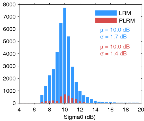
Figure 28. Histogram of science-valid sigma0 over oceans and lakes for LRM (blue) and PLRM (red) for 30/07/2017. The mean ( \mu ) and standard deviation ( \sigma ) are also shown. Note that values outside [4 20] dB are excluded from the histogram for the sake of readability but not from the computation of \mu and \sigma .
