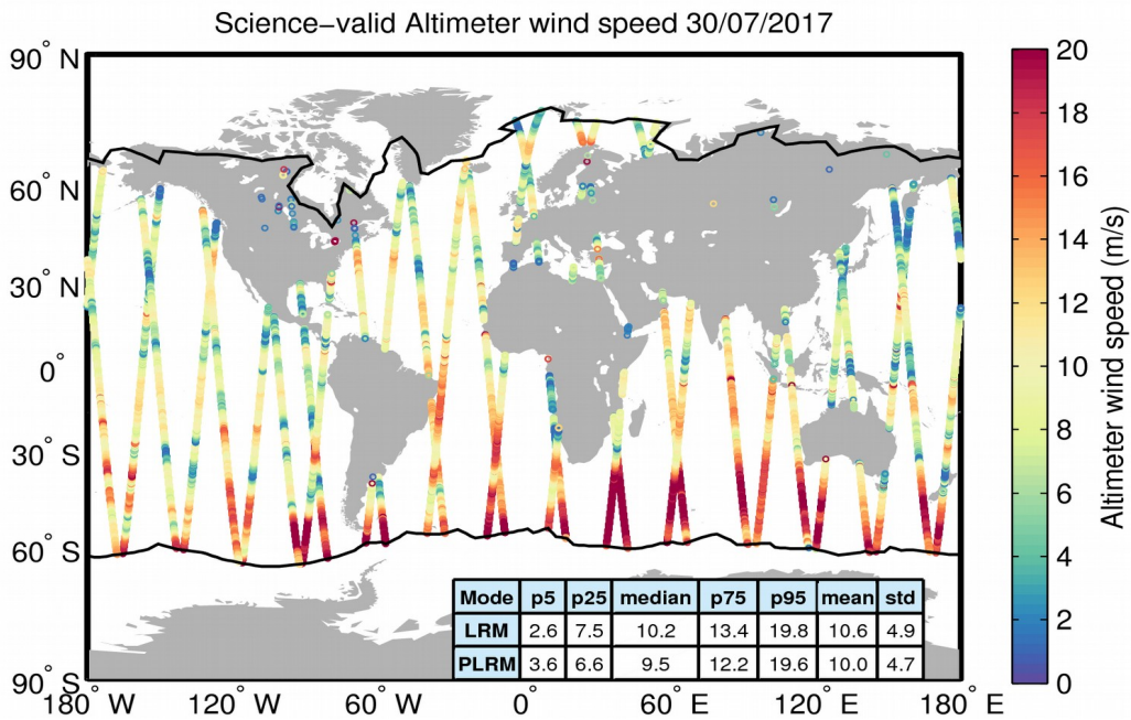
Figure 34. Geographical distribution of science-valid wind data over oceans and lakes for 30/07/2017. The statistical values shown in the table refer to the wind in m/s and are calculated separately for LRM and PLRM regions. The black lines mark the outer limit of the Arctic and Antarctic polar polygons. Gray circles denote records that have been rejected based on the editing criteria described in Table 5.
