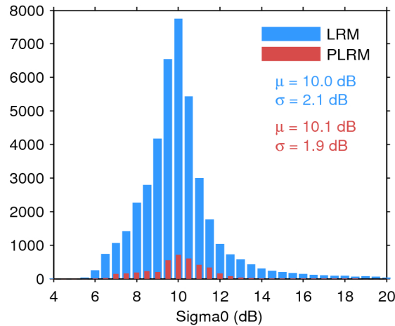
Figure 25. Histogram of flag-valid sigma0 over oceans and lakes for LRM (blue) and PLRM (red) for 30/07/2017. The mean ( \mu ) and standard deviation ( \sigma ) are also shown. Note that values outside [4 20] dB are excluded from the histogram for the sake of readability but not from the computation of \mu and \sigma .
