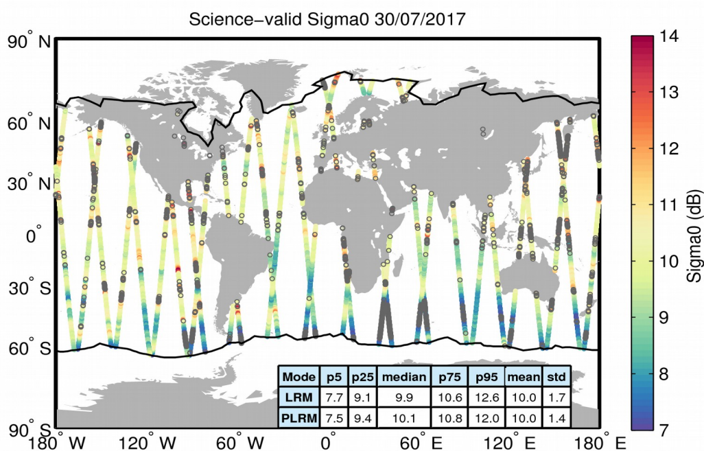
Figure 27. Geographical distribution of science-valid sigma0 data over oceans and lakes for 30/07/2017. The statistical values shown in the table refer to the sigma0 in dB and are calculated separately for LRM and PLRM regions. The black lines mark the outer limit of the Arctic and Antarctic polar polygons. Gray circles denote records that have been rejected based on the editing criteria described in Table 4.
