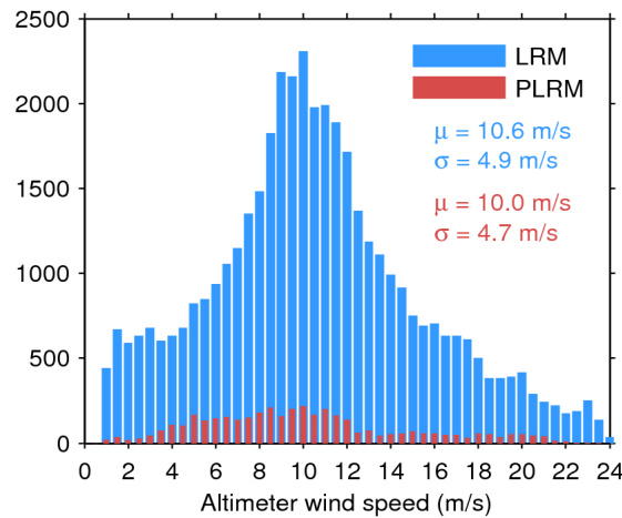
Figure 33. Histogram of flag-valid wind over oceans and lakes for LRM (blue) and PLRM (red) for 30/07/2017. The mean ( \mu ) and standard deviation ( \sigma ) are also shown. Note that values larger than 24 m/s are excluded from the histogram for the sake of readability but not from the computation of \mu and \sigma .
