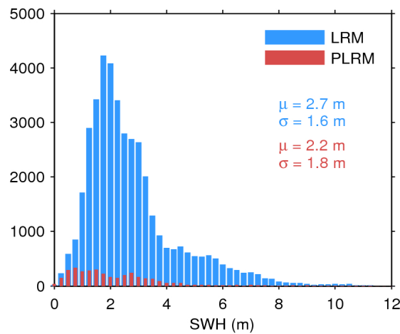
Figure 20. Histogram of science-valid SWH over oceans and lakes for LRM (blue) and PLRM (red) for 30/07/2017. The mean ( \mu ) and standard deviation ( \sigma ) are also shown. Note that values larger than 12 m are excluded from the histogram for the sake of readability but not from the computation of \mu and \sigma .
