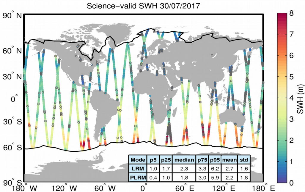
Figure 19. Geographical distribution of science-valid SWH data over oceans and lakes for 30/07/2017. The statistical values shown in the table refer to the SWH in m and are calculated separately for LRM and PLRM regions. The black lines mark the outer limit of the Arctic and Antarctic polar polygons. Gray circles denote records that have been rejected based on the editing criteria described in Table 3.
