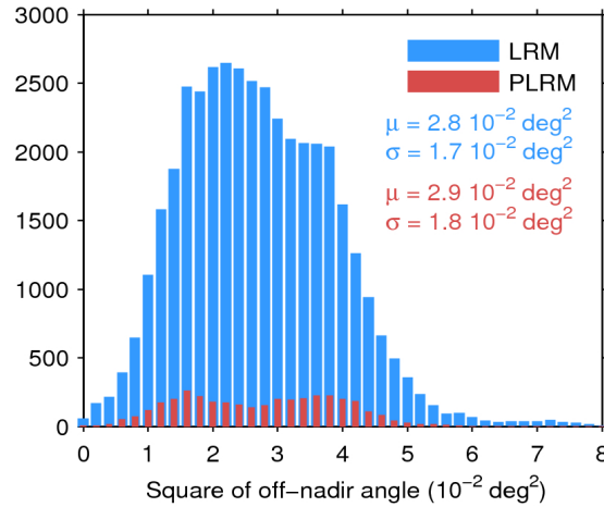
Figure 39. Histogram of flag-valid mispointing over oceans and lakes for LRM (blue) and PLRM (red) for 30/07/2017. Only positive values have been considered. The mean ( \mu ) and standard deviation ( \sigma ) are also shown. Note that values larger than 8 \cdot 10^{-2} \text{ deg}^2 are excluded from the histogram for the sake of readability but not from the computation of \mu and \sigma .
