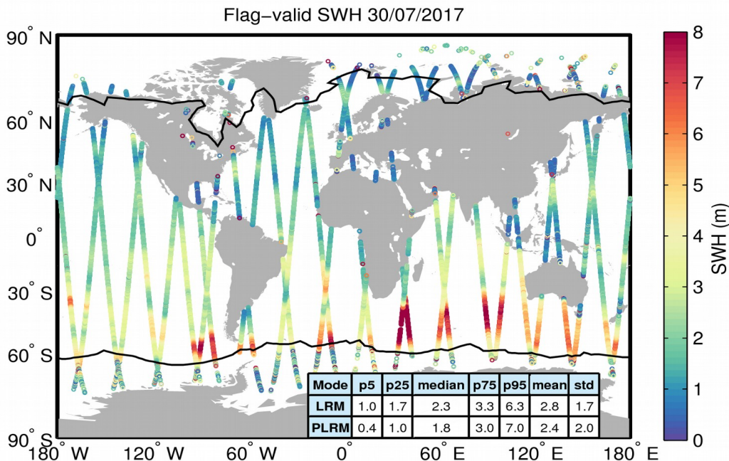
Figure 15. Geographical distribution of flag-valid SWH data over oceans and lakes for 30/07/2017. The statistical values shown in the table refer to the SWH in m and are calculated separately for LRM and PLRM regions. Measurements taken over polar polygons have been excluded from the computation of the statistical values. The black lines mark the outer limit of the Arctic and Antarctic polar polygons.
