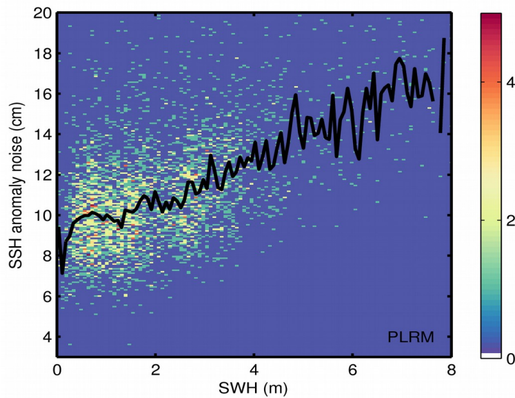
Figure 9. 2D histogram showing flag-valid SSH anomaly noise as a function of SWH for LRM (top) and PLRM (bottom) for 30/07/2017. The black line denotes the median SSH anomaly noise as a function of SWH.
