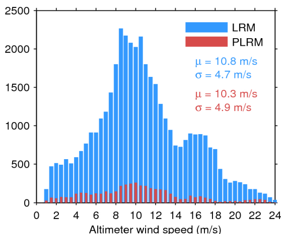
Figure 33. Histogram of flag-valid wind over oceans and lakes for LRM (blue) and PLRM (red) for 29/07/2017. The mean ( \mu ) and standard deviation ( \sigma ) are also shown. Note that values larger than 24 m/s are excluded from the histogram for the sake of readability but not from the computation of \mu and \sigma .
