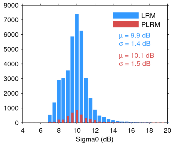
Figure 28. Histogram of science-valid sigma0 over oceans and lakes for LRM (blue) and PLRM (red) for 29/07/2017. The mean ( \mu ) and standard deviation ( \sigma ) are also shown. Note that values outside [4 20] dB are excluded from the histogram for the sake of readability but not from the computation of \mu and \sigma .
