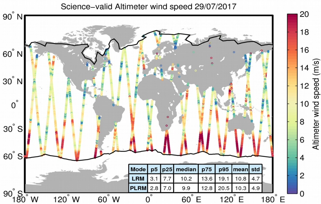
Figure 34. Geographical distribution of science-valid wind data over oceans and lakes for 29/07/2017. The statistical values shown in the table refer to the wind in m/s and are calculated separately for LRM and PLRM regions. The black lines mark the outer limit of the Arctic and Antarctic polar polygons. Gray circles denote records that have been rejected based on the editing criteria described in Table 5.
