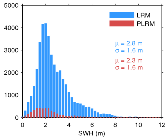
Figure 17. Histogram of flag-valid SWH over oceans and lakes for LRM (blue) and PLRM (red) for 29/07/2017. The mean ( \mu ) and standard deviation ( \sigma ) are also shown. Note that values larger than 12 m are excluded from the histogram for the sake of readability but not from the computation of \mu and \sigma .
