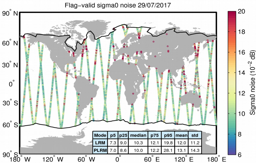
Figure 26. Geographical distribution of flag-valid 20-Hz sigma0 measurement noise over oceans and lakes for 29/07/2017. The statistical values shown in the table refer to the sigma0 noise and are calculated separately for LRM and PLRM regions. Measurements taken over polar polygons have been excluded from the computation of the statistical values. The black lines mark the outer limit of the Arctic and Antarctic polar polygons.
