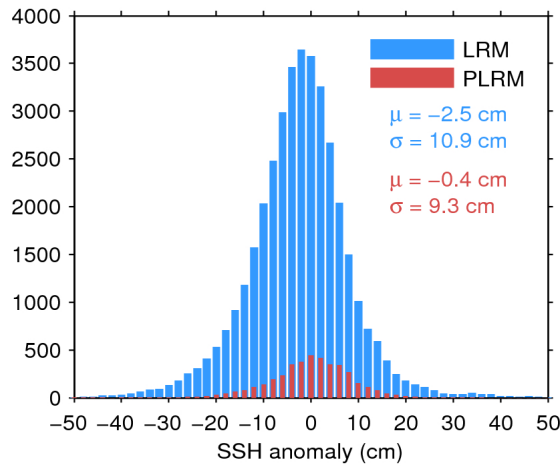
Figure 11. Histogram of science-valid SSH anomaly over oceans and lakes for LRM (blue) and PLRM (red) for 29/07/2017. The mean ( \mu ) and standard deviation ( \sigma ) are also shown. Note that values outside [-50\ 50] cm are excluded from the histogram for the sake of readability but not from the computation of \mu and \sigma .
