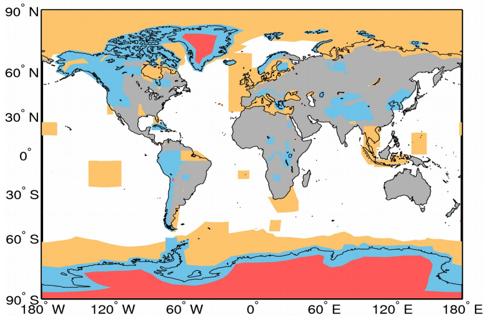
Figure A1. Extent of the regions defining the geographical mode mask for 29/07/2017. The regions where SAR, and SARIn are operated are denoted by the orange and blue polygons, respectively. LRM is operated over areas of the continental ice sheets (red polygons) and over oceans and land not covered by other modes.
