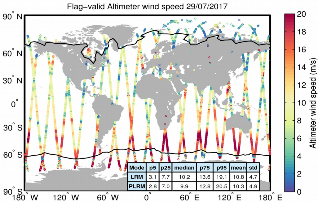
Figure 31. Geographical distribution of flag-valid wind data over oceans and lakes for 29/07/2017. The statistical values shown in the table refer to the wind in m/s and are calculated separately for LRM and PLRM regions. Measurements taken over polar polygons have been excluded from the computation of the statistical values. The black lines mark the outer limit of the Arctic and Antarctic polar polygons.
