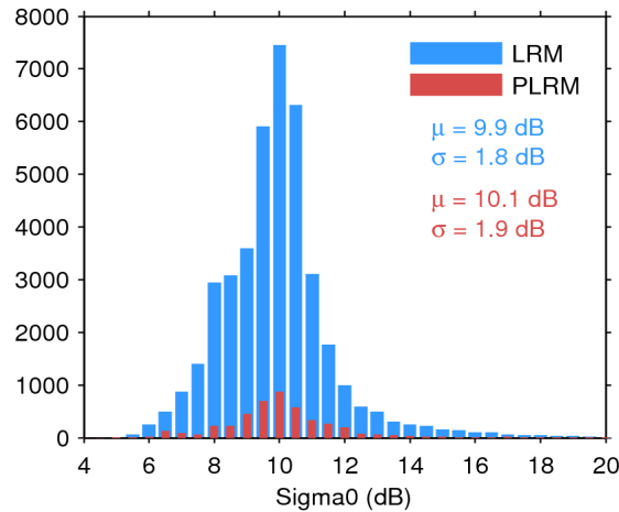
Figure 25. Histogram of flag-valid sigma0 over oceans and lakes for LRM (blue) and PLRM (red) for 29/07/2017. The mean ( \mu ) and standard deviation ( \sigma ) are also shown. Note that values outside [4 20] dB are excluded from the histogram for the sake of readability but not from the computation of \mu and \sigma .
