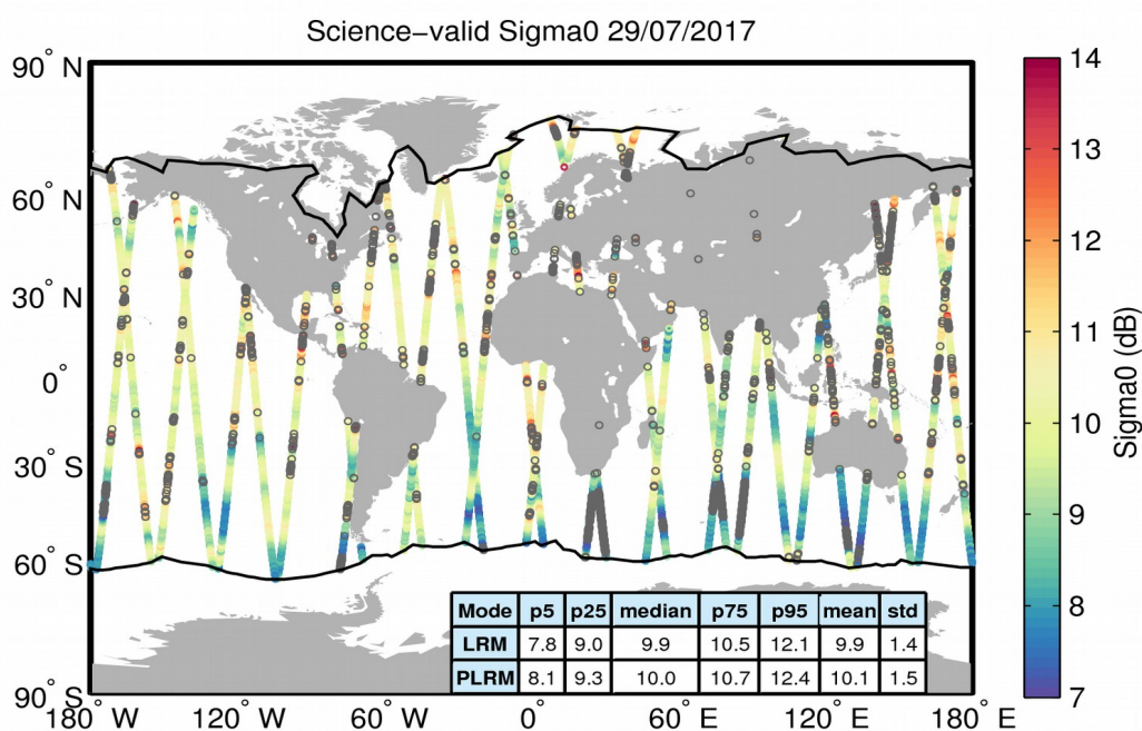
Figure 27. Geographical distribution of science-valid sigma0 data over oceans and lakes for 29/07/2017. The statistical values shown in the table refer to the sigma0 in dB and are calculated separately for LRM and PLRM regions. The black lines mark the outer limit of the Arctic and Antarctic polar polygons. Gray circles denote records that have been rejected based on the editing criteria described in Table 4.
