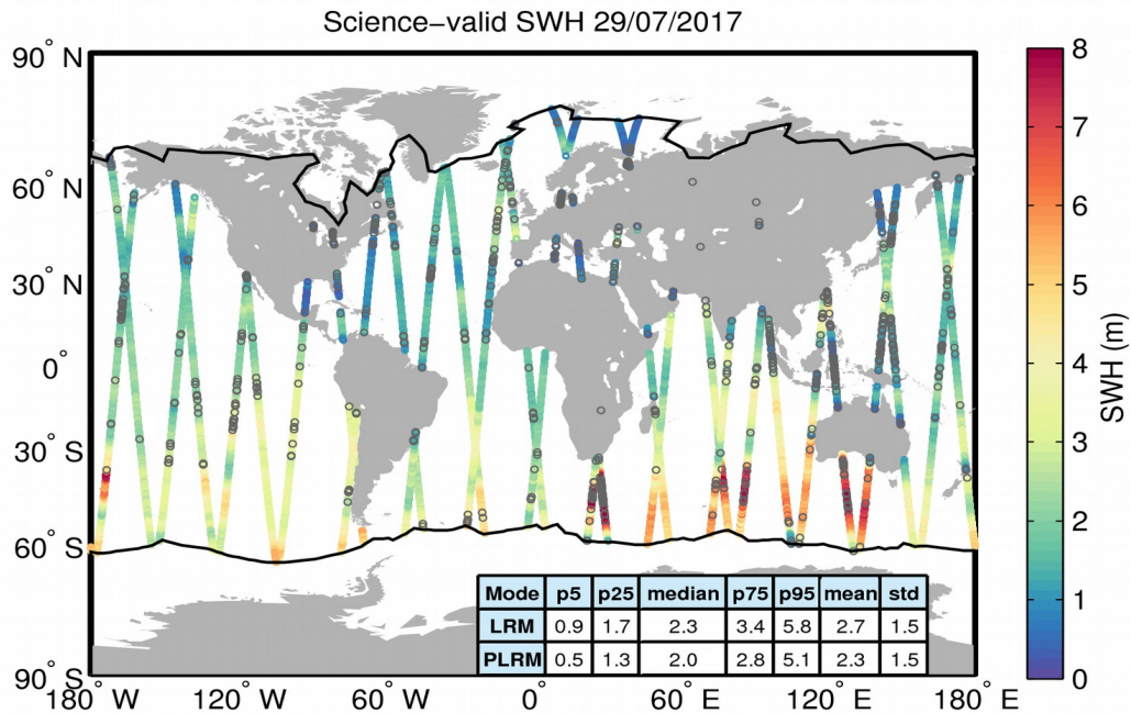
Figure 19. Geographical distribution of science-valid SWH data over oceans and lakes for 29/07/2017. The statistical values shown in the table refer to the SWH in m and are calculated separately for LRM and PLRM regions. The black lines mark the outer limit of the Arctic and Antarctic polar polygons. Gray circles denote records that have been rejected based on the editing criteria described in Table 3.
