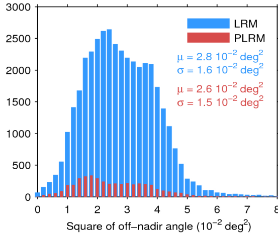
Figure 39. Histogram of flag-valid mispointing over oceans and lakes for LRM (blue) and PLRM (red) for 29/07/2017. Only positive values have been considered. The mean ( \mu ) and standard deviation ( \sigma ) are also shown. Note that values larger than 8 \cdot 10^{-2} \text{ deg}^2 are excluded from the histogram for the sake of readability but not from the computation of \mu and \sigma .
