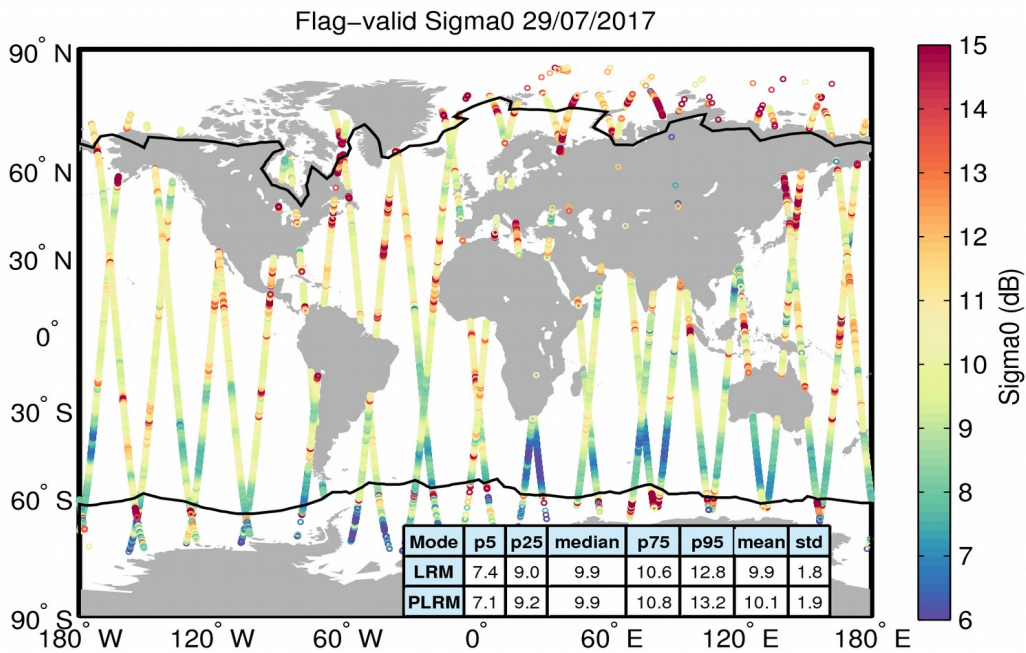
Figure 23. Geographical distribution of flag-valid sigma0 data over oceans and lakes for 29/07/2017. The statistical values shown in the table refer to the sigma0 in dB and are calculated separately for LRM and PLRM regions. Measurements taken over polar polygons have been excluded from the computation of the statistical values. The black lines mark the outer limit of the Arctic and Antarctic polar polygons.
