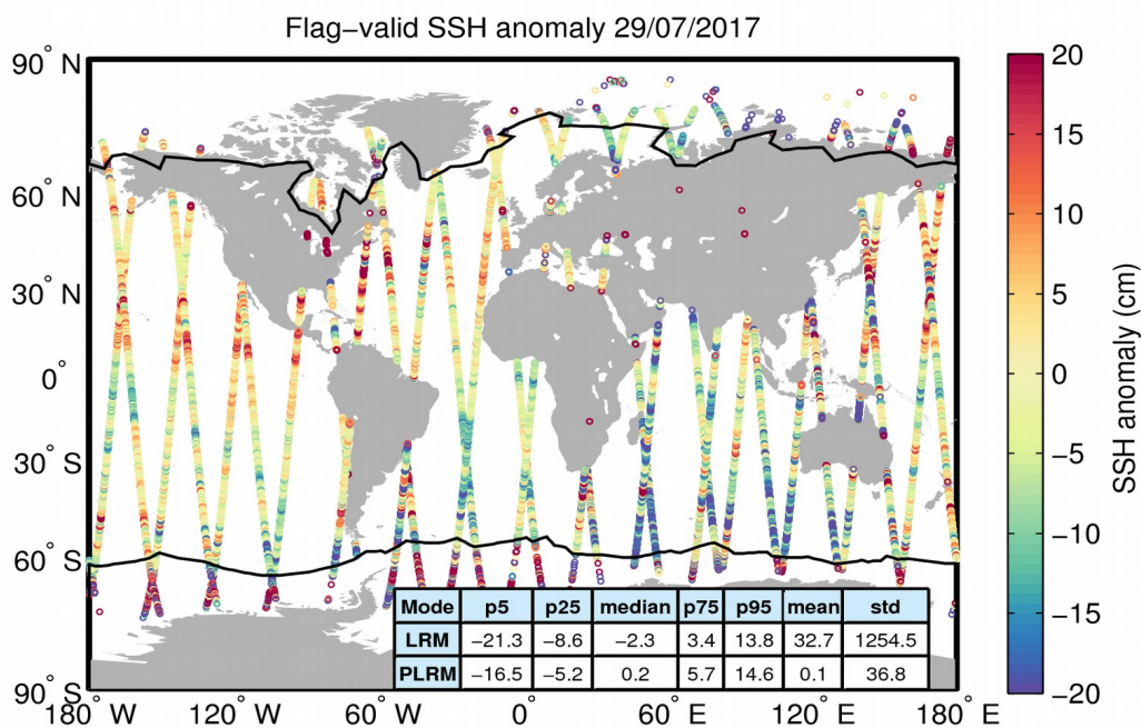
Figure 5. Geographical distribution of flag-valid 1-Hz SSH anomaly data over oceans and lakes for 29/07/2017. The statistical values shown in the table refer to the SSH anomaly in cm and are calculated separately for LRM and PLRM regions. Measurements taken over polar polygons have been excluded from the computation of the statistical values. The black lines mark the outer limit of the Arctic and Antarctic polar polygons.
