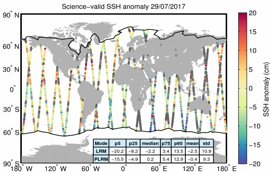
Figure 10. Geographical distribution of science-valid SSH anomaly data over oceans and lakes for 29/07/2017. The statistical values shown in the table refer to the SSH anomaly in cm and are calculated separately for LRM and PLRM regions. The black lines mark the outer limit of the Arctic and Antarctic polar polygons. Gray circles denote records that have been rejected based on the editing criteria described in Table 2.
