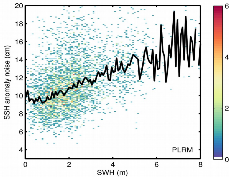
Figure 9. 2D histogram showing flag-valid SSH anomaly noise as a function of SWH for LRM (top) and PLRM (bottom) for 29/07/2017. The black line denotes the median SSH anomaly noise as a function of SWH.
