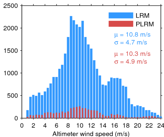
Figure 35. Histogram of science-valid wind over oceans and lakes for LRM (blue) and PLRM (red) for 29/07/2017. The mean ( \mu ) and standard deviation ( \sigma ) are also shown. Note that values larger than 24 m/s are excluded from the histogram for the sake of readability but not from the computation of \mu and \sigma .
