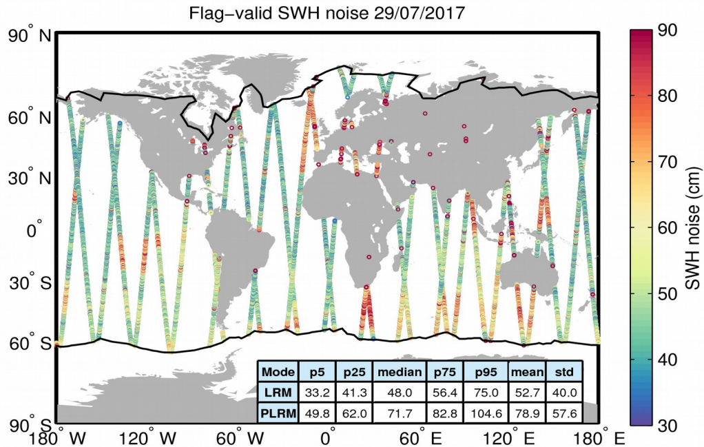
Figure 18. Geographical distribution of flag-valid 20-Hz SWH measurement noise over oceans and lakes for 29/07/2017. The statistical values shown in the table refer to the SWH noise and are calculated separately for LRM and PLRM regions. Measurements taken over polar polygons have been excluded from the computation of the statistical values. The black lines mark the outer limit of the Arctic and Antarctic polar polygons.
