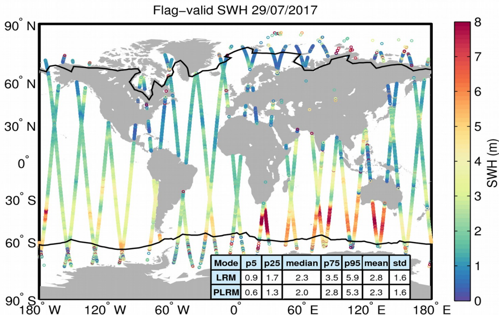
Figure 15. Geographical distribution of flag-valid SWH data over oceans and lakes for 29/07/2017. The statistical values shown in the table refer to the SWH in m and are calculated separately for LRM and PLRM regions. Measurements taken over polar polygons have been excluded from the computation of the statistical values. The black lines mark the outer limit of the Arctic and Antarctic polar polygons.
