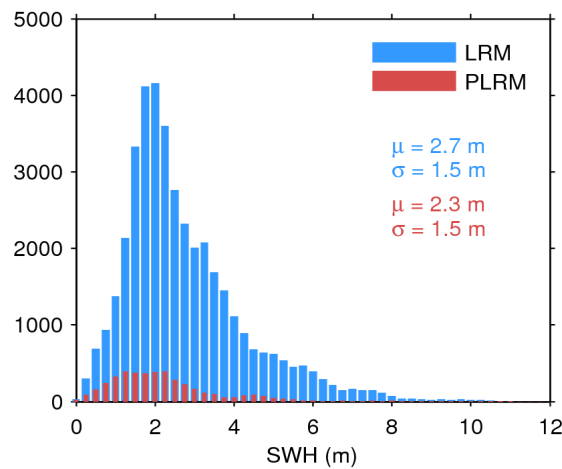
Figure 20. Histogram of science-valid SWH over oceans and lakes for LRM (blue) and PLRM (red) for 29/07/2017. The mean ( \mu ) and standard deviation ( \sigma ) are also shown. Note that values larger than 12 m are excluded from the histogram for the sake of readability but not from the computation of \mu and \sigma .
