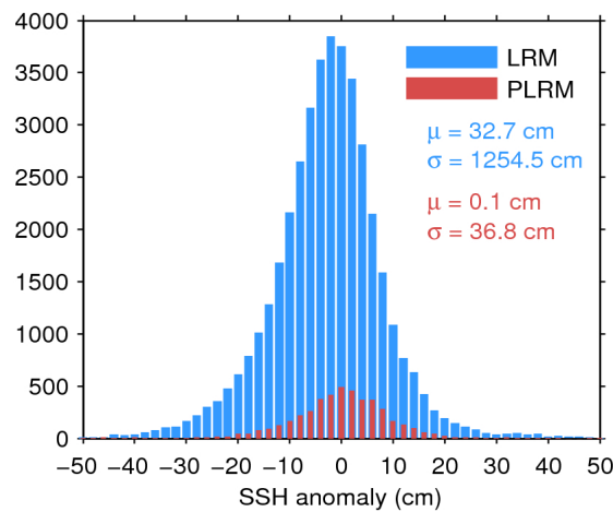
Figure 7. Histogram of flag-valid SSH anomaly over oceans and lakes for LRM (blue) and PLRM (red) for 29/07/2017. The mean ( \mu ) and standard deviation ( \sigma ) are also shown. Note that values outside [-50 50] cm are excluded from the histogram for the sake of readability but not from the computation of \mu and \sigma .
