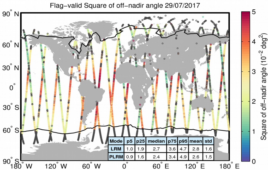
Figure 37. Geographical distribution of flag-valid mispointing data over oceans and lakes for 29/07/2017. The statistical values shown in the table refer to the mispointing in 10^{-2} deg 2 and are calculated separately for LRM and PLRM regions. Measurements taken over polar polygons have been excluded from the computation of the statistical values. The black lines mark the outer limit of the Arctic and Antarctic polar polygons. Gray circles denote negative values.
