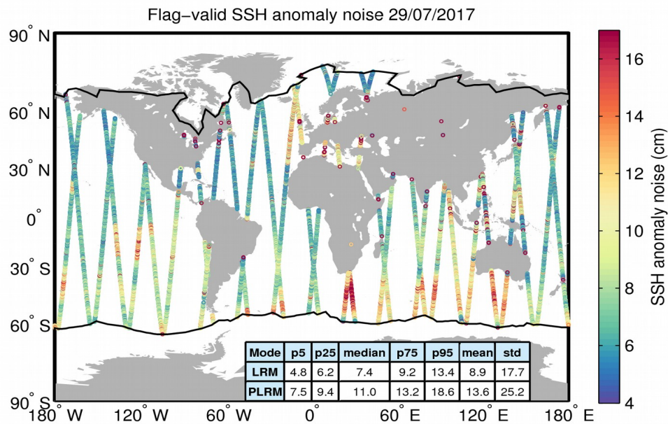
Figure 8. Geographical distribution of flag-valid 20-Hz SSH anomaly measurement noise over oceans and lakes for 29/07/2017. The statistical values shown in the table refer to the SSH anomaly noise and are calculated separately for LRM and PLRM regions. Measurements taken over polar polygons have been excluded from the computation of the statistical values. The black lines mark the outer limit of the Arctic and Antarctic polar polygons.
