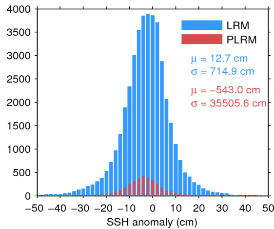
Figure 7. Histogram of flag-valid SSH anomaly over oceans and lakes for LRM (blue) and PLRM (red) for 26/07/2017. The mean ( \mu ) and standard deviation ( \sigma ) are also shown. Note that values outside [-50 \ 50] cm are excluded from the histogram for the sake of readability but not from the computation of \mu and \sigma .
