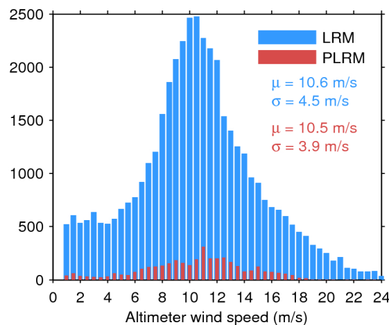
Figure 35. Histogram of science-valid wind over oceans and lakes for LRM (blue) and PLRM (red) for 26/07/2017. The mean ( \mu ) and standard deviation ( \sigma ) are also shown. Note that values larger than 24 m/s are excluded from the histogram for the sake of readability but not from the computation of \mu and \sigma .
