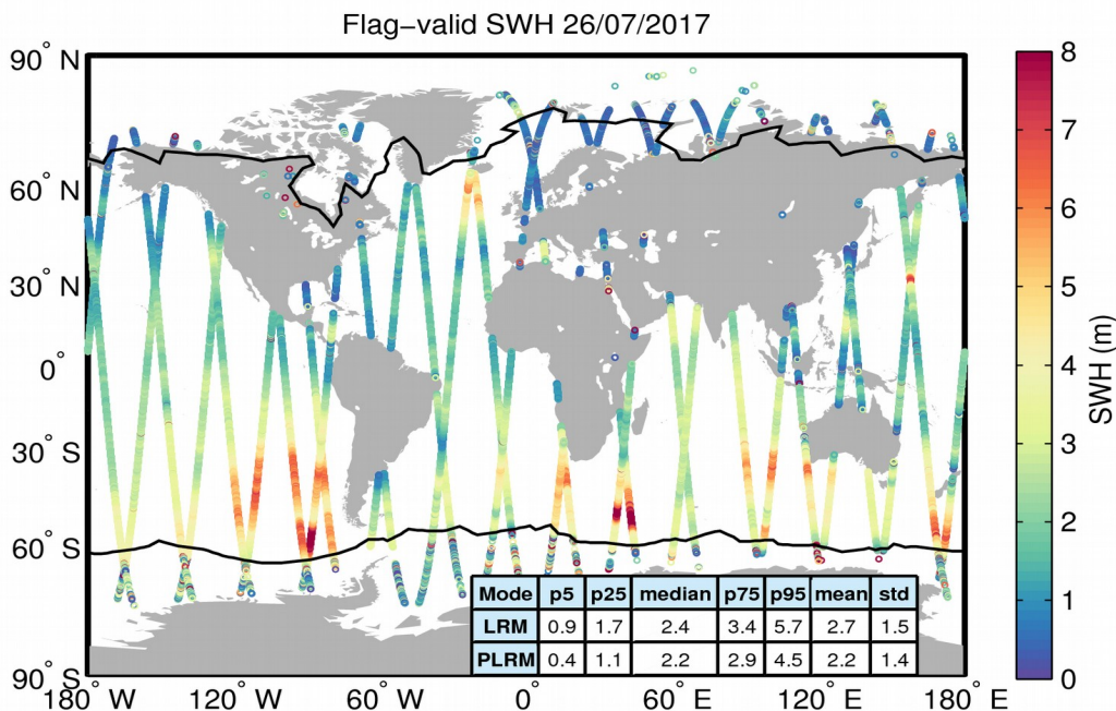
Figure 15. Geographical distribution of flag-valid SWH data over oceans and lakes for 26/07/2017. The statistical values shown in the table refer to the SWH in m and are calculated separately for LRM and PLRM regions. Measurements taken over polar polygons have been excluded from the computation of the statistical values. The black lines mark the outer limit of the Arctic and Antarctic polar polygons.
