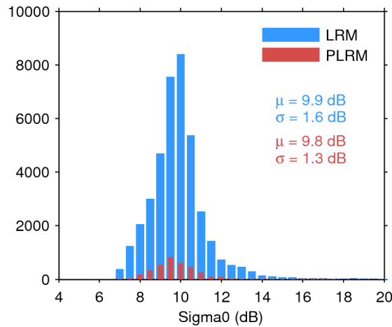
Figure 28. Histogram of science-valid sigma0 over oceans and lakes for LRM (blue) and PLRM (red) for 26/07/2017. The mean ( \mu ) and standard deviation ( \sigma ) are also shown. Note that values outside [4 20] dB are excluded from the histogram for the sake of readability but not from the computation of \mu and \sigma .
