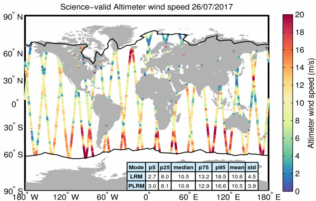
Figure 34. Geographical distribution of science-valid wind data over oceans and lakes for 26/07/2017. The statistical values shown in the table refer to the wind in m/s and are calculated separately for LRM and PLRM regions. The black lines mark the outer limit of the Arctic and Antarctic polar polygons. Gray circles denote records that have been rejected based on the editing criteria described in Table 5.
