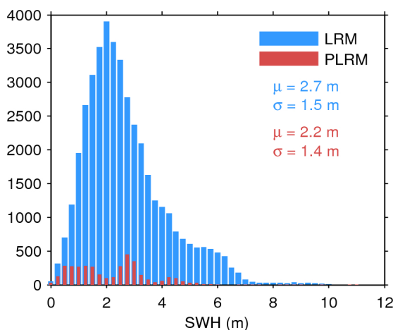
Figure 17. Histogram of flag-valid SWH over oceans and lakes for LRM (blue) and PLRM (red) for 26/07/2017. The mean ( \mu ) and standard deviation ( \sigma ) are also shown. Note that values larger than 12 m are excluded from the histogram for the sake of readability but not from the computation of \mu and \sigma .
