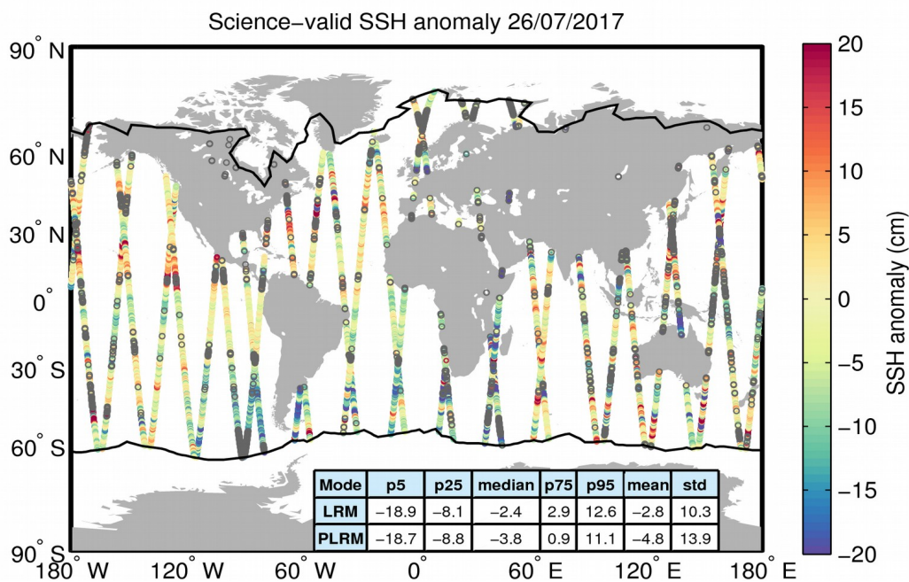
Figure 10. Geographical distribution of science-valid SSH anomaly data over oceans and lakes for 26/07/2017. The statistical values shown in the table refer to the SSH anomaly in cm and are calculated separately for LRM and PLRM regions. The black lines mark the outer limit of the Arctic and Antarctic polar polygons. Gray circles denote records that have been rejected based on the editing criteria described in Table 2.
