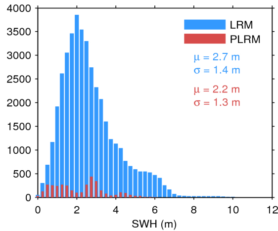
Figure 20. Histogram of science-valid SWH over oceans and lakes for LRM (blue) and PLRM (red) for 26/07/2017. The mean ( \mu ) and standard deviation ( \sigma ) are also shown. Note that values larger than 12 m are excluded from the histogram for the sake of readability but not from the computation of \mu and \sigma .
