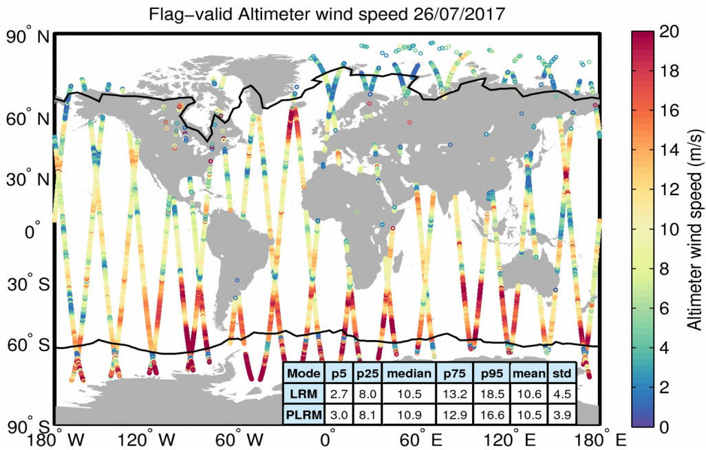
Figure 31. Geographical distribution of flag-valid wind data over oceans and lakes for 26/07/2017. The statistical values shown in the table refer to the wind in m/s and are calculated separately for LRM and PLRM regions. Measurements taken over polar polygons have been excluded from the computation of the statistical values. The black lines mark the outer limit of the Arctic and Antarctic polar polygons.
