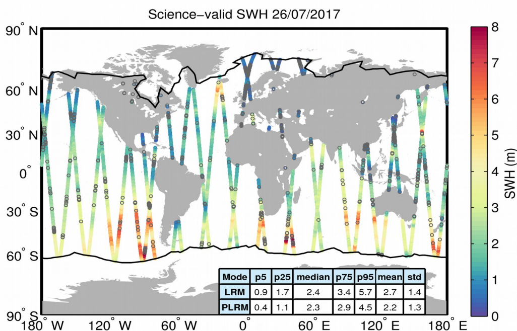
Figure 19. Geographical distribution of science-valid SWH data over oceans and lakes for 26/07/2017. The statistical values shown in the table refer to the SWH in m and are calculated separately for LRM and PLRM regions. The black lines mark the outer limit of the Arctic and Antarctic polar polygons. Gray circles denote records that have been rejected based on the editing criteria described in Table 3.
