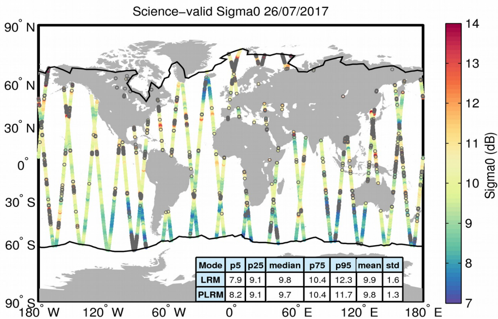
Figure 27. Geographical distribution of science-valid sigma0 data over oceans and lakes for 26/07/2017. The statistical values shown in the table refer to the sigma0 in dB and are calculated separately for LRM and PLRM regions. The black lines mark the outer limit of the Arctic and Antarctic polar polygons. Gray circles denote records that have been rejected based on the editing criteria described in Table 4.
