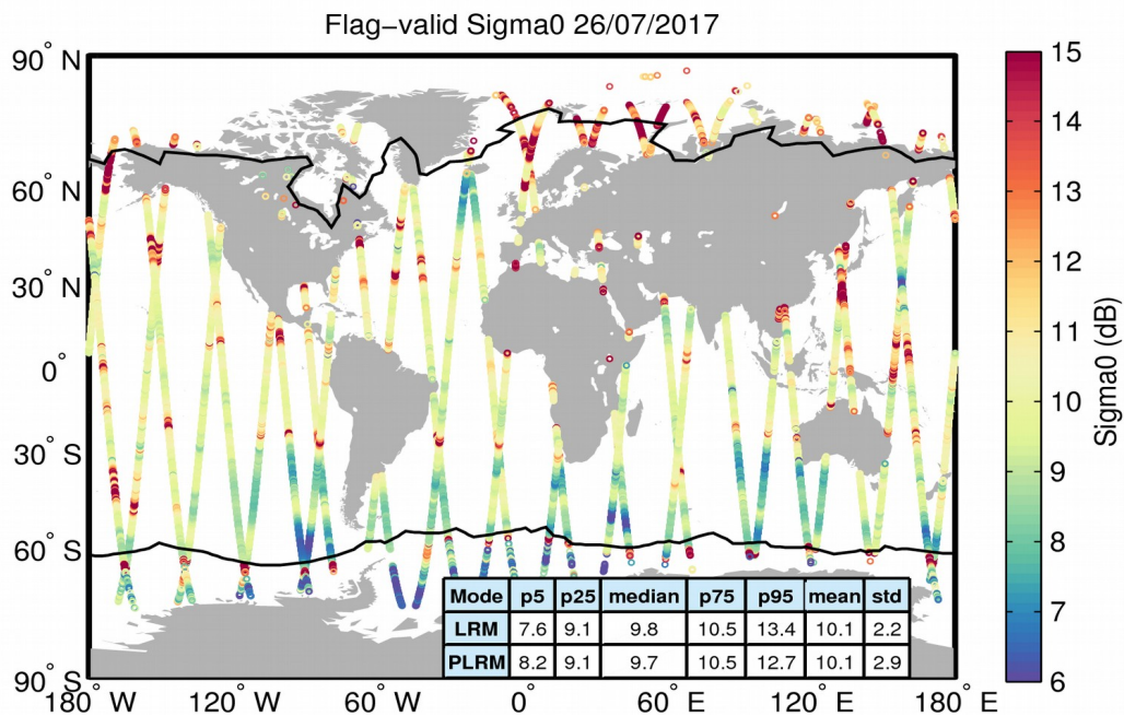
Figure 23. Geographical distribution of flag-valid sigma0 data over oceans and lakes for 26/07/2017. The statistical values shown in the table refer to the sigma0 in dB and are calculated separately for LRM and PLRM regions. Measurements taken over polar polygons have been excluded from the computation of the statistical values. The black lines mark the outer limit of the Arctic and Antarctic polar polygons.
