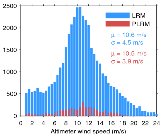
Figure 33. Histogram of flag-valid wind over oceans and lakes for LRM (blue) and PLRM (red) for 26/07/2017. The mean ( \mu ) and standard deviation ( \sigma ) are also shown. Note that values larger than 24 m/s are excluded from the histogram for the sake of readability but not from the computation of \mu and \sigma .
