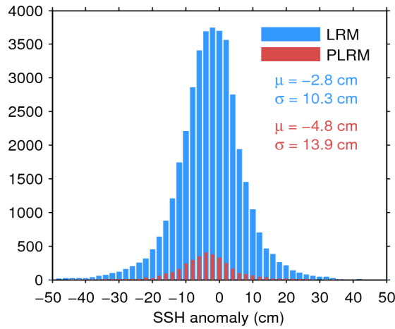
Figure 11. Histogram of science-valid SSH anomaly over oceans and lakes for LRM (blue) and PLRM (red) for 26/07/2017. The mean ( \mu ) and standard deviation ( \sigma ) are also shown. Note that values outside [-50\ 50] cm are excluded from the histogram for the sake of readability but not from the computation of \mu and \sigma .
