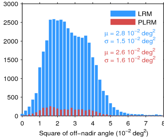
Figure 39. Histogram of flag-valid mispointing over oceans and lakes for LRM (blue) and PLRM (red) for 26/07/2017. Only positive values have been considered. The mean ( \mu ) and standard deviation ( \sigma ) are also shown. Note that values larger than 8 \cdot 10^{-2} \text{ deg}^2 are excluded from the histogram for the sake of readability but not from the computation of \mu and \sigma .
