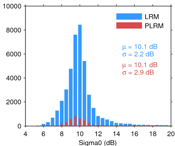
Figure 25. Histogram of flag-valid sigma0 over oceans and lakes for LRM (blue) and PLRM (red) for 26/07/2017. The mean ( \mu ) and standard deviation ( \sigma ) are also shown. Note that values outside [4 20] dB are excluded from the histogram for the sake of readability but not from the computation of \mu and \sigma .
