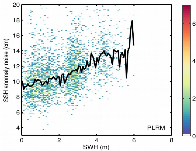
Figure 9. 2D histogram showing flag-valid SSH anomaly noise as a function of SWH for LRM (top) and PLRM (bottom) for 26/07/2017. The black line denotes the median SSH anomaly noise as a function of SWH.
