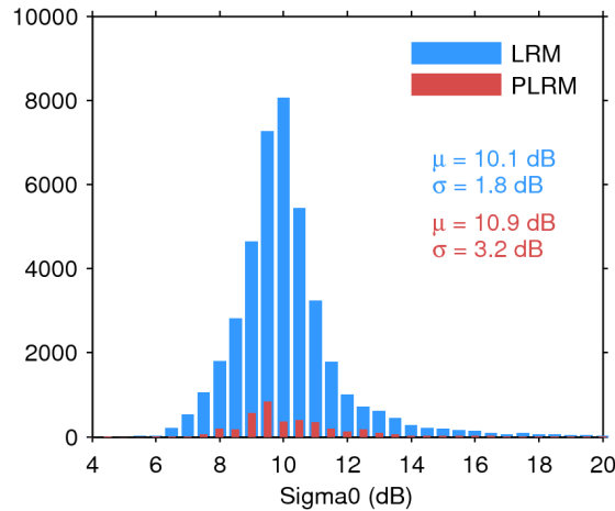
Figure 25. Histogram of flag-valid sigma0 over oceans and lakes for LRM (blue) and PLRM (red) for 25/07/2017. The mean ( \mu ) and standard deviation ( \sigma ) are also shown. Note that values outside [4 20] dB are excluded from the histogram for the sake of readability but not from the computation of \mu and \sigma .
