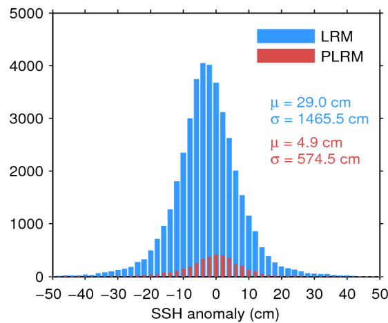
Figure 7. Histogram of flag-valid SSH anomaly over oceans and lakes for LRM (blue) and PLRM (red) for 25/07/2017. The mean ( \mu ) and standard deviation ( \sigma ) are also shown. Note that values outside [-50 50] cm are excluded from the histogram for the sake of readability but not from the computation of \mu and \sigma .
