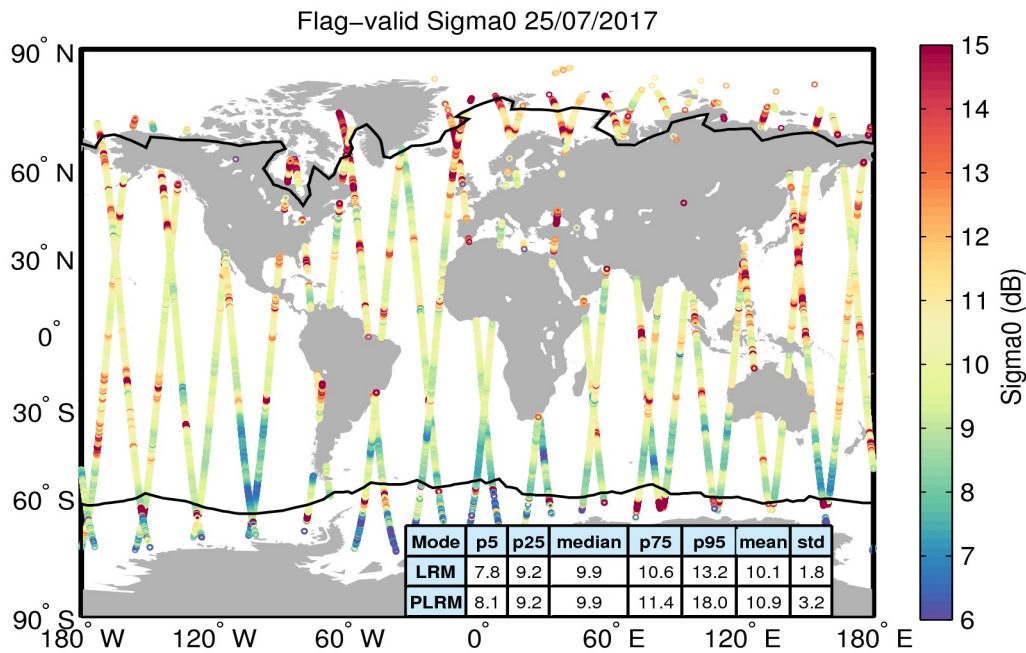
Figure 23. Geographical distribution of flag-valid sigma0 data over oceans and lakes for 25/07/2017. The statistical values shown in the table refer to the sigma0 in dB and are calculated separately for LRM and PLRM regions. Measurements taken over polar polygons have been excluded from the computation of the statistical values. The black lines mark the outer limit of the Arctic and Antarctic polar polygons.
