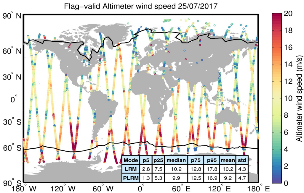
Figure 31. Geographical distribution of flag-valid wind data over oceans and lakes for 25/07/2017. The statistical values shown in the table refer to the wind in m/s and are calculated separately for LRM and PLRM regions. Measurements taken over polar polygons have been excluded from the computation of the statistical values. The black lines mark the outer limit of the Arctic and Antarctic polar polygons.
