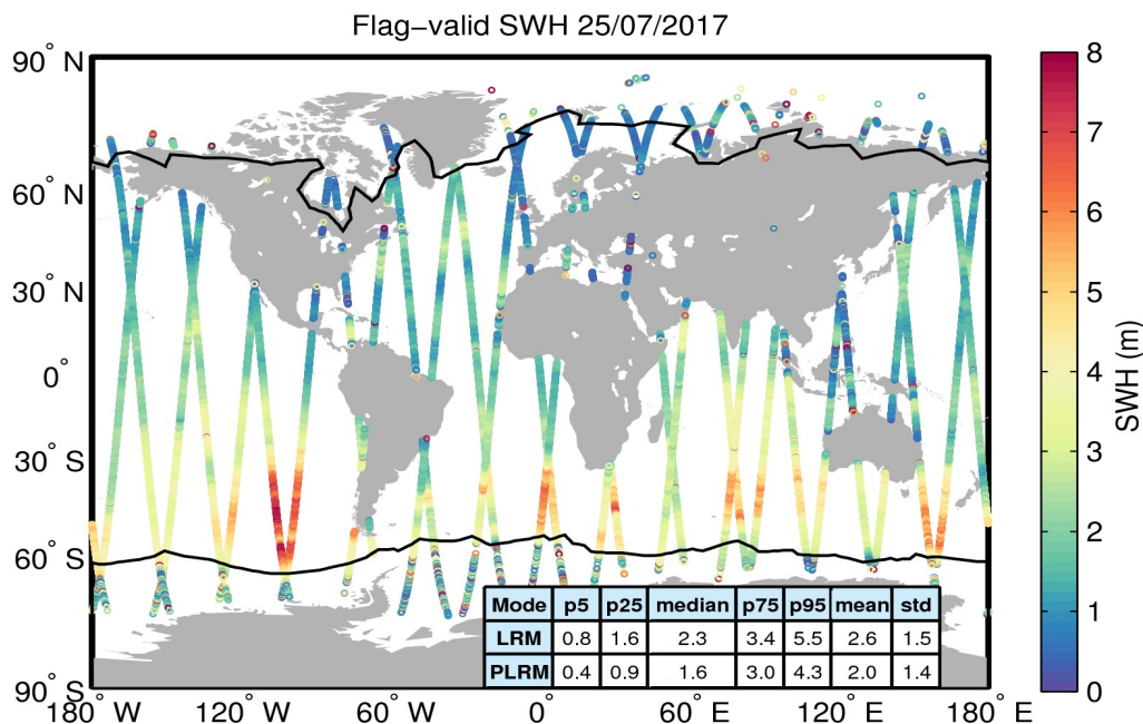
Figure 15. Geographical distribution of flag-valid SWH data over oceans and lakes for 25/07/2017. The statistical values shown in the table refer to the SWH in m and are calculated separately for LRM and PLRM regions. Measurements taken over polar polygons have been excluded from the computation of the statistical values. The black lines mark the outer limit of the Arctic and Antarctic polar polygons.
