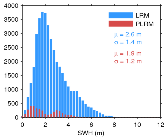
Figure 20. Histogram of science-valid SWH over oceans and lakes for LRM (blue) and PLRM (red) for 25/07/2017. The mean ( \mu ) and standard deviation ( \sigma ) are also shown. Note that values larger than 12 m are excluded from the histogram for the sake of readability but not from the computation of \mu and \sigma .
