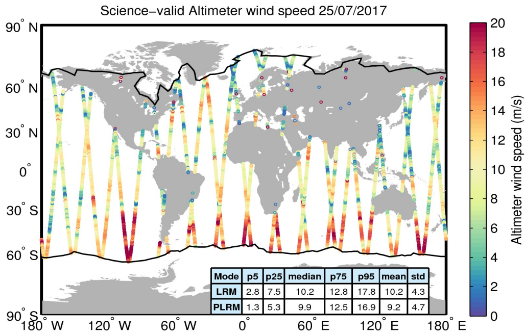
Figure 34. Geographical distribution of science-valid wind data over oceans and lakes for 25/07/2017. The statistical values shown in the table refer to the wind in m/s and are calculated separately for LRM and PLRM regions. The black lines mark the outer limit of the Arctic and Antarctic polar polygons. Gray circles denote records that have been rejected based on the editing criteria described in Table 5.
