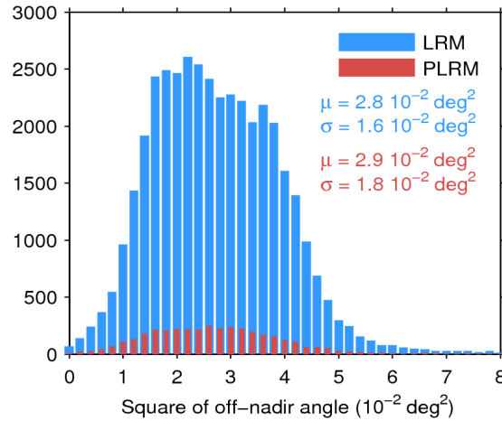
Figure 39. Histogram of flag-valid mispointing over oceans and lakes for LRM (blue) and PLRM (red) for 25/07/2017. Only positive values have been considered. The mean ( \mu ) and standard deviation ( \sigma ) are also shown. Note that values larger than 8 \cdot 10^{-2} \text{ deg}^2 are excluded from the histogram for the sake of readability but not from the computation of \mu and \sigma .
