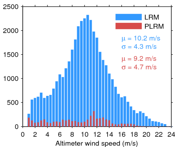
Figure 33. Histogram of flag-valid wind over oceans and lakes for LRM (blue) and PLRM (red) for 25/07/2017. The mean ( \mu ) and standard deviation ( \sigma ) are also shown. Note that values larger than 24 m/s are excluded from the histogram for the sake of readability but not from the computation of \mu and \sigma .
