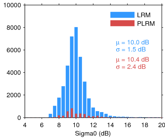
Figure 28. Histogram of science-valid sigma0 over oceans and lakes for LRM (blue) and PLRM (red) for 25/07/2017. The mean ( \mu ) and standard deviation ( \sigma ) are also shown. Note that values outside [4 20] dB are excluded from the histogram for the sake of readability but not from the computation of \mu and \sigma .
