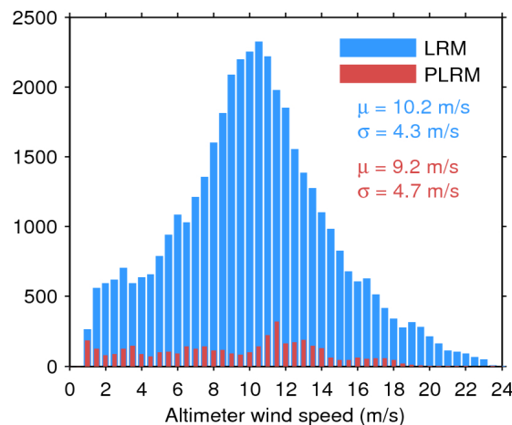
Figure 35. Histogram of science-valid wind over oceans and lakes for LRM (blue) and PLRM (red) for 25/07/2017. The mean ( \mu ) and standard deviation ( \sigma ) are also shown. Note that values larger than 24 m/s are excluded from the histogram for the sake of readability but not from the computation of \mu and \sigma .
