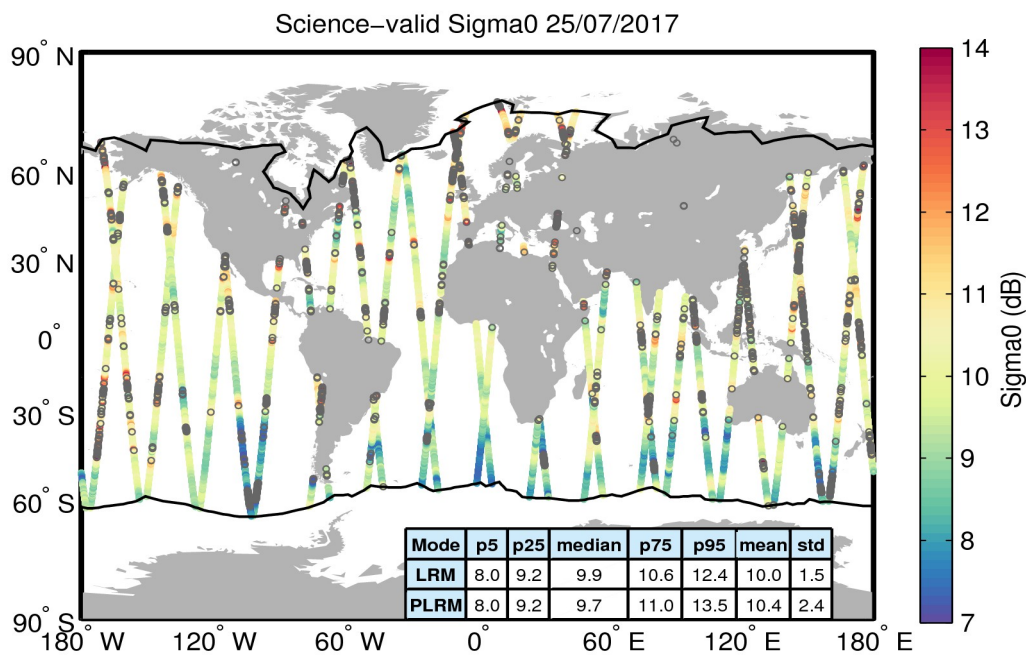
Figure 27. Geographical distribution of science-valid sigma0 data over oceans and lakes for 25/07/2017. The statistical values shown in the table refer to the sigma0 in dB and are calculated separately for LRM and PLRM regions. The black lines mark the outer limit of the Arctic and Antarctic polar polygons. Gray circles denote records that have been rejected based on the editing criteria described in Table 4.
