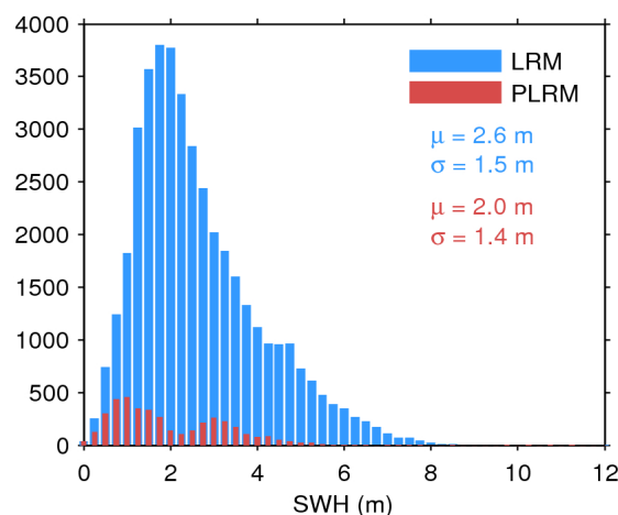
Figure 17. Histogram of flag-valid SWH over oceans and lakes for LRM (blue) and PLRM (red) for 25/07/2017. The mean ( \mu ) and standard deviation ( \sigma ) are also shown. Note that values larger than 12 m are excluded from the histogram for the sake of readability but not from the computation of \mu and \sigma .
