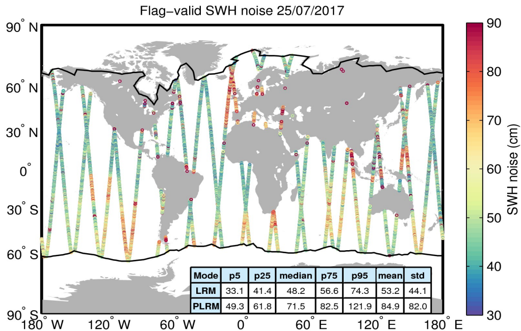
Figure 18. Geographical distribution of flag-valid 20-Hz SWH measurement noise over oceans and lakes for 25/07/2017. The statistical values shown in the table refer to the SWH noise and are calculated separately for LRM and PLRM regions. Measurements taken over polar polygons have been excluded from the computation of the statistical values. The black lines mark the outer limit of the Arctic and Antarctic polar polygons.
