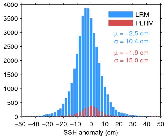
Figure 11. Histogram of science-valid SSH anomaly over oceans and lakes for LRM (blue) and PLRM (red) for 25/07/2017. The mean ( \mu ) and standard deviation ( \sigma ) are also shown. Note that values outside [-50\ 50] cm are excluded from the histogram for the sake of readability but not from the computation of \mu and \sigma .
