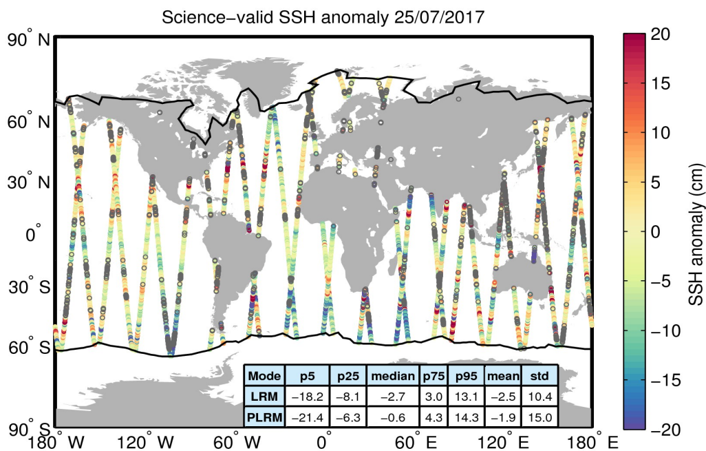
Figure 10. Geographical distribution of science-valid SSH anomaly data over oceans and lakes for 25/07/2017. The statistical values shown in the table refer to the SSH anomaly in cm and are calculated separately for LRM and PLRM regions. The black lines mark the outer limit of the Arctic and Antarctic polar polygons. Gray circles denote records that have been rejected based on the editing criteria described in Table 2.
