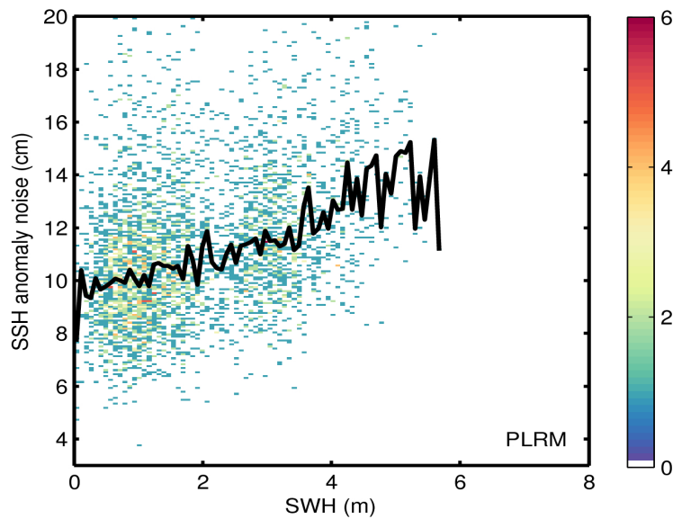
Figure 9. 2D histogram showing flag-valid SSH anomaly noise as a function of SWH for LRM (top) and PLRM (bottom) for 25/07/2017. The black line denotes the median SSH anomaly noise as a function of SWH.
