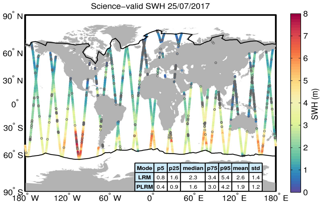
Figure 19. Geographical distribution of science-valid SWH data over oceans and lakes for 25/07/2017. The statistical values shown in the table refer to the SWH in m and are calculated separately for LRM and PLRM regions. The black lines mark the outer limit of the Arctic and Antarctic polar polygons. Gray circles denote records that have been rejected based on the editing criteria described in Table 3.
