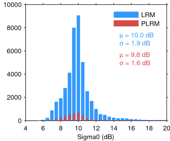
Figure 25. Histogram of flag-valid sigma0 over oceans and lakes for LRM (blue) and PLRM (red) for 24/07/2017. The mean ( \mu ) and standard deviation ( \sigma ) are also shown. Note that values outside [4 20] dB are excluded from the histogram for the sake of readability but not from the computation of \mu and \sigma .
