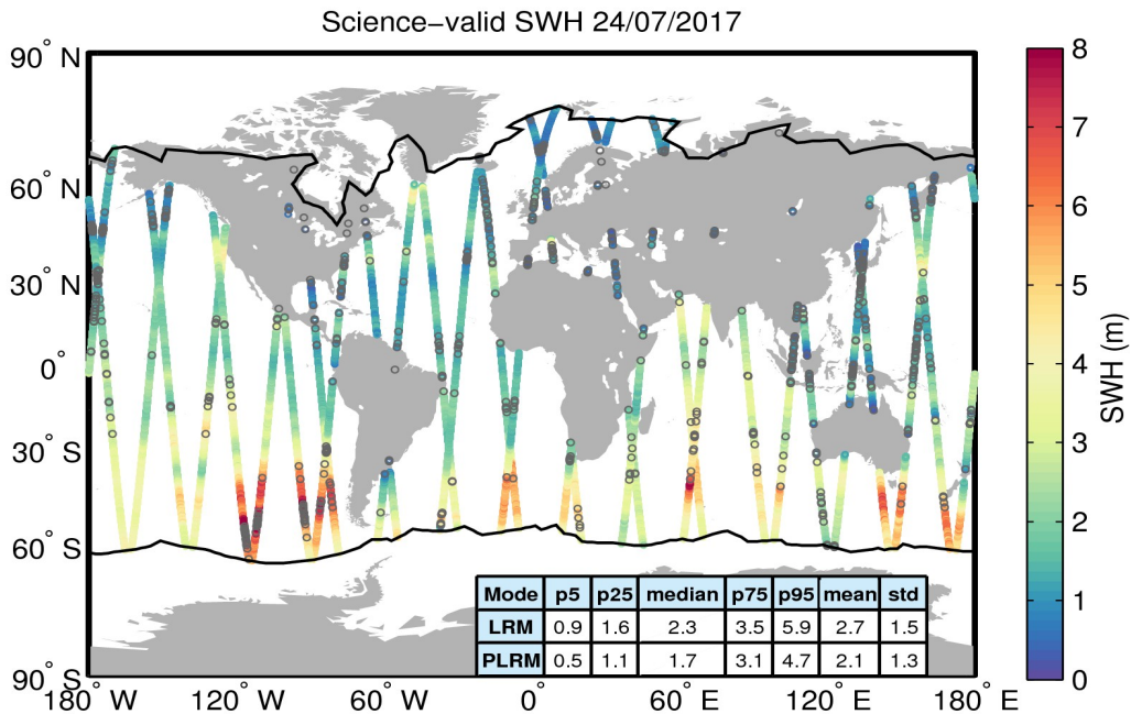
Figure 19. Geographical distribution of science-valid SWH data over oceans and lakes for 24/07/2017. The statistical values shown in the table refer to the SWH in m and are calculated separately for LRM and PLRM regions. The black lines mark the outer limit of the Arctic and Antarctic polar polygons. Gray circles denote records that have been rejected based on the editing criteria described in Table 3.
