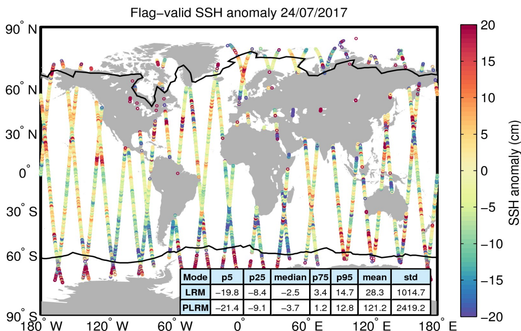
Figure 5. Geographical distribution of flag-valid 1-Hz SSH anomaly data over oceans and lakes for 24/07/2017. The statistical values shown in the table refer to the SSH anomaly in cm and are calculated separately for LRM and PLRM regions. Measurements taken over polar polygons have been excluded from the computation of the statistical values. The black lines mark the outer limit of the Arctic and Antarctic polar polygons.
