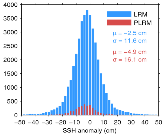
Figure 11. Histogram of science-valid SSH anomaly over oceans and lakes for LRM (blue) and PLRM (red) for 24/07/2017. The mean ( \mu ) and standard deviation ( \sigma ) are also shown. Note that values outside [-50\ 50] cm are excluded from the histogram for the sake of readability but not from the computation of \mu and \sigma .
