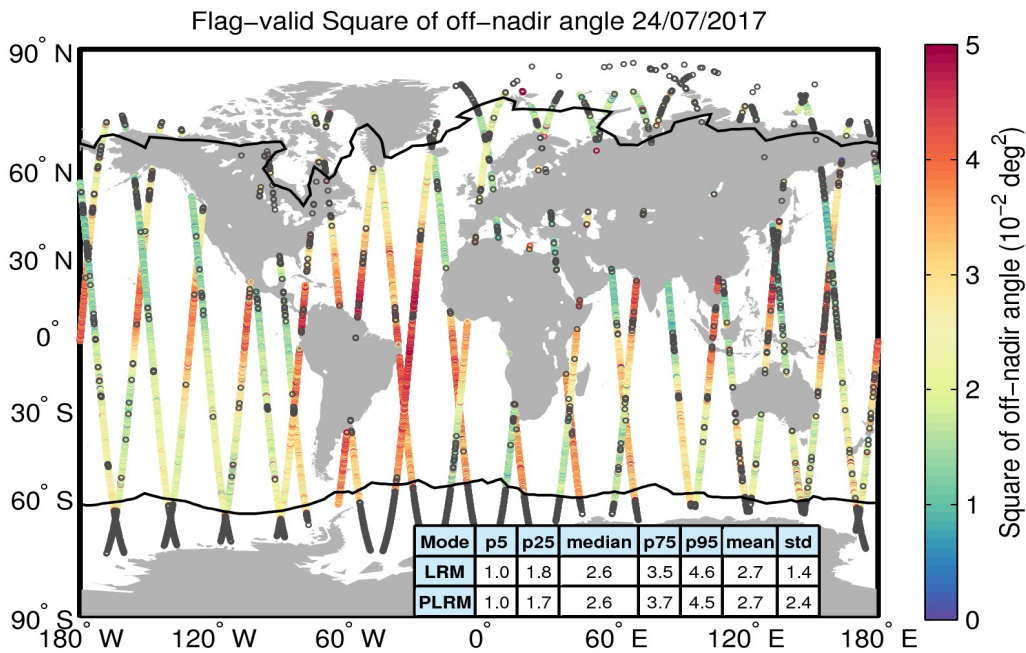
Figure 37. Geographical distribution of flag-valid mispointing data over oceans and lakes for 24/07/2017. The statistical values shown in the table refer to the mispointing in 10^{-2} deg 2 and are calculated separately for LRM and PLRM regions. Measurements taken over polar polygons have been excluded from the computation of the statistical values. The black lines mark the outer limit of the Arctic and Antarctic polar polygons. Gray circles denote negative values.
