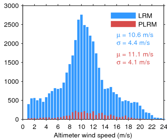
Figure 35. Histogram of science-valid wind over oceans and lakes for LRM (blue) and PLRM (red) for 24/07/2017. The mean ( \mu ) and standard deviation ( \sigma ) are also shown. Note that values larger than 24 m/s are excluded from the histogram for the sake of readability but not from the computation of \mu and \sigma .
