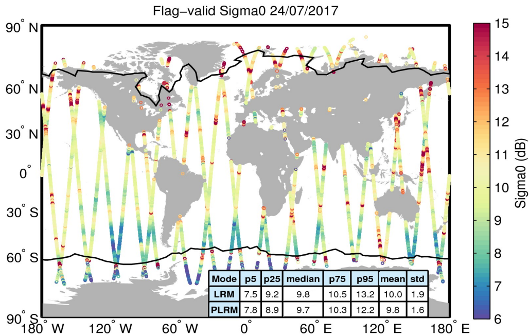
Figure 23. Geographical distribution of flag-valid sigma0 data over oceans and lakes for 24/07/2017. The statistical values shown in the table refer to the sigma0 in dB and are calculated separately for LRM and PLRM regions. Measurements taken over polar polygons have been excluded from the computation of the statistical values. The black lines mark the outer limit of the Arctic and Antarctic polar polygons.
