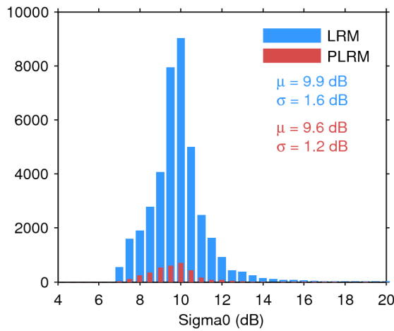
Figure 28. Histogram of science-valid sigma0 over oceans and lakes for LRM (blue) and PLRM (red) for 24/07/2017. The mean ( \mu ) and standard deviation ( \sigma ) are also shown. Note that values outside [4 20] dB are excluded from the histogram for the sake of readability but not from the computation of \mu and \sigma .
