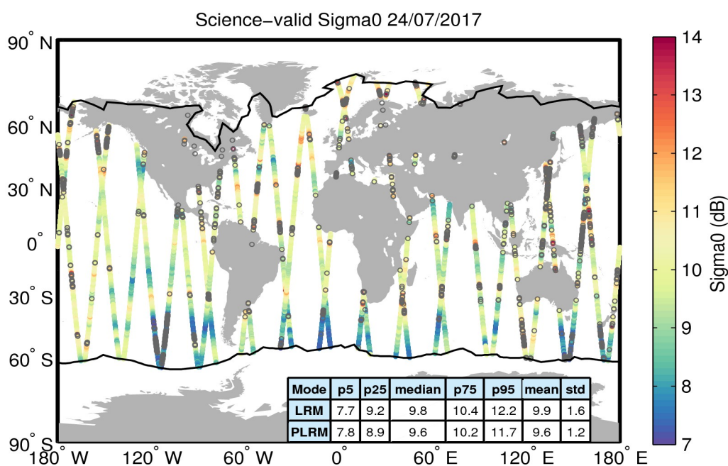
Figure 27. Geographical distribution of science-valid sigma0 data over oceans and lakes for 24/07/2017. The statistical values shown in the table refer to the sigma0 in dB and are calculated separately for LRM and PLRM regions. The black lines mark the outer limit of the Arctic and Antarctic polar polygons. Gray circles denote records that have been rejected based on the editing criteria described in Table 4.
