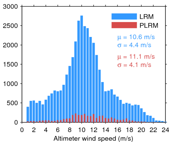
Figure 33. Histogram of flag-valid wind over oceans and lakes for LRM (blue) and PLRM (red) for 24/07/2017. The mean ( \mu ) and standard deviation ( \sigma ) are also shown. Note that values larger than 24 m/s are excluded from the histogram for the sake of readability but not from the computation of \mu and \sigma .
