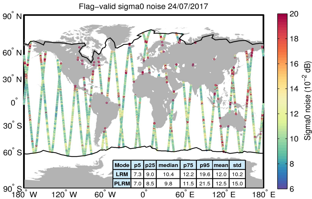
Figure 26. Geographical distribution of flag-valid 20-Hz sigma0 measurement noise over oceans and lakes for 24/07/2017. The statistical values shown in the table refer to the sigma0 noise and are calculated separately for LRM and PLRM regions. Measurements taken over polar polygons have been excluded from the computation of the statistical values. The black lines mark the outer limit of the Arctic and Antarctic polar polygons.
