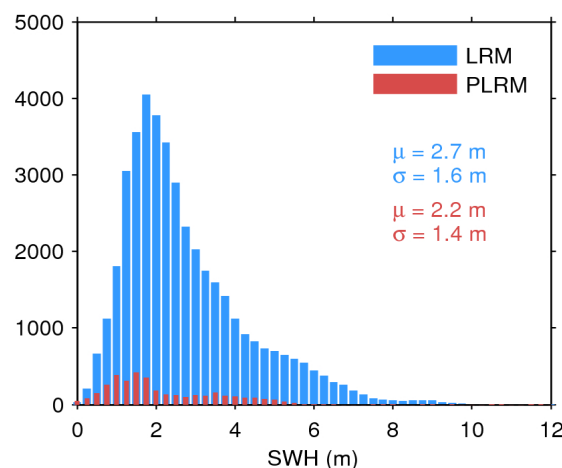
Figure 17. Histogram of flag-valid SWH over oceans and lakes for LRM (blue) and PLRM (red) for 24/07/2017. The mean ( \mu ) and standard deviation ( \sigma ) are also shown. Note that values larger than 12 m are excluded from the histogram for the sake of readability but not from the computation of \mu and \sigma .
