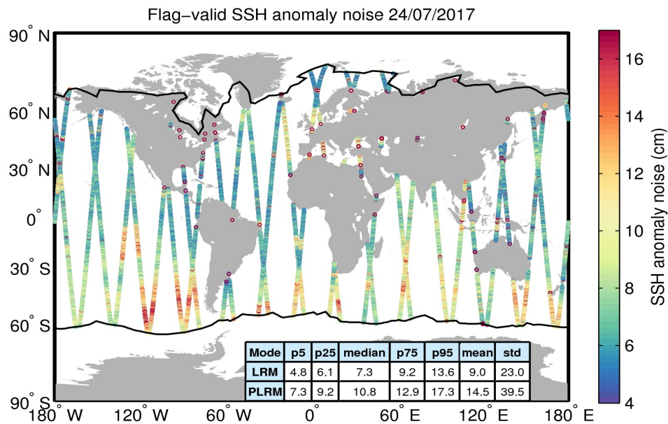
Figure 8. Geographical distribution of flag-valid 20-Hz SSH anomaly measurement noise over oceans and lakes for 24/07/2017. The statistical values shown in the table refer to the SSH anomaly noise and are calculated separately for LRM and PLRM regions. Measurements taken over polar polygons have been excluded from the computation of the statistical values. The black lines mark the outer limit of the Arctic and Antarctic polar polygons.
