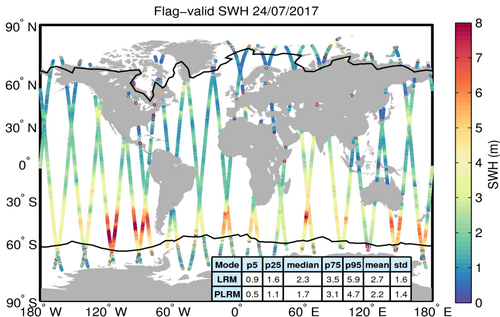
Figure 15. Geographical distribution of flag-valid SWH data over oceans and lakes for 24/07/2017. The statistical values shown in the table refer to the SWH in m and are calculated separately for LRM and PLRM regions. Measurements taken over polar polygons have been excluded from the computation of the statistical values. The black lines mark the outer limit of the Arctic and Antarctic polar polygons.
