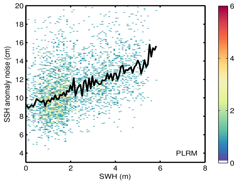
Figure 9. 2D histogram showing flag-valid SSH anomaly noise as a function of SWH for LRM (top) and PLRM (bottom) for 24/07/2017. The black line denotes the median SSH anomaly noise as a function of SWH.
