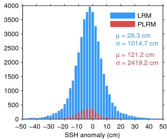
Figure 7. Histogram of flag-valid SSH anomaly over oceans and lakes for LRM (blue) and PLRM (red) for 24/07/2017. The mean ( \mu ) and standard deviation ( \sigma ) are also shown. Note that values outside [-50 50] cm are excluded from the histogram for the sake of readability but not from the computation of \mu and \sigma .
