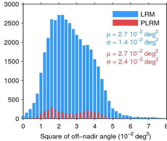
Figure 39. Histogram of flag-valid mispointing over oceans and lakes for LRM (blue) and PLRM (red) for 24/07/2017. Only positive values have been considered. The mean ( \mu ) and standard deviation ( \sigma ) are also shown. Note that values larger than 8 \cdot 10^{-2} \text{ deg}^2 are excluded from the histogram for the sake of readability but not from the computation of \mu and \sigma .
