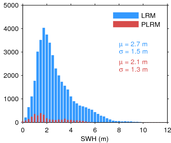
Figure 20. Histogram of science-valid SWH over oceans and lakes for LRM (blue) and PLRM (red) for 24/07/2017. The mean ( \mu ) and standard deviation ( \sigma ) are also shown. Note that values larger than 12 m are excluded from the histogram for the sake of readability but not from the computation of \mu and \sigma .
