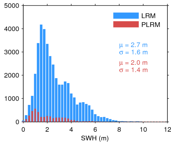
Figure 17. Histogram of flag-valid SWH over oceans and lakes for LRM (blue) and PLRM (red) for 23/07/2017. The mean ( \mu ) and standard deviation ( \sigma ) are also shown. Note that values larger than 12 m are excluded from the histogram for the sake of readability but not from the computation of \mu and \sigma .
