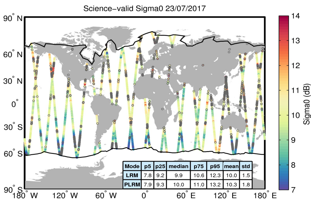
Figure 27. Geographical distribution of science-valid sigma0 data over oceans and lakes for 23/07/2017. The statistical values shown in the table refer to the sigma0 in dB and are calculated separately for LRM and PLRM regions. The black lines mark the outer limit of the Arctic and Antarctic polar polygons. Gray circles denote records that have been rejected based on the editing criteria described in Table 4.
