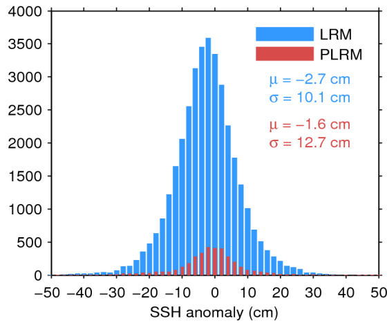
Figure 11. Histogram of science-valid SSH anomaly over oceans and lakes for LRM (blue) and PLRM (red) for 23/07/2017. The mean ( \mu ) and standard deviation ( \sigma ) are also shown. Note that values outside [-50 50] cm are excluded from the histogram for the sake of readability but not from the computation of \mu and \sigma .
