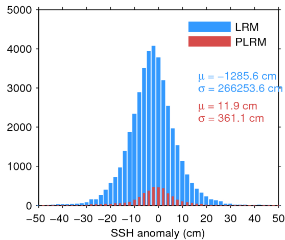
Figure 7. Histogram of flag-valid SSH anomaly over oceans and lakes for LRM (blue) and PLRM (red) for 23/07/2017. The mean ( \mu ) and standard deviation ( \sigma ) are also shown. Note that values outside [-50\ 50] cm are excluded from the histogram for the sake of readability but not from the computation of \mu and \sigma .
