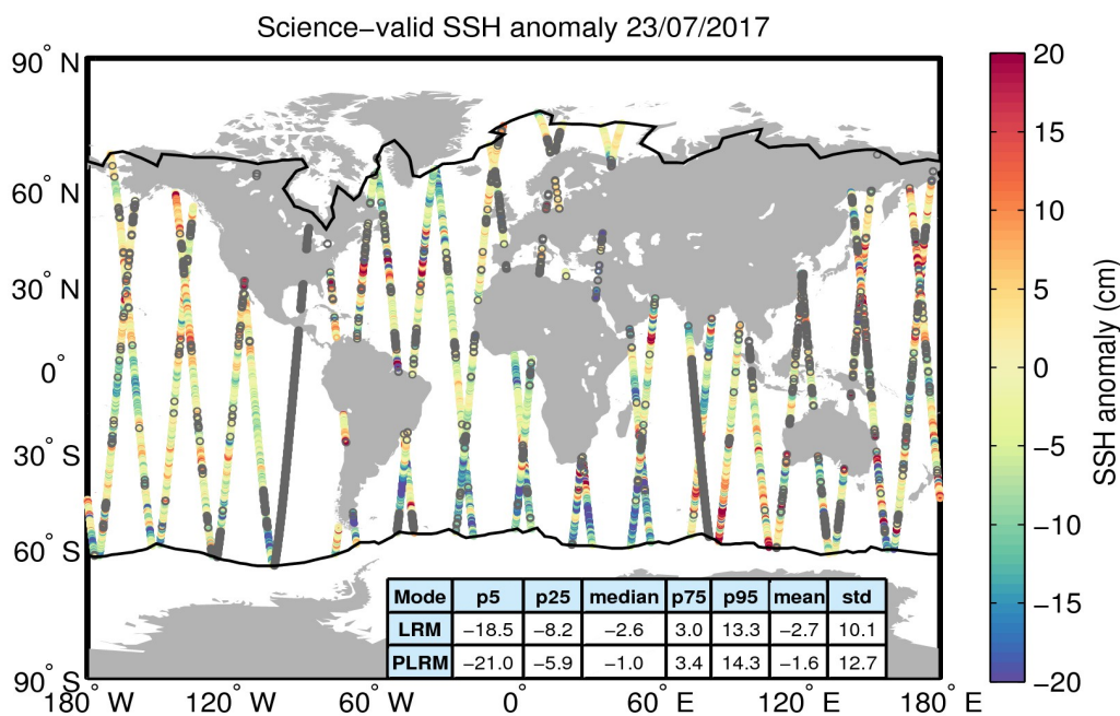
Figure 10. Geographical distribution of science-valid SSH anomaly data over oceans and lakes for 23/07/2017. The statistical values shown in the table refer to the SSH anomaly in cm and are calculated separately for LRM and PLRM regions. The black lines mark the outer limit of the Arctic and Antarctic polar polygons. Gray circles denote records that have been rejected based on the editing criteria described in Table 2.
