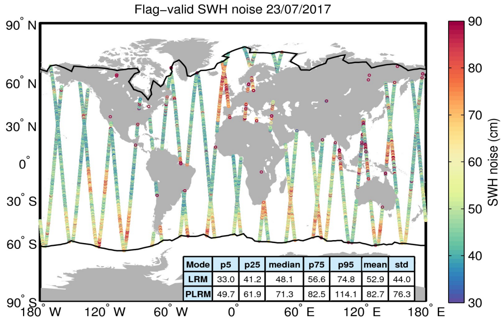
Figure 18. Geographical distribution of flag-valid 20-Hz SWH measurement noise over oceans and lakes for 23/07/2017. The statistical values shown in the table refer to the SWH noise and are calculated separately for LRM and PLRM regions. Measurements taken over polar polygons have been excluded from the computation of the statistical values. The black lines mark the outer limit of the Arctic and Antarctic polar polygons.
