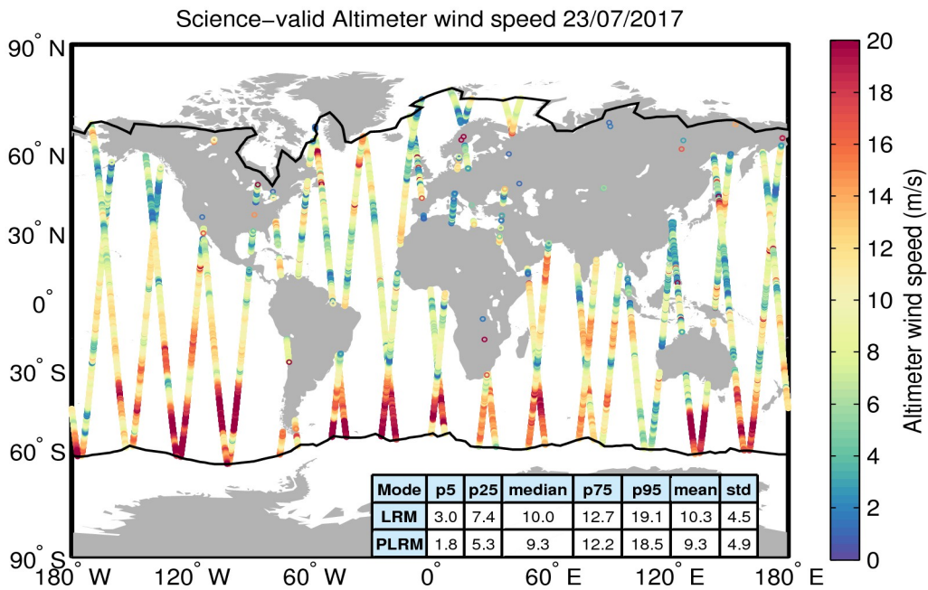
Figure 34. Geographical distribution of science-valid wind data over oceans and lakes for 23/07/2017. The statistical values shown in the table refer to the wind in m/s and are calculated separately for LRM and PLRM regions. The black lines mark the outer limit of the Arctic and Antarctic polar polygons. Gray circles denote records that have been rejected based on the editing criteria described in Table 5.
