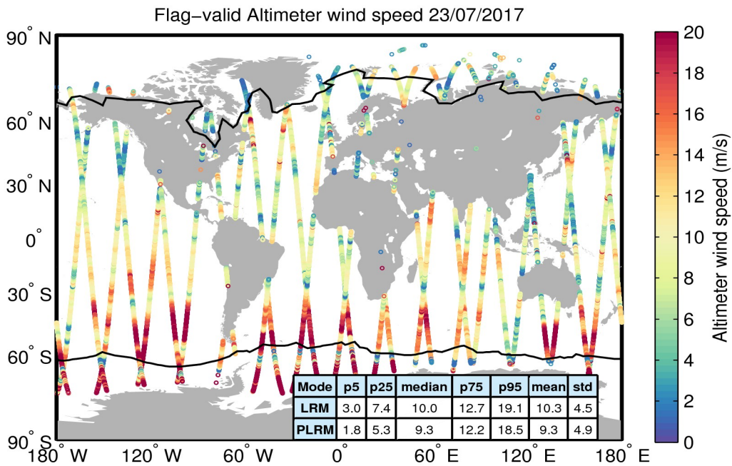
Figure 31. Geographical distribution of flag-valid wind data over oceans and lakes for 23/07/2017. The statistical values shown in the table refer to the wind in m/s and are calculated separately for LRM and PLRM regions. Measurements taken over polar polygons have been excluded from the computation of the statistical values. The black lines mark the outer limit of the Arctic and Antarctic polar polygons.
