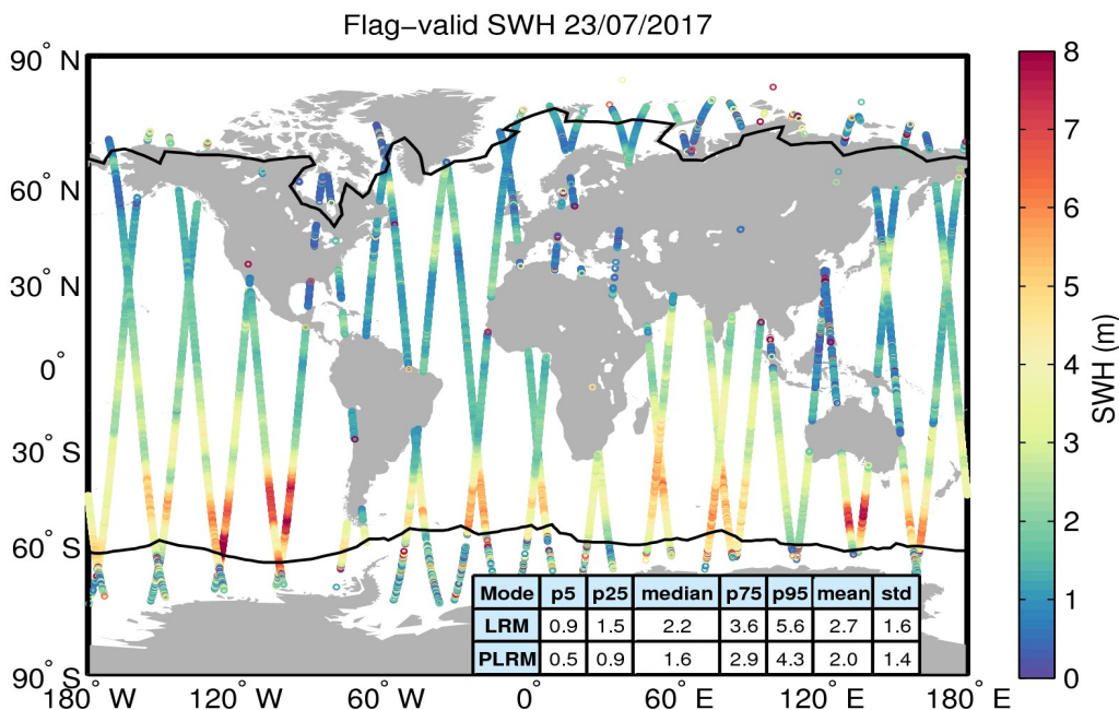
Figure 15. Geographical distribution of flag-valid SWH data over oceans and lakes for 23/07/2017. The statistical values shown in the table refer to the SWH in m and are calculated separately for LRM and PLRM regions. Measurements taken over polar polygons have been excluded from the computation of the statistical values. The black lines mark the outer limit of the Arctic and Antarctic polar polygons.
