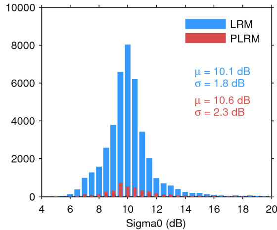
Figure 25. Histogram of flag-valid sigma0 over oceans and lakes for LRM (blue) and PLRM (red) for 23/07/2017. The mean ( \mu ) and standard deviation ( \sigma ) are also shown. Note that values outside [4 20] dB are excluded from the histogram for the sake of readability but not from the computation of \mu and \sigma .
