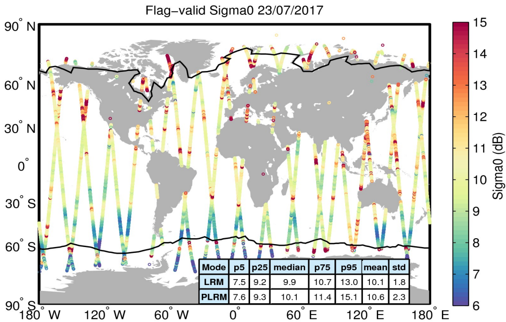
Figure 23. Geographical distribution of flag-valid sigma0 data over oceans and lakes for 23/07/2017. The statistical values shown in the table refer to the sigma0 in dB and are calculated separately for LRM and PLRM regions. Measurements taken over polar polygons have been excluded from the computation of the statistical values. The black lines mark the outer limit of the Arctic and Antarctic polar polygons.
