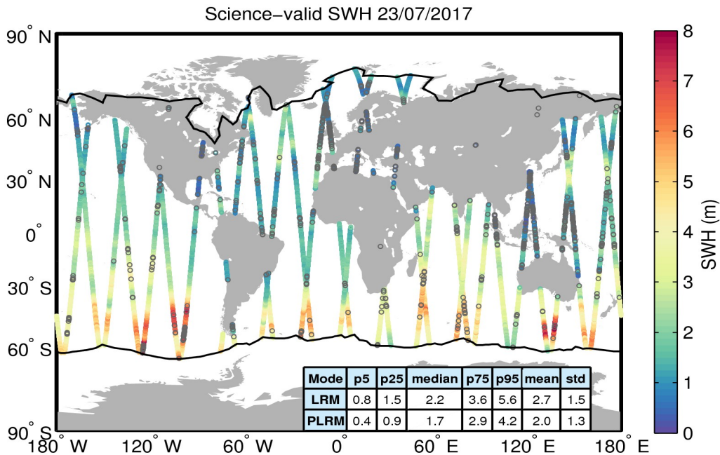
Figure 19. Geographical distribution of science-valid SWH data over oceans and lakes for 23/07/2017. The statistical values shown in the table refer to the SWH in m and are calculated separately for LRM and PLRM regions. The black lines mark the outer limit of the Arctic and Antarctic polar polygons. Gray circles denote records that have been rejected based on the editing criteria described in Table 3.
