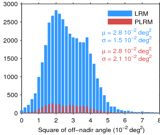
Figure 39. Histogram of flag-valid mispointing over oceans and lakes for LRM (blue) and PLRM (red) for 23/07/2017. Only positive values have been considered. The mean ( \mu ) and standard deviation ( \sigma ) are also shown. Note that values larger than 8 \cdot 10^{-2} \text{ deg}^2 are excluded from the histogram for the sake of readability but not from the computation of \mu and \sigma .
