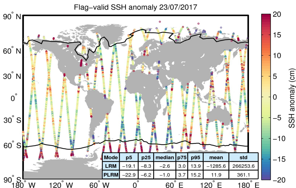
Figure 5. Geographical distribution of flag-valid 1-Hz SSH anomaly data over oceans and lakes for 23/07/2017. The statistical values shown in the table refer to the SSH anomaly in cm and are calculated separately for LRM and PLRM regions. Measurements taken over polar polygons have been excluded from the computation of the statistical values. The black lines mark the outer limit of the Arctic and Antarctic polar polygons.
