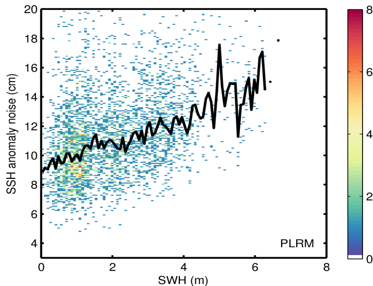
Figure 9. 2D histogram showing flag-valid SSH anomaly noise as a function of SWH for LRM (top) and PLRM (bottom) for 23/07/2017. The black line denotes the median SSH anomaly noise as a function of SWH.
