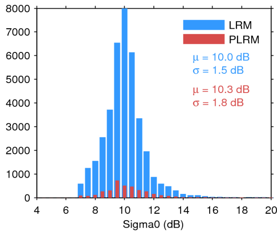
Figure 28. Histogram of science-valid sigma0 over oceans and lakes for LRM (blue) and PLRM (red) for 23/07/2017. The mean ( \mu ) and standard deviation ( \sigma ) are also shown. Note that values outside [4 20] dB are excluded from the histogram for the sake of readability but not from the computation of \mu and \sigma .
