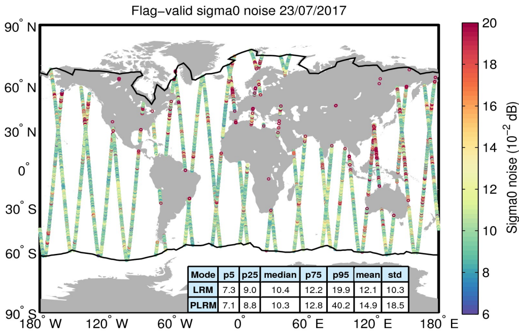
Figure 26. Geographical distribution of flag-valid 20-Hz sigma0 measurement noise over oceans and lakes for 23/07/2017. The statistical values shown in the table refer to the sigma0 noise and are calculated separately for LRM and PLRM regions. Measurements taken over polar polygons have been excluded from the computation of the statistical values. The black lines mark the outer limit of the Arctic and Antarctic polar polygons.
