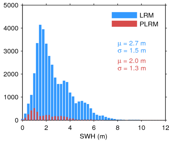
Figure 20. Histogram of science-valid SWH over oceans and lakes for LRM (blue) and PLRM (red) for 23/07/2017. The mean ( \mu ) and standard deviation ( \sigma ) are also shown. Note that values larger than 12 m are excluded from the histogram for the sake of readability but not from the computation of \mu and \sigma .
