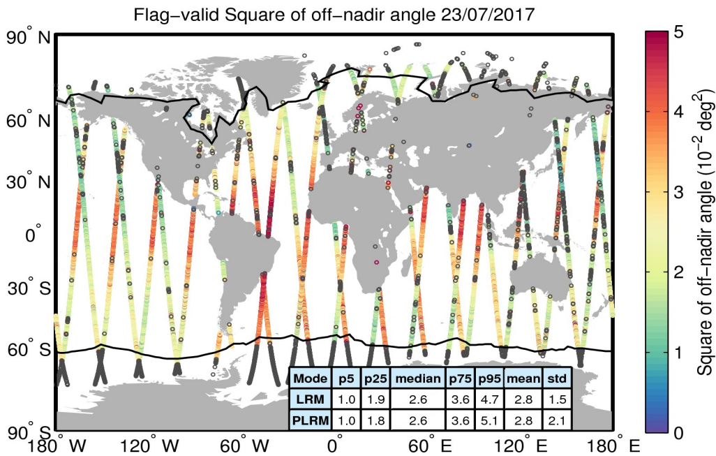
Figure 37. Geographical distribution of flag-valid mispointing data over oceans and lakes for 23/07/2017. The statistical values shown in the table refer to the mispointing in 10^{-2} deg 2 and are calculated separately for LRM and PLRM regions. Measurements taken over polar polygons have been excluded from the computation of the statistical values. The black lines mark the outer limit of the Arctic and Antarctic polar polygons. Gray circles denote negative values.
