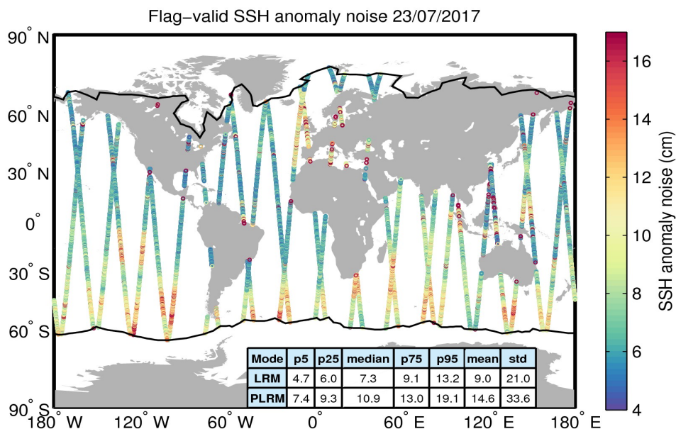
Figure 8. Geographical distribution of flag-valid 20-Hz SSH anomaly measurement noise over oceans and lakes for 23/07/2017. The statistical values shown in the table refer to the SSH anomaly noise and are calculated separately for LRM and PLRM regions. Measurements taken over polar polygons have been excluded from the computation of the statistical values. The black lines mark the outer limit of the Arctic and Antarctic polar polygons.
