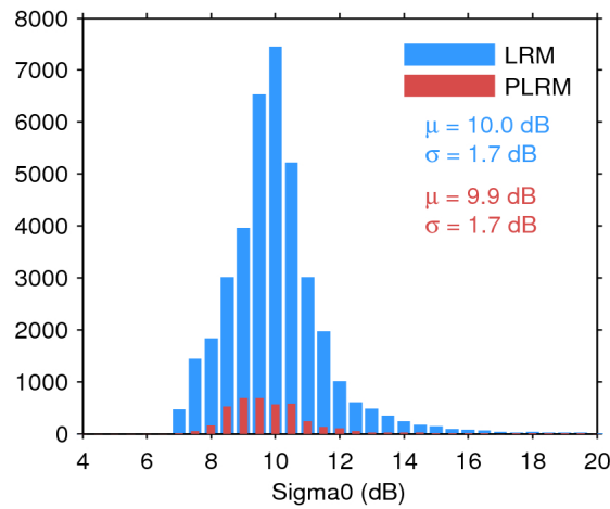
Figure 28. Histogram of science-valid sigma0 over oceans and lakes for LRM (blue) and PLRM (red) for 21/07/2017. The mean ( \mu ) and standard deviation ( \sigma ) are also shown. Note that values outside [4 20] dB are excluded from the histogram for the sake of readability but not from the computation of \mu and \sigma .
