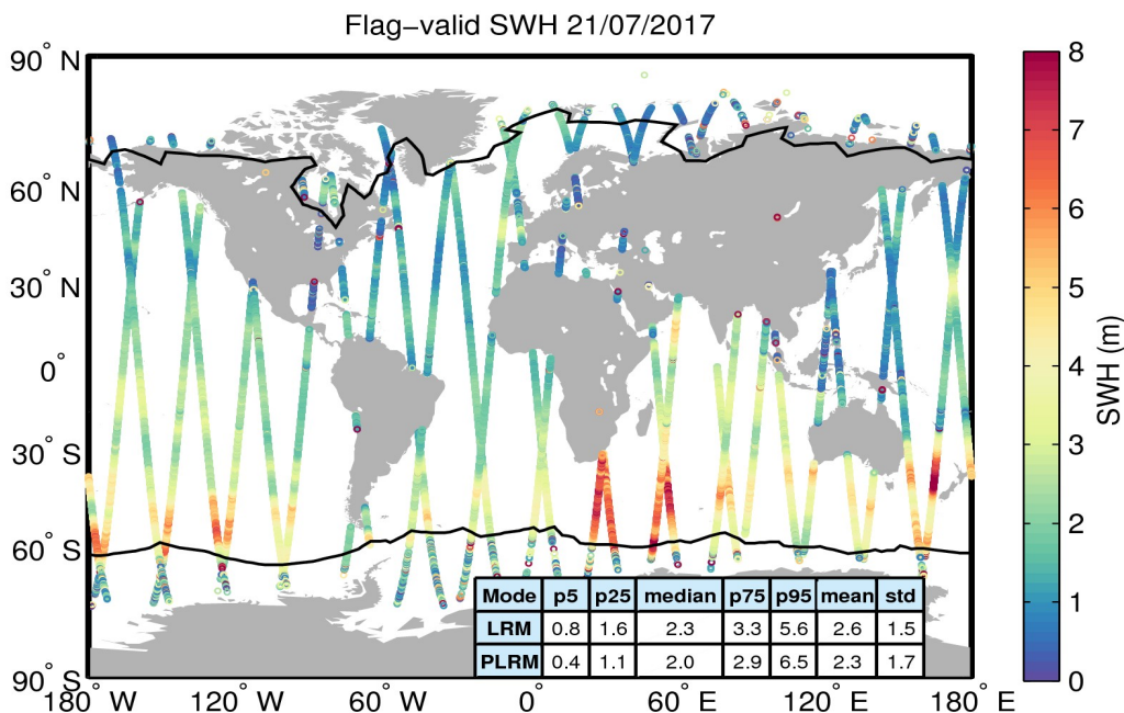
Figure 15. Geographical distribution of flag-valid SWH data over oceans and lakes for 21/07/2017. The statistical values shown in the table refer to the SWH in m and are calculated separately for LRM and PLRM regions. Measurements taken over polar polygons have been excluded from the computation of the statistical values. The black lines mark the outer limit of the Arctic and Antarctic polar polygons.
