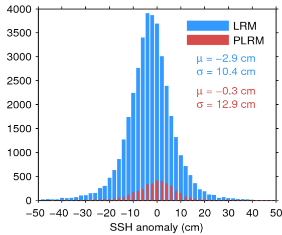
Figure 11. Histogram of science-valid SSH anomaly over oceans and lakes for LRM (blue) and PLRM (red) for 21/07/2017. The mean ( \mu ) and standard deviation ( \sigma ) are also shown. Note that values outside [-50 50] cm are excluded from the histogram for the sake of readability but not from the computation of \mu and \sigma .
