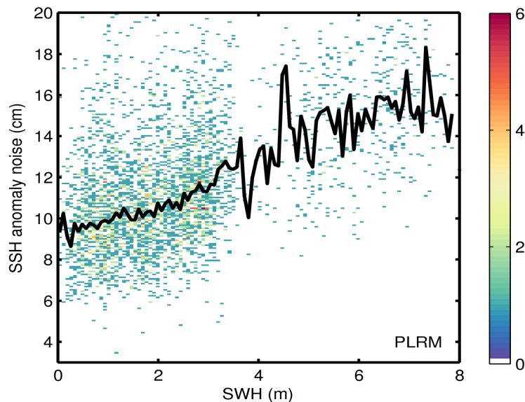
Figure 9. 2D histogram showing flag-valid SSH anomaly noise as a function of SWH for LRM (top) and PLRM (bottom) for 21/07/2017. The black line denotes the median SSH anomaly noise as a function of SWH.
