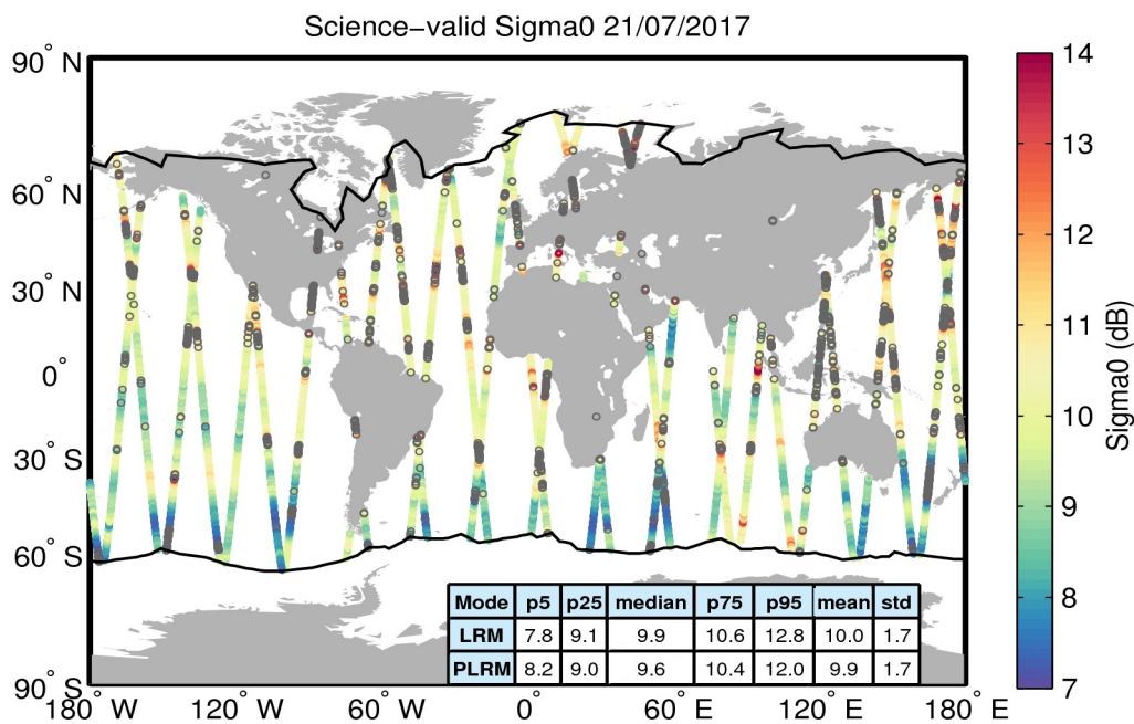
Figure 27. Geographical distribution of science-valid sigma0 data over oceans and lakes for 21/07/2017. The statistical values shown in the table refer to the sigma0 in dB and are calculated separately for LRM and PLRM regions. The black lines mark the outer limit of the Arctic and Antarctic polar polygons. Gray circles denote records that have been rejected based on the editing criteria described in Table 4.
