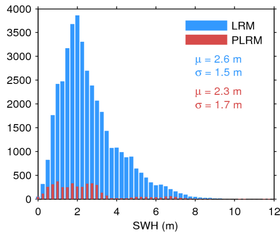
Figure 17. Histogram of flag-valid SWH over oceans and lakes for LRM (blue) and PLRM (red) for 21/07/2017. The mean ( \mu ) and standard deviation ( \sigma ) are also shown. Note that values larger than 12 m are excluded from the histogram for the sake of readability but not from the computation of \mu and \sigma .
