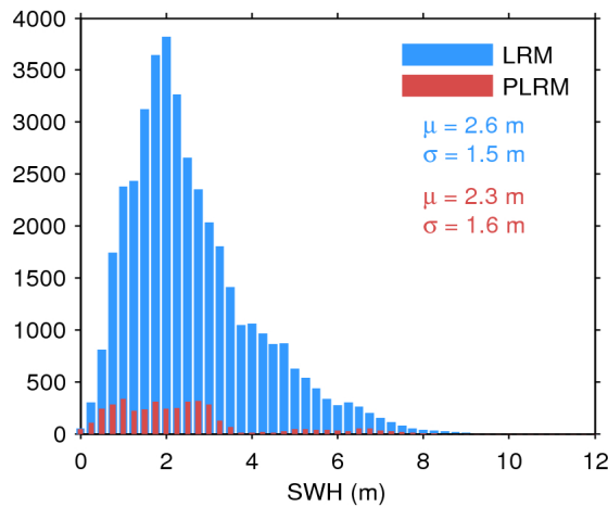
Figure 20. Histogram of science-valid SWH over oceans and lakes for LRM (blue) and PLRM (red) for 21/07/2017. The mean ( \mu ) and standard deviation ( \sigma ) are also shown. Note that values larger than 12 m are excluded from the histogram for the sake of readability but not from the computation of \mu and \sigma .
