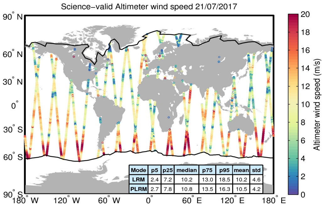
Figure 34. Geographical distribution of science-valid wind data over oceans and lakes for 21/07/2017. The statistical values shown in the table refer to the wind in m/s and are calculated separately for LRM and PLRM regions. The black lines mark the outer limit of the Arctic and Antarctic polar polygons. Gray circles denote records that have been rejected based on the editing criteria described in Table 5.
