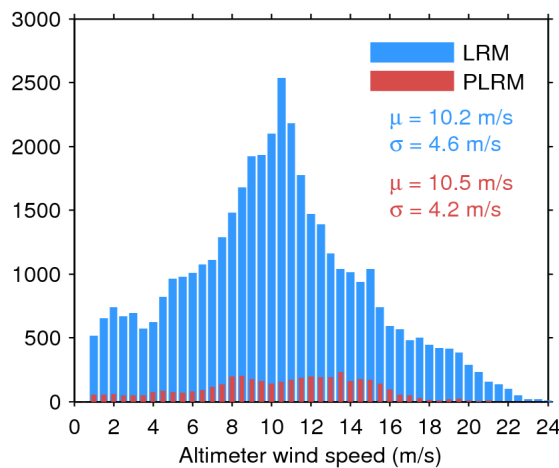
Figure 35. Histogram of science-valid wind over oceans and lakes for LRM (blue) and PLRM (red) for 21/07/2017. The mean ( \mu ) and standard deviation ( \sigma ) are also shown. Note that values larger than 24 m/s are excluded from the histogram for the sake of readability but not from the computation of \mu and \sigma .
