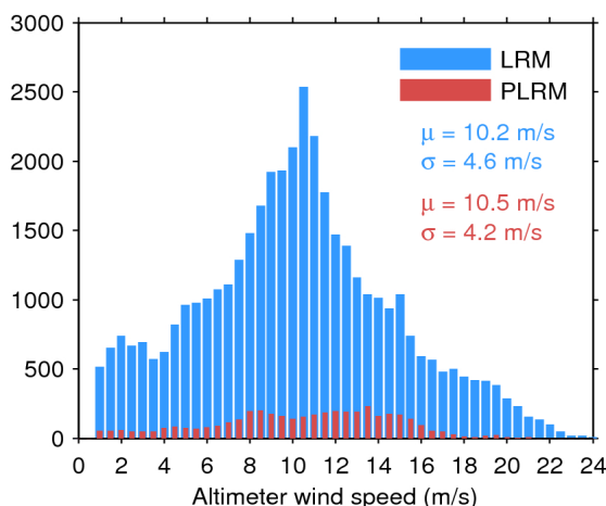
Figure 33. Histogram of flag-valid wind over oceans and lakes for LRM (blue) and PLRM (red) for 21/07/2017. The mean ( \mu ) and standard deviation ( \sigma ) are also shown. Note that values larger than 24 m/s are excluded from the histogram for the sake of readability but not from the computation of \mu and \sigma .
