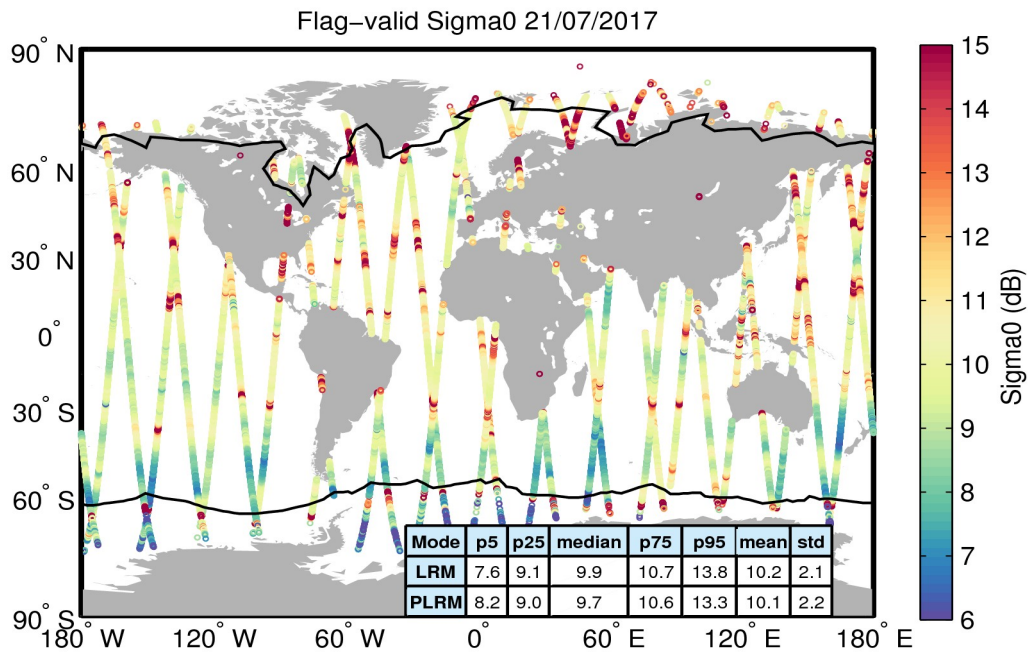
Figure 23. Geographical distribution of flag-valid sigma0 data over oceans and lakes for 21/07/2017. The statistical values shown in the table refer to the sigma0 in dB and are calculated separately for LRM and PLRM regions. Measurements taken over polar polygons have been excluded from the computation of the statistical values. The black lines mark the outer limit of the Arctic and Antarctic polar polygons.
