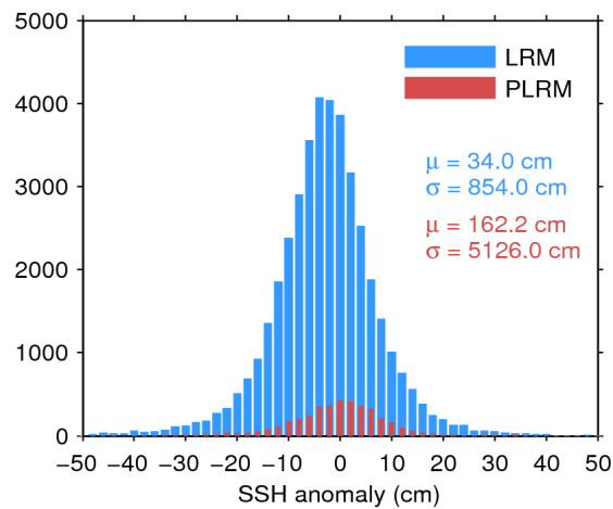
Figure 7. Histogram of flag-valid SSH anomaly over oceans and lakes for LRM (blue) and PLRM (red) for 21/07/2017. The mean ( \mu ) and standard deviation ( \sigma ) are also shown. Note that values outside [-50 50] cm are excluded from the histogram for the sake of readability but not from the computation of \mu and \sigma .
