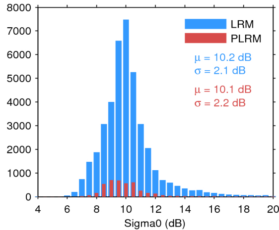
Figure 25. Histogram of flag-valid sigma0 over oceans and lakes for LRM (blue) and PLRM (red) for 21/07/2017. The mean ( \mu ) and standard deviation ( \sigma ) are also shown. Note that values outside [4 20] dB are excluded from the histogram for the sake of readability but not from the computation of \mu and \sigma .
