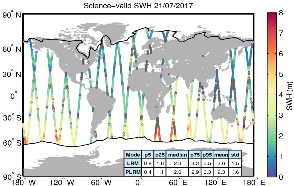
Figure 19. Geographical distribution of science-valid SWH data over oceans and lakes for 21/07/2017. The statistical values shown in the table refer to the SWH in m and are calculated separately for LRM and PLRM regions. The black lines mark the outer limit of the Arctic and Antarctic polar polygons. Gray circles denote records that have been rejected based on the editing criteria described in Table 3.
