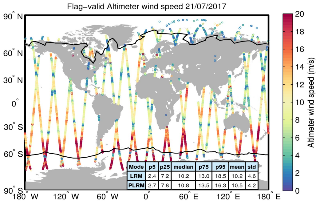
Figure 31. Geographical distribution of flag-valid wind data over oceans and lakes for 21/07/2017. The statistical values shown in the table refer to the wind in m/s and are calculated separately for LRM and PLRM regions. Measurements taken over polar polygons have been excluded from the computation of the statistical values. The black lines mark the outer limit of the Arctic and Antarctic polar polygons.
