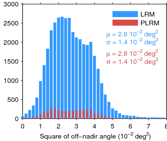
Figure 39. Histogram of flag-valid mispointing over oceans and lakes for LRM (blue) and PLRM (red) for 21/07/2017. Only positive values have been considered. The mean ( \mu ) and standard deviation ( \sigma ) are also shown. Note that values larger than 8 \cdot 10^{-2} \text{ deg}^2 are excluded from the histogram for the sake of readability but not from the computation of \mu and \sigma .
