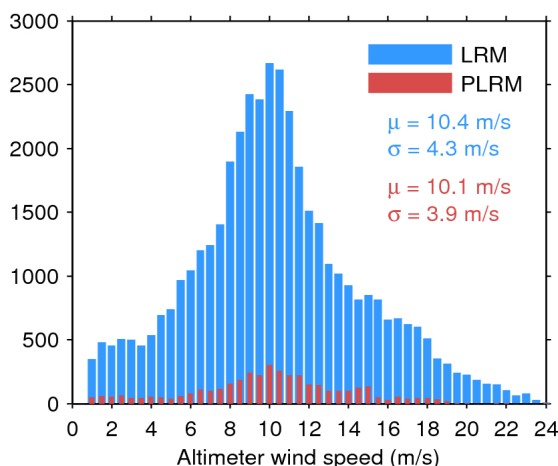
Figure 33. Histogram of flag-valid wind over oceans and lakes for LRM (blue) and PLRM (red) for 20/07/2017. The mean ( \mu ) and standard deviation ( \sigma ) are also shown. Note that values larger than 24 m/s are excluded from the histogram for the sake of readability but not from the computation of \mu and \sigma .
