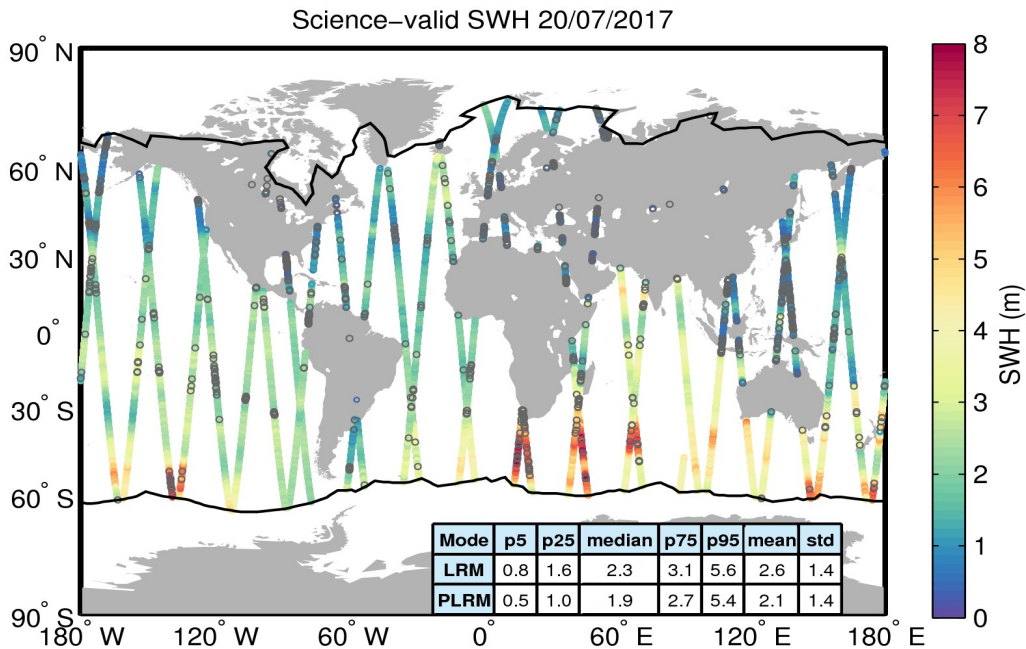
Figure 19. Geographical distribution of science-valid SWH data over oceans and lakes for 20/07/2017. The statistical values shown in the table refer to the SWH in m and are calculated separately for LRM and PLRM regions. The black lines mark the outer limit of the Arctic and Antarctic polar polygons. Gray circles denote records that have been rejected based on the editing criteria described in Table 3.
