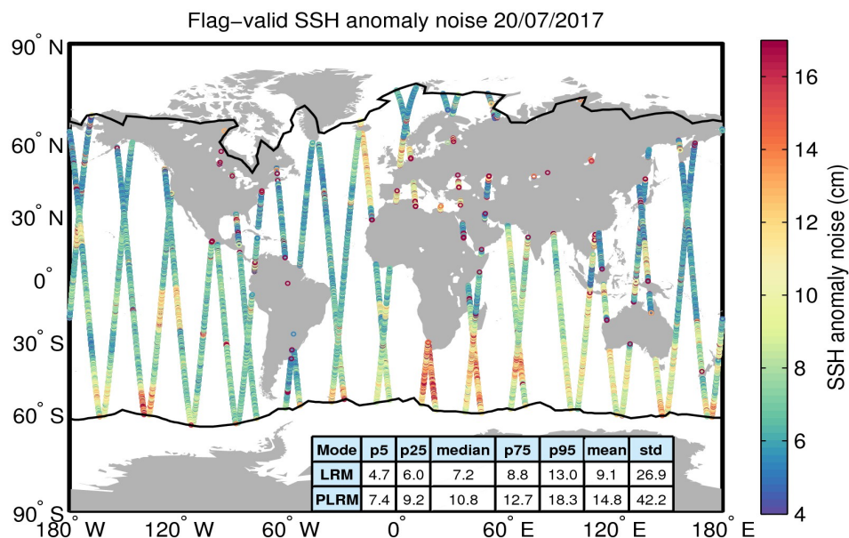
Figure 8. Geographical distribution of flag-valid 20-Hz SSH anomaly measurement noise over oceans and lakes for 20/07/2017. The statistical values shown in the table refer to the SSH anomaly noise and are calculated separately for LRM and PLRM regions. Measurements taken over polar polygons have been excluded from the computation of the statistical values. The black lines mark the outer limit of the Arctic and Antarctic polar polygons.
