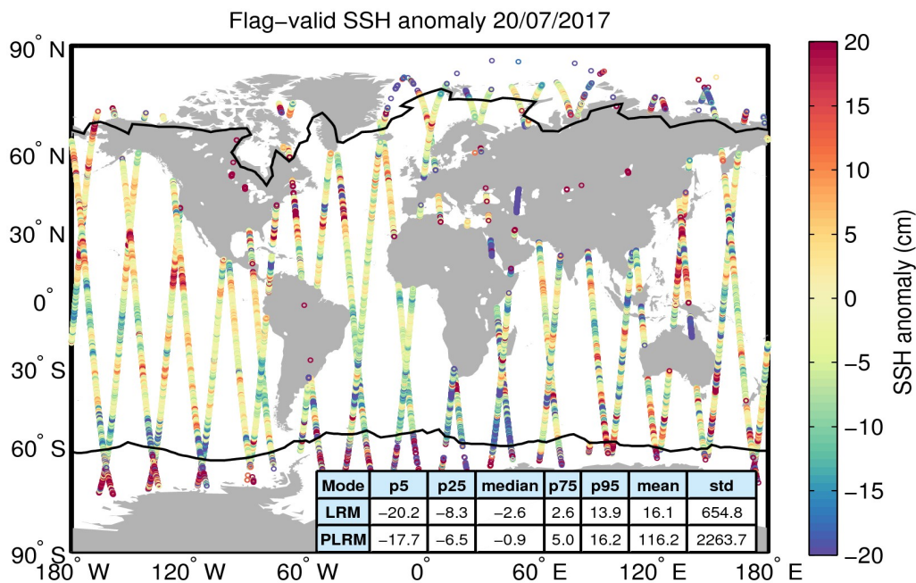
Figure 5. Geographical distribution of flag-valid 1-Hz SSH anomaly data over oceans and lakes for 20/07/2017. The statistical values shown in the table refer to the SSH anomaly in cm and are calculated separately for LRM and PLRM regions. Measurements taken over polar polygons have been excluded from the computation of the statistical values. The black lines mark the outer limit of the Arctic and Antarctic polar polygons.
