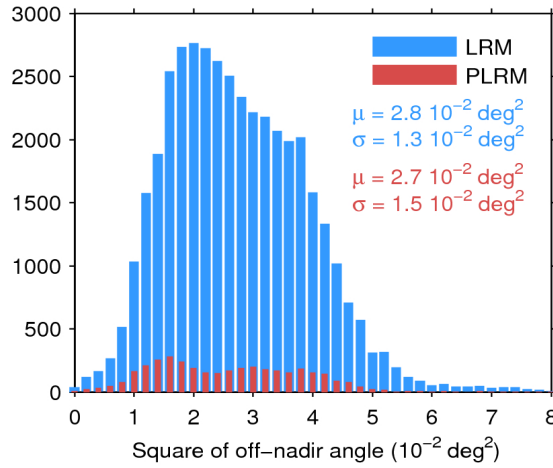
Figure 39. Histogram of flag-valid mispointing over oceans and lakes for LRM (blue) and PLRM (red) for 20/07/2017. Only positive values have been considered. The mean ( \mu ) and standard deviation ( \sigma ) are also shown. Note that values larger than 8 \cdot 10^{-2} \text{ deg}^2 are excluded from the histogram for the sake of readability but not from the computation of \mu and \sigma .
