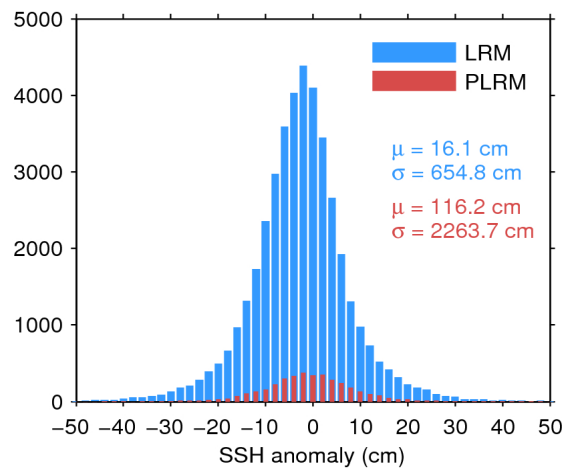
Figure 7. Histogram of flag-valid SSH anomaly over oceans and lakes for LRM (blue) and PLRM (red) for 20/07/2017. The mean ( \mu ) and standard deviation ( \sigma ) are also shown. Note that values outside [-50 50] cm are excluded from the histogram for the sake of readability but not from the computation of \mu and \sigma .
