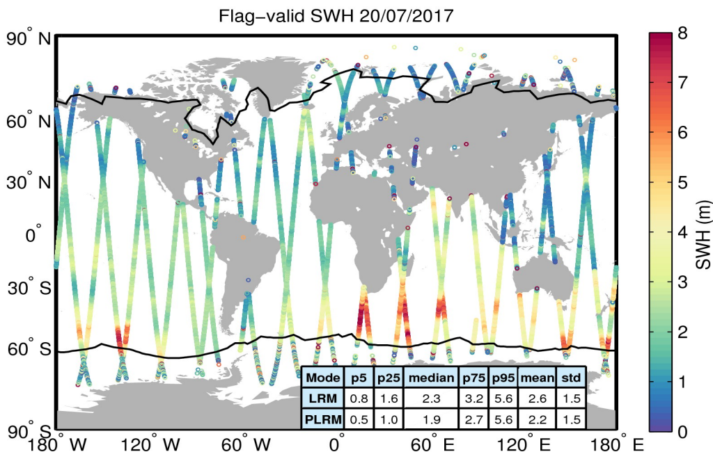
Figure 15. Geographical distribution of flag-valid SWH data over oceans and lakes for 20/07/2017. The statistical values shown in the table refer to the SWH in m and are calculated separately for LRM and PLRM regions. Measurements taken over polar polygons have been excluded from the computation of the statistical values. The black lines mark the outer limit of the Arctic and Antarctic polar polygons.
