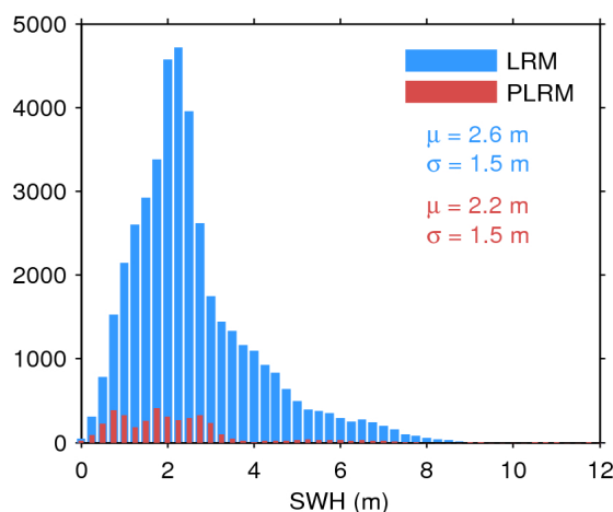
Figure 17. Histogram of flag-valid SWH over oceans and lakes for LRM (blue) and PLRM (red) for 20/07/2017. The mean ( \mu ) and standard deviation ( \sigma ) are also shown. Note that values larger than 12 m are excluded from the histogram for the sake of readability but not from the computation of \mu and \sigma .
