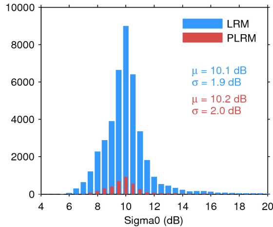
Figure 25. Histogram of flag-valid sigma0 over oceans and lakes for LRM (blue) and PLRM (red) for 20/07/2017. The mean ( \mu ) and standard deviation ( \sigma ) are also shown. Note that values outside [4 20] dB are excluded from the histogram for the sake of readability but not from the computation of \mu and \sigma .
