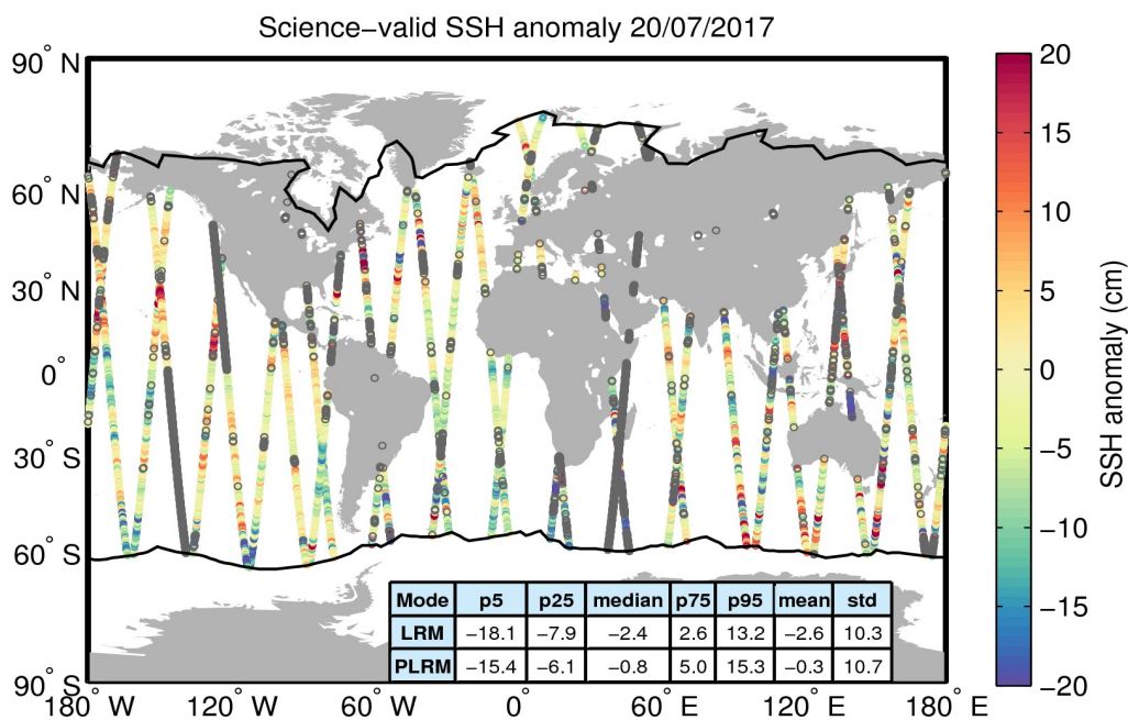
Figure 10. Geographical distribution of science-valid SSH anomaly data over oceans and lakes for 20/07/2017. The statistical values shown in the table refer to the SSH anomaly in cm and are calculated separately for LRM and PLRM regions. The black lines mark the outer limit of the Arctic and Antarctic polar polygons. Gray circles denote records that have been rejected based on the editing criteria described in Table 2.
