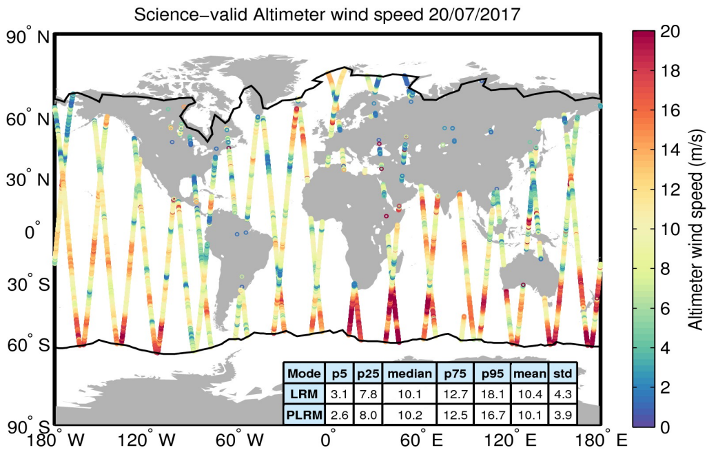
Figure 34. Geographical distribution of science-valid wind data over oceans and lakes for 20/07/2017. The statistical values shown in the table refer to the wind in m/s and are calculated separately for LRM and PLRM regions. The black lines mark the outer limit of the Arctic and Antarctic polar polygons. Gray circles denote records that have been rejected based on the editing criteria described in Table 5.
