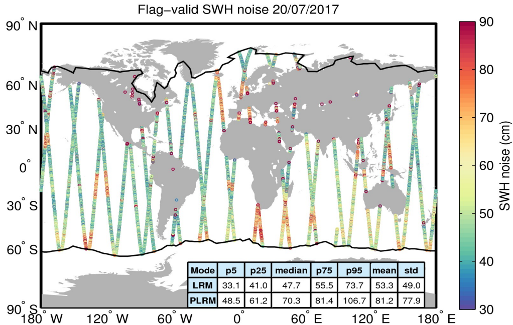
Figure 18. Geographical distribution of flag-valid 20-Hz SWH measurement noise over oceans and lakes for 20/07/2017. The statistical values shown in the table refer to the SWH noise and are calculated separately for LRM and PLRM regions. Measurements taken over polar polygons have been excluded from the computation of the statistical values. The black lines mark the outer limit of the Arctic and Antarctic polar polygons.
