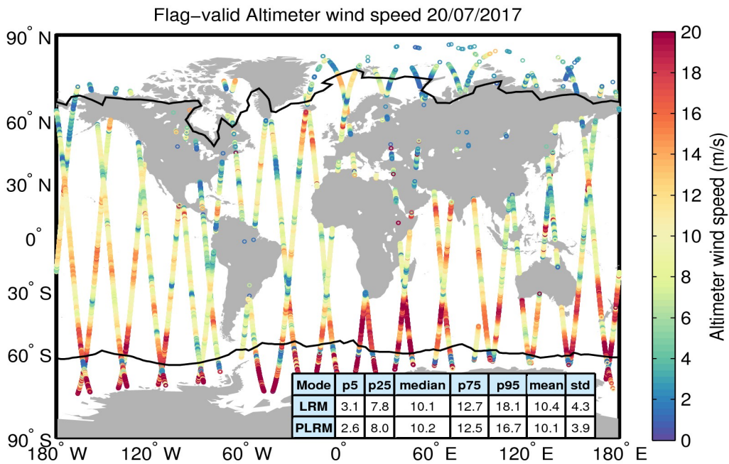
Figure 31. Geographical distribution of flag-valid wind data over oceans and lakes for 20/07/2017. The statistical values shown in the table refer to the wind in m/s and are calculated separately for LRM and PLRM regions. Measurements taken over polar polygons have been excluded from the computation of the statistical values. The black lines mark the outer limit of the Arctic and Antarctic polar polygons.
