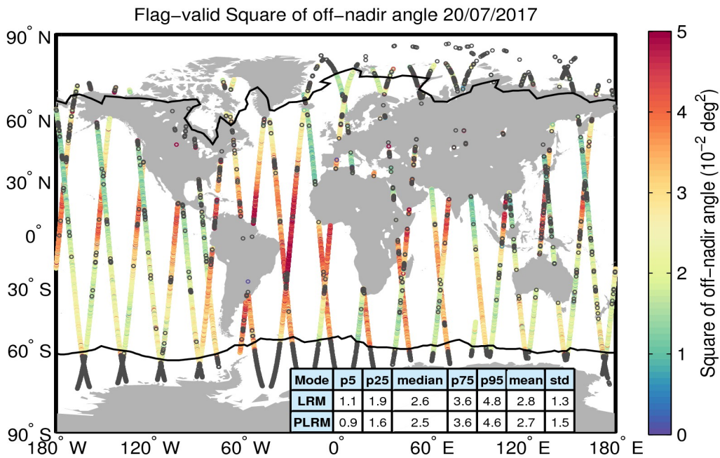
Figure 37. Geographical distribution of flag-valid mispointing data over oceans and lakes for 20/07/2017. The statistical values shown in the table refer to the mispointing in 10^{-2} deg 2 and are calculated separately for LRM and PLRM regions. Measurements taken over polar polygons have been excluded from the computation of the statistical values. The black lines mark the outer limit of the Arctic and Antarctic polar polygons. Gray circles denote negative values.
