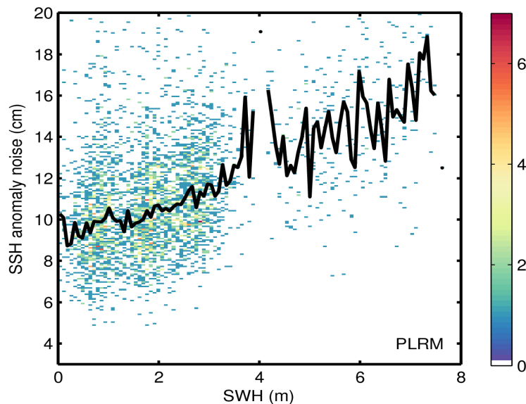
Figure 9. 2D histogram showing flag-valid SSH anomaly noise as a function of SWH for LRM (top) and PLRM (bottom) for 20/07/2017. The black line denotes the median SSH anomaly noise as a function of SWH.
