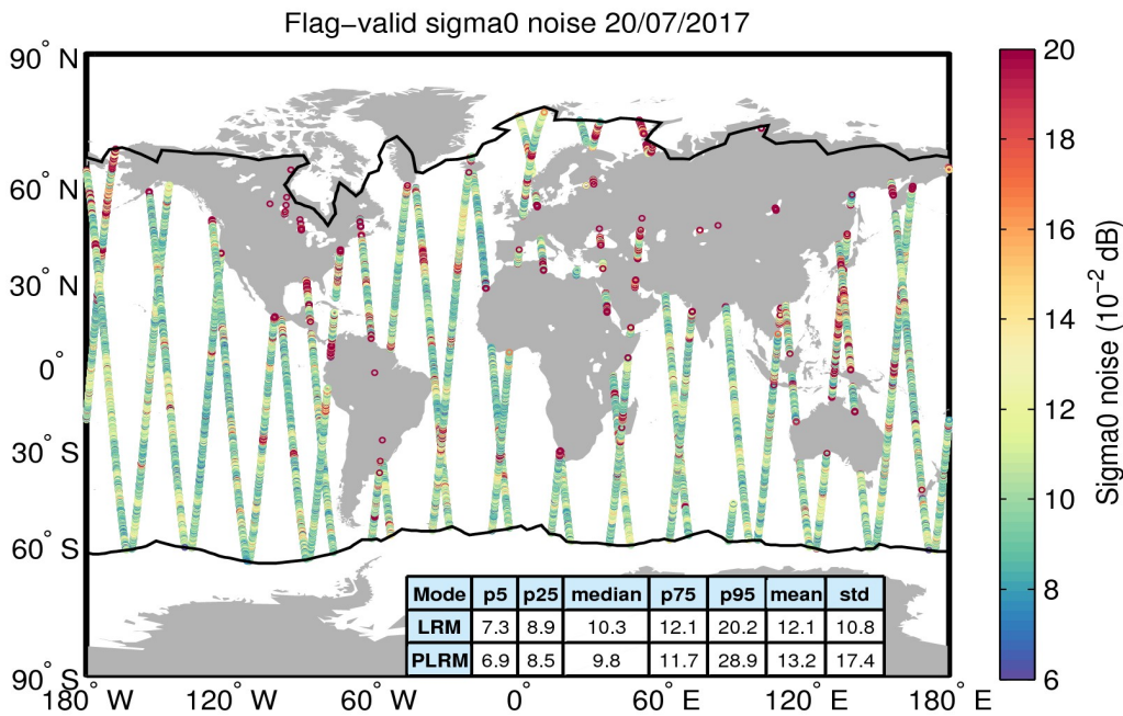
Figure 26. Geographical distribution of flag-valid 20-Hz sigma0 measurement noise over oceans and lakes for 20/07/2017. The statistical values shown in the table refer to the sigma0 noise and are calculated separately for LRM and PLRM regions. Measurements taken over polar polygons have been excluded from the computation of the statistical values. The black lines mark the outer limit of the Arctic and Antarctic polar polygons.
