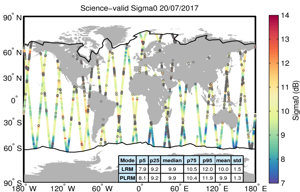
Figure 27. Geographical distribution of science-valid sigma0 data over oceans and lakes for 20/07/2017. The statistical values shown in the table refer to the sigma0 in dB and are calculated separately for LRM and PLRM regions. The black lines mark the outer limit of the Arctic and Antarctic polar polygons. Gray circles denote records that have been rejected based on the editing criteria described in Table 4.
