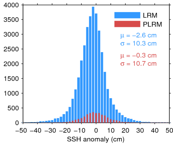
Figure 11. Histogram of science-valid SSH anomaly over oceans and lakes for LRM (blue) and PLRM (red) for 20/07/2017. The mean ( \mu ) and standard deviation ( \sigma ) are also shown. Note that values outside [-50 50] cm are excluded from the histogram for the sake of readability but not from the computation of \mu and \sigma .
