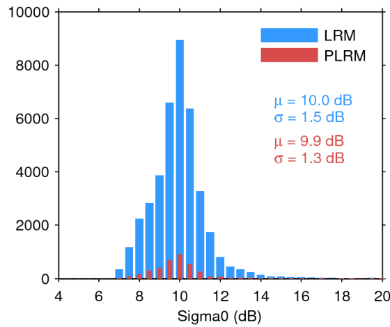
Figure 28. Histogram of science-valid sigma0 over oceans and lakes for LRM (blue) and PLRM (red) for 20/07/2017. The mean ( \mu ) and standard deviation ( \sigma ) are also shown. Note that values outside [4 20] dB are excluded from the histogram for the sake of readability but not from the computation of \mu and \sigma .
