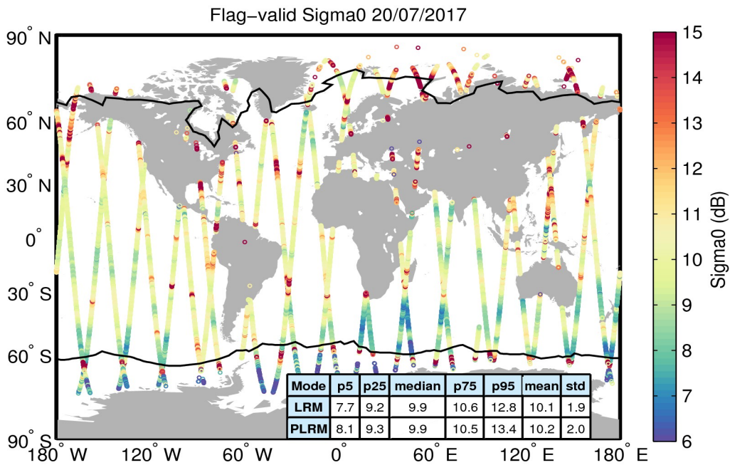
Figure 23. Geographical distribution of flag-valid sigma0 data over oceans and lakes for 20/07/2017. The statistical values shown in the table refer to the sigma0 in dB and are calculated separately for LRM and PLRM regions. Measurements taken over polar polygons have been excluded from the computation of the statistical values. The black lines mark the outer limit of the Arctic and Antarctic polar polygons.
