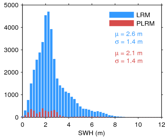
Figure 20. Histogram of science-valid SWH over oceans and lakes for LRM (blue) and PLRM (red) for 20/07/2017. The mean ( \mu ) and standard deviation ( \sigma ) are also shown. Note that values larger than 12 m are excluded from the histogram for the sake of readability but not from the computation of \mu and \sigma .
