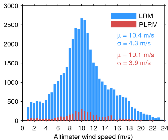
Figure 35. Histogram of science-valid wind over oceans and lakes for LRM (blue) and PLRM (red) for 20/07/2017. The mean ( \mu ) and standard deviation ( \sigma ) are also shown. Note that values larger than 24 m/s are excluded from the histogram for the sake of readability but not from the computation of \mu and \sigma .
