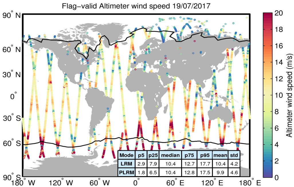
Figure 31. Geographical distribution of flag-valid wind data over oceans and lakes for 19/07/2017. The statistical values shown in the table refer to the wind in m/s and are calculated separately for LRM and PLRM regions. Measurements taken over polar polygons have been excluded from the computation of the statistical values. The black lines mark the outer limit of the Arctic and Antarctic polar polygons.
