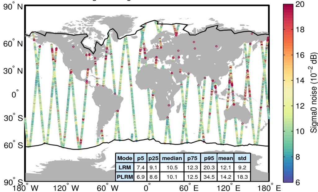
Flag-valid sigma0 noise 19/07/2017
