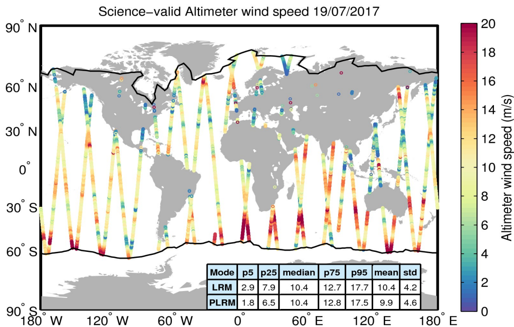
Figure 34. Geographical distribution of science-valid wind data over oceans and lakes for 19/07/2017. The statistical values shown in the table refer to the wind in m/s and are calculated separately for LRM and PLRM regions. The black lines mark the outer limit of the Arctic and Antarctic polar polygons. Gray circles denote records that have been rejected based on the editing criteria described in Table 5.
