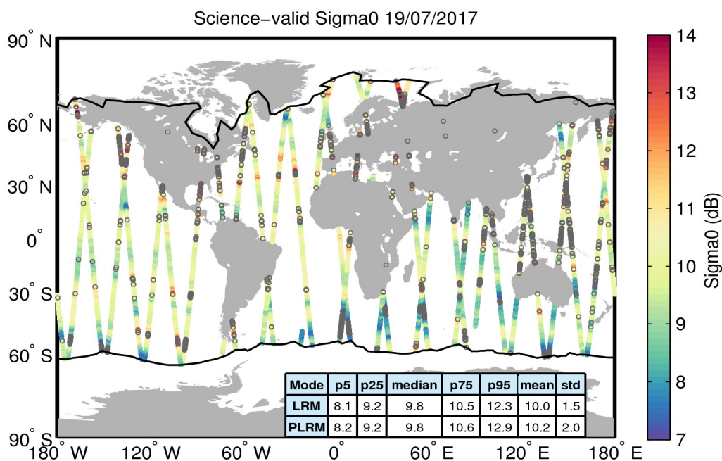
Figure 27. Geographical distribution of science-valid sigma0 data over oceans and lakes for 19/07/2017. The statistical values shown in the table refer to the sigma0 in dB and are calculated separately for LRM and PLRM regions. The black lines mark the outer limit of the Arctic and Antarctic polar polygons. Gray circles denote records that have been rejected based on the editing criteria described in Table 4.
