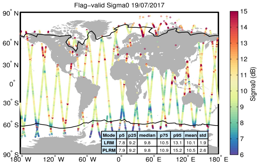
Figure 23. Geographical distribution of flag-valid sigma0 data over oceans and lakes for 19/07/2017. The statistical values shown in the table refer to the sigma0 in dB and are calculated separately for LRM and PLRM regions. Measurements taken over polar polygons have been excluded from the computation of the statistical values. The black lines mark the outer limit of the Arctic and Antarctic polar polygons.
