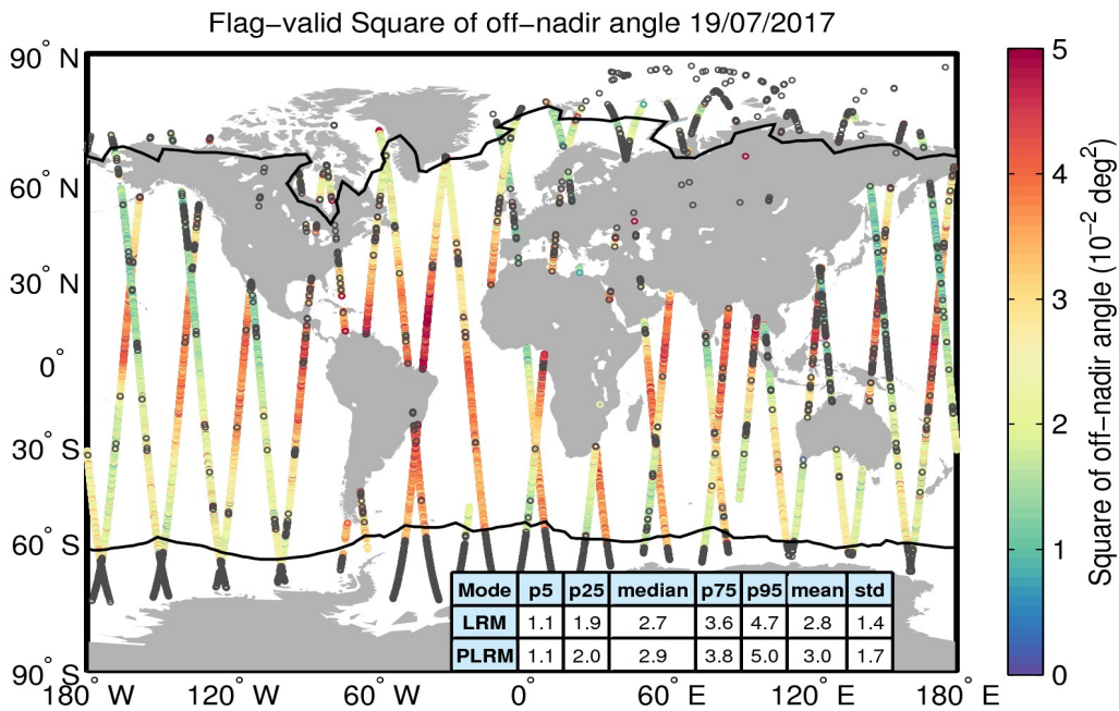
Figure 37. Geographical distribution of flag-valid mispointing data over oceans and lakes for 19/07/2017. The statistical values shown in the table refer to the mispointing in 10^{-2} deg 2 and are calculated separately for LRM and PLRM regions. Measurements taken over polar polygons have been excluded from the computation of the statistical values. The black lines mark the outer limit of the Arctic and Antarctic polar polygons. Gray circles denote negative values.
