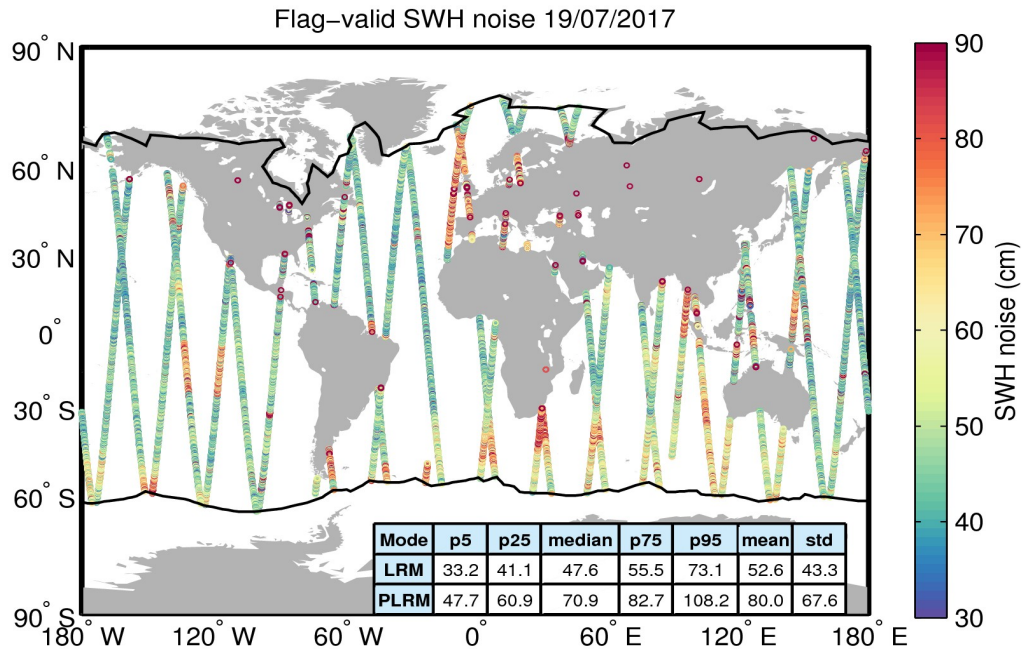
Figure 18. Geographical distribution of flag-valid 20-Hz SWH measurement noise over oceans and lakes for 19/07/2017. The statistical values shown in the table refer to the SWH noise and are calculated separately for LRM and PLRM regions. Measurements taken over polar polygons have been excluded from the computation of the statistical values. The black lines mark the outer limit of the Arctic and Antarctic polar polygons.
