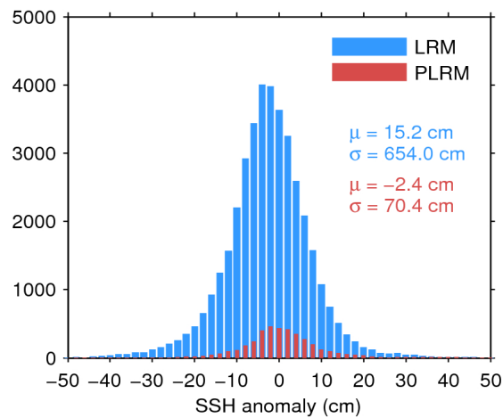
Figure 7. Histogram of flag-valid SSH anomaly over oceans and lakes for LRM (blue) and PLRM (red) for 19/07/2017. The mean ( \mu ) and standard deviation ( \sigma ) are also shown. Note that values outside [-50 50] cm are excluded from the histogram for the sake of readability but not from the computation of \mu and \sigma .
