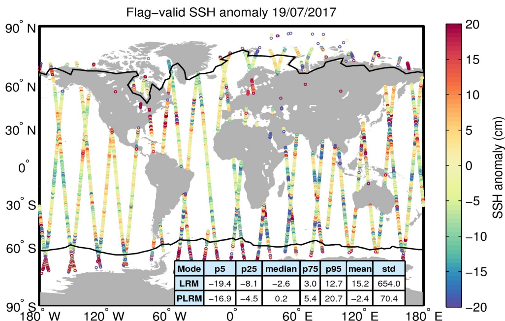
Figure 5. Geographical distribution of flag-valid 1-Hz SSH anomaly data over oceans and lakes for 19/07/2017. The statistical values shown in the table refer to the SSH anomaly in cm and are calculated separately for LRM and PLRM regions. Measurements taken over polar polygons have been excluded from the computation of the statistical values. The black lines mark the outer limit of the Arctic and Antarctic polar polygons.
