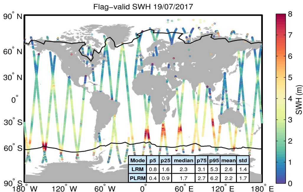
Figure 15. Geographical distribution of flag-valid SWH data over oceans and lakes for 19/07/2017. The statistical values shown in the table refer to the SWH in m and are calculated separately for LRM and PLRM regions. Measurements taken over polar polygons have been excluded from the computation of the statistical values. The black lines mark the outer limit of the Arctic and Antarctic polar polygons.
