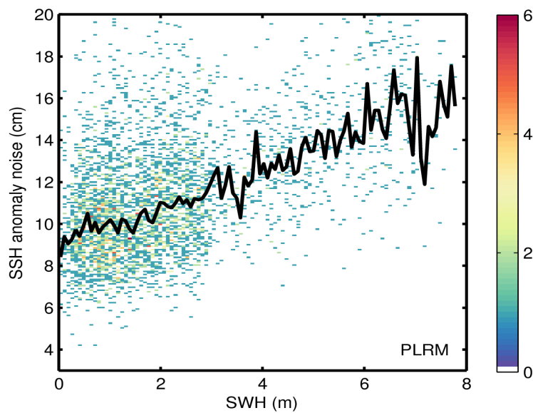
Figure 9. 2D histogram showing flag-valid SSH anomaly noise as a function of SWH for LRM (top) and PLRM (bottom) for 19/07/2017. The black line denotes the median SSH anomaly noise as a function of SWH.
