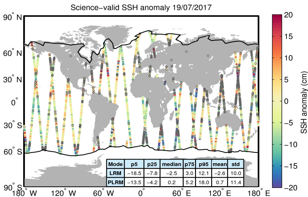
Figure 10. Geographical distribution of science-valid SSH anomaly data over oceans and lakes for 19/07/2017. The statistical values shown in the table refer to the SSH anomaly in cm and are calculated separately for LRM and PLRM regions. The black lines mark the outer limit of the Arctic and Antarctic polar polygons. Gray circles denote records that have been rejected based on the editing criteria described in Table 2.
