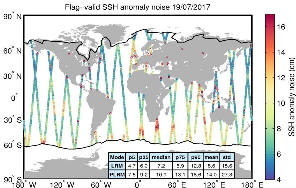
Figure 8. Geographical distribution of flag-valid 20-Hz SSH anomaly measurement noise over oceans and lakes for 19/07/2017. The statistical values shown in the table refer to the SSH anomaly noise and are calculated separately for LRM and PLRM regions. Measurements taken over polar polygons have been excluded from the computation of the statistical values. The black lines mark the outer limit of the Arctic and Antarctic polar polygons.
