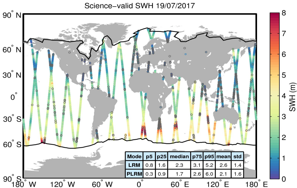
Figure 19. Geographical distribution of science-valid SWH data over oceans and lakes for 19/07/2017. The statistical values shown in the table refer to the SWH in m and are calculated separately for LRM and PLRM regions. The black lines mark the outer limit of the Arctic and Antarctic polar polygons. Gray circles denote records that have been rejected based on the editing criteria described in Table 3.
