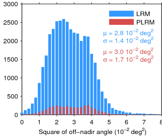
Figure 39. Histogram of flag-valid mispointing over oceans and lakes for LRM (blue) and PLRM (red) for 19/07/2017. Only positive values have been considered. The mean ( \mu ) and standard deviation ( \sigma ) are also shown. Note that values larger than 8 \cdot 10^{-2} \text{ deg}^2 are excluded from the histogram for the sake of readability but not from the computation of \mu and \sigma .
