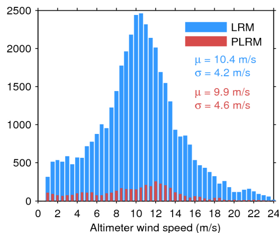
Figure 35. Histogram of science-valid wind over oceans and lakes for LRM (blue) and PLRM (red) for 19/07/2017. The mean ( \mu ) and standard deviation ( \sigma ) are also shown. Note that values larger than 24 m/s are excluded from the histogram for the sake of readability but not from the computation of \mu and \sigma .
