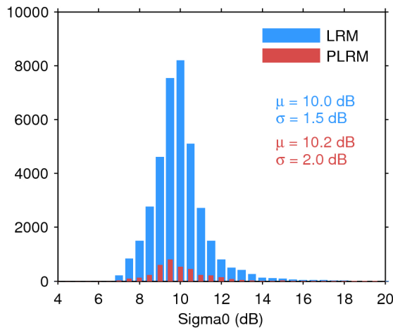
Figure 28. Histogram of science-valid sigma0 over oceans and lakes for LRM (blue) and PLRM (red) for 19/07/2017. The mean ( \mu ) and standard deviation ( \sigma ) are also shown. Note that values outside [4 20] dB are excluded from the histogram for the sake of readability but not from the computation of \mu and \sigma .
