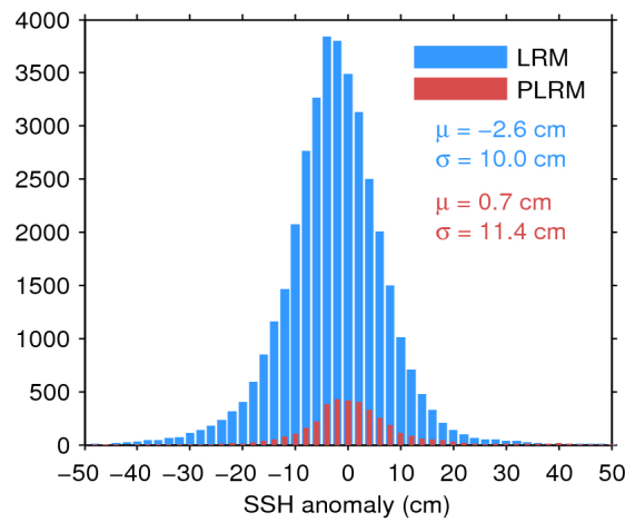
Figure 11. Histogram of science-valid SSH anomaly over oceans and lakes for LRM (blue) and PLRM (red) for 19/07/2017. The mean ( \mu ) and standard deviation ( \sigma ) are also shown. Note that values outside [-50\ 50] cm are excluded from the histogram for the sake of readability but not from the computation of \mu and \sigma .
