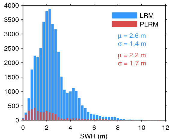
Figure 17. Histogram of flag-valid SWH over oceans and lakes for LRM (blue) and PLRM (red) for 19/07/2017. The mean ( \mu ) and standard deviation ( \sigma ) are also shown. Note that values larger than 12 m are excluded from the histogram for the sake of readability but not from the computation of \mu and \sigma .
