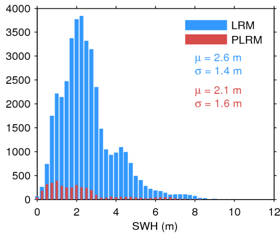
Figure 20. Histogram of science-valid SWH over oceans and lakes for LRM (blue) and PLRM (red) for 19/07/2017. The mean ( \mu ) and standard deviation ( \sigma ) are also shown. Note that values larger than 12 m are excluded from the histogram for the sake of readability but not from the computation of \mu and \sigma .
