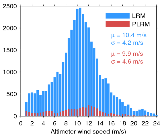
Figure 33. Histogram of flag-valid wind over oceans and lakes for LRM (blue) and PLRM (red) for 19/07/2017. The mean ( \mu ) and standard deviation ( \sigma ) are also shown. Note that values larger than 24 m/s are excluded from the histogram for the sake of readability but not from the computation of \mu and \sigma .
