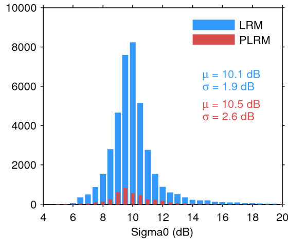
Figure 25. Histogram of flag-valid sigma0 over oceans and lakes for LRM (blue) and PLRM (red) for 19/07/2017. The mean ( \mu ) and standard deviation ( \sigma ) are also shown. Note that values outside [4 20] dB are excluded from the histogram for the sake of readability but not from the computation of \mu and \sigma .
