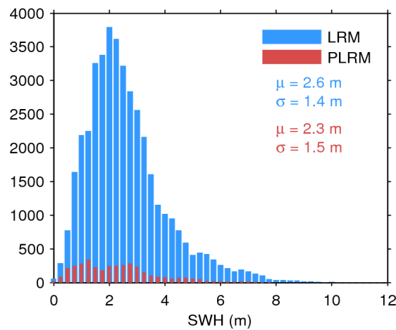
Figure 20. Histogram of science-valid SWH over oceans and lakes for LRM (blue) and PLRM (red) for 18/07/2017. The mean ( \mu ) and standard deviation ( \sigma ) are also shown. Note that values larger than 12 m are excluded from the histogram for the sake of readability but not from the computation of \mu and \sigma .
