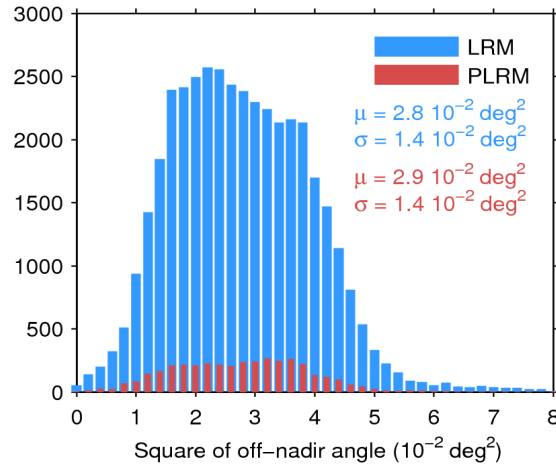
Figure 39. Histogram of flag-valid mispointing over oceans and lakes for LRM (blue) and PLRM (red) for 18/07/2017. Only positive values have been considered. The mean ( \mu ) and standard deviation ( \sigma ) are also shown. Note that values larger than 8 \cdot 10^{-2} \text{ deg}^2 are excluded from the histogram for the sake of readability but not from the computation of \mu and \sigma .
