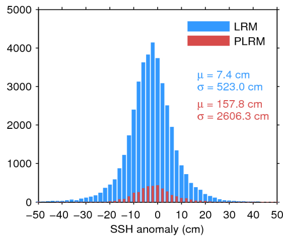
Figure 7. Histogram of flag-valid SSH anomaly over oceans and lakes for LRM (blue) and PLRM (red) for 18/07/2017. The mean ( \mu ) and standard deviation ( \sigma ) are also shown. Note that values outside [-50\ 50] cm are excluded from the histogram for the sake of readability but not from the computation of \mu and \sigma .
