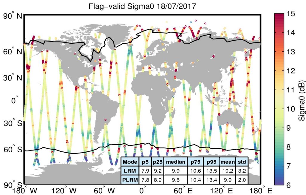
Figure 23. Geographical distribution of flag-valid sigma0 data over oceans and lakes for 18/07/2017. The statistical values shown in the table refer to the sigma0 in dB and are calculated separately for LRM and PLRM regions. Measurements taken over polar polygons have been excluded from the computation of the statistical values. The black lines mark the outer limit of the Arctic and Antarctic polar polygons.
