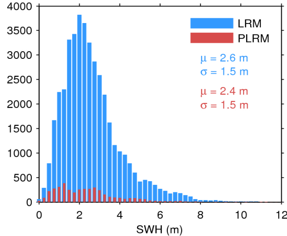
Figure 17. Histogram of flag-valid SWH over oceans and lakes for LRM (blue) and PLRM (red) for 18/07/2017. The mean ( \mu ) and standard deviation ( \sigma ) are also shown. Note that values larger than 12 m are excluded from the histogram for the sake of readability but not from the computation of \mu and \sigma .
