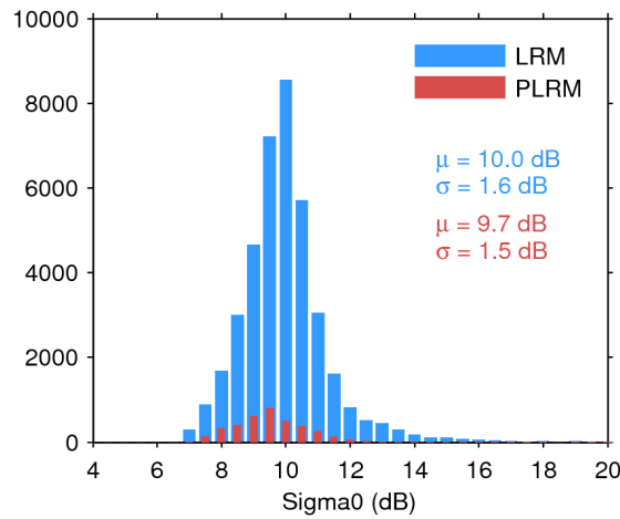
Figure 28. Histogram of science-valid sigma0 over oceans and lakes for LRM (blue) and PLRM (red) for 18/07/2017. The mean ( \mu ) and standard deviation ( \sigma ) are also shown. Note that values outside [4 20] dB are excluded from the histogram for the sake of readability but not from the computation of \mu and \sigma .
