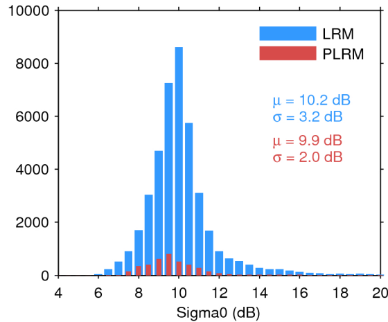
Figure 25. Histogram of flag-valid sigma0 over oceans and lakes for LRM (blue) and PLRM (red) for 18/07/2017. The mean ( \mu ) and standard deviation ( \sigma ) are also shown. Note that values outside [4 20] dB are excluded from the histogram for the sake of readability but not from the computation of \mu and \sigma .
