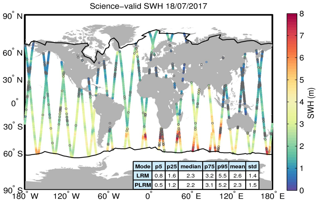
Figure 19. Geographical distribution of science-valid SWH data over oceans and lakes for 18/07/2017. The statistical values shown in the table refer to the SWH in m and are calculated separately for LRM and PLRM regions. The black lines mark the outer limit of the Arctic and Antarctic polar polygons. Gray circles denote records that have been rejected based on the editing criteria described in Table 3.
