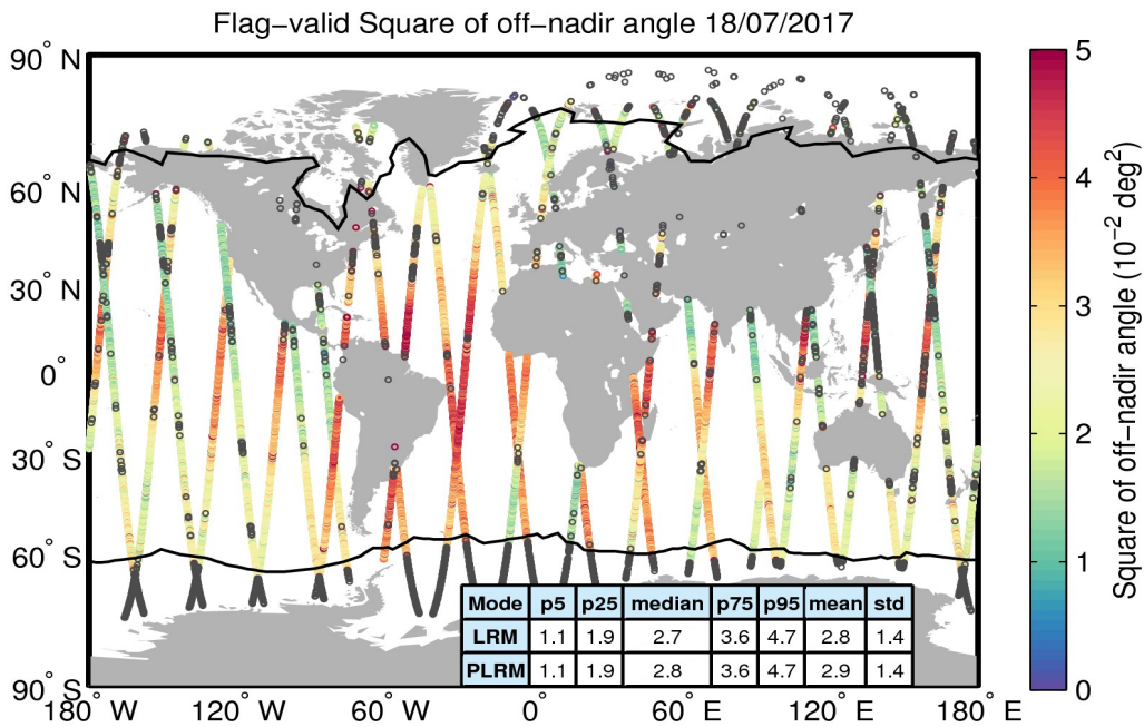
Figure 37. Geographical distribution of flag-valid mispointing data over oceans and lakes for 18/07/2017. The statistical values shown in the table refer to the mispointing in 10^{-2} deg 2 and are calculated separately for LRM and PLRM regions. Measurements taken over polar polygons have been excluded from the computation of the statistical values. The black lines mark the outer limit of the Arctic and Antarctic polar polygons. Gray circles denote negative values.
