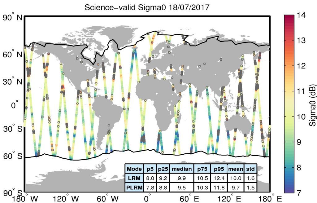
Figure 27. Geographical distribution of science-valid sigma0 data over oceans and lakes for 18/07/2017. The statistical values shown in the table refer to the sigma0 in dB and are calculated separately for LRM and PLRM regions. The black lines mark the outer limit of the Arctic and Antarctic polar polygons. Gray circles denote records that have been rejected based on the editing criteria described in Table 4.
