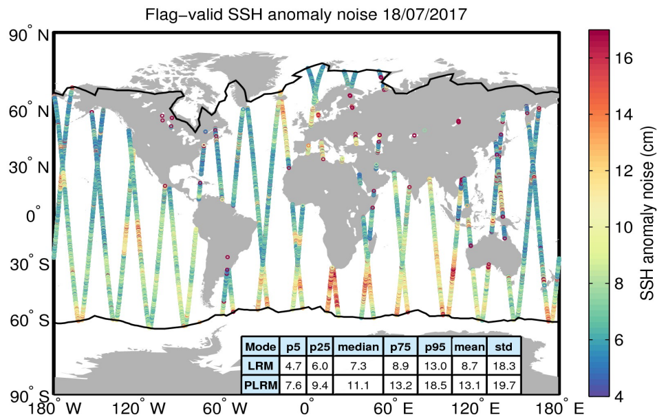
Figure 8. Geographical distribution of flag-valid 20-Hz SSH anomaly measurement noise over oceans and lakes for 18/07/2017. The statistical values shown in the table refer to the SSH anomaly noise and are calculated separately for LRM and PLRM regions. Measurements taken over polar polygons have been excluded from the computation of the statistical values. The black lines mark the outer limit of the Arctic and Antarctic polar polygons.
