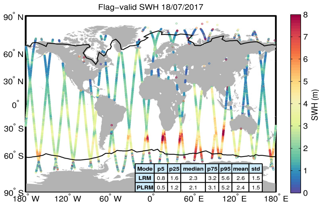
Figure 15. Geographical distribution of flag-valid SWH data over oceans and lakes for 18/07/2017. The statistical values shown in the table refer to the SWH in m and are calculated separately for LRM and PLRM regions. Measurements taken over polar polygons have been excluded from the computation of the statistical values. The black lines mark the outer limit of the Arctic and Antarctic polar polygons.
