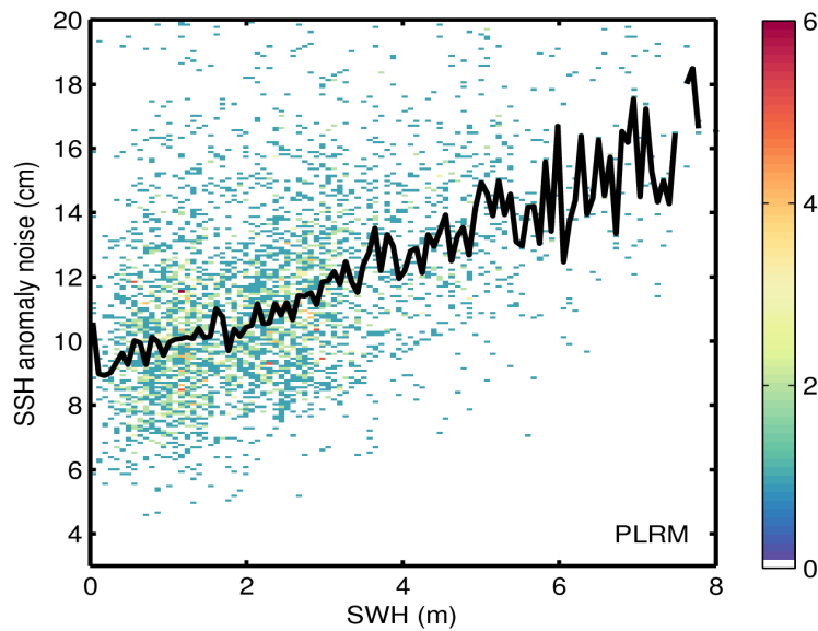
Figure 9. 2D histogram showing flag-valid SSH anomaly noise as a function of SWH for LRM (top) and PLRM (bottom) for 18/07/2017. The black line denotes the median SSH anomaly noise as a function of SWH.
