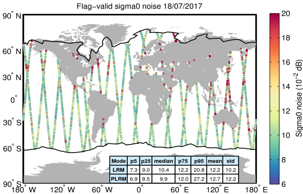
Figure 26. Geographical distribution of flag-valid 20-Hz sigma0 measurement noise over oceans and lakes for 18/07/2017. The statistical values shown in the table refer to the sigma0 noise and are calculated separately for LRM and PLRM regions. Measurements taken over polar polygons have been excluded from the computation of the statistical values. The black lines mark the outer limit of the Arctic and Antarctic polar polygons.
