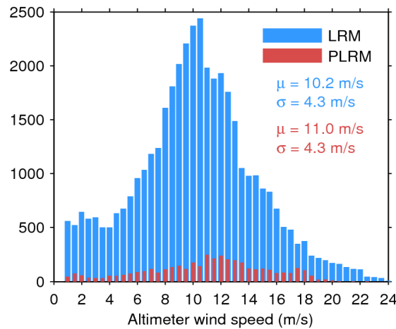
Figure 33. Histogram of flag-valid wind over oceans and lakes for LRM (blue) and PLRM (red) for 18/07/2017. The mean ( \mu ) and standard deviation ( \sigma ) are also shown. Note that values larger than 24 m/s are excluded from the histogram for the sake of readability but not from the computation of \mu and \sigma .
