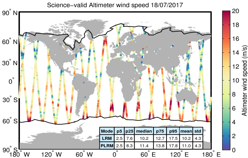
Figure 34. Geographical distribution of science-valid wind data over oceans and lakes for 18/07/2017. The statistical values shown in the table refer to the wind in m/s and are calculated separately for LRM and PLRM regions. The black lines mark the outer limit of the Arctic and Antarctic polar polygons. Gray circles denote records that have been rejected based on the editing criteria described in Table 5.
