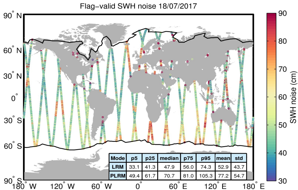
Figure 18. Geographical distribution of flag-valid 20-Hz SWH measurement noise over oceans and lakes for 18/07/2017. The statistical values shown in the table refer to the SWH noise and are calculated separately for LRM and PLRM regions. Measurements taken over polar polygons have been excluded from the computation of the statistical values. The black lines mark the outer limit of the Arctic and Antarctic polar polygons.
