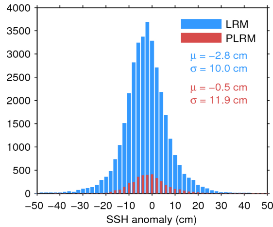
Figure 11. Histogram of science-valid SSH anomaly over oceans and lakes for LRM (blue) and PLRM (red) for 18/07/2017. The mean ( \mu ) and standard deviation ( \sigma ) are also shown. Note that values outside [-50 50] cm are excluded from the histogram for the sake of readability but not from the computation of \mu and \sigma .
