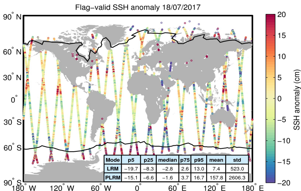
Figure 5. Geographical distribution of flag-valid 1-Hz SSH anomaly data over oceans and lakes for 18/07/2017. The statistical values shown in the table refer to the SSH anomaly in cm and are calculated separately for LRM and PLRM regions. Measurements taken over polar polygons have been excluded from the computation of the statistical values. The black lines mark the outer limit of the Arctic and Antarctic polar polygons.
