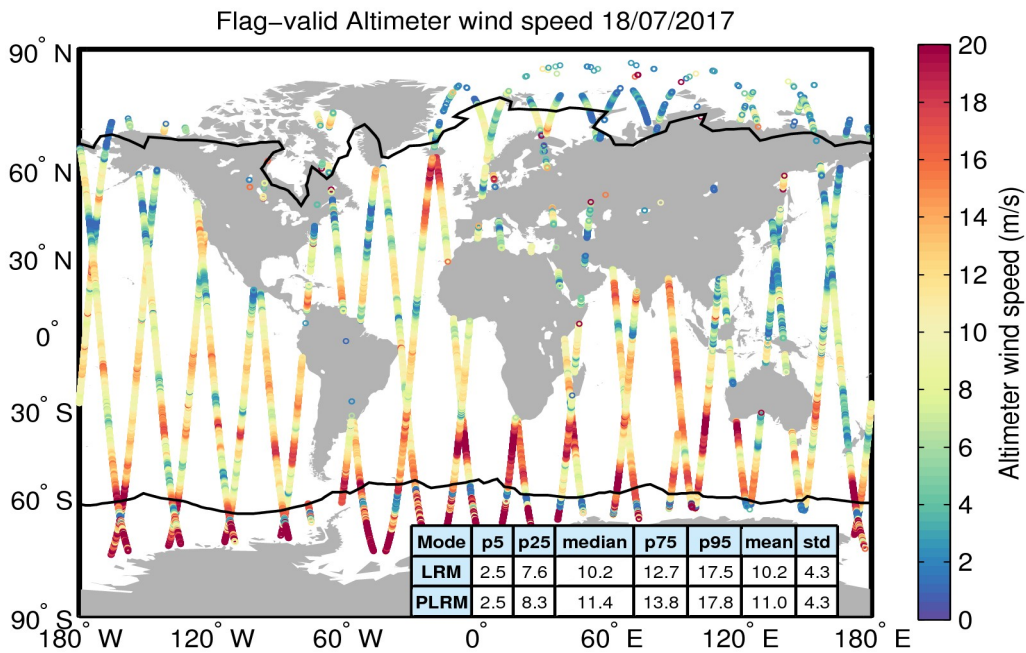
Figure 31. Geographical distribution of flag-valid wind data over oceans and lakes for 18/07/2017. The statistical values shown in the table refer to the wind in m/s and are calculated separately for LRM and PLRM regions. Measurements taken over polar polygons have been excluded from the computation of the statistical values. The black lines mark the outer limit of the Arctic and Antarctic polar polygons.
