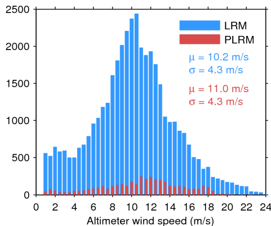
Figure 35. Histogram of science-valid wind over oceans and lakes for LRM (blue) and PLRM (red) for 18/07/2017. The mean ( \mu ) and standard deviation ( \sigma ) are also shown. Note that values larger than 24 m/s are excluded from the histogram for the sake of readability but not from the computation of \mu and \sigma .
