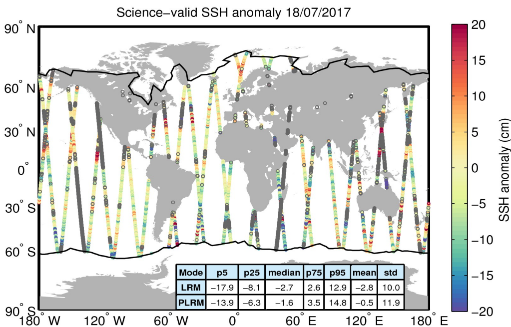
Figure 10. Geographical distribution of science-valid SSH anomaly data over oceans and lakes for 18/07/2017. The statistical values shown in the table refer to the SSH anomaly in cm and are calculated separately for LRM and PLRM regions. The black lines mark the outer limit of the Arctic and Antarctic polar polygons. Gray circles denote records that have been rejected based on the editing criteria described in Table 2.
