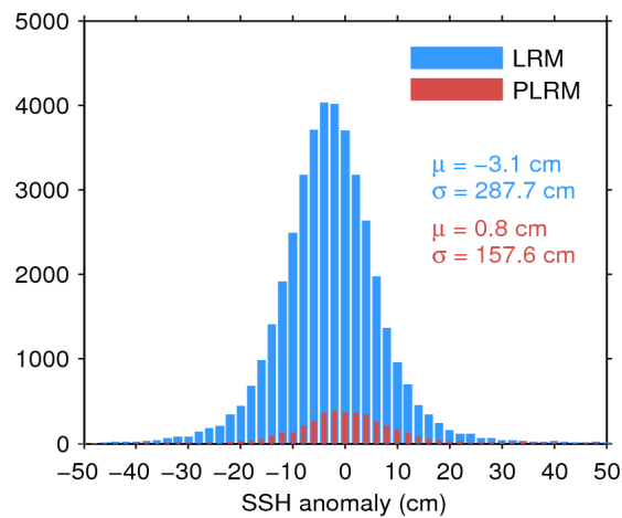
Figure 7. Histogram of flag-valid SSH anomaly over oceans and lakes for LRM (blue) and PLRM (red) for 17/07/2017. The mean ( \mu ) and standard deviation ( \sigma ) are also shown. Note that values outside [-50\ 50] cm are excluded from the histogram for the sake of readability but not from the computation of \mu and \sigma .
