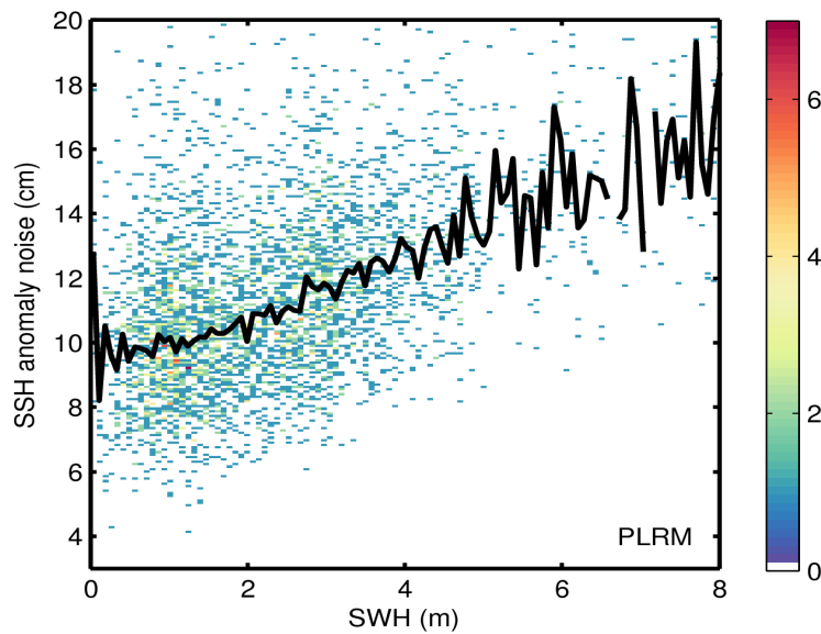
Figure 9. 2D histogram showing flag-valid SSH anomaly noise as a function of SWH for LRM (top) and PLRM (bottom) for 17/07/2017. The black line denotes the median SSH anomaly noise as a function of SWH.
