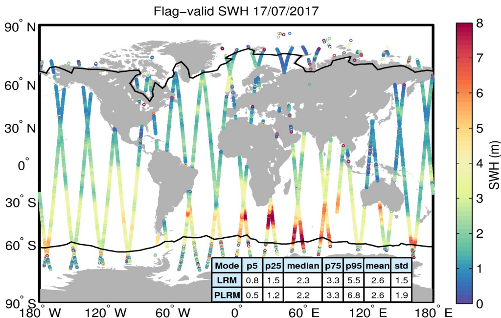
Figure 15. Geographical distribution of flag-valid SWH data over oceans and lakes for 17/07/2017. The statistical values shown in the table refer to the SWH in m and are calculated separately for LRM and PLRM regions. Measurements taken over polar polygons have been excluded from the computation of the statistical values. The black lines mark the outer limit of the Arctic and Antarctic polar polygons.
