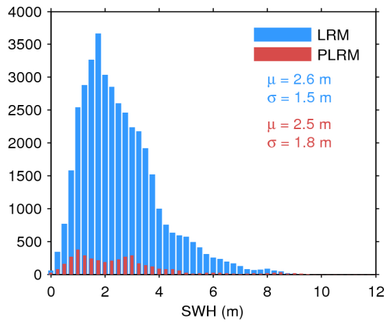
Figure 20. Histogram of science-valid SWH over oceans and lakes for LRM (blue) and PLRM (red) for 17/07/2017. The mean ( \mu ) and standard deviation ( \sigma ) are also shown. Note that values larger than 12 m are excluded from the histogram for the sake of readability but not from the computation of \mu and \sigma .
