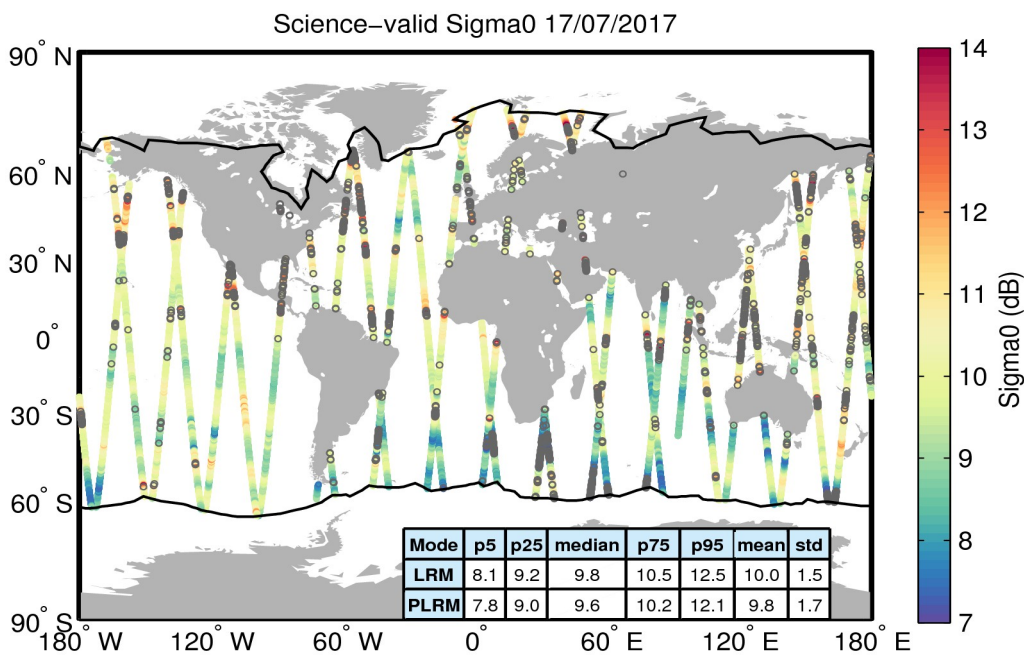
Figure 27. Geographical distribution of science-valid sigma0 data over oceans and lakes for 17/07/2017. The statistical values shown in the table refer to the sigma0 in dB and are calculated separately for LRM and PLRM regions. The black lines mark the outer limit of the Arctic and Antarctic polar polygons. Gray circles denote records that have been rejected based on the editing criteria described in Table 4.
