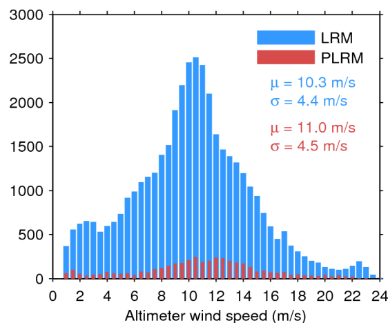
Figure 35. Histogram of science-valid wind over oceans and lakes for LRM (blue) and PLRM (red) for 17/07/2017. The mean ( \mu ) and standard deviation ( \sigma ) are also shown. Note that values larger than 24 m/s are excluded from the histogram for the sake of readability but not from the computation of \mu and \sigma .
