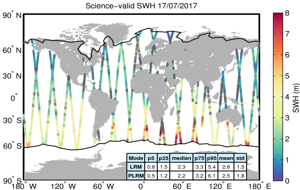
Figure 19. Geographical distribution of science-valid SWH data over oceans and lakes for 17/07/2017. The statistical values shown in the table refer to the SWH in m and are calculated separately for LRM and PLRM regions. The black lines mark the outer limit of the Arctic and Antarctic polar polygons. Gray circles denote records that have been rejected based on the editing criteria described in Table 3.
