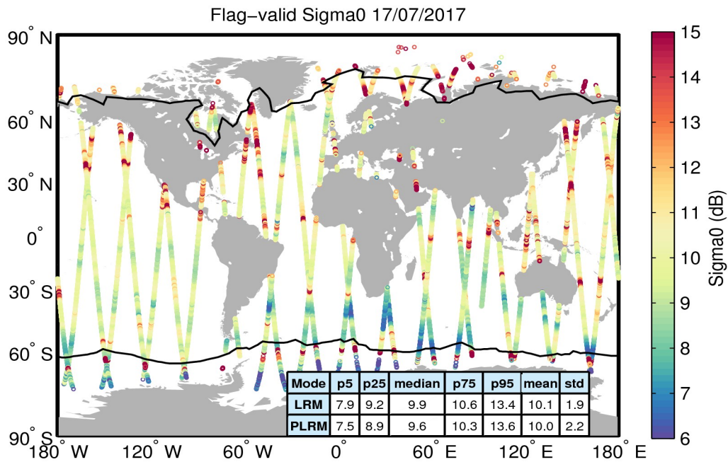
Figure 23. Geographical distribution of flag-valid sigma0 data over oceans and lakes for 17/07/2017. The statistical values shown in the table refer to the sigma0 in dB and are calculated separately for LRM and PLRM regions. Measurements taken over polar polygons have been excluded from the computation of the statistical values. The black lines mark the outer limit of the Arctic and Antarctic polar polygons.
