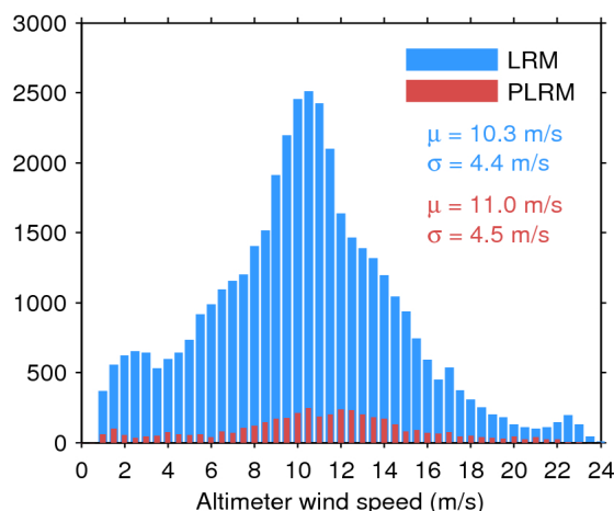
Figure 33. Histogram of flag-valid wind over oceans and lakes for LRM (blue) and PLRM (red) for 17/07/2017. The mean ( \mu ) and standard deviation ( \sigma ) are also shown. Note that values larger than 24 m/s are excluded from the histogram for the sake of readability but not from the computation of \mu and \sigma .
