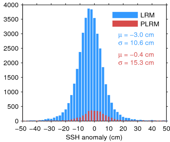
Figure 11. Histogram of science-valid SSH anomaly over oceans and lakes for LRM (blue) and PLRM (red) for 17/07/2017. The mean ( \mu ) and standard deviation ( \sigma ) are also shown. Note that values outside [-50 50] cm are excluded from the histogram for the sake of readability but not from the computation of \mu and \sigma .
