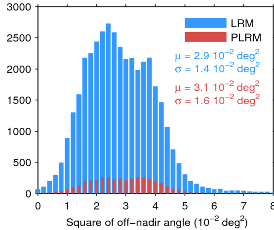
Figure 39. Histogram of flag-valid mispointing over oceans and lakes for LRM (blue) and PLRM (red) for 17/07/2017. Only positive values have been considered. The mean ( \mu ) and standard deviation ( \sigma ) are also shown. Note that values larger than 8 \cdot 10^{-2} \text{ deg}^2 are excluded from the histogram for the sake of readability but not from the computation of \mu and \sigma .
