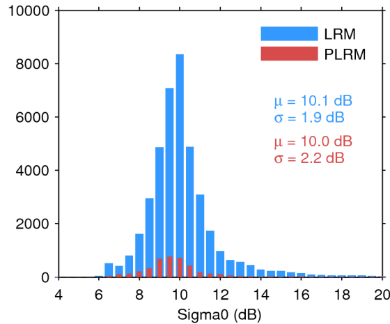
Figure 25. Histogram of flag-valid sigma0 over oceans and lakes for LRM (blue) and PLRM (red) for 17/07/2017. The mean ( \mu ) and standard deviation ( \sigma ) are also shown. Note that values outside [4 20] dB are excluded from the histogram for the sake of readability but not from the computation of \mu and \sigma .
