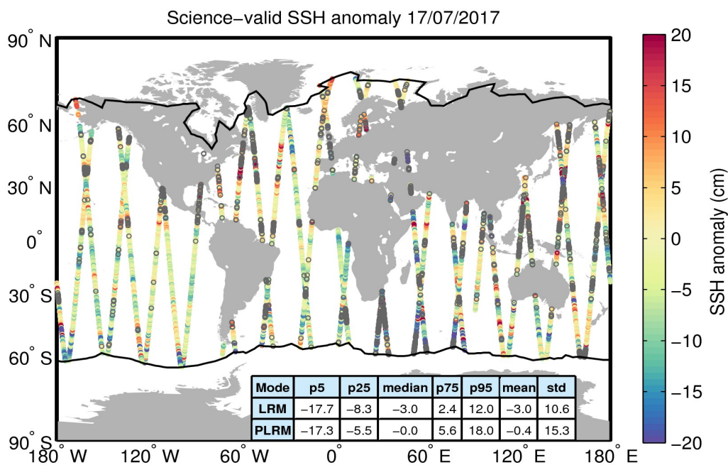
Figure 10. Geographical distribution of science-valid SSH anomaly data over oceans and lakes for 17/07/2017. The statistical values shown in the table refer to the SSH anomaly in cm and are calculated separately for LRM and PLRM regions. The black lines mark the outer limit of the Arctic and Antarctic polar polygons. Gray circles denote records that have been rejected based on the editing criteria described in Table 2.
