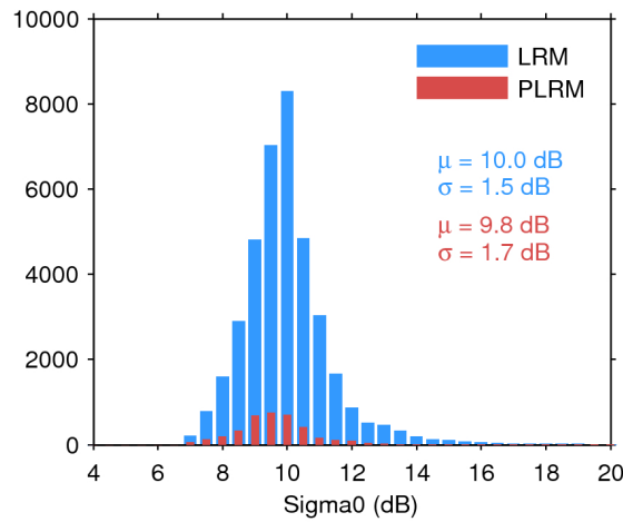
Figure 28. Histogram of science-valid sigma0 over oceans and lakes for LRM (blue) and PLRM (red) for 17/07/2017. The mean ( \mu ) and standard deviation ( \sigma ) are also shown. Note that values outside [4 20] dB are excluded from the histogram for the sake of readability but not from the computation of \mu and \sigma .
