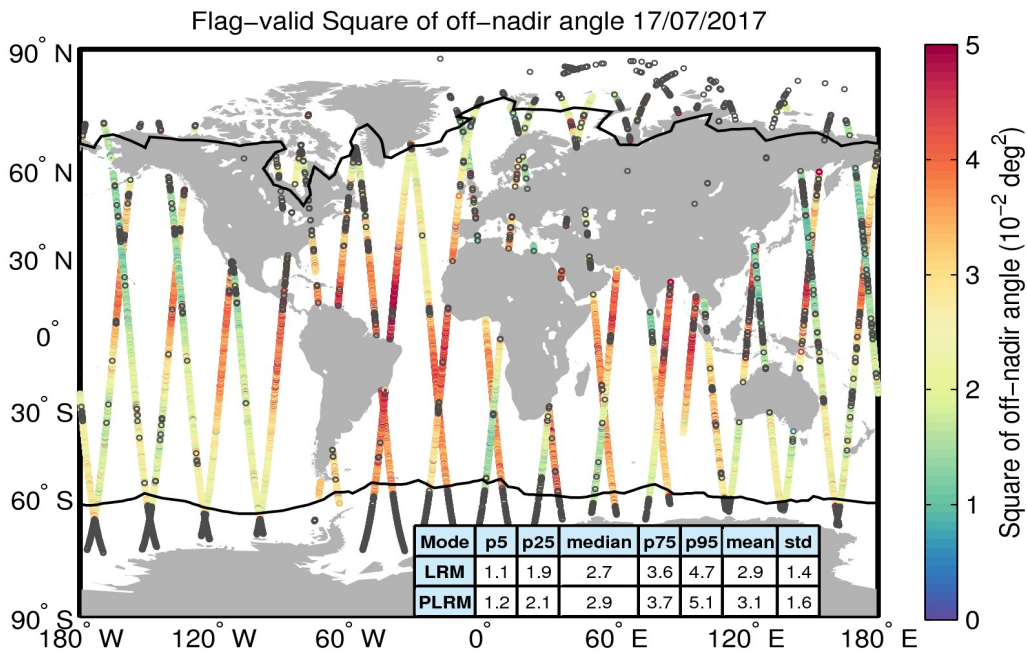
Figure 37. Geographical distribution of flag-valid mispointing data over oceans and lakes for 17/07/2017. The statistical values shown in the table refer to the mispointing in 10^{-2} deg 2 and are calculated separately for LRM and PLRM regions. Measurements taken over polar polygons have been excluded from the computation of the statistical values. The black lines mark the outer limit of the Arctic and Antarctic polar polygons. Gray circles denote negative values.
