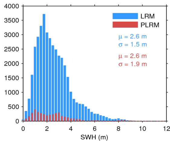
Figure 17. Histogram of flag-valid SWH over oceans and lakes for LRM (blue) and PLRM (red) for 17/07/2017. The mean ( \mu ) and standard deviation ( \sigma ) are also shown. Note that values larger than 12 m are excluded from the histogram for the sake of readability but not from the computation of \mu and \sigma .
