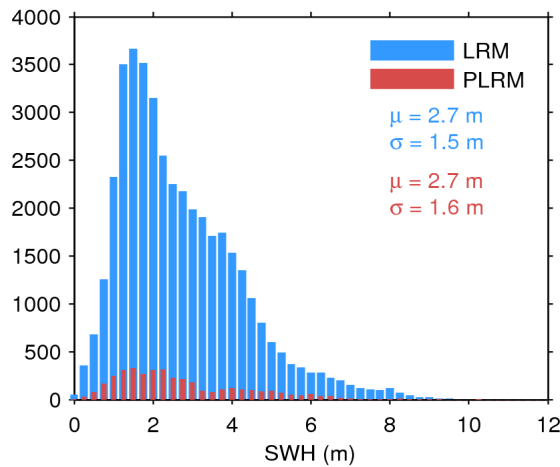
Figure 20. Histogram of science-valid SWH over oceans and lakes for LRM (blue) and PLRM (red) for 16/07/2017. The mean ( \mu ) and standard deviation ( \sigma ) are also shown. Note that values larger than 12 m are excluded from the histogram for the sake of readability but not from the computation of \mu and \sigma .
