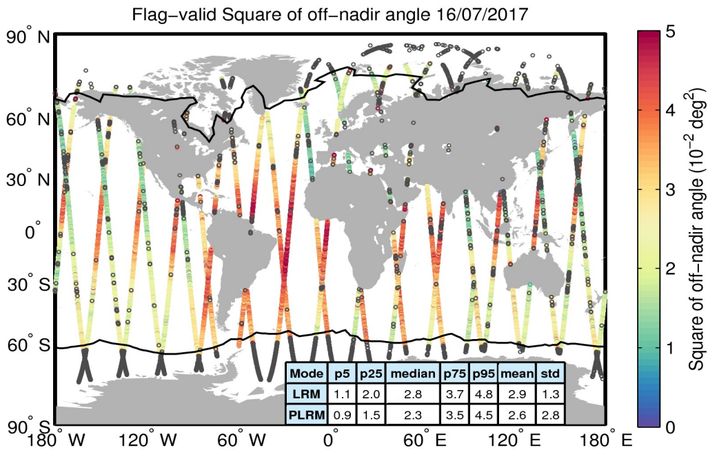
Figure 37. Geographical distribution of flag-valid mispointing data over oceans and lakes for 16/07/2017. The statistical values shown in the table refer to the mispointing in 10^{-2} \text{ deg}^2 and are calculated separately for LRM and PLRM regions. Measurements taken over polar polygons have been excluded from the computation of the statistical values. The black lines mark the outer limit of the Arctic and Antarctic polar polygons. Gray circles denote negative values.
