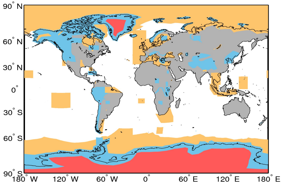
Figure A1. Extent of the regions defining the geographical mode mask for 16/07/2017. The regions where SAR, and SARIn are operated are denoted by the orange and blue polygons, respectively. LRM is operated over areas of the continental ice sheets (red polygons) and over oceans and land not covered by other modes.
