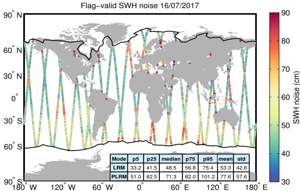
Figure 18. Geographical distribution of flag-valid 20-Hz SWH measurement noise over oceans and lakes for 16/07/2017. The statistical values shown in the table refer to the SWH noise and are calculated separately for LRM and PLRM regions. Measurements taken over polar polygons have been excluded from the computation of the statistical values. The black lines mark the outer limit of the Arctic and Antarctic polar polygons.
