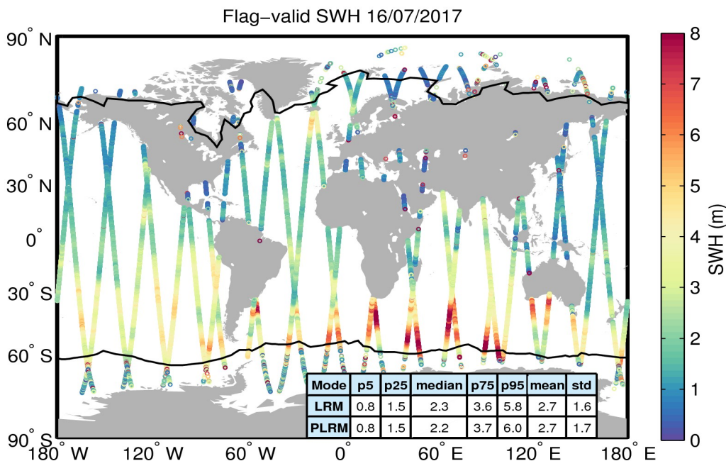
Figure 15. Geographical distribution of flag-valid SWH data over oceans and lakes for 16/07/2017. The statistical values shown in the table refer to the SWH in m and are calculated separately for LRM and PLRM regions. Measurements taken over polar polygons have been excluded from the computation of the statistical values. The black lines mark the outer limit of the Arctic and Antarctic polar polygons.
