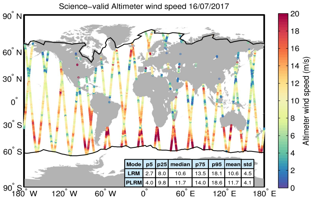
Figure 34. Geographical distribution of science-valid wind data over oceans and lakes for 16/07/2017. The statistical values shown in the table refer to the wind in m/s and are calculated separately for LRM and PLRM regions. The black lines mark the outer limit of the Arctic and Antarctic polar polygons. Gray circles denote records that have been rejected based on the editing criteria described in Table 5.
