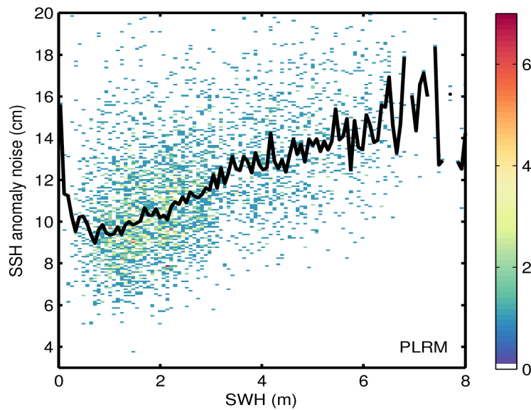
Figure 9. 2D histogram showing flag-valid SSH anomaly noise as a function of SWH for LRM (top) and PLRM (bottom) for 16/07/2017. The black line denotes the median SSH anomaly noise as a function of SWH.
