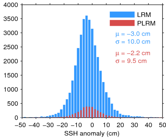
Figure 11. Histogram of science-valid SSH anomaly over oceans and lakes for LRM (blue) and PLRM (red) for 16/07/2017. The mean ( \mu ) and standard deviation ( \sigma ) are also shown. Note that values outside [-50\ 50] cm are excluded from the histogram for the sake of readability but not from the computation of \mu and \sigma .
