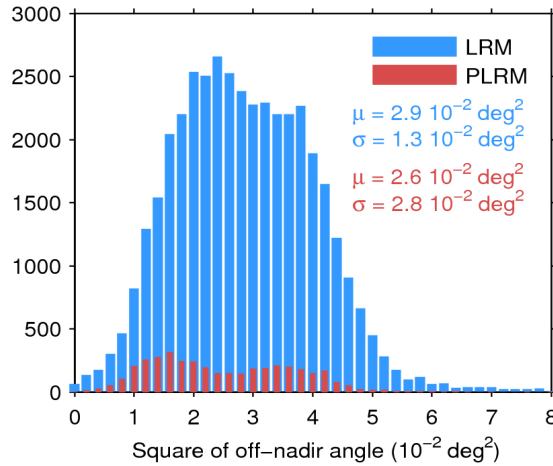
Figure 39. Histogram of flag-valid mispointing over oceans and lakes for LRM (blue) and PLRM (red) for 16/07/2017. Only positive values have been considered. The mean ( \mu ) and standard deviation ( \sigma ) are also shown. Note that values larger than 8 \cdot 10^{-2} \text{ deg}^2 are excluded from the histogram for the sake of readability but not from the computation of \mu and \sigma .
