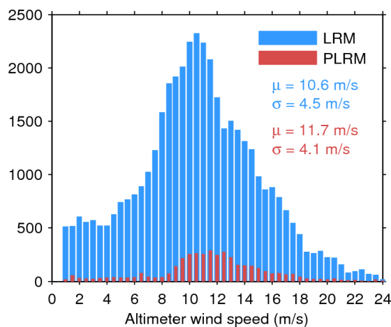
Figure 33. Histogram of flag-valid wind over oceans and lakes for LRM (blue) and PLRM (red) for 16/07/2017. The mean ( \mu ) and standard deviation ( \sigma ) are also shown. Note that values larger than 24 m/s are excluded from the histogram for the sake of readability but not from the computation of \mu and \sigma .
