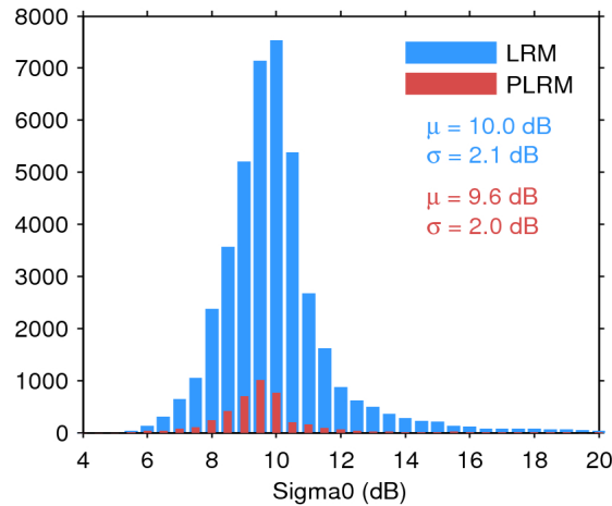
Figure 25. Histogram of flag-valid sigma0 over oceans and lakes for LRM (blue) and PLRM (red) for 16/07/2017. The mean ( \mu ) and standard deviation ( \sigma ) are also shown. Note that values outside [4 20] dB are excluded from the histogram for the sake of readability but not from the computation of \mu and \sigma .
