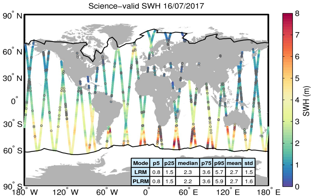
Figure 19. Geographical distribution of science-valid SWH data over oceans and lakes for 16/07/2017. The statistical values shown in the table refer to the SWH in m and are calculated separately for LRM and PLRM regions. The black lines mark the outer limit of the Arctic and Antarctic polar polygons. Gray circles denote records that have been rejected based on the editing criteria described in Table 3.
