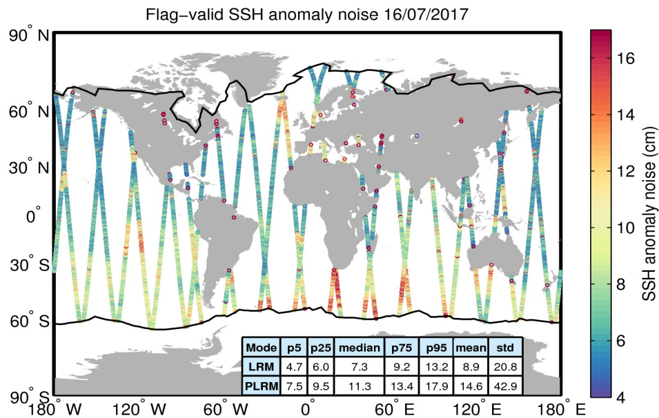
Figure 8. Geographical distribution of flag-valid 20-Hz SSH anomaly measurement noise over oceans and lakes for 16/07/2017. The statistical values shown in the table refer to the SSH anomaly noise and are calculated separately for LRM and PLRM regions. Measurements taken over polar polygons have been excluded from the computation of the statistical values. The black lines mark the outer limit of the Arctic and Antarctic polar polygons.
