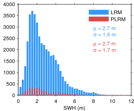
Figure 17. Histogram of flag-valid SWH over oceans and lakes for LRM (blue) and PLRM (red) for 16/07/2017. The mean ( \mu ) and standard deviation ( \sigma ) are also shown. Note that values larger than 12 m are excluded from the histogram for the sake of readability but not from the computation of \mu and \sigma .
