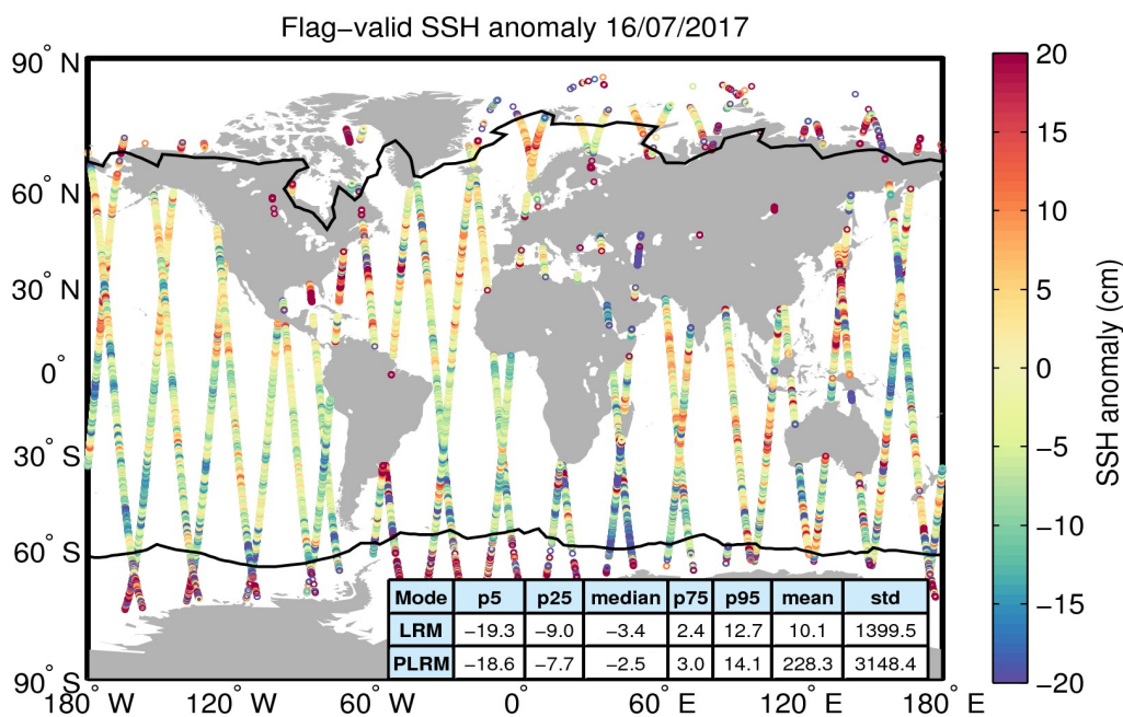
Figure 5. Geographical distribution of flag-valid 1-Hz SSH anomaly data over oceans and lakes for 16/07/2017. The statistical values shown in the table refer to the SSH anomaly in cm and are calculated separately for LRM and PLRM regions. Measurements taken over polar polygons have been excluded from the computation of the statistical values. The black lines mark the outer limit of the Arctic and Antarctic polar polygons.
