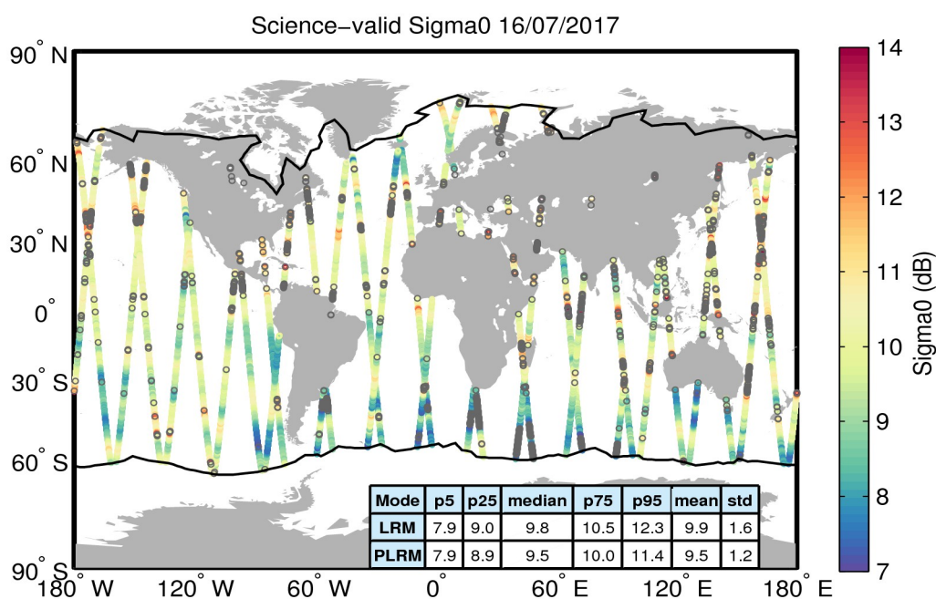
Figure 27. Geographical distribution of science-valid sigma0 data over oceans and lakes for 16/07/2017. The statistical values shown in the table refer to the sigma0 in dB and are calculated separately for LRM and PLRM regions. The black lines mark the outer limit of the Arctic and Antarctic polar polygons. Gray circles denote records that have been rejected based on the editing criteria described in Table 4.
