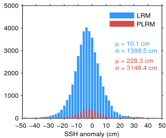
Figure 7. Histogram of flag-valid SSH anomaly over oceans and lakes for LRM (blue) and PLRM (red) for 16/07/2017. The mean ( \mu ) and standard deviation ( \sigma ) are also shown. Note that values outside [-50\ 50] cm are excluded from the histogram for the sake of readability but not from the computation of \mu and \sigma .
