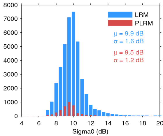
Figure 28. Histogram of science-valid sigma0 over oceans and lakes for LRM (blue) and PLRM (red) for 16/07/2017. The mean ( \mu ) and standard deviation ( \sigma ) are also shown. Note that values outside [4 20] dB are excluded from the histogram for the sake of readability but not from the computation of \mu and \sigma .
