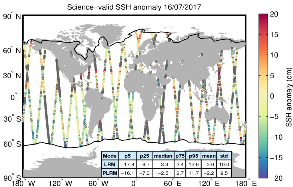
Figure 10. Geographical distribution of science-valid SSH anomaly data over oceans and lakes for 16/07/2017. The statistical values shown in the table refer to the SSH anomaly in cm and are calculated separately for LRM and PLRM regions. The black lines mark the outer limit of the Arctic and Antarctic polar polygons. Gray circles denote records that have been rejected based on the editing criteria described in Table 2.
