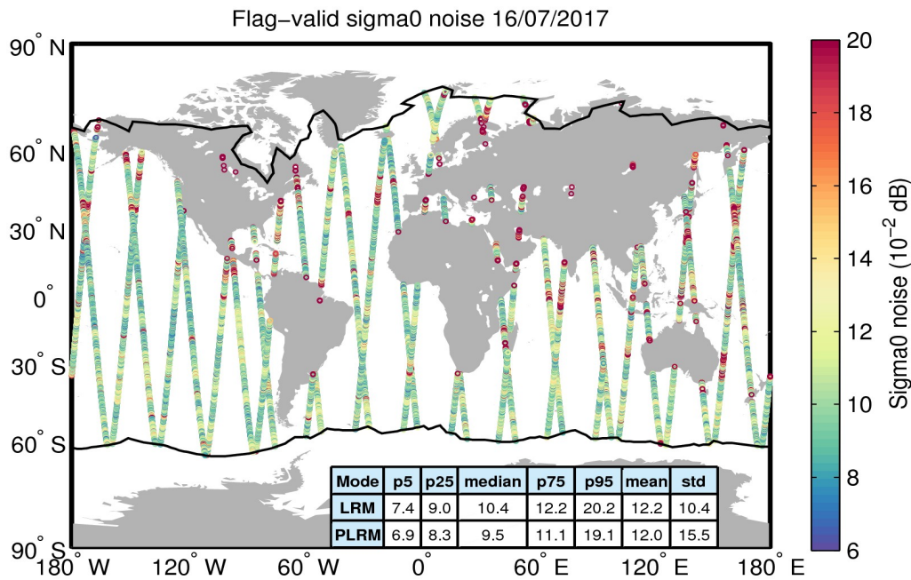
Figure 26. Geographical distribution of flag-valid 20-Hz sigma0 measurement noise over oceans and lakes for 16/07/2017. The statistical values shown in the table refer to the sigma0 noise and are calculated separately for LRM and PLRM regions. Measurements taken over polar polygons have been excluded from the computation of the statistical values. The black lines mark the outer limit of the Arctic and Antarctic polar polygons.
