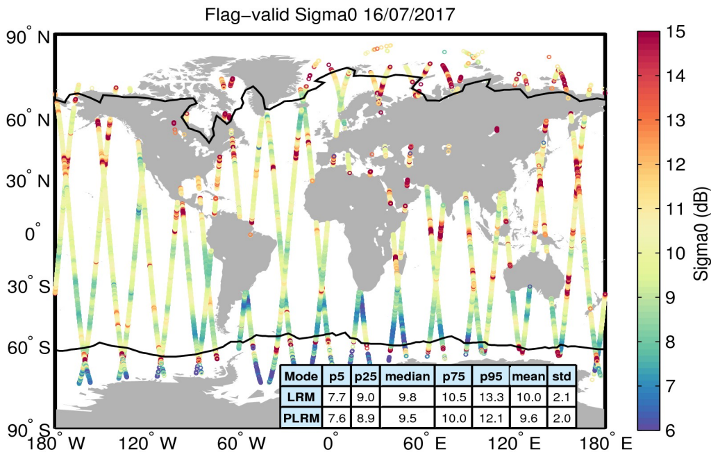
Figure 23. Geographical distribution of flag-valid sigma0 data over oceans and lakes for 16/07/2017. The statistical values shown in the table refer to the sigma0 in dB and are calculated separately for LRM and PLRM regions. Measurements taken over polar polygons have been excluded from the computation of the statistical values. The black lines mark the outer limit of the Arctic and Antarctic polar polygons.
