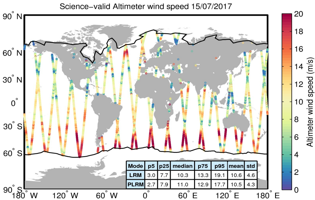
Figure 34. Geographical distribution of science-valid wind data over oceans and lakes for 15/07/2017. The statistical values shown in the table refer to the wind in m/s and are calculated separately for LRM and PLRM regions. The black lines mark the outer limit of the Arctic and Antarctic polar polygons. Gray circles denote records that have been rejected based on the editing criteria described in Table 5.
