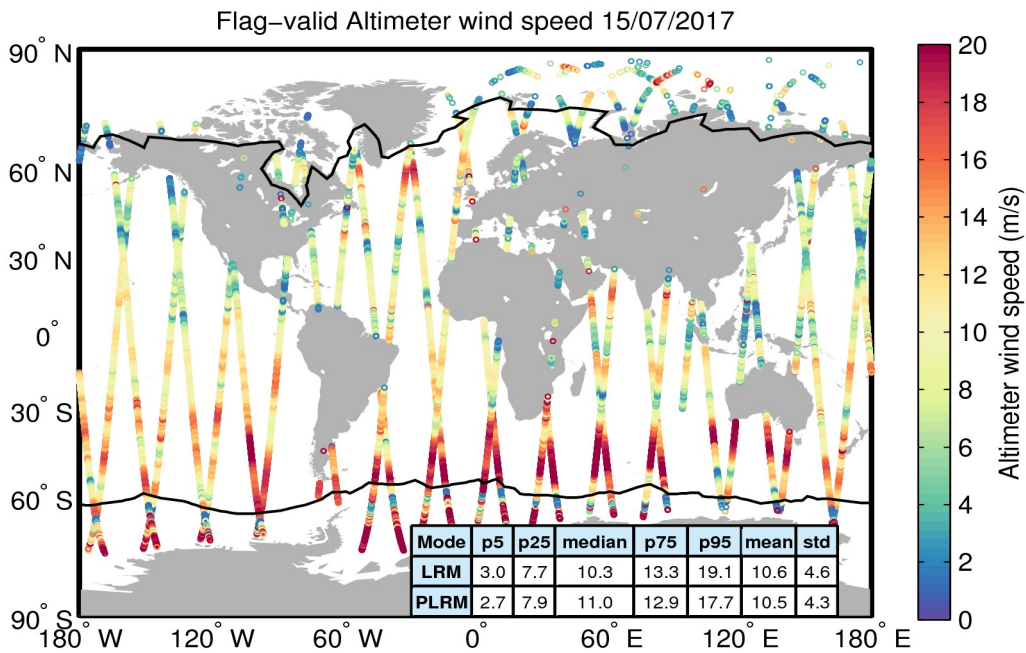
Figure 31. Geographical distribution of flag-valid wind data over oceans and lakes for 15/07/2017. The statistical values shown in the table refer to the wind in m/s and are calculated separately for LRM and PLRM regions. Measurements taken over polar polygons have been excluded from the computation of the statistical values. The black lines mark the outer limit of the Arctic and Antarctic polar polygons.
