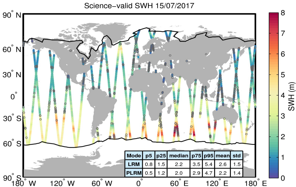
Figure 19. Geographical distribution of science-valid SWH data over oceans and lakes for 15/07/2017. The statistical values shown in the table refer to the SWH in m and are calculated separately for LRM and PLRM regions. The black lines mark the outer limit of the Arctic and Antarctic polar polygons. Gray circles denote records that have been rejected based on the editing criteria described in Table 3.
