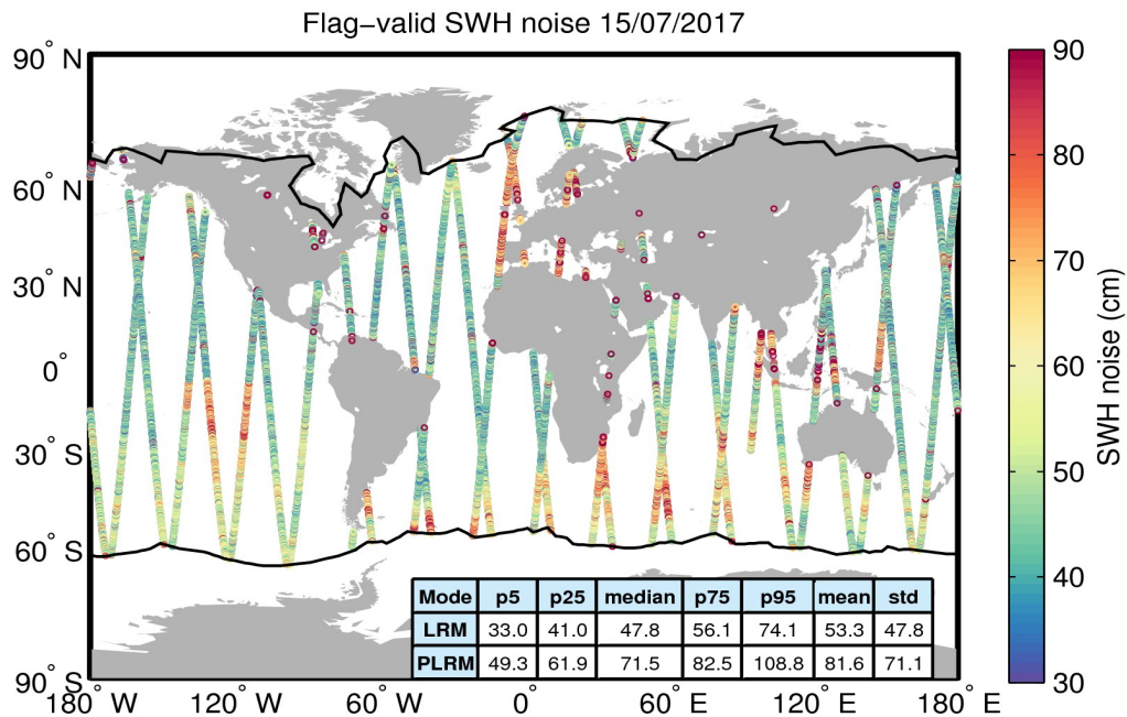
Figure 18. Geographical distribution of flag-valid 20-Hz SWH measurement noise over oceans and lakes for 15/07/2017. The statistical values shown in the table refer to the SWH noise and are calculated separately for LRM and PLRM regions. Measurements taken over polar polygons have been excluded from the computation of the statistical values. The black lines mark the outer limit of the Arctic and Antarctic polar polygons.
