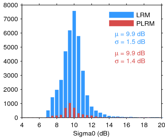
Figure 28. Histogram of science-valid sigma0 over oceans and lakes for LRM (blue) and PLRM (red) for 15/07/2017. The mean ( \mu ) and standard deviation ( \sigma ) are also shown. Note that values outside [4 20] dB are excluded from the histogram for the sake of readability but not from the computation of \mu and \sigma .
