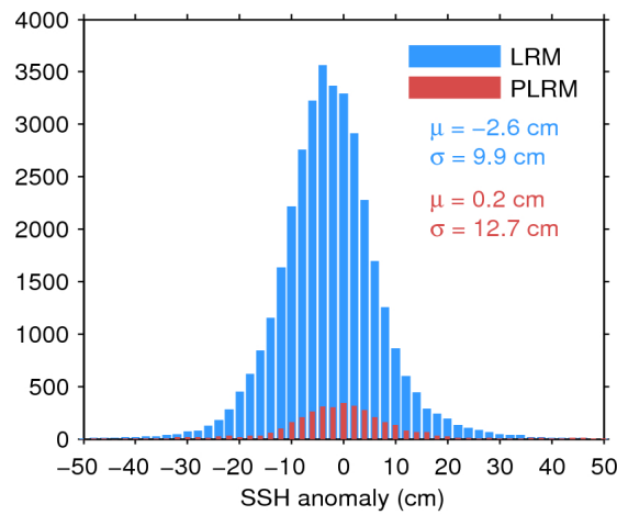
Figure 11. Histogram of science-valid SSH anomaly over oceans and lakes for LRM (blue) and PLRM (red) for 15/07/2017. The mean ( \mu ) and standard deviation ( \sigma ) are also shown. Note that values outside [-50 50] cm are excluded from the histogram for the sake of readability but not from the computation of \mu and \sigma .
