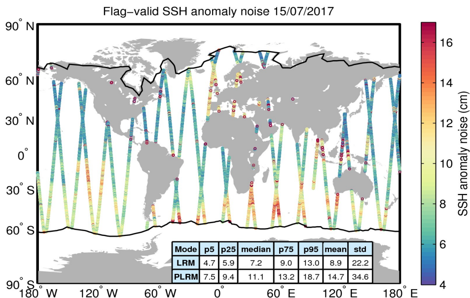
Figure 8. Geographical distribution of flag-valid 20-Hz SSH anomaly measurement noise over oceans and lakes for 15/07/2017. The statistical values shown in the table refer to the SSH anomaly noise and are calculated separately for LRM and PLRM regions. Measurements taken over polar polygons have been excluded from the computation of the statistical values. The black lines mark the outer limit of the Arctic and Antarctic polar polygons.
