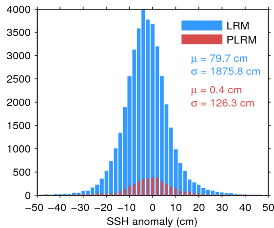
Figure 7. Histogram of flag-valid SSH anomaly over oceans and lakes for LRM (blue) and PLRM (red) for 15/07/2017. The mean ( \mu ) and standard deviation ( \sigma ) are also shown. Note that values outside [-50 50] cm are excluded from the histogram for the sake of readability but not from the computation of \mu and \sigma .
