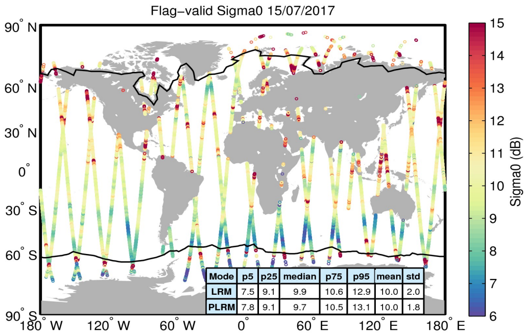
Figure 23. Geographical distribution of flag-valid sigma0 data over oceans and lakes for 15/07/2017. The statistical values shown in the table refer to the sigma0 in dB and are calculated separately for LRM and PLRM regions. Measurements taken over polar polygons have been excluded from the computation of the statistical values. The black lines mark the outer limit of the Arctic and Antarctic polar polygons.
