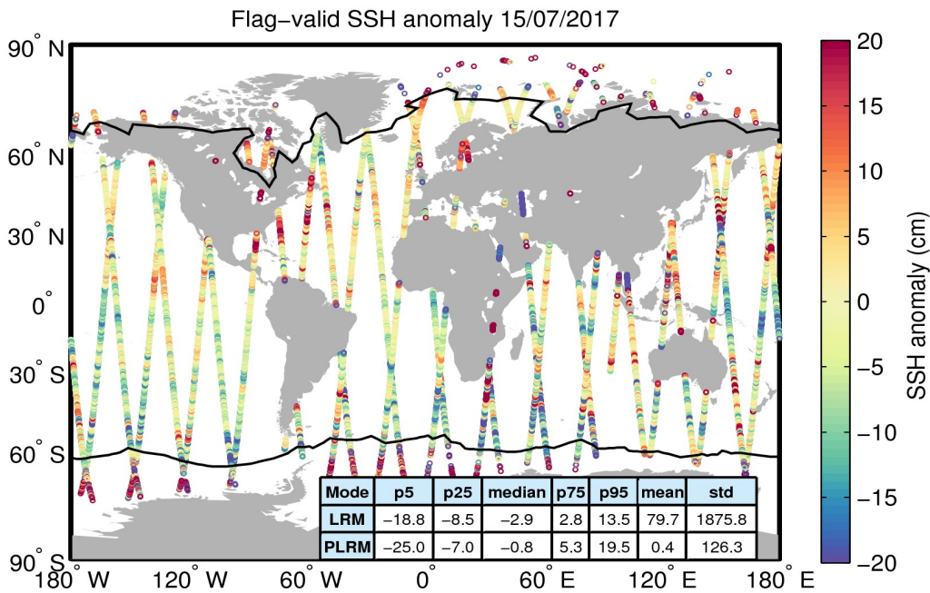
Figure 5. Geographical distribution of flag-valid 1-Hz SSH anomaly data over oceans and lakes for 15/07/2017. The statistical values shown in the table refer to the SSH anomaly in cm and are calculated separately for LRM and PLRM regions. Measurements taken over polar polygons have been excluded from the computation of the statistical values. The black lines mark the outer limit of the Arctic and Antarctic polar polygons.
