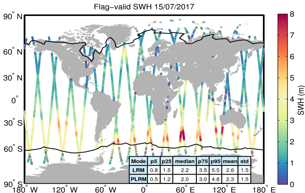
Figure 15. Geographical distribution of flag-valid SWH data over oceans and lakes for 15/07/2017. The statistical values shown in the table refer to the SWH in m and are calculated separately for LRM and PLRM regions. Measurements taken over polar polygons have been excluded from the computation of the statistical values. The black lines mark the outer limit of the Arctic and Antarctic polar polygons.
