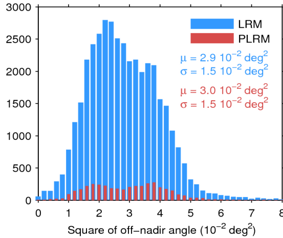
Figure 39. Histogram of flag-valid mispointing over oceans and lakes for LRM (blue) and PLRM (red) for 15/07/2017. Only positive values have been considered. The mean ( \mu ) and standard deviation ( \sigma ) are also shown. Note that values larger than 8 \cdot 10^{-2} \text{ deg}^2 are excluded from the histogram for the sake of readability but not from the computation of \mu and \sigma .
