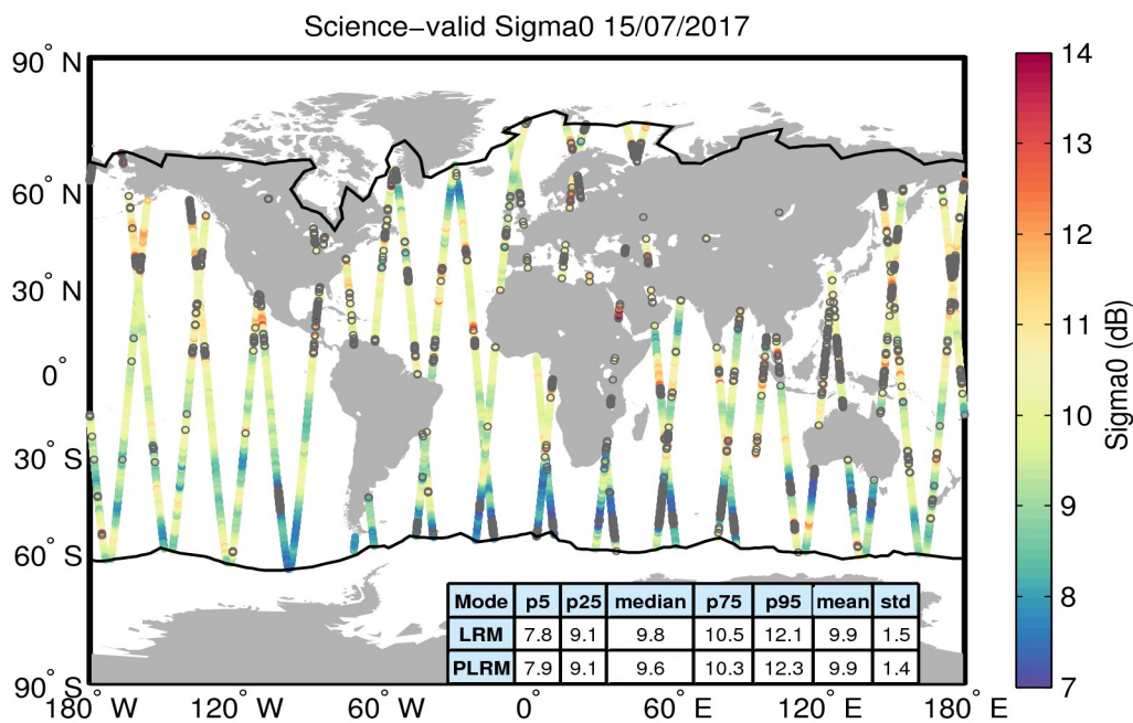
Figure 27. Geographical distribution of science-valid sigma0 data over oceans and lakes for 15/07/2017. The statistical values shown in the table refer to the sigma0 in dB and are calculated separately for LRM and PLRM regions. The black lines mark the outer limit of the Arctic and Antarctic polar polygons. Gray circles denote records that have been rejected based on the editing criteria described in Table 4.
