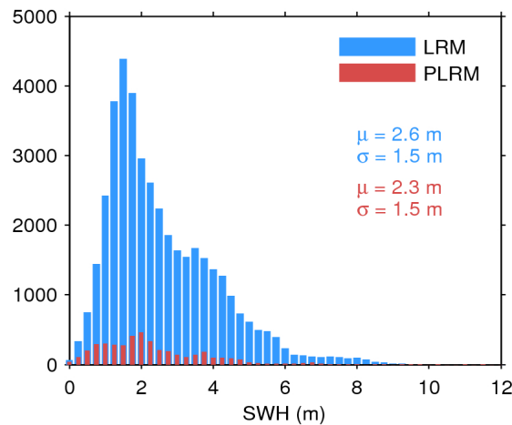
Figure 17. Histogram of flag-valid SWH over oceans and lakes for LRM (blue) and PLRM (red) for 15/07/2017. The mean ( \mu ) and standard deviation ( \sigma ) are also shown. Note that values larger than 12 m are excluded from the histogram for the sake of readability but not from the computation of \mu and \sigma .
