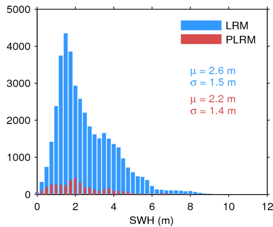
Figure 20. Histogram of science-valid SWH over oceans and lakes for LRM (blue) and PLRM (red) for 15/07/2017. The mean ( \mu ) and standard deviation ( \sigma ) are also shown. Note that values larger than 12 m are excluded from the histogram for the sake of readability but not from the computation of \mu and \sigma .
