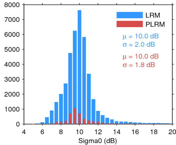
Figure 25. Histogram of flag-valid sigma0 over oceans and lakes for LRM (blue) and PLRM (red) for 15/07/2017. The mean ( \mu ) and standard deviation ( \sigma ) are also shown. Note that values outside [4 20] dB are excluded from the histogram for the sake of readability but not from the computation of \mu and \sigma .
