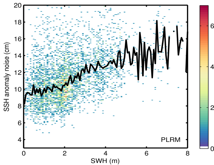
Figure 9. 2D histogram showing flag-valid SSH anomaly noise as a function of SWH for LRM (top) and PLRM (bottom) for 15/07/2017. The black line denotes the median SSH anomaly noise as a function of SWH.
