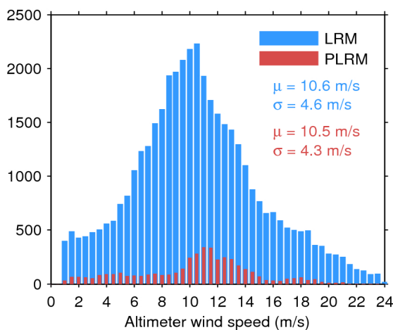
Figure 33. Histogram of flag-valid wind over oceans and lakes for LRM (blue) and PLRM (red) for 15/07/2017. The mean ( \mu ) and standard deviation ( \sigma ) are also shown. Note that values larger than 24 m/s are excluded from the histogram for the sake of readability but not from the computation of \mu and \sigma .
