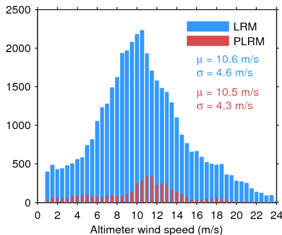
Figure 35. Histogram of science-valid wind over oceans and lakes for LRM (blue) and PLRM (red) for 15/07/2017. The mean ( \mu ) and standard deviation ( \sigma ) are also shown. Note that values larger than 24 m/s are excluded from the histogram for the sake of readability but not from the computation of \mu and \sigma .
