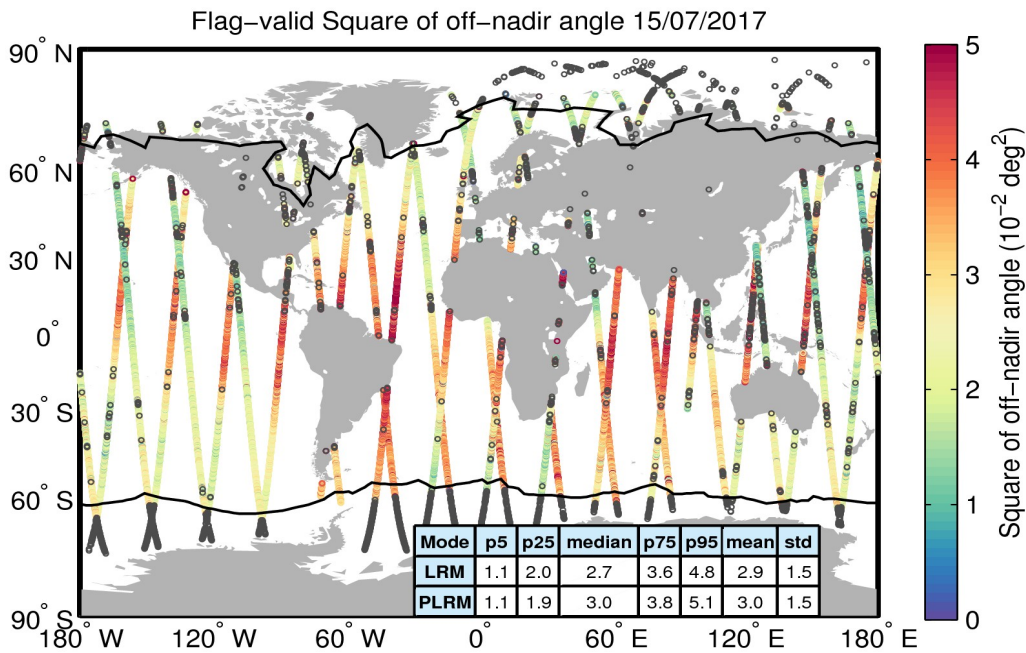
Figure 37. Geographical distribution of flag-valid mispointing data over oceans and lakes for 15/07/2017. The statistical values shown in the table refer to the mispointing in 10^{-2} deg 2 and are calculated separately for LRM and PLRM regions. Measurements taken over polar polygons have been excluded from the computation of the statistical values. The black lines mark the outer limit of the Arctic and Antarctic polar polygons. Gray circles denote negative values.
