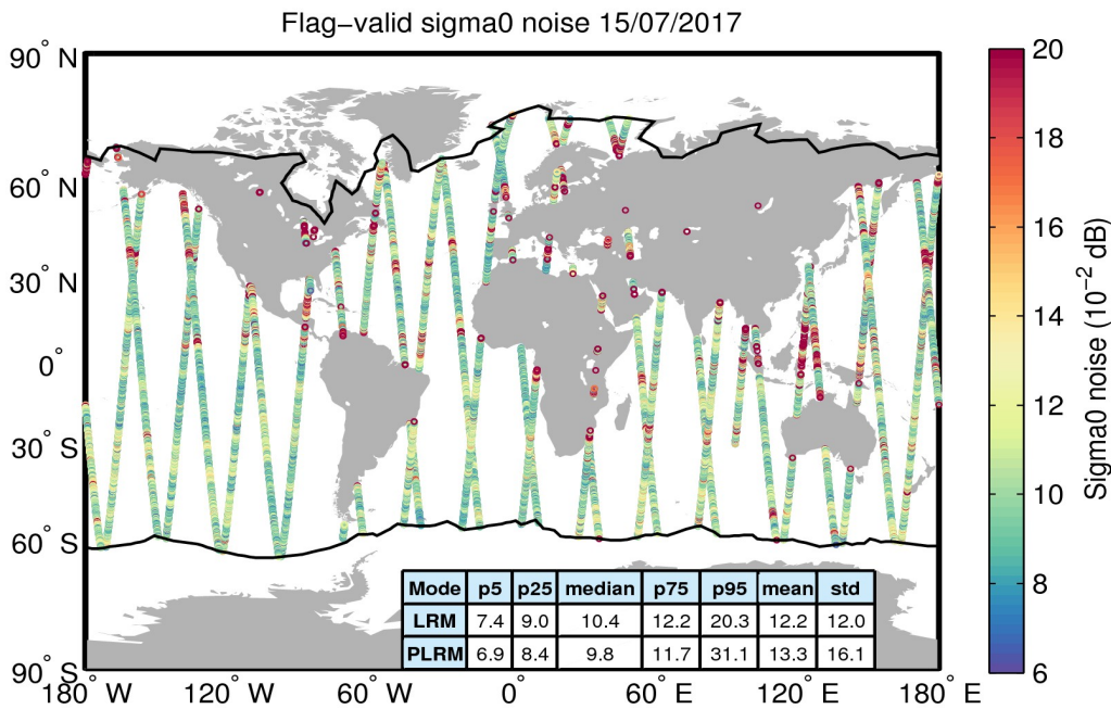
Figure 26. Geographical distribution of flag-valid 20-Hz sigma0 measurement noise over oceans and lakes for 15/07/2017. The statistical values shown in the table refer to the sigma0 noise and are calculated separately for LRM and PLRM regions. Measurements taken over polar polygons have been excluded from the computation of the statistical values. The black lines mark the outer limit of the Arctic and Antarctic polar polygons.
