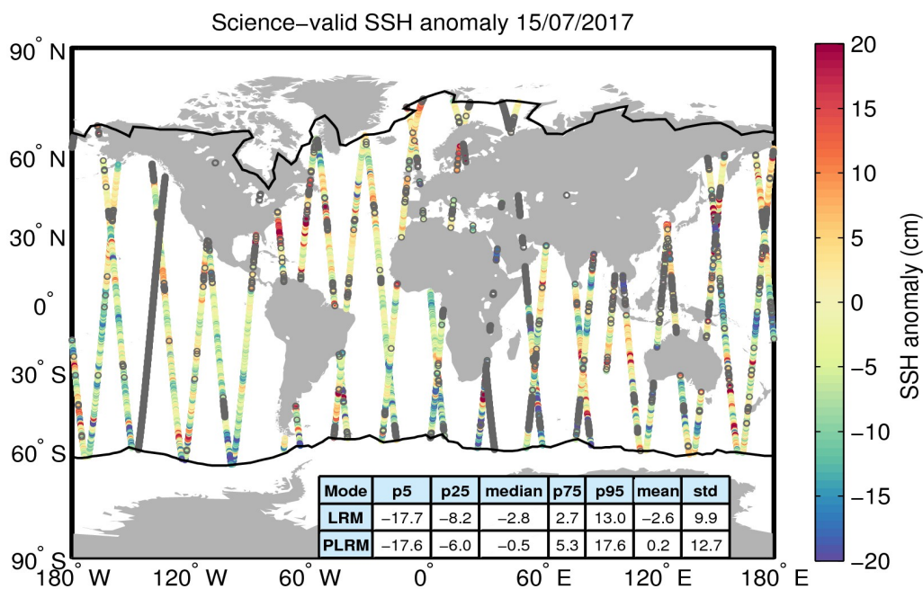
Figure 10. Geographical distribution of science-valid SSH anomaly data over oceans and lakes for 15/07/2017. The statistical values shown in the table refer to the SSH anomaly in cm and are calculated separately for LRM and PLRM regions. The black lines mark the outer limit of the Arctic and Antarctic polar polygons. Gray circles denote records that have been rejected based on the editing criteria described in Table 2.
