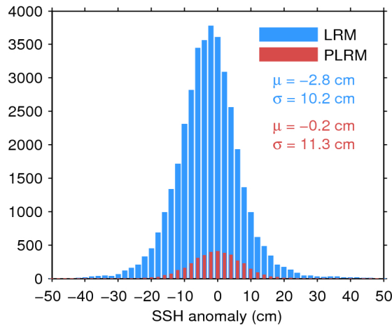
Figure 11. Histogram of science-valid SSH anomaly over oceans and lakes for LRM (blue) and PLRM (red) for 14/07/2017. The mean ( \mu ) and standard deviation ( \sigma ) are also shown. Note that values outside [-50 50] cm are excluded from the histogram for the sake of readability but not from the computation of \mu and \sigma .
