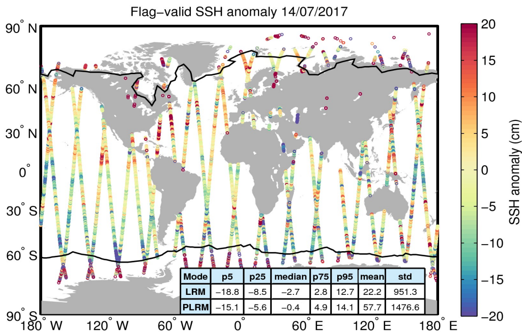
Figure 5. Geographical distribution of flag-valid 1-Hz SSH anomaly data over oceans and lakes for 14/07/2017. The statistical values shown in the table refer to the SSH anomaly in cm and are calculated separately for LRM and PLRM regions. Measurements taken over polar polygons have been excluded from the computation of the statistical values. The black lines mark the outer limit of the Arctic and Antarctic polar polygons.
