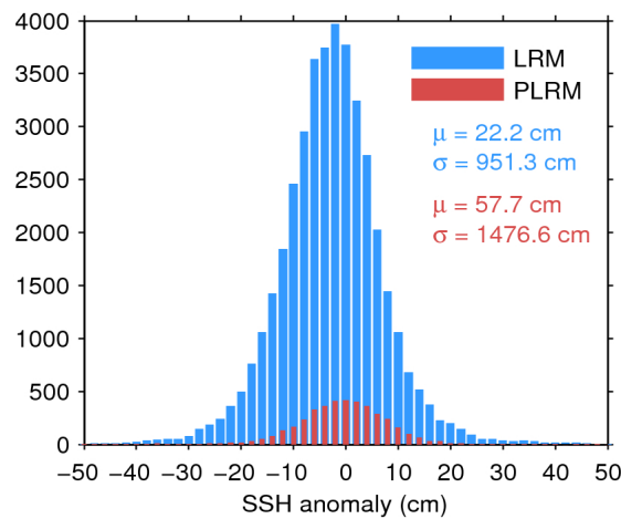
Figure 7. Histogram of flag-valid SSH anomaly over oceans and lakes for LRM (blue) and PLRM (red) for 14/07/2017. The mean ( \mu ) and standard deviation ( \sigma ) are also shown. Note that values outside [-50 \ 50] cm are excluded from the histogram for the sake of readability but not from the computation of \mu and \sigma .
