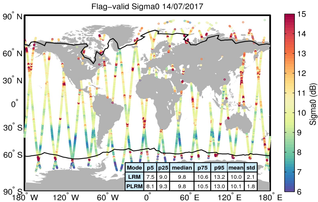
Figure 23. Geographical distribution of flag-valid sigma0 data over oceans and lakes for 14/07/2017. The statistical values shown in the table refer to the sigma0 in dB and are calculated separately for LRM and PLRM regions. Measurements taken over polar polygons have been excluded from the computation of the statistical values. The black lines mark the outer limit of the Arctic and Antarctic polar polygons.
