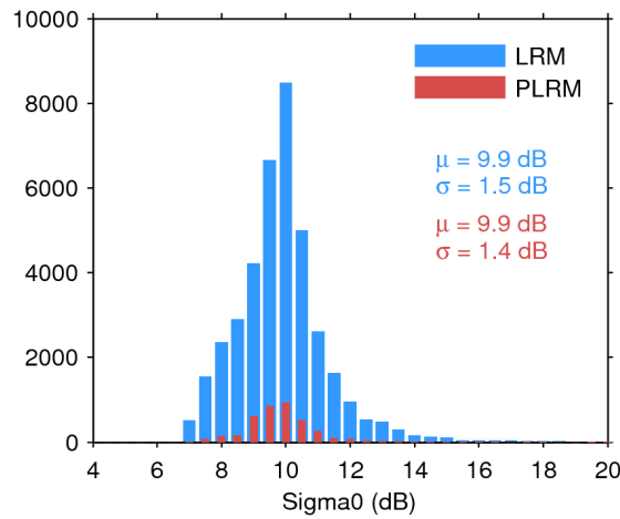
Figure 28. Histogram of science-valid sigma0 over oceans and lakes for LRM (blue) and PLRM (red) for 14/07/2017. The mean ( \mu ) and standard deviation ( \sigma ) are also shown. Note that values outside [4 20] dB are excluded from the histogram for the sake of readability but not from the computation of \mu and \sigma .
