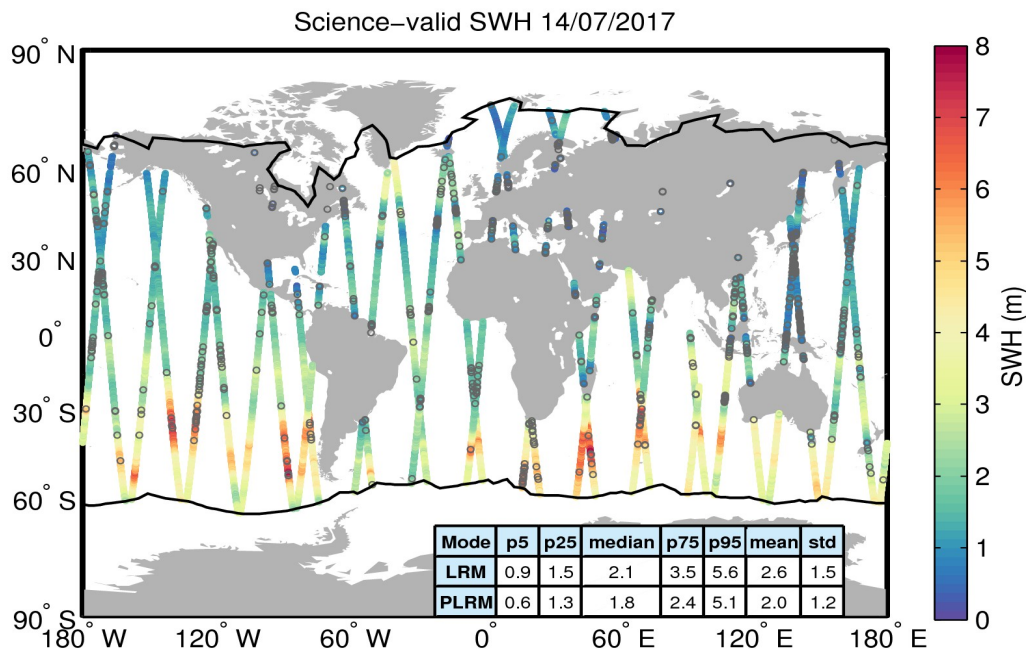
Figure 19. Geographical distribution of science-valid SWH data over oceans and lakes for 14/07/2017. The statistical values shown in the table refer to the SWH in m and are calculated separately for LRM and PLRM regions. The black lines mark the outer limit of the Arctic and Antarctic polar polygons. Gray circles denote records that have been rejected based on the editing criteria described in Table 3.
