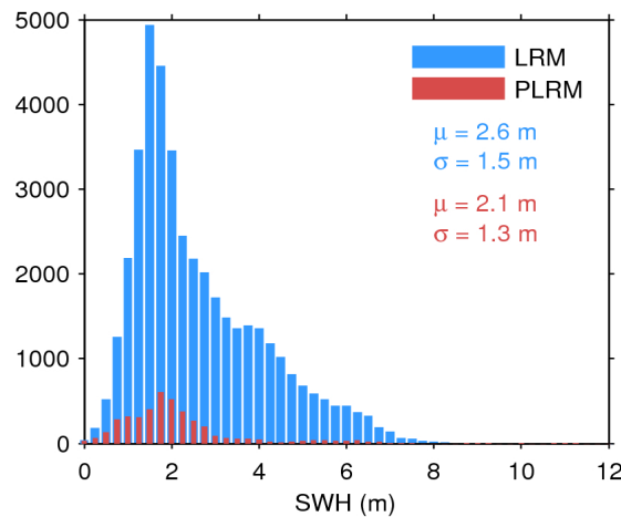
Figure 17. Histogram of flag-valid SWH over oceans and lakes for LRM (blue) and PLRM (red) for 14/07/2017. The mean ( \mu ) and standard deviation ( \sigma ) are also shown. Note that values larger than 12 m are excluded from the histogram for the sake of readability but not from the computation of \mu and \sigma .
