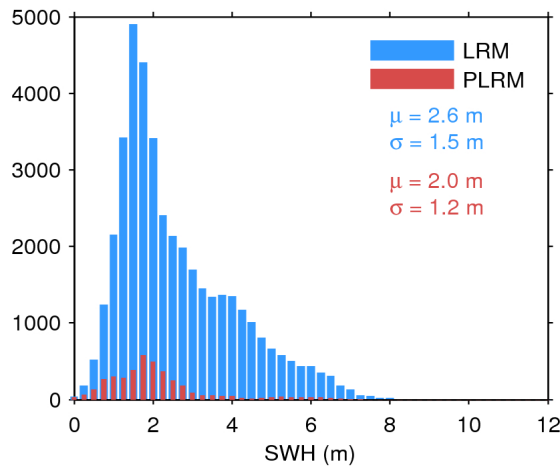
Figure 20. Histogram of science-valid SWH over oceans and lakes for LRM (blue) and PLRM (red) for 14/07/2017. The mean ( \mu ) and standard deviation ( \sigma ) are also shown. Note that values larger than 12 m are excluded from the histogram for the sake of readability but not from the computation of \mu and \sigma .
