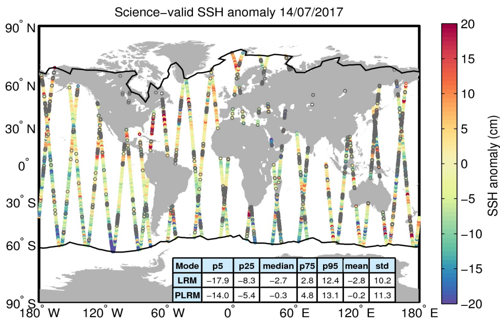
Figure 10. Geographical distribution of science-valid SSH anomaly data over oceans and lakes for 14/07/2017. The statistical values shown in the table refer to the SSH anomaly in cm and are calculated separately for LRM and PLRM regions. The black lines mark the outer limit of the Arctic and Antarctic polar polygons. Gray circles denote records that have been rejected based on the editing criteria described in Table 2.
