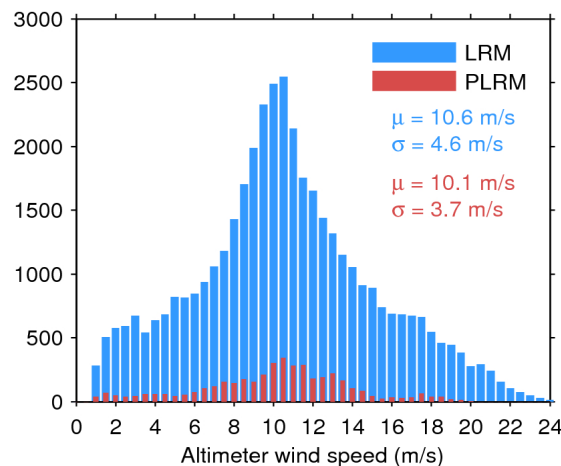
Figure 35. Histogram of science-valid wind over oceans and lakes for LRM (blue) and PLRM (red) for 14/07/2017. The mean ( \mu ) and standard deviation ( \sigma ) are also shown. Note that values larger than 24 m/s are excluded from the histogram for the sake of readability but not from the computation of \mu and \sigma .
