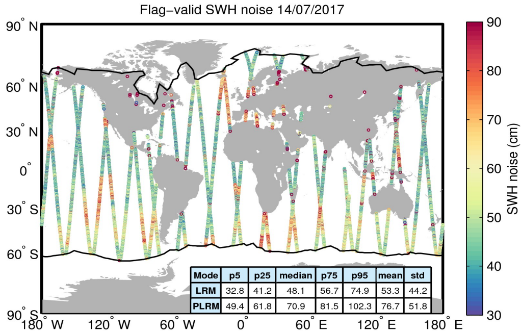
Figure 18. Geographical distribution of flag-valid 20-Hz SWH measurement noise over oceans and lakes for 14/07/2017. The statistical values shown in the table refer to the SWH noise and are calculated separately for LRM and PLRM regions. Measurements taken over polar polygons have been excluded from the computation of the statistical values. The black lines mark the outer limit of the Arctic and Antarctic polar polygons.
