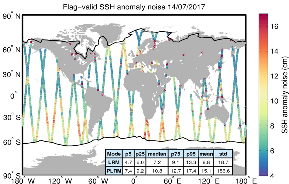
Figure 8. Geographical distribution of flag-valid 20-Hz SSH anomaly measurement noise over oceans and lakes for 14/07/2017. The statistical values shown in the table refer to the SSH anomaly noise and are calculated separately for LRM and PLRM regions. Measurements taken over polar polygons have been excluded from the computation of the statistical values. The black lines mark the outer limit of the Arctic and Antarctic polar polygons.
