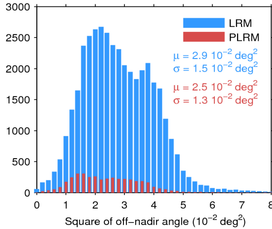
Figure 39. Histogram of flag-valid mispointing over oceans and lakes for LRM (blue) and PLRM (red) for 14/07/2017. Only positive values have been considered. The mean ( \mu ) and standard deviation ( \sigma ) are also shown. Note that values larger than 8 \cdot 10^{-2} \text{ deg}^2 are excluded from the histogram for the sake of readability but not from the computation of \mu and \sigma .
