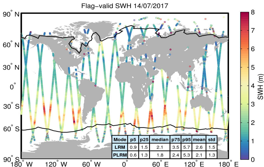
Figure 15. Geographical distribution of flag-valid SWH data over oceans and lakes for 14/07/2017. The statistical values shown in the table refer to the SWH in m and are calculated separately for LRM and PLRM regions. Measurements taken over polar polygons have been excluded from the computation of the statistical values. The black lines mark the outer limit of the Arctic and Antarctic polar polygons.
