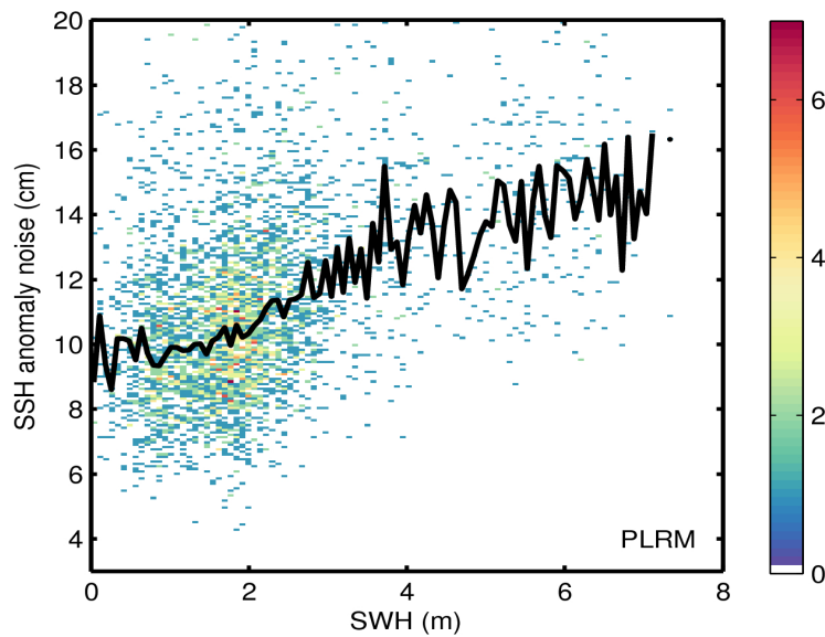
Figure 9. 2D histogram showing flag-valid SSH anomaly noise as a function of SWH for LRM (top) and PLRM (bottom) for 14/07/2017. The black line denotes the median SSH anomaly noise as a function of SWH.
