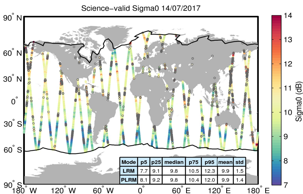
Figure 27. Geographical distribution of science-valid sigma0 data over oceans and lakes for 14/07/2017. The statistical values shown in the table refer to the sigma0 in dB and are calculated separately for LRM and PLRM regions. The black lines mark the outer limit of the Arctic and Antarctic polar polygons. Gray circles denote records that have been rejected based on the editing criteria described in Table 4.
