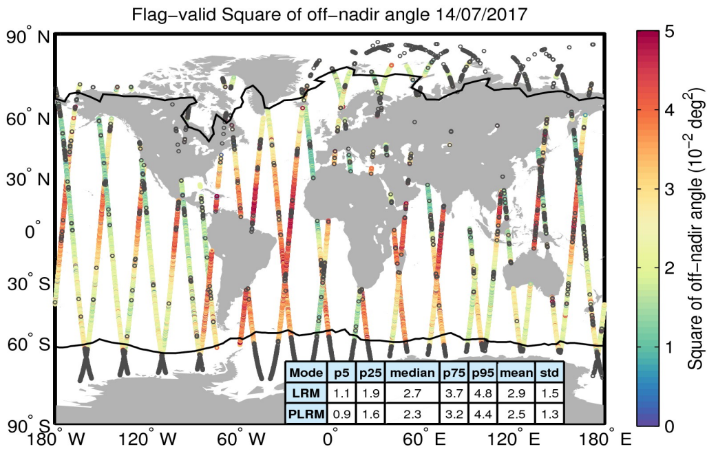
Figure 37. Geographical distribution of flag-valid mispointing data over oceans and lakes for 14/07/2017. The statistical values shown in the table refer to the mispointing in 10^{-2} deg 2 and are calculated separately for LRM and PLRM regions. Measurements taken over polar polygons have been excluded from the computation of the statistical values. The black lines mark the outer limit of the Arctic and Antarctic polar polygons. Gray circles denote negative values.
