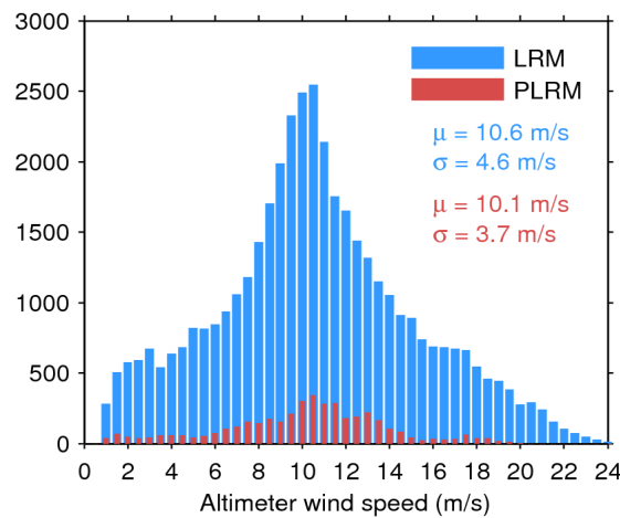
Figure 33. Histogram of flag-valid wind over oceans and lakes for LRM (blue) and PLRM (red) for 14/07/2017. The mean ( \mu ) and standard deviation ( \sigma ) are also shown. Note that values larger than 24 m/s are excluded from the histogram for the sake of readability but not from the computation of \mu and \sigma .
