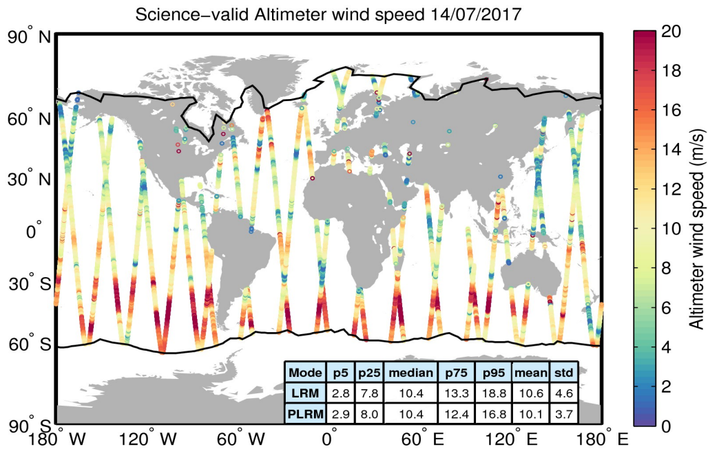
Figure 34. Geographical distribution of science-valid wind data over oceans and lakes for 14/07/2017. The statistical values shown in the table refer to the wind in m/s and are calculated separately for LRM and PLRM regions. The black lines mark the outer limit of the Arctic and Antarctic polar polygons. Gray circles denote records that have been rejected based on the editing criteria described in Table 5.
