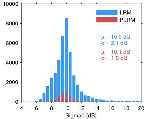
Figure 25. Histogram of flag-valid sigma0 over oceans and lakes for LRM (blue) and PLRM (red) for 14/07/2017. The mean ( \mu ) and standard deviation ( \sigma ) are also shown. Note that values outside [4 20] dB are excluded from the histogram for the sake of readability but not from the computation of \mu and \sigma .
