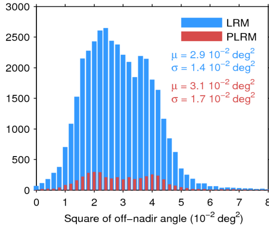
Figure 39. Histogram of flag-valid mispointing over oceans and lakes for LRM (blue) and PLRM (red) for 13/07/2017. Only positive values have been considered. The mean ( \mu ) and standard deviation ( \sigma ) are also shown. Note that values larger than 8 \cdot 10^{-2} \text{ deg}^2 are excluded from the histogram for the sake of readability but not from the computation of \mu and \sigma .
