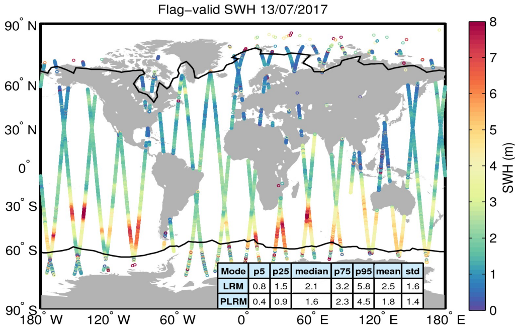
Figure 15. Geographical distribution of flag-valid SWH data over oceans and lakes for 13/07/2017. The statistical values shown in the table refer to the SWH in m and are calculated separately for LRM and PLRM regions. Measurements taken over polar polygons have been excluded from the computation of the statistical values. The black lines mark the outer limit of the Arctic and Antarctic polar polygons.
