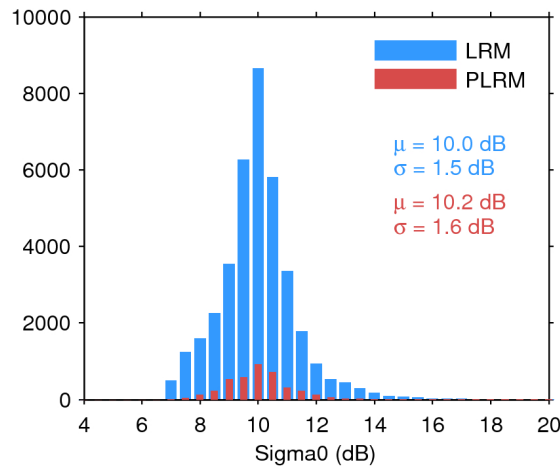
Figure 28. Histogram of science-valid sigma0 over oceans and lakes for LRM (blue) and PLRM (red) for 13/07/2017. The mean ( \mu ) and standard deviation ( \sigma ) are also shown. Note that values outside [4 20] dB are excluded from the histogram for the sake of readability but not from the computation of \mu and \sigma .
