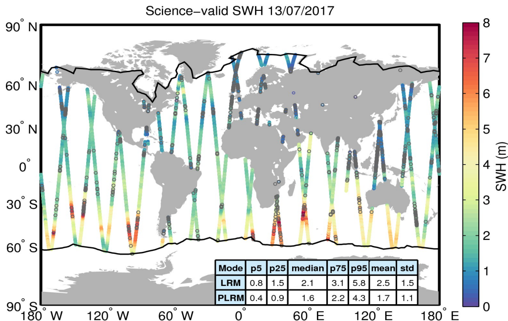
Figure 19. Geographical distribution of science-valid SWH data over oceans and lakes for 13/07/2017. The statistical values shown in the table refer to the SWH in m and are calculated separately for LRM and PLRM regions. The black lines mark the outer limit of the Arctic and Antarctic polar polygons. Gray circles denote records that have been rejected based on the editing criteria described in Table 3.
