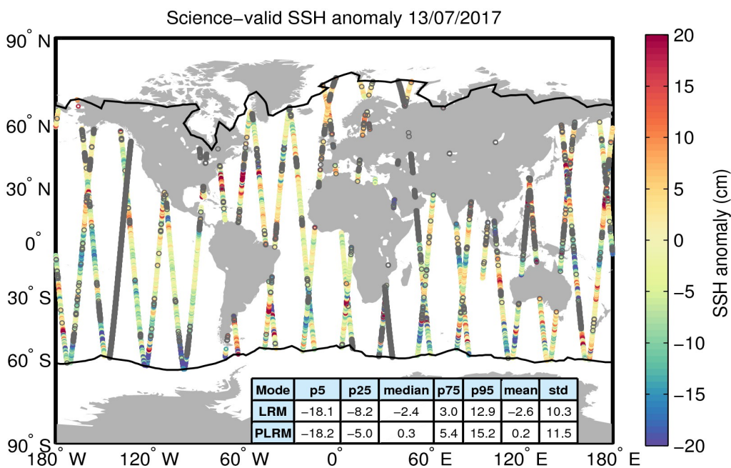
Figure 10. Geographical distribution of science-valid SSH anomaly data over oceans and lakes for 13/07/2017. The statistical values shown in the table refer to the SSH anomaly in cm and are calculated separately for LRM and PLRM regions. The black lines mark the outer limit of the Arctic and Antarctic polar polygons. Gray circles denote records that have been rejected based on the editing criteria described in Table 2.
