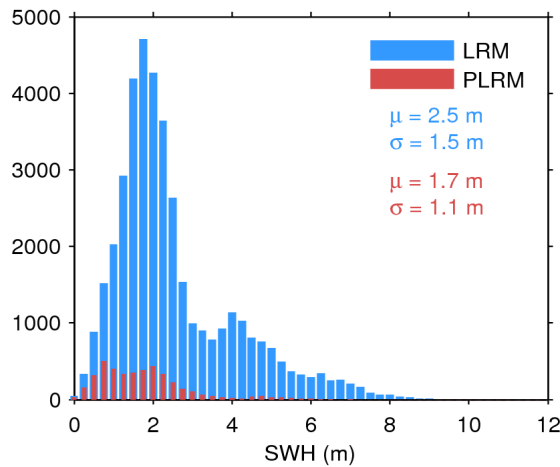
Figure 20. Histogram of science-valid SWH over oceans and lakes for LRM (blue) and PLRM (red) for 13/07/2017. The mean ( \mu ) and standard deviation ( \sigma ) are also shown. Note that values larger than 12 m are excluded from the histogram for the sake of readability but not from the computation of \mu and \sigma .
