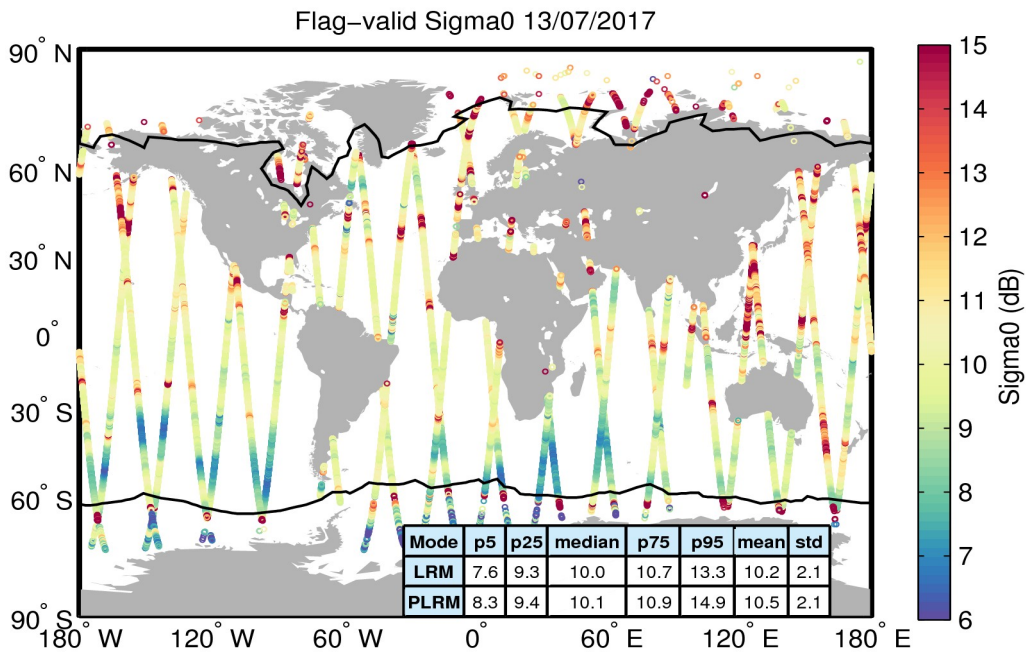
Figure 23. Geographical distribution of flag-valid sigma0 data over oceans and lakes for 13/07/2017. The statistical values shown in the table refer to the sigma0 in dB and are calculated separately for LRM and PLRM regions. Measurements taken over polar polygons have been excluded from the computation of the statistical values. The black lines mark the outer limit of the Arctic and Antarctic polar polygons.
