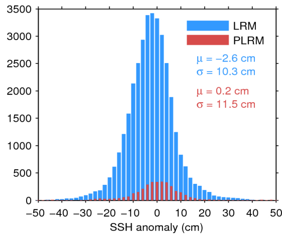
Figure 11. Histogram of science-valid SSH anomaly over oceans and lakes for LRM (blue) and PLRM (red) for 13/07/2017. The mean ( \mu ) and standard deviation ( \sigma ) are also shown. Note that values outside [-50 50] cm are excluded from the histogram for the sake of readability but not from the computation of \mu and \sigma .
