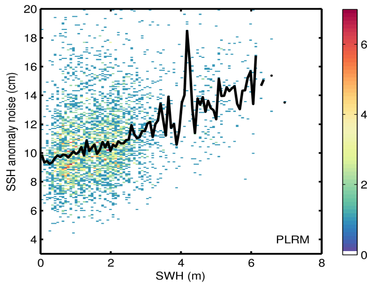
Figure 9. 2D histogram showing flag-valid SSH anomaly noise as a function of SWH for LRM (top) and PLRM (bottom) for 13/07/2017. The black line denotes the median SSH anomaly noise as a function of SWH.
