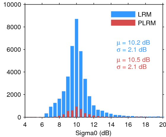
Figure 25. Histogram of flag-valid sigma0 over oceans and lakes for LRM (blue) and PLRM (red) for 13/07/2017. The mean ( \mu ) and standard deviation ( \sigma ) are also shown. Note that values outside [4 20] dB are excluded from the histogram for the sake of readability but not from the computation of \mu and \sigma .
