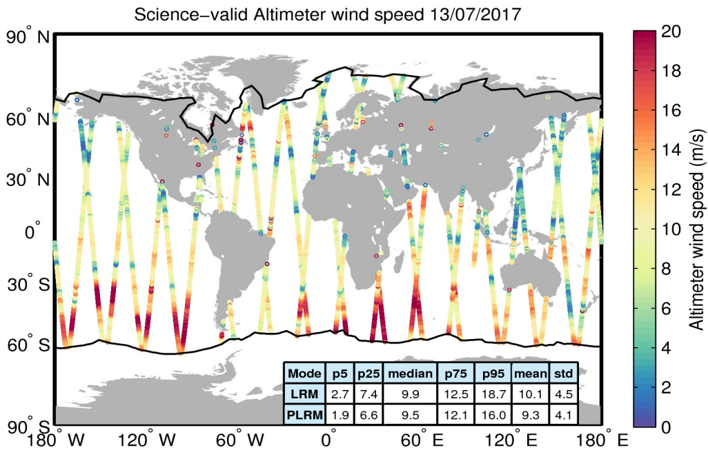
Figure 34. Geographical distribution of science-valid wind data over oceans and lakes for 13/07/2017. The statistical values shown in the table refer to the wind in m/s and are calculated separately for LRM and PLRM regions. The black lines mark the outer limit of the Arctic and Antarctic polar polygons. Gray circles denote records that have been rejected based on the editing criteria described in Table 5.
