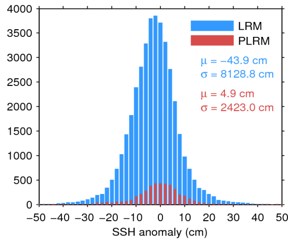
Figure 7. Histogram of flag-valid SSH anomaly over oceans and lakes for LRM (blue) and PLRM (red) for 13/07/2017. The mean ( \mu ) and standard deviation ( \sigma ) are also shown. Note that values outside [-50 \ 50] cm are excluded from the histogram for the sake of readability but not from the computation of \mu and \sigma .
