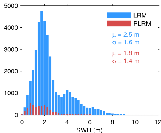
Figure 17. Histogram of flag-valid SWH over oceans and lakes for LRM (blue) and PLRM (red) for 13/07/2017. The mean ( \mu ) and standard deviation ( \sigma ) are also shown. Note that values larger than 12 m are excluded from the histogram for the sake of readability but not from the computation of \mu and \sigma .
