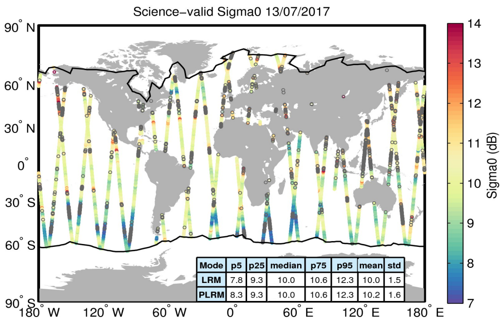
Figure 27. Geographical distribution of science-valid sigma0 data over oceans and lakes for 13/07/2017. The statistical values shown in the table refer to the sigma0 in dB and are calculated separately for LRM and PLRM regions. The black lines mark the outer limit of the Arctic and Antarctic polar polygons. Gray circles denote records that have been rejected based on the editing criteria described in Table 4.
