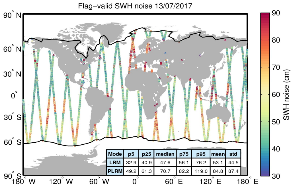
Figure 18. Geographical distribution of flag-valid 20-Hz SWH measurement noise over oceans and lakes for 13/07/2017. The statistical values shown in the table refer to the SWH noise and are calculated separately for LRM and PLRM regions. Measurements taken over polar polygons have been excluded from the computation of the statistical values. The black lines mark the outer limit of the Arctic and Antarctic polar polygons.
