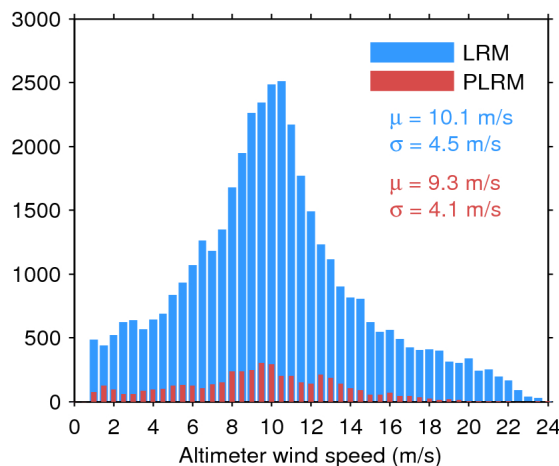
Figure 35. Histogram of science-valid wind over oceans and lakes for LRM (blue) and PLRM (red) for 13/07/2017. The mean ( \mu ) and standard deviation ( \sigma ) are also shown. Note that values larger than 24 m/s are excluded from the histogram for the sake of readability but not from the computation of \mu and \sigma .
