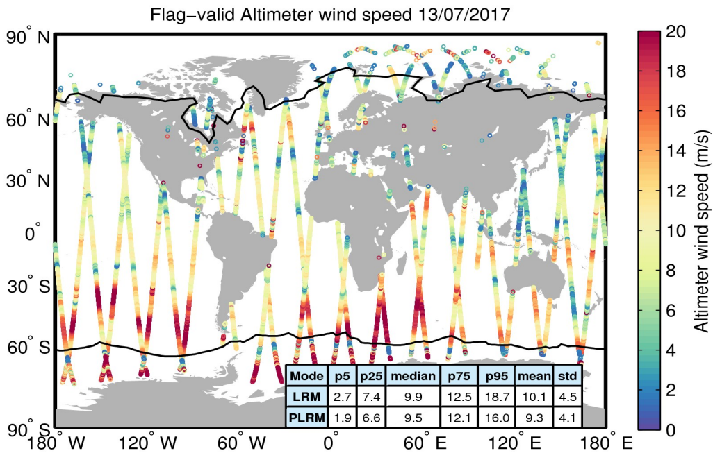
Figure 31. Geographical distribution of flag-valid wind data over oceans and lakes for 13/07/2017. The statistical values shown in the table refer to the wind in m/s and are calculated separately for LRM and PLRM regions. Measurements taken over polar polygons have been excluded from the computation of the statistical values. The black lines mark the outer limit of the Arctic and Antarctic polar polygons.
