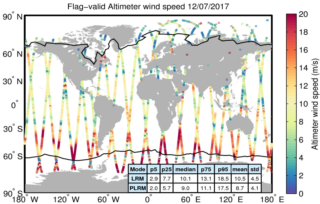
Figure 31. Geographical distribution of flag-valid wind data over oceans and lakes for 12/07/2017. The statistical values shown in the table refer to the wind in m/s and are calculated separately for LRM and PLRM regions. Measurements taken over polar polygons have been excluded from the computation of the statistical values. The black lines mark the outer limit of the Arctic and Antarctic polar polygons.
