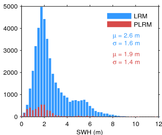
Figure 17. Histogram of flag-valid SWH over oceans and lakes for LRM (blue) and PLRM (red) for 12/07/2017. The mean ( \mu ) and standard deviation ( \sigma ) are also shown. Note that values larger than 12 m are excluded from the histogram for the sake of readability but not from the computation of \mu and \sigma .
