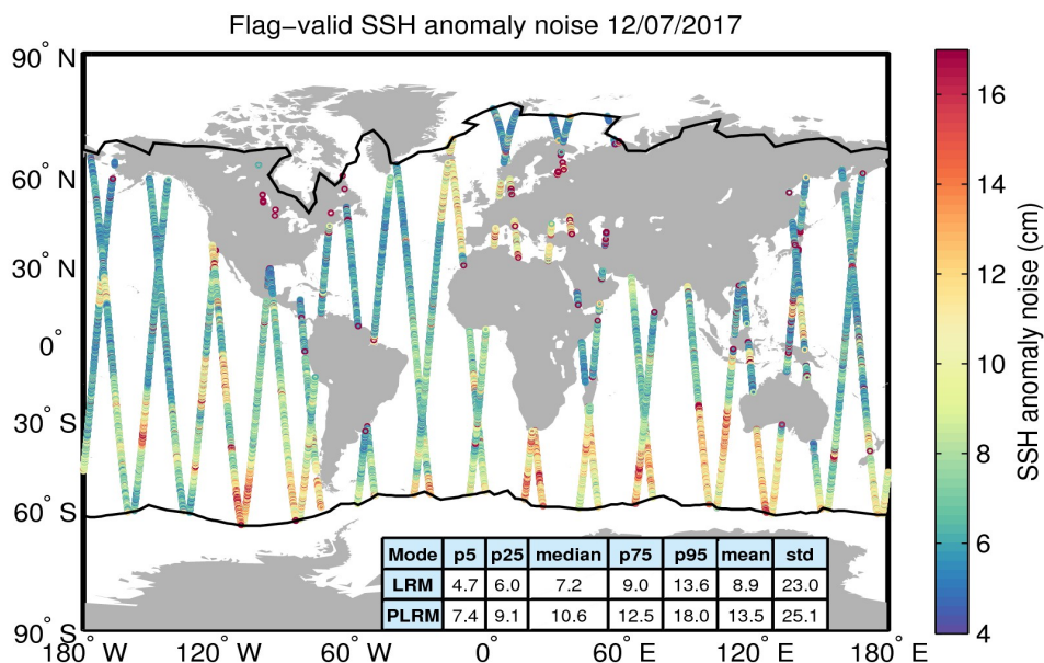
Figure 8. Geographical distribution of flag-valid 20-Hz SSH anomaly measurement noise over oceans and lakes for 12/07/2017. The statistical values shown in the table refer to the SSH anomaly noise and are calculated separately for LRM and PLRM regions. Measurements taken over polar polygons have been excluded from the computation of the statistical values. The black lines mark the outer limit of the Arctic and Antarctic polar polygons.
