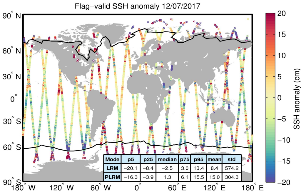
Figure 5. Geographical distribution of flag-valid 1-Hz SSH anomaly data over oceans and lakes for 12/07/2017. The statistical values shown in the table refer to the SSH anomaly in cm and are calculated separately for LRM and PLRM regions. Measurements taken over polar polygons have been excluded from the computation of the statistical values. The black lines mark the outer limit of the Arctic and Antarctic polar polygons.
