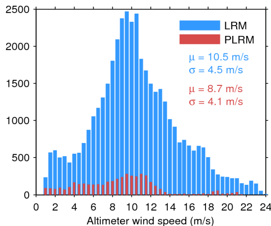
Figure 35. Histogram of science-valid wind over oceans and lakes for LRM (blue) and PLRM (red) for 12/07/2017. The mean ( \mu ) and standard deviation ( \sigma ) are also shown. Note that values larger than 24 m/s are excluded from the histogram for the sake of readability but not from the computation of \mu and \sigma .
