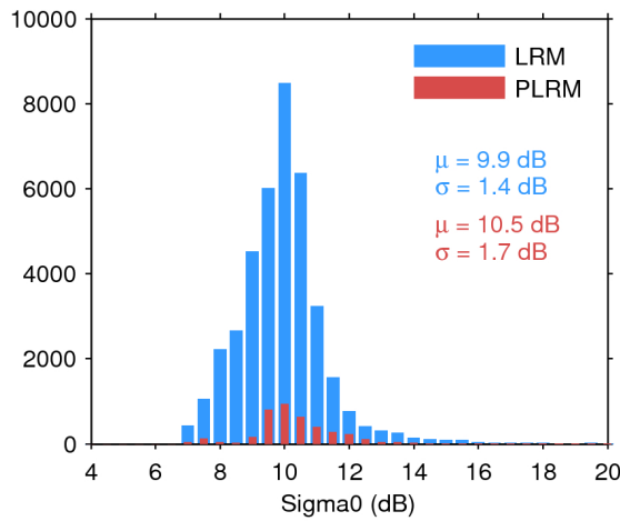
Figure 28. Histogram of science-valid sigma0 over oceans and lakes for LRM (blue) and PLRM (red) for 12/07/2017. The mean ( \mu ) and standard deviation ( \sigma ) are also shown. Note that values outside [4 20] dB are excluded from the histogram for the sake of readability but not from the computation of \mu and \sigma .
