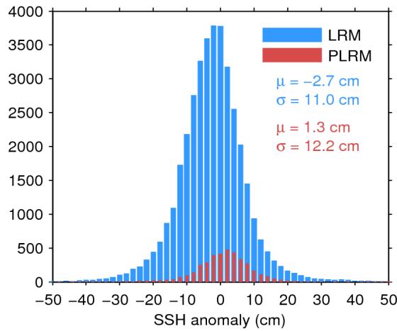
Figure 11. Histogram of science-valid SSH anomaly over oceans and lakes for LRM (blue) and PLRM (red) for 12/07/2017. The mean ( \mu ) and standard deviation ( \sigma ) are also shown. Note that values outside [-50\ 50] cm are excluded from the histogram for the sake of readability but not from the computation of \mu and \sigma .
