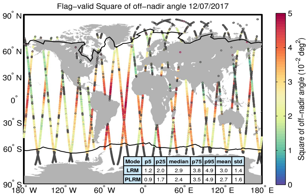
Figure 37. Geographical distribution of flag-valid mispointing data over oceans and lakes for 12/07/2017. The statistical values shown in the table refer to the mispointing in 10^{-2} deg 2 and are calculated separately for LRM and PLRM regions. Measurements taken over polar polygons have been excluded from the computation of the statistical values. The black lines mark the outer limit of the Arctic and Antarctic polar polygons. Gray circles denote negative values.
