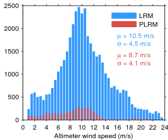
Figure 33. Histogram of flag-valid wind over oceans and lakes for LRM (blue) and PLRM (red) for 12/07/2017. The mean ( \mu ) and standard deviation ( \sigma ) are also shown. Note that values larger than 24 m/s are excluded from the histogram for the sake of readability but not from the computation of \mu and \sigma .
