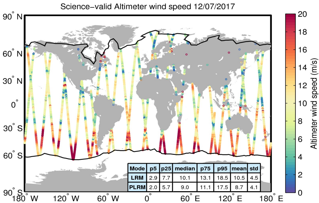
Figure 34. Geographical distribution of science-valid wind data over oceans and lakes for 12/07/2017. The statistical values shown in the table refer to the wind in m/s and are calculated separately for LRM and PLRM regions. The black lines mark the outer limit of the Arctic and Antarctic polar polygons. Gray circles denote records that have been rejected based on the editing criteria described in Table 5.
