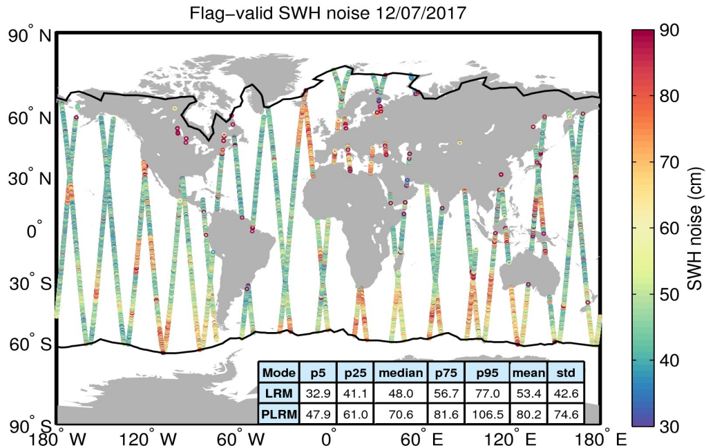
Figure 18. Geographical distribution of flag-valid 20-Hz SWH measurement noise over oceans and lakes for 12/07/2017. The statistical values shown in the table refer to the SWH noise and are calculated separately for LRM and PLRM regions. Measurements taken over polar polygons have been excluded from the computation of the statistical values. The black lines mark the outer limit of the Arctic and Antarctic polar polygons.
