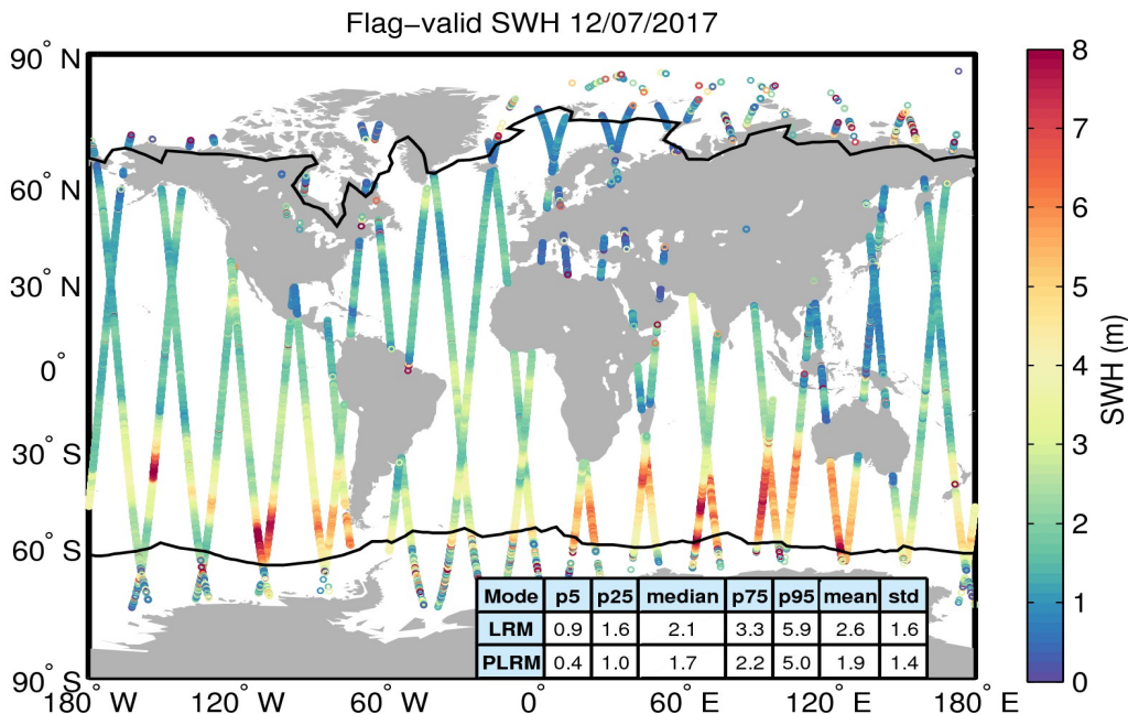
Figure 15. Geographical distribution of flag-valid SWH data over oceans and lakes for 12/07/2017. The statistical values shown in the table refer to the SWH in m and are calculated separately for LRM and PLRM regions. Measurements taken over polar polygons have been excluded from the computation of the statistical values. The black lines mark the outer limit of the Arctic and Antarctic polar polygons.
