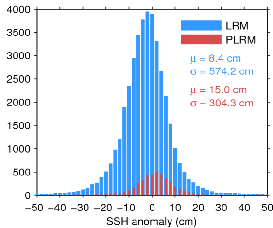
Figure 7. Histogram of flag-valid SSH anomaly over oceans and lakes for LRM (blue) and PLRM (red) for 12/07/2017. The mean ( \mu ) and standard deviation ( \sigma ) are also shown. Note that values outside [-50 50] cm are excluded from the histogram for the sake of readability but not from the computation of \mu and \sigma .
