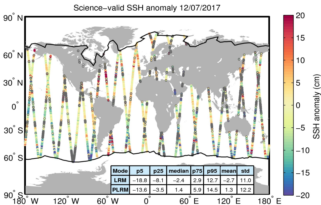
Figure 10. Geographical distribution of science-valid SSH anomaly data over oceans and lakes for 12/07/2017. The statistical values shown in the table refer to the SSH anomaly in cm and are calculated separately for LRM and PLRM regions. The black lines mark the outer limit of the Arctic and Antarctic polar polygons. Gray circles denote records that have been rejected based on the editing criteria described in Table 2.
