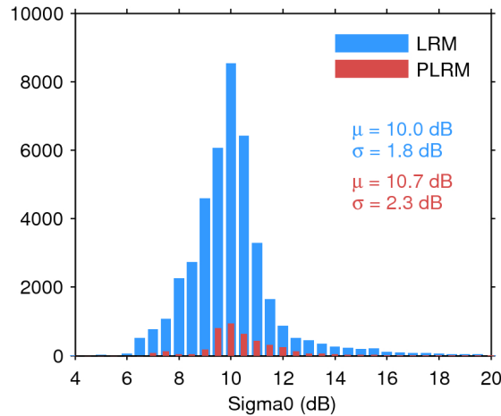
Figure 25. Histogram of flag-valid sigma0 over oceans and lakes for LRM (blue) and PLRM (red) for 12/07/2017. The mean ( \mu ) and standard deviation ( \sigma ) are also shown. Note that values outside [4 20] dB are excluded from the histogram for the sake of readability but not from the computation of \mu and \sigma .
