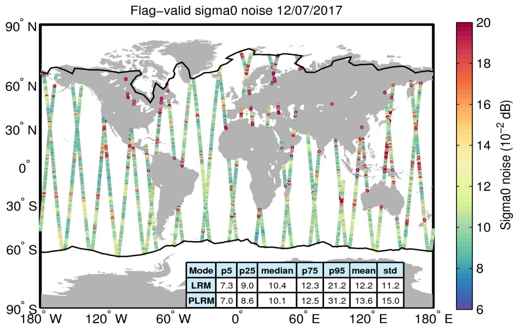
Figure 26. Geographical distribution of flag-valid 20-Hz sigma0 measurement noise over oceans and lakes for 12/07/2017. The statistical values shown in the table refer to the sigma0 noise and are calculated separately for LRM and PLRM regions. Measurements taken over polar polygons have been excluded from the computation of the statistical values. The black lines mark the outer limit of the Arctic and Antarctic polar polygons.
