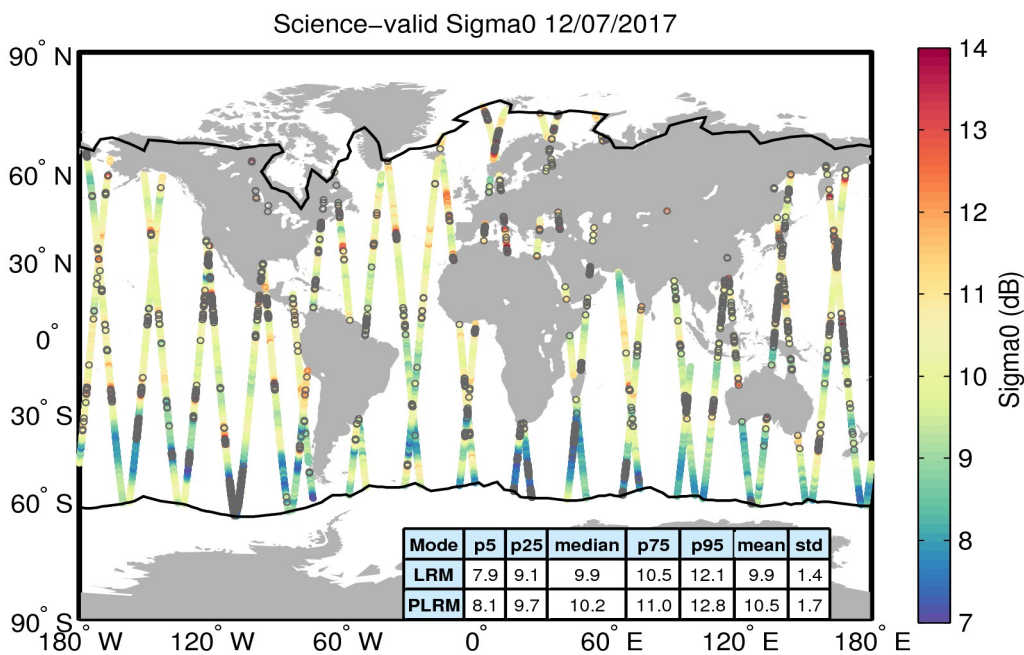
Figure 27. Geographical distribution of science-valid sigma0 data over oceans and lakes for 12/07/2017. The statistical values shown in the table refer to the sigma0 in dB and are calculated separately for LRM and PLRM regions. The black lines mark the outer limit of the Arctic and Antarctic polar polygons. Gray circles denote records that have been rejected based on the editing criteria described in Table 4.
