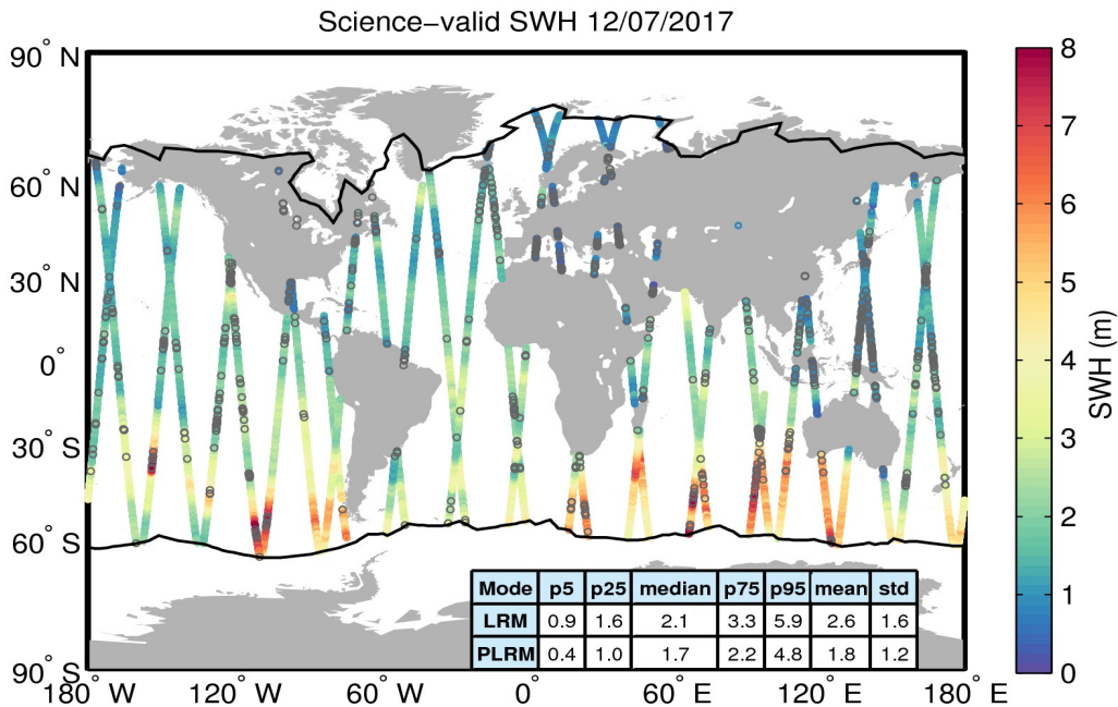
Figure 19. Geographical distribution of science-valid SWH data over oceans and lakes for 12/07/2017. The statistical values shown in the table refer to the SWH in m and are calculated separately for LRM and PLRM regions. The black lines mark the outer limit of the Arctic and Antarctic polar polygons. Gray circles denote records that have been rejected based on the editing criteria described in Table 3.
