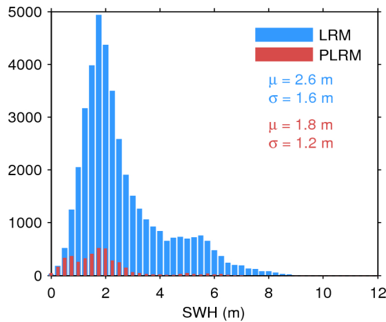
Figure 20. Histogram of science-valid SWH over oceans and lakes for LRM (blue) and PLRM (red) for 12/07/2017. The mean ( \mu ) and standard deviation ( \sigma ) are also shown. Note that values larger than 12 m are excluded from the histogram for the sake of readability but not from the computation of \mu and \sigma .
