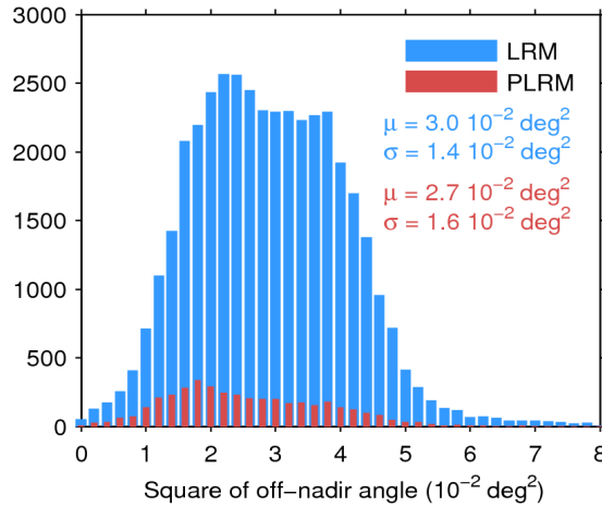
Figure 39. Histogram of flag-valid mispointing over oceans and lakes for LRM (blue) and PLRM (red) for 12/07/2017. Only positive values have been considered. The mean ( \mu ) and standard deviation ( \sigma ) are also shown. Note that values larger than 8 \cdot 10^{-2} \text{ deg}^2 are excluded from the histogram for the sake of readability but not from the computation of \mu and \sigma .
