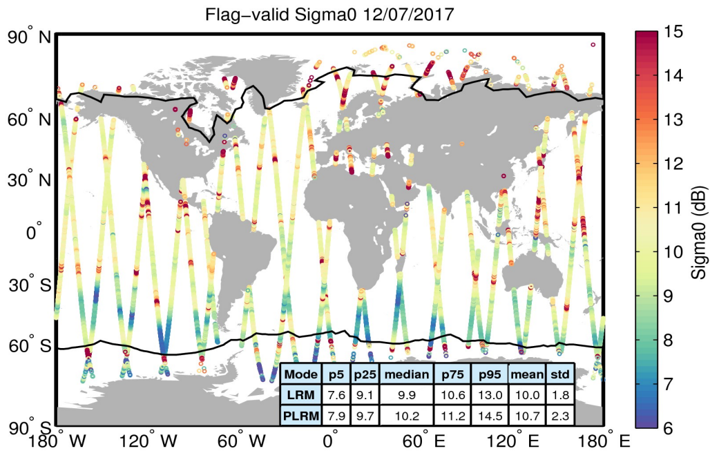
Figure 23. Geographical distribution of flag-valid sigma0 data over oceans and lakes for 12/07/2017. The statistical values shown in the table refer to the sigma0 in dB and are calculated separately for LRM and PLRM regions. Measurements taken over polar polygons have been excluded from the computation of the statistical values. The black lines mark the outer limit of the Arctic and Antarctic polar polygons.
