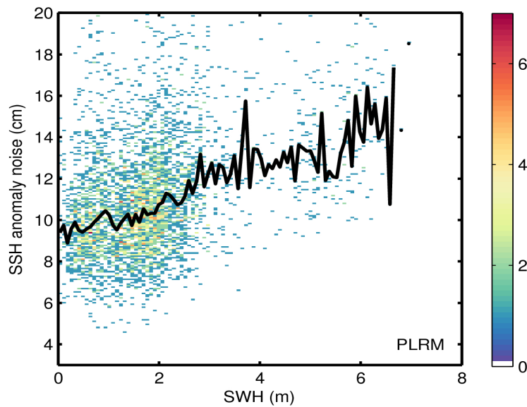
Figure 9. 2D histogram showing flag-valid SSH anomaly noise as a function of SWH for LRM (top) and PLRM (bottom) for 12/07/2017. The black line denotes the median SSH anomaly noise as a function of SWH.
